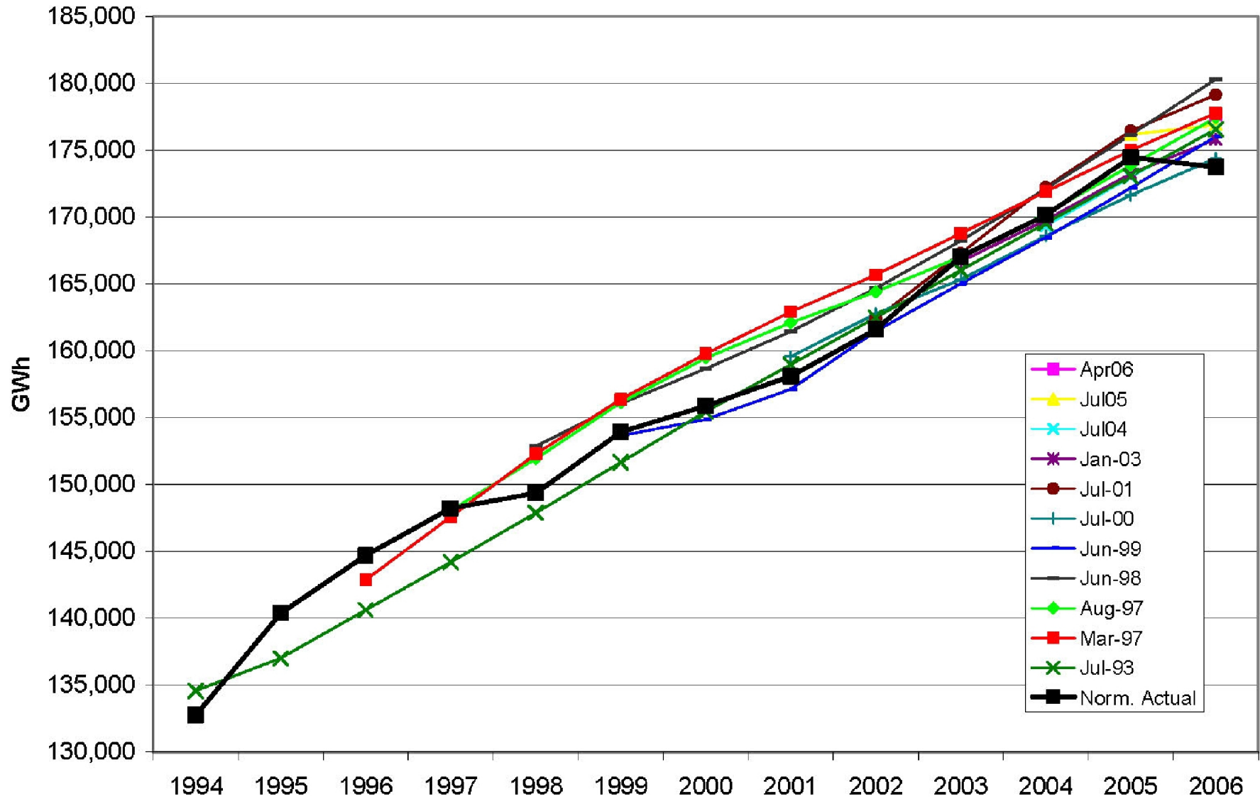
FIGURE 8.2-1 Comparison of Actual and Forecast Net System Requirements
