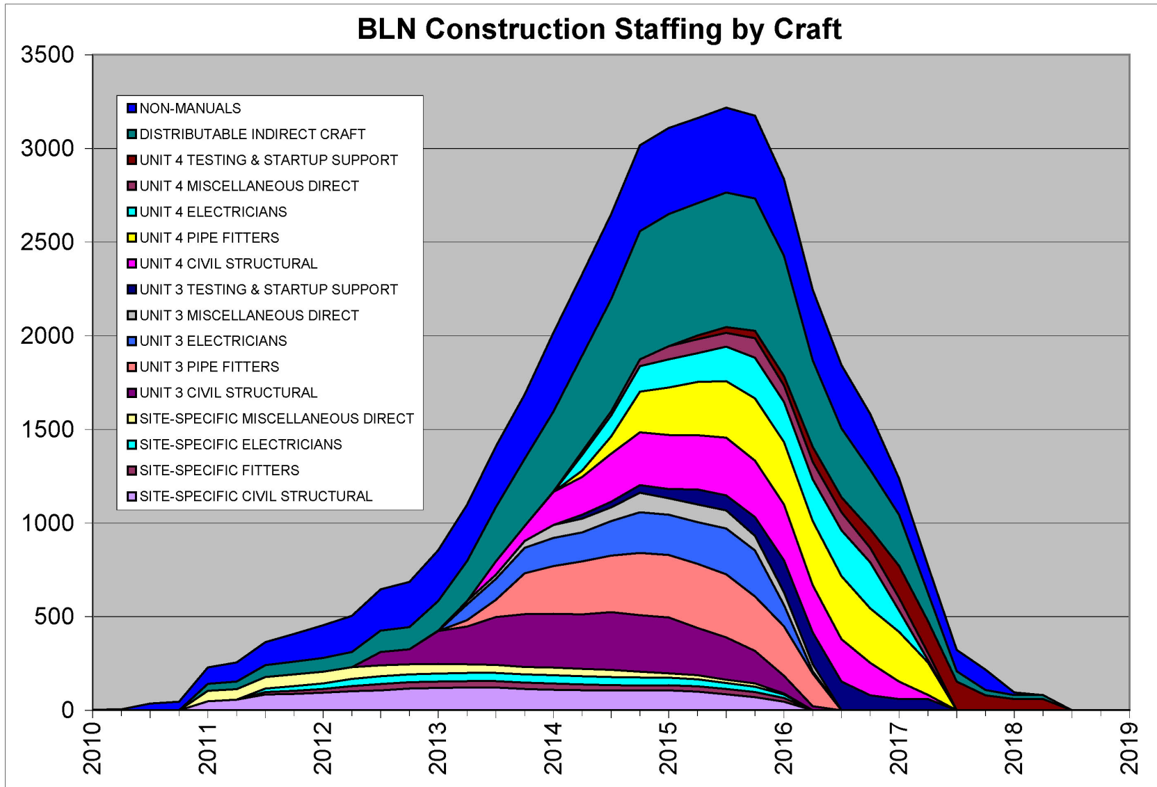
FIGURE 4.4-2 BLN Construction Staffing by Craft
