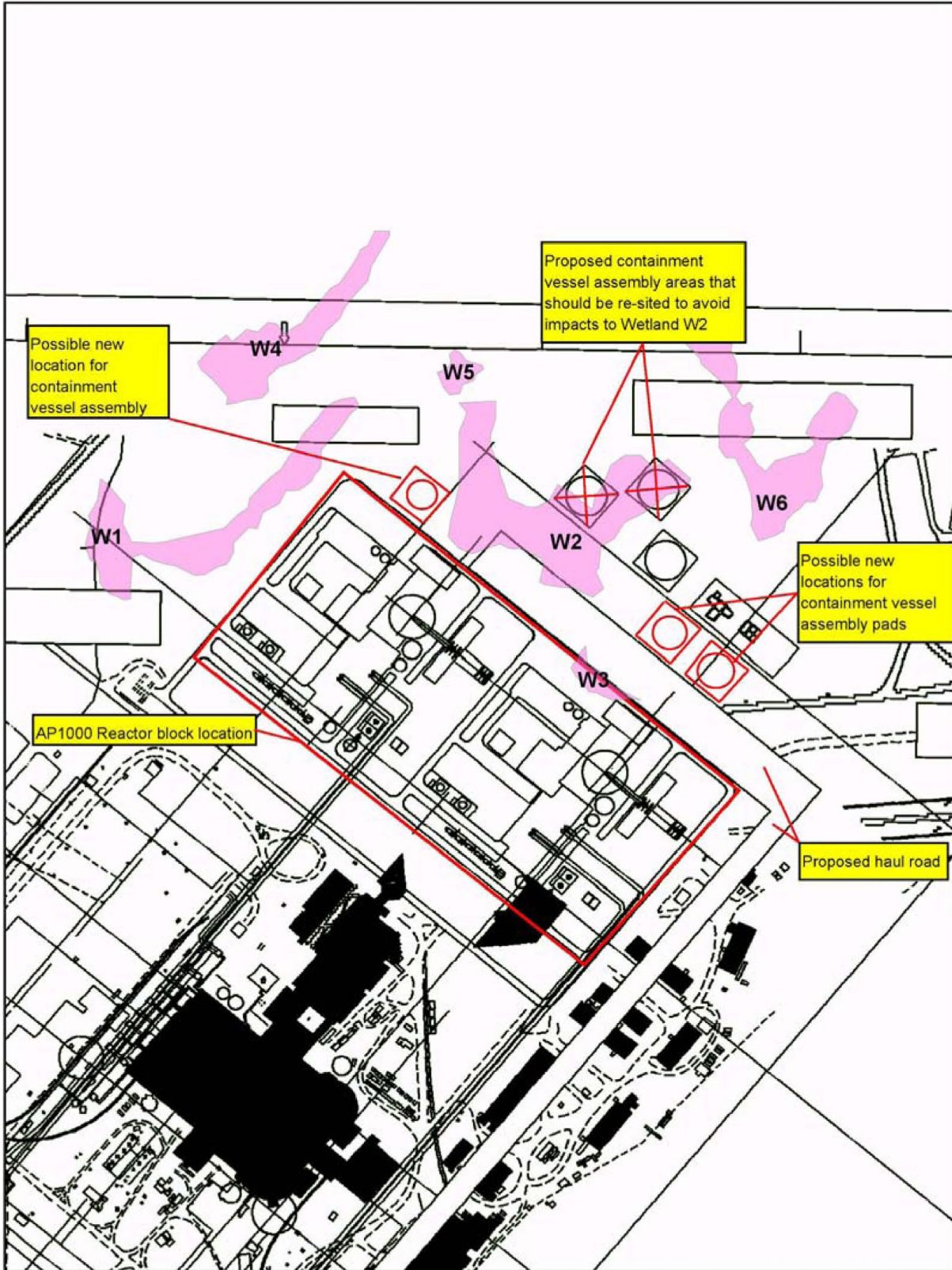
FIGURE 4.2-3 Alternate Containment Vessel Assembly Pad Locations to Minimize Impacts to Wetland W2, BLN AP1000 Construction Site
