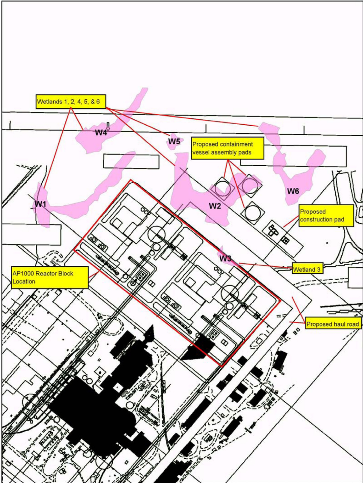
FIGURE 4.2-2 Location of Wetlands at Proposed BLN AP1000 Reactor Block Construction Site
