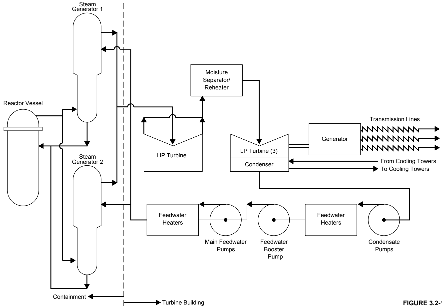
FIGURE 3.2-1 Reactor Power Conversion System Simplified Flow Diagram
