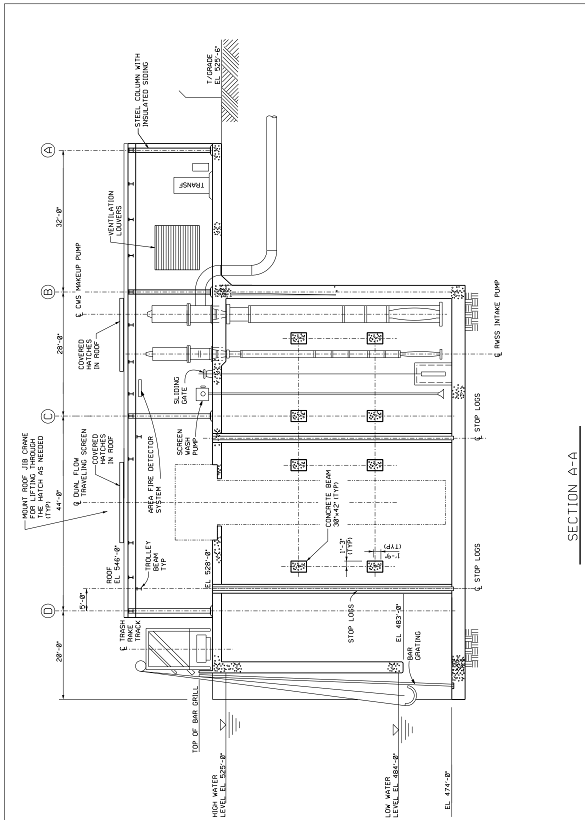
Figure 3.4-5 {Section View of CWS Makeup Water Intake Structure}
