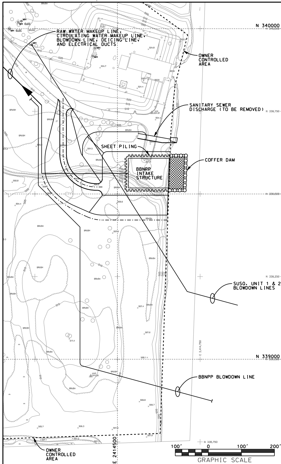
Figure 3.4-11 {CWS Makeup Water Intake Structure Construction Cofferd Dam}
