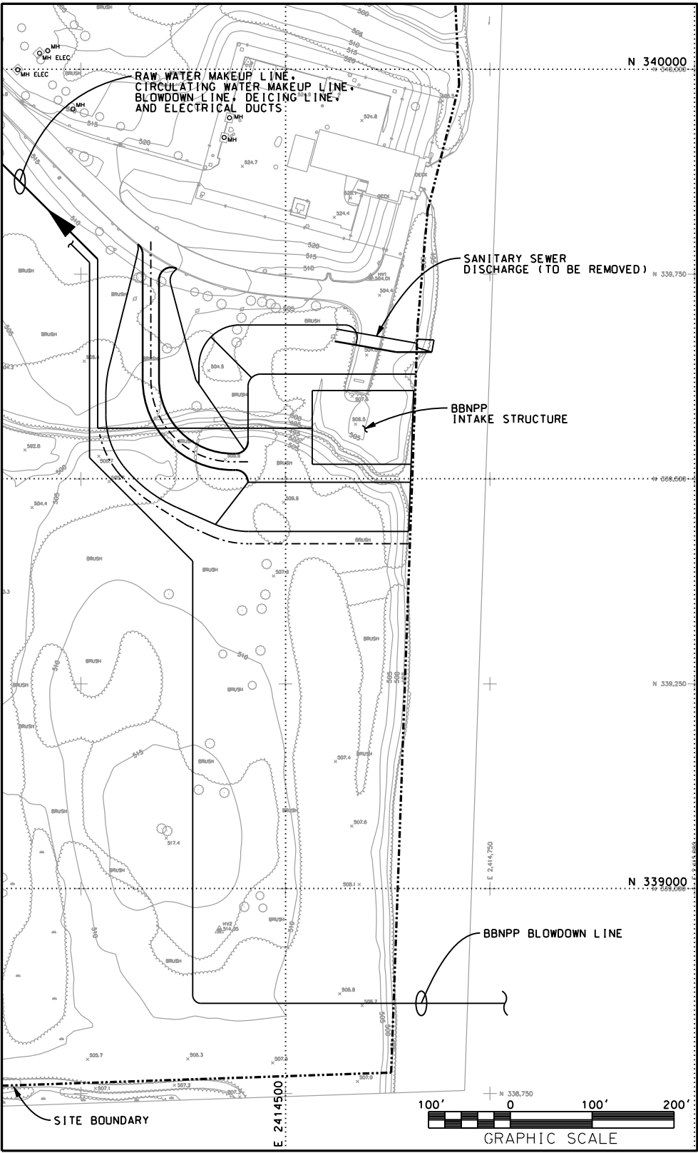
Figure 3.4-3 {Circulating Water System Intake/Discharge Structure Location Plan}
