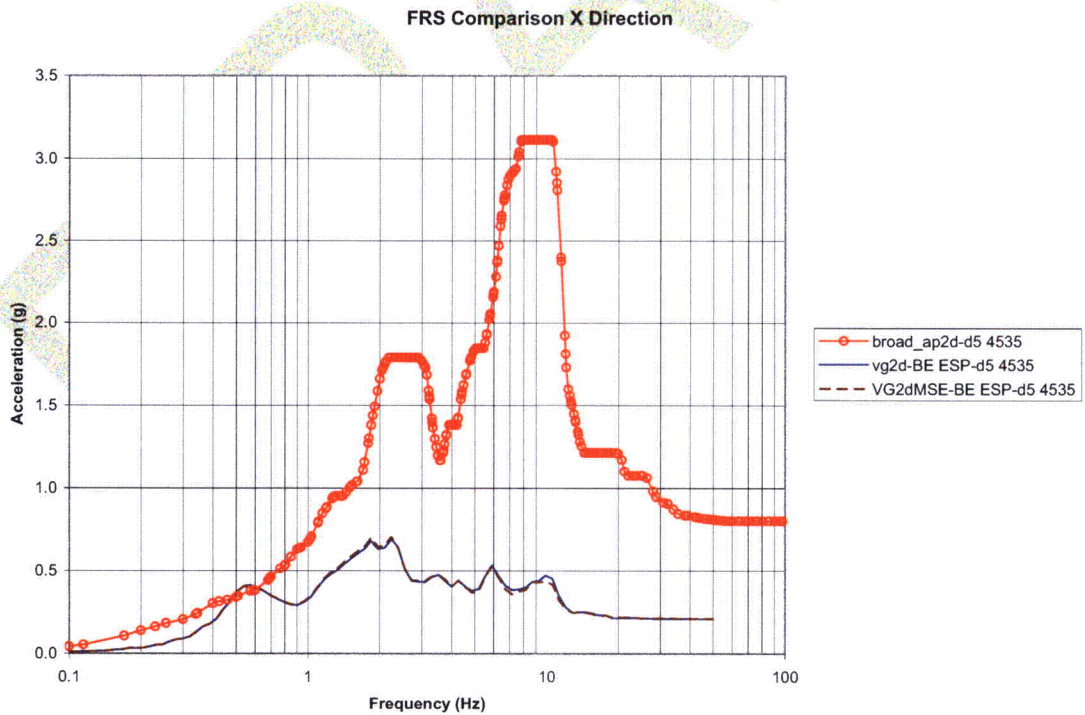
Figure 5.3-17 – FRS Comparison at Node 4535 (X Direction)
