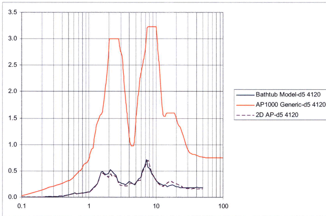
Figure A-4: FRS Comparison at Node 4120
