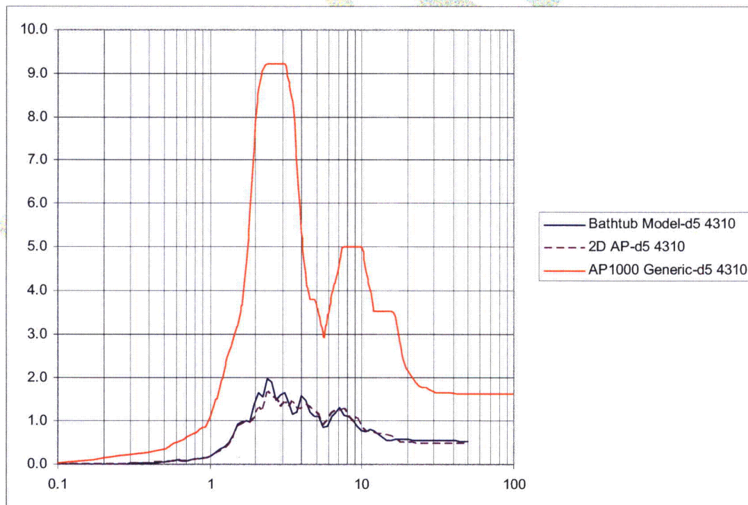
Figure A-5: FRS Comparison at Node 4310
