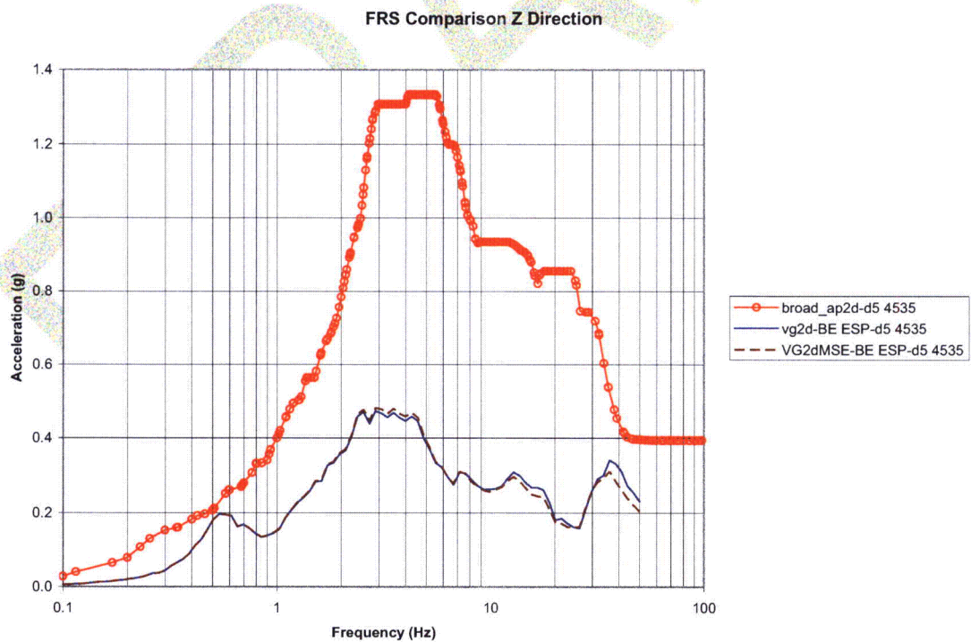
Figure 5.3-19 – FRS Comparison at Node 4535 (Z Direction)
