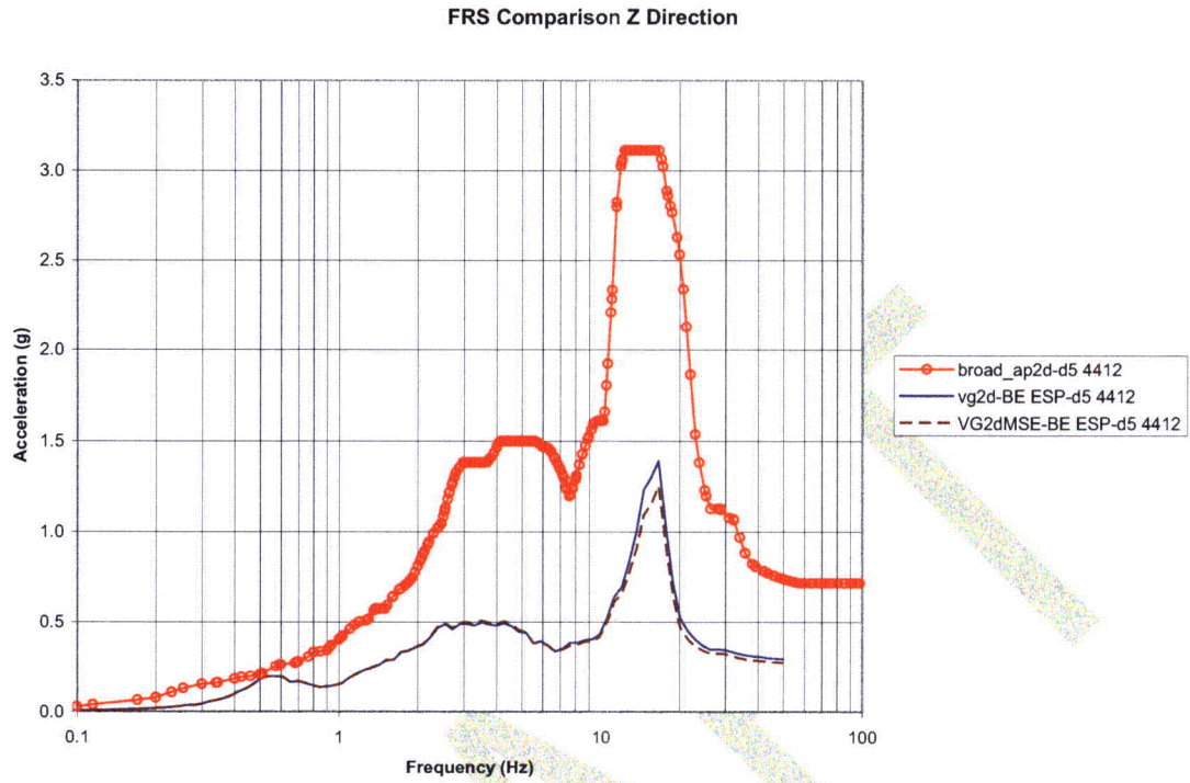
Figure 5.3-16 – FRS Comparison at Node 4412 (Z Direction)
