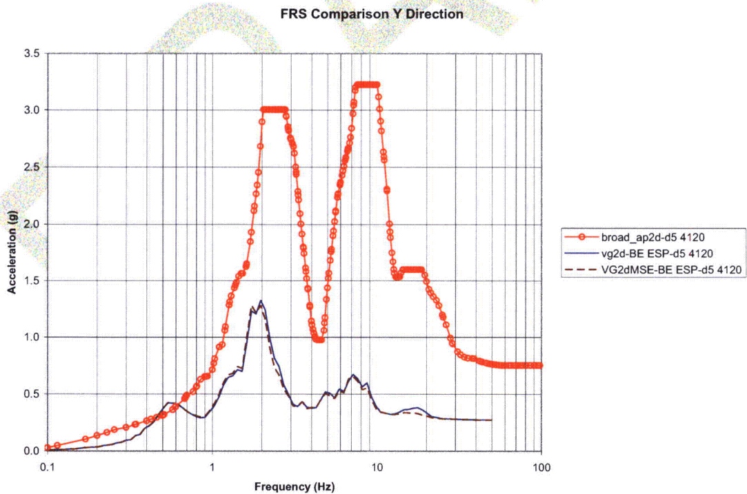
Figure 5.3-9 – FRS Comparison at Node 4120 (Y Direction)
