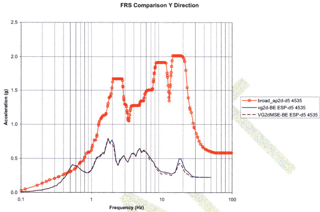
Figure 5.3-18 – FRS Comparison at Node 4535 (Y Direction)
