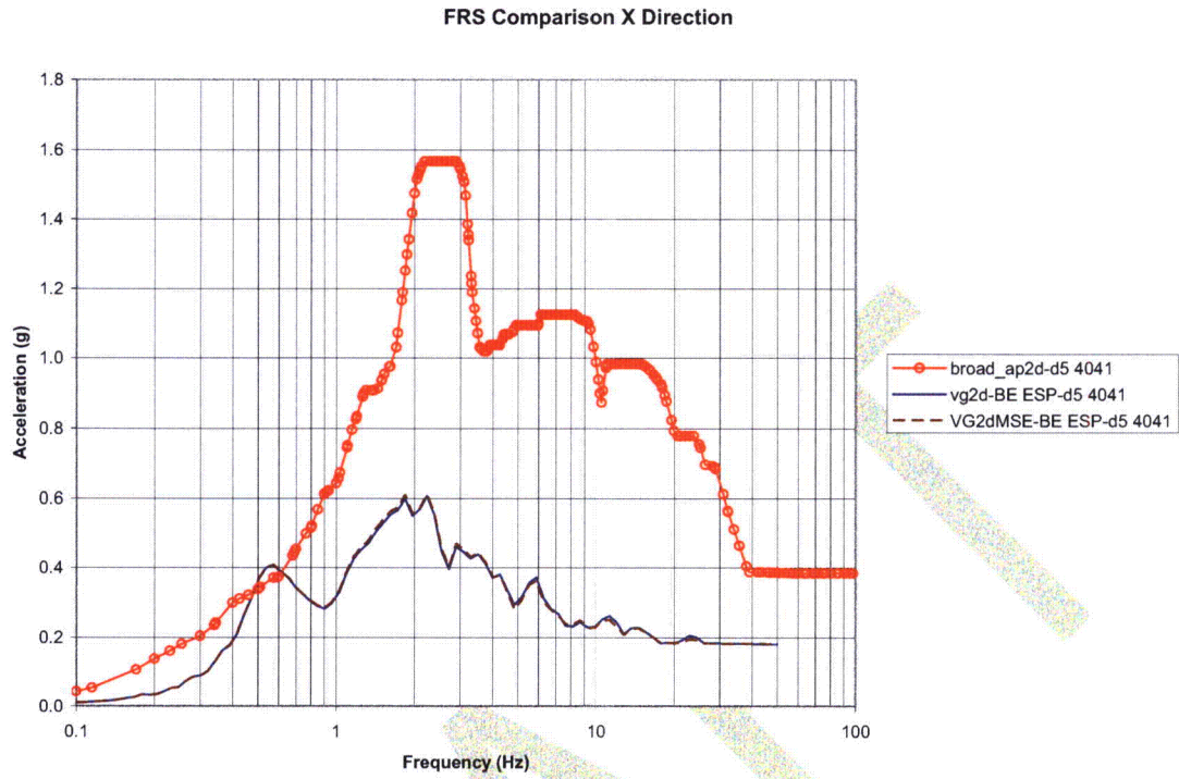
Figure 5.3-2 – FRS Comparison at Node 4041 (X Direction)
