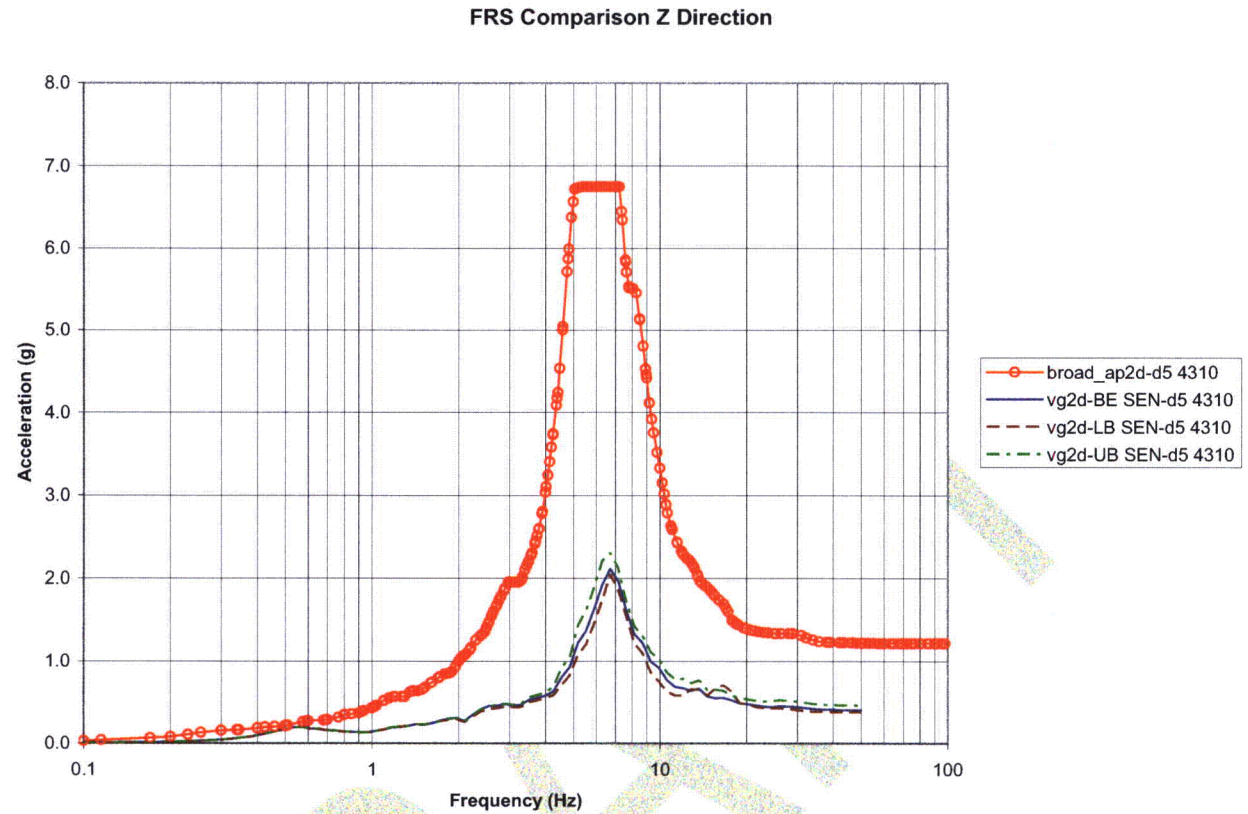
Figure 5.1-30 - Comparison of Node 4310 SEN to AP1000 SSI Envelope, Vertical Dir
