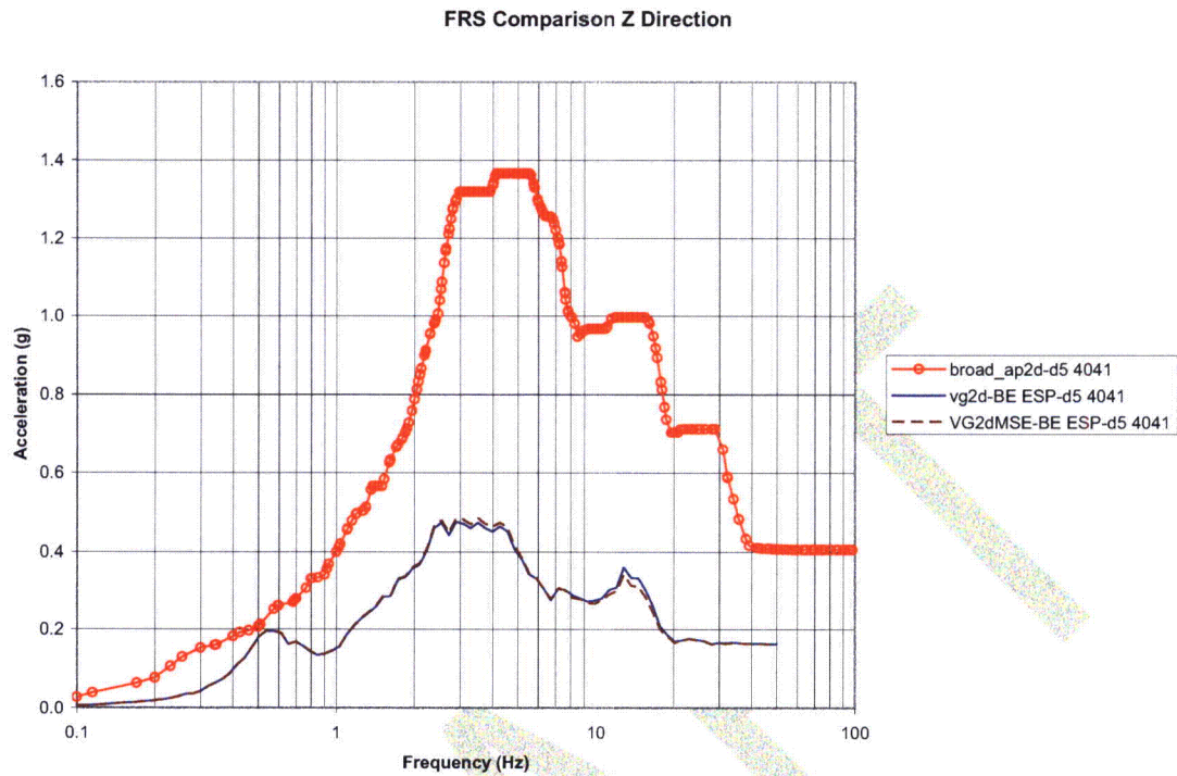
Figure 5.3-4 – FRS Comparison at Node 4041 (Z Direction)
