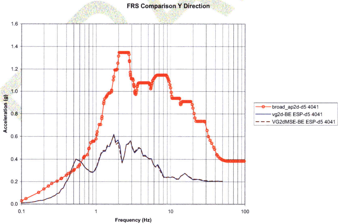
Figure 5.3-3 – FRS Comparison at Node 4041 (Y Direction)
