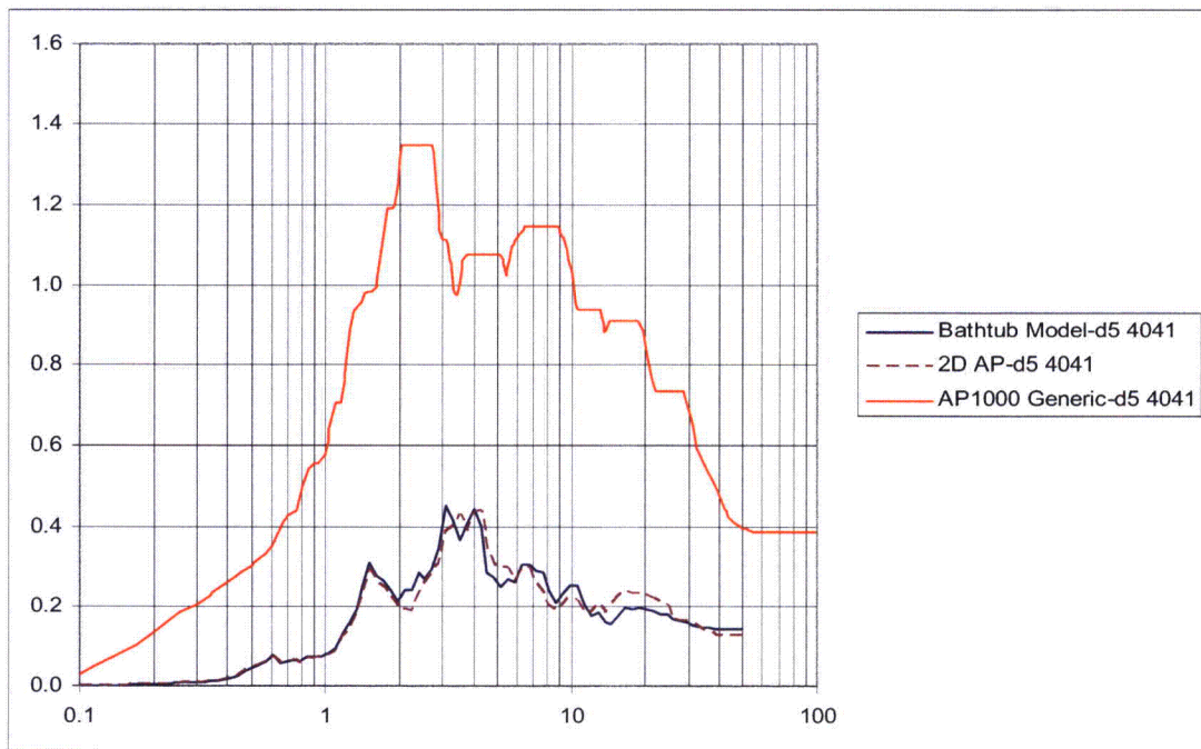
Figure A-2: FRS Comparison at Node 4041
