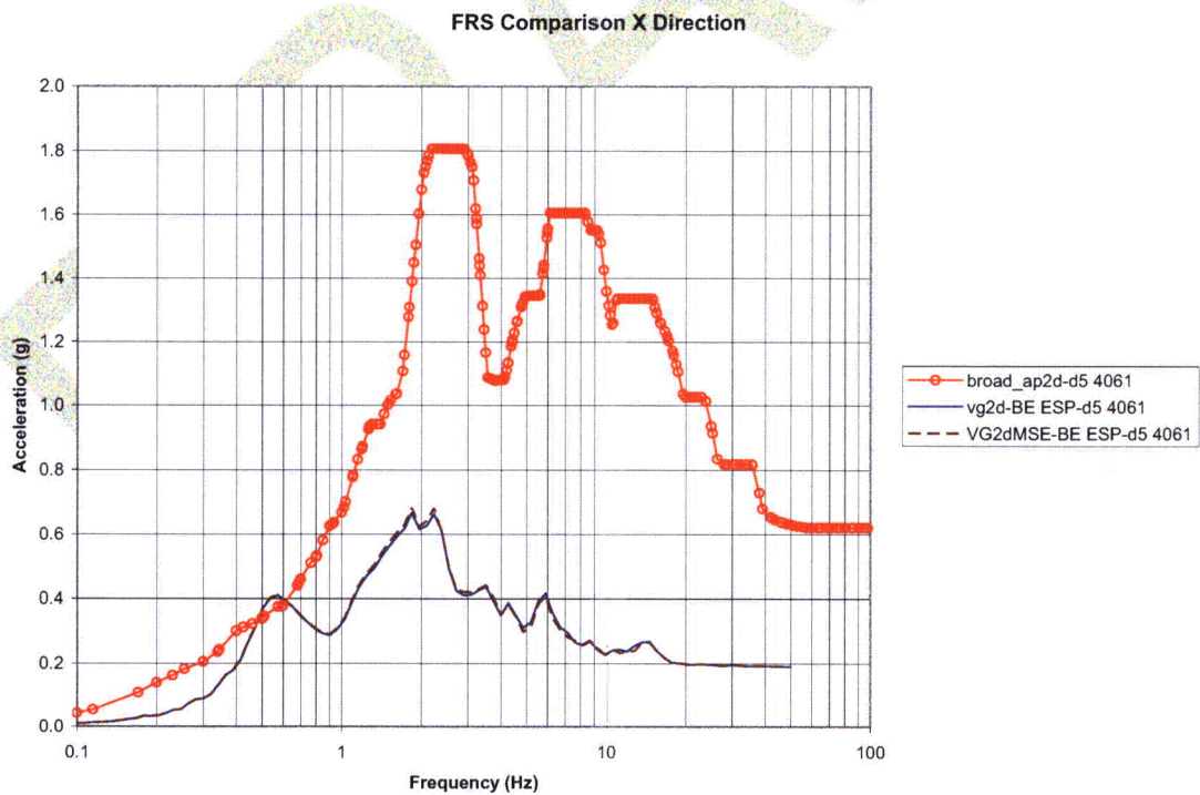
Figure 5.3-5 – FRS Comparison at Node 4061 (X Direction)
