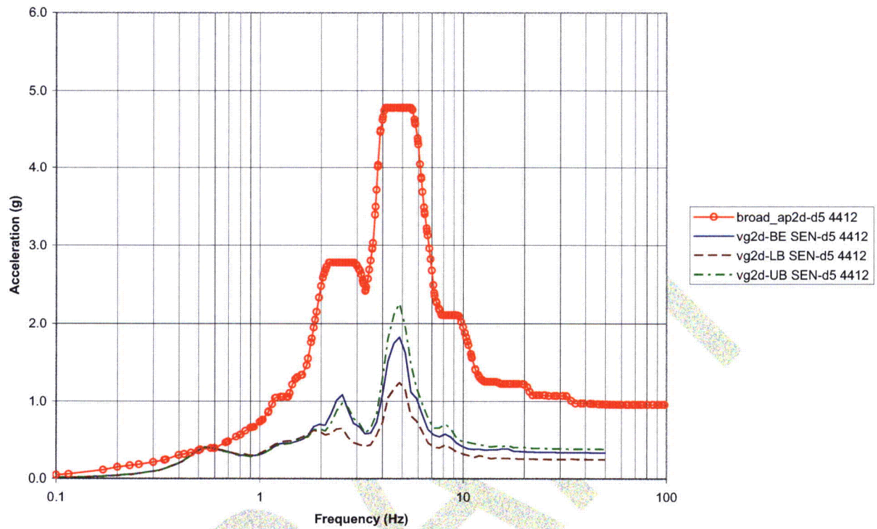
Figure 5.1-31 - Comparison of Node 4412 SEN to AP1000 SSI Envelope, NS Dir
