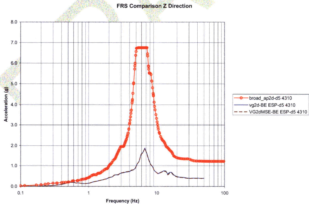
Figure 5.3-13 – FRS Comparison at Node 4310 (Z Direction)
