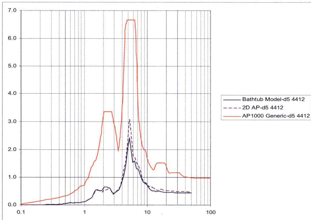
Figure A-6: FRS Comparison at Node 4412
