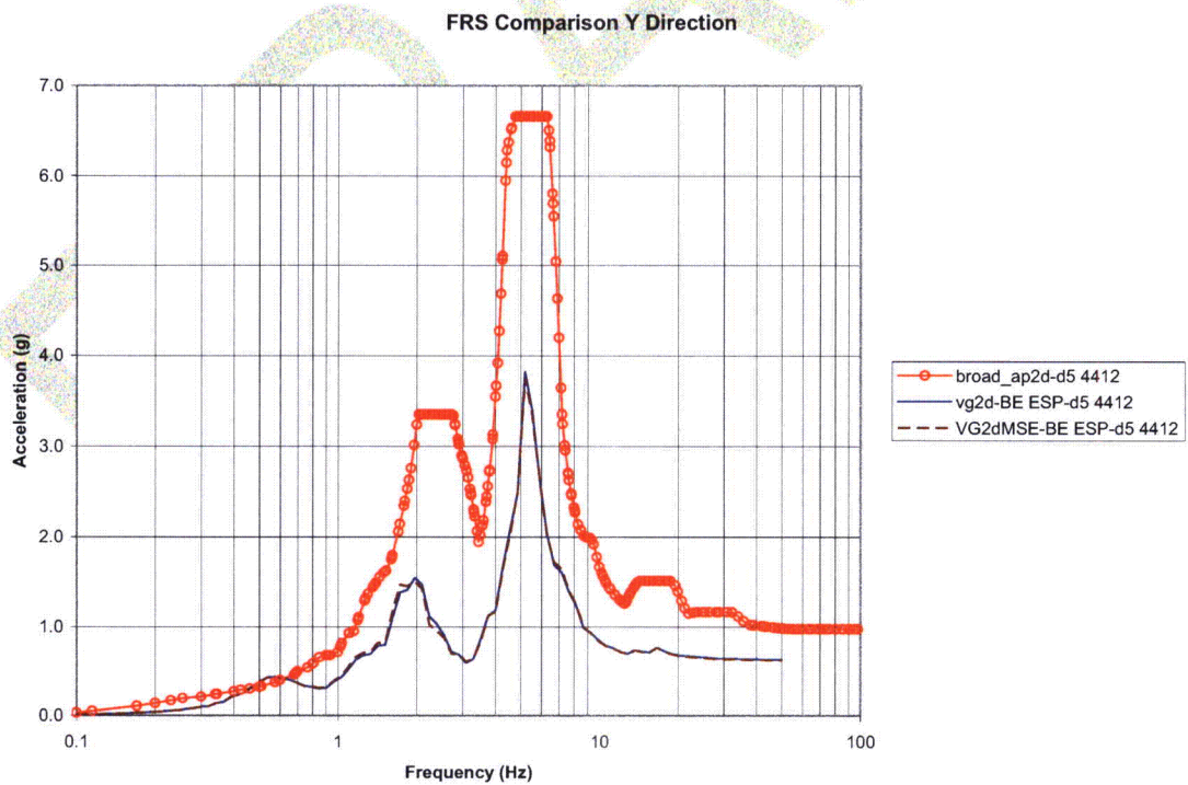
Figure 5.3-15 – FRS Comparison at Node 4412 (Y Direction)
