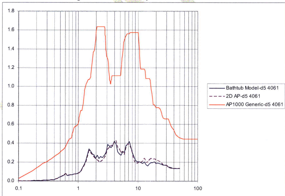
Figure A-3: FRS Comparison at Node 4061
