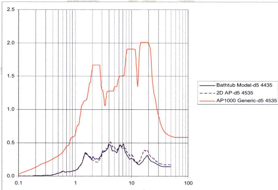
Figure A-7: FRS Comparison at Node 4535
