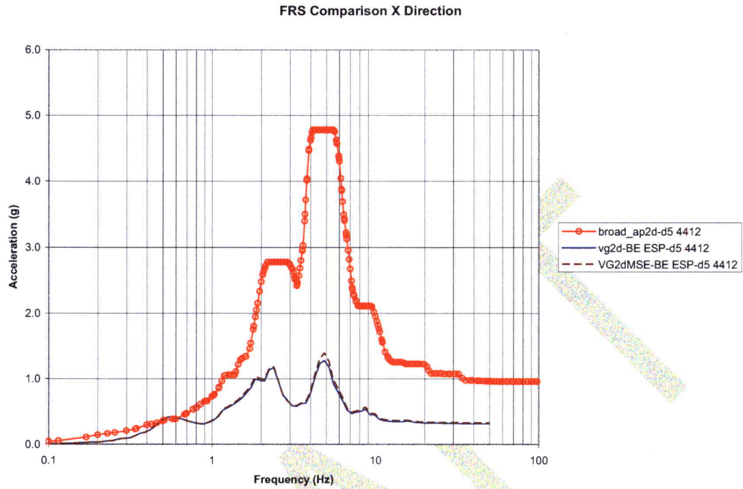
Figure 5.3-14 – FRS Comparison at Node 4412 (X Direction)
