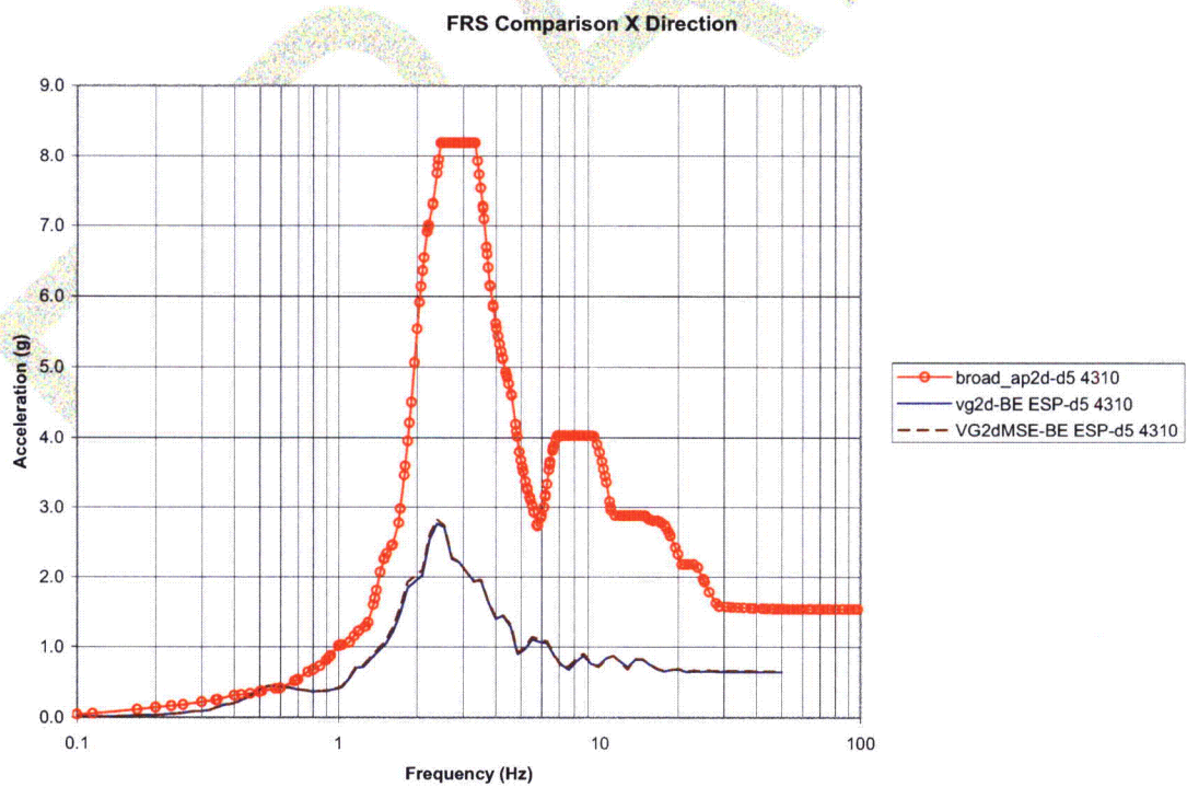
Figure 5.3-11 – FRS Comparison at Node 4310 (X Direction)
