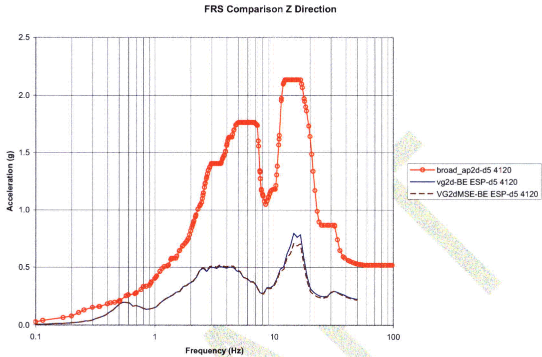
Figure 5.3-10 – FRS Comparison at Node 4120 (Z Direction)
