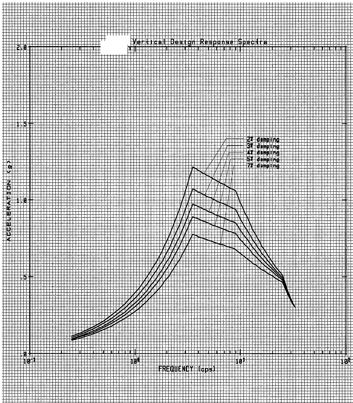
Figure 3-2 – AP1000 Vertical Design Response Spectra Safe Shutdown Earthquake
