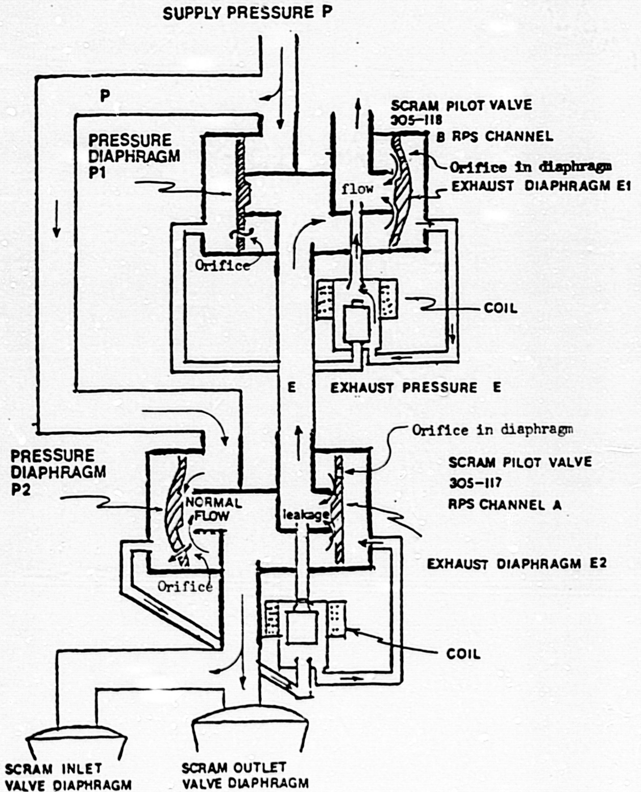
Scram Pilot Valve Configuration
