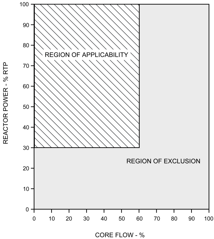
FIGURE 3.3.1.1-1 OSCILLATION POWER RANGE FUNCTION CONDITIONS OF OPERABILITY
