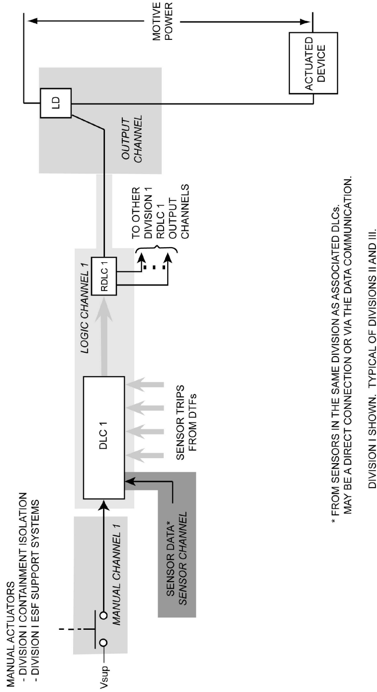
FIGURE B3.3.1.4-1 ESF ACTUATION CHANNEL STRUCTURE FOR CONTAINMENT ISOLATION, ESF SUPPORT
