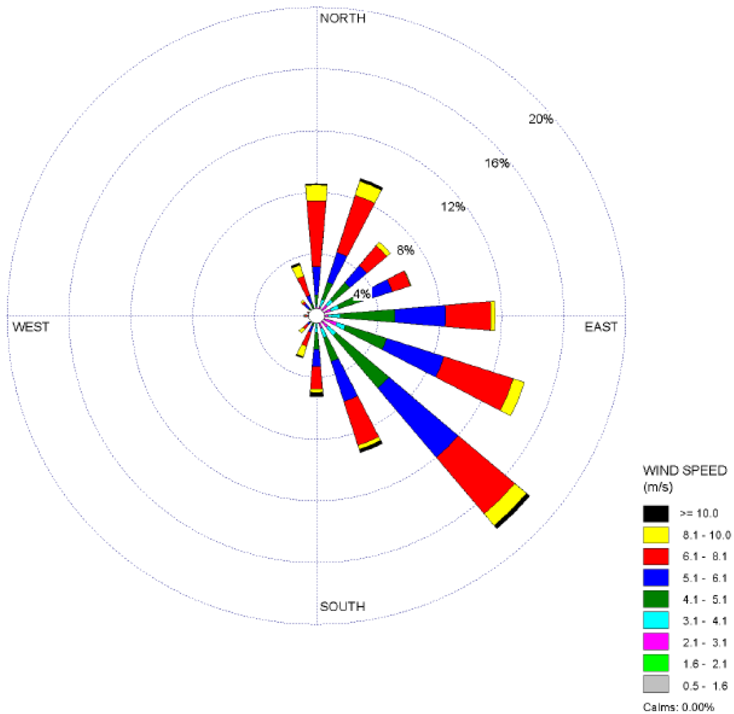
Figure 2.7-13 STP 60-Meter Level 3-Year Composite Wind Rose - October (1997, 1999, and 2000) - Page 10 of 12
