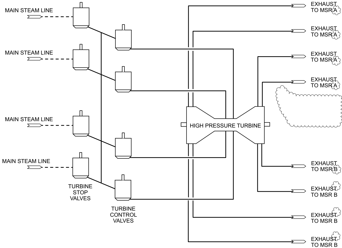
Figure 10.3-2 Main Steam Turbine System
