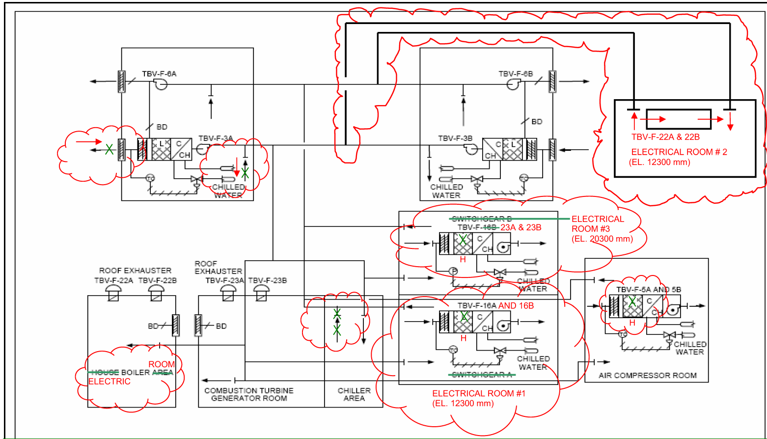
Figure 9.4-2c Electrical Building HVAC System Diagram Turbine Building Electrical Equipment Areas (EEA) HVAC System Diagram
