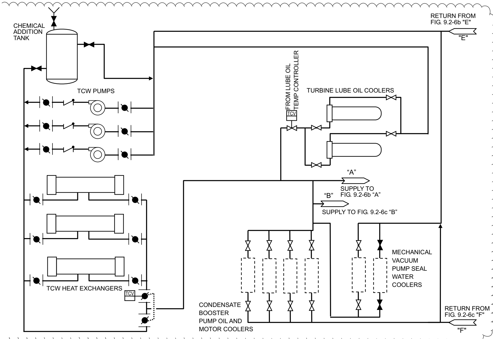
Figure 9.2-6a Turbine Building Cooling Water System Diagram
