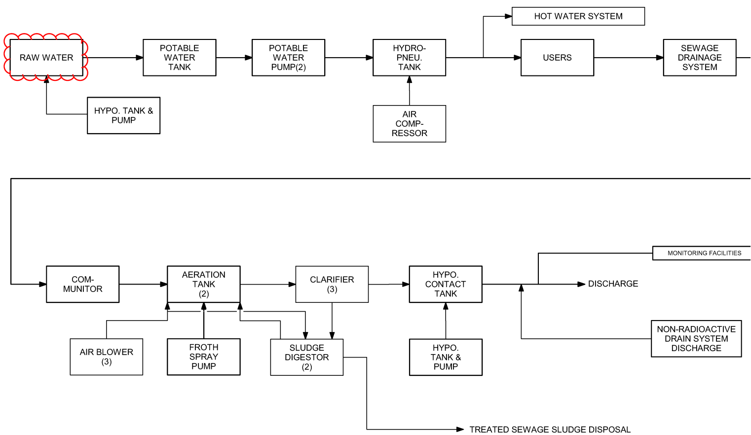
Figure 9.2-9 Potable and Sanitary Water System (Sheet 1 of 2)
