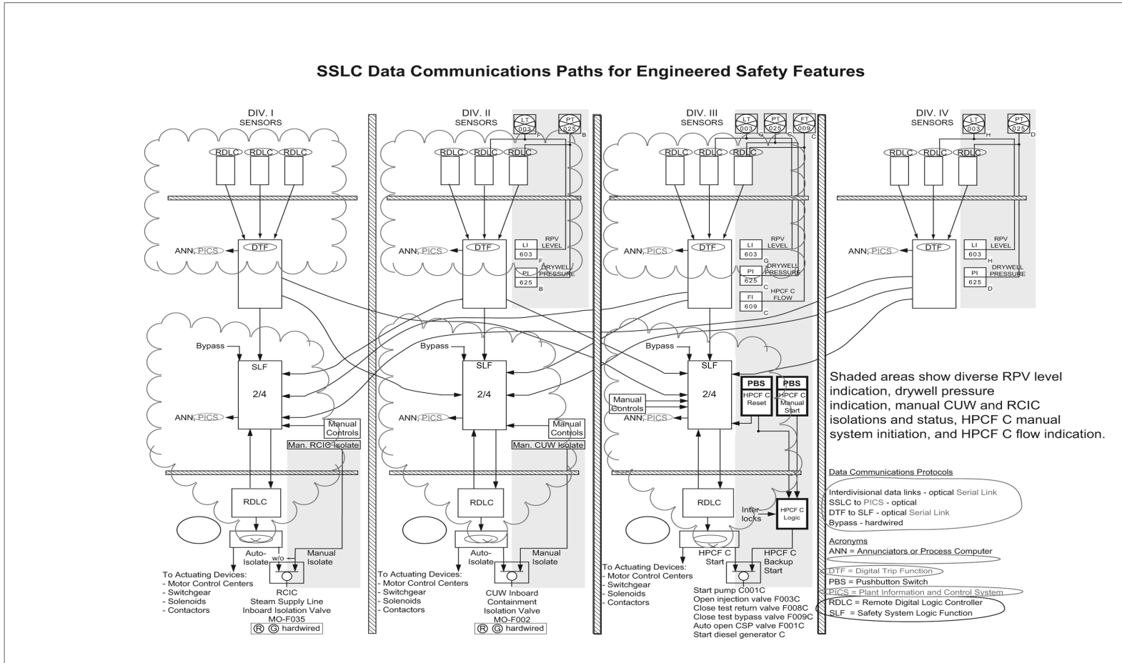
Figure 7C-1 Implementation of Additional Diversity in SSLC to Mitigate Effects of Common-Mode Failures
