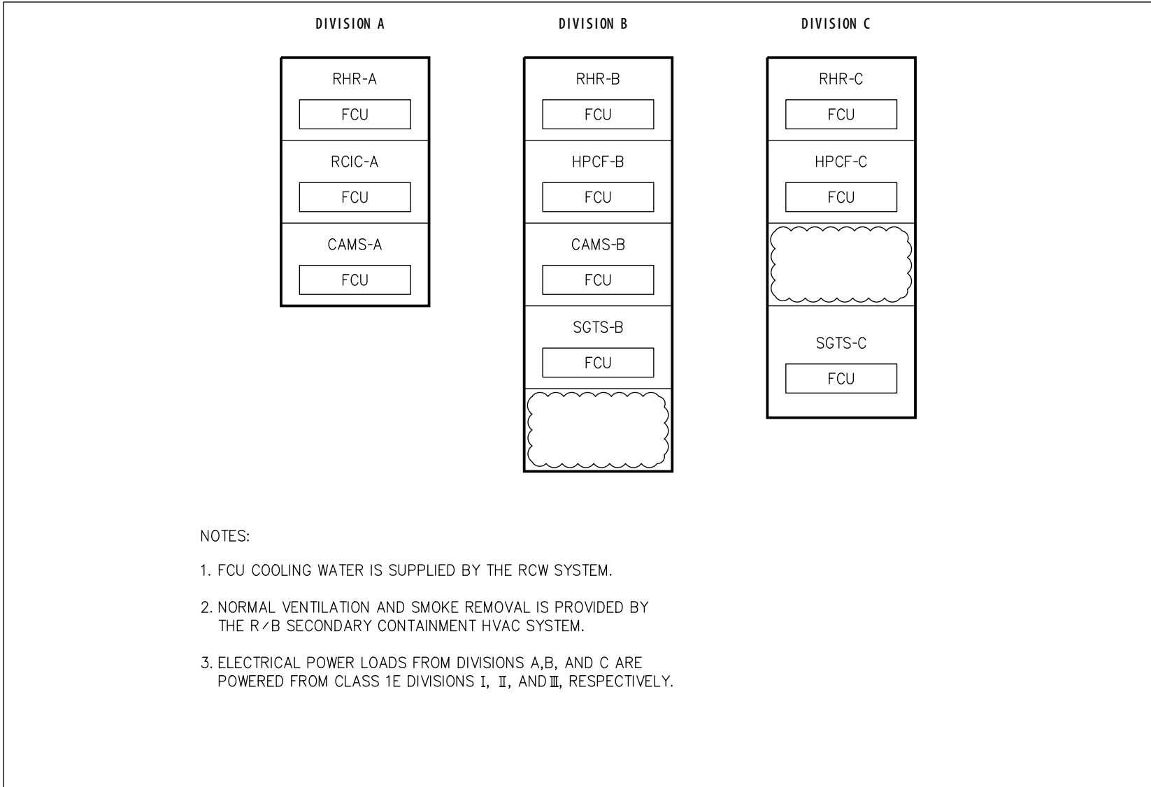
Figure 2.15.5e Reactor Building Safety-Related Equipment HVAC System
