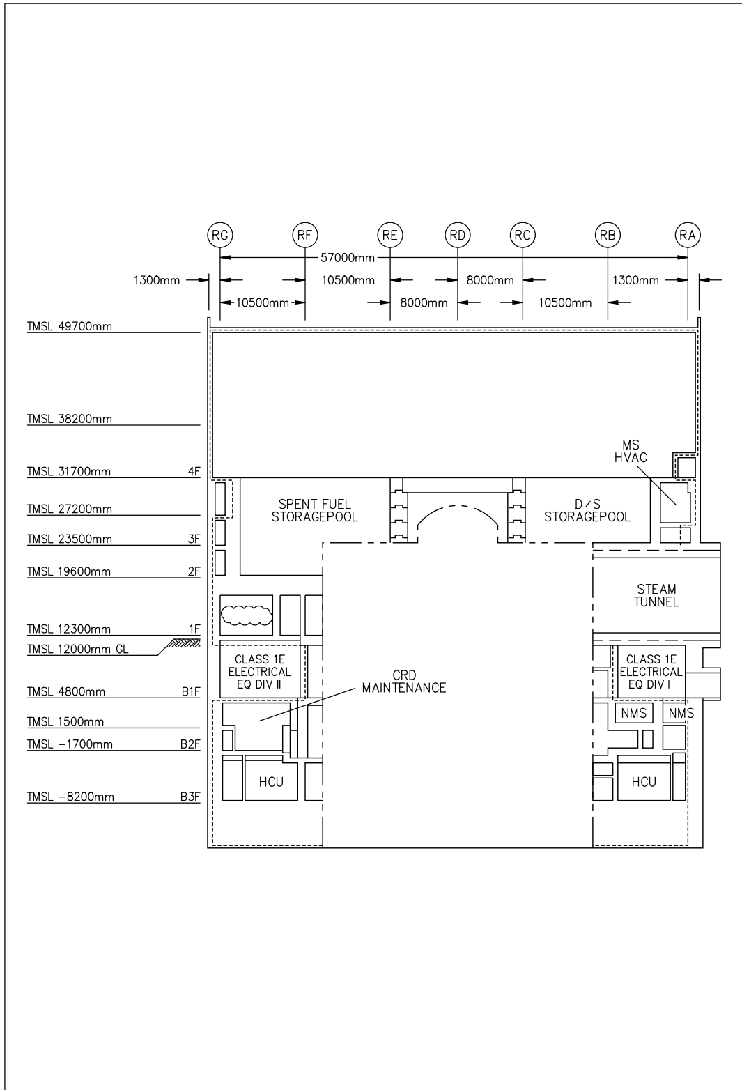
Figure 2.15.10a Reactor Building Arrangement - Section A-A
