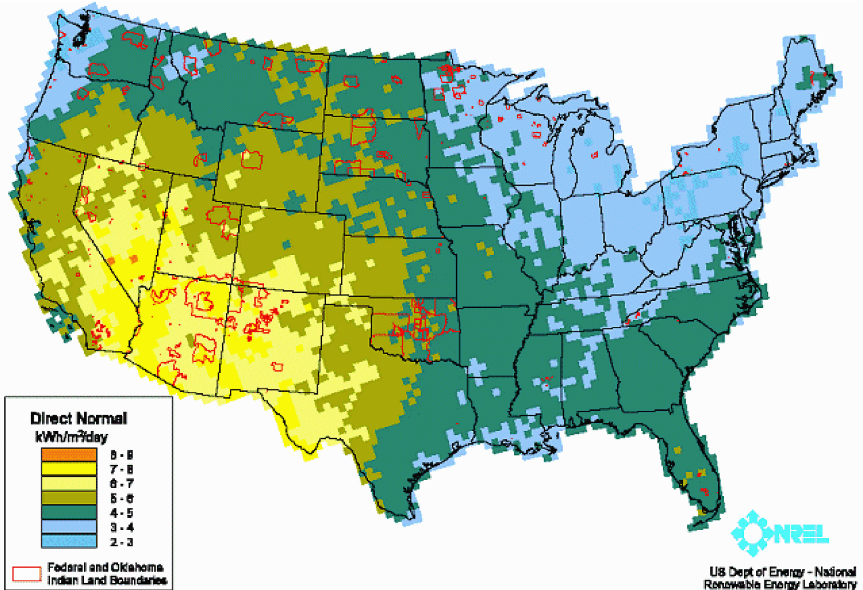
Figure 9.2-5 Concentrated Solar Power Resource Potential
