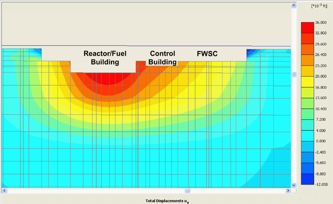
a) Profile View Through Cross-Section A-A (Center Line of R/FB)
