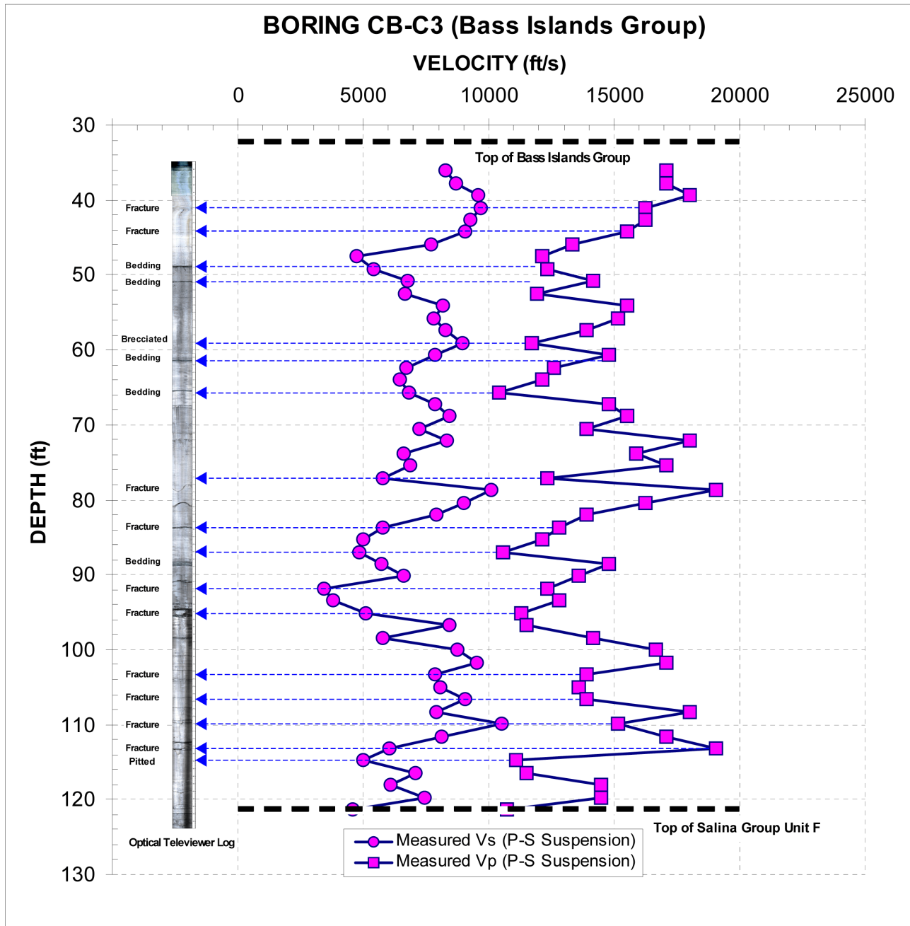
Figure 2.5.4-211 Influence of geologic features within Bass Islands Group on measured seismic wave velocities in Borehole CB-C3
