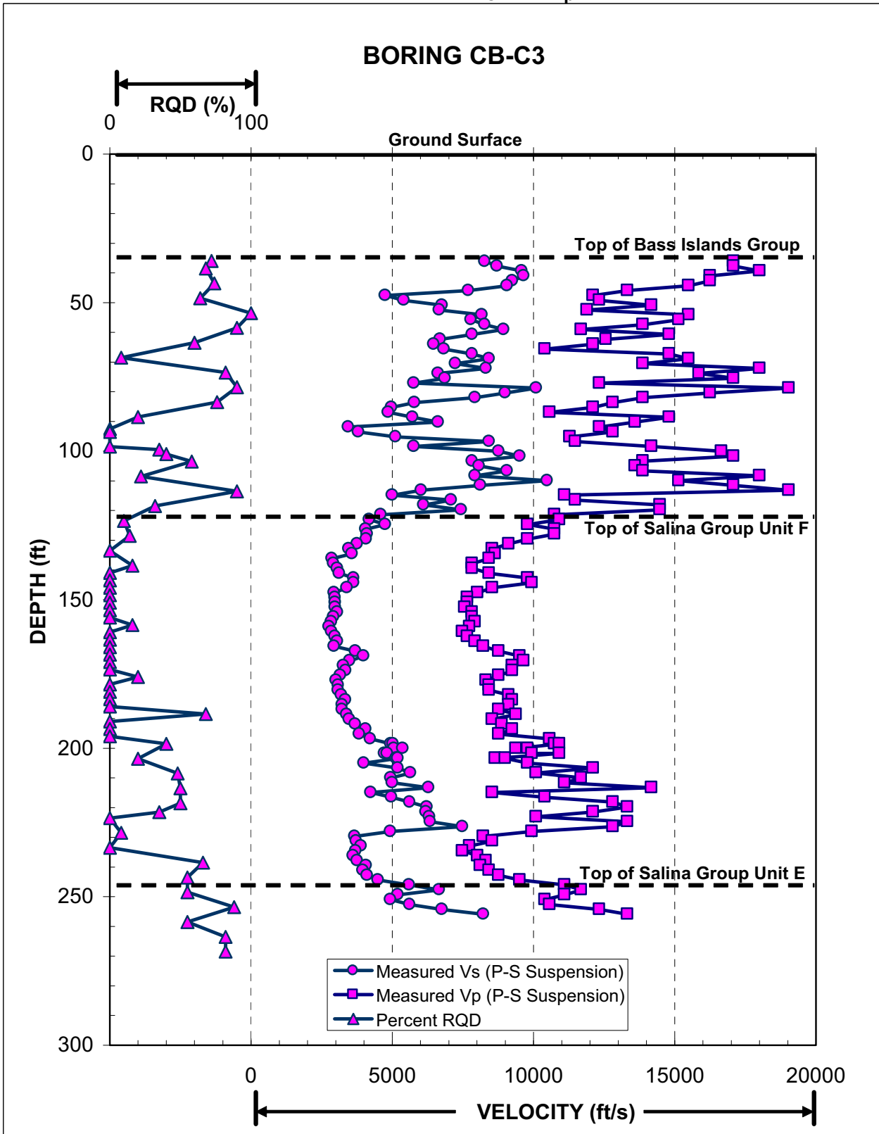
Figure 2.5.4-207 Comparison of measured V_s and V_p with RQD for Boring CB-C3
