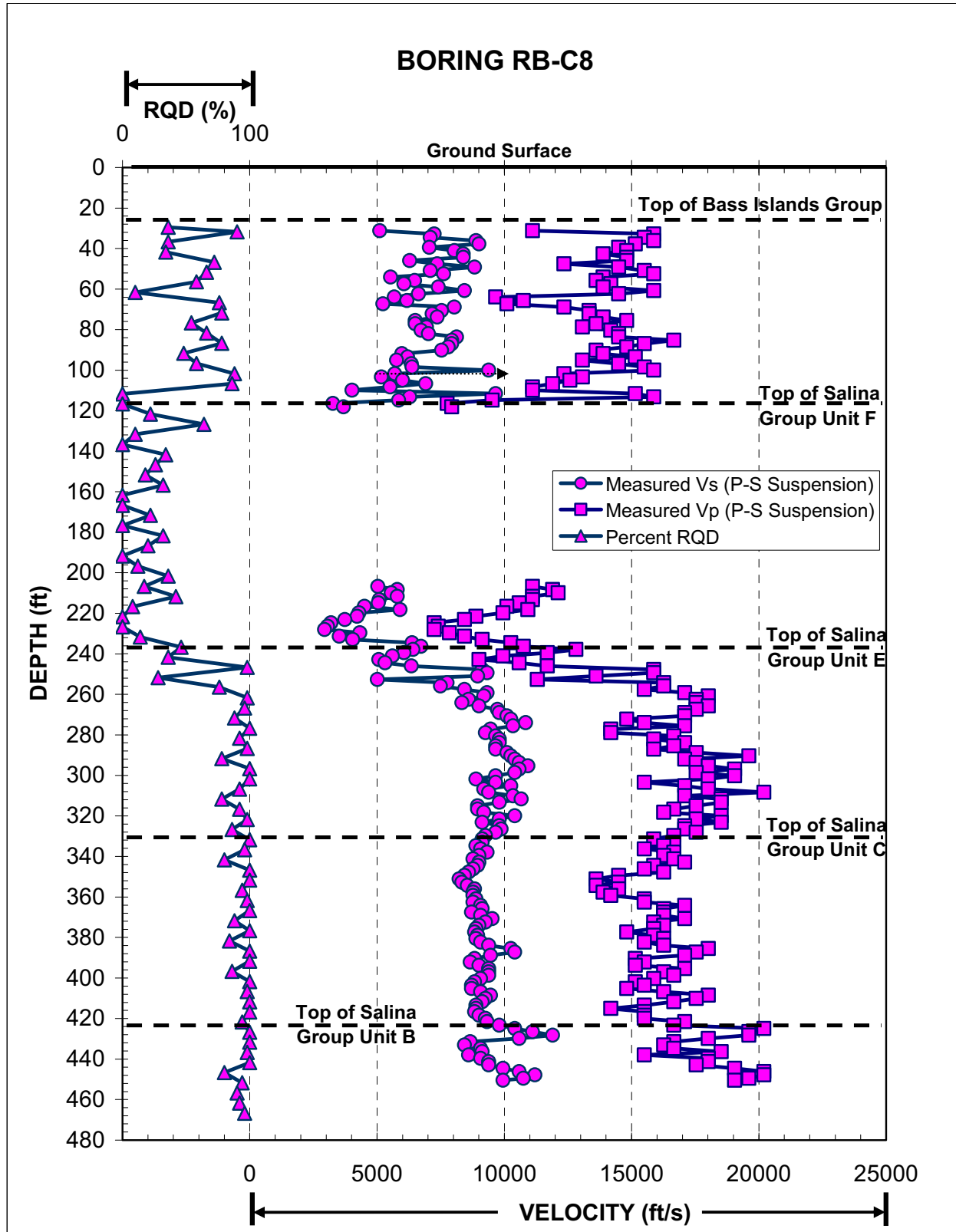
Figure 2.5.4-206 Comparison of measured V_s and V_p with RQD for Boring RB-C8
