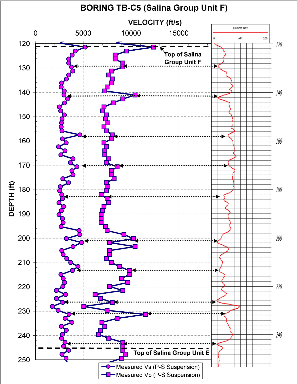
Figure 2.5.4-213 Influence of shale or claystone content within Salina Group Unit F on measured seismic wave velocities in Boring TB-C5
