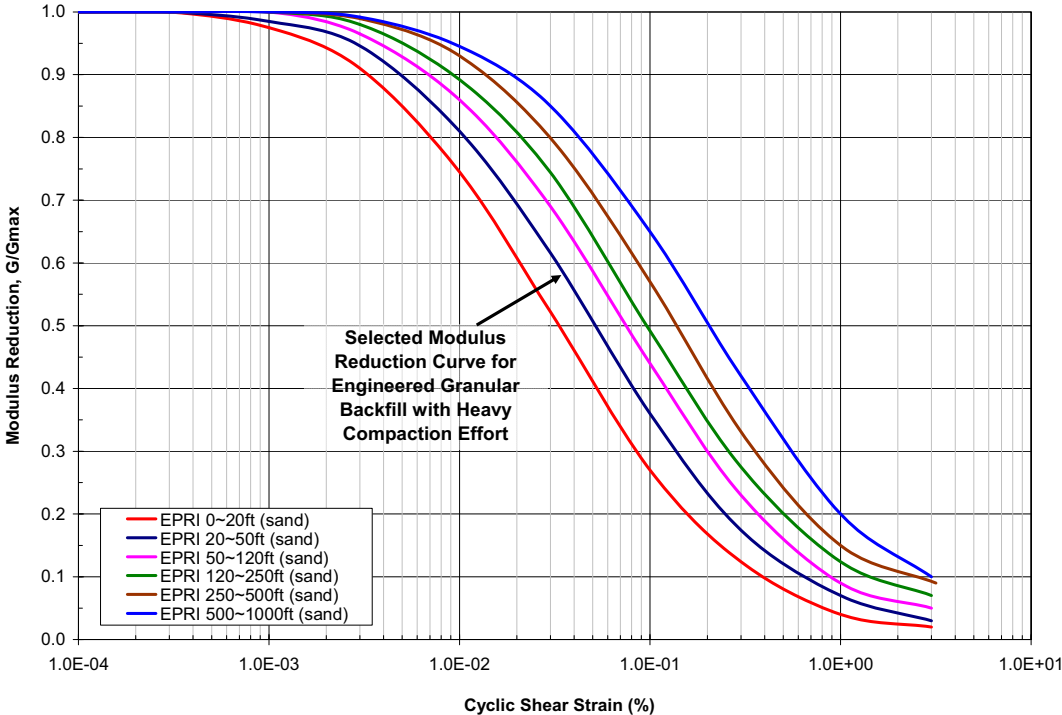
Figure 2.5.4-227 Selected Shear Modulus Reduction and Damping Curves for Engineered Granular Backfill
