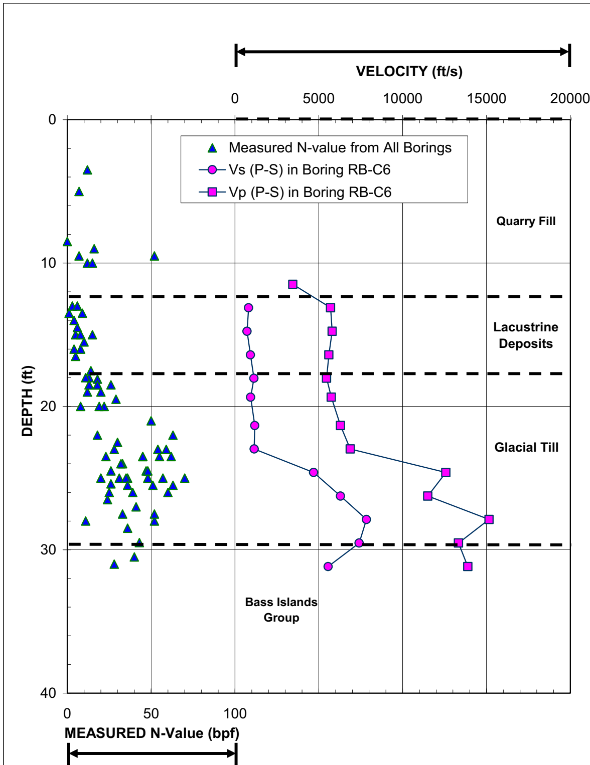
Figure 2.5.4-217 Comparison of measured shear and compression wave velocity profile using P-S suspension method in Boring RB-C6 with measured N-values within overburden
