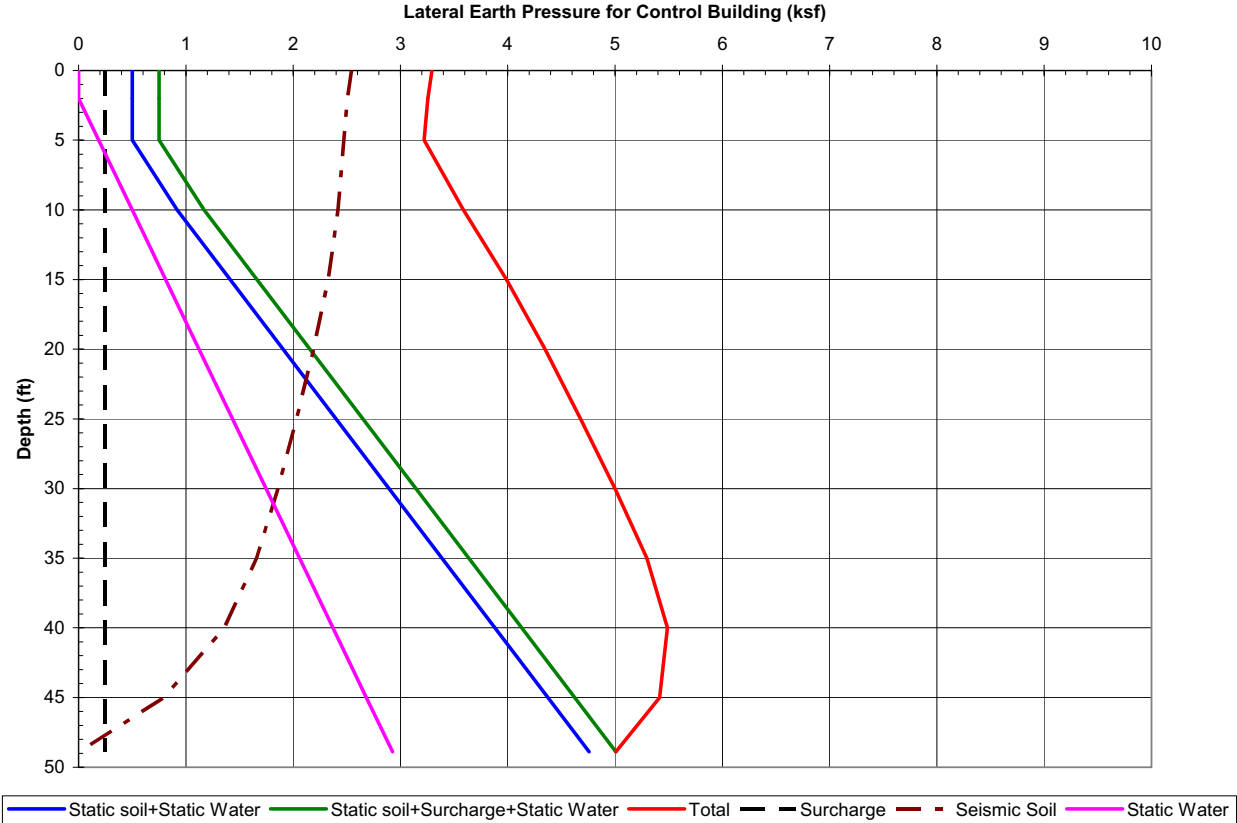
Figure 2.5.4-231 Lateral Earth Pressure on Control Building Walls
