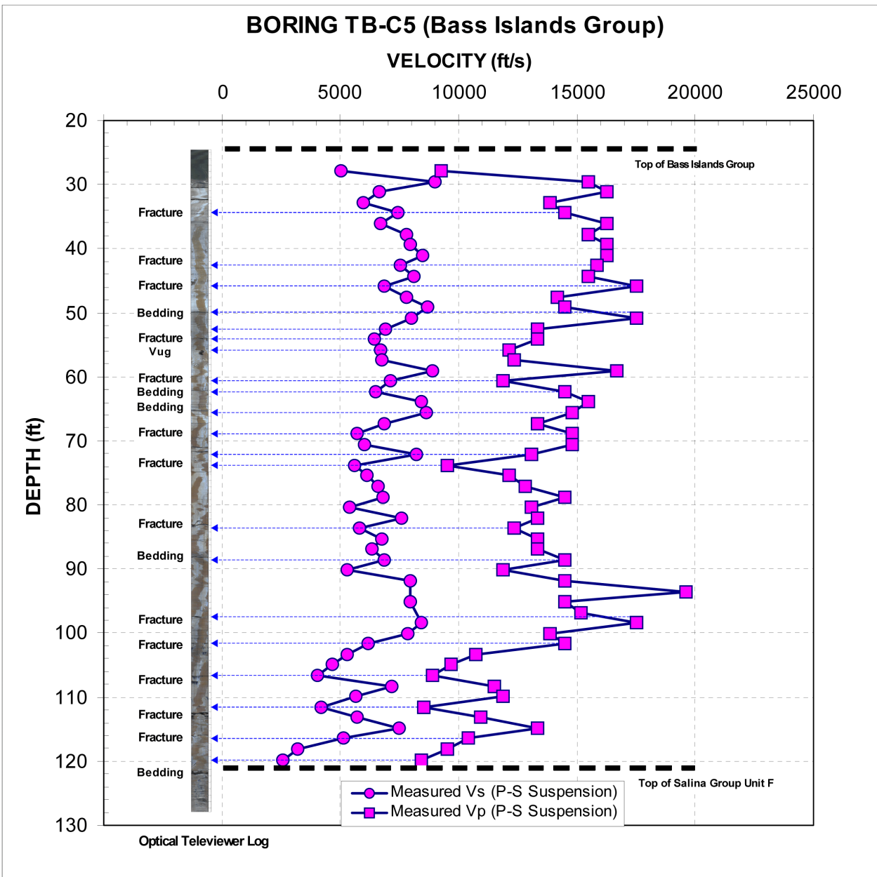
Figure 2.5.4-209 Influence of geologic features within Bass Islands Group on measured seismic wave velocities in Borehole TB-C5
