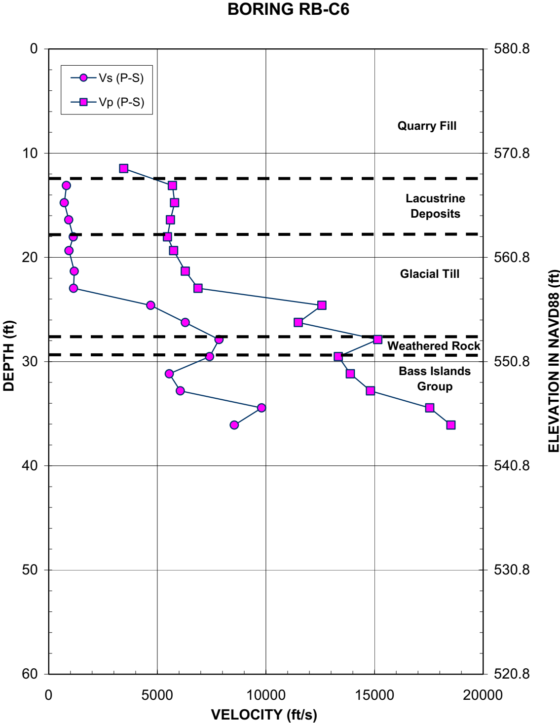
Figure 2.5.4-224 Measured shear and compression wave velocity profiles in the overburden using P-S Suspension Logger in Boring RB-C6
