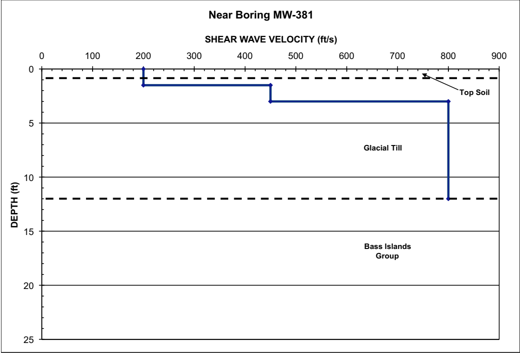
Figure 2.5.4-219 Measured shear wave velocity profile using SASW method in the overburden near Borings RB-C4, RW-C1, MW-381 and MW-393 (Sheet 2 of 2)
