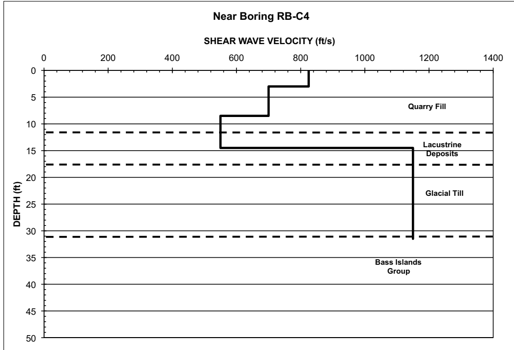
Figure 2.5.4-219 Measured shear wave velocity profile using SASW method in the overburden near Borings RB-C4, RW-C1, MW-381 and MW-393 (Sheet 1 of 2)
