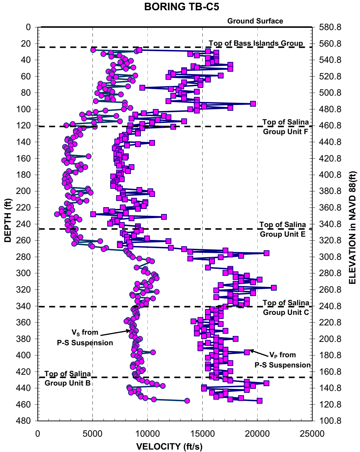
Figure 2.5.4-220 Measured shear and compression wave velocity profiles using P-S Suspension method in Boring TB-C5
