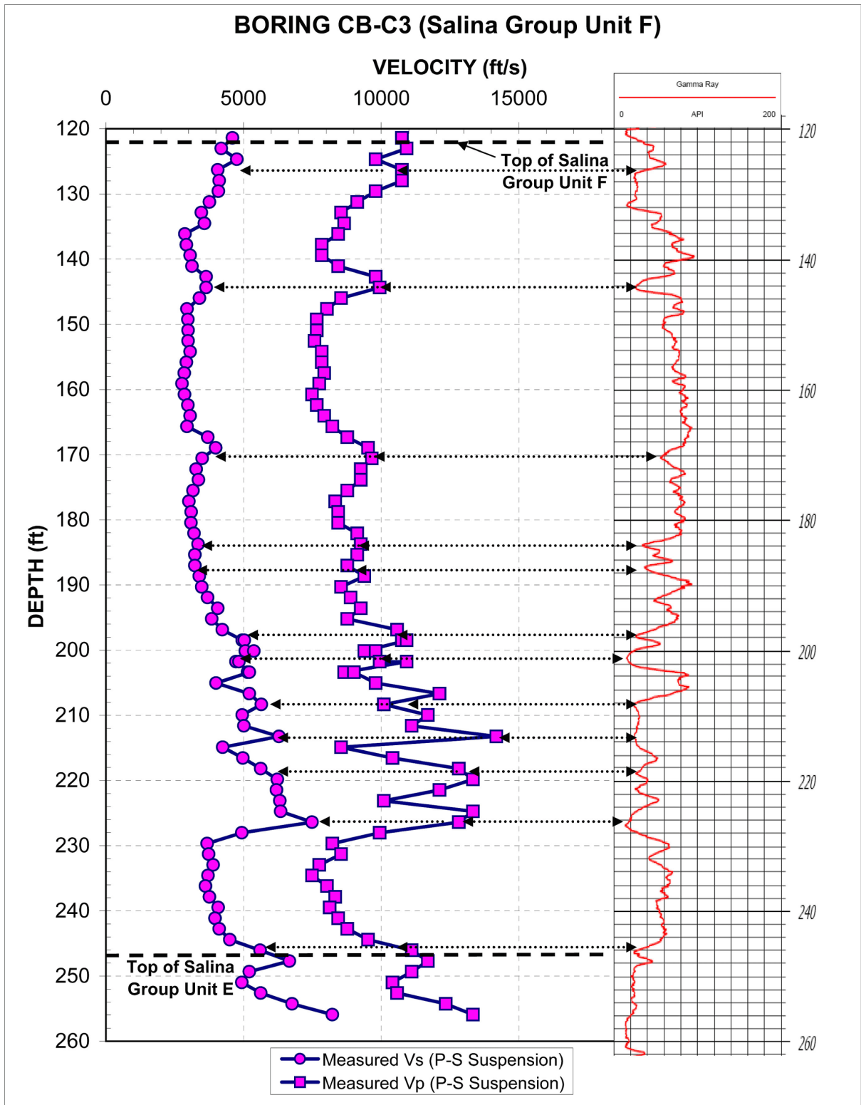
Figure 2.5.4-214 Influence of shale or claystone content within Salina Group Unit F on measured seismic wave velocities in Boring CB-C3
