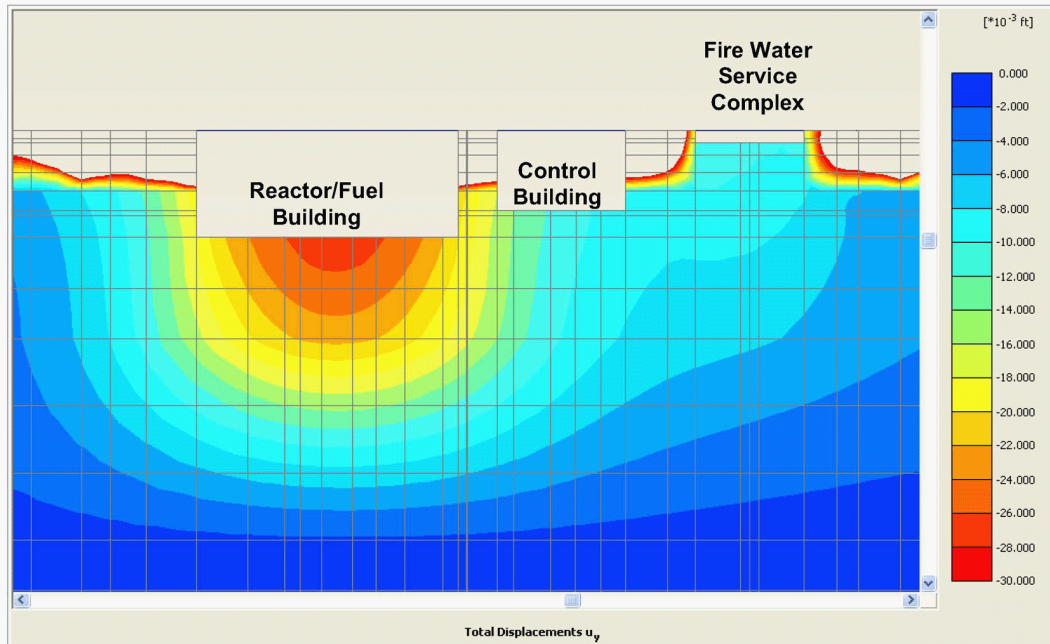
b) Profile View Through Cross-Section A-A (Center Line of R/FB)
