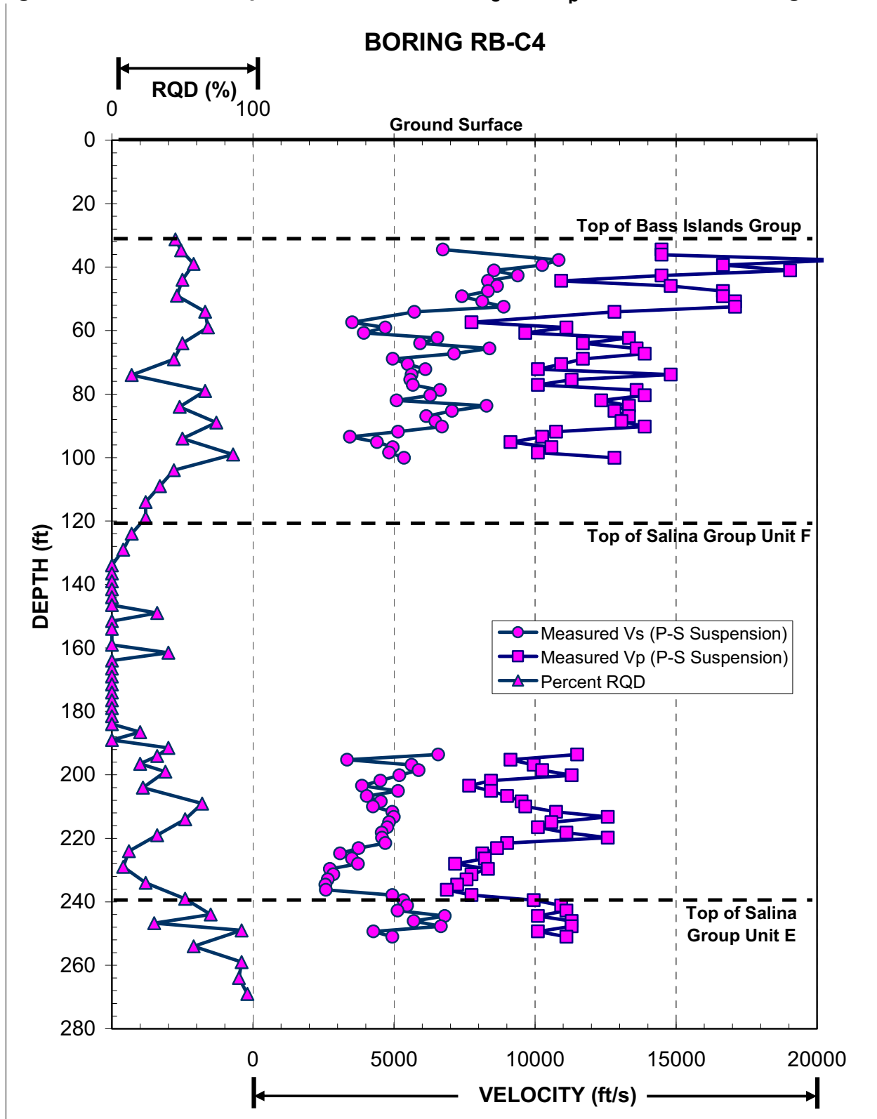
Figure 2.5.4-208 Comparison of measured V_s and V_p with RQD for Boring RB-C4
