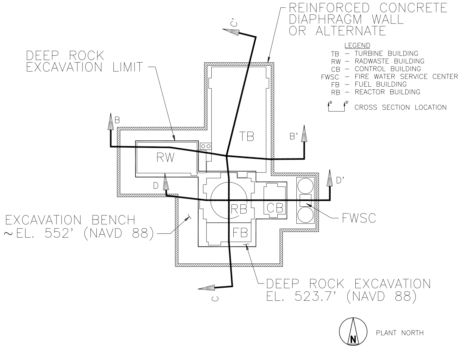
Figure 2.5.4-201 Excavation Site Plan
