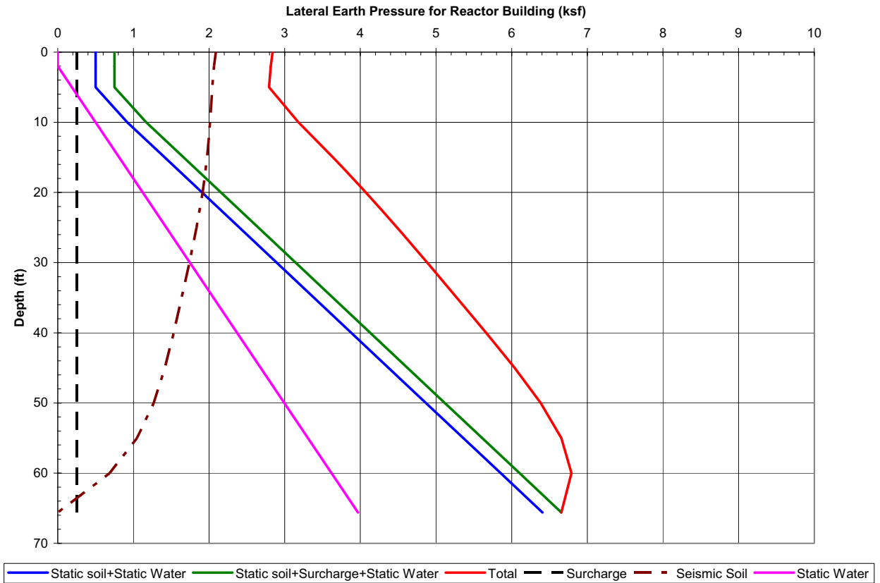
Figure 2.5.4-230 Lateral Earth Pressure on Reactor Building Walls
