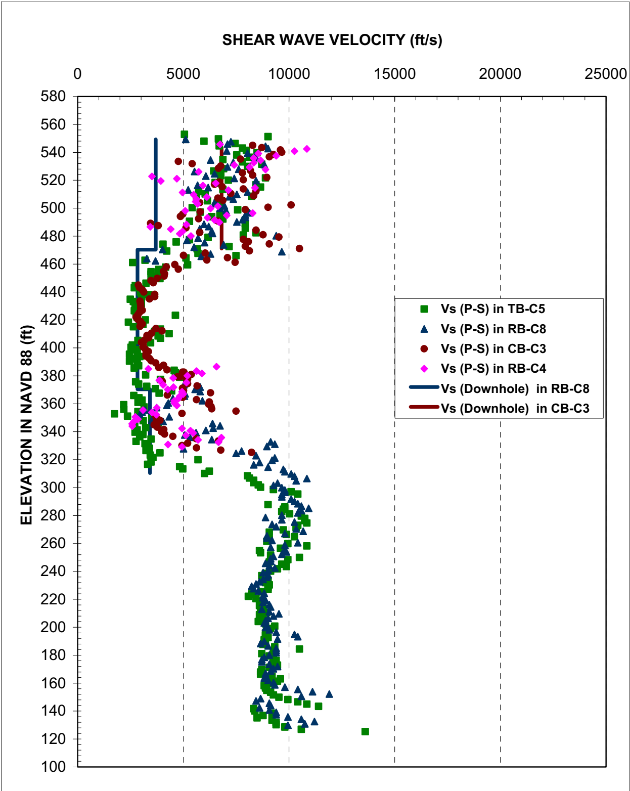
Figure 2.5.4-216 Shear wave velocity measurements using both P-S and Downhole Methods in Borings TB-C5, RB-C8, CB-C3, and RB-C4
