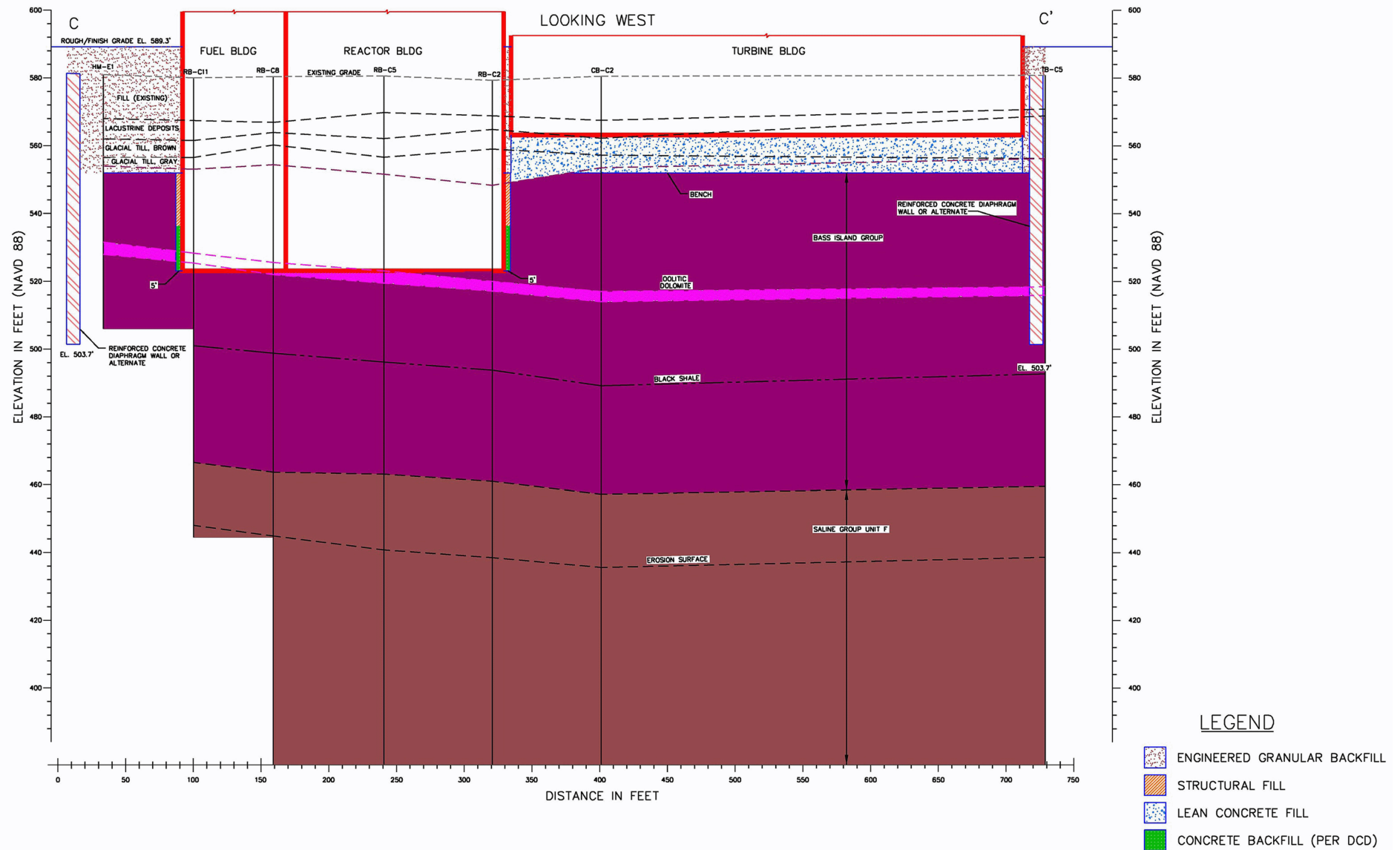
Figure 2.5.4-203 Excavation Cross Section C-C
