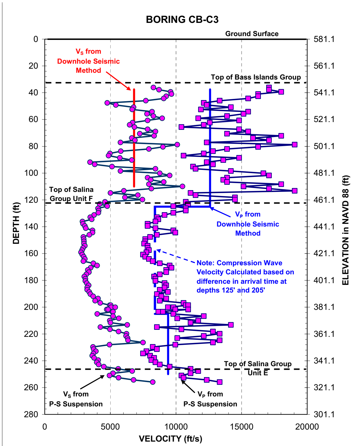
Figure 2.5.4-222 Measured shear and compression wave velocity profiles using P-S Suspension and Downhole Seismic methods in Boring CB-C3
