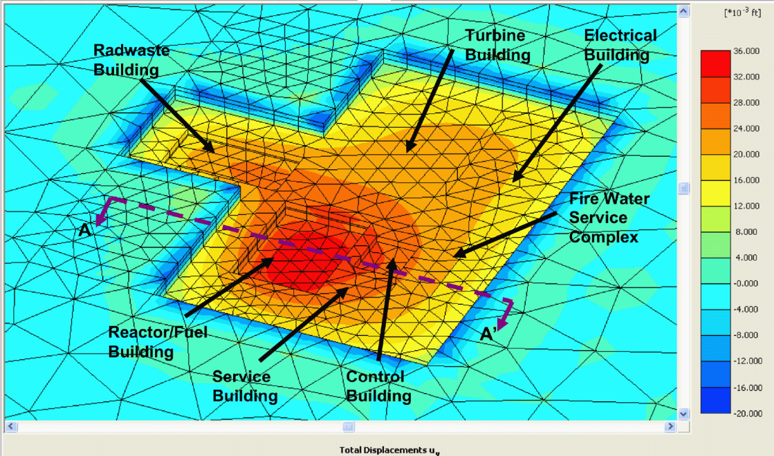
Figure 2.5.4-228 Total vertical displacement at end of excavation stage (Rebound due to Excavation)
