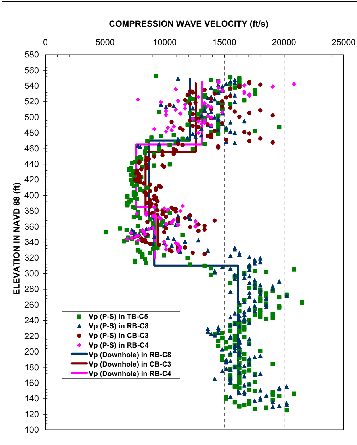
Figure 2.5.4-215 Compression wave velocity measurements using both P-S and Downhole methods in Borings TB-C5, RB-C8, CB-C3, and RB-C4
