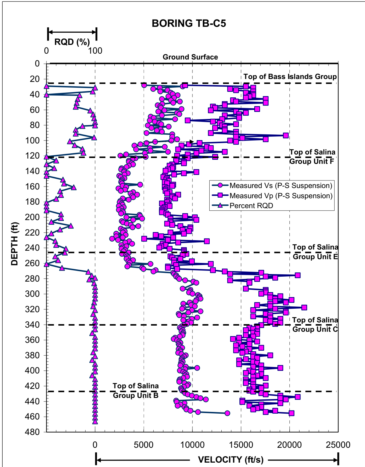
Figure 2.5.4-205 Comparison of measured V_s and V_p with RQD for Boring TB-C5
