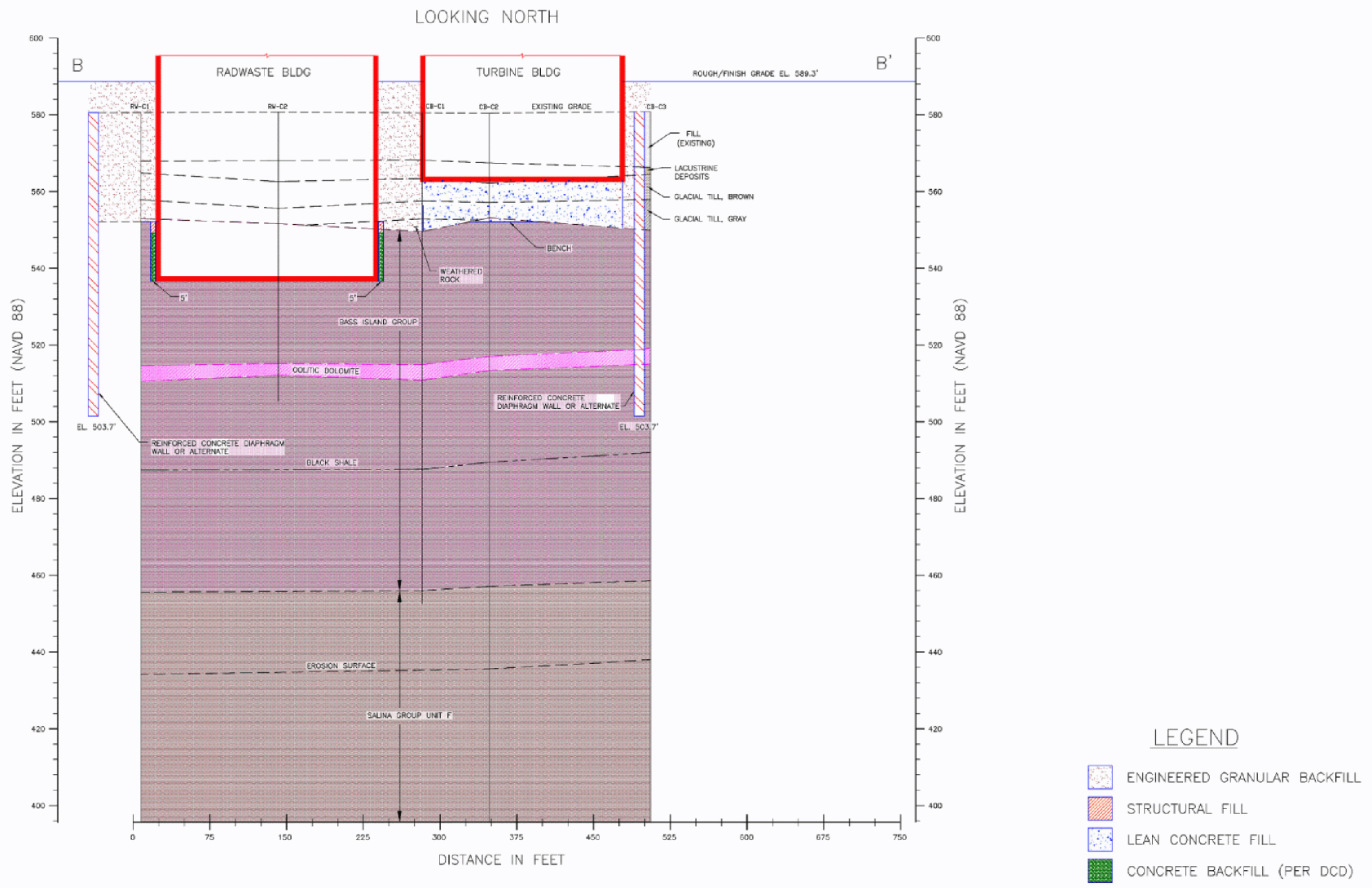
Figure 2.5.4-204 Excavation Cross Section B-B'
