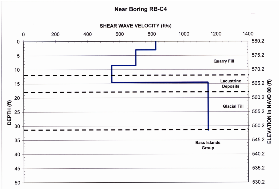
Figure 2.5.4-225 Measured shear and compression wave velocity profiles in the overburden using SASW method near Borings RB-C4 and RW-C1
