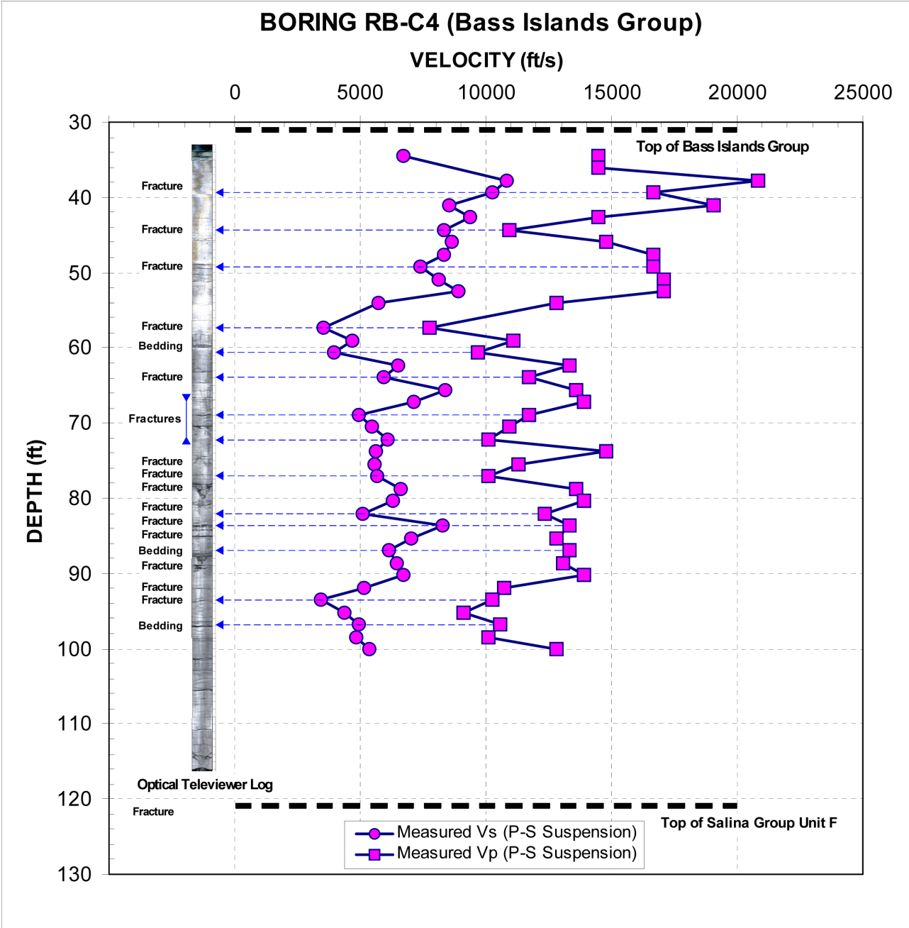
Figure 2.5.4-212 Influence of geologic features within Bass Islands Group on measured seismic wave velocities in Borehole RB-C4
