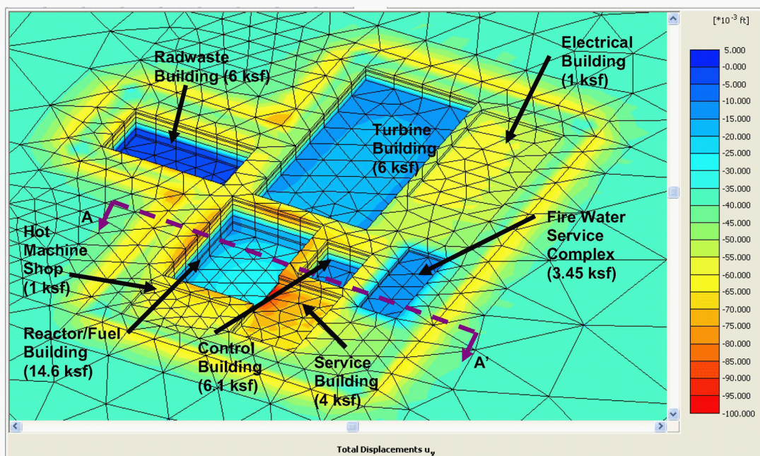
a) Plan View (Net Settlement)
