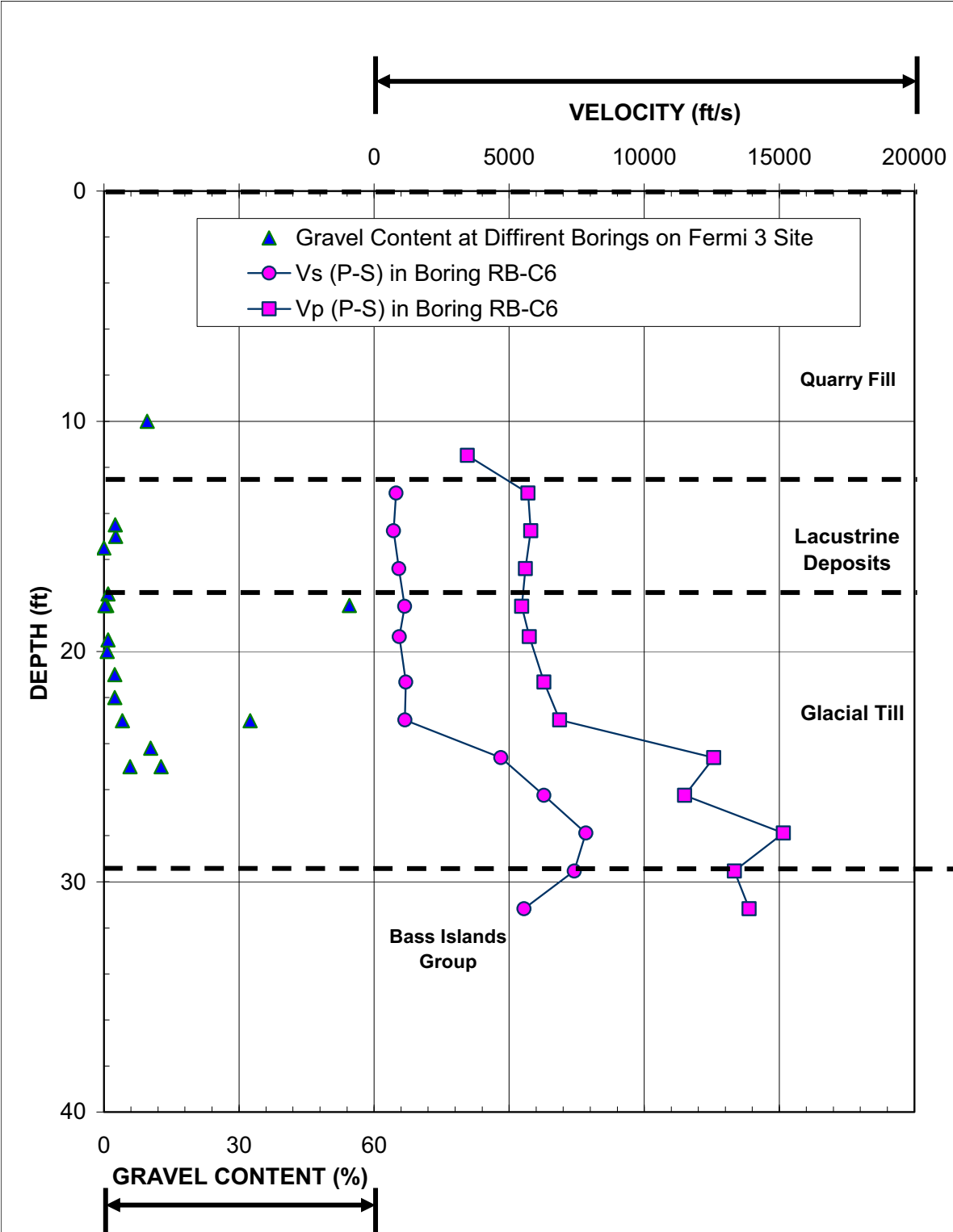
Figure 2.5.4-218 Comparison of measured shear and compression wave velocity profile using P-S suspension method in Boring RB-C6 with gravel content within overburden
