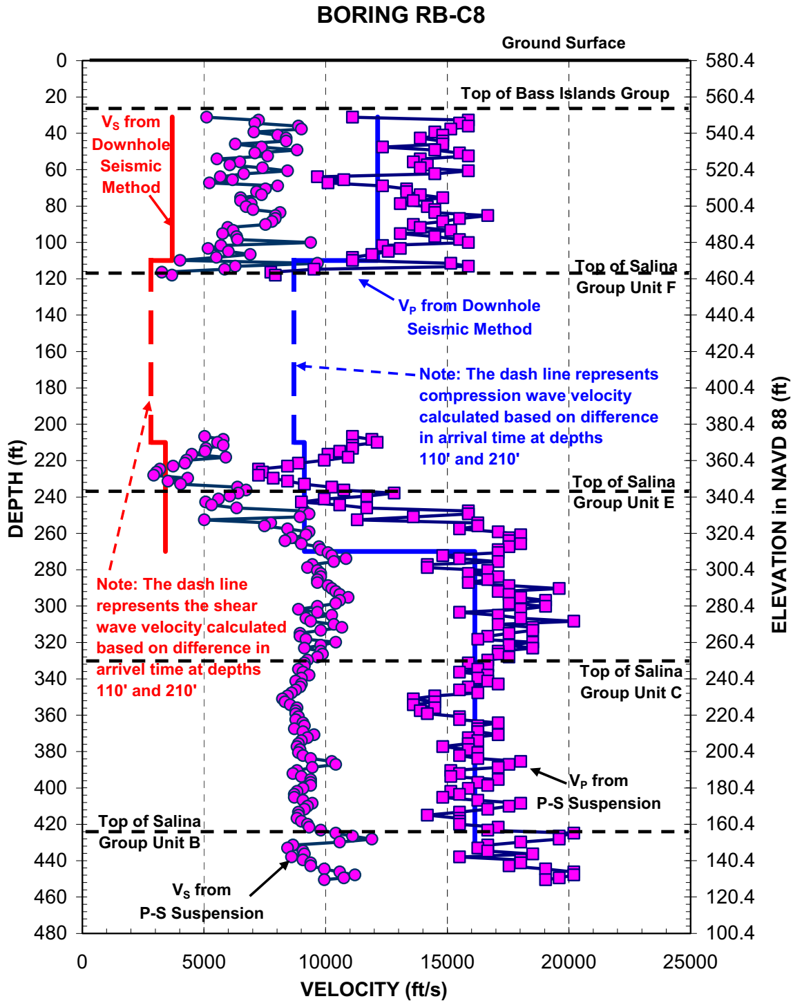
Figure 2.5.4-221 Measured shear and compression wave velocity profiles using P-S Suspension and Downhole Seismic methods in Boring RB-C8
