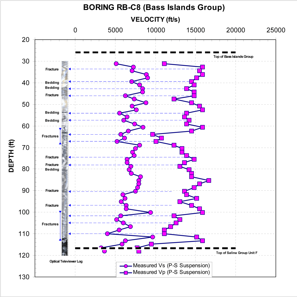
Figure 2.5.4-210 Influence of geologic features within Bass Islands Group on measured seismic wave velocities in Borehole RB-C8
