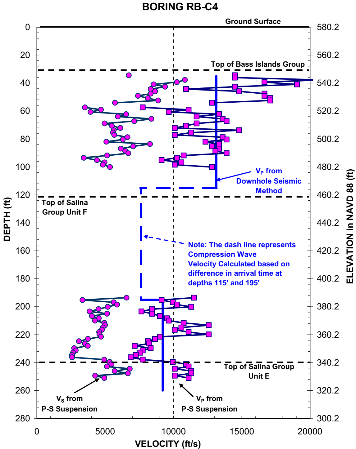
Figure 2.5.4-223 Measured shear and compression wave velocity profiles using P-S Suspension and Downhole Seismic methods in Boring RB-C4
