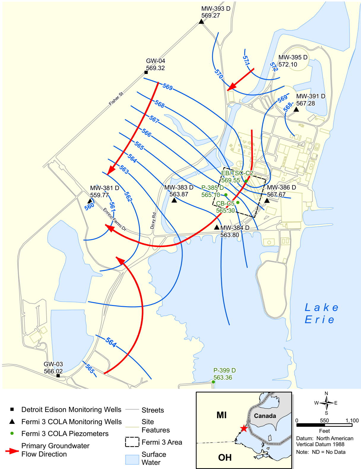
Figure 2.4-247 Bass Islands Aquifer Potentiometric Surface Map 09/28/2007-09/29/2007
