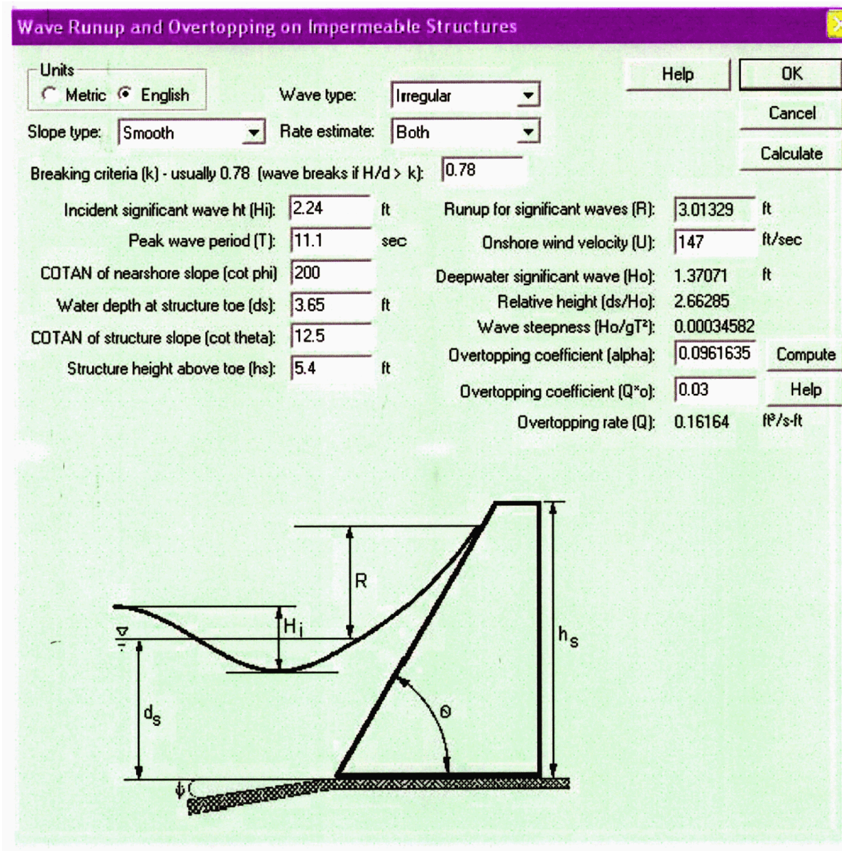
Figure 2.4-230 Wave Run-up and Overtopping on Impermeable Structures (Example)
