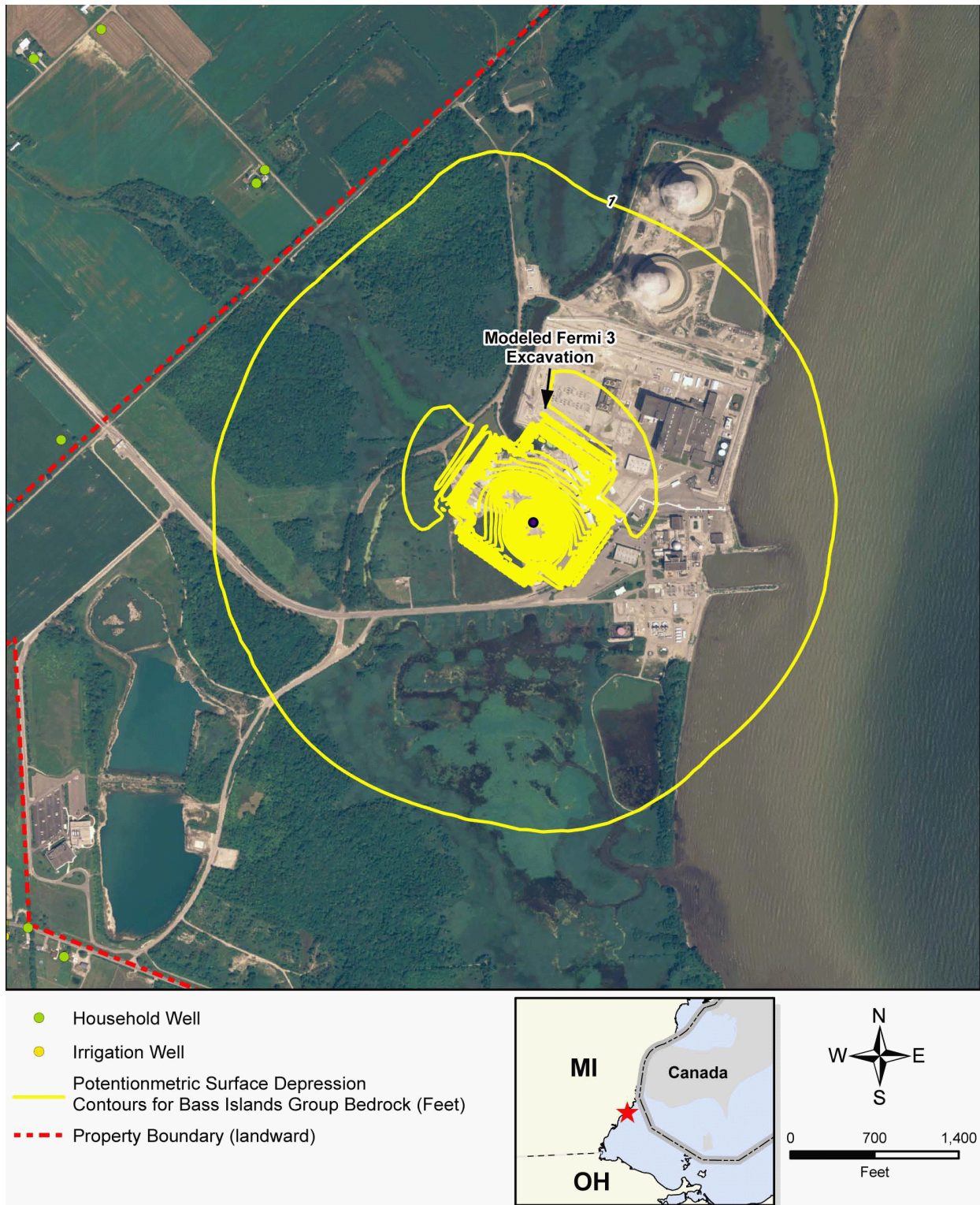
Figure 2.4-255 Dewatering Bass Islands Group: Drawdown Contours - Reinforced Diaphragm Concrete Wall With Grouted Base Combination
