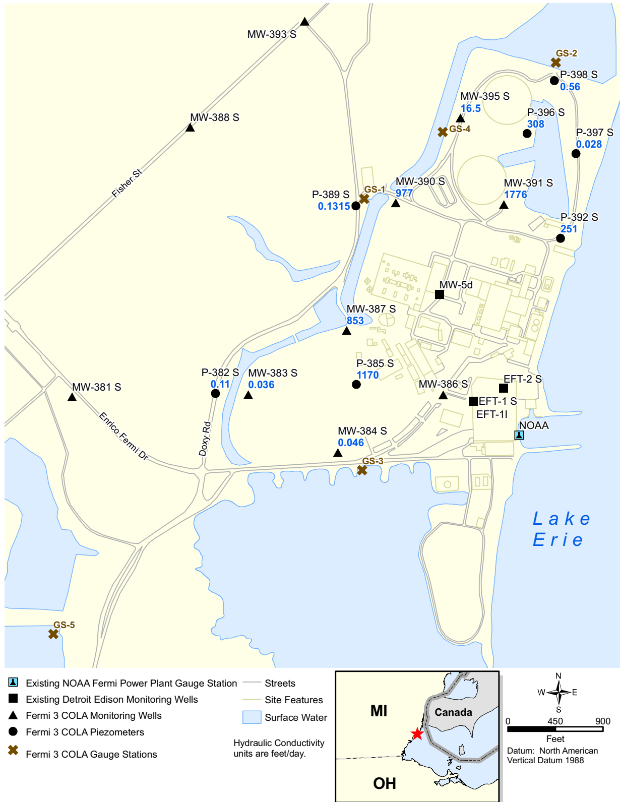
Figure 2.4-252 Fermi 3 Overburden Hydraulic Conductivity
