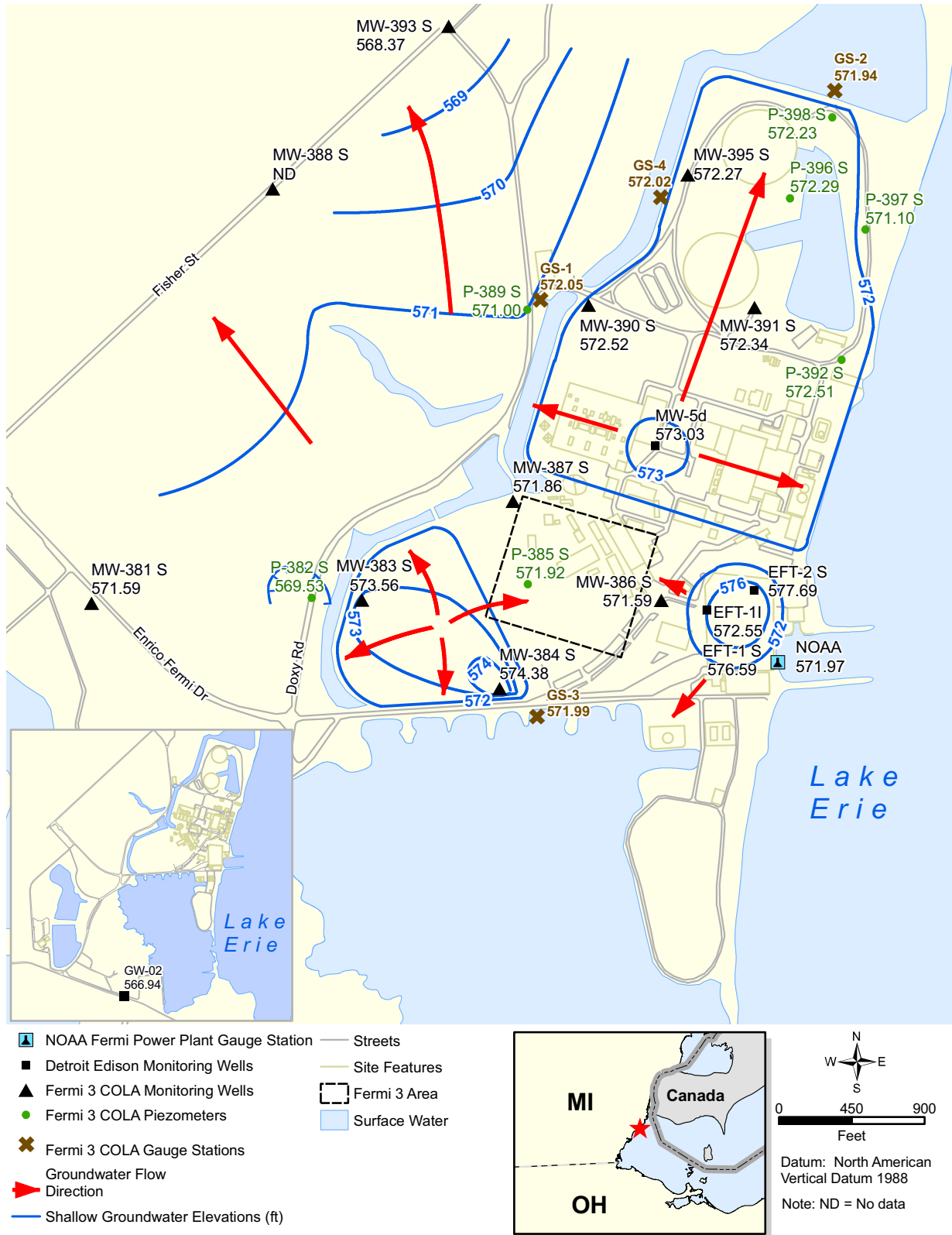
Figure 2.4-242 Overburden Water Table Map 06/29/2007
