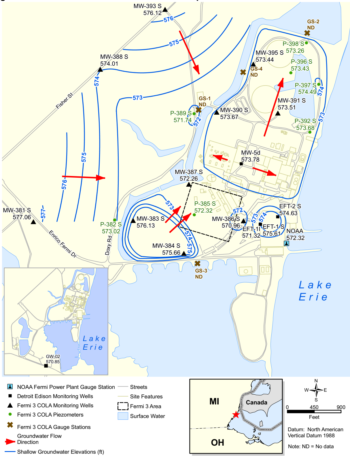
Figure 2.4-245 Overburden Water Table Map 03/29/2008
