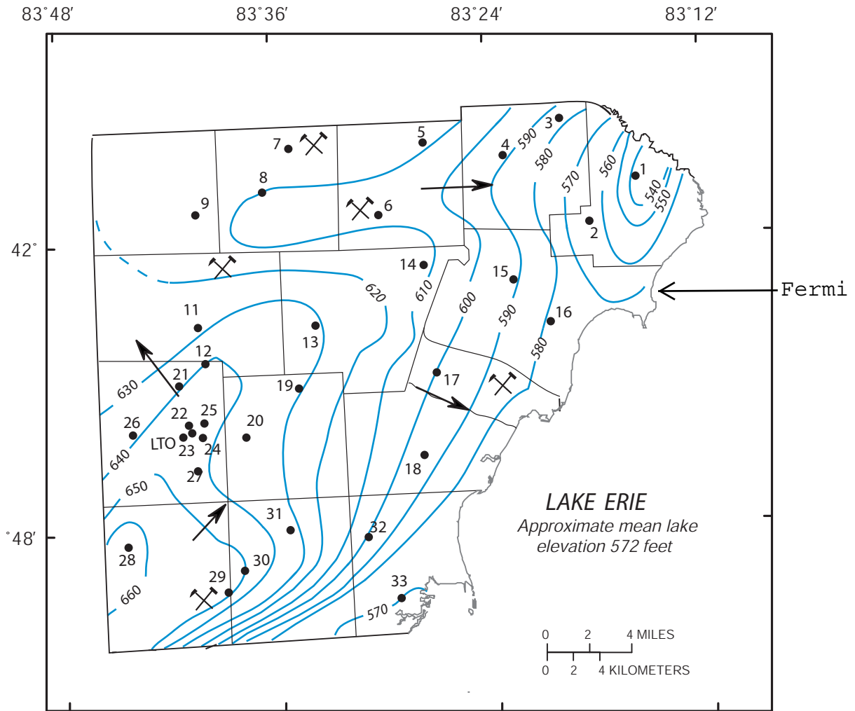
Figure 2.4-240 1993 Bedrock Aquifer Potentiometric Surface in Monroe County, MI
