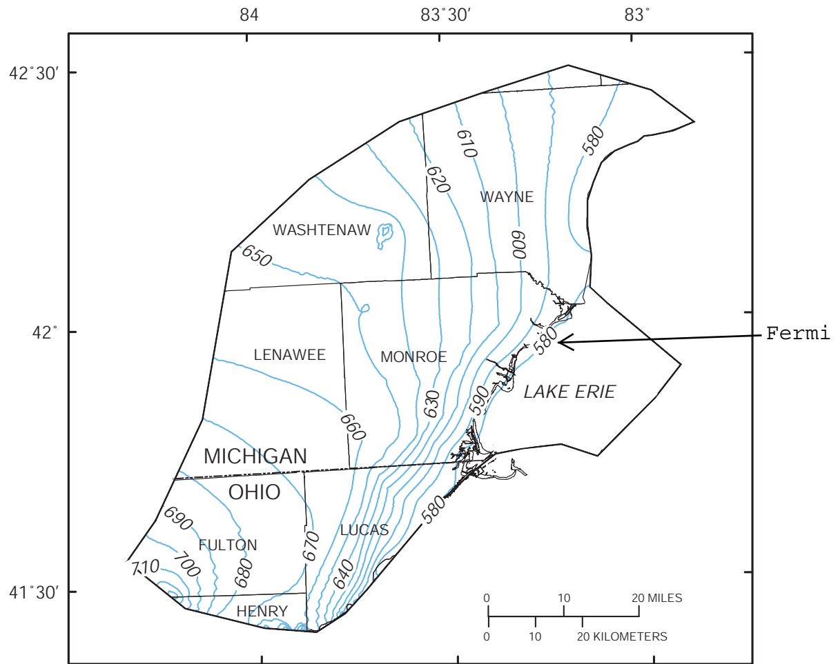
Figure 2.4-239 Simulated Pre-Development Water Levels in Bedrock Aquifer
