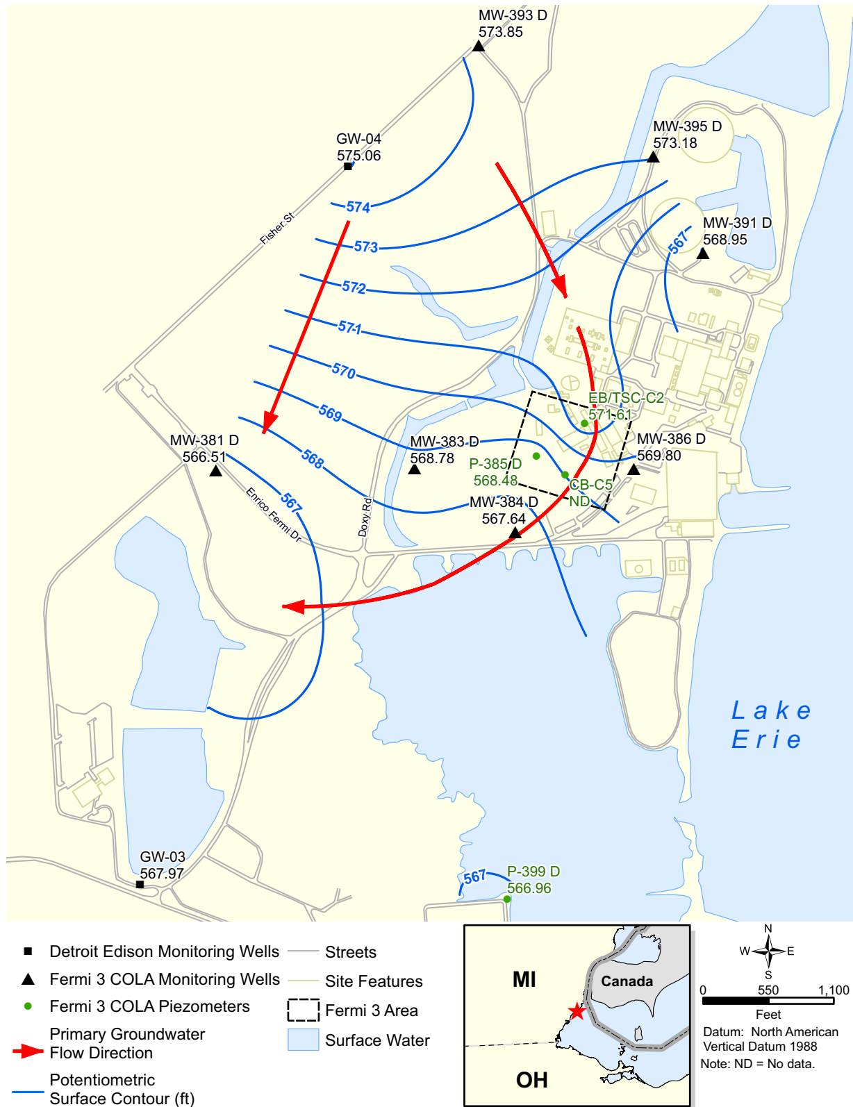
Figure 2.4-249 Bass Islands Aquifer Potentiometric Surface Map 03/29/2008
