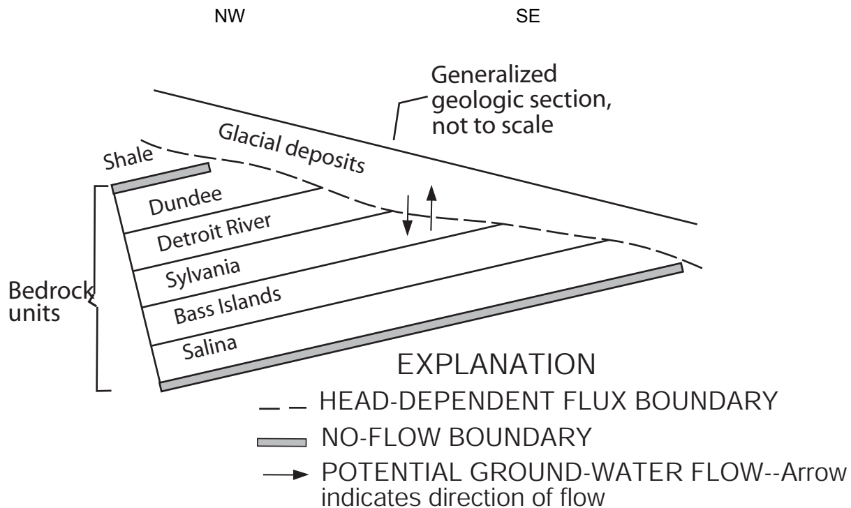
Figure 2.4-233 Conceptual Cross-Section of Regional Aquifer System
