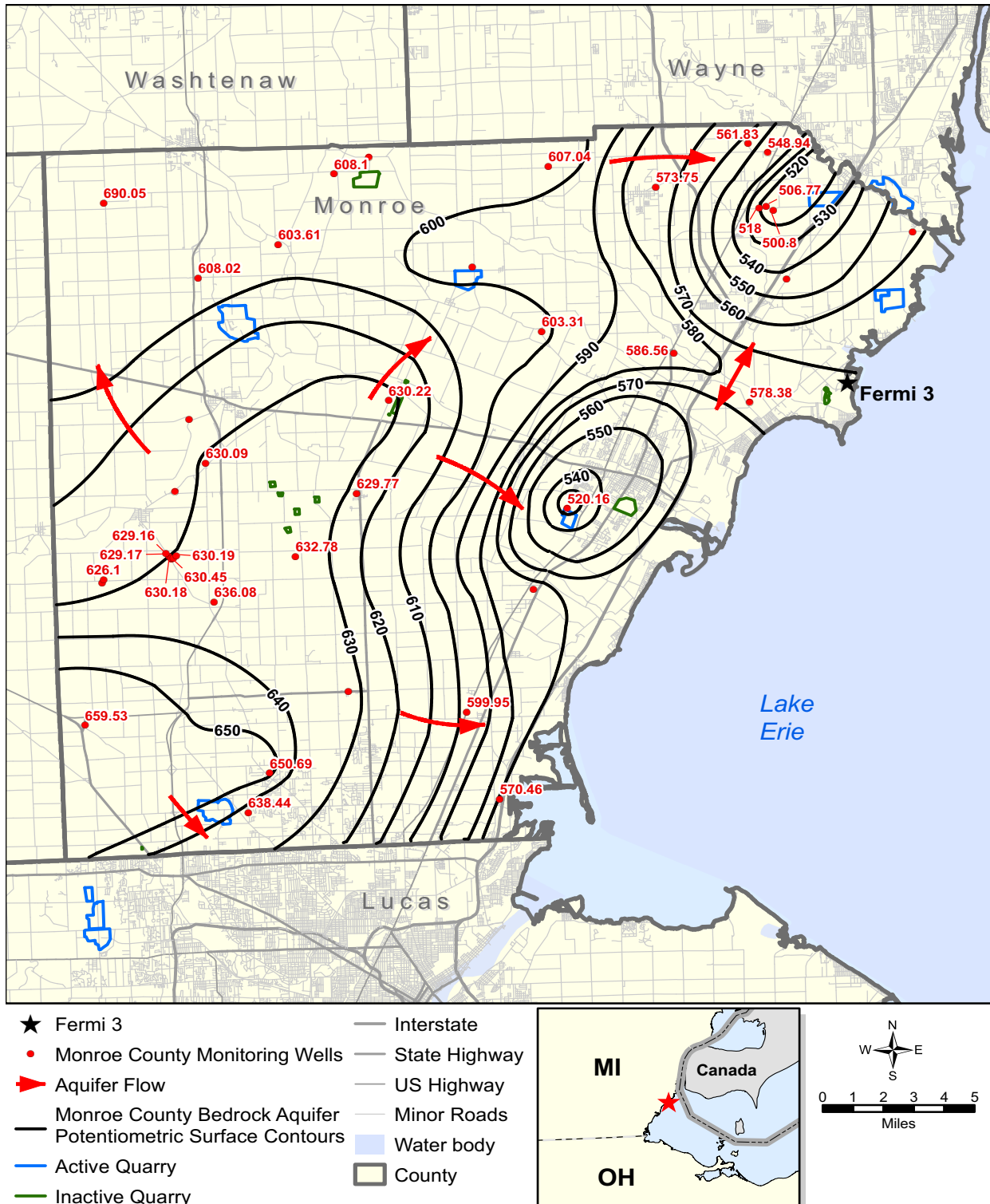
Figure 2.4-241 2008 Bedrock Aquifer Potentiometric Surface in Monroe County, MI
