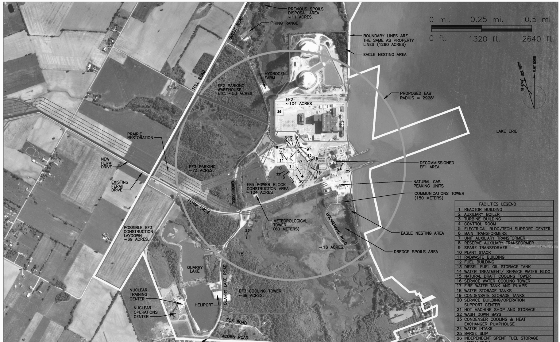
Figure 2.4-211 Fermi 3 Site Plan
