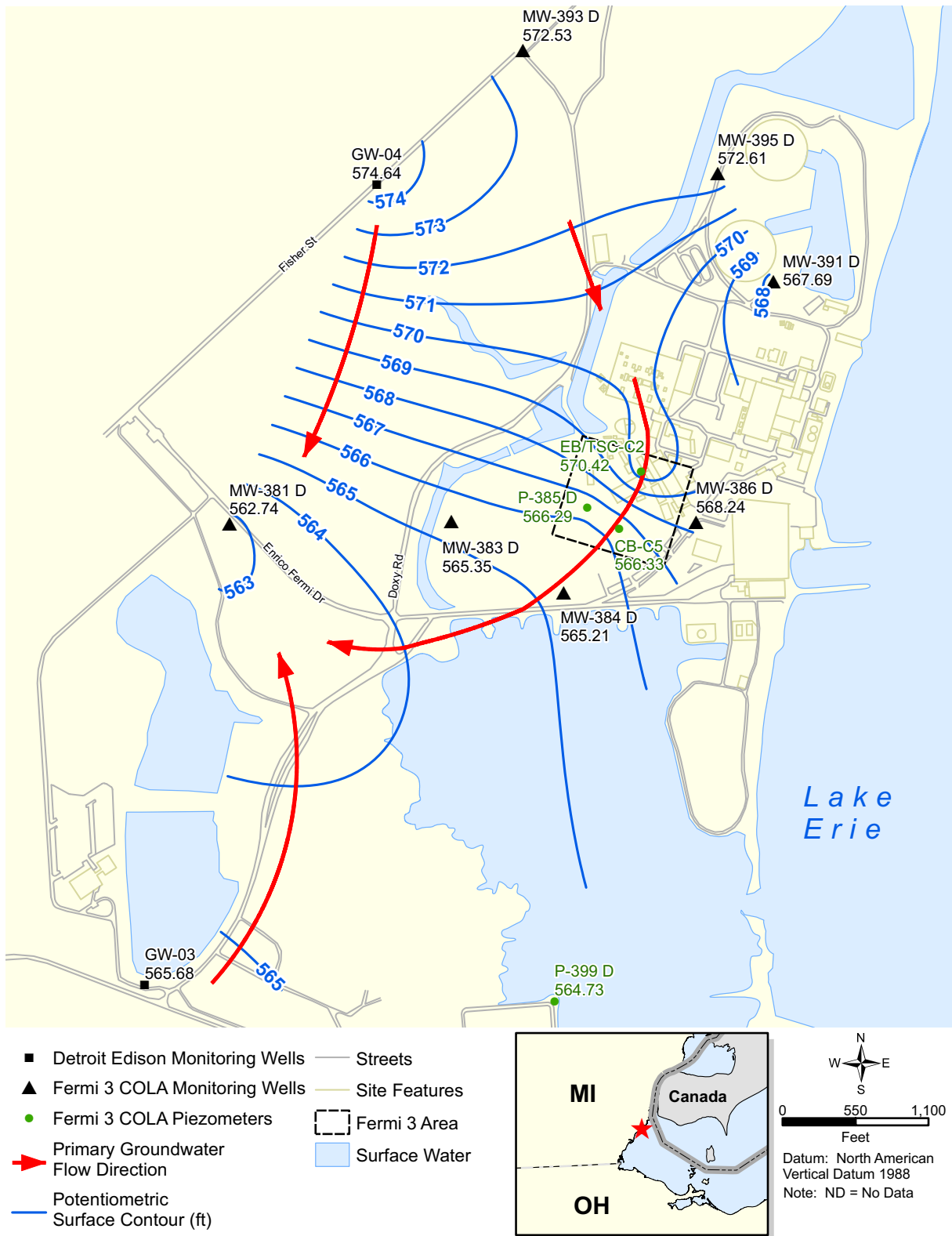
Figure 2.4-248 Bass Islands Aquifer Potentiometric Surface Map 12/29/2007
