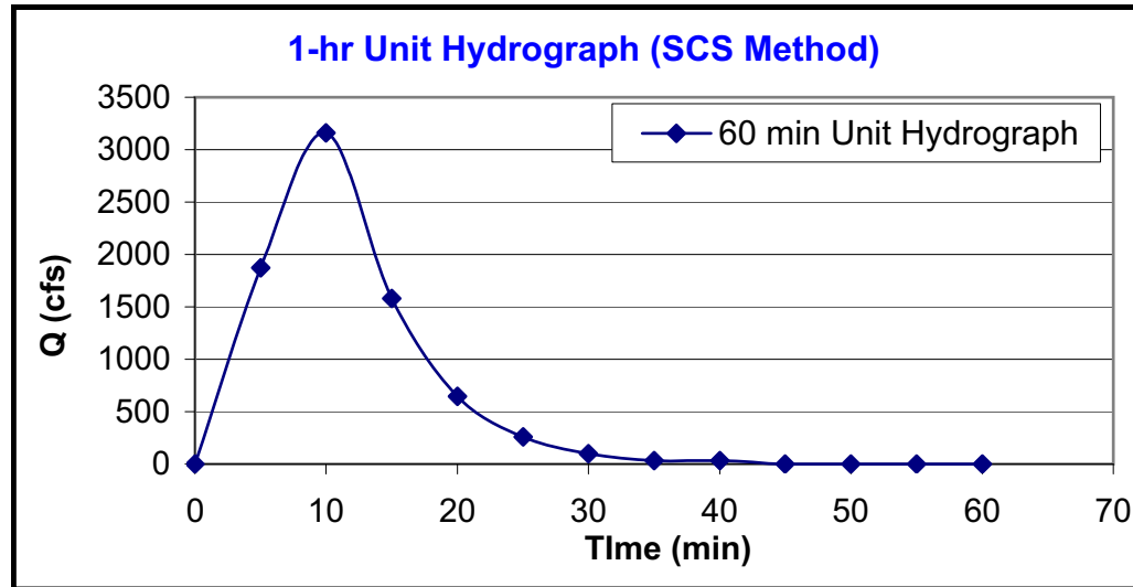
Figure 2.4-216 NRCS Dimensional Unit Hydrograph Q Results for One Square Mi PMF of Fermi 3
