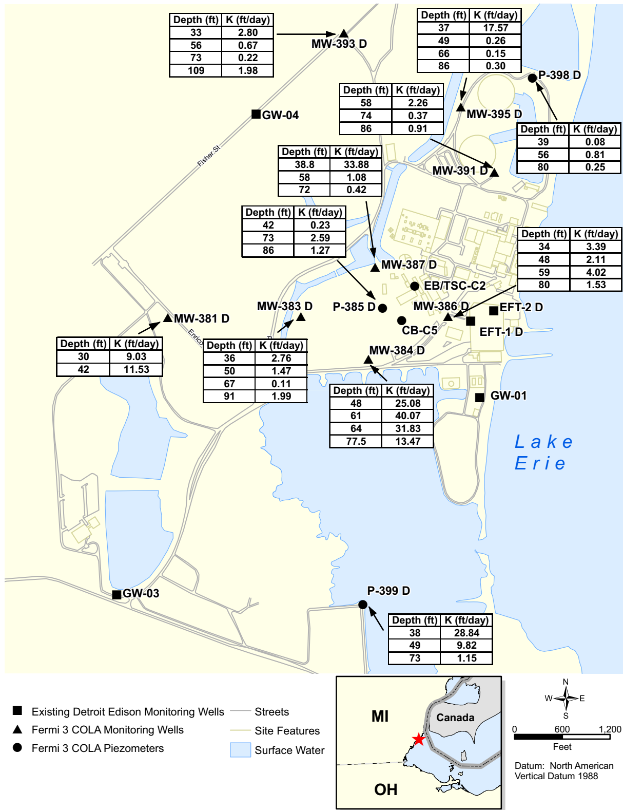
Figure 2.4-253 Fermi 3 Bedrock Hydraulic Conductivity
