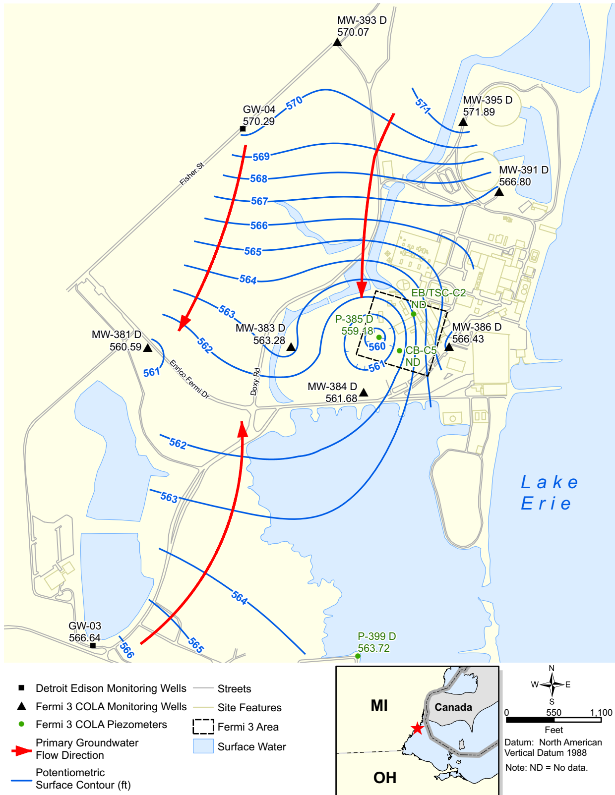
Figure 2.4-246 Bass Islands Aquifer Potentiometric Surface Map 06/29/2007
