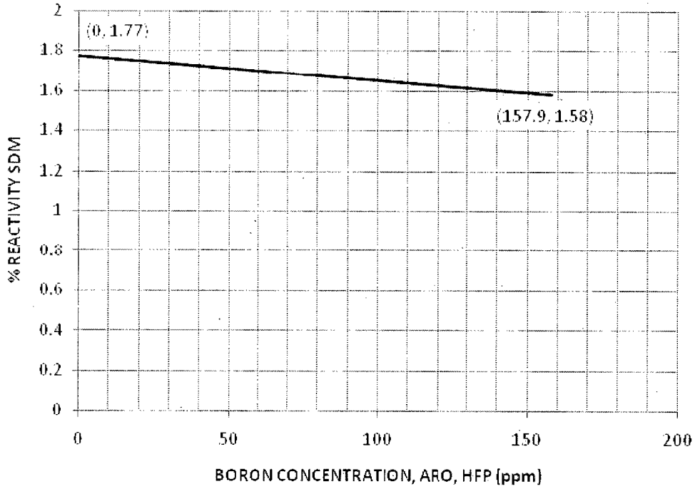
Figure 5.0, Shutdown Margin Versus Boron Concentration
