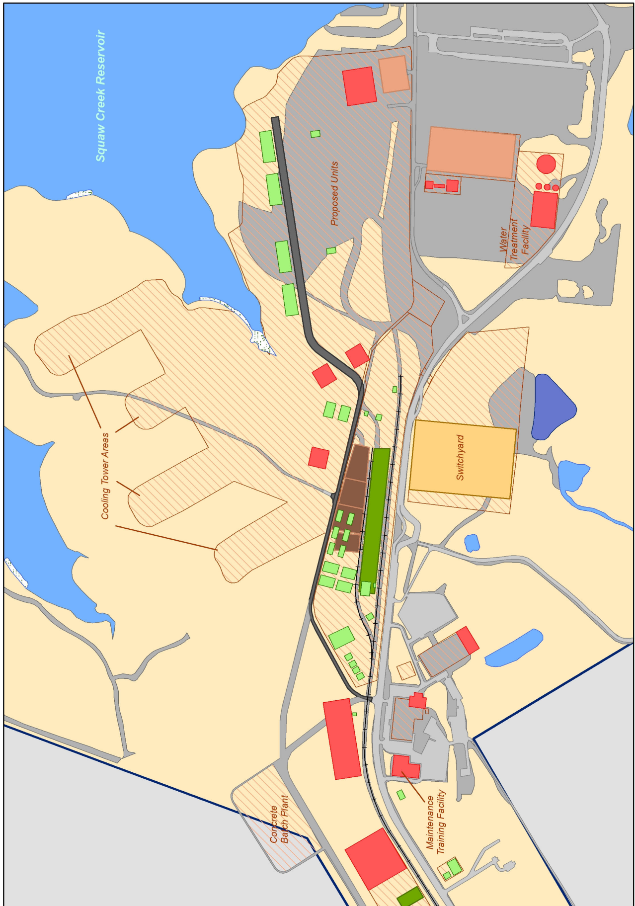
CPNPP Units 3 and 4 Construction Plan and Adjacent Water Bodies FIGURE 4.2-1
