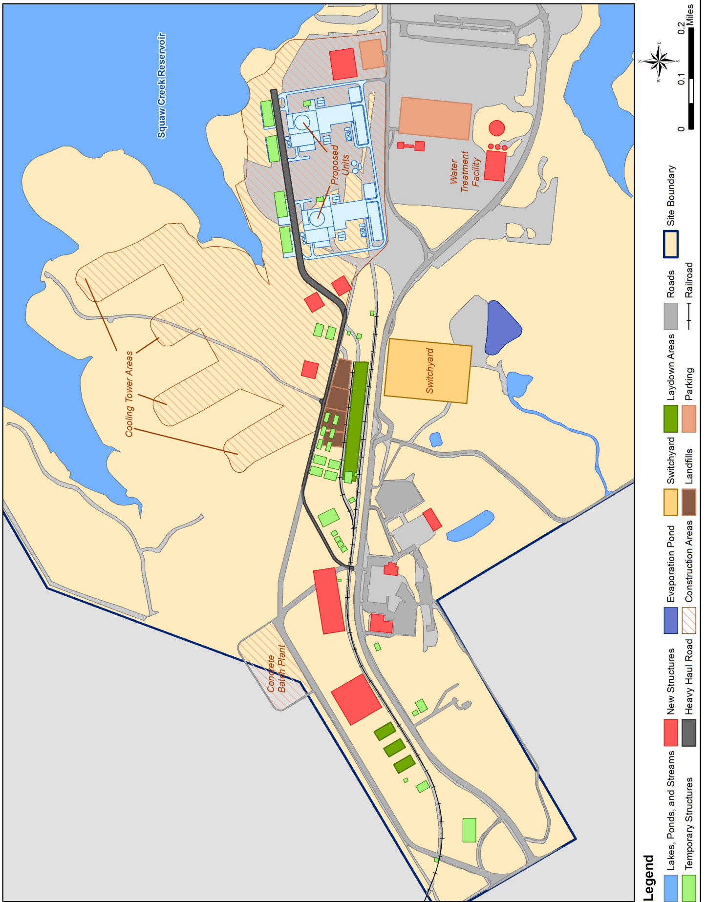
Detailed Site Plot plan with Construction Laydown Areas FIGURE 4.1-1 Rev 0
