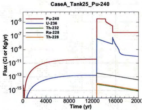
Figure A.1-829 - Flux Leaving Liner for CaseA Tank25 Pu-240
