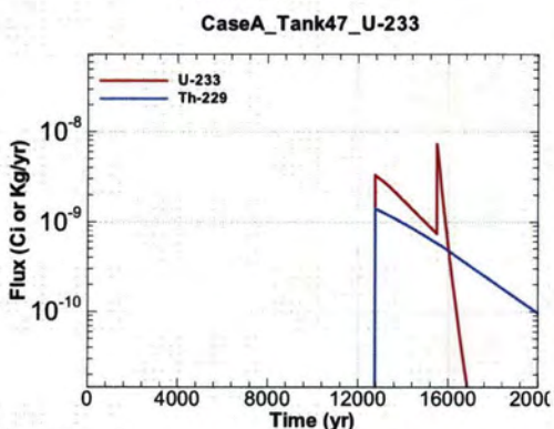
Figure A.1-1397 - Flux Leaving Liner for CaseA Tank47 U-233
