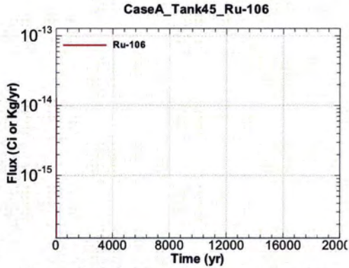
Figure A.1-1225 - Flux Leaving Liner for CaseA Tank45 Ru-106
