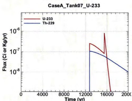
Figure A.1-539 - Flux Leaving Liner for CaseA Tank07 U-233
