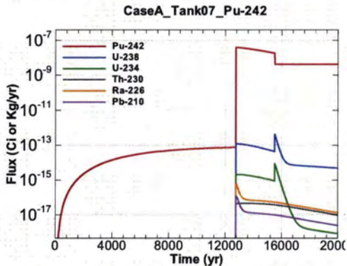
Figure A.1-519 - Flux Leaving Liner for CaseA Tank07 Pu-242
