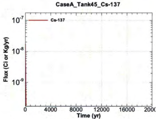
Figure A.1-1195 - Flux Leaving Liner for CaseA Tank45 Cs-137
