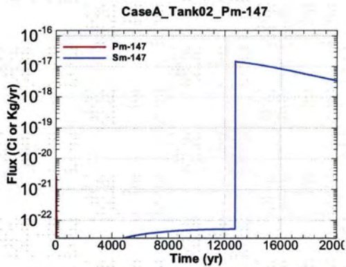
Figure A.1-123 - Flux Leaving Liner for CaseA Tank02 Pm-147
