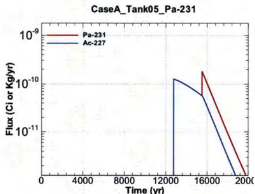
Figure A.1-355 - Flux Leaving Liner for CaseA Tank05 Pa-231
