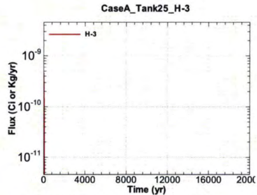
Figure A.1-812 - Flux Leaving Liner for CaseA Tank25 H-3
