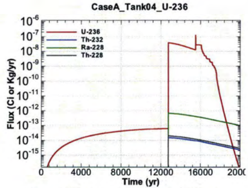
Figure A.1-308 - Flux Leaving Liner for CaseA Tank04 U-236
