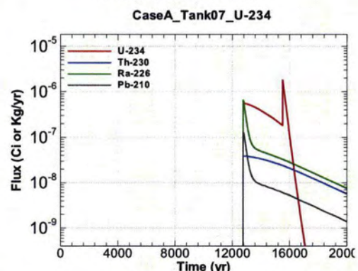
Figure A.1-540 - Flux Leaving Liner for CaseA Tank07 U-234
