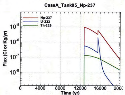
Figure A.1-354 - Flux Leaving Liner for CaseA Tank05 Np-237
