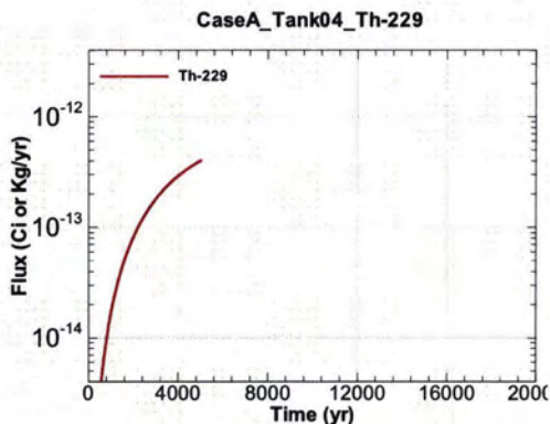
Figure A.1-301 - Flux Leaving Liner for CaseA Tank04 Th-229
