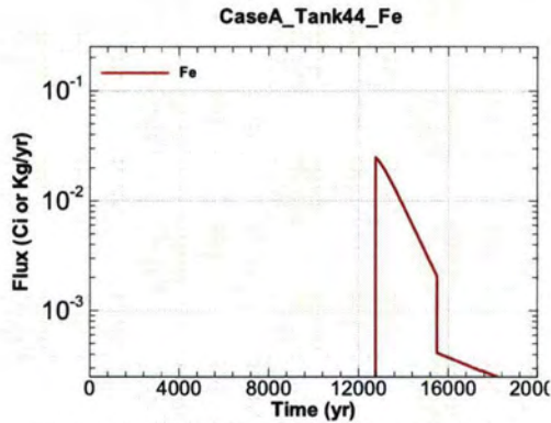
Figure A.1-1123 - Flux Leaving Liner for CaseA Tank44 Fe
