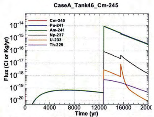
Figure A.1-1266 - Flux Leaving Liner for CaseA Tank46 Cm-245
