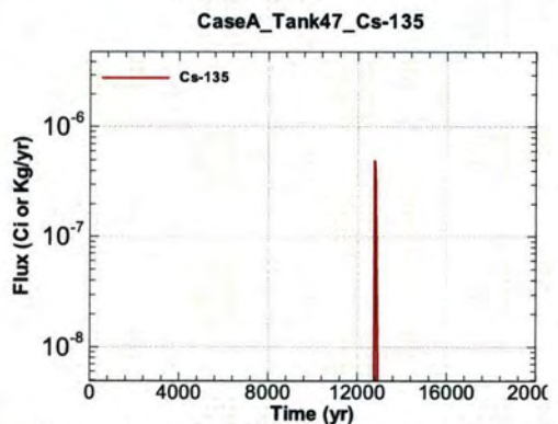
Figure A.1-1350 - Flux Leaving Liner for CaseA Tank47 Cs-135
