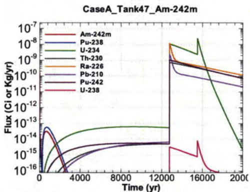
Figure A.1-1331 - Flux Leaving Liner for CaseA Tank47 Am-242m
