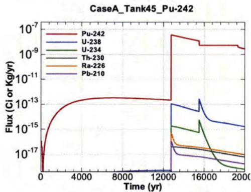
Figure A.1-1221 - Flux Leaving Liner for CaseA Tank45 Pu-242
