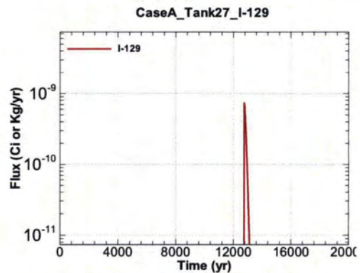
Figure A.1-970 - Flux Leaving Liner for CaseA Tank27 I-129
