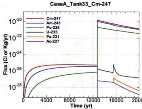
Figure A.1-643 - Flux Leaving Liner for CaseA Tank33 Cm-247
