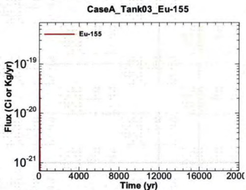
Figure A.1-185 - Flux Leaving Liner for CaseA Tank03 Eu-155
