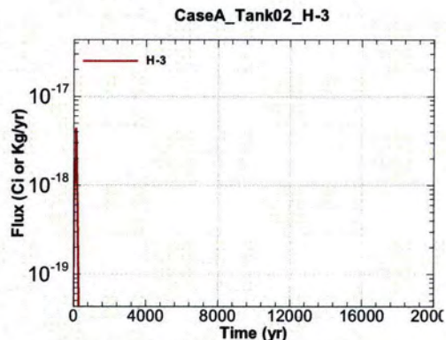
Figure A.1-110 - Flux Leaving Liner for CaseA Tank02 H-3
