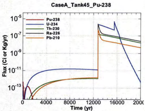
Figure A.1-1217 - Flux Leaving Liner for CaseA Tank45 Pu-238
