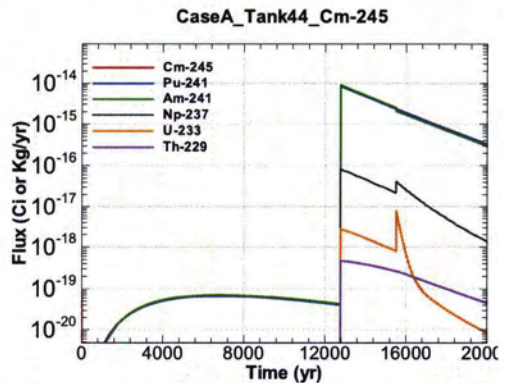
Figure A.1-1110 - Flux Leaving Liner for CaseA Tank44 Cm-245
