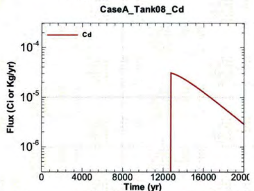
Figure A.1-558 - Flux Leaving Liner for CaseA Tank08 Cd
