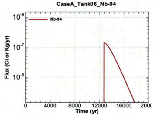
Figure A.1-428 - Flux Leaving Liner for CaseA Tank06 Nb-94
