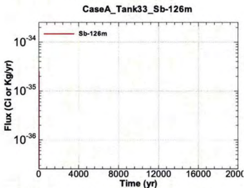
Figure A.1-683 - Flux Leaving Liner for CaseA Tank33 Sb-126m
