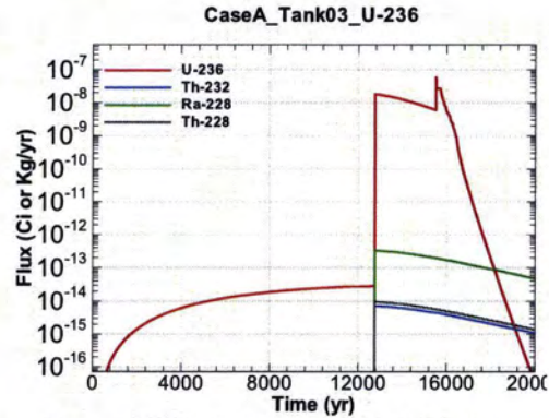
Figure A.1-230 - Flux Leaving Liner for CaseA Tank03 U-236
