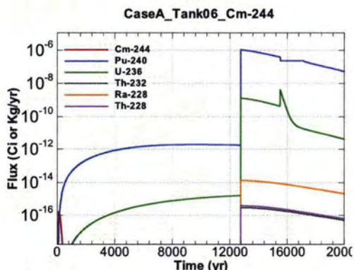
Figure A.1-407 - Flux Leaving Liner for CaseA Tank06 Cm-244
