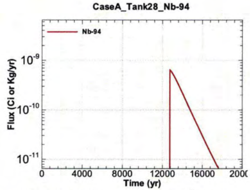
Figure A.1-1052 - Flux Leaving Liner for CaseA Tank28 Nb-94
