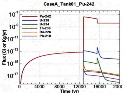
Figure A.1-51 - Flux Leaving Liner for CaseA Tank01 Pu-242
