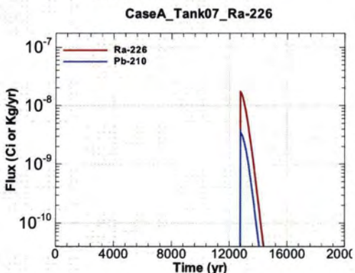
Figure A.1-521 - Flux Leaving Liner for CaseA Tank07 Ra-226
