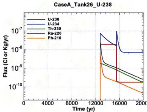
Figure A.1-933 - Flux Leaving Liner for CaseA Tank26 U-238
