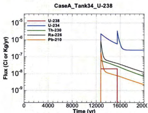
Figure A.1-777 - Flux Leaving Liner for CaseA Tank34 U-238
