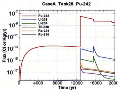
Figure A.1-1065 - Flux Leaving Liner for CaseA Tank28 Pu-242
