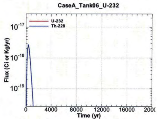
Figure A.1-460 - Flux Leaving Liner for CaseA Tank06 U-232
