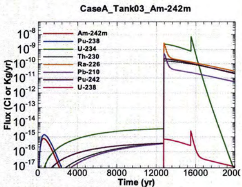
Figure A.1-161 - Flux Leaving Liner for CaseA Tank03 Am-242m
