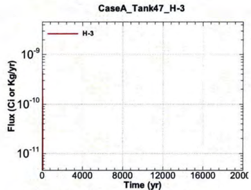
Figure A.1-1358 - Flux Leaving Liner for CaseA Tank47 H-3
