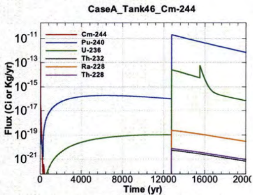
Figure A.1-1265 - Flux Leaving Liner for CaseA Tank46 Cm-244
