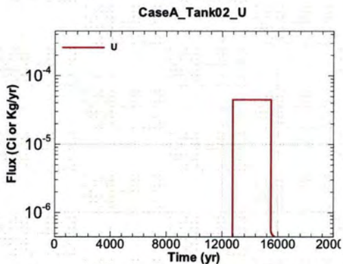
Figure A.1-147 - Flux Leaving Liner for CaseA Tank02 U
