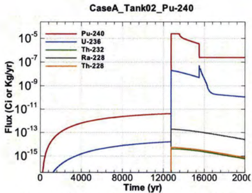
Figure A.1-127 - Flux Leaving Liner for CaseA Tank02 Pu-240
