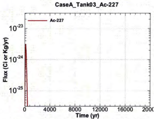
Figure A.1-157 - Flux Leaving Liner for CaseA Tank03 Ac-227
