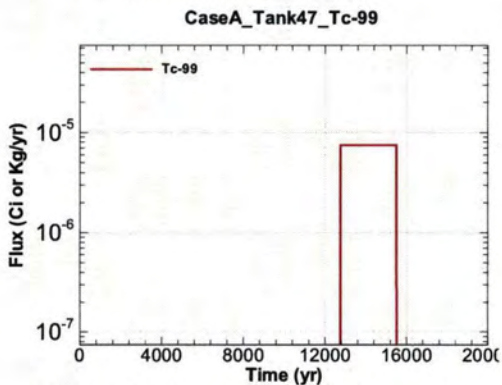
Figure A.1-1391 - Flux Leaving Liner for CaseA Tank47 Tc-99
