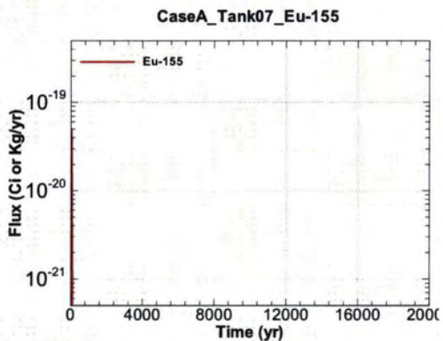
Figure A.1-497 - Flux Leaving Liner for CaseA Tank07 Eu-155
