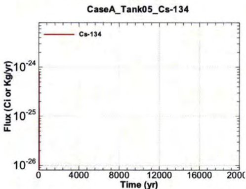
Figure A.1-335 - Flux Leaving Liner for CaseA Tank05 Cs-134
