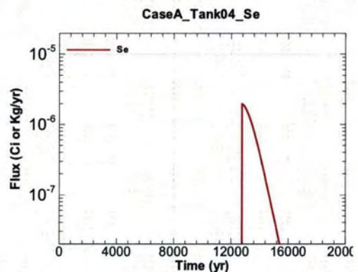
Figure A.1-294 - Flux Leaving Liner for CaseA Tank04 Se
