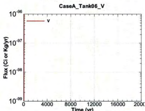
Figure A.1-466 - Flux Leaving Liner for CaseA Tank06 V
