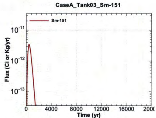
Figure A.1-218 - Flux Leaving Liner for CaseA Tank03 Sm-151
