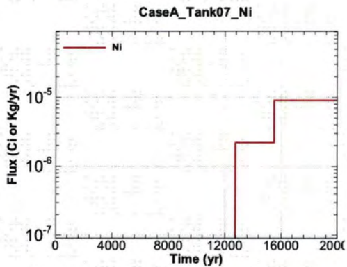
Figure A.1-507 - Flux Leaving Liner for CaseA Tank07 Ni
