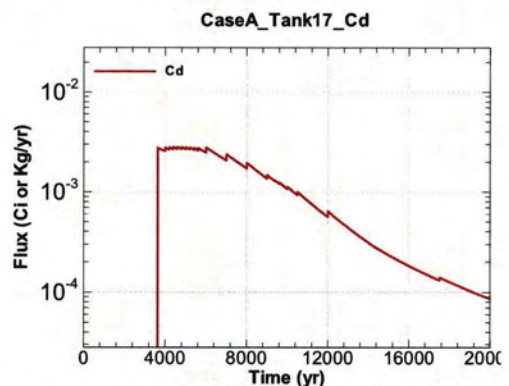
Figure A.1-1416 - Flux Leaving Liner for CaseA Tank17 Cd
