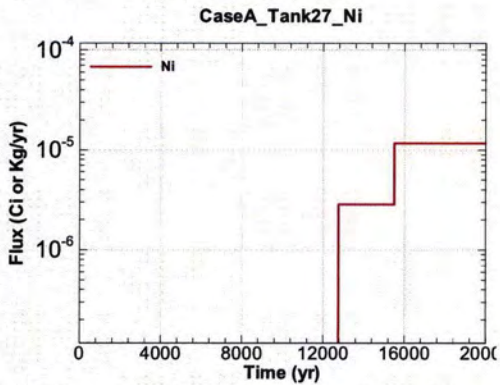
Figure A.1-975 - Flux Leaving Liner for CaseA Tank27 Ni
