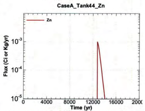
Figure A.1-1170 - Flux Leaving Liner for CaseA Tank44 Zn
