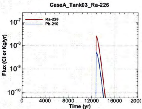
Figure A.1-209 - Flux Leaving Liner for CaseA Tank03 Ra-226
