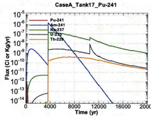
Figure A.1-1454 - Flux Leaving Liner for CaseA Tank17 Pu-241
