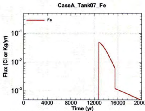
Figure A.1-499 - Flux Leaving Liner for CaseA Tank07 Fe
