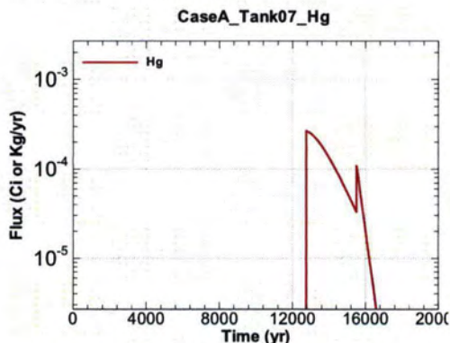
Figure A.1-501 - Flux Leaving Liner for CaseA Tank07 Hg
