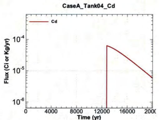
Figure A.1-246 - Flux Leaving Liner for CaseA Tank04 Cd
