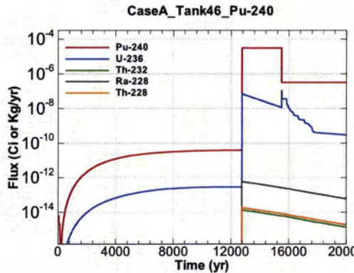
Figure A.1-1297 - Flux Leaving Liner for CaseA Tank46 Pu-240
