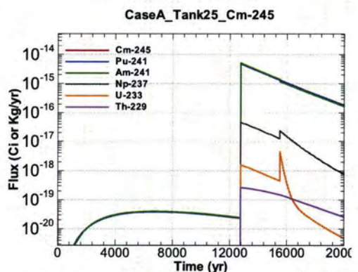
Figure A.1-798 - Flux Leaving Liner for CaseA Tank25 Cm-245
