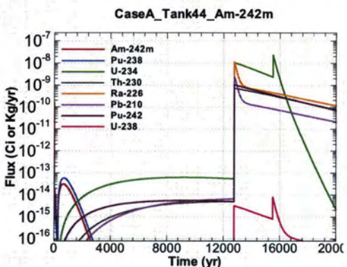
Figure A.1-1097 - Flux Leaving Liner for CaseA Tank44 Am-242m
