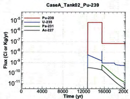
Figure A.1-126 - Flux Leaving Liner for CaseA Tank02 Pu-239
