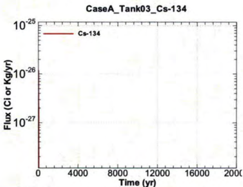
Figure A.1-179 - Flux Leaving Liner for CaseA Tank03 Cs-134
