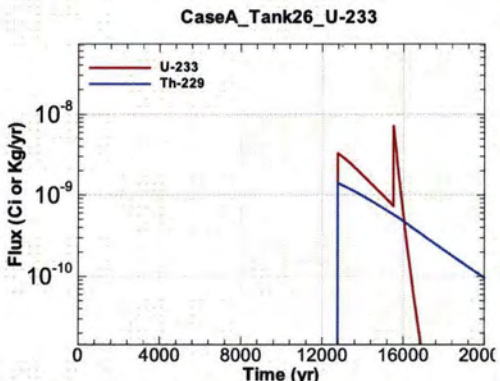
Figure A.1-929 - Flux Leaving Liner for CaseA Tank26 U-233
