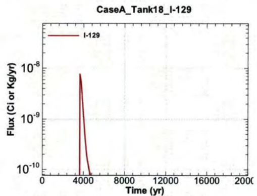
Figure A.1-1516 - Flux Leaving Liner for CaseA Tank18 I-129
