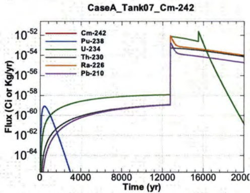
Figure A.1-483 - Flux Leaving Liner for CaseA Tank07 Cm-242
