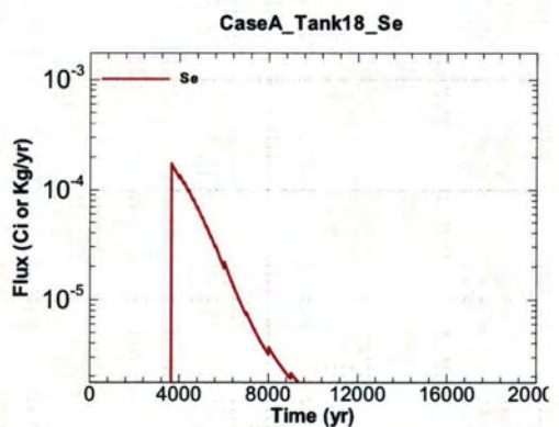
Figure A.1-1542 - Flux Leaving Liner for CaseA Tank18 Se
