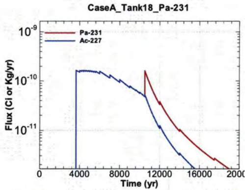
Figure A.1-1525 - Flux Leaving Liner for CaseA Tank18 Pa-231
