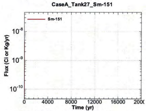
Figure A.1-998 - Flux Leaving Liner for CaseA Tank27 Sm-151
