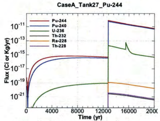
Figure A.1-988 - Flux Leaving Liner for CaseA Tank27 Pu-244
