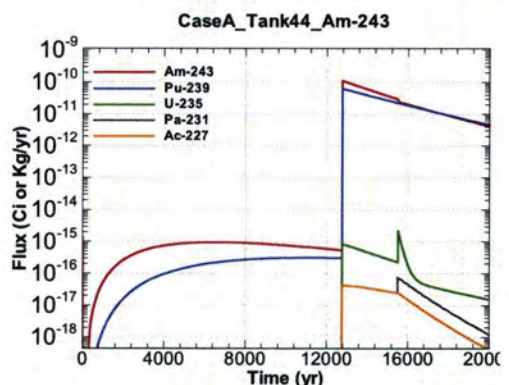
Figure A.1-1098 - Flux Leaving Liner for CaseA Tank44 Am-243
