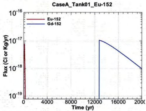
Figure A.1-27 - Flux Leaving Liner for CaseA Tank01 Eu-152
