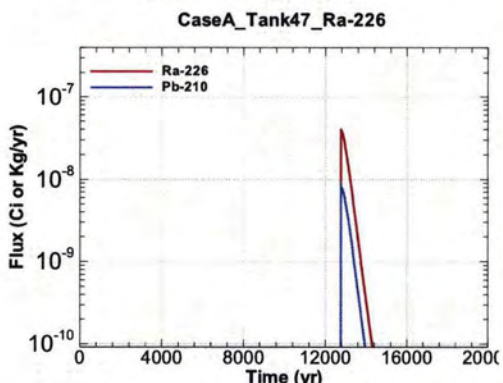
Figure A.1-1379 - Flux Leaving Liner for CaseA Tank47 Ra-226
