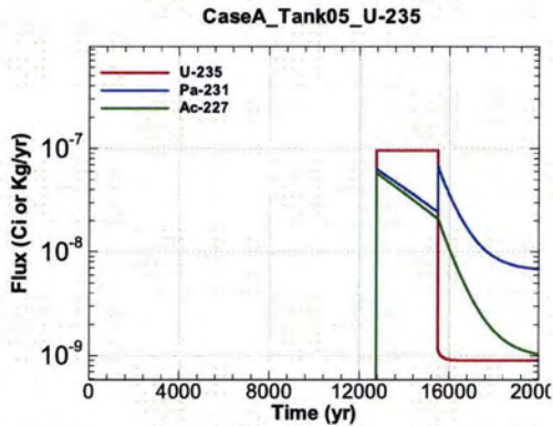
Figure A.1-385 - Flux Leaving Liner for CaseA Tank05 U-235
