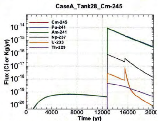
Figure A.1-1032 - Flux Leaving Liner for CaseA Tank28 Cm-245
