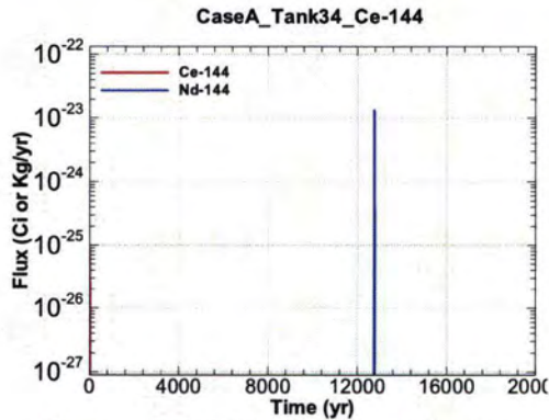
Figure A.1-715 - Flux Leaving Liner for CaseA Tank34 Ce-144
