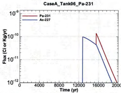
Figure A.1-433 - Flux Leaving Liner for CaseA Tank06 Pa-231
