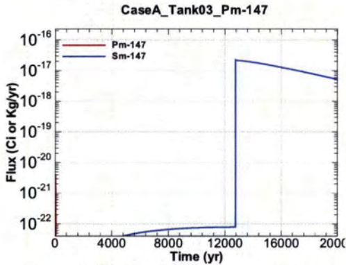
Figure A.1-201 - Flux Leaving Liner for CaseA Tank03 Pm-147
