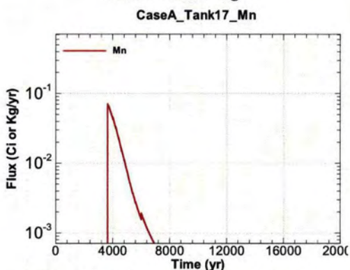
Figure A.1-1439 - Flux Leaving Liner for CaseA Tank17 Mn
