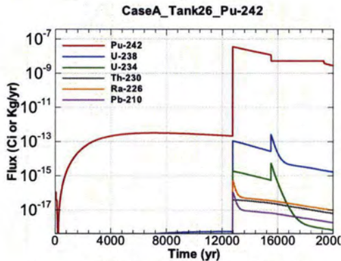
Figure A.1-909 - Flux Leaving Liner for CaseA Tank26 Pu-242
