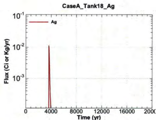
Figure A.1-1484 - Flux Leaving Liner for CaseA Tank18 Ag
