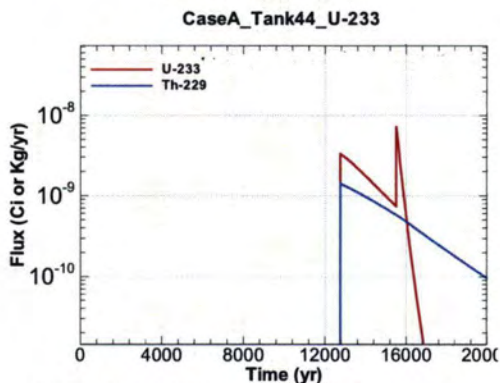
Figure A.1-1163 - Flux Leaving Liner for CaseA Tank44 U-233
