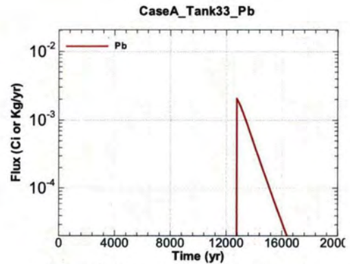
Figure A.1-668 - Flux Leaving Liner for CaseA Tank33 Pb
