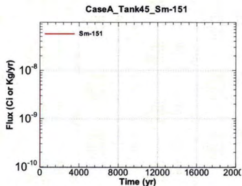
Figure A.1-1232 - Flux Leaving Liner for CaseA Tank45 Sm-151
