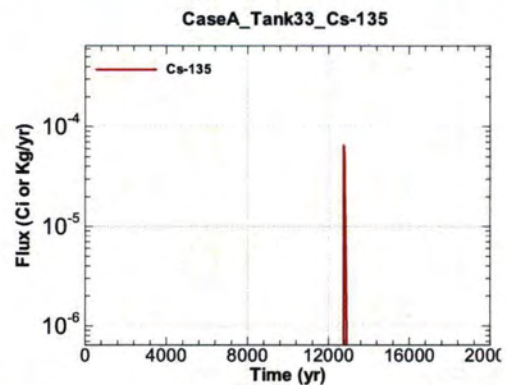
Figure A.1-648 - Flux Leaving Liner for CaseA Tank33 Cs-135
