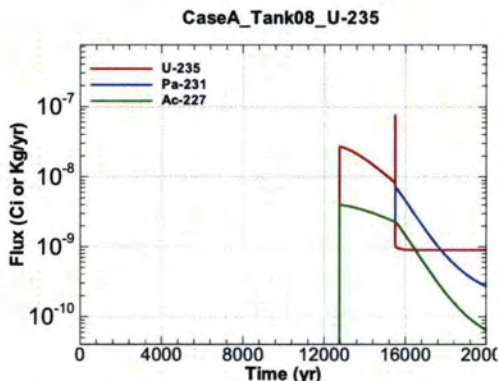
Figure A.1-619 - Flux Leaving Liner for CaseA Tank08 U-235
