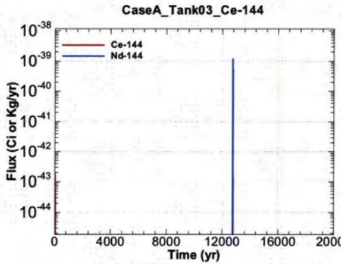
Figure A.1-169 - Flux Leaving Liner for CaseA Tank03 Ce-144
