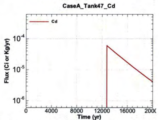
Figure A.1-1338 - Flux Leaving Liner for CaseA Tank47 Cd
