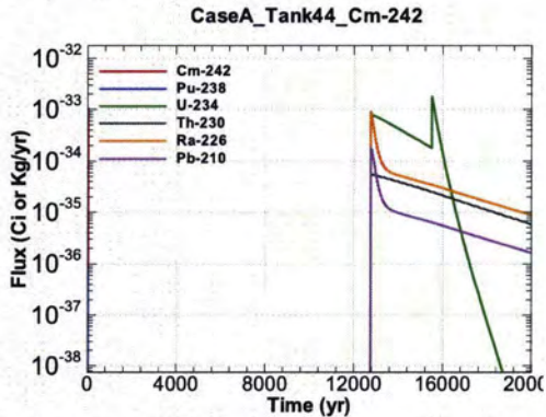
Figure A.1-1107 - Flux Leaving Liner for CaseA Tank44 Cm-242
