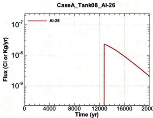
Figure A.1-549 - Flux Leaving Liner for CaseA Tank08 Al-26
