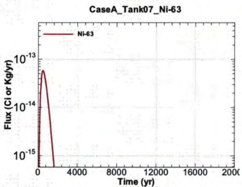
Figure A.1-509 - Flux Leaving Liner for CaseA Tank07 Ni-63
