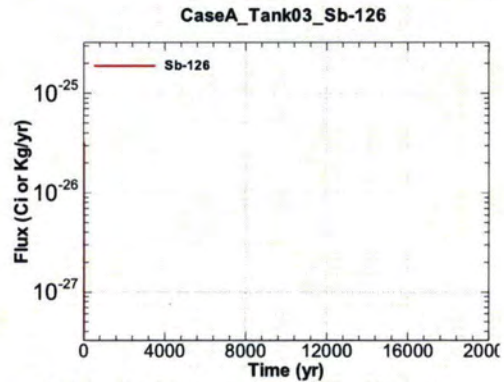
Figure A.1-214 - Flux Leaving Liner for CaseA Tank03 Sb-126
