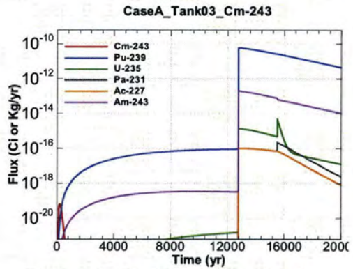
Figure A.1-172 - Flux Leaving Liner for CaseA Tank03 Cm-243
