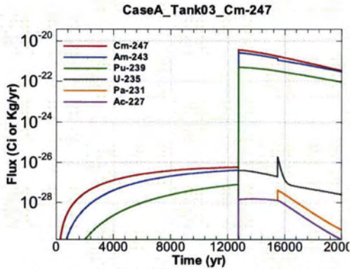
Figure A.1-175 - Flux Leaving Liner for CaseA Tank03 Cm-247
