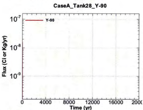
Figure A.1-1091 - Flux Leaving Liner for CaseA Tank28 Y-90
