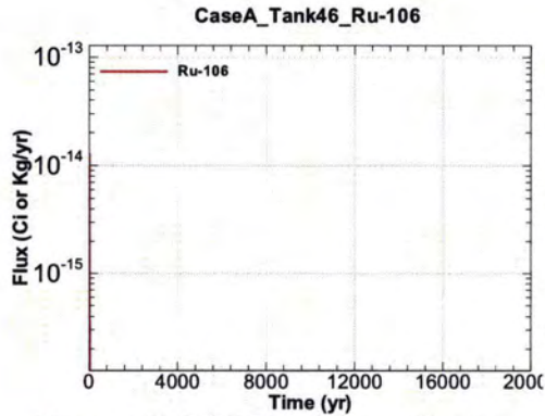
Figure A.1-1303 - Flux Leaving Liner for CaseA Tank46 Ru-106
