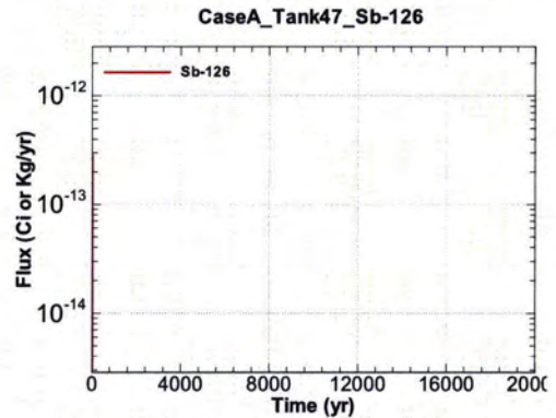
Figure A.1-1384 - Flux Leaving Liner for CaseA Tank47 Sb-126
