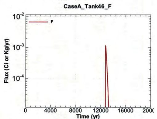
Figure A.1-1278 - Flux Leaving Liner for CaseA Tank46 F
