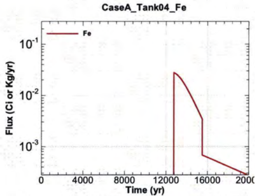
Figure A.1-265 - Flux Leaving Liner for CaseA Tank04 Fe
