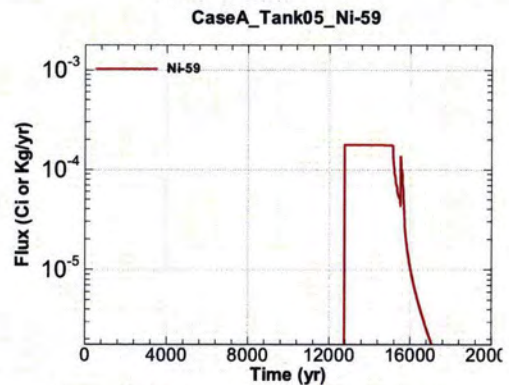
Figure A.1-352 - Flux Leaving Liner for CaseA Tank05 Ni-59
