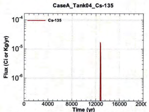
Figure A.1-258 - Flux Leaving Liner for CaseA Tank04 Cs-135
