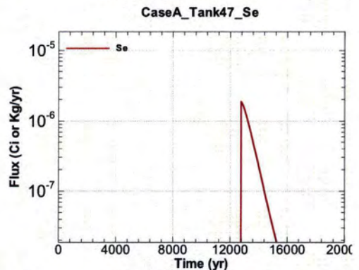
Figure A.1-1386 - Flux Leaving Liner for CaseA Tank47 Se
