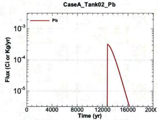
Figure A.1-122 - Flux Leaving Liner for CaseA Tank02 Pb
