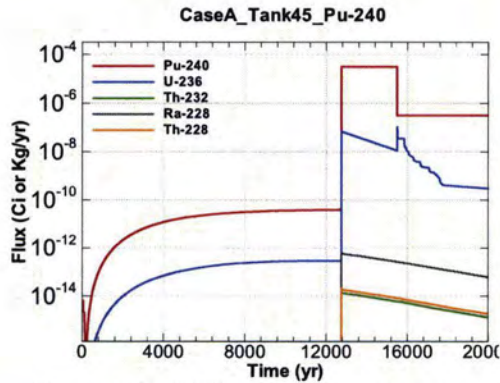
Figure A.1-1219 - Flux Leaving Liner for CaseA Tank45 Pu-240
