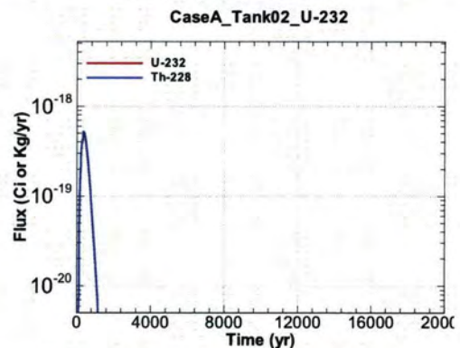
Figure A.1-148 - Flux Leaving Liner for CaseA Tank02 U-232
