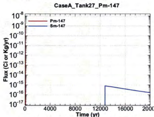
Figure A.1-981 - Flux Leaving Liner for CaseA Tank27 Pm-147
