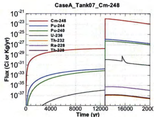
Figure A.1-488 - Flux Leaving Liner for CaseA Tank07 Cm-248
