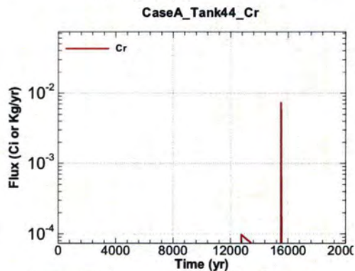
Figure A.1-1114 - Flux Leaving Liner for CaseA Tank44 Cr
