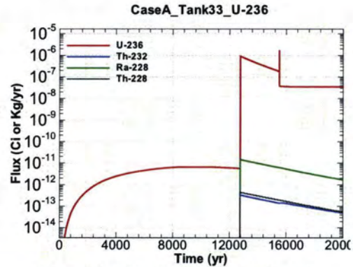
Figure A.1-698 - Flux Leaving Liner for CaseA Tank33 U-236
