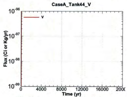
Figure A.1-1168 - Flux Leaving Liner for CaseA Tank44 V
