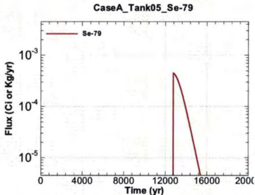
Figure A.1-373 - Flux Leaving Liner for CaseA Tank05 Se-79
