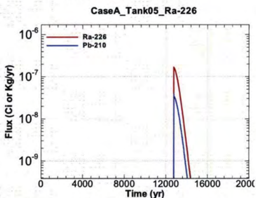
Figure A.1-365 - Flux Leaving Liner for CaseA Tank05 Ra-226
