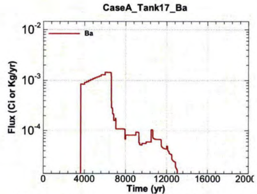
Figure A.1-1412 - Flux Leaving Liner for CaseA Tank17 Ba
