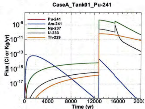
Figure A.1-50 - Flux Leaving Liner for CaseA Tank01 Pu-241
