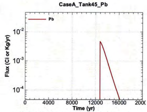
Figure A.1-1214 - Flux Leaving Liner for CaseA Tank45 Pb
