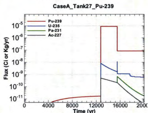
Figure A.1-984 - Flux Leaving Liner for CaseA Tank27 Pu-239
