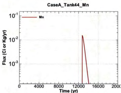
Figure A.1-1127 - Flux Leaving Liner for CaseA Tank44 Mn
