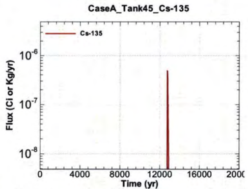
Figure A.1-1194 - Flux Leaving Liner for CaseA Tank45 Cs-135
