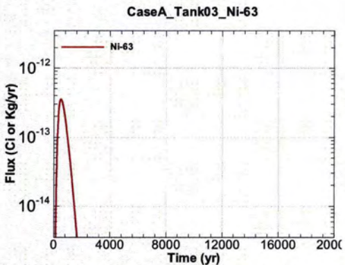
Figure A.1-197 - Flux Leaving Liner for CaseA Tank03 Ni-63
