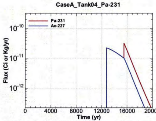
Figure A.1-277 - Flux Leaving Liner for CaseA Tank04 Pa-231
