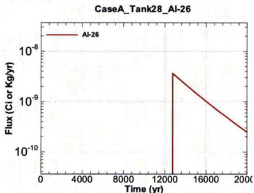
Figure A.1-1017 - Flux Leaving Liner for CaseA Tank28 Al-26
