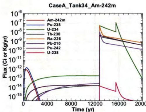
Figure A.1-707 - Flux Leaving Liner for CaseA Tank34 Am-242m
