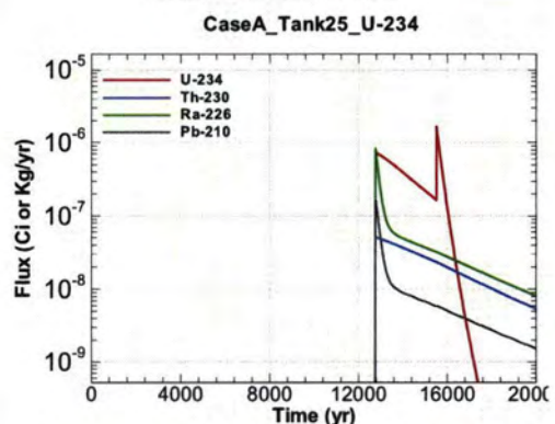
Figure A.1-852 - Flux Leaving Liner for CaseA Tank25 U-234
