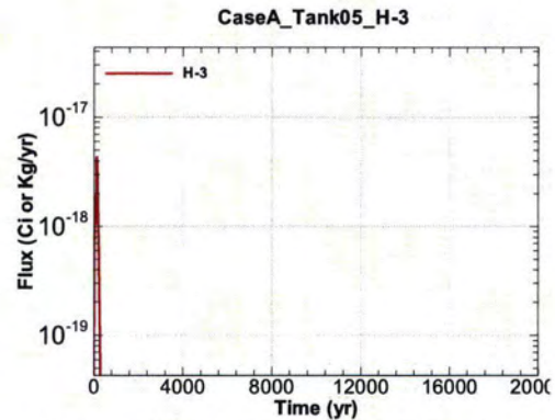
Figure A.1-344 - Flux Leaving Liner for CaseA Tank05 H-3
