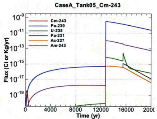
Figure A.1-328 - Flux Leaving Liner for CaseA Tank05 Cm-243
