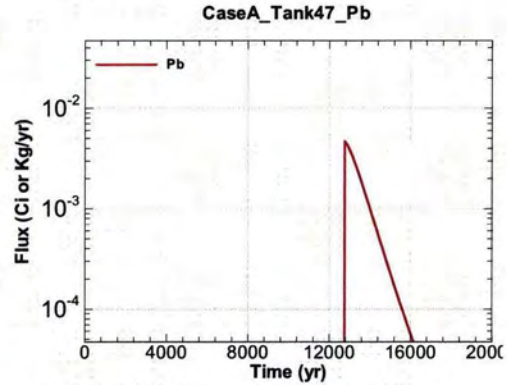
Figure A.1-1370 - Flux Leaving Liner for CaseA Tank47 Pb
