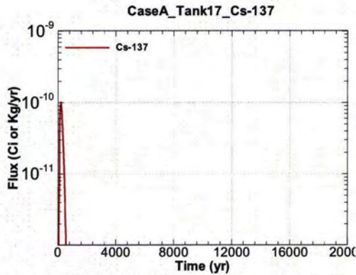
Figure A.1-1429 - Flux Leaving Liner for CaseA Tank17 Cs-137
