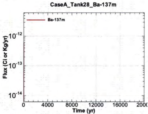
Figure A.1-1023 - Flux Leaving Liner for CaseA Tank28 Ba-137m
