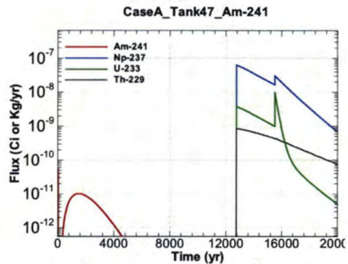
Figure A.1-1330 - Flux Leaving Liner for CaseA Tank47 Am-241
