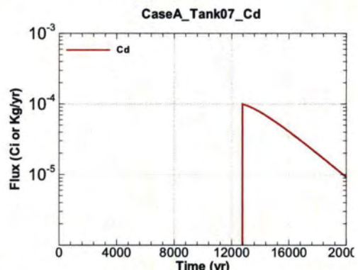
Figure A.1-480 - Flux Leaving Liner for CaseA Tank07 Cd
