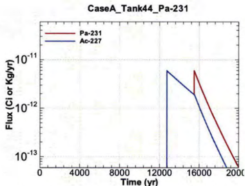
Figure A.1-1135 - Flux Leaving Liner for CaseA Tank44 Pa-231
