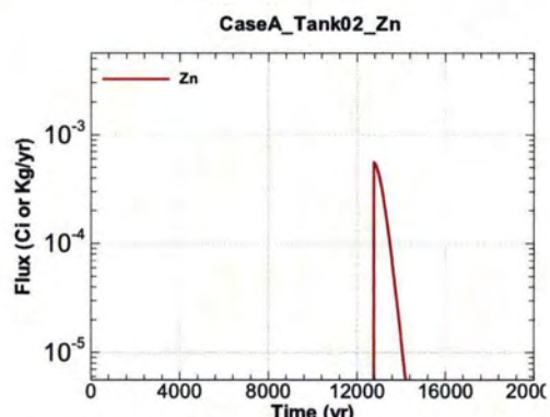
Figure A.1-156 - Flux Leaving Liner for CaseA Tank02 Zn
