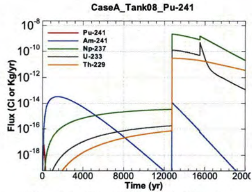
Figure A.1-596 - Flux Leaving Liner for CaseA Tank08 Pu-241
