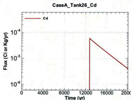
Figure A.1-870 - Flux Leaving Liner for CaseA Tank26 Cd
