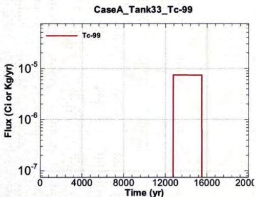
Figure A.1-689 - Flux Leaving Liner for CaseA Tank33 Tc-99
