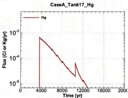
Figure A.1-1437 - Flux Leaving Liner for CaseA Tank17 Hg
