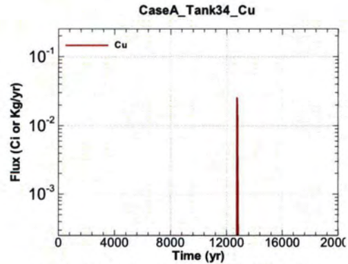
Figure A.1-728 - Flux Leaving Liner for CaseA Tank34 Cu
