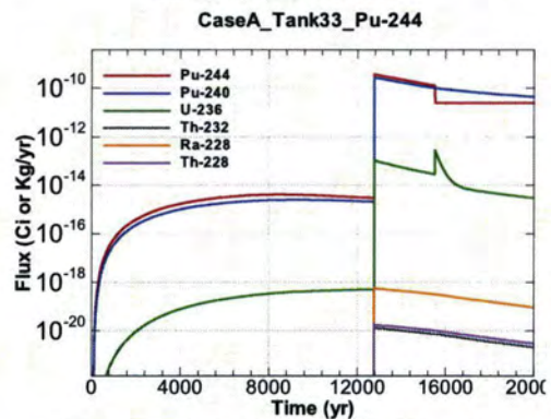
Figure A.1-676 - Flux Leaving Liner for CaseA Tank33 Pu-244
