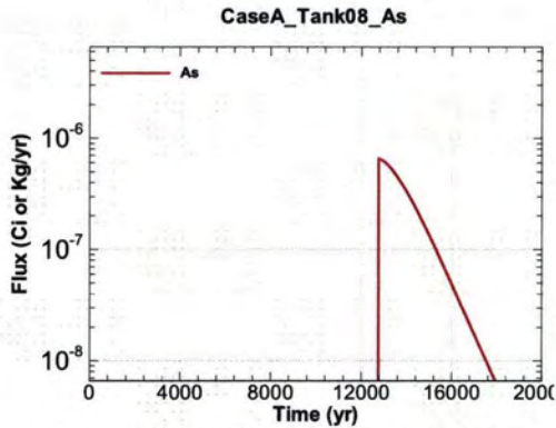
Figure A.1-553 - Flux Leaving Liner for CaseA Tank08 As
