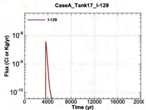
Figure A.1-1438 - Flux Leaving Liner for CaseA Tank17 I-129
