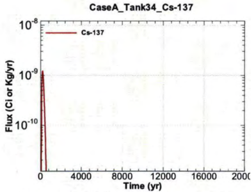
Figure A.1-727 - Flux Leaving Liner for CaseA Tank34 Cs-137
