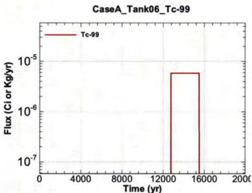
Figure A.1-455 - Flux Leaving Liner for CaseA Tank06 Tc-99
