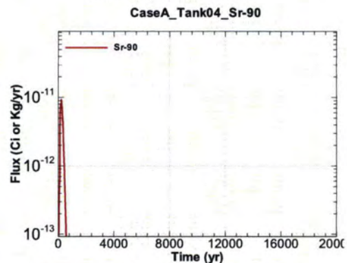
Figure A.1-298 - Flux Leaving Liner for CaseA Tank04 Sr-90
