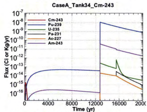
Figure A.1-718 - Flux Leaving Liner for CaseA Tank34 Cm-243
