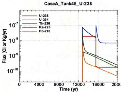
Figure A.1-1245 - Flux Leaving Liner for CaseA Tank45 U-238
