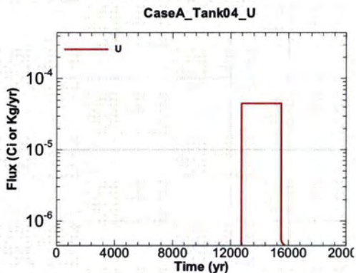
Figure A.1-303 - Flux Leaving Liner for CaseA Tank04 U
