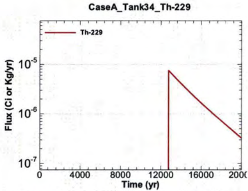
Figure A.1-769 - Flux Leaving Liner for CaseA Tank34 Th-229
