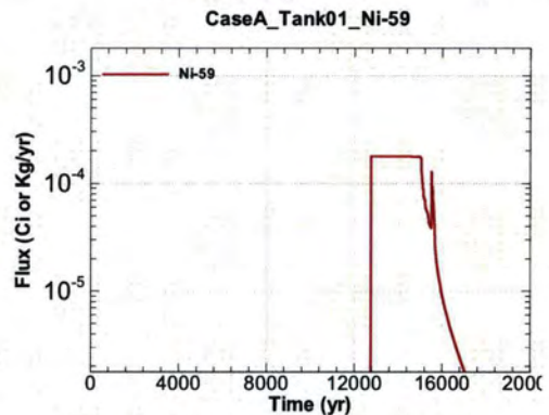
Figure A.1-40 - Flux Leaving Liner for CaseA Tank01 Ni-59
