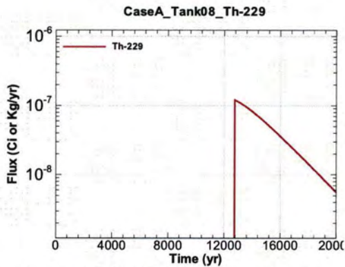
Figure A.1-613 - Flux Leaving Liner for CaseA Tank08 Th-229
