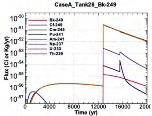
Figure A.1-1024 - Flux Leaving Liner for CaseA Tank28 Bk-249
