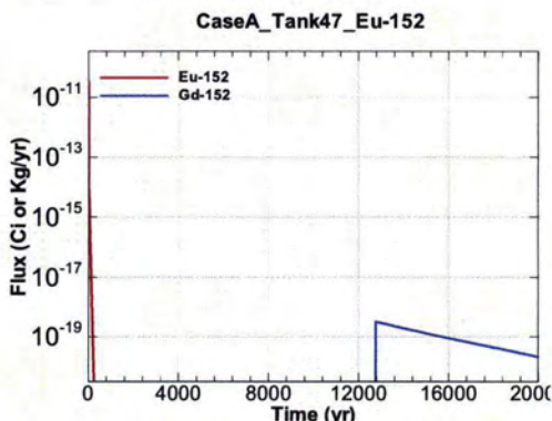
Figure A.1-1353 - Flux Leaving Liner for CaseA Tank47 Eu-152
