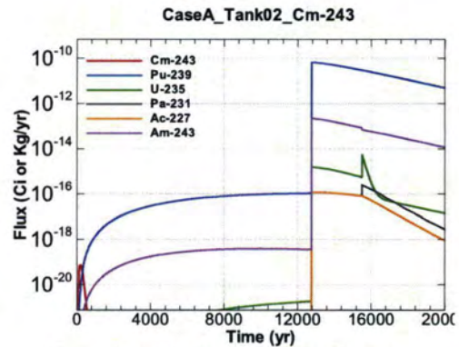
Figure A.1-94 - Flux Leaving Liner for CaseA Tank02 Cm-243
