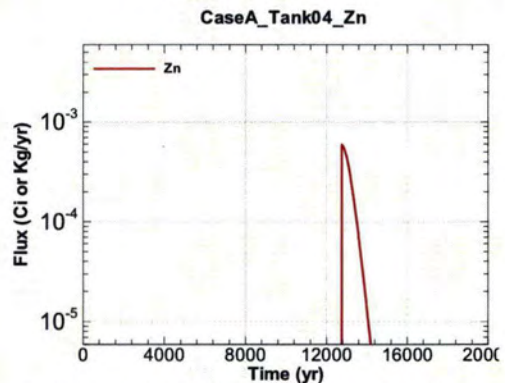
Figure A.1-312 - Flux Leaving Liner for CaseA Tank04 Zn
