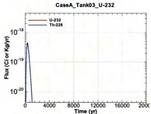
Figure A.1-226 - Flux Leaving Liner for CaseA Tank03 U-232
