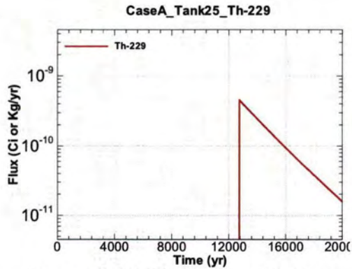
Figure A.1-847 - Flux Leaving Liner for CaseA Tank25 Th-229
