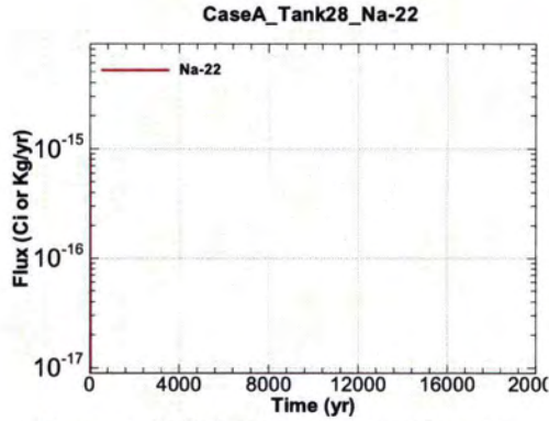
Figure A.1-1051 - Flux Leaving Liner for CaseA Tank28 Na-22
