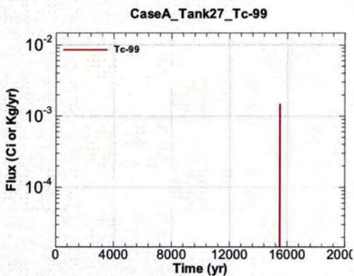
Figure A.1-1001 - Flux Leaving Liner for CaseA Tank27 Tc-99
