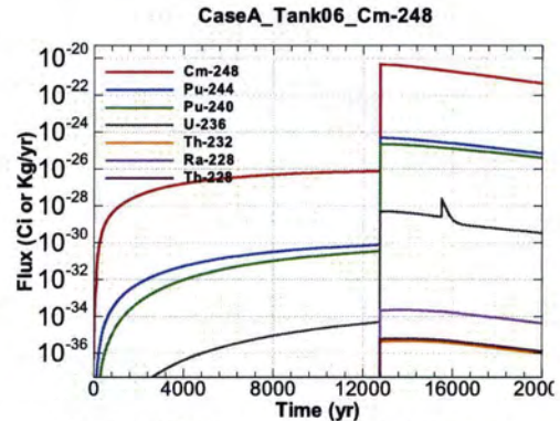
Figure A.1-410 - Flux Leaving Liner for CaseA Tank06 Cm-248
