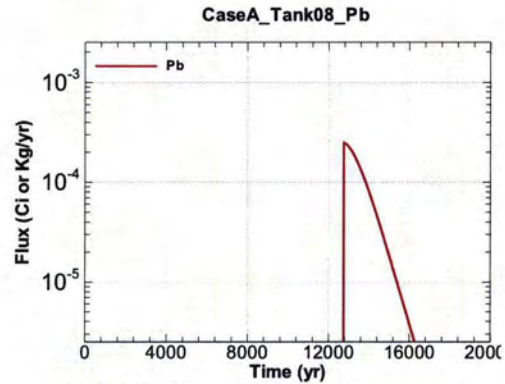
Figure A.1-590 - Flux Leaving Liner for CaseA Tank08 Pb
