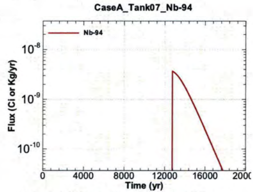
Figure A.1-506 - Flux Leaving Liner for CaseA Tank07 Nb-94
