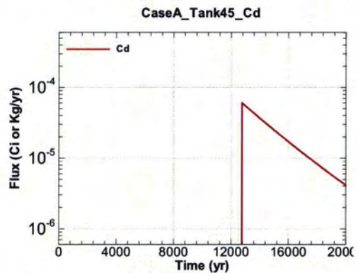
Figure A.1-1182 - Flux Leaving Liner for CaseA Tank45 Cd
