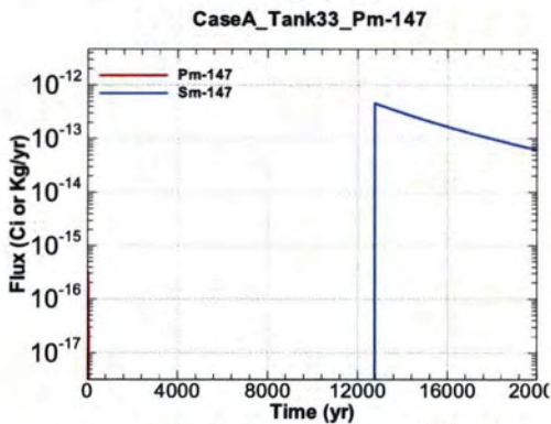
Figure A.1-669 - Flux Leaving Liner for CaseA Tank33 Pm-147
