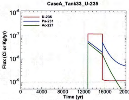
Figure A.1-697 - Flux Leaving Liner for CaseA Tank33 U-235
