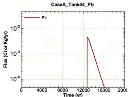
Figure A.1-1136 - Flux Leaving Liner for CaseA Tank44 Pb
