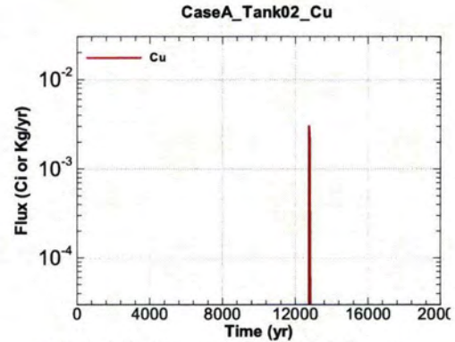
Figure A.1-104 - Flux Leaving Liner for CaseA Tank02 Cu
