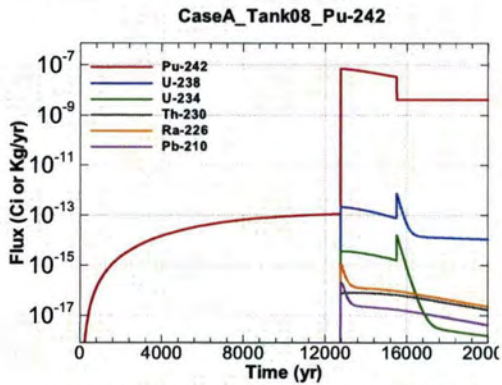
Figure A.1-597 - Flux Leaving Liner for CaseA Tank08 Pu-242
