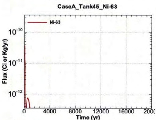
Figure A.1-1211 - Flux Leaving Liner for CaseA Tank45 Ni-63
