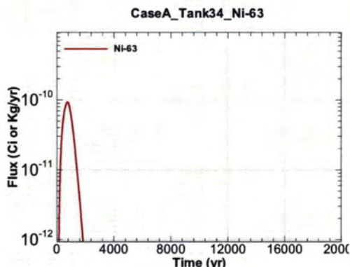
Figure A.1-743 - Flux Leaving Liner for CaseA Tank34 Ni-63
