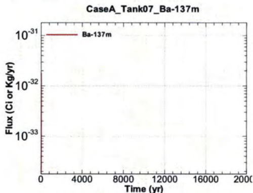
Figure A.1-477 - Flux Leaving Liner for CaseA Tank07 Ba-137m
