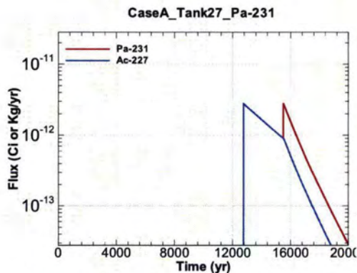
Figure A.1-979 - Flux Leaving Liner for CaseA Tank27 Pa-231
