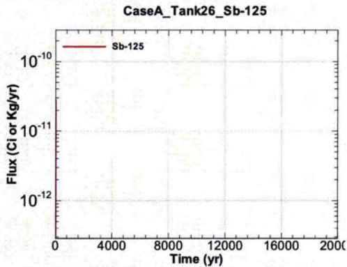
Figure A.1-915 - Flux Leaving Liner for CaseA Tank26 Sb-125
