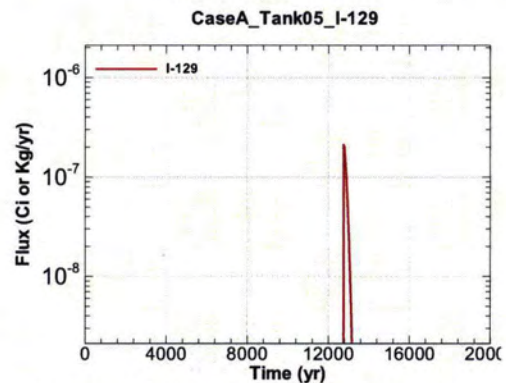
Figure A.1-346 - Flux Leaving Liner for CaseA Tank05 I-129
