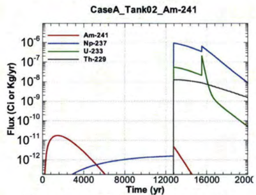
Figure A.1-82 - Flux Leaving Liner for CaseA Tank02 Am-241
