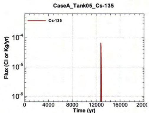
Figure A.1-336 - Flux Leaving Liner for CaseA Tank05 Cs-135
