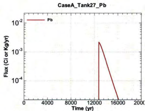
Figure A.1-980 - Flux Leaving Liner for CaseA Tank27 Pb
