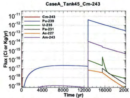
Figure A.1-1186 - Flux Leaving Liner for CaseA Tank45 Cm-243
