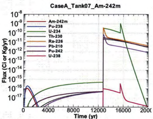
Figure A.1-473 - Flux Leaving Liner for CaseA Tank07 Am-242m
