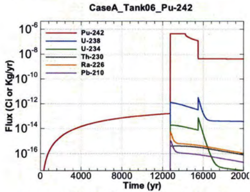
Figure A.1-441 - Flux Leaving Liner for CaseA Tank06 Pu-242
