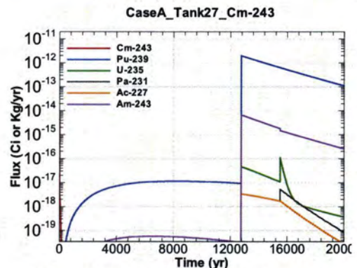
Figure A.1-952 - Flux Leaving Liner for CaseA Tank27 Cm-243
