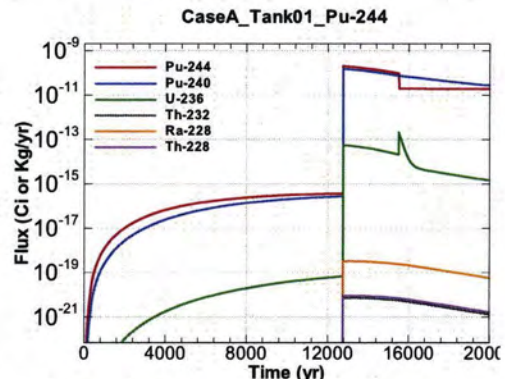
Figure A.1-52 - Flux Leaving Liner for CaseA Tank01 Pu-244
