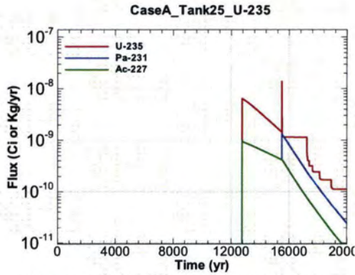
Figure A.1-853 - Flux Leaving Liner for CaseA Tank25 U-235
