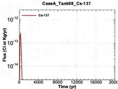
Figure A.1-571 - Flux Leaving Liner for CaseA Tank08 Cs-137
