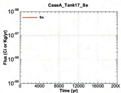
Figure A.1-1464 - Flux Leaving Liner for CaseA Tank17 Se
