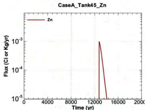
Figure A.1-1248 - Flux Leaving Liner for CaseA Tank45 Zn
