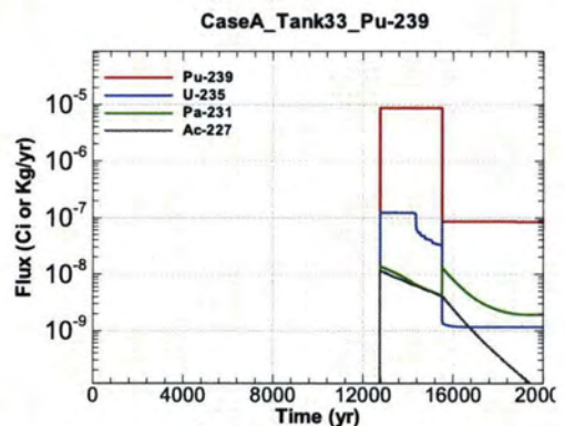
Figure A.1-672 - Flux Leaving Liner for CaseA Tank33 Pu-239
