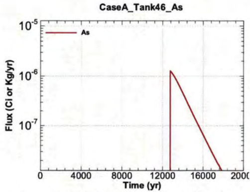
Figure A.1-1255 - Flux Leaving Liner for CaseA Tank46 As
