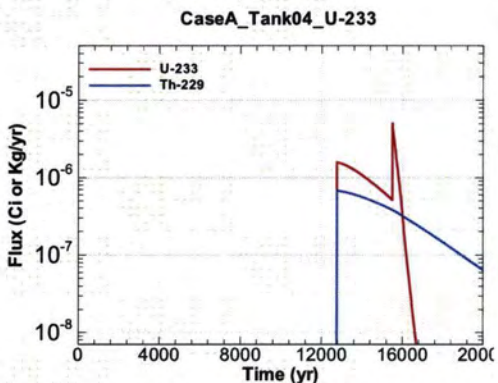
Figure A.1-305 - Flux Leaving Liner for CaseA Tank04 U-233
