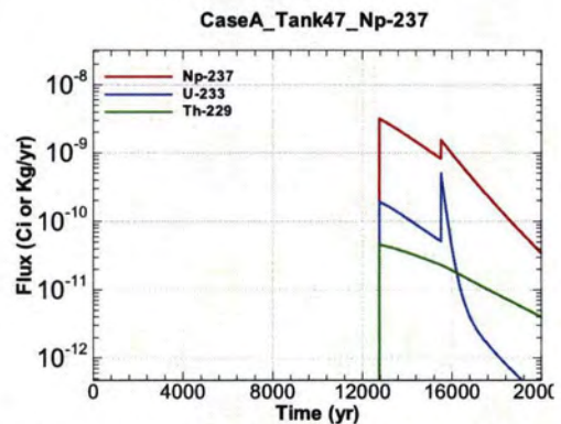
Figure A.1-1368 - Flux Leaving Liner for CaseA Tank47 Np-237
