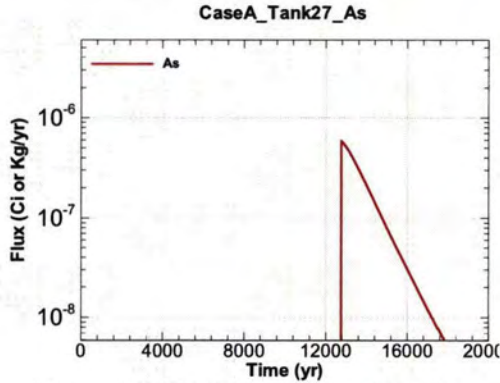
Figure A.1-943 - Flux Leaving Liner for CaseA Tank27 As
