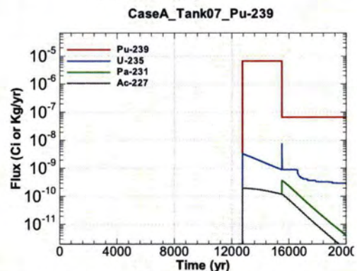
Figure A.1-516 - Flux Leaving Liner for CaseA Tank07 Pu-239
