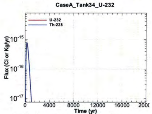
Figure A.1-772 - Flux Leaving Liner for CaseA Tank34 U-232
