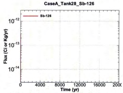
Figure A.1-1072 - Flux Leaving Liner for CaseA Tank28 Sb-126
