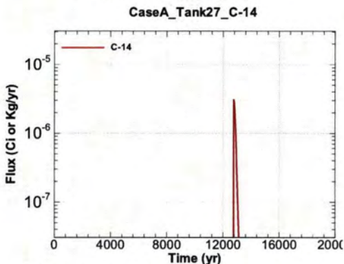
Figure A.1-947 - Flux Leaving Liner for CaseA Tank27 C-14
