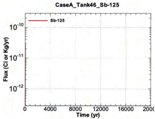
Figure A.1-1305 - Flux Leaving Liner for CaseA Tank46 Sb-125
