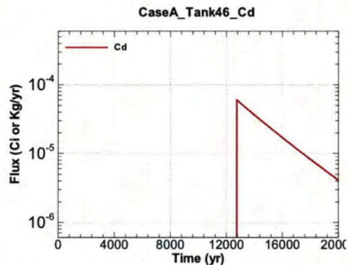
Figure A.1-1260 - Flux Leaving Liner for CaseA Tank46 Cd
