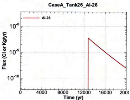
Figure A.1-861 - Flux Leaving Liner for CaseA Tank26 Al-26
