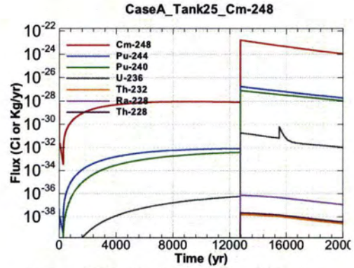
Figure A.1-800 - Flux Leaving Liner for CaseA Tank25 Cm-248
