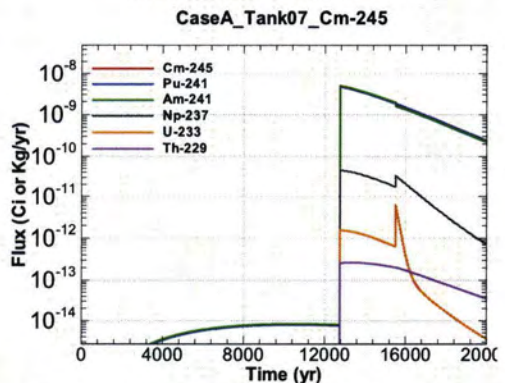
Figure A.1-486 - Flux Leaving Liner for CaseA Tank07 Cm-245
