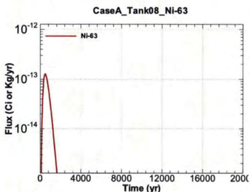
Figure A.1-587 - Flux Leaving Liner for CaseA Tank08 Ni-63
