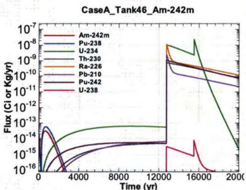
Figure A.1-1253 - Flux Leaving Liner for CaseA Tank46 Am-242m
