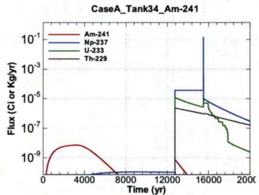
Figure A.1-706 - Flux Leaving Liner for CaseA Tank34 Am-241
