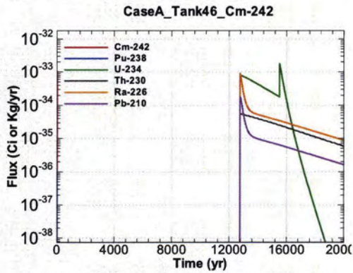
Figure A.1-1263 - Flux Leaving Liner for CaseA Tank46 Cm-242
