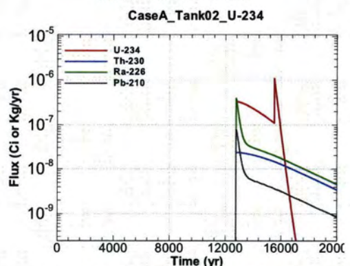
Figure A.1-150 - Flux Leaving Liner for CaseA Tank02 U-234
