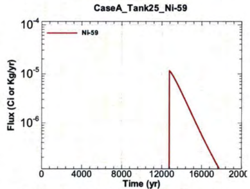
Figure A.1-820 - Flux Leaving Liner for CaseA Tank25 Ni-59
