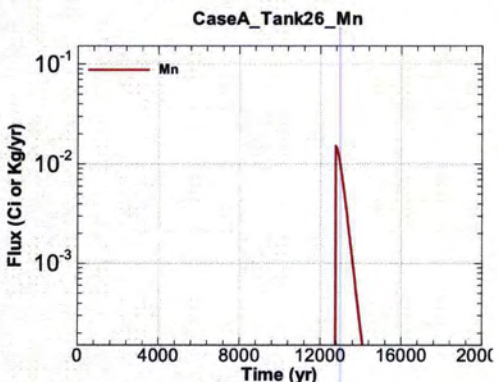
Figure A.1-893 - Flux Leaving Liner for CaseA Tank26 Mn
