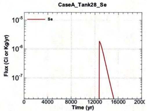
Figure A.1-1074 - Flux Leaving Liner for CaseA Tank28 Se
