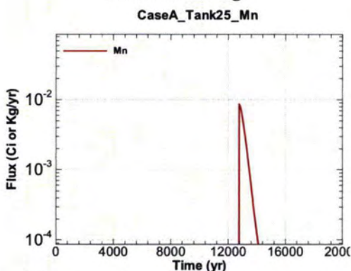
Figure A.1-815 - Flux Leaving Liner for CaseA Tank25 Mn
