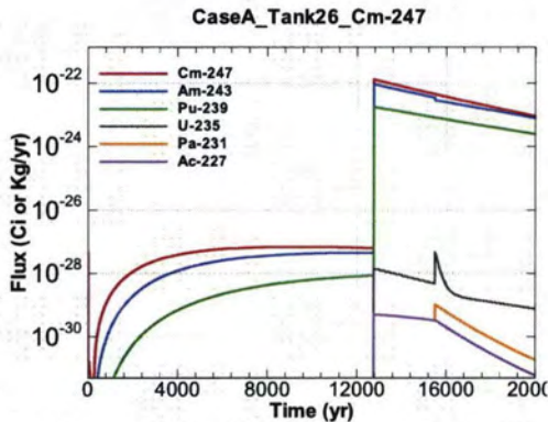
Figure A.1-877 - Flux Leaving Liner for CaseA Tank26 Cm-247
