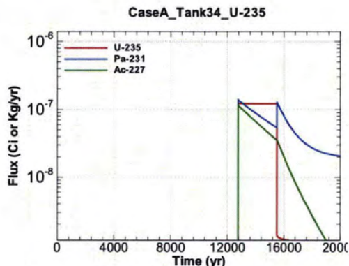
Figure A.1-775 - Flux Leaving Liner for CaseA Tank34 U-235
