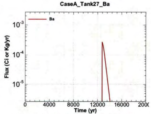
Figure A.1-944 - Flux Leaving Liner for CaseA Tank27 Ba
