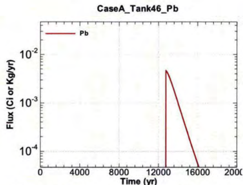
Figure A.1-1292 - Flux Leaving Liner for CaseA Tank46 Pb
