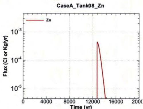
Figure A.1-624 - Flux Leaving Liner for CaseA Tank08 Zn
