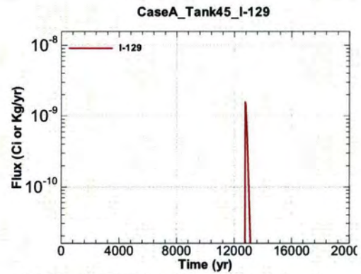
Figure A.1-1204 - Flux Leaving Liner for CaseA Tank45 I-129
