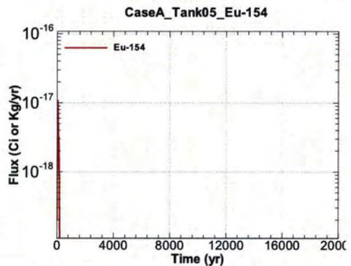
Figure A.1-340 - Flux Leaving Liner for CaseA Tank05 Eu-154
