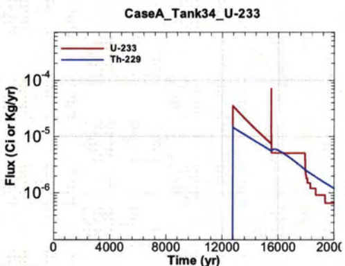
Figure A.1-773 - Flux Leaving Liner for CaseA Tank34 U-233
