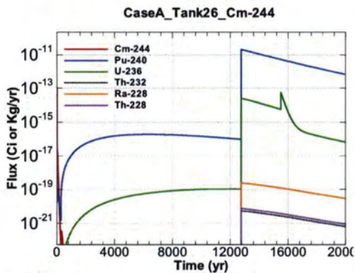
Figure A.1-875 - Flux Leaving Liner for CaseA Tank26 Cm-244
