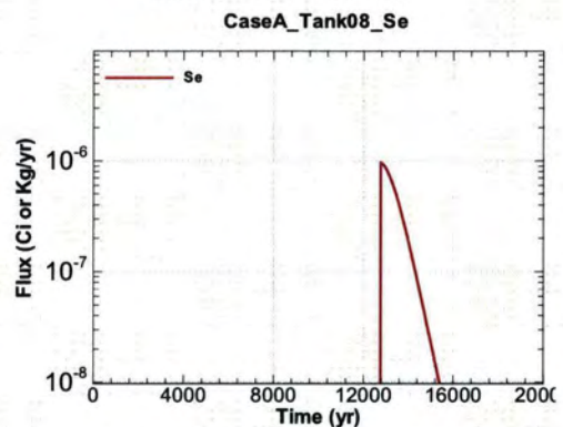
Figure A.1-606 - Flux Leaving Liner for CaseA Tank08 Se
