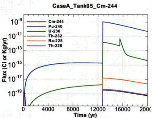
Figure A.1-329 - Flux Leaving Liner for CaseA Tank05 Cm-244
