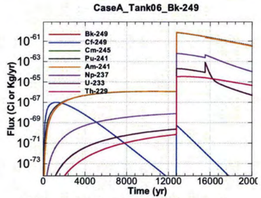
Figure A.1-400 - Flux Leaving Liner for CaseA Tank06 Bk-249
