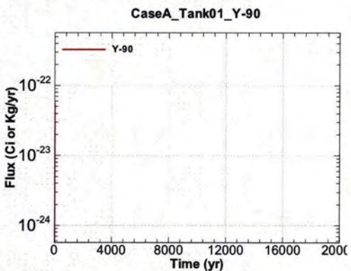
Figure A.1-77 - Flux Leaving Liner for CaseA Tank01 Y-90
