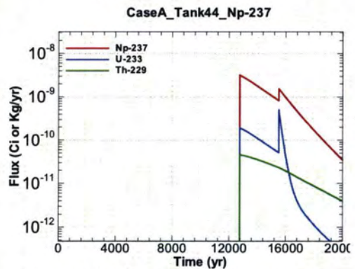
Figure A.1-1134 - Flux Leaving Liner for CaseA Tank44 Np-237
