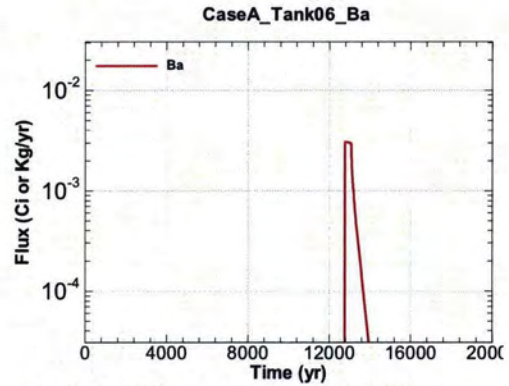
Figure A.1-398 - Flux Leaving Liner for CaseA Tank06 Ba
