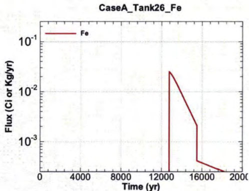
Figure A.1-889 - Flux Leaving Liner for CaseA Tank26 Fe
