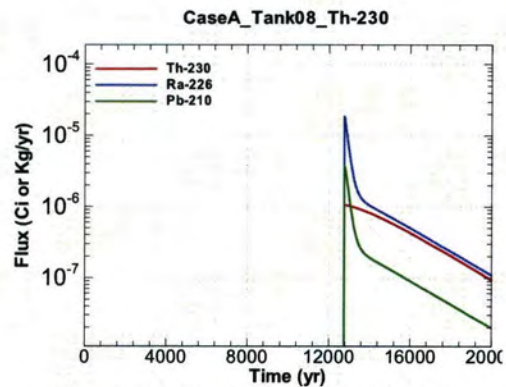
Figure A.1-614 - Flux Leaving Liner for CaseA Tank08 Th-230
