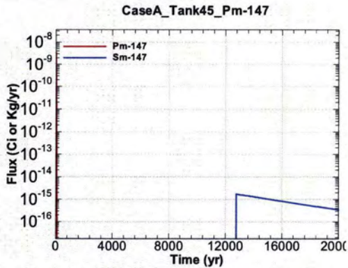
Figure A.1-1215 - Flux Leaving Liner for CaseA Tank45 Pm-147
