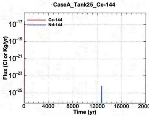
Figure A.1-793 - Flux Leaving Liner for CaseA Tank25 Ce-144
