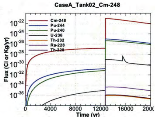
Figure A.1-98 - Flux Leaving Liner for CaseA Tank02 Cm-248
