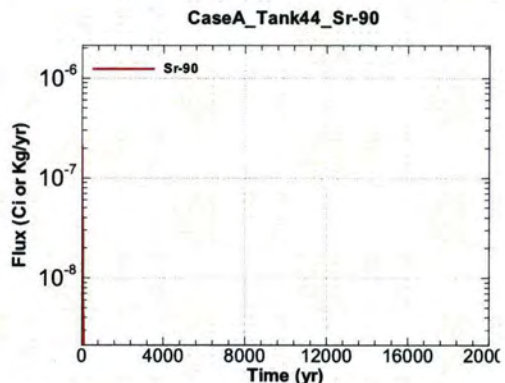
Figure A.1-1156 - Flux Leaving Liner for CaseA Tank44 Sr-90
