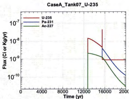
Figure A.1-541 - Flux Leaving Liner for CaseA Tank07 U-235
