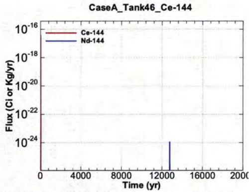
Figure A.1-1261 - Flux Leaving Liner for CaseA Tank46 Ce-144
