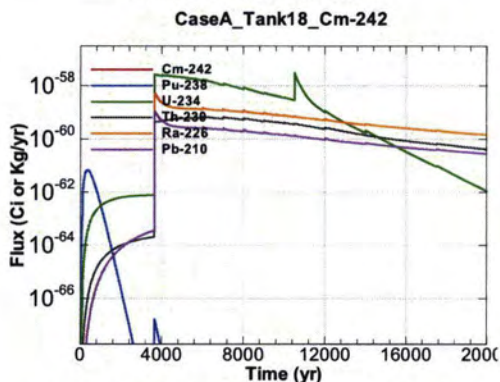
Figure A.1-1497 - Flux Leaving Liner for CaseA Tank18 Cm-242
