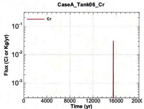
Figure A.1-412 - Flux Leaving Liner for CaseA Tank06 Cr
