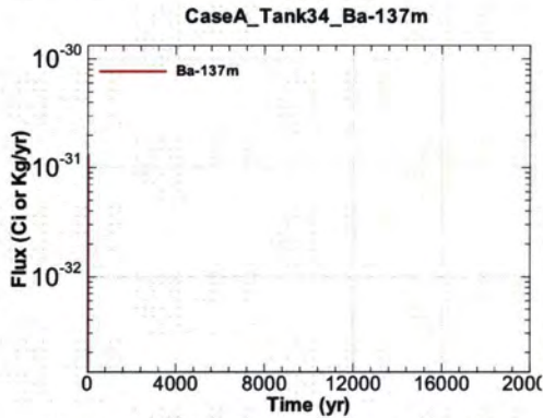
Figure A.1-711 - Flux Leaving Liner for CaseA Tank34 Ba-137m
