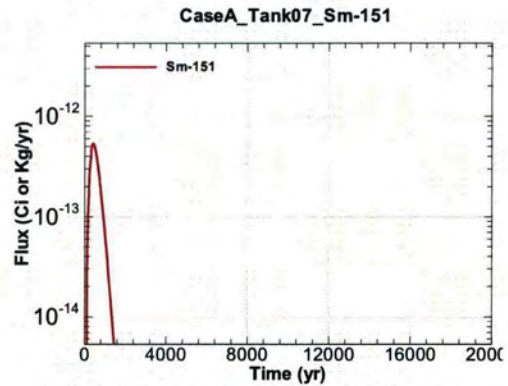
Figure A.1-530 - Flux Leaving Liner for CaseA Tank07 Sm-151
