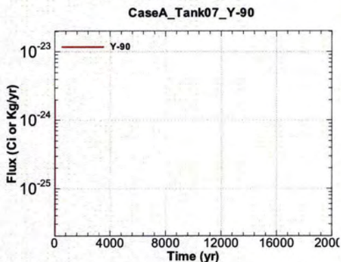
Figure A.1-545 - Flux Leaving Liner for CaseA Tank07 Y-90
