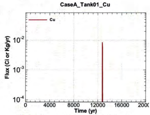
Figure A.1-26 - Flux Leaving Liner for CaseA Tank01 Cu
