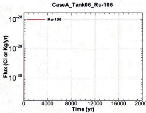
Figure A.1-445 - Flux Leaving Liner for CaseA Tank06 Ru-106
