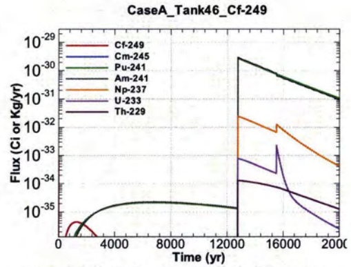
Figure A.1-1262 - Flux Leaving Liner for CaseA Tank46 Cf-249
