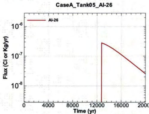
Figure A.1-315 - Flux Leaving Liner for CaseA Tank05 Al-26
