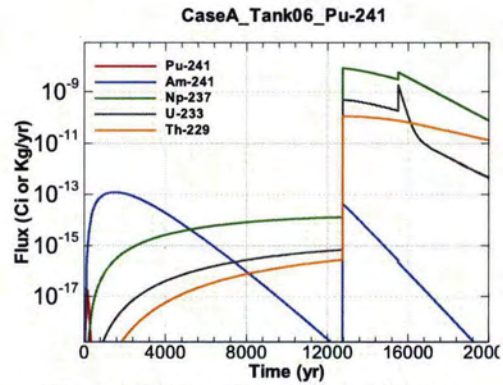
Figure A.1-440 - Flux Leaving Liner for CaseA Tank06 Pu-241
