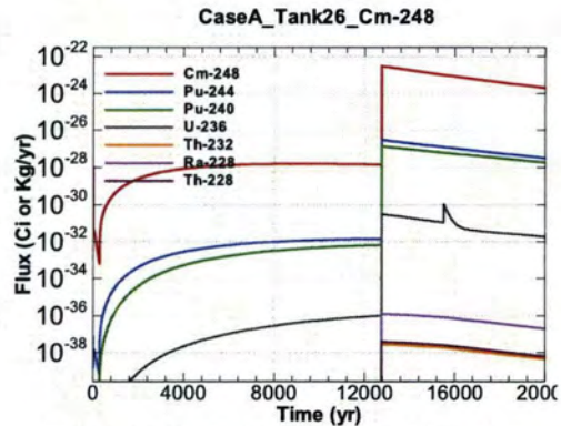
Figure A.1-878 - Flux Leaving Liner for CaseA Tank26 Cm-248
