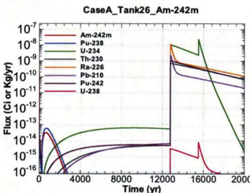
Figure A.1-863 - Flux Leaving Liner for CaseA Tank26 Am-242m
