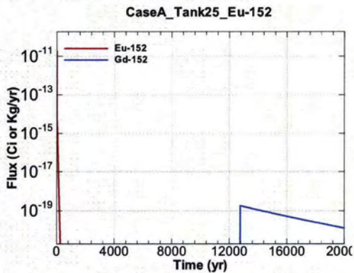
Figure A.1-807 - Flux Leaving Liner for CaseA Tank25 Eu-152
