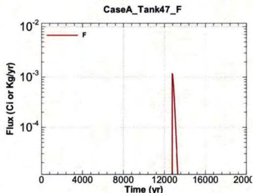
Figure A.1-1356 - Flux Leaving Liner for CaseA Tank47 F
