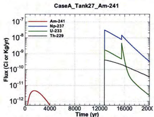
Figure A.1-940 - Flux Leaving Liner for CaseA Tank27 Am-241
