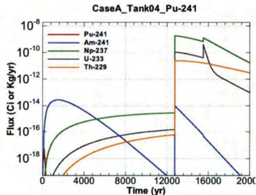
Figure A.1-284 - Flux Leaving Liner for CaseA Tank04 Pu-241
