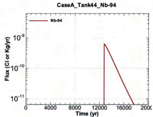
Figure A.1-1130 - Flux Leaving Liner for CaseA Tank44 Nb-94
