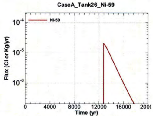
Figure A.1-898 - Flux Leaving Liner for CaseA Tank26 Ni-59
