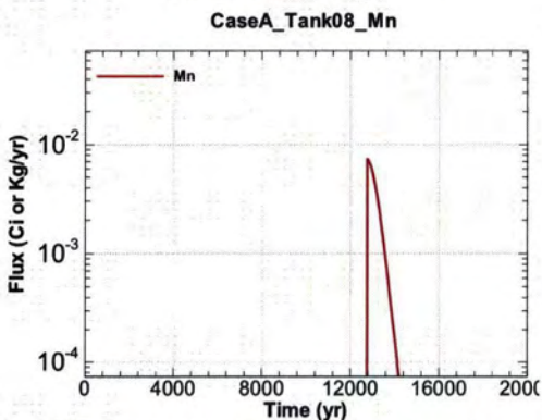
Figure A.1-581 - Flux Leaving Liner for CaseA Tank08 Mn
