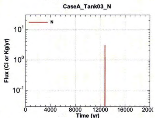
Figure A.1-192 - Flux Leaving Liner for CaseA Tank03 N
