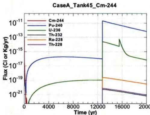
Figure A.1-1187 - Flux Leaving Liner for CaseA Tank45 Cm-244
