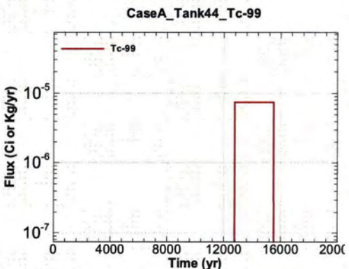
Figure A.1-1157 - Flux Leaving Liner for CaseA Tank44 Tc-99
