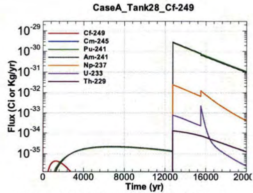
Figure A.1-1028 - Flux Leaving Liner for CaseA Tank28 Cf-249
