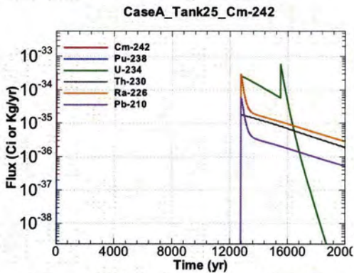
Figure A.1-795 - Flux Leaving Liner for CaseA Tank25 Cm-242
