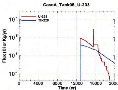
Figure A.1-383 - Flux Leaving Liner for CaseA Tank05 U-233
