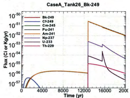
Figure A.1-868 - Flux Leaving Liner for CaseA Tank26 Bk-249
