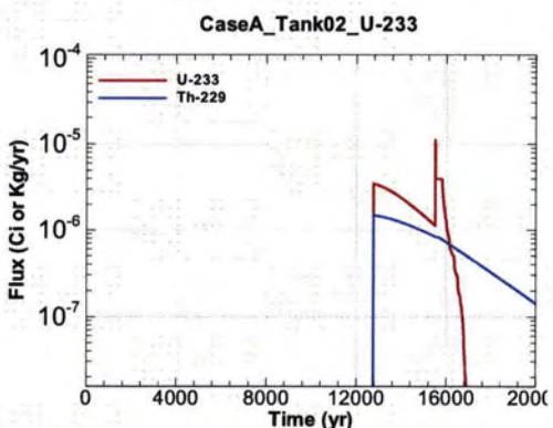
Figure A.1-149 - Flux Leaving Liner for CaseA Tank02 U-233
