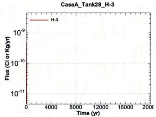
Figure A.1-1046 - Flux Leaving Liner for CaseA Tank28 H-3
