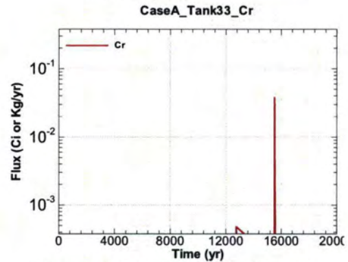
Figure A.1-646 - Flux Leaving Liner for CaseA Tank33 Cr
