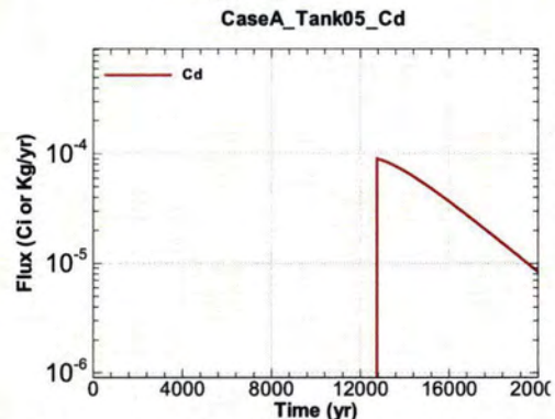
Figure A.1-324 - Flux Leaving Liner for CaseA Tank05 Cd
