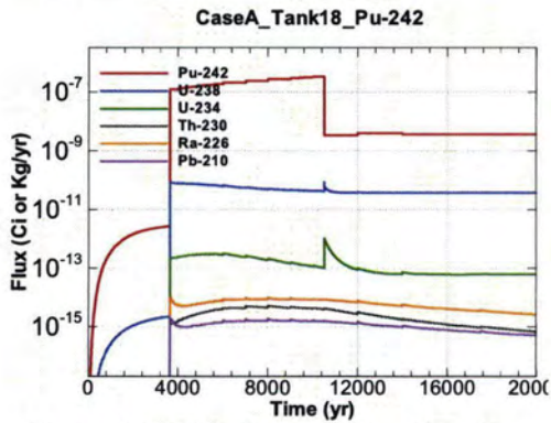
Figure A.1-1533 - Flux Leaving Liner for CaseA Tank18 Pu-242
