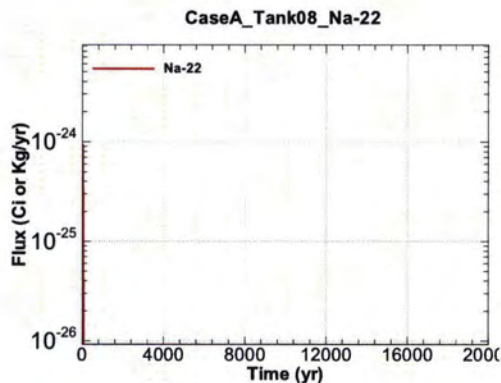
Figure A.1-583 - Flux Leaving Liner for CaseA Tank08 Na-22
