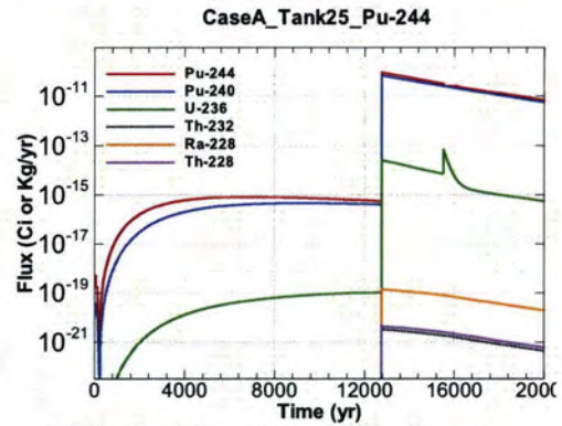
Figure A.1-832 - Flux Leaving Liner for CaseA Tank25 Pu-244
