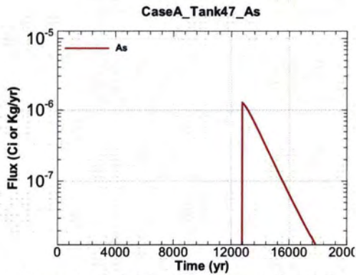
Figure A.1-1333 - Flux Leaving Liner for CaseA Tank47 As
