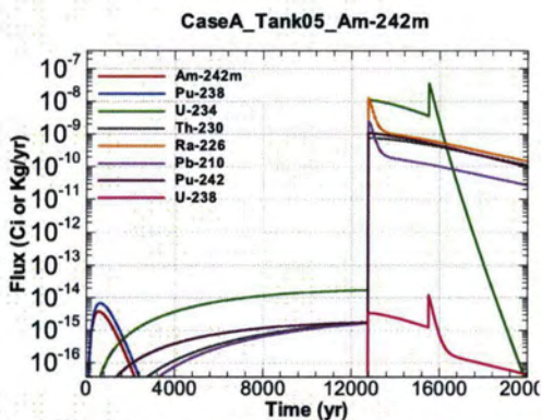
Figure A.1-317 - Flux Leaving Liner for CaseA Tank05 Am-242m
