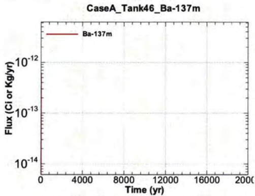
Figure A.1-1257 - Flux Leaving Liner for CaseA Tank46 Ba-137m
