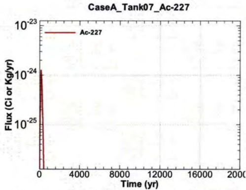
Figure A.1-469 - Flux Leaving Liner for CaseA Tank07 Ac-227
