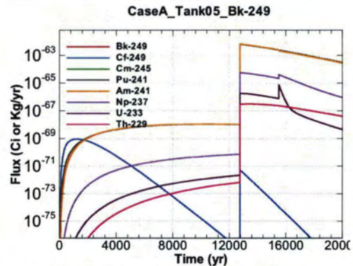
Figure A.1-322 - Flux Leaving Liner for CaseA Tank05 Bk-249
