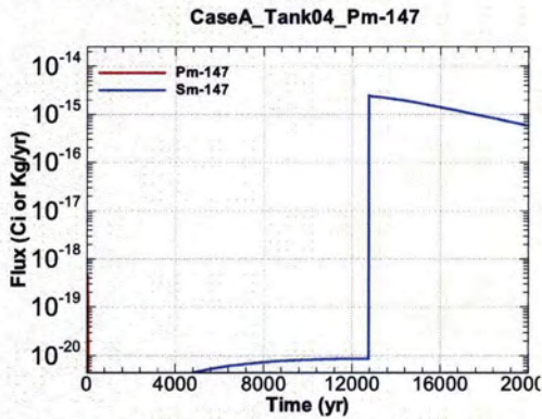
Figure A.1-279 - Flux Leaving Liner for CaseA Tank04 Pm-147
