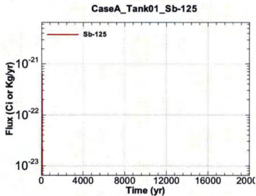
Figure A.1-57 - Flux Leaving Liner for CaseA Tank01 Sb-125
