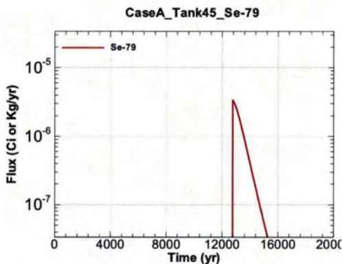
Figure A.1-1231 - Flux Leaving Liner for CaseA Tank45 Se-79
