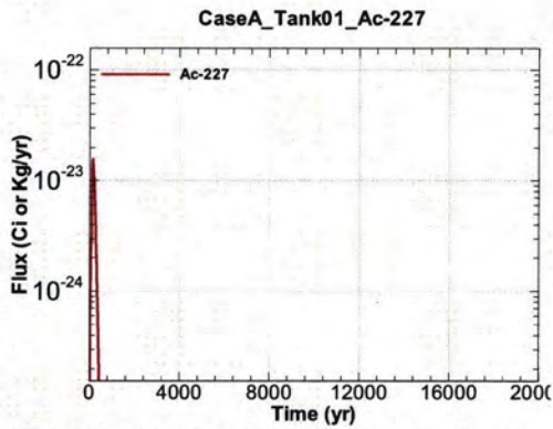
Figure A.1-1 - Flux Leaving Liner for CaseA Tank01 Ac-227
