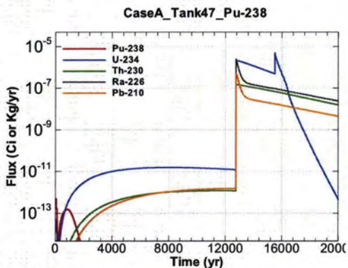
Figure A.1-1373 - Flux Leaving Liner for CaseA Tank47 Pu-238
