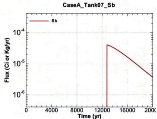
Figure A.1-524 - Flux Leaving Liner for CaseA Tank07 Sb
