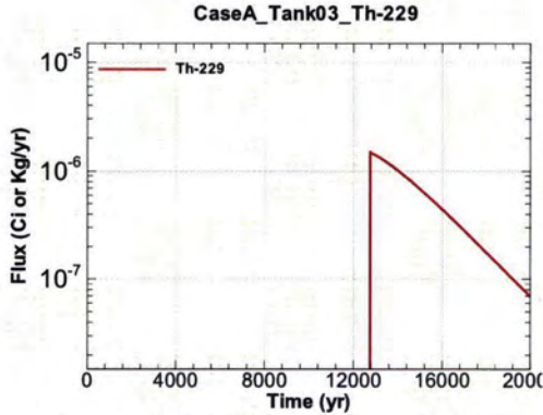
Figure A.1-223 - Flux Leaving Liner for CaseA Tank03 Th-229
