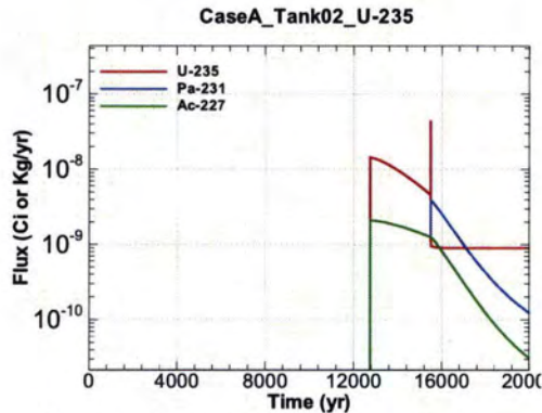
Figure A.1-151 - Flux Leaving Liner for CaseA Tank02 U-235
