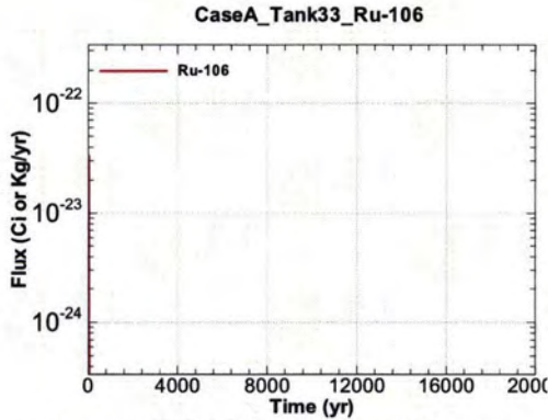
Figure A.1-679 - Flux Leaving Liner for CaseA Tank33 Ru-106
