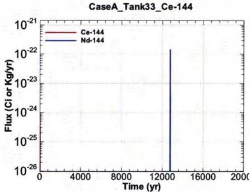
Figure A.1-637 - Flux Leaving Liner for CaseA Tank33 Ce-144
