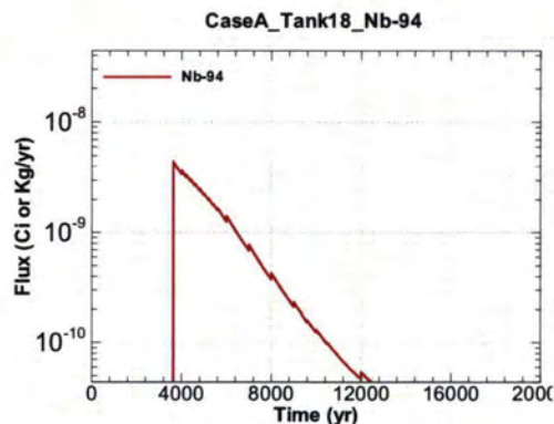
Figure A.1-1520 - Flux Leaving Liner for CaseA Tank18 Nb-94
