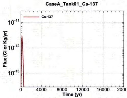
Figure A.1-25 - Flux Leaving Liner for CaseA Tank01 Cs-137
