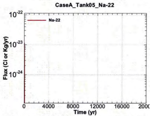
Figure A.1-349 - Flux Leaving Liner for CaseA Tank05 Na-22
