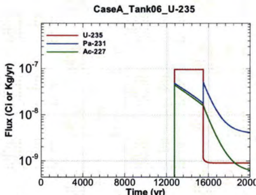
Figure A.1-463 - Flux Leaving Liner for CaseA Tank06 U-235
