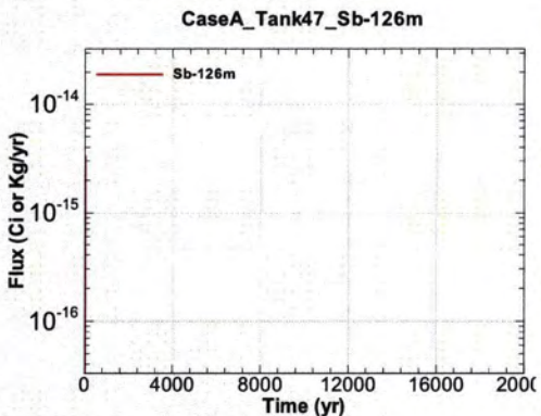
Figure A.1-1385 - Flux Leaving Liner for CaseA Tank47 Sb-126m
