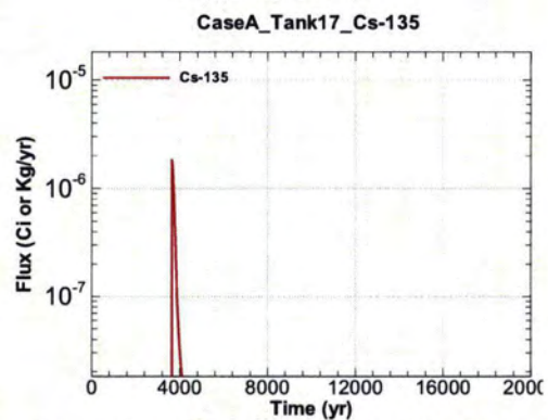
Figure A.1-1428 - Flux Leaving Liner for CaseA Tank17 Cs-135
