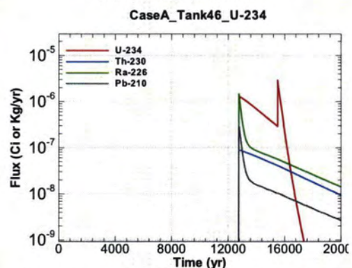
Figure A.1-1320 - Flux Leaving Liner for CaseA Tank46 U-234
