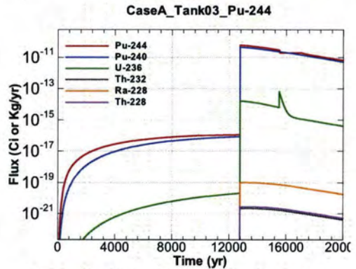
Figure A.1-208 - Flux Leaving Liner for CaseA Tank03 Pu-244
