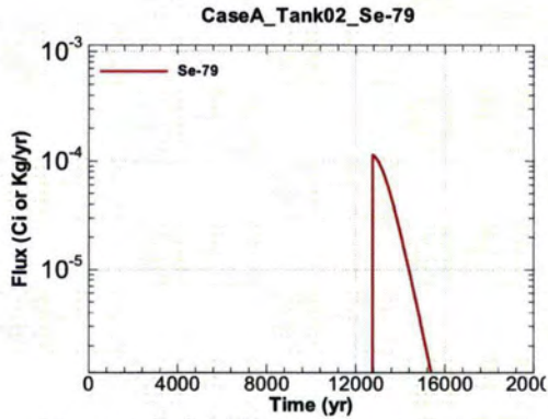
Figure A.1-139 - Flux Leaving Liner for CaseA Tank02 Se-79
