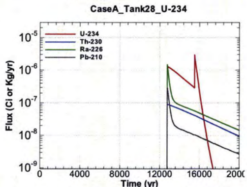
Figure A.1-1086 - Flux Leaving Liner for CaseA Tank28 U-234
