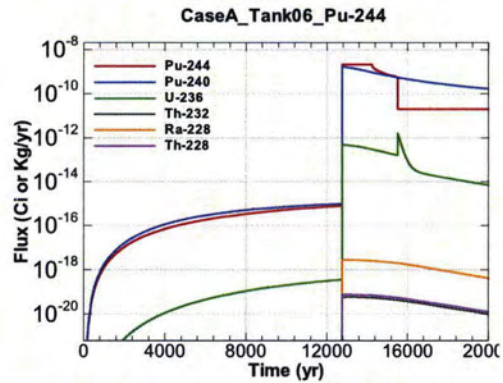
Figure A.1-442 - Flux Leaving Liner for CaseA Tank06 Pu-244
