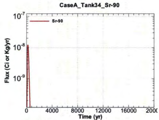
Figure A.1-766 - Flux Leaving Liner for CaseA Tank34 Sr-90
