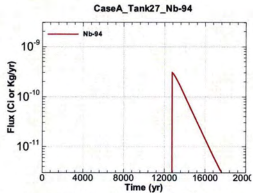
Figure A.1-974 - Flux Leaving Liner for CaseA Tank27 Nb-94
