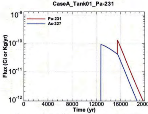
Figure A.1-43 - Flux Leaving Liner for CaseA Tank01 Pa-231
