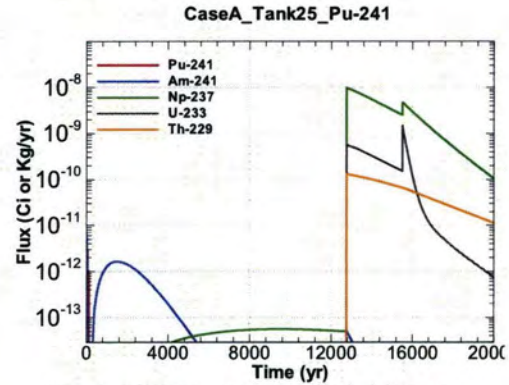
Figure A.1-830 - Flux Leaving Liner for CaseA Tank25 Pu-241
