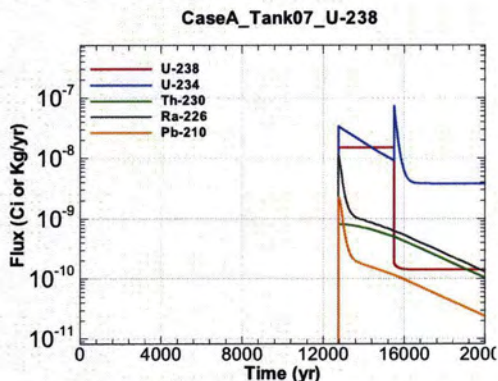
Figure A.1-543 - Flux Leaving Liner for CaseA Tank07 U-238
