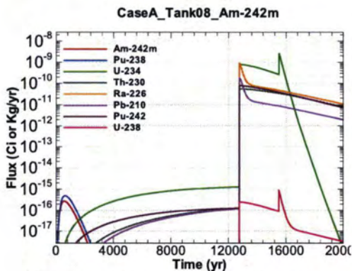
Figure A.1-551 - Flux Leaving Liner for CaseA Tank08 Am-242m
