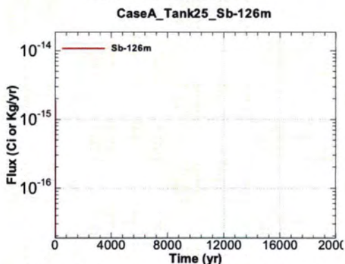
Figure A.1-839 - Flux Leaving Liner for CaseA Tank25 Sb-126m
