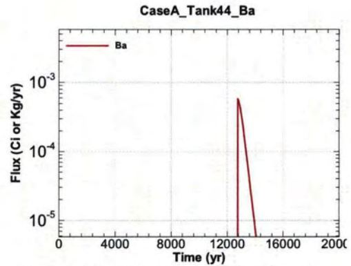
Figure A.1-1100 - Flux Leaving Liner for CaseA Tank44 Ba
