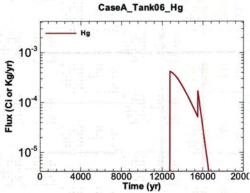
Figure A.1-423 - Flux Leaving Liner for CaseA Tank06 Hg
