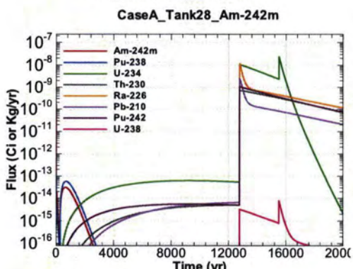
Figure A.1-1019 - Flux Leaving Liner for CaseA Tank28 Am-242m
