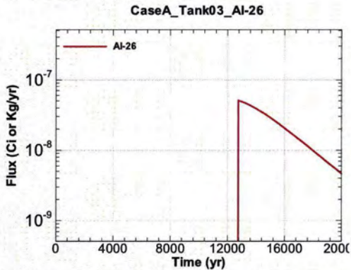
Figure A.1-159 - Flux Leaving Liner for CaseA Tank03 Al-26
