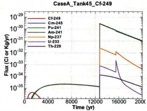
Figure A.1-1184 - Flux Leaving Liner for CaseA Tank45 Cf-249
