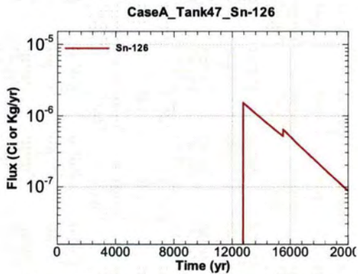
Figure A.1-1389 - Flux Leaving Liner for CaseA Tank47 Sn-126
