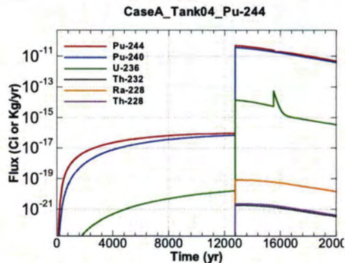
Figure A.1-286 - Flux Leaving Liner for CaseA Tank04 Pu-244
