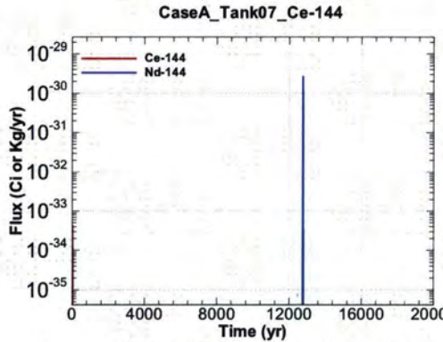
Figure A.1-481 - Flux Leaving Liner for CaseA Tank07 Ce-144
