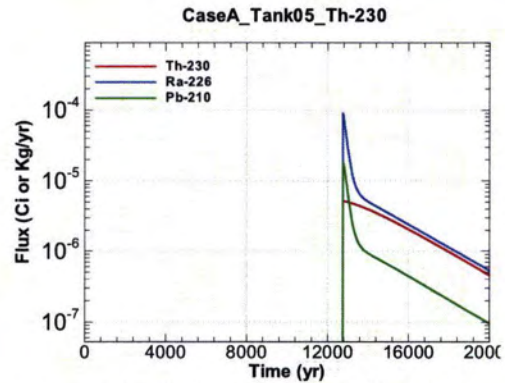
Figure A.1-380 - Flux Leaving Liner for CaseA Tank05 Th-230
