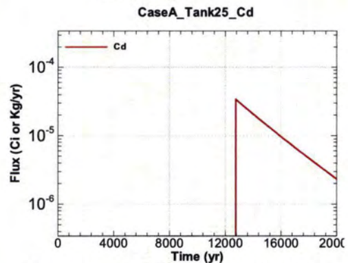
Figure A.1-792 - Flux Leaving Liner for CaseA Tank25 Cd
