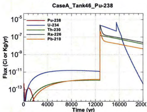
Figure A.1-1295 - Flux Leaving Liner for CaseA Tank46 Pu-238
