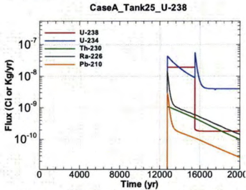
Figure A.1-855 - Flux Leaving Liner for CaseA Tank25 U-238
