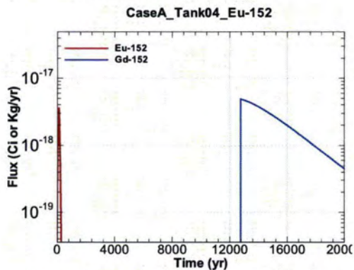
Figure A.1-261 - Flux Leaving Liner for CaseA Tank04 Eu-152
