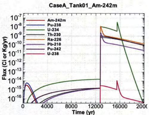
Figure A.1-5 - Flux Leaving Liner for CaseA Tank01 Am-242m
