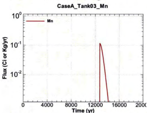
Figure A.1-191 - Flux Leaving Liner for CaseA Tank03 Mn
