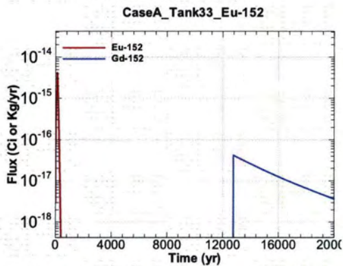
Figure A.1-651 - Flux Leaving Liner for CaseA Tank33 Eu-152
