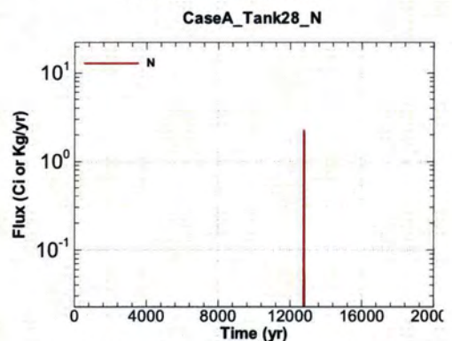
Figure A.1-1050 - Flux Leaving Liner for CaseA Tank28 N
