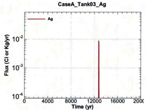
Figure A.1-158 - Flux Leaving Liner for CaseA Tank03 Ag
