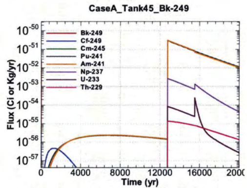
Figure A.1-1180 - Flux Leaving Liner for CaseA Tank45 Bk-249
