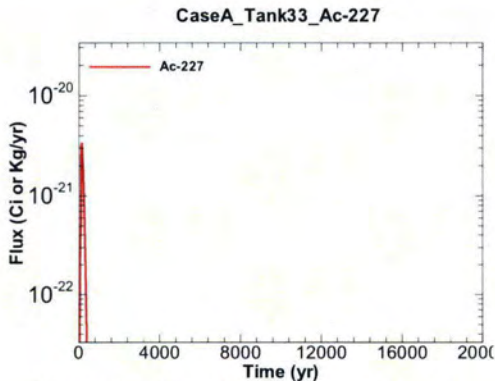
Figure A.1-625 - Flux Leaving Liner for CaseA Tank33 Ac-227
