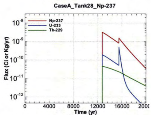
Figure A.1-1056 - Flux Leaving Liner for CaseA Tank28 Np-237
