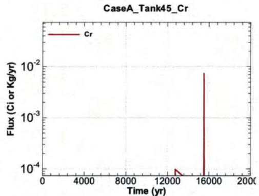
Figure A.1-1192 - Flux Leaving Liner for CaseA Tank45 Cr
