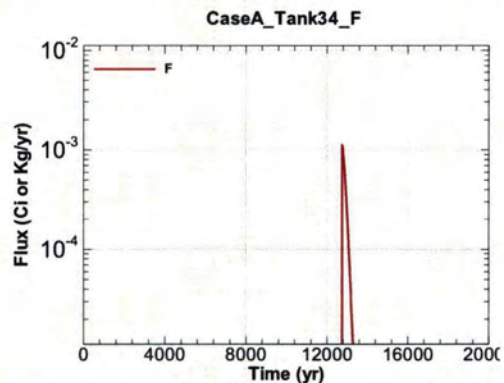
Figure A.1-732 - Flux Leaving Liner for CaseA Tank34 F
