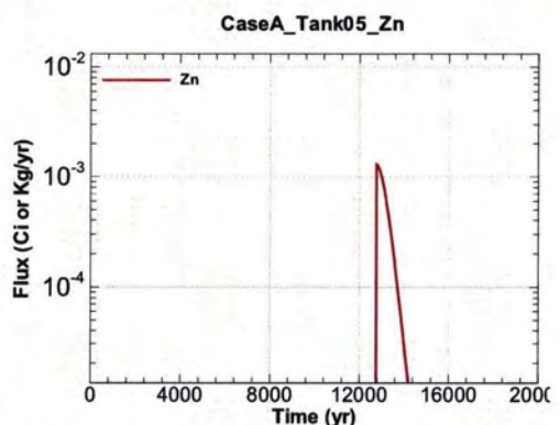
Figure A.1-390 - Flux Leaving Liner for CaseA Tank05 Zn
