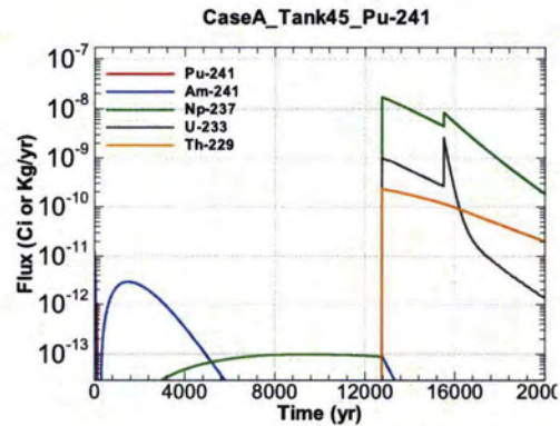
Figure A.1-1220 - Flux Leaving Liner for CaseA Tank45 Pu-241
