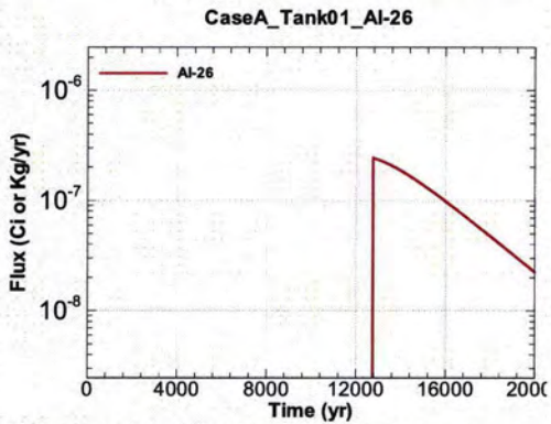
Figure A.1-3 - Flux Leaving Liner for CaseA Tank01 Al-26
