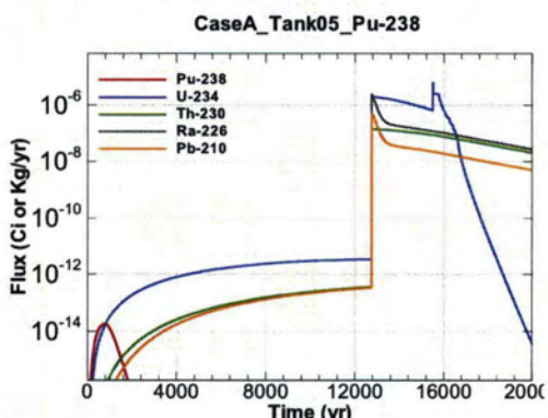
Figure A.1-359 - Flux Leaving Liner for CaseA Tank05 Pu-238
