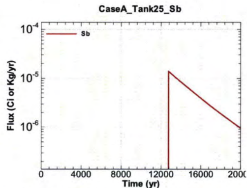
Figure A.1-836 - Flux Leaving Liner for CaseA Tank25 Sb
