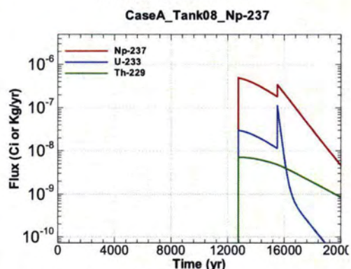
Figure A.1-588 - Flux Leaving Liner for CaseA Tank08 Np-237
