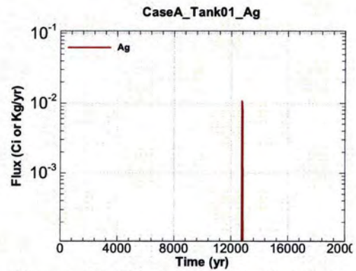
Figure A.1-2 - Flux Leaving Liner for CaseA Tank01 Ag
