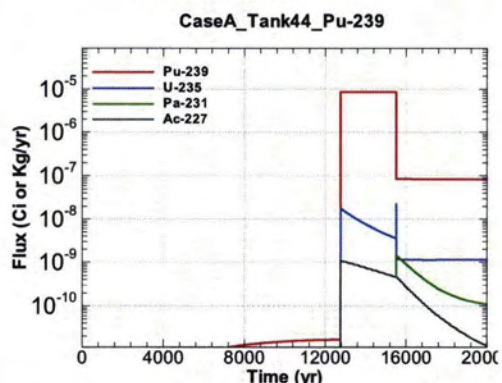
Figure A.1-1140 - Flux Leaving Liner for CaseA Tank44 Pu-239
