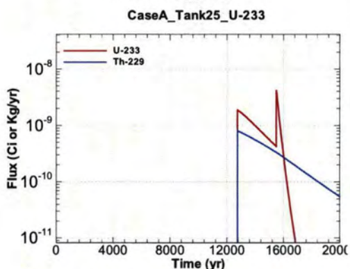
Figure A.1-851 - Flux Leaving Liner for CaseA Tank25 U-233
