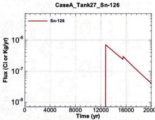
Figure A.1-999 - Flux Leaving Liner for CaseA Tank27 Sn-126
