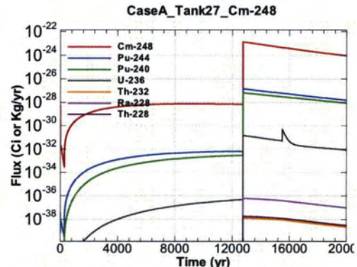
Figure A.1-956 - Flux Leaving Liner for CaseA Tank27 Cm-248
