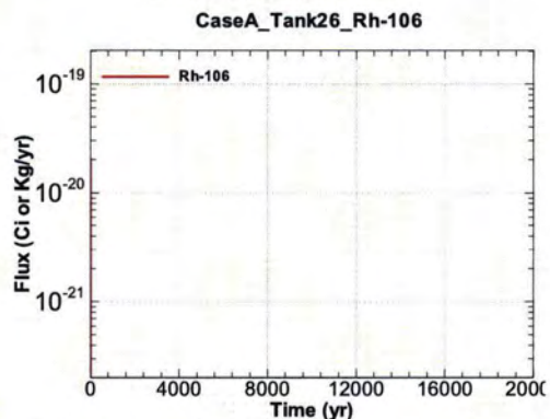
Figure A.1-912 - Flux Leaving Liner for CaseA Tank26 Rh-106
