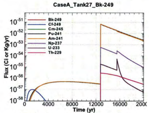
Figure A.1-946 - Flux Leaving Liner for CaseA Tank27 Bk-249
