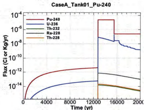
Figure A.1-49 - Flux Leaving Liner for CaseA Tank01 Pu-240
