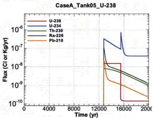
Figure A.1-387 - Flux Leaving Liner for CaseA Tank05 U-238
