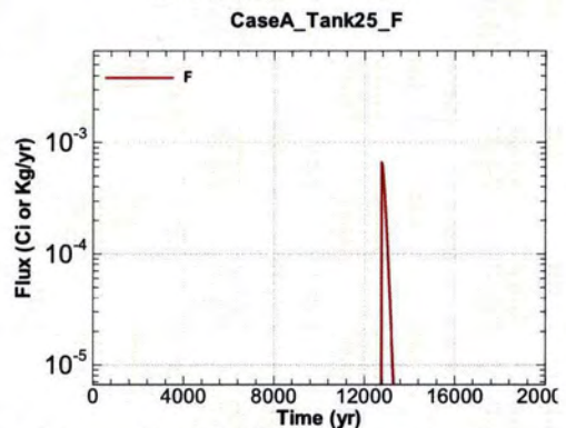
Figure A.1-810 - Flux Leaving Liner for CaseA Tank25 F
