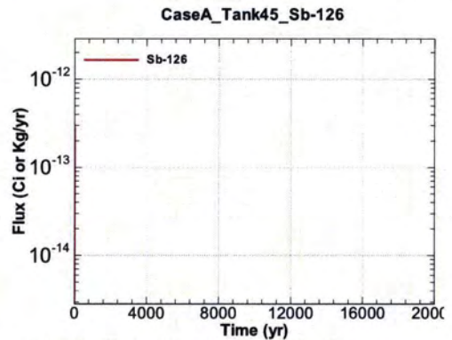
Figure A.1-1228 - Flux Leaving Liner for CaseA Tank45 Sb-126
