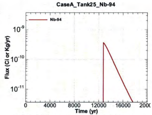
Figure A.1-818 - Flux Leaving Liner for CaseA Tank25 Nb-94
