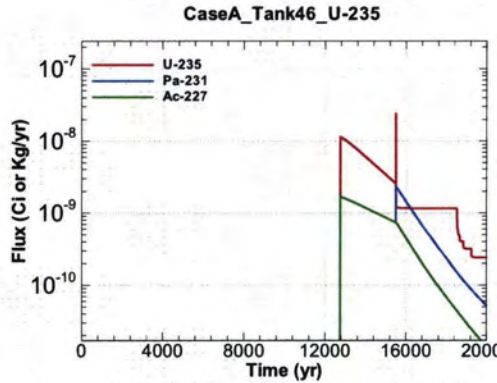
Figure A.1-1321 - Flux Leaving Liner for CaseA Tank46 U-235
