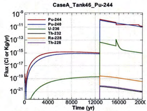
Figure A.1-1300 - Flux Leaving Liner for CaseA Tank46 Pu-244
