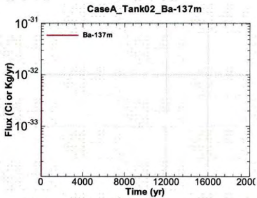
Figure A.1-87 - Flux Leaving Liner for CaseA Tank02 Ba-137m
