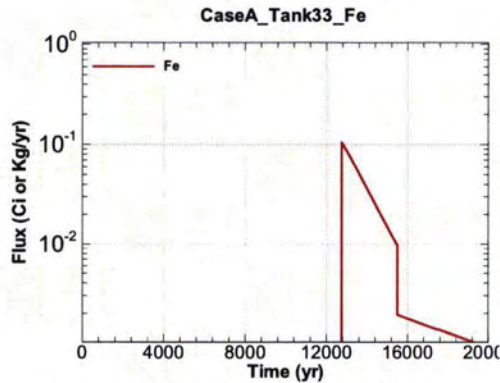
Figure A.1-655 - Flux Leaving Liner for CaseA Tank33 Fe
