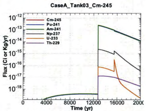
Figure A.1-174 - Flux Leaving Liner for CaseA Tank03 Cm-245
