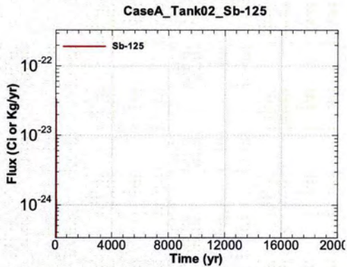
Figure A.1-135 - Flux Leaving Liner for CaseA Tank02 Sb-125
