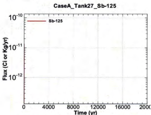
Figure A.1-993 - Flux Leaving Liner for CaseA Tank27 Sb-125
