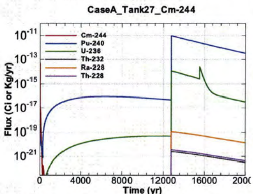
Figure A.1-953 - Flux Leaving Liner for CaseA Tank27 Cm-244
