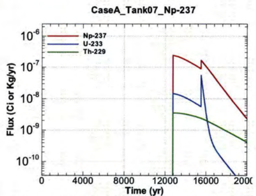
Figure A.1-510 - Flux Leaving Liner for CaseA Tank07 Np-237
