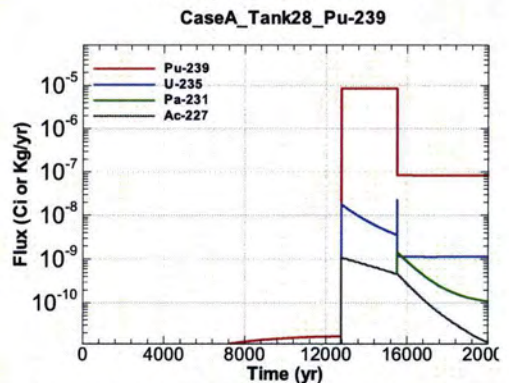
Figure A.1-1062 - Flux Leaving Liner for CaseA Tank28 Pu-239
