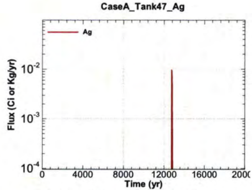
Figure A.1-1328 - Flux Leaving Liner for CaseA Tank47 Ag
