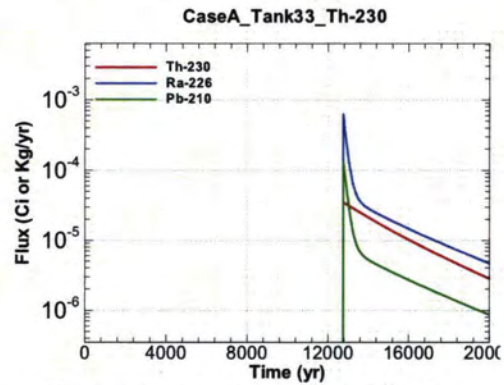
Figure A.1-692 - Flux Leaving Liner for CaseA Tank33 Th-230
