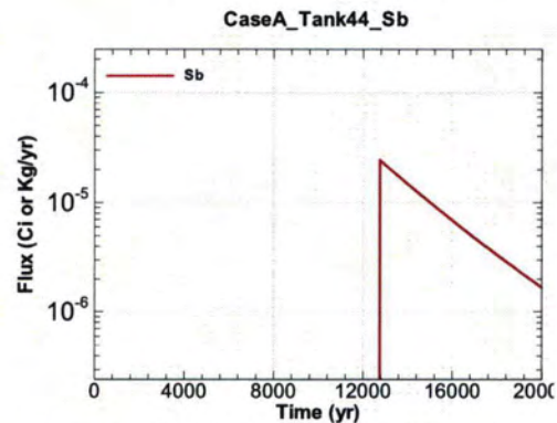
Figure A.1-1148 - Flux Leaving Liner for CaseA Tank44 Sb
