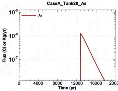
Figure A.1-1021 - Flux Leaving Liner for CaseA Tank28 As
