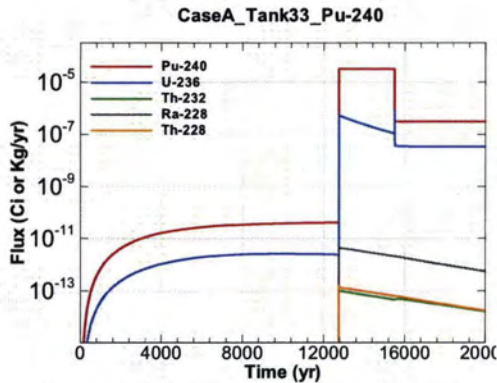
Figure A.1-673 - Flux Leaving Liner for CaseA Tank33 Pu-240
