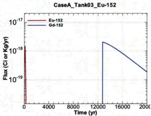
Figure A.1-183 - Flux Leaving Liner for CaseA Tank03 Eu-152
