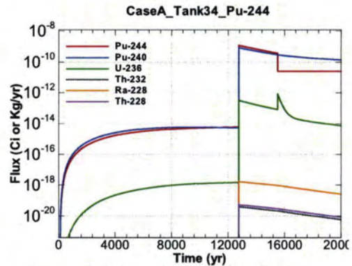
Figure A.1-754 - Flux Leaving Liner for CaseA Tank34 Pu-244
