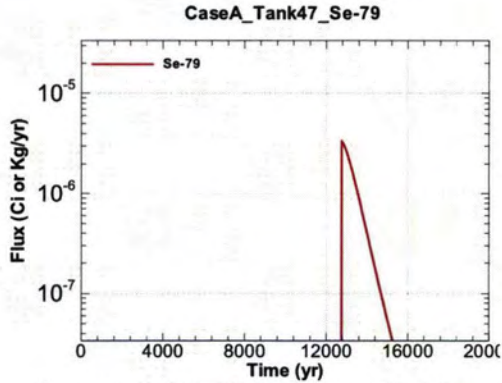
Figure A.1-1387 - Flux Leaving Liner for CaseA Tank47 Se-79
