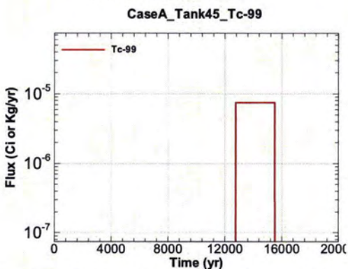
Figure A.1-1235 - Flux Leaving Liner for CaseA Tank45 Tc-99
