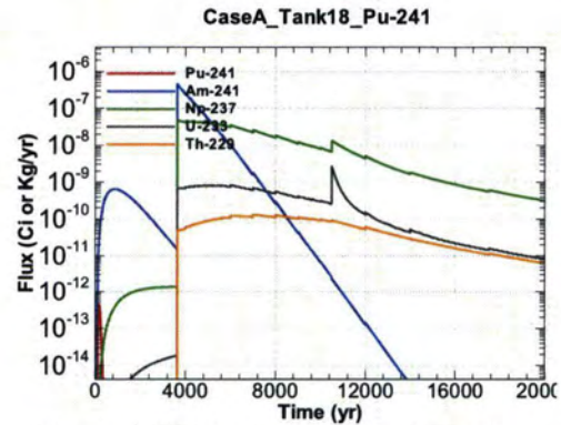
Figure A.1-1532 - Flux Leaving Liner for CaseA Tank18 Pu-241
