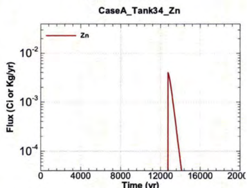
Figure A.1-780 - Flux Leaving Liner for CaseA Tank34 Zn
