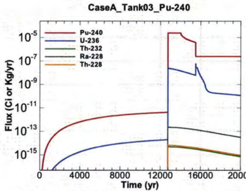
Figure A.1-205 - Flux Leaving Liner for CaseA Tank03 Pu-240
