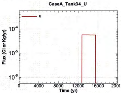
Figure A.1-771 - Flux Leaving Liner for CaseA Tank34 U
