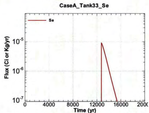
Figure A.1-684 - Flux Leaving Liner for CaseA Tank33 Se
