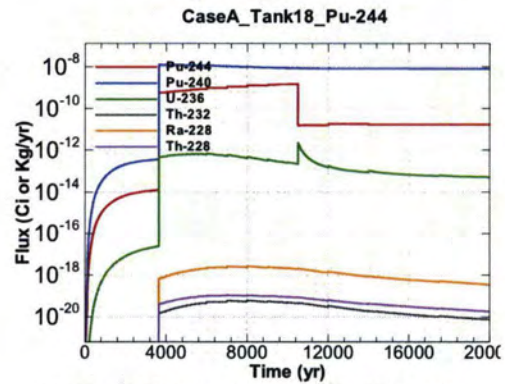
Figure A.1-1534 - Flux Leaving Liner for CaseA Tank18 Pu-244
