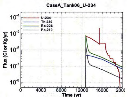
Figure A.1-462 - Flux Leaving Liner for CaseA Tank06 U-234
