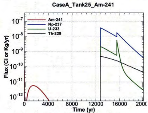
Figure A.1-784 - Flux Leaving Liner for CaseA Tank25 Am-241
