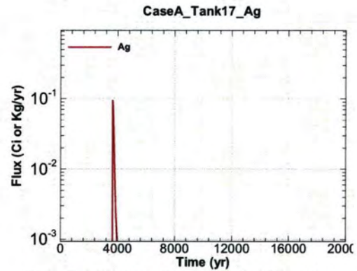
Figure A.1-1406 - Flux Leaving Liner for CaseA Tank17 Ag
