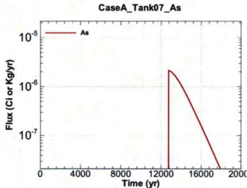
Figure A.1-475 - Flux Leaving Liner for CaseA Tank07 As
