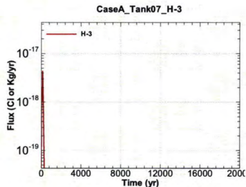
Figure A.1-500 - Flux Leaving Liner for CaseA Tank07 H-3
