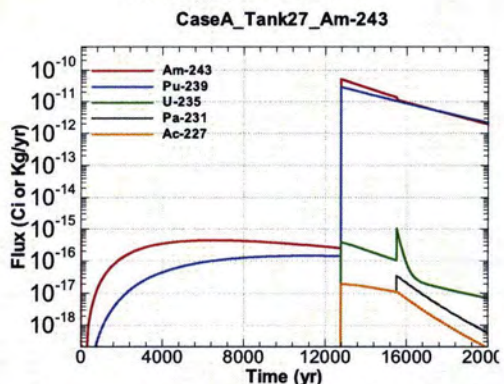
Figure A.1-942 - Flux Leaving Liner for CaseA Tank27 Am-243
