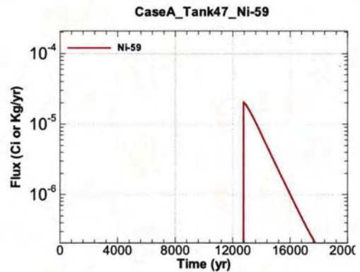
Figure A.1-1366 - Flux Leaving Liner for CaseA Tank47 Ni-59
