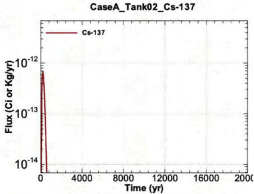
Figure A.1-103 - Flux Leaving Liner for CaseA Tank02 Cs-137
