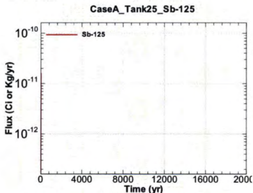
Figure A.1-837 - Flux Leaving Liner for CaseA Tank25 Sb-125
