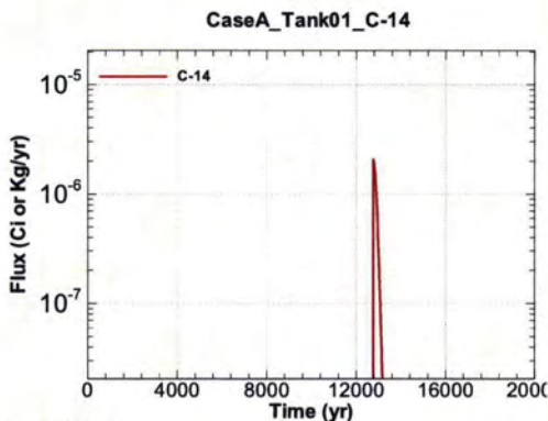
Figure A.1-11 - Flux Leaving Liner for CaseA Tank01 C-14
