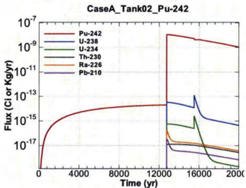
Figure A.1-129 - Flux Leaving Liner for CaseA Tank02 Pu-242
