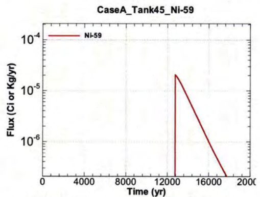
Figure A.1-1210 - Flux Leaving Liner for CaseA Tank45 Ni-59
