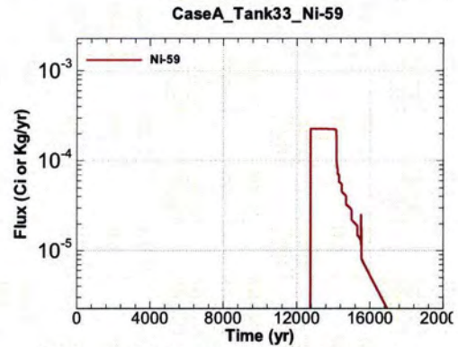
Figure A.1-664 - Flux Leaving Liner for CaseA Tank33 Ni-59
