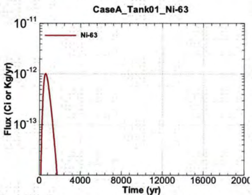
Figure A.1-41 - Flux Leaving Liner for CaseA Tank01 Ni-63
