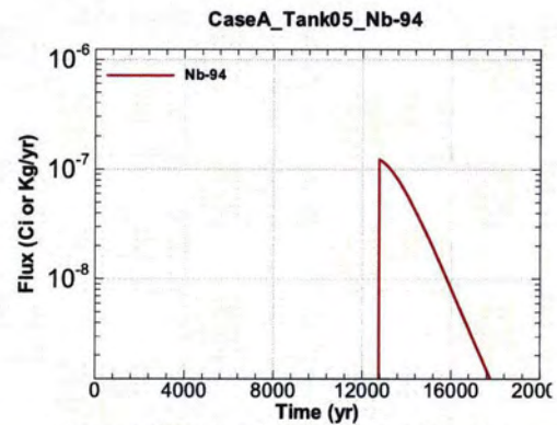
Figure A.1-350 - Flux Leaving Liner for CaseA Tank05 Nb-94
