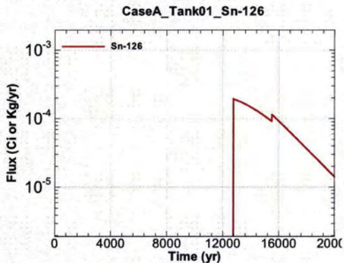
Figure A.1-63 - Flux Leaving Liner for CaseA Tank01 Sn-126
