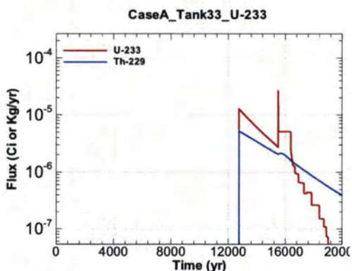
Figure A.1-695 - Flux Leaving Liner for CaseA Tank33 U-233
