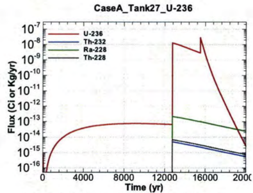
Figure A.1-1010 - Flux Leaving Liner for CaseA Tank27 U-236
