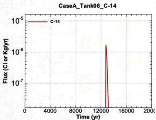
Figure A.1-401 - Flux Leaving Liner for CaseA Tank06 C-14
