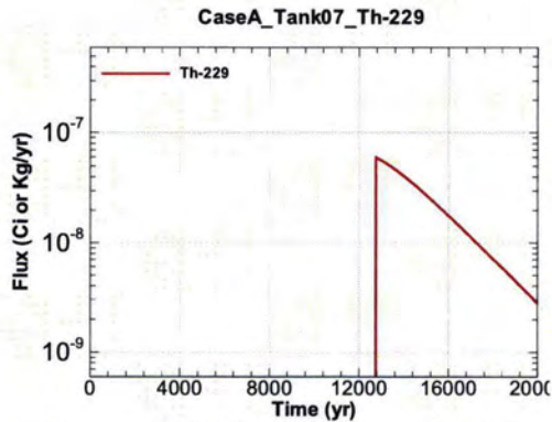
Figure A.1-535 - Flux Leaving Liner for CaseA Tank07 Th-229
