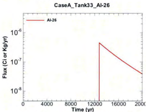
Figure A.1-627 - Flux Leaving Liner for CaseA Tank33 Al-26
