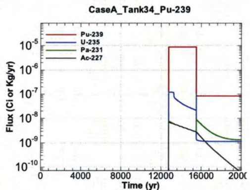
Figure A.1-750 - Flux Leaving Liner for CaseA Tank34 Pu-239
