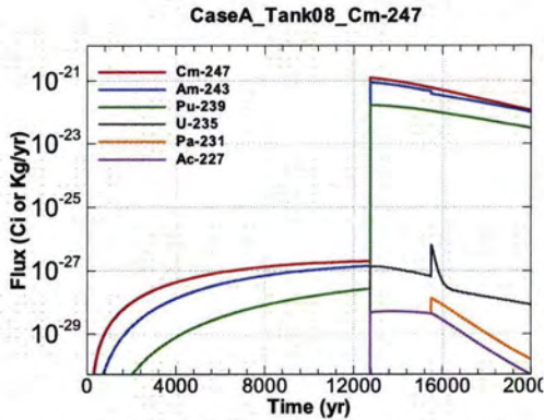
Figure A.1-565 - Flux Leaving Liner for CaseA Tank08 Cm-247
