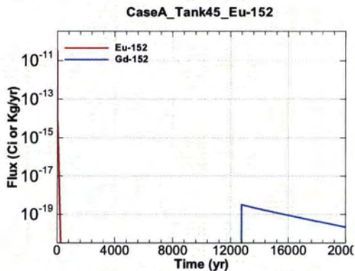
Figure A.1-1197 - Flux Leaving Liner for CaseA Tank45 Eu-152
