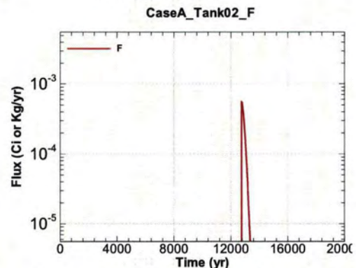
Figure A.1-108 - Flux Leaving Liner for CaseA Tank02 F
