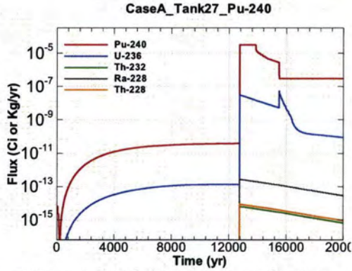
Figure A.1-985 - Flux Leaving Liner for CaseA Tank27 Pu-240
