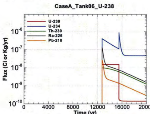
Figure A.1-465 - Flux Leaving Liner for CaseA Tank06 U-238
