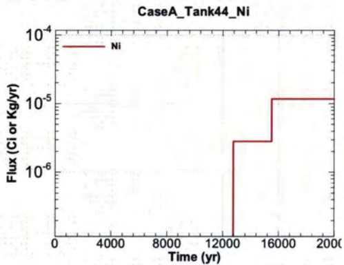
Figure A.1-1131 - Flux Leaving Liner for CaseA Tank44 Ni
