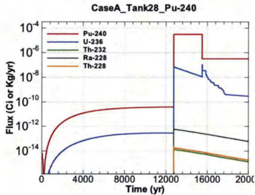
Figure A.1-1063 - Flux Leaving Liner for CaseA Tank28 Pu-240
