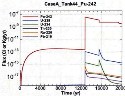
Figure A.1-1143 - Flux Leaving Liner for CaseA Tank44 Pu-242
