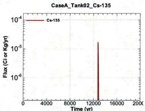
Figure A.1-102 - Flux Leaving Liner for CaseA Tank02 Cs-135
