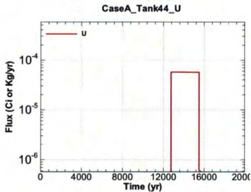
Figure A.1-1161 - Flux Leaving Liner for CaseA Tank44 U
