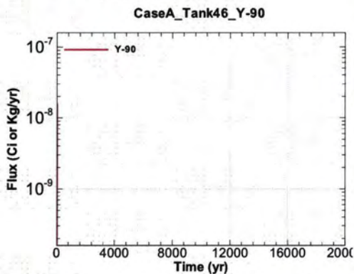
Figure A.1-1325 - Flux Leaving Liner for CaseA Tank46 Y-90
