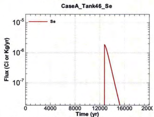
Figure A.1-1308 - Flux Leaving Liner for CaseA Tank46 Se
