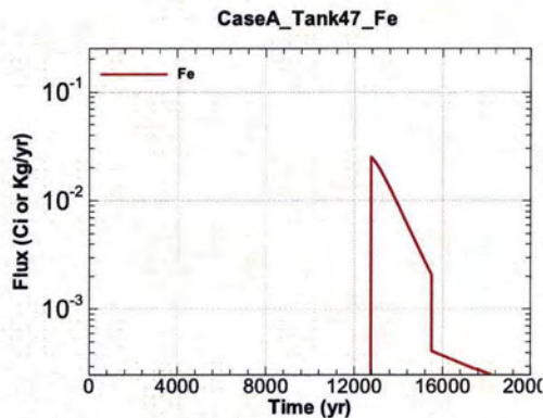
Figure A.1-1357 - Flux Leaving Liner for CaseA Tank47 Fe
