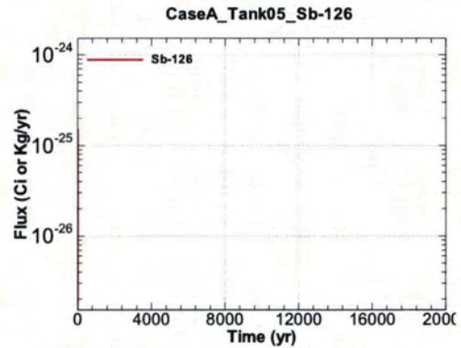
Figure A.1-370 - Flux Leaving Liner for CaseA Tank05 Sb-126
