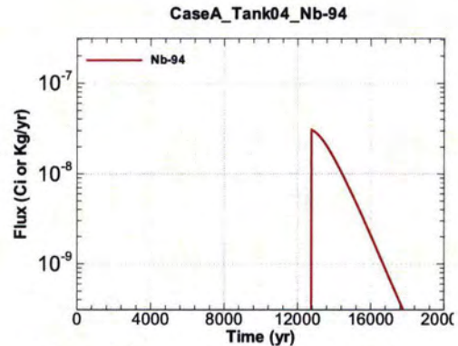
Figure A.1-272 - Flux Leaving Liner for CaseA Tank04 Nb-94
