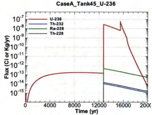
Figure A.1-1244 - Flux Leaving Liner for CaseA Tank45 U-236
