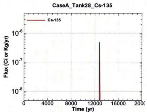
Figure A.1-1038 - Flux Leaving Liner for CaseA Tank28 Cs-135
