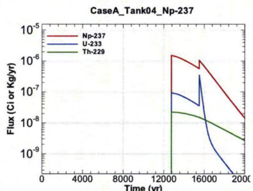
Figure A.1-276 - Flux Leaving Liner for CaseA Tank04 Np-237
