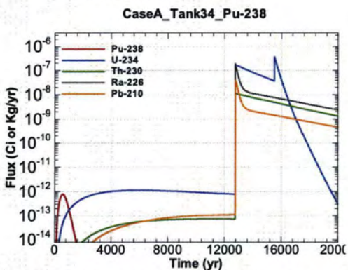
Figure A.1-749 - Flux Leaving Liner for CaseA Tank34 Pu-238
