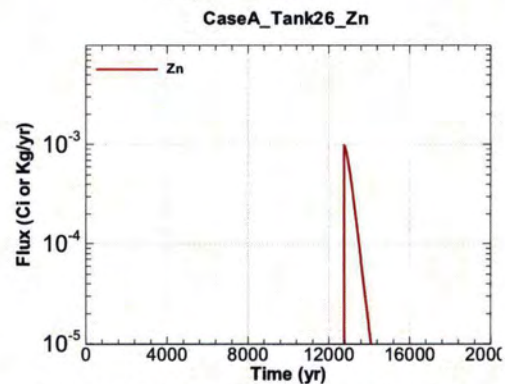
Figure A.1-936 - Flux Leaving Liner for CaseA Tank26 Zn
