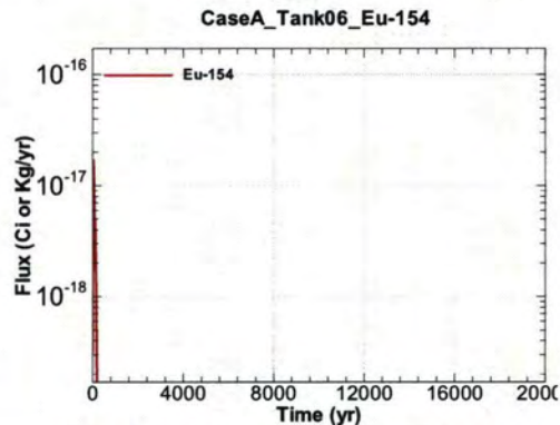
Figure A.1-418 - Flux Leaving Liner for CaseA Tank06 Eu-154
