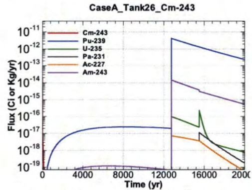
Figure A.1-874 - Flux Leaving Liner for CaseA Tank26 Cm-243
