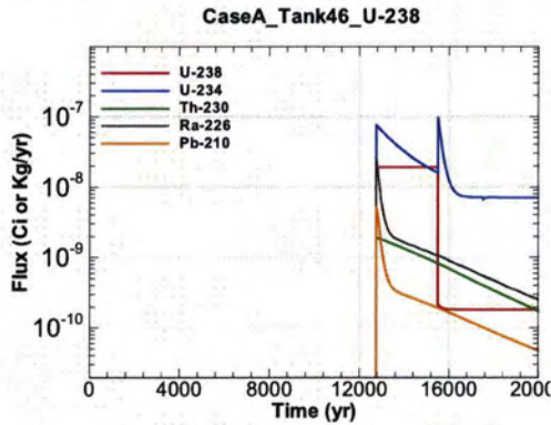
Figure A.1-1323 - Flux Leaving Liner for CaseA Tank46 U-238
