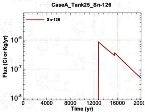
Figure A.1-843 - Flux Leaving Liner for CaseA Tank25 Sn-126
