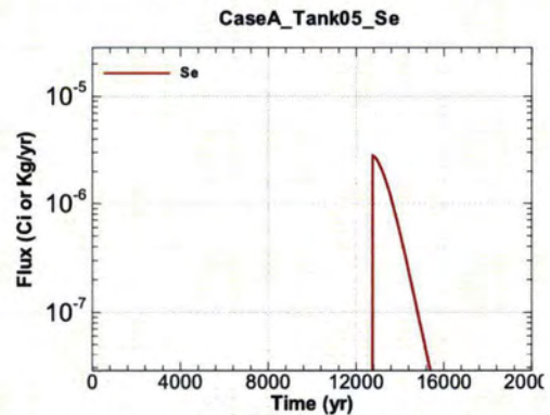
Figure A.1-372 - Flux Leaving Liner for CaseA Tank05 Se
