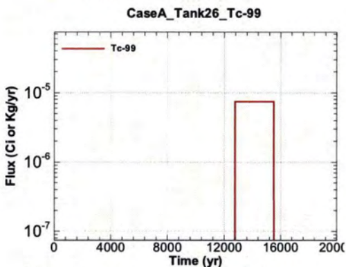
Figure A.1-923 - Flux Leaving Liner for CaseA Tank26 Tc-99
