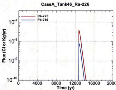
Figure A.1-1301 - Flux Leaving Liner for CaseA Tank46 Ra-226
