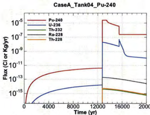
Figure A.1-283 - Flux Leaving Liner for CaseA Tank04 Pu-240
