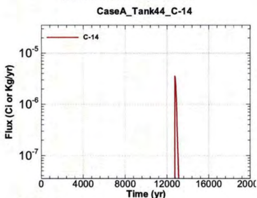
Figure A.1-1103 - Flux Leaving Liner for CaseA Tank44 C-14
