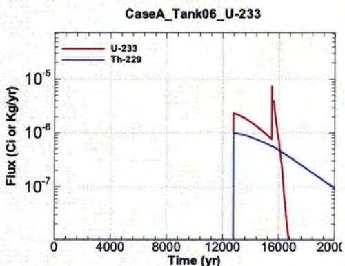
Figure A.1-461 - Flux Leaving Liner for CaseA Tank06 U-233
