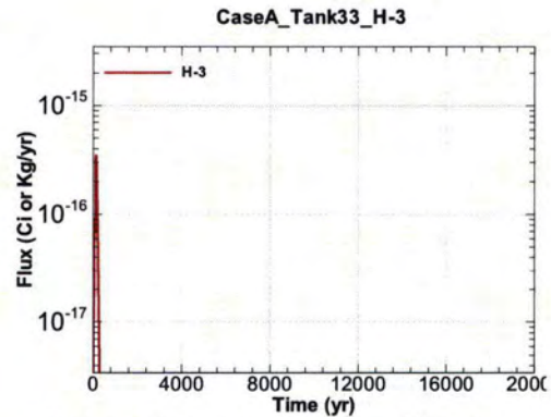
Figure A.1-656 - Flux Leaving Liner for CaseA Tank33 H-3
