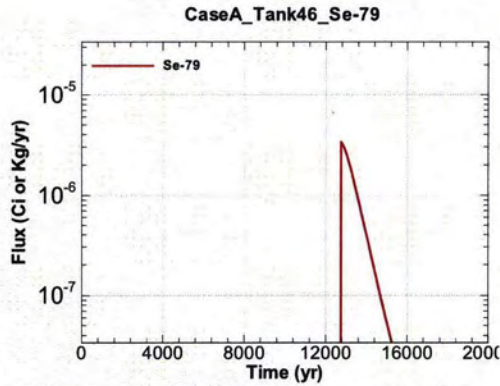
Figure A.1-1309 - Flux Leaving Liner for CaseA Tank46 Se-79
