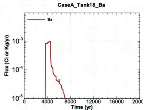
Figure A.1-1490 - Flux Leaving Liner for CaseA Tank18 Ba
