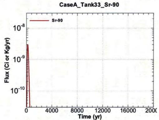
Figure A.1-688 - Flux Leaving Liner for CaseA Tank33 Sr-90
