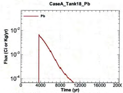
Figure A.1-1526 - Flux Leaving Liner for CaseA Tank18 Pb
