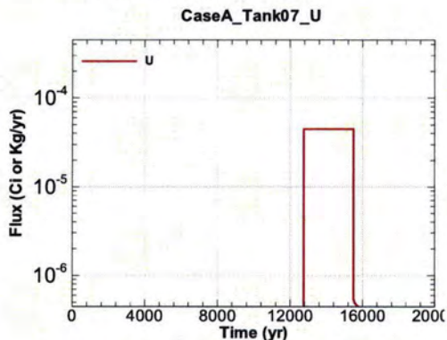
Figure A.1-537 - Flux Leaving Liner for CaseA Tank07 U
