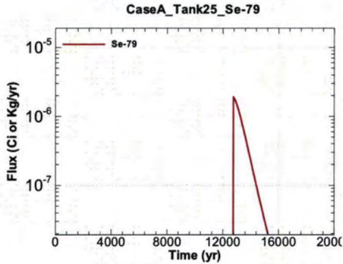
Figure A.1-841 - Flux Leaving Liner for CaseA Tank25 Se-79
