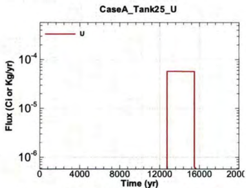
Figure A.1-849 - Flux Leaving Liner for CaseA Tank25 U
