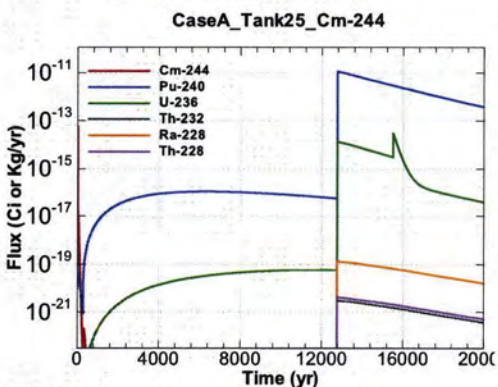
Figure A.1-797 - Flux Leaving Liner for CaseA Tank25 Cm-244
