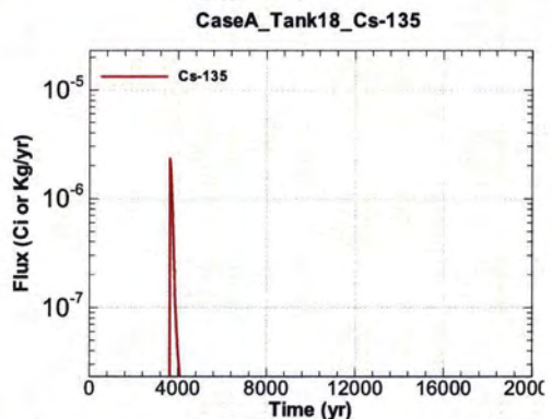
Figure A.1-1506 - Flux Leaving Liner for CaseA Tank18 Cs-135
