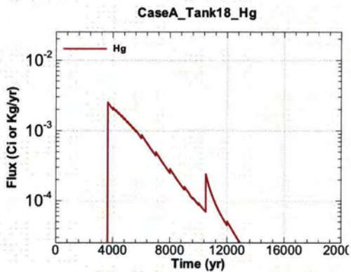
Figure A.1-1515 - Flux Leaving Liner for CaseA Tank18 Hg
