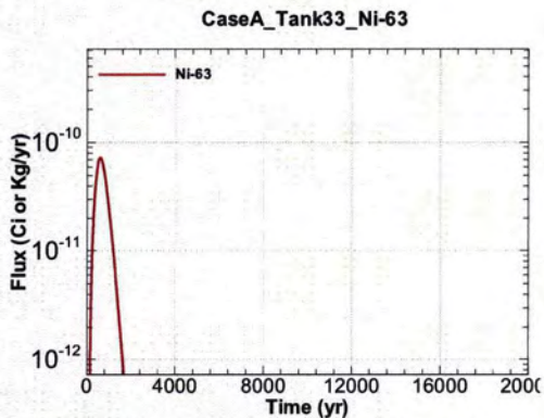
Figure A.1-665 - Flux Leaving Liner for CaseA Tank33 Ni-63
