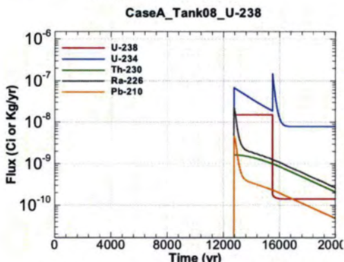
Figure A.1-621 - Flux Leaving Liner for CaseA Tank08 U-238
