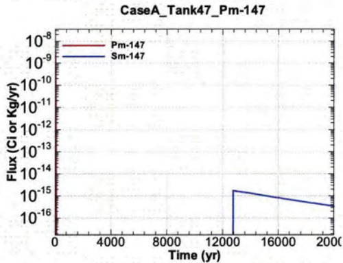
Figure A.1-1371 - Flux Leaving Liner for CaseA Tank47 Pm-147
