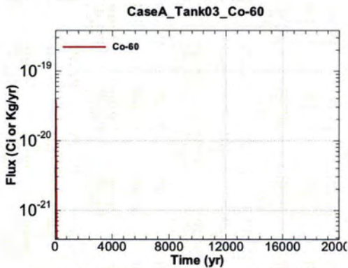
Figure A.1-177 - Flux Leaving Liner for CaseA Tank03 Co-60
