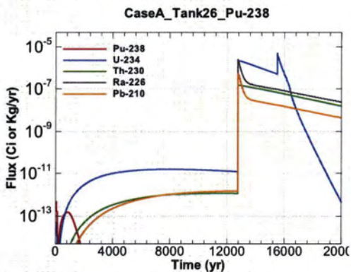
Figure A.1-905 - Flux Leaving Liner for CaseA Tank26 Pu-238
