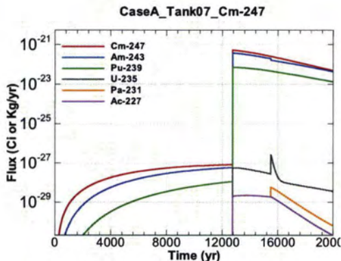
Figure A.1-487 - Flux Leaving Liner for CaseA Tank07 Cm-247
