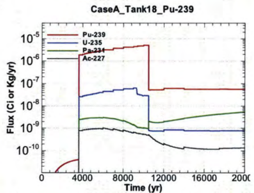
Figure A.1-1530 - Flux Leaving Liner for CaseA Tank18 Pu-239
