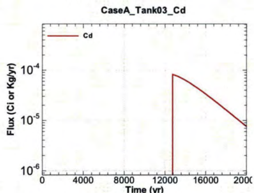
Figure A.1-168 - Flux Leaving Liner for CaseA Tank03 Cd
