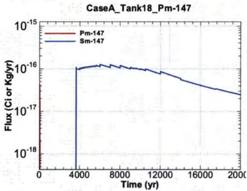
Figure A.1-1527 - Flux Leaving Liner for CaseA Tank18 Pm-147
