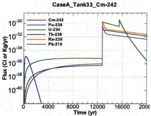
Figure A.1-639 - Flux Leaving Liner for CaseA Tank33 Cm-242
