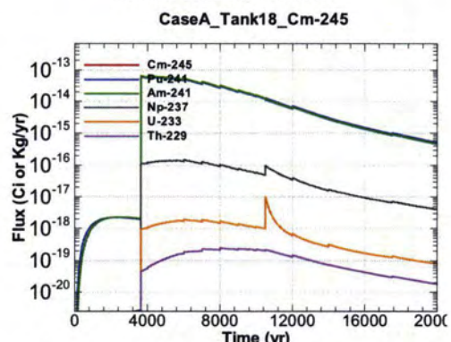
Figure A.1-1500 - Flux Leaving Liner for CaseA Tank18 Cm-245
