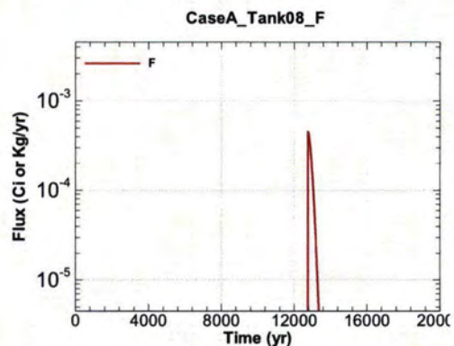
Figure A.1-576 - Flux Leaving Liner for CaseA Tank08 F
