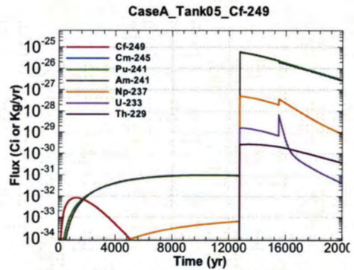
Figure A.1-326 - Flux Leaving Liner for CaseA Tank05 Cf-249
