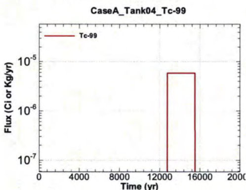
Figure A.1-299 - Flux Leaving Liner for CaseA Tank04 Tc-99
