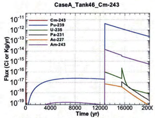
Figure A.1-1264 - Flux Leaving Liner for CaseA Tank46 Cm-243
