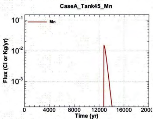
Figure A.1-1205 - Flux Leaving Liner for CaseA Tank45 Mn
