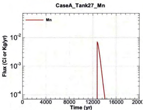
Figure A.1-971 - Flux Leaving Liner for CaseA Tank27 Mn
