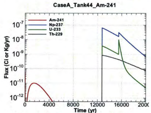
Figure A.1-1096 - Flux Leaving Liner for CaseA Tank44 Am-241
