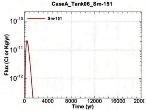
Figure A.1-452 - Flux Leaving Liner for CaseA Tank06 Sm-151
