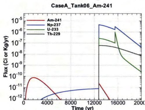
Figure A.1-394 - Flux Leaving Liner for CaseA Tank06 Am-241
