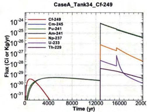
Figure A.1-716 - Flux Leaving Liner for CaseA Tank34 Cf-249
