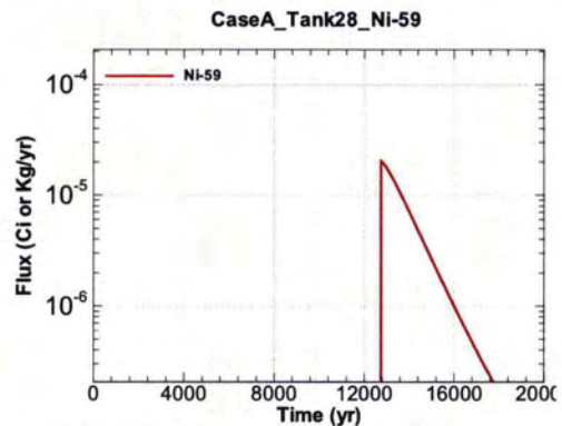
Figure A.1-1054 - Flux Leaving Liner for CaseA Tank28 Ni-59
