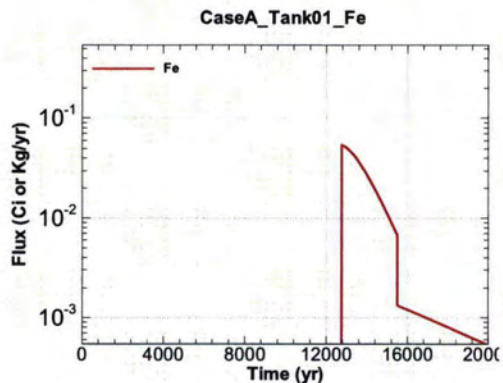
Figure A.1-31 - Flux Leaving Liner for CaseA Tank01 Fe
