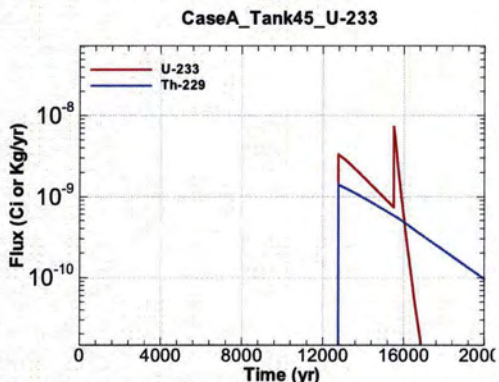
Figure A.1-1241 - Flux Leaving Liner for CaseA Tank45 U-233
