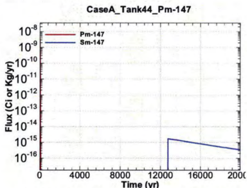
Figure A.1-1137 - Flux Leaving Liner for CaseA Tank44 Pm-147
