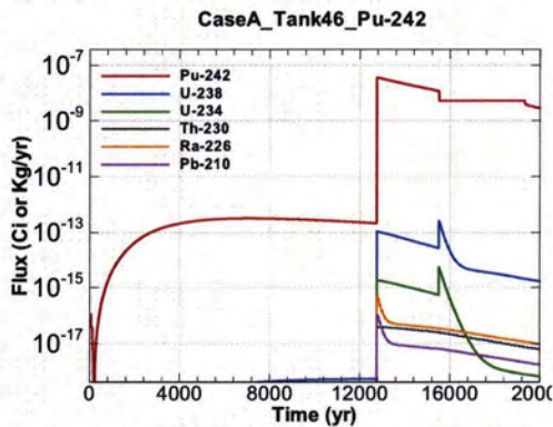
Figure A.1-1299 - Flux Leaving Liner for CaseA Tank46 Pu-242
