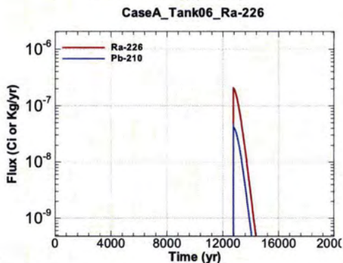
Figure A.1-443 - Flux Leaving Liner for CaseA Tank06 Ra-226
