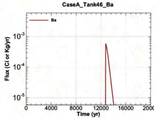
Figure A.1-1256 - Flux Leaving Liner for CaseA Tank46 Ba
