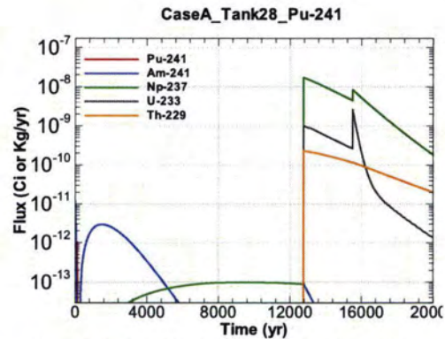
Figure A.1-1064 - Flux Leaving Liner for CaseA Tank28 Pu-241
