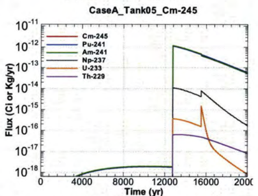
Figure A.1-330 - Flux Leaving Liner for CaseA Tank05 Cm-245
