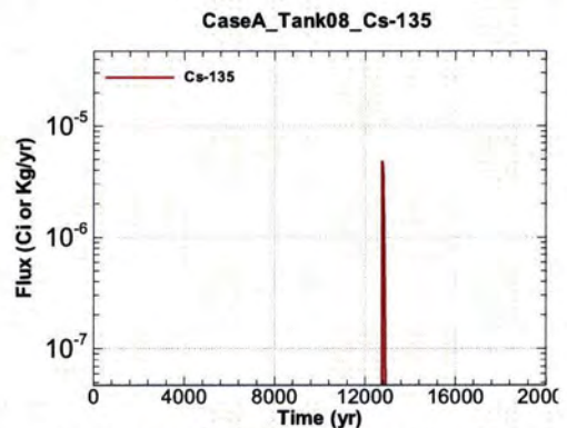
Figure A.1-570 - Flux Leaving Liner for CaseA Tank08 Cs-135
