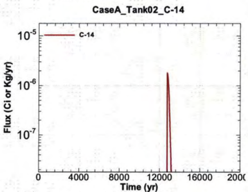
Figure A.1-89 - Flux Leaving Liner for CaseA Tank02 C-14
