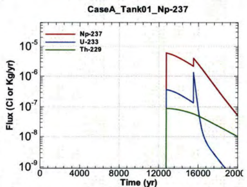
Figure A.1-42 - Flux Leaving Liner for CaseA Tank01 Np-237
