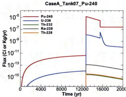
Figure A.1-517 - Flux Leaving Liner for CaseA Tank07 Pu-240
