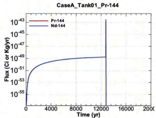
Figure A.1-46 - Flux Leaving Liner for CaseA Tank01 Pr-144
