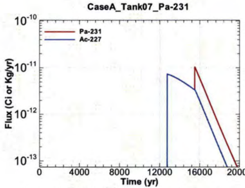
Figure A.1-511 - Flux Leaving Liner for CaseA Tank07 Pa-231
