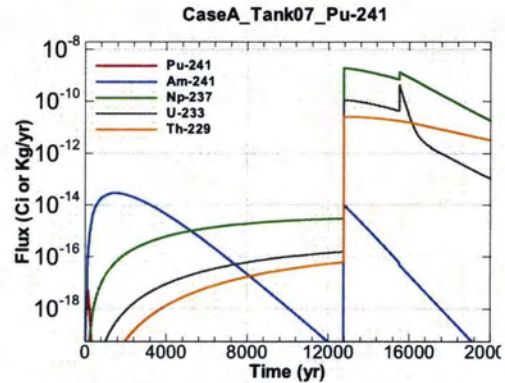
Figure A.1-518 - Flux Leaving Liner for CaseA Tank07 Pu-241
