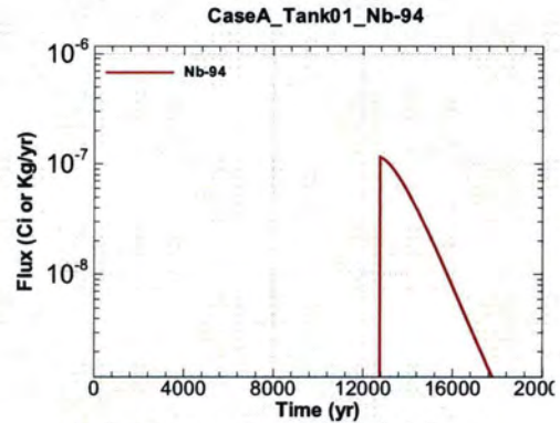
Figure A.1-38 - Flux Leaving Liner for CaseA Tank01 Nb-94
