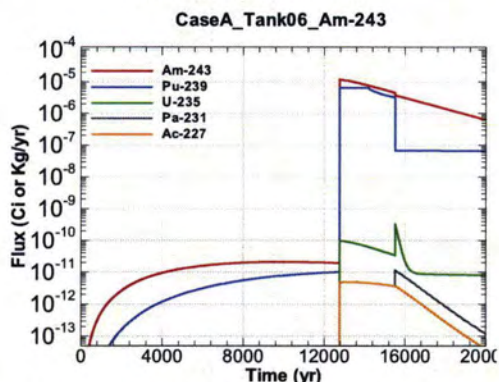
Figure A.1-396 - Flux Leaving Liner for CaseA Tank06 Am-243
