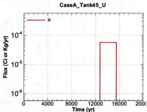
Figure A.1-1239 - Flux Leaving Liner for CaseA Tank45 U
