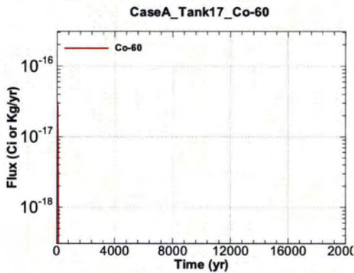
Figure A.1-1425 - Flux Leaving Liner for CaseA Tank17 Co-60
