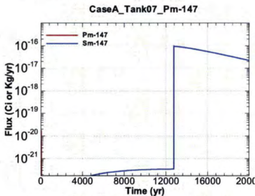
Figure A.1-513 - Flux Leaving Liner for CaseA Tank07 Pm-147
