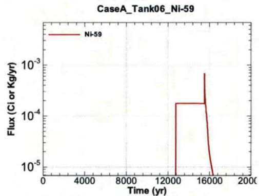
Figure A.1-430 - Flux Leaving Liner for CaseA Tank06 Ni-59
