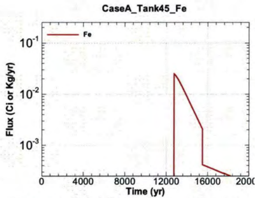
Figure A.1-1201 - Flux Leaving Liner for CaseA Tank45 Fe
