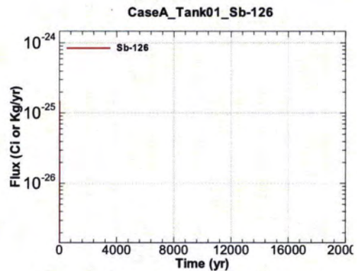
Figure A.1-58 - Flux Leaving Liner for CaseA Tank01 Sb-126
