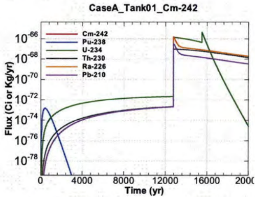
Figure A.1-15 - Flux Leaving Liner for CaseA Tank01 Cm-242
