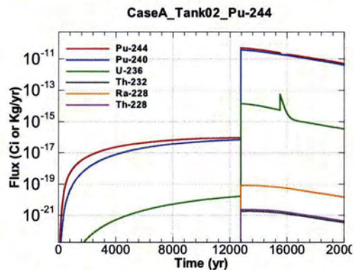
Figure A.1-130 - Flux Leaving Liner for CaseA Tank02 Pu-244
