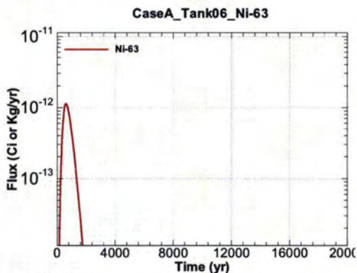
Figure A.1-431 - Flux Leaving Liner for CaseA Tank06 Ni-63
