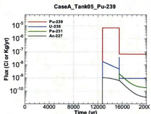
Figure A.1-360 - Flux Leaving Liner for CaseA Tank05 Pu-239
