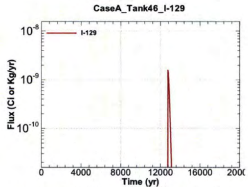
Figure A.1-1282 - Flux Leaving Liner for CaseA Tank46 I-129
