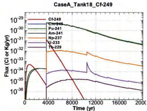
Figure A.1-1496 - Flux Leaving Liner for CaseA Tank18 Cf-249
