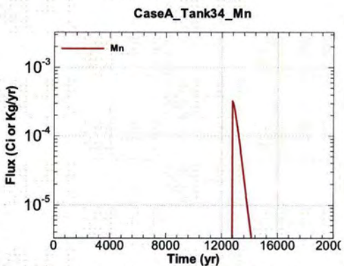
Figure A.1-737 - Flux Leaving Liner for CaseA Tank34 Mn
