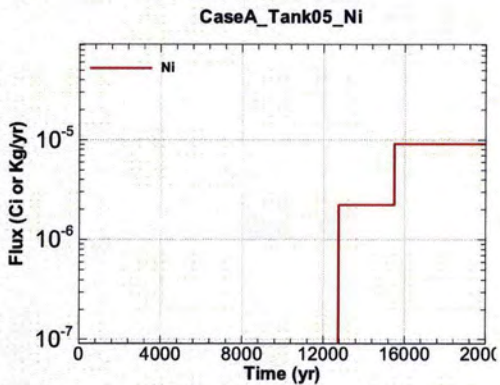
Figure A.1-351 - Flux Leaving Liner for CaseA Tank05 Ni
