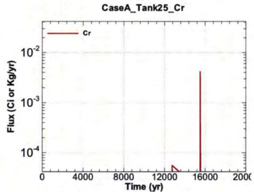
Figure A.1-802 - Flux Leaving Liner for CaseA Tank25 Cr
