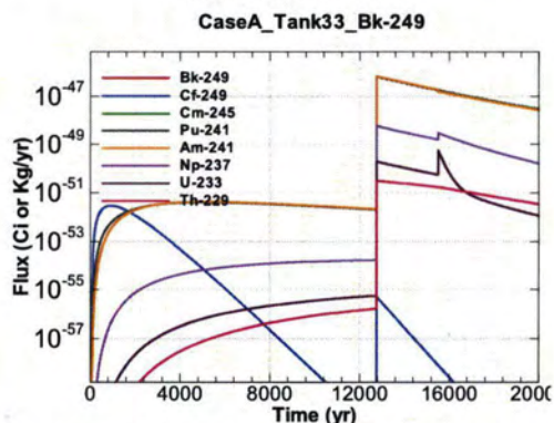
Figure A.1-634 - Flux Leaving Liner for CaseA Tank33 Bk-249
