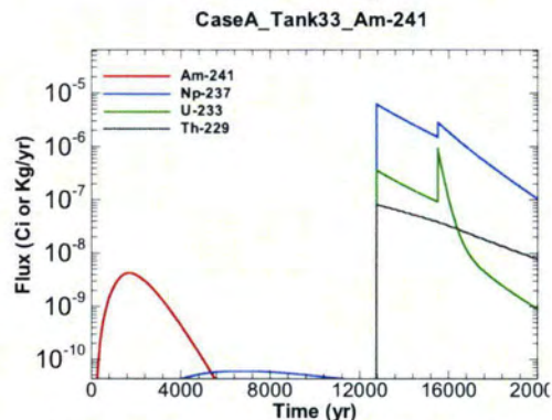
Figure A.1-628 - Flux Leaving Liner for CaseA Tank33 Am-241
