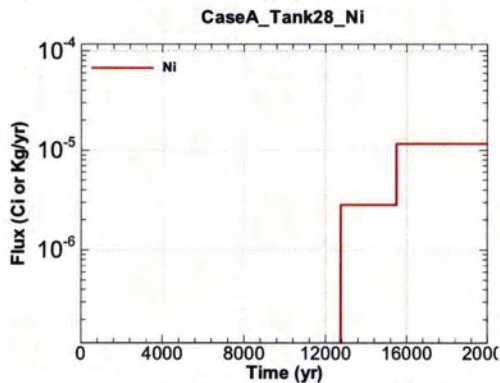
Figure A.1-1053 - Flux Leaving Liner for CaseA Tank28 Ni
