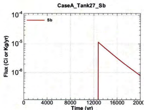
Figure A.1-992 - Flux Leaving Liner for CaseA Tank27 Sb
