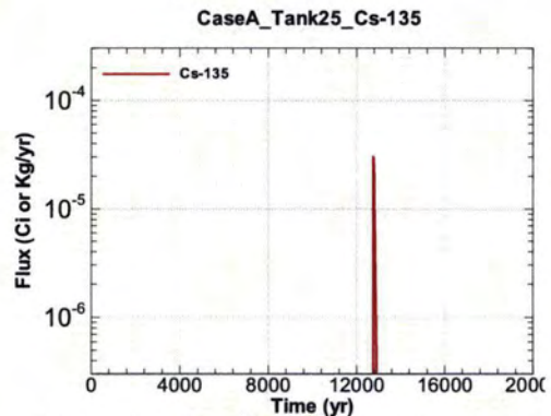
Figure A.1-804 - Flux Leaving Liner for CaseA Tank25 Cs-135
