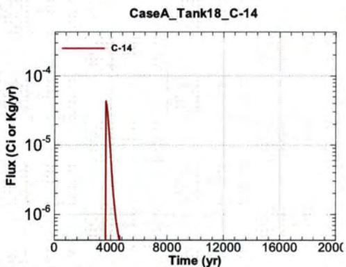
Figure A.1-1493 - Flux Leaving Liner for CaseA Tank18 C-14
