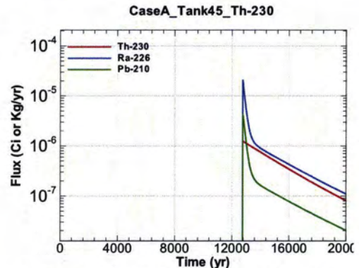
Figure A.1-1238 - Flux Leaving Liner for CaseA Tank45 Th-230
