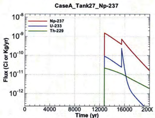
Figure A.1-978 - Flux Leaving Liner for CaseA Tank27 Np-237
