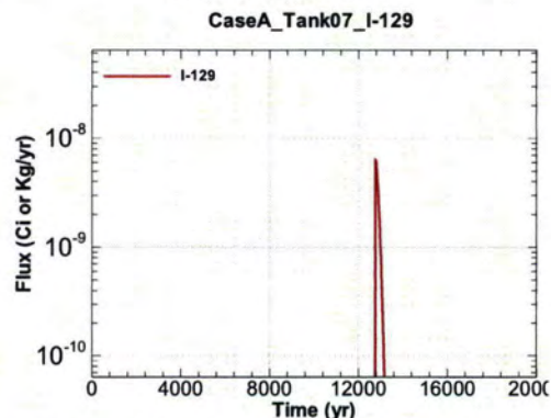
Figure A.1-502 - Flux Leaving Liner for CaseA Tank07 I-129
