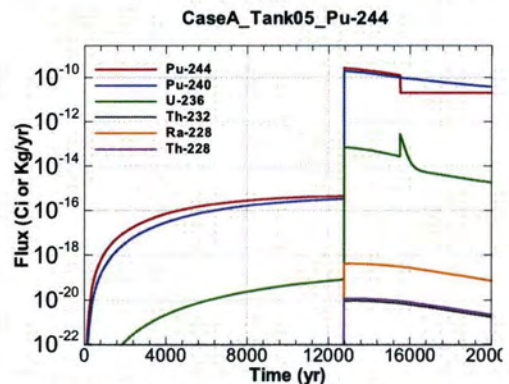
Figure A.1-364 - Flux Leaving Liner for CaseA Tank05 Pu-244
