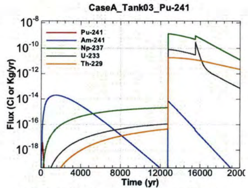
Figure A.1-206 - Flux Leaving Liner for CaseA Tank03 Pu-241
