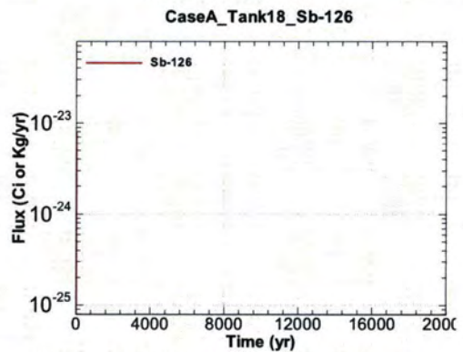
Figure A.1-1540 - Flux Leaving Liner for CaseA Tank18 Sb-126
