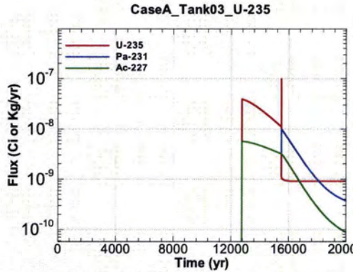
Figure A.1-229 - Flux Leaving Liner for CaseA Tank03 U-235
