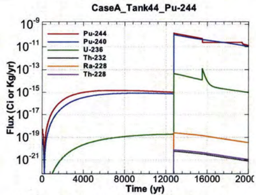
Figure A.1-1144 - Flux Leaving Liner for CaseA Tank44 Pu-244
