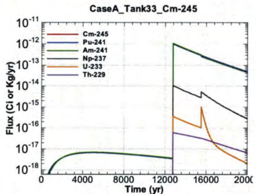
Figure A.1-642 - Flux Leaving Liner for CaseA Tank33 Cm-245
