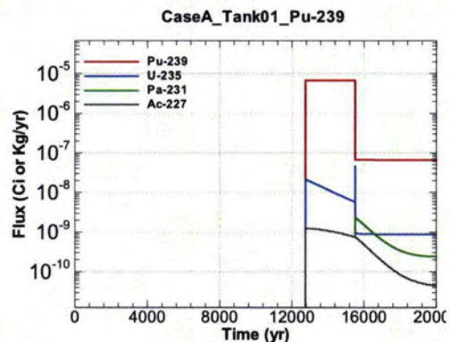
Figure A.1-48 - Flux Leaving Liner for CaseA Tank01 Pu-239
