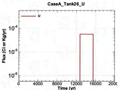
Figure A.1-927 - Flux Leaving Liner for CaseA Tank26 U
