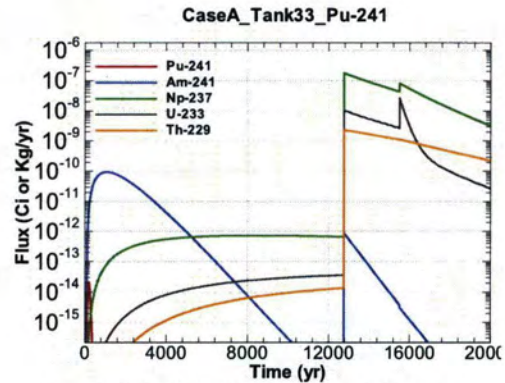
Figure A.1-674 - Flux Leaving Liner for CaseA Tank33 Pu-241
