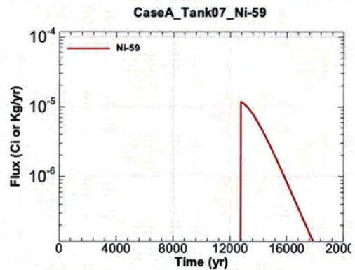
Figure A.1-508 - Flux Leaving Liner for CaseA Tank07 Ni-59
