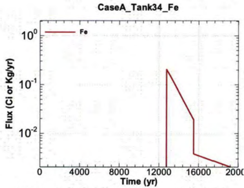
Figure A.1-733 - Flux Leaving Liner for CaseA Tank34 Fe
