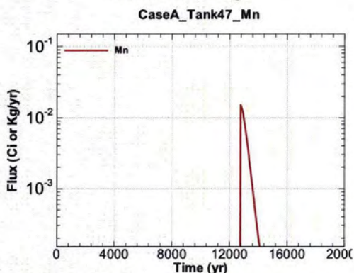
Figure A.1-1361 - Flux Leaving Liner for CaseA Tank47 Mn
