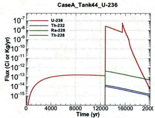
Figure A.1-1166 - Flux Leaving Liner for CaseA Tank44 U-236
