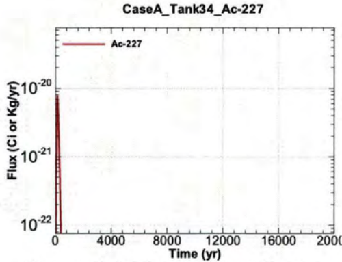
Figure A.1-703 - Flux Leaving Liner for CaseA Tank34 Ac-227
