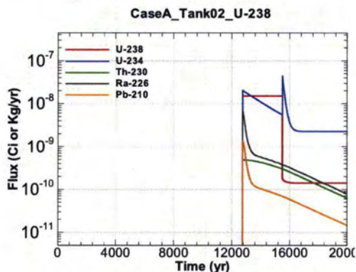
Figure A.1-153 - Flux Leaving Liner for CaseA Tank02 U-238
