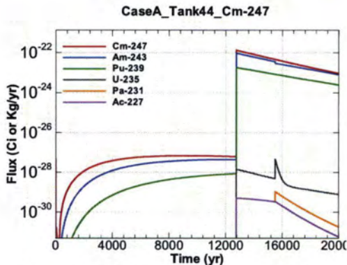
Figure A.1-1111 - Flux Leaving Liner for CaseA Tank44 Cm-247
