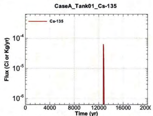
Figure A.1-24 - Flux Leaving Liner for CaseA Tank01 Cs-135
