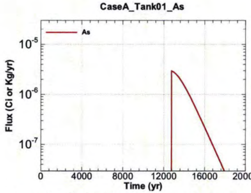
Figure A.1-7 - Flux Leaving Liner for CaseA Tank01 As
