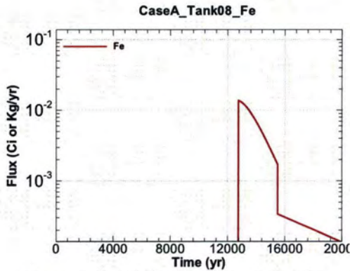
Figure A.1-577 - Flux Leaving Liner for CaseA Tank08 Fe
