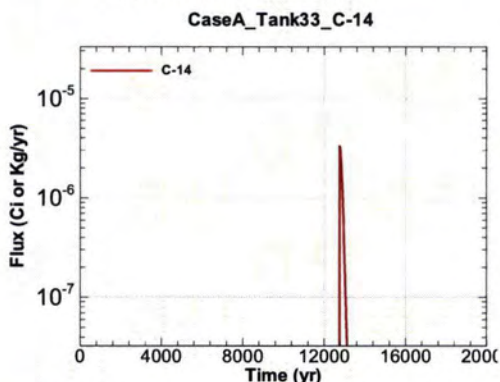
Figure A.1-635 - Flux Leaving Liner for CaseA Tank33 C-14
