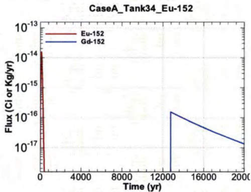
Figure A.1-729 - Flux Leaving Liner for CaseA Tank34 Eu-152
