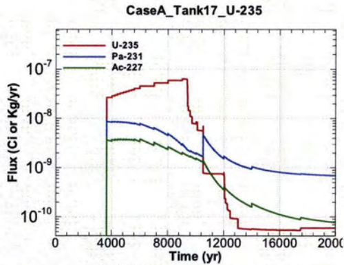
Figure A.1-1477 - Flux Leaving Liner for CaseA Tank17 U-235
