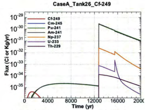
Figure A.1-872 - Flux Leaving Liner for CaseA Tank26 Cf-249
