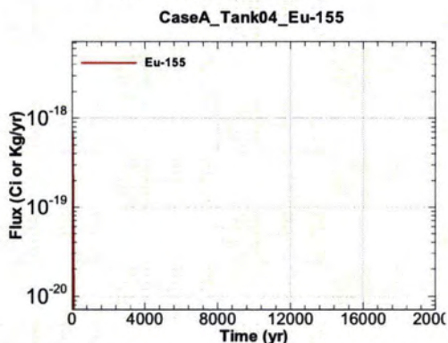
Figure A.1-263 - Flux Leaving Liner for CaseA Tank04 Eu-155
