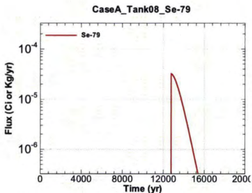
Figure A.1-607 - Flux Leaving Liner for CaseA Tank08 Se-79
