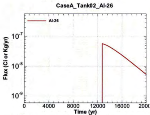
Figure A.1-81 - Flux Leaving Liner for CaseA Tank02 Al-26
