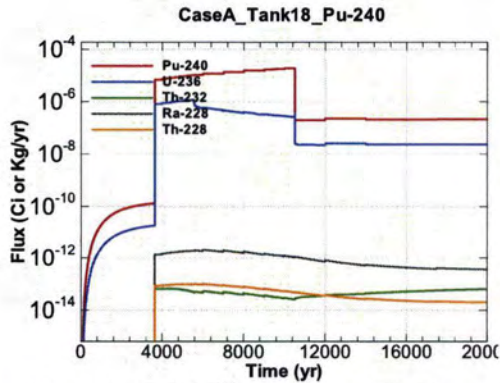
Figure A.1-1531 - Flux Leaving Liner for CaseA Tank18 Pu-240
