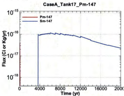
Figure A.1-1449 - Flux Leaving Liner for CaseA Tank17 Pm-147
