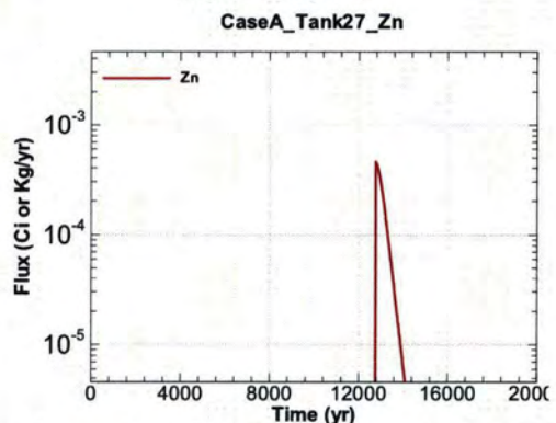
Figure A.1-1014 - Flux Leaving Liner for CaseA Tank27 Zn
