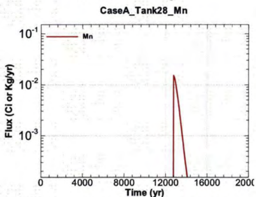
Figure A.1-1049 - Flux Leaving Liner for CaseA Tank28 Mn
