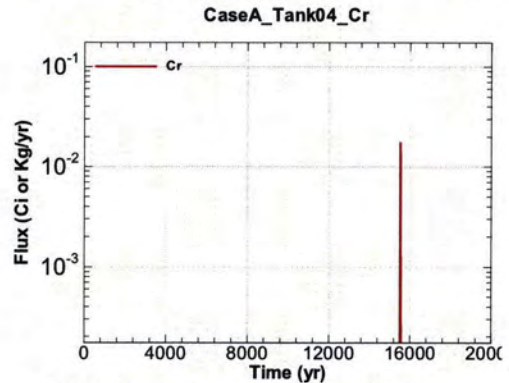
Figure A.1-256 - Flux Leaving Liner for CaseA Tank04 Cr
