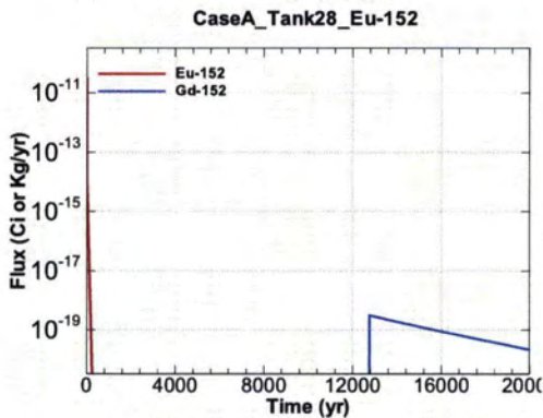
Figure A.1-1041 - Flux Leaving Liner for CaseA Tank28 Eu-152
