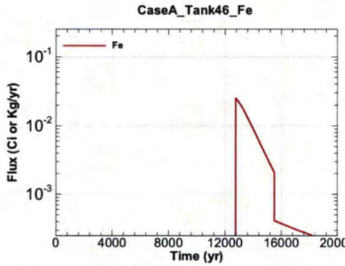
Figure A.1-1279 - Flux Leaving Liner for CaseA Tank46 Fe
