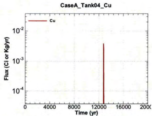
Figure A.1-260 - Flux Leaving Liner for CaseA Tank04 Cu
