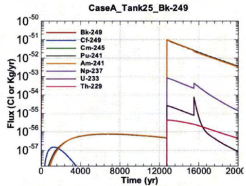
Figure A.1-790 - Flux Leaving Liner for CaseA Tank25 Bk-249
