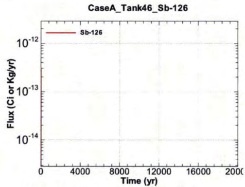
Figure A.1-1306 - Flux Leaving Liner for CaseA Tank46 Sb-126
