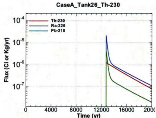
Figure A.1-926 - Flux Leaving Liner for CaseA Tank26 Th-230
