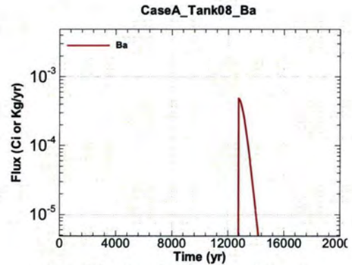
Figure A.1-554 - Flux Leaving Liner for CaseA Tank08 Ba
