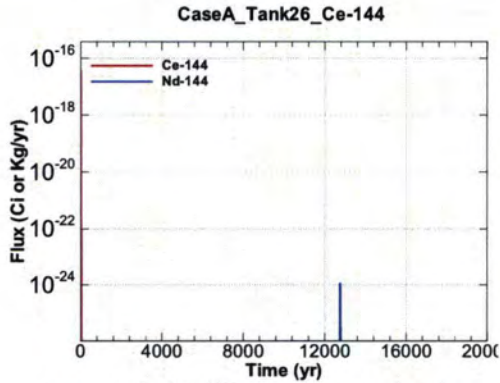
Figure A.1-871 - Flux Leaving Liner for CaseA Tank26 Ce-144
