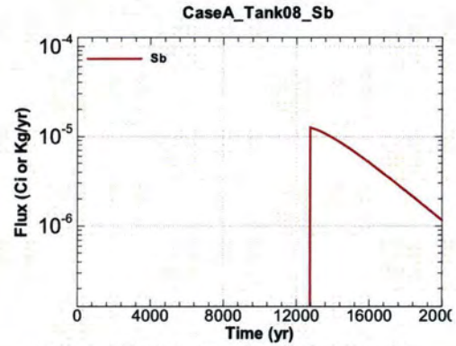
Figure A.1-602 - Flux Leaving Liner for CaseA Tank08 Sb
