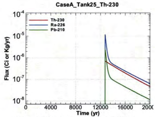
Figure A.1-848 - Flux Leaving Liner for CaseA Tank25 Th-230
