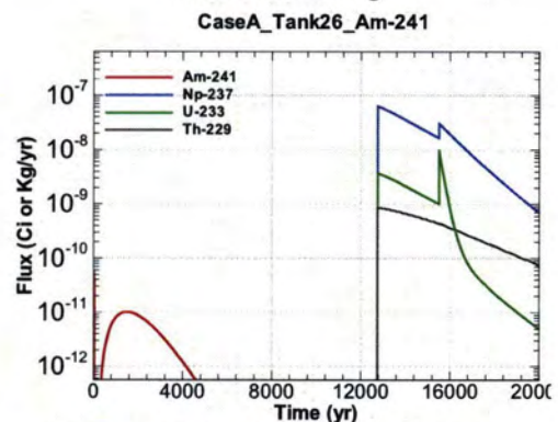
Figure A.1-862 - Flux Leaving Liner for CaseA Tank26 Am-241
