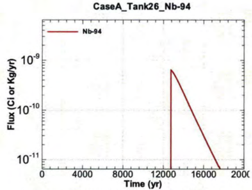
Figure A.1-896 - Flux Leaving Liner for CaseA Tank26 Nb-94
