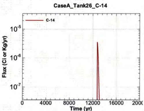
Figure A.1-869 - Flux Leaving Liner for CaseA Tank26 C-14
