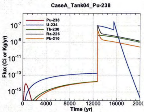
Figure A.1-281 - Flux Leaving Liner for CaseA Tank04 Pu-238
