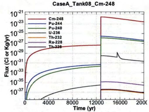
Figure A.1-566 - Flux Leaving Liner for CaseA Tank08 Cm-248
