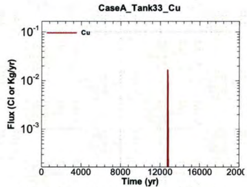
Figure A.1-650 - Flux Leaving Liner for CaseA Tank33 Cu
