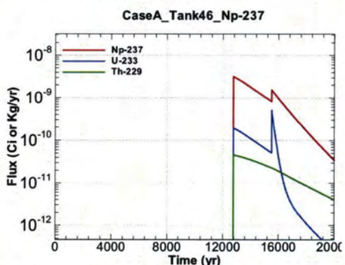
Figure A.1-1290 - Flux Leaving Liner for CaseA Tank46 Np-237
