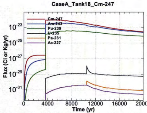
Figure A.1-1501 - Flux Leaving Liner for CaseA Tank18 Cm-247
