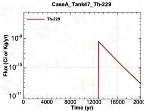
Figure A.1-1393 - Flux Leaving Liner for CaseA Tank47 Th-229
