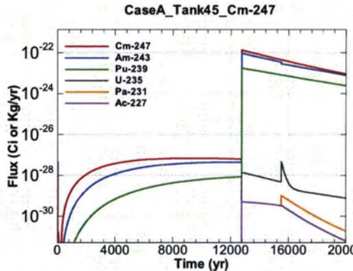
Figure A.1-1189 - Flux Leaving Liner for CaseA Tank45 Cm-247
