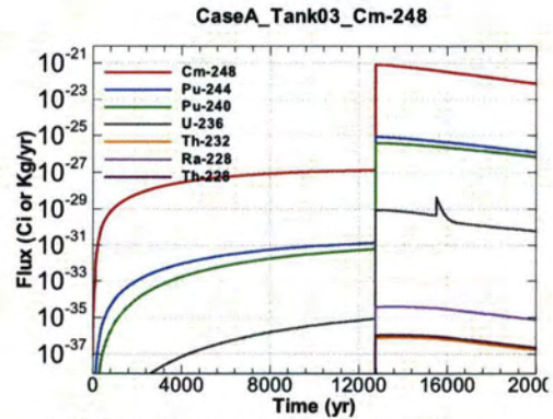
Figure A.1-176 - Flux Leaving Liner for CaseA Tank03 Cm-248
