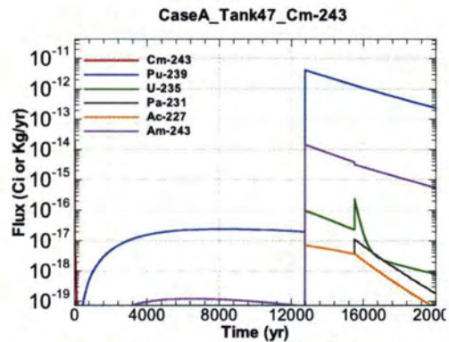
Figure A.1-1342 - Flux Leaving Liner for CaseA Tank47 Cm-243
