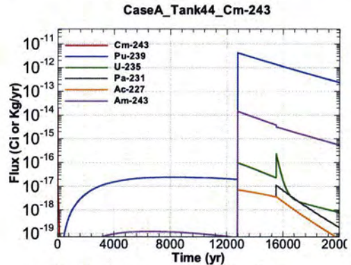
Figure A.1-1108 - Flux Leaving Liner for CaseA Tank44 Cm-243
