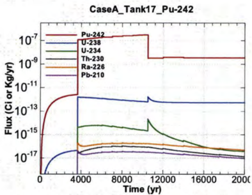
Figure A.1-1455 - Flux Leaving Liner for CaseA Tank17 Pu-242
