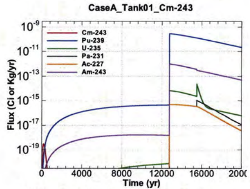
Figure A.1-16 - Flux Leaving Liner for CaseA Tank01 Cm-243
