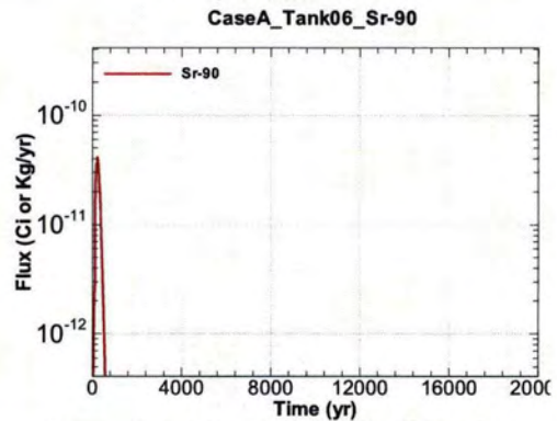
Figure A.1-454 - Flux Leaving Liner for CaseA Tank06 Sr-90
