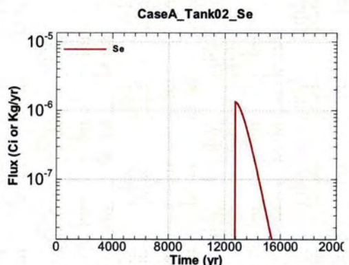
Figure A.1-138 - Flux Leaving Liner for CaseA Tank02 Se
