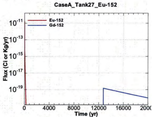
Figure A.1-963 - Flux Leaving Liner for CaseA Tank27 Eu-152
