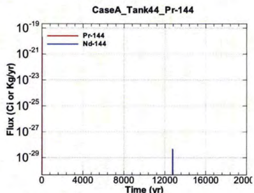
Figure A.1-1138 - Flux Leaving Liner for CaseA Tank44 Pr-144
