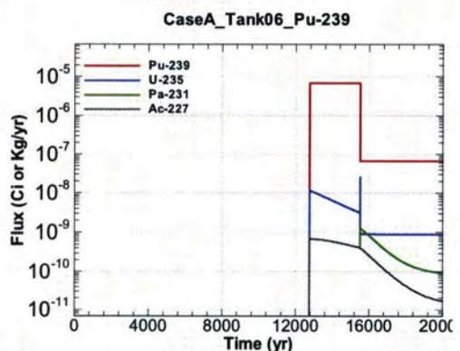
Figure A.1-438 - Flux Leaving Liner for CaseA Tank06 Pu-239
