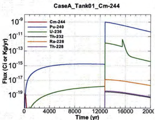
Figure A.1-17 - Flux Leaving Liner for CaseA Tank01 Cm-244
