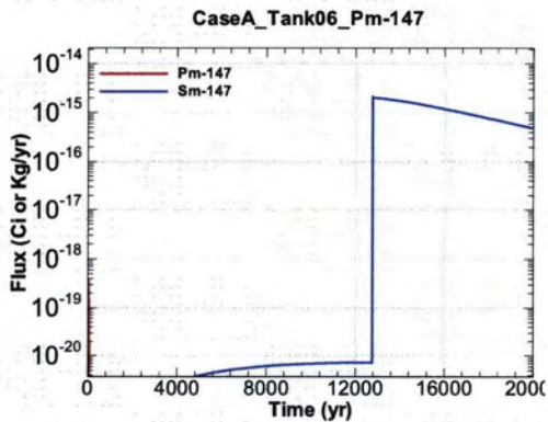
Figure A.1-435 - Flux Leaving Liner for CaseA Tank06 Pm-147
