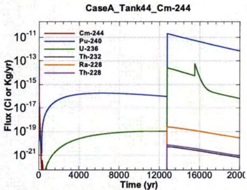
Figure A.1-1109 - Flux Leaving Liner for CaseA Tank44 Cm-244
