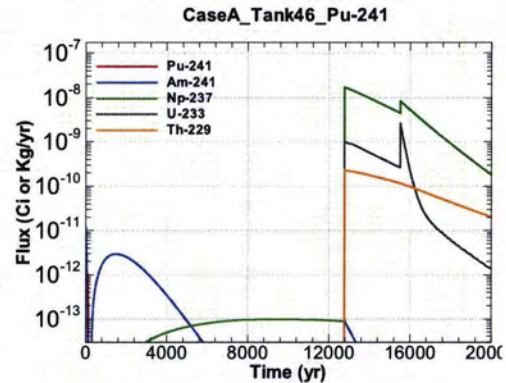
Figure A.1-1298 - Flux Leaving Liner for CaseA Tank46 Pu-241
