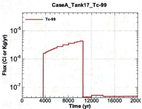
Figure A.1-1469 - Flux Leaving Liner for CaseA Tank17 Tc-99
