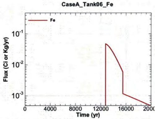
Figure A.1-421 - Flux Leaving Liner for CaseA Tank06 Fe
