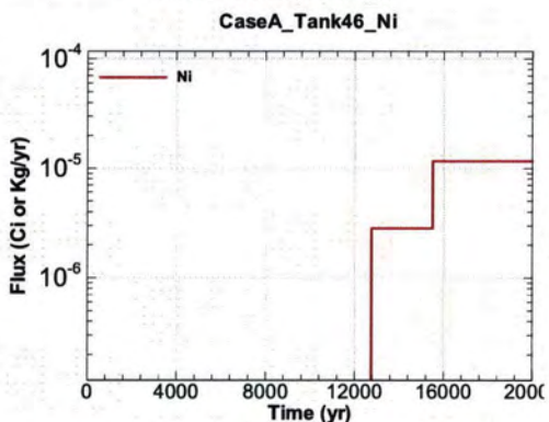
Figure A.1-1287 - Flux Leaving Liner for CaseA Tank46 Ni
