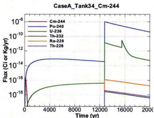
Figure A.1-719 - Flux Leaving Liner for CaseA Tank34 Cm-244
