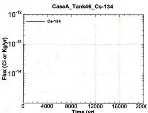
Figure A.1-1271 - Flux Leaving Liner for CaseA Tank46 Cs-134
