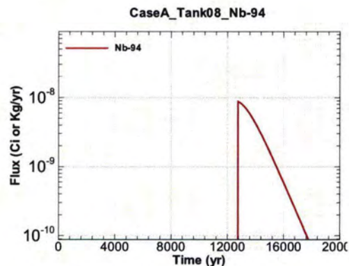
Figure A.1-584 - Flux Leaving Liner for CaseA Tank08 Nb-94
