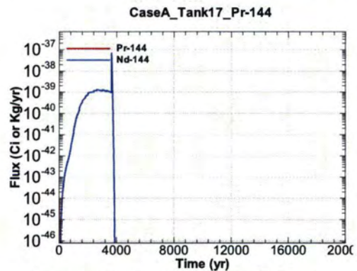
Figure A.1-1450 - Flux Leaving Liner for CaseA Tank17 Pr-144
