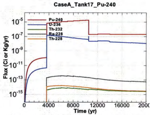
Figure A.1-1453 - Flux Leaving Liner for CaseA Tank17 Pu-240
