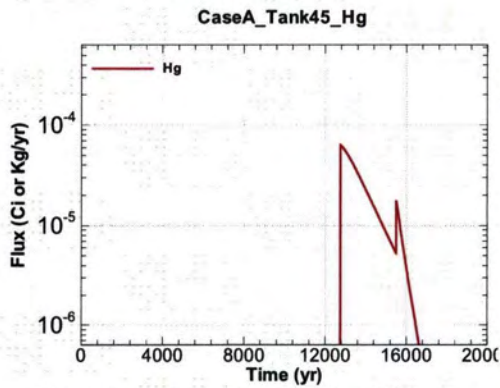
Figure A.1-1203 - Flux Leaving Liner for CaseA Tank45 Hg
