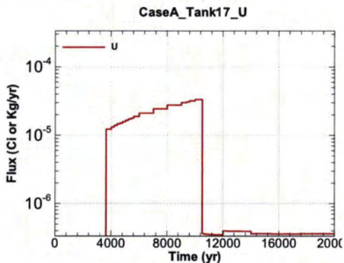
Figure A.1-1473 - Flux Leaving Liner for CaseA Tank17 U
