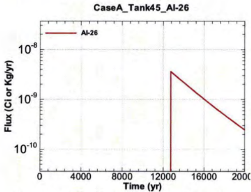
Figure A.1-1173 - Flux Leaving Liner for CaseA Tank45 Al-26
