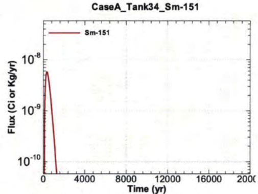
Figure A.1-764 - Flux Leaving Liner for CaseA Tank34 Sm-151
