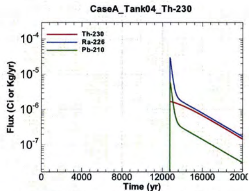
Figure A.1-302 - Flux Leaving Liner for CaseA Tank04 Th-230
