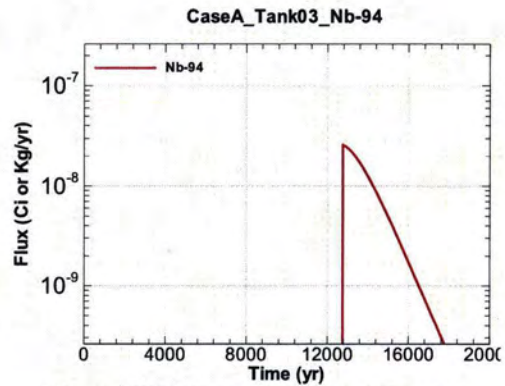
Figure A.1-194 - Flux Leaving Liner for CaseA Tank03 Nb-94
