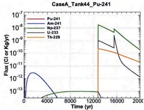
Figure A.1-1142 - Flux Leaving Liner for CaseA Tank44 Pu-241
