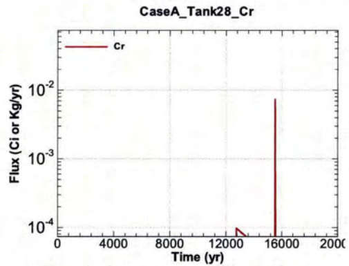
Figure A.1-1036 - Flux Leaving Liner for CaseA Tank28 Cr
