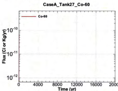
Figure A.1-957 - Flux Leaving Liner for CaseA Tank27 Co-60
