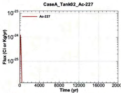
Figure A.1-79 - Flux Leaving Liner for CaseA Tank02 Ac-227
