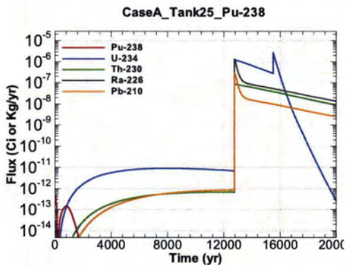
Figure A.1-827 - Flux Leaving Liner for CaseA Tank25 Pu-238
