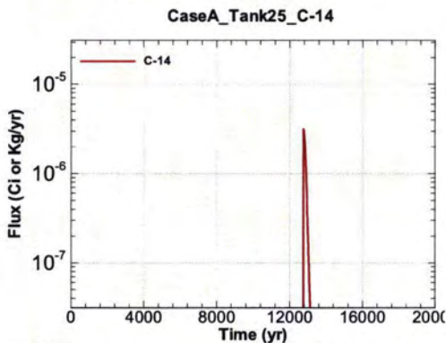
Figure A.1-791 - Flux Leaving Liner for CaseA Tank25 C-14
