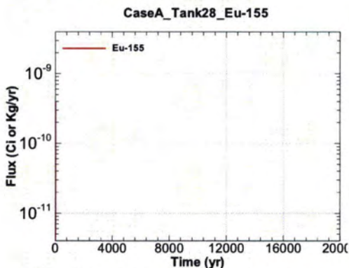
Figure A.1-1043 - Flux Leaving Liner for CaseA Tank28 Eu-155
