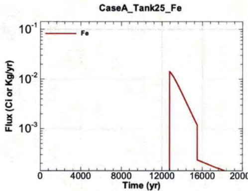
Figure A.1-811 - Flux Leaving Liner for CaseA Tank25 Fe
