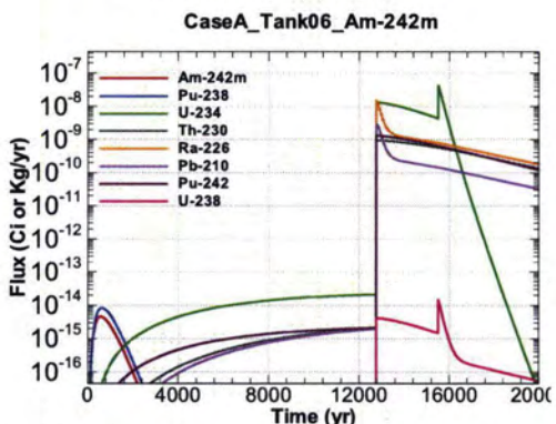
Figure A.1-395 - Flux Leaving Liner for CaseA Tank06 Am-242m
