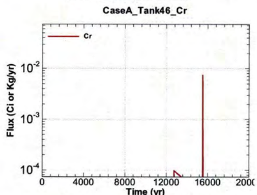
Figure A.1-1270 - Flux Leaving Liner for CaseA Tank46 Cr
