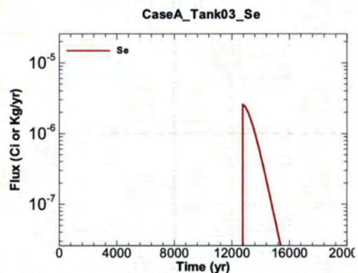
Figure A.1-216 - Flux Leaving Liner for CaseA Tank03 Se
