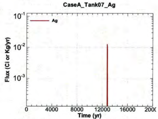
Figure A.1-470 - Flux Leaving Liner for CaseA Tank07 Ag
