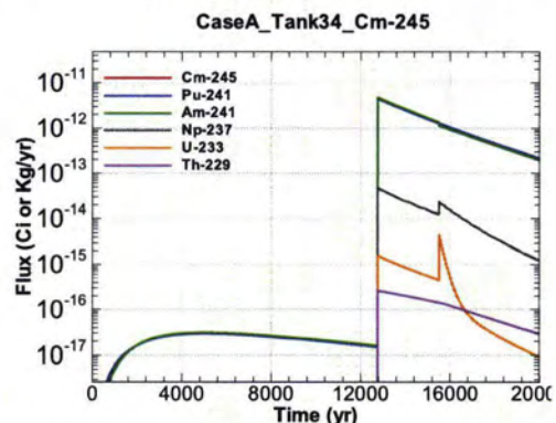
Figure A.1-720 - Flux Leaving Liner for CaseA Tank34 Cm-245
