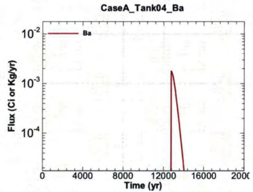
Figure A.1-242 - Flux Leaving Liner for CaseA Tank04 Ba
