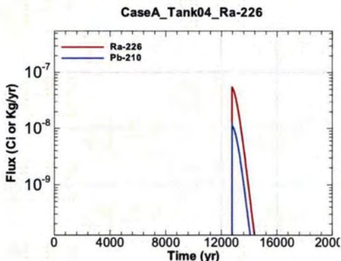
Figure A.1-287 - Flux Leaving Liner for CaseA Tank04 Ra-226
