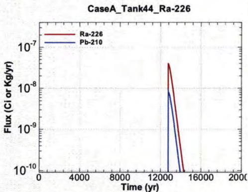
Figure A.1-1145 - Flux Leaving Liner for CaseA Tank44 Ra-226
