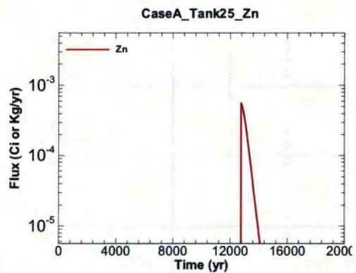
Figure A.1-858 - Flux Leaving Liner for CaseA Tank25 Zn
