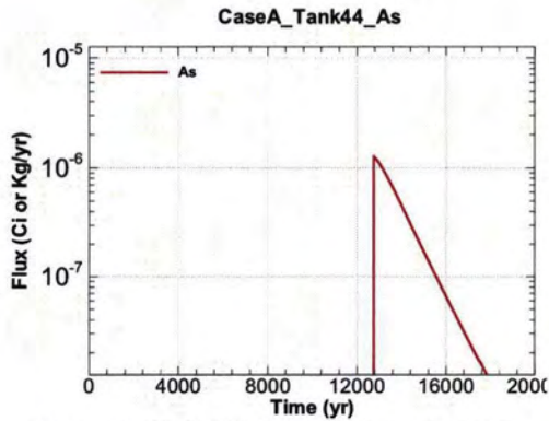
Figure A.1-1099 - Flux Leaving Liner for CaseA Tank44 As
