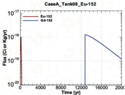
Figure A.1-573 - Flux Leaving Liner for CaseA Tank08 Eu-152
