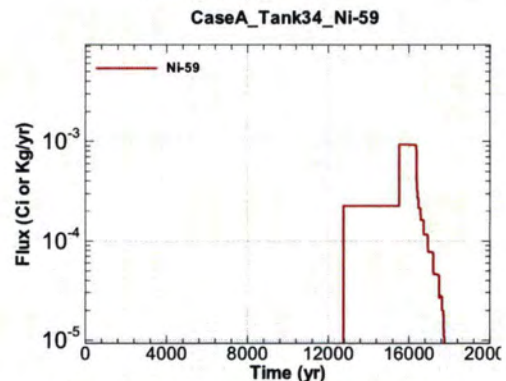
Figure A.1-742 - Flux Leaving Liner for CaseA Tank34 Ni-59
