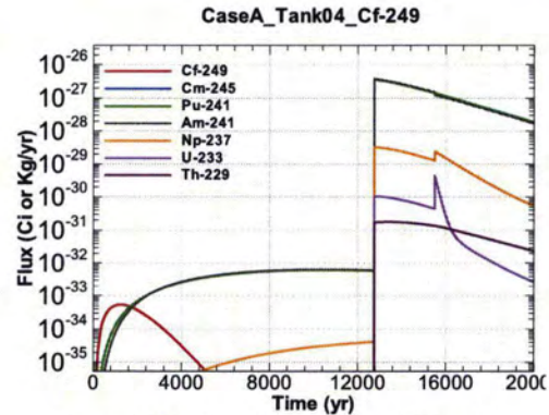
Figure A.1-248 - Flux Leaving Liner for CaseA Tank04 Cf-249
