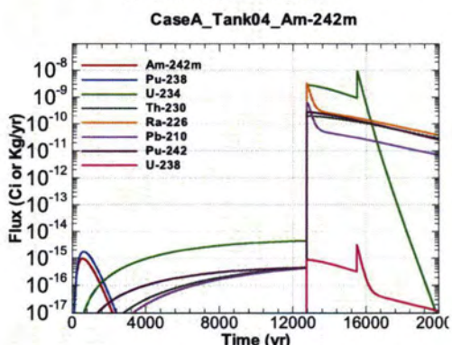
Figure A.1-239 - Flux Leaving Liner for CaseA Tank04 Am-242m
