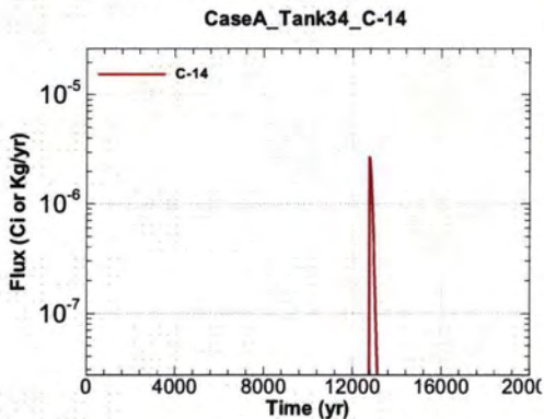
Figure A.1-713 - Flux Leaving Liner for CaseA Tank34 C-14
