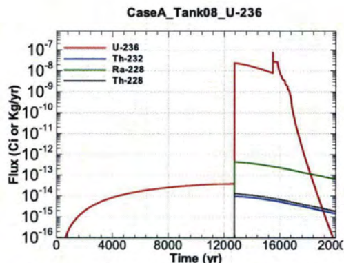
Figure A.1-620 - Flux Leaving Liner for CaseA Tank08 U-236
