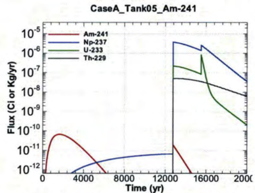
Figure A.1-316 - Flux Leaving Liner for CaseA Tank05 Am-241
