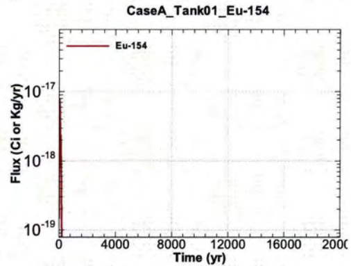
Figure A.1-28 - Flux Leaving Liner for CaseA Tank01 Eu-154
