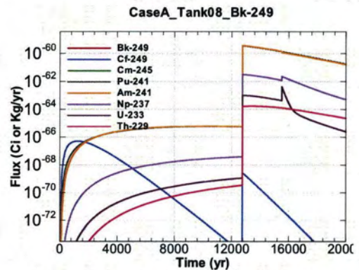
Figure A.1-556 - Flux Leaving Liner for CaseA Tank08 Bk-249
