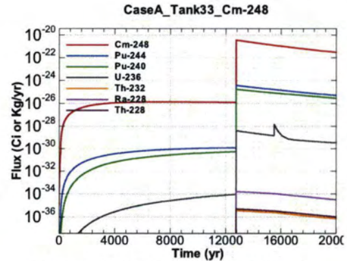
Figure A.1-644 - Flux Leaving Liner for CaseA Tank33 Cm-248
