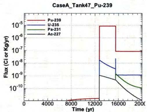
Figure A.1-1374 - Flux Leaving Liner for CaseA Tank47 Pu-239
