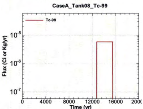
Figure A.1-611 - Flux Leaving Liner for CaseA Tank08 Tc-99
