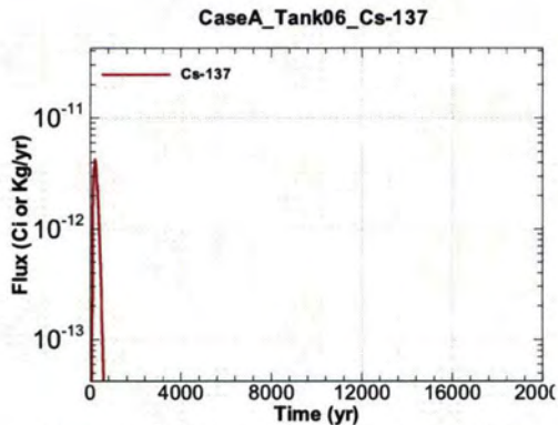
Figure A.1-415 - Flux Leaving Liner for CaseA Tank06 Cs-137
