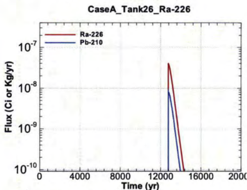
Figure A.1-911 - Flux Leaving Liner for CaseA Tank26 Ra-226
