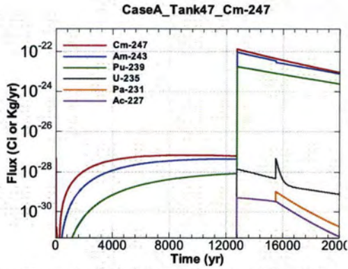
Figure A.1-1345 - Flux Leaving Liner for CaseA Tank47 Cm-247
