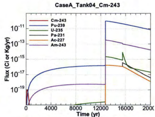
Figure A.1-250 - Flux Leaving Liner for CaseA Tank04 Cm-243
