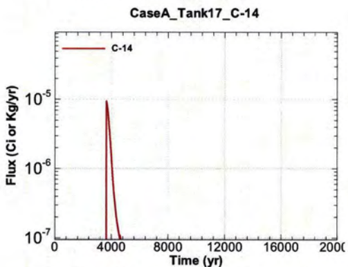
Figure A.1-1415 - Flux Leaving Liner for CaseA Tank17 C-14
