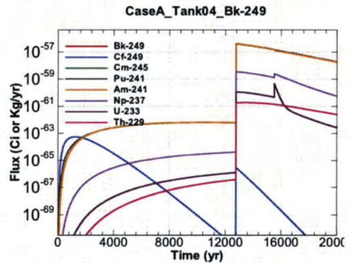
Figure A.1-244 - Flux Leaving Liner for CaseA Tank04 Bk-249
