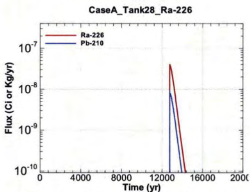
Figure A.1-1067 - Flux Leaving Liner for CaseA Tank28 Ra-226
