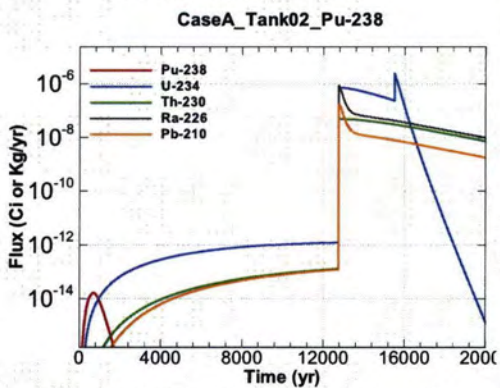
Figure A.1-125 - Flux Leaving Liner for CaseA Tank02 Pu-238
