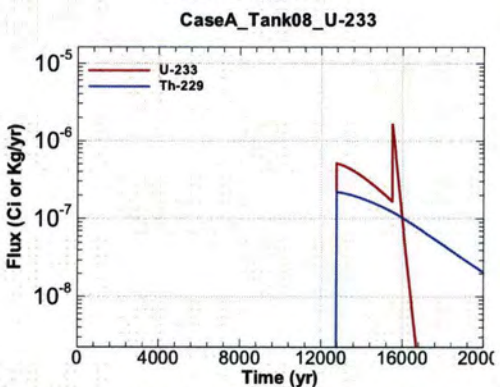
Figure A.1-617 - Flux Leaving Liner for CaseA Tank08 U-233
