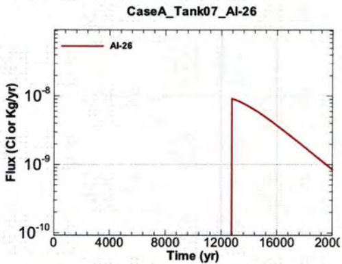
Figure A.1-471 - Flux Leaving Liner for CaseA Tank07 Al-26
