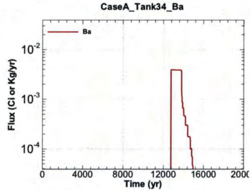
Figure A.1-710 - Flux Leaving Liner for CaseA Tank34 Ba
