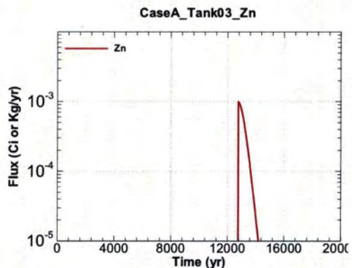
Figure A.1-234 - Flux Leaving Liner for CaseA Tank03 Zn
