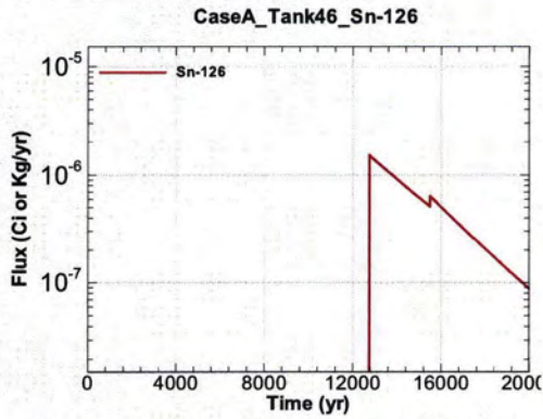
Figure A.1-1311 - Flux Leaving Liner for CaseA Tank46 Sn-126
