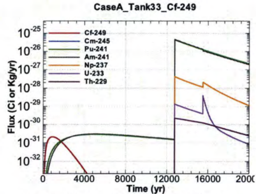
Figure A.1-638 - Flux Leaving Liner for CaseA Tank33 Cf-249
