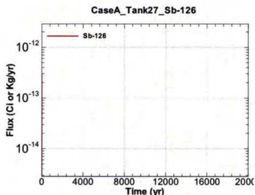
Figure A.1-994 - Flux Leaving Liner for CaseA Tank27 Sb-126
