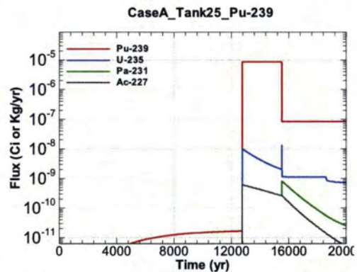
Figure A.1-828 - Flux Leaving Liner for CaseA Tank25 Pu-239
