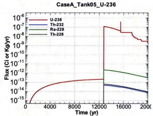
Figure A.1-386 - Flux Leaving Liner for CaseA Tank05 U-236
