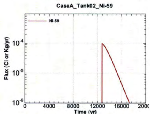
Figure A.1-118 - Flux Leaving Liner for CaseA Tank02 Ni-59
