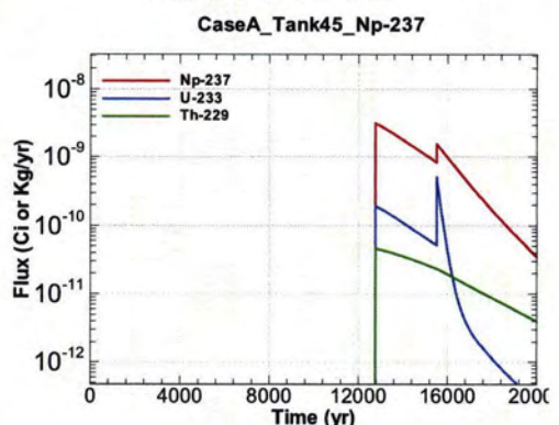
Figure A.1-1212 - Flux Leaving Liner for CaseA Tank45 Np-237
