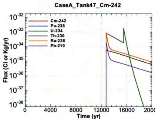
Figure A.1-1341 - Flux Leaving Liner for CaseA Tank47 Cm-242
