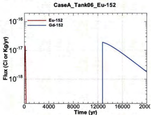
Figure A.1-417 - Flux Leaving Liner for CaseA Tank06 Eu-152
