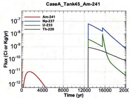
Figure A.1-1174 - Flux Leaving Liner for CaseA Tank45 Am-241
