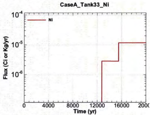
Figure A.1-663 - Flux Leaving Liner for CaseA Tank33 Ni
