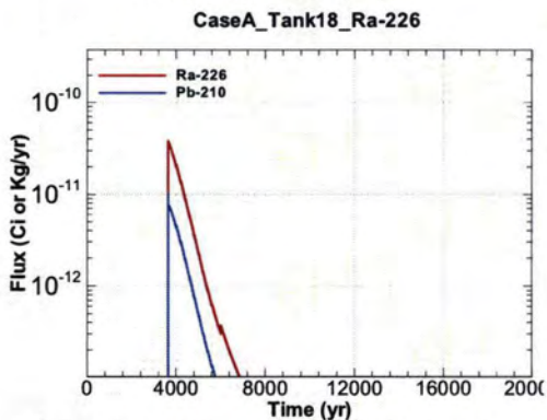
Figure A.1-1535 - Flux Leaving Liner for CaseA Tank18 Ra-226
