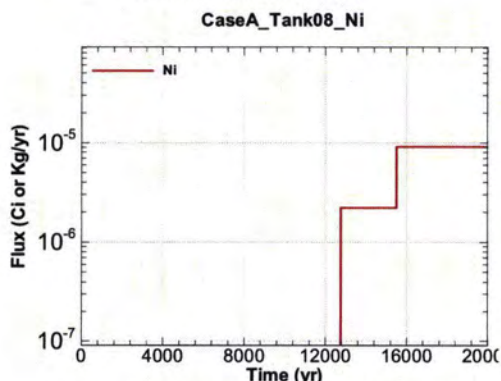
Figure A.1-585 - Flux Leaving Liner for CaseA Tank08 Ni
