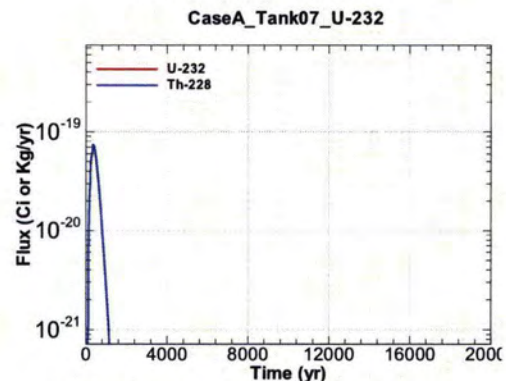
Figure A.1-538 - Flux Leaving Liner for CaseA Tank07 U-232
