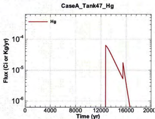
Figure A.1-1359 - Flux Leaving Liner for CaseA Tank47 Hg
