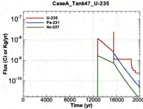
Figure A.1-1399 - Flux Leaving Liner for CaseA Tank47 U-235
