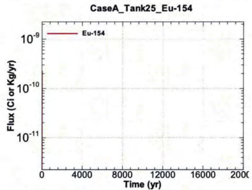
Figure A.1-808 - Flux Leaving Liner for CaseA Tank25 Eu-154
