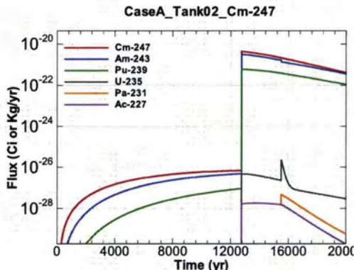
Figure A.1-97 - Flux Leaving Liner for CaseA Tank02 Cm-247
