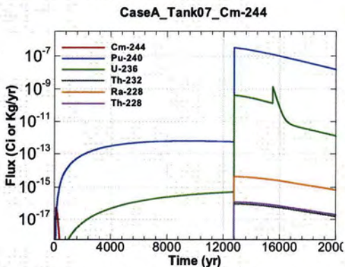
Figure A.1-485 - Flux Leaving Liner for CaseA Tank07 Cm-244
