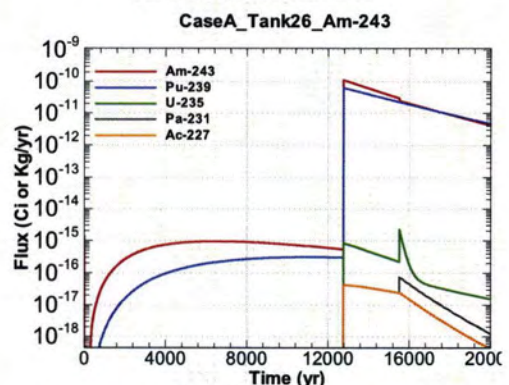
Figure A.1-864 - Flux Leaving Liner for CaseA Tank26 Am-243
