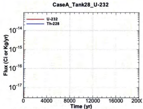
Figure A.1-1084 - Flux Leaving Liner for CaseA Tank28 U-232
