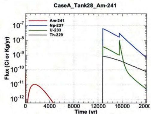
Figure A.1-1018 - Flux Leaving Liner for CaseA Tank28 Am-241
