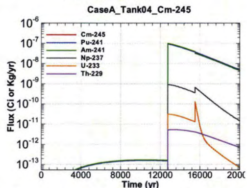
Figure A.1-252 - Flux Leaving Liner for CaseA Tank04 Cm-245
