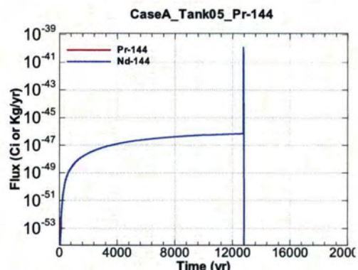
Figure A.1-358 - Flux Leaving Liner for CaseA Tank05 Pr-144
