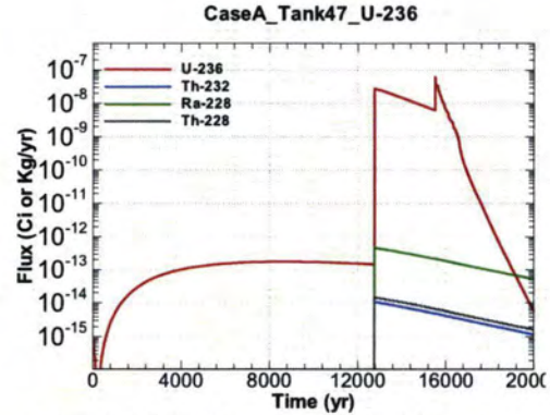
Figure A.1-1400 - Flux Leaving Liner for CaseA Tank47 U-236
