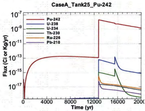
Figure A.1-831 - Flux Leaving Liner for CaseA Tank25 Pu-242
