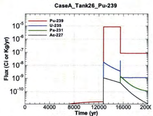
Figure A.1-906 - Flux Leaving Liner for CaseA Tank26 Pu-239
