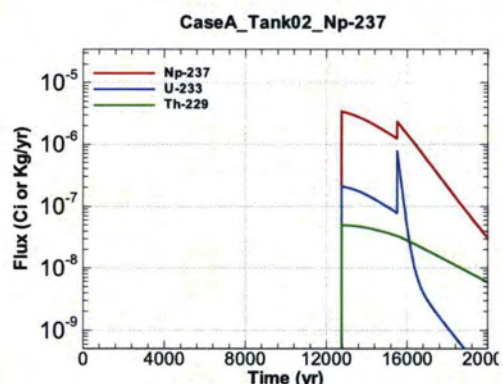
Figure A.1-120 - Flux Leaving Liner for CaseA Tank02 Np-237
