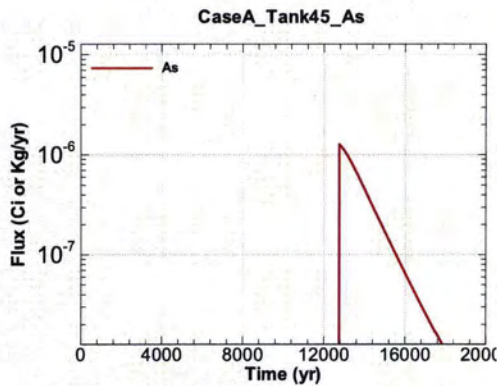
Figure A.1-1177 - Flux Leaving Liner for CaseA Tank45 As
