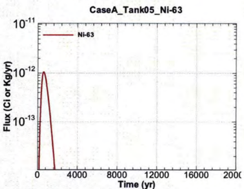
Figure A.1-353 - Flux Leaving Liner for CaseA Tank05 Ni-63
