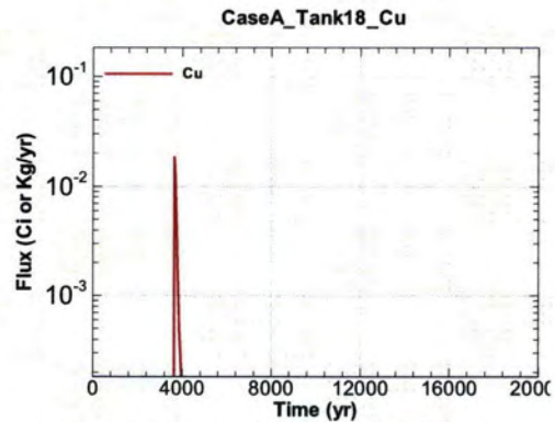
Figure A.1-1508 - Flux Leaving Liner for CaseA Tank18 Cu
