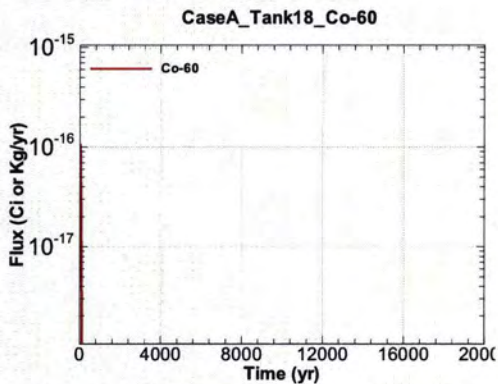
Figure A.1-1503 - Flux Leaving Liner for CaseA Tank18 Co-60
