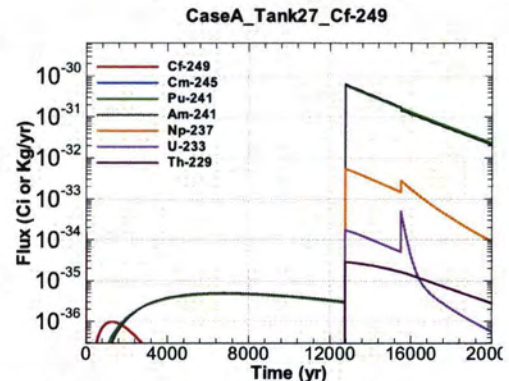
Figure A.1-950 - Flux Leaving Liner for CaseA Tank27 Cf-249
