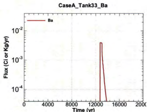
Figure A.1-632 - Flux Leaving Liner for CaseA Tank33 Ba
