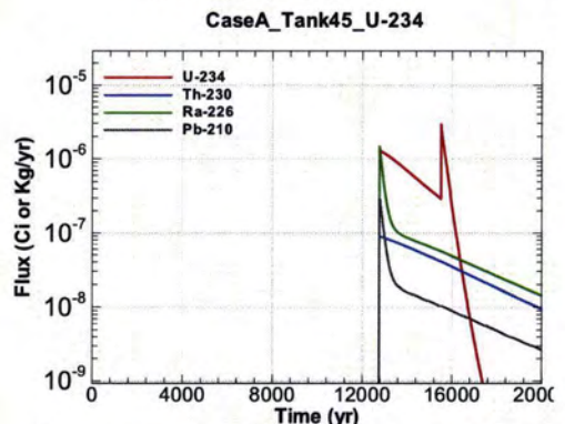
Figure A.1-1242 - Flux Leaving Liner for CaseA Tank45 U-234
