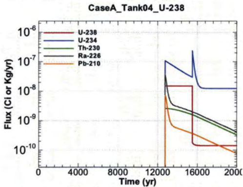
Figure A.1-309 - Flux Leaving Liner for CaseA Tank04 U-238
