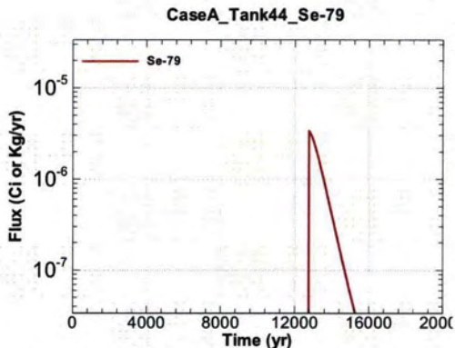
Figure A.1-1153 - Flux Leaving Liner for CaseA Tank44 Se-79
