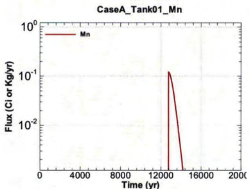
Figure A.1-35 - Flux Leaving Liner for CaseA Tank01 Mn
