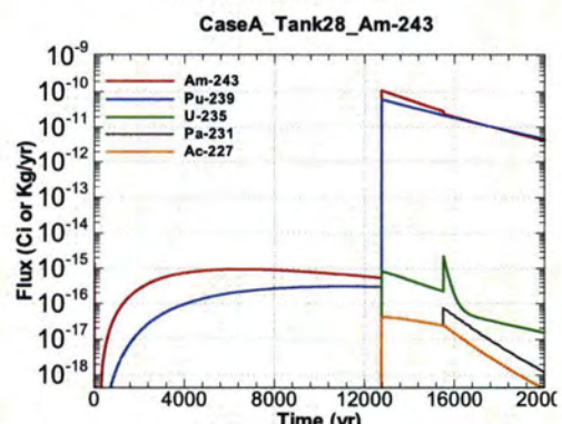
Figure A.1-1020 - Flux Leaving Liner for CaseA Tank28 Am-243
