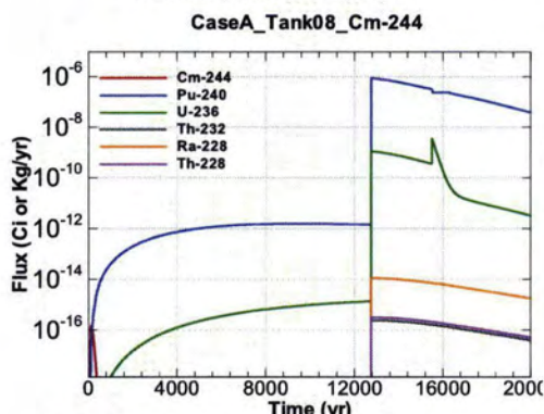
Figure A.1-563 - Flux Leaving Liner for CaseA Tank08 Cm-244
