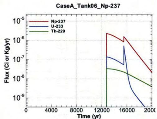
Figure A.1-432 - Flux Leaving Liner for CaseA Tank06 Np-237
