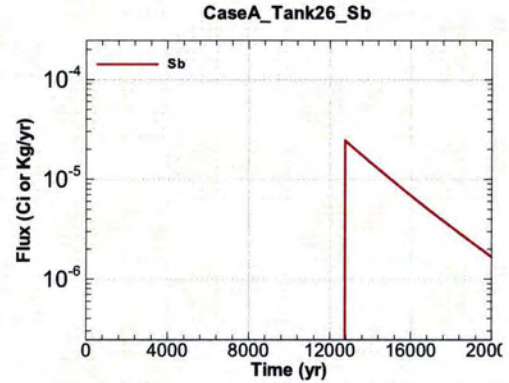
Figure A.1-914 - Flux Leaving Liner for CaseA Tank26 Sb
