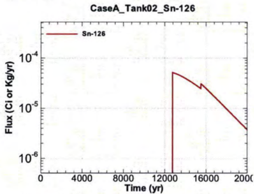
Figure A.1-141 - Flux Leaving Liner for CaseA Tank02 Sn-126
