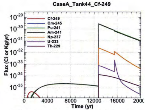
Figure A.1-1106 - Flux Leaving Liner for CaseA Tank44 Cf-249
