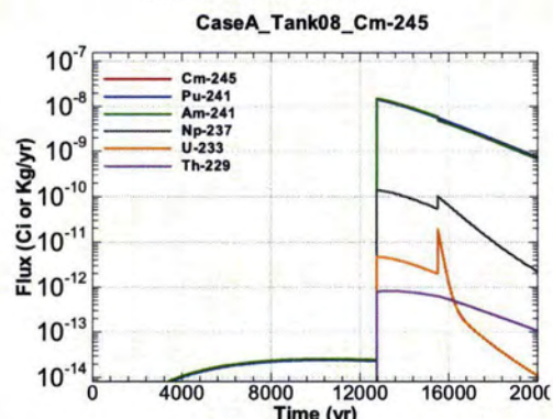
Figure A.1-564 - Flux Leaving Liner for CaseA Tank08 Cm-245
