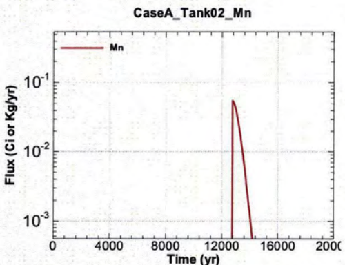
Figure A.1-113 - Flux Leaving Liner for CaseA Tank02 Mn
