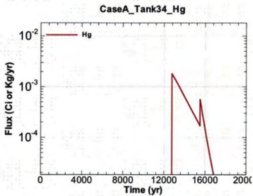
Figure A.1-735 - Flux Leaving Liner for CaseA Tank34 Hg
