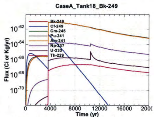
Figure A.1-1492 - Flux Leaving Liner for CaseA Tank18 Bk-249
