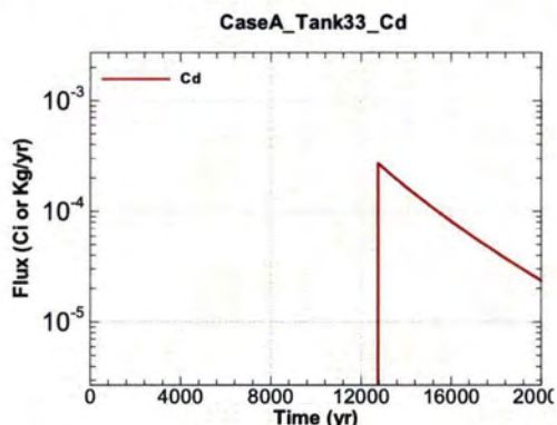
Figure A.1-636 - Flux Leaving Liner for CaseA Tank33 Cd
