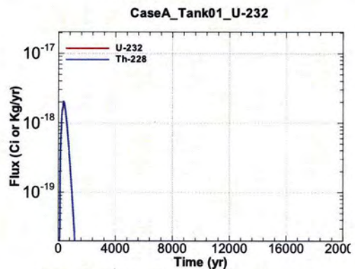
Figure A.1-70 - Flux Leaving Liner for CaseA Tank01 U-232
