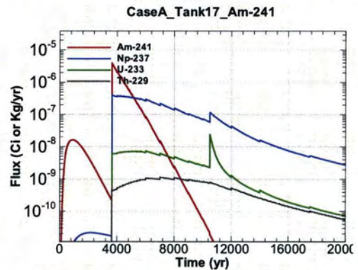
Figure A.1-1408 - Flux Leaving Liner for CaseA Tank17 Am-241
