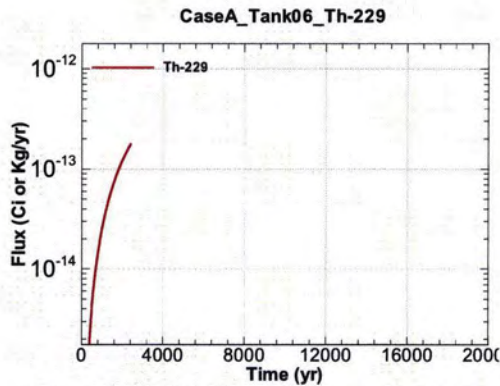
Figure A.1-457 - Flux Leaving Liner for CaseA Tank06 Th-229
