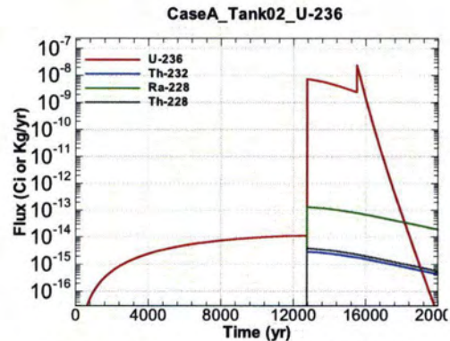
Figure A.1-152 - Flux Leaving Liner for CaseA Tank02 U-236
