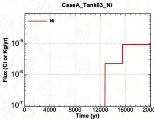
Figure A.1-195 - Flux Leaving Liner for CaseA Tank03 Ni
