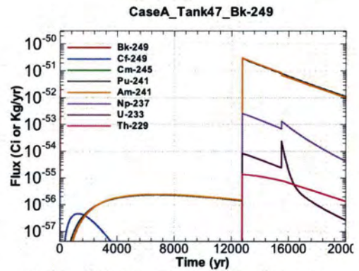
Figure A.1-1336 - Flux Leaving Liner for CaseA Tank47 Bk-249
