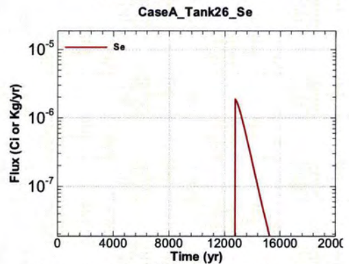
Figure A.1-918 - Flux Leaving Liner for CaseA Tank26 Se
