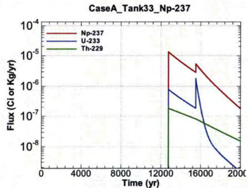
Figure A.1-666 - Flux Leaving Liner for CaseA Tank33 Np-237
