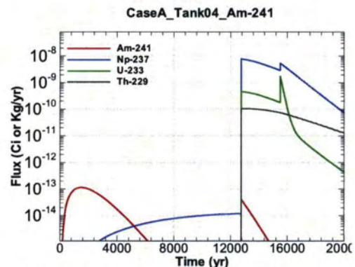
Figure A.1-238 - Flux Leaving Liner for CaseA Tank04 Am-241
