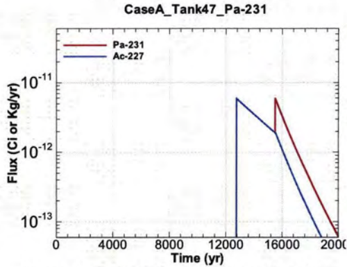
Figure A.1-1369 - Flux Leaving Liner for CaseA Tank47 Pa-231
