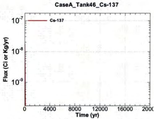
Figure A.1-1273 - Flux Leaving Liner for CaseA Tank46 Cs-137
