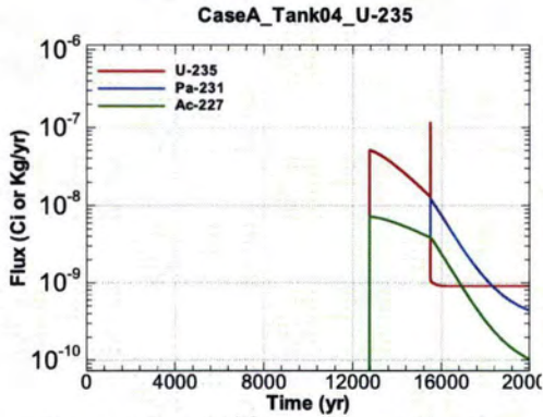
Figure A.1-307 - Flux Leaving Liner for CaseA Tank04 U-235
