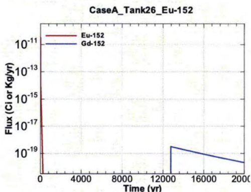
Figure A.1-885 - Flux Leaving Liner for CaseA Tank26 Eu-152
