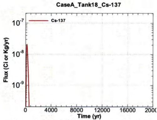
Figure A.1-1507 - Flux Leaving Liner for CaseA Tank18 Cs-137
