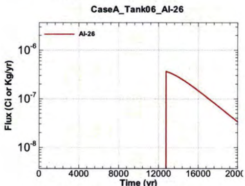
Figure A.1-393 - Flux Leaving Liner for CaseA Tank06 Al-26
