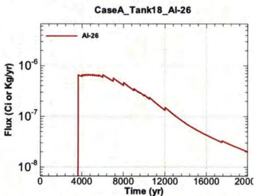
Figure A.1-1485 - Flux Leaving Liner for CaseA Tank18 Al-26
