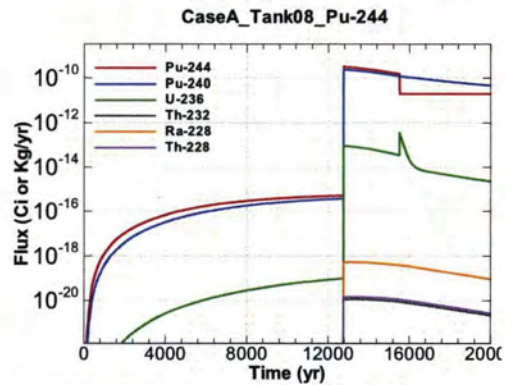
Figure A.1-598 - Flux Leaving Liner for CaseA Tank08 Pu-244
