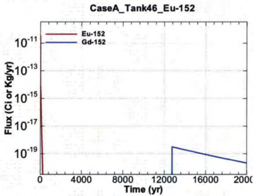
Figure A.1-1275 - Flux Leaving Liner for CaseA Tank46 Eu-152
