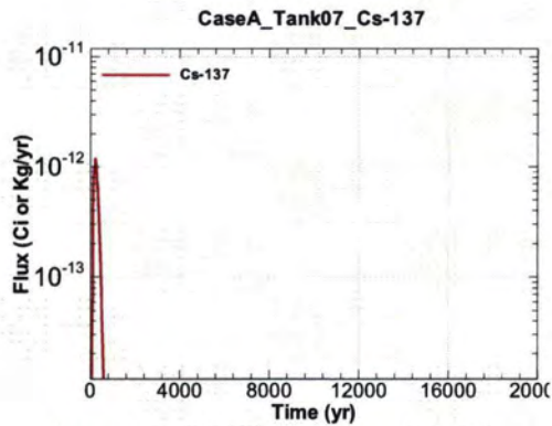
Figure A.1-493 - Flux Leaving Liner for CaseA Tank07 Cs-137
