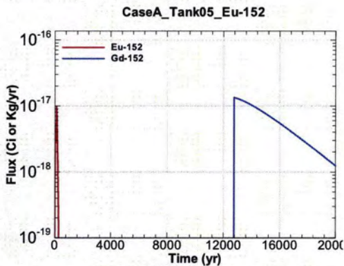
Figure A.1-339 - Flux Leaving Liner for CaseA Tank05 Eu-152
