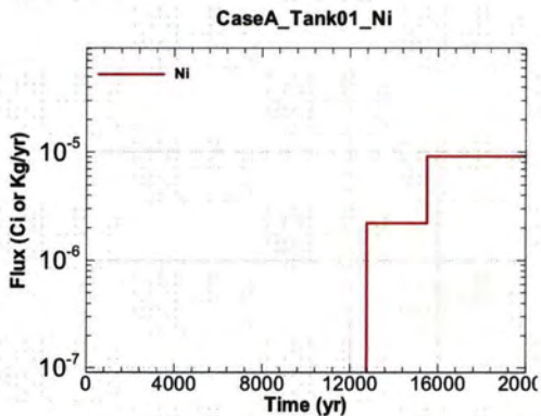
Figure A.1-39 - Flux Leaving Liner for CaseA Tank01 Ni
