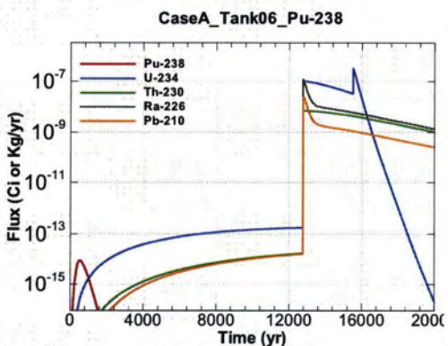
Figure A.1-437 - Flux Leaving Liner for CaseA Tank06 Pu-238
