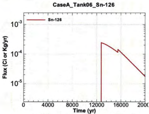
Figure A.1-453 - Flux Leaving Liner for CaseA Tank06 Sn-126
