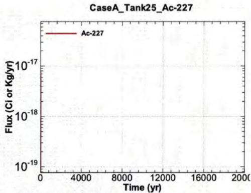
Figure A.1-781 - Flux Leaving Liner for CaseA Tank25 Ac-227
