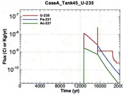
Figure A.1-1243 - Flux Leaving Liner for CaseA Tank45 U-235
