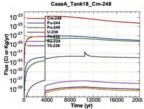
Figure A.1-1502 - Flux Leaving Liner for CaseA Tank18 Cm-248
