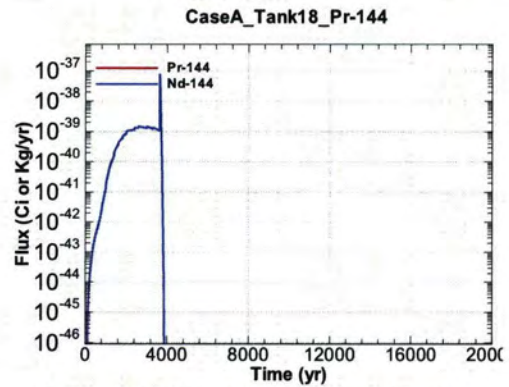
Figure A.1-1528 - Flux Leaving Liner for CaseA Tank18 Pr-144
