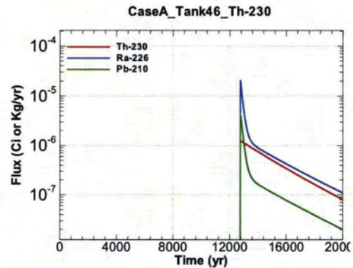
Figure A.1-1316 - Flux Leaving Liner for CaseA Tank46 Th-230
