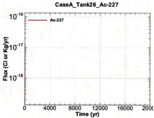
Figure A.1-859 - Flux Leaving Liner for CaseA Tank26 Ac-227
