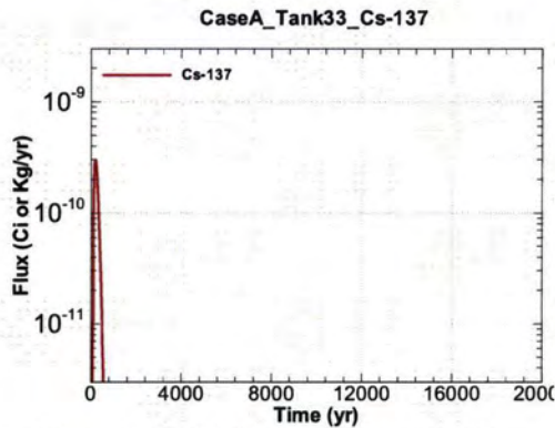
Figure A.1-649 - Flux Leaving Liner for CaseA Tank33 Cs-137
