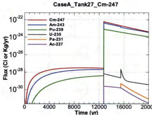
Figure A.1-955 - Flux Leaving Liner for CaseA Tank27 Cm-247
