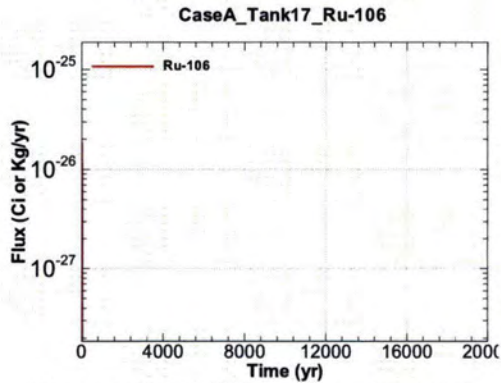
Figure A.1-1459 - Flux Leaving Liner for CaseA Tank17 Ru-106
