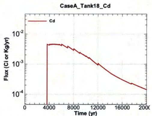
Figure A.1-1494 - Flux Leaving Liner for CaseA Tank18 Cd
