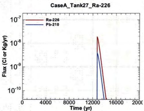
Figure A.1-989 - Flux Leaving Liner for CaseA Tank27 Ra-226
