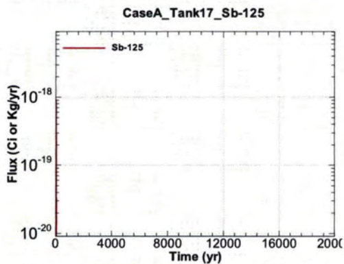
Figure A.1-1461 - Flux Leaving Liner for CaseA Tank17 Sb-125
