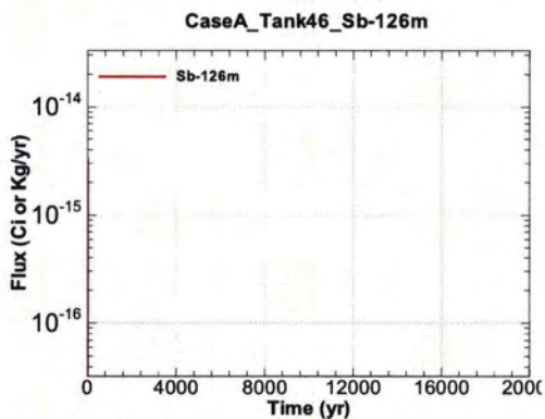
Figure A.1-1307 - Flux Leaving Liner for CaseA Tank46 Sb-126m
