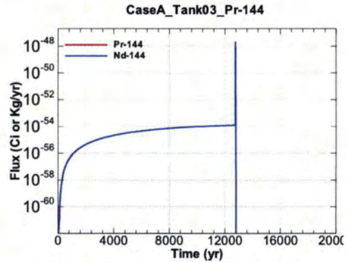
Figure A.1-202 - Flux Leaving Liner for CaseA Tank03 Pr-144
