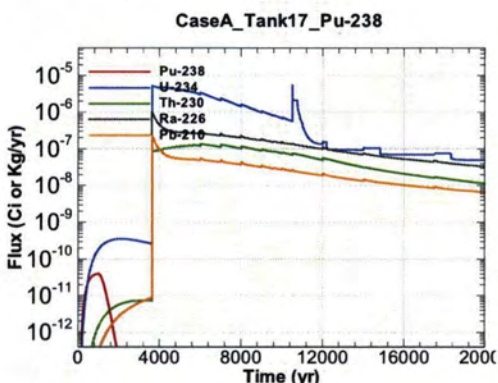
Figure A.1-1451 - Flux Leaving Liner for CaseA Tank17 Pu-238
