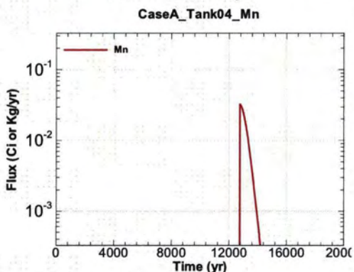
Figure A.1-269 - Flux Leaving Liner for CaseA Tank04 Mn
