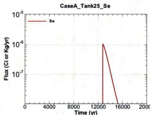
Figure A.1-840 - Flux Leaving Liner for CaseA Tank25 Se
