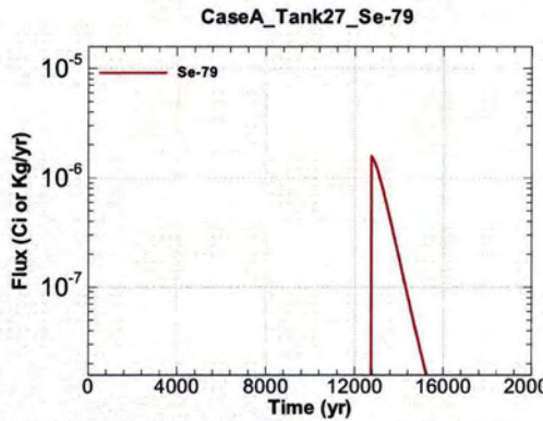
Figure A.1-997 - Flux Leaving Liner for CaseA Tank27 Se-79
