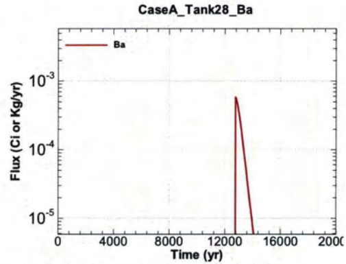
Figure A.1-1022 - Flux Leaving Liner for CaseA Tank28 Ba
