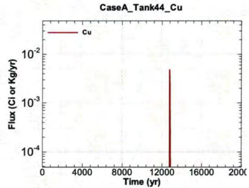
Figure A.1-1118 - Flux Leaving Liner for CaseA Tank44 Cu
