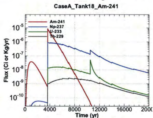
Figure A.1-1486 - Flux Leaving Liner for CaseA Tank18 Am-241
