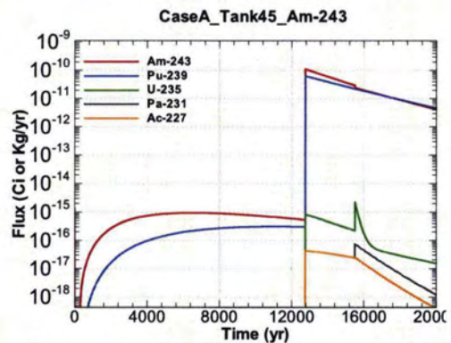
Figure A.1-1176 - Flux Leaving Liner for CaseA Tank45 Am-243
