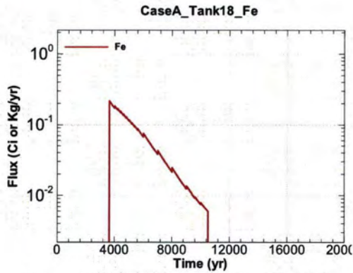
Figure A.1-1513 - Flux Leaving Liner for CaseA Tank18 Fe
