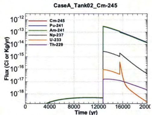
Figure A.1-96 - Flux Leaving Liner for CaseA Tank02 Cm-245
