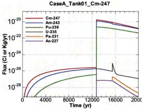
Figure A.1-19 - Flux Leaving Liner for CaseA Tank01 Cm-247
