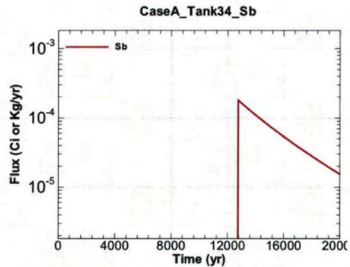
Figure A.1-758 - Flux Leaving Liner for CaseA Tank34 Sb
