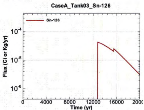
Figure A.1-219 - Flux Leaving Liner for CaseA Tank03 Sn-126
