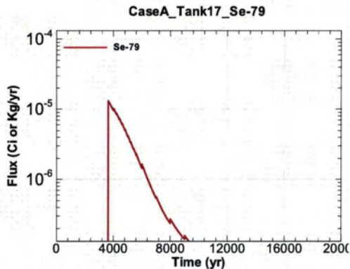
Figure A.1-1465 - Flux Leaving Liner for CaseA Tank17 Se-79
