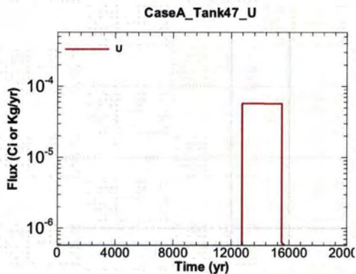
Figure A.1-1395 - Flux Leaving Liner for CaseA Tank47 U
