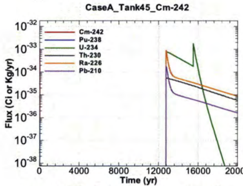
Figure A.1-1185 - Flux Leaving Liner for CaseA Tank45 Cm-242
