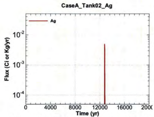
Figure A.1-80 - Flux Leaving Liner for CaseA Tank02 Ag
