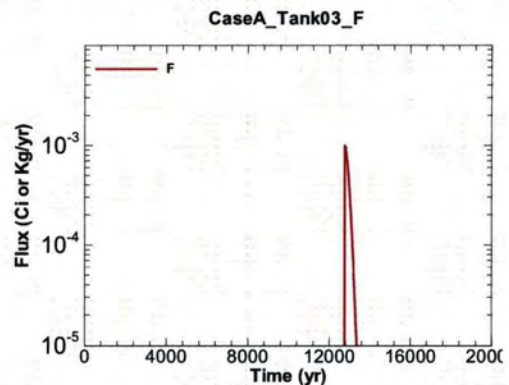
Figure A.1-186 - Flux Leaving Liner for CaseA Tank03 F
