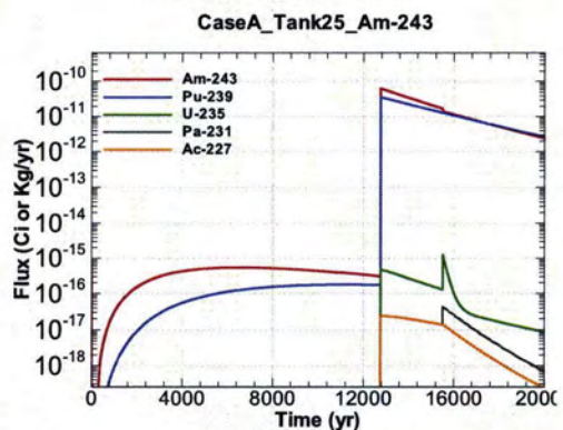
Figure A.1-786 - Flux Leaving Liner for CaseA Tank25 Am-243
