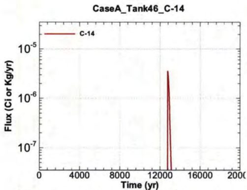
Figure A.1-1259 - Flux Leaving Liner for CaseA Tank46 C-14
