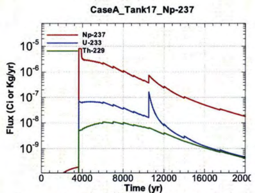
Figure A.1-1446 - Flux Leaving Liner for CaseA Tank17 Np-237
