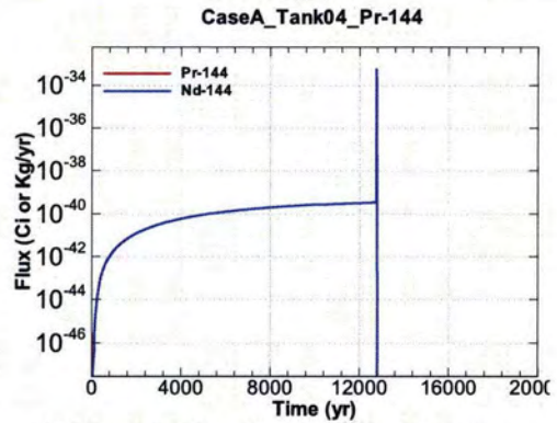
Figure A.1-280 - Flux Leaving Liner for CaseA Tank04 Pr-144
