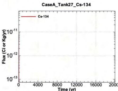
Figure A.1-959 - Flux Leaving Liner for CaseA Tank27 Cs-134
