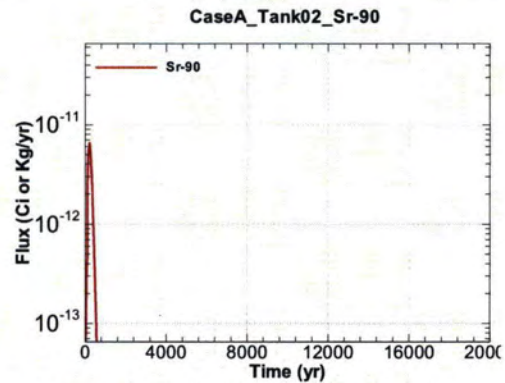
Figure A.1-142 - Flux Leaving Liner for CaseA Tank02 Sr-90
