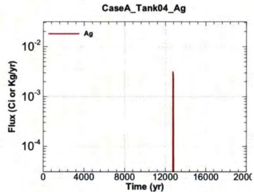
Figure A.1-236 - Flux Leaving Liner for CaseA Tank04 Ag
