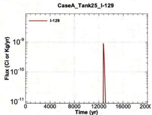
Figure A.1-814 - Flux Leaving Liner for CaseA Tank25 I-129
