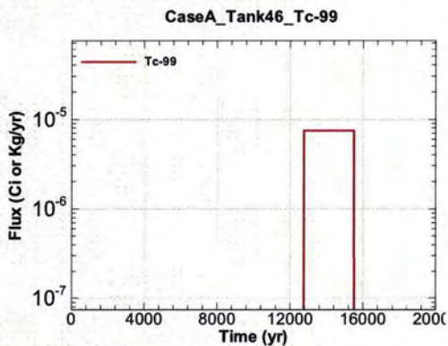
Figure A.1-1313 - Flux Leaving Liner for CaseA Tank46 Tc-99
