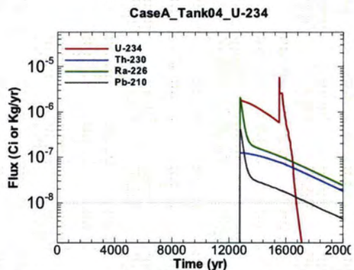
Figure A.1-306 - Flux Leaving Liner for CaseA Tank04 U-234
