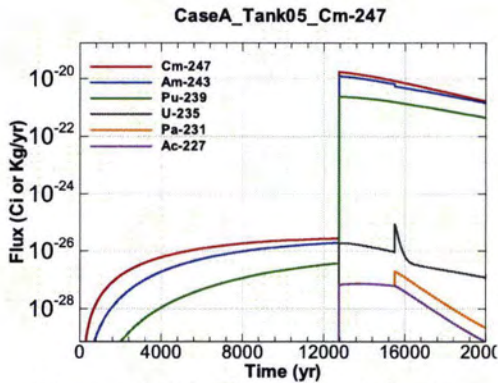
Figure A.1-331 - Flux Leaving Liner for CaseA Tank05 Cm-247
