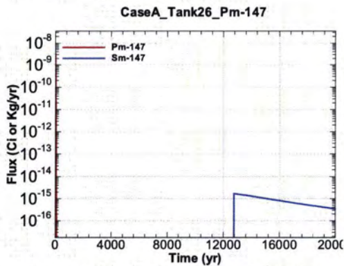
Figure A.1-903 - Flux Leaving Liner for CaseA Tank26 Pm-147
