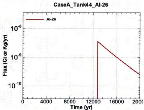
Figure A.1-1095 - Flux Leaving Liner for CaseA Tank44 Al-26
