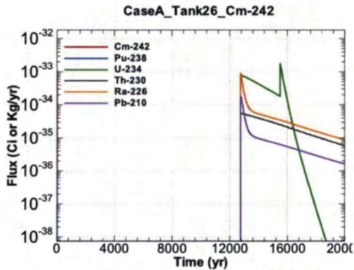
Figure A.1-873 - Flux Leaving Liner for CaseA Tank26 Cm-242
