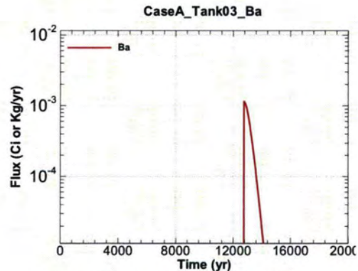
Figure A.1-164 - Flux Leaving Liner for CaseA Tank03 Ba
