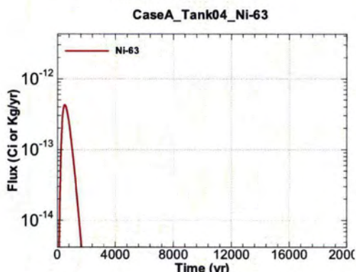
Figure A.1-275 - Flux Leaving Liner for CaseA Tank04 Ni-63
