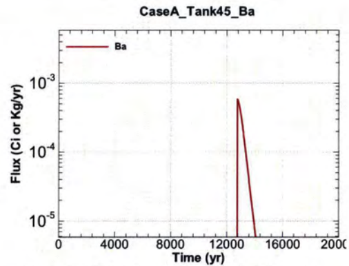
Figure A.1-1178 - Flux Leaving Liner for CaseA Tank45 Ba
