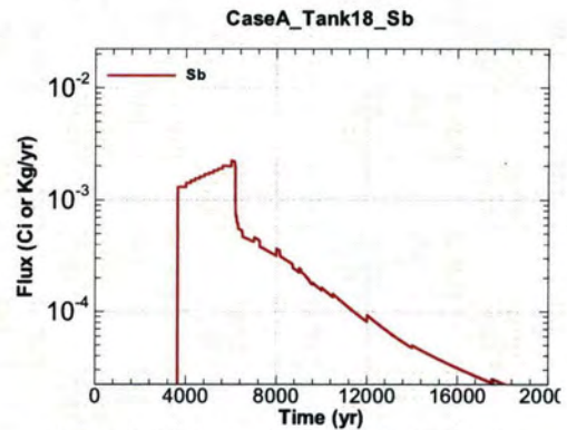
Figure A.1-1538 - Flux Leaving Liner for CaseA Tank18 Sb
