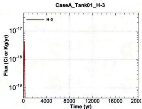
Figure A.1-32 - Flux Leaving Liner for CaseA Tank01 H-3
