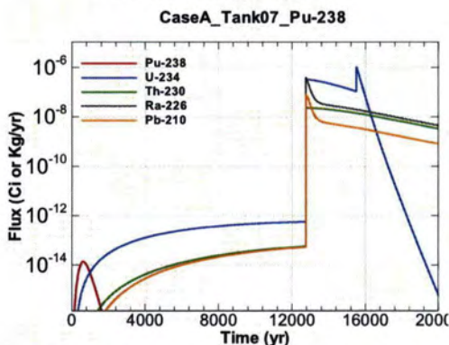
Figure A.1-515 - Flux Leaving Liner for CaseA Tank07 Pu-238
