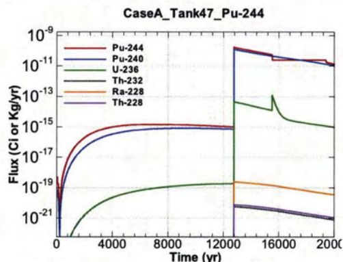
Figure A.1-1378 - Flux Leaving Liner for CaseA Tank47 Pu-244
