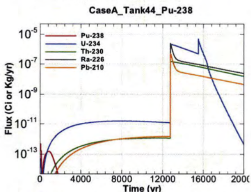
Figure A.1-1139 - Flux Leaving Liner for CaseA Tank44 Pu-238
