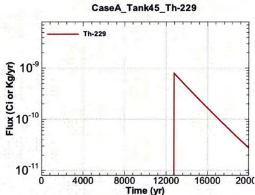
Figure A.1-1237 - Flux Leaving Liner for CaseA Tank45 Th-229
