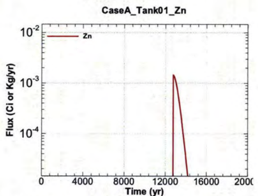
Figure A.1-78 - Flux Leaving Liner for CaseA Tank01 Zn
