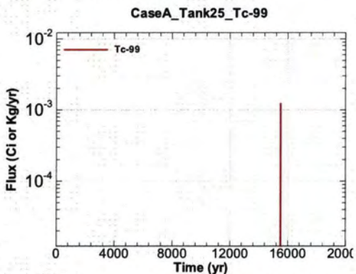
Figure A.1-845 - Flux Leaving Liner for CaseA Tank25 Tc-99
