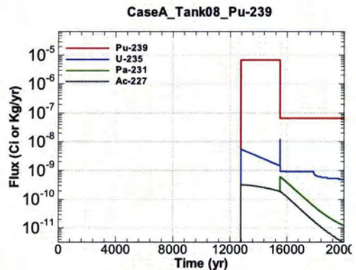
Figure A.1-594 - Flux Leaving Liner for CaseA Tank08 Pu-239
