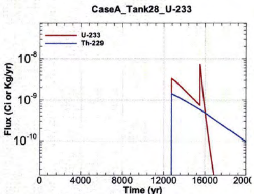
Figure A.1-1085 - Flux Leaving Liner for CaseA Tank28 U-233
