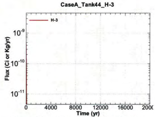
Figure A.1-1124 - Flux Leaving Liner for CaseA Tank44 H-3
