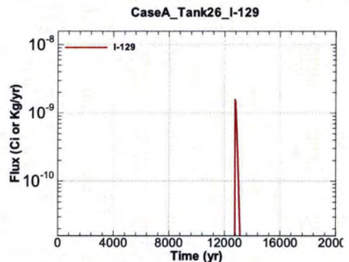
Figure A.1-892 - Flux Leaving Liner for CaseA Tank26 I-129
