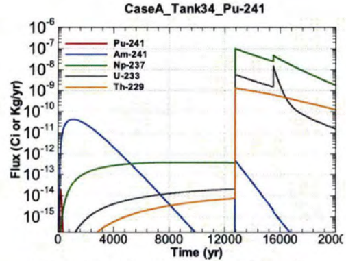
Figure A.1-752 - Flux Leaving Liner for CaseA Tank34 Pu-241
