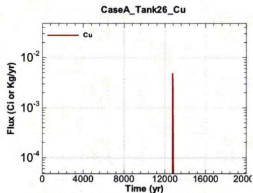
Figure A.1-884 - Flux Leaving Liner for CaseA Tank26 Cu
