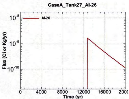
Figure A.1-939 - Flux Leaving Liner for CaseA Tank27 Al-26
