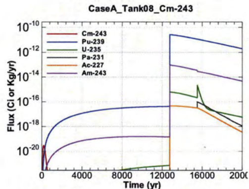
Figure A.1-562 - Flux Leaving Liner for CaseA Tank08 Cm-243
