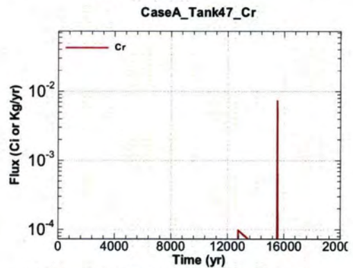
Figure A.1-1348 - Flux Leaving Liner for CaseA Tank47 Cr
