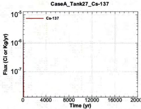
Figure A.1-961 - Flux Leaving Liner for CaseA Tank27 Cs-137
