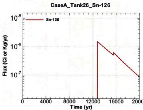
Figure A.1-921 - Flux Leaving Liner for CaseA Tank26 Sn-126
