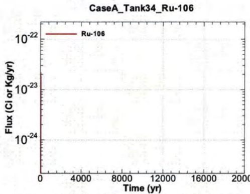
Figure A.1-757 - Flux Leaving Liner for CaseA Tank34 Ru-106
