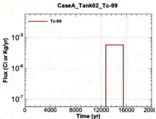
Figure A.1-143 - Flux Leaving Liner for CaseA Tank02 Tc-99
