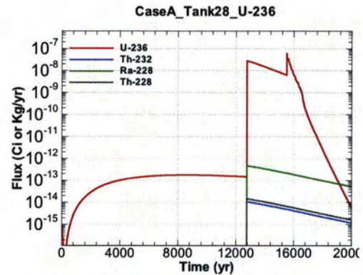
Figure A.1-1088 - Flux Leaving Liner for CaseA Tank28 U-236
