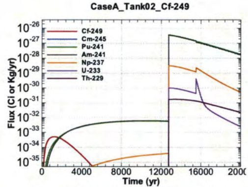
Figure A.1-92 - Flux Leaving Liner for CaseA Tank02 Cf-249
