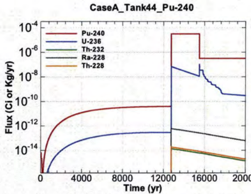
Figure A.1-1141 - Flux Leaving Liner for CaseA Tank44 Pu-240
