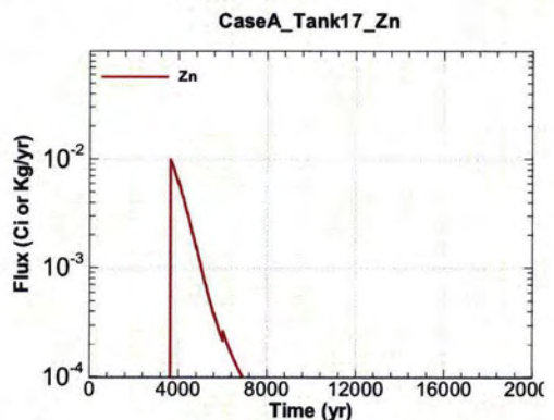
Figure A.1-1482 - Flux Leaving Liner for CaseA Tank17 Zn
