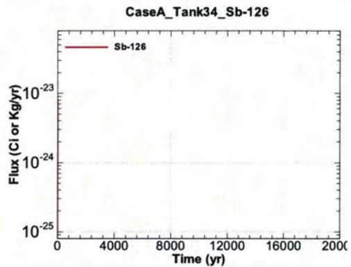
Figure A.1-760 - Flux Leaving Liner for CaseA Tank34 Sb-126
