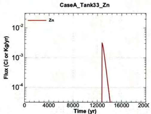
Figure A.1-702 - Flux Leaving Liner for CaseA Tank33 Zn
