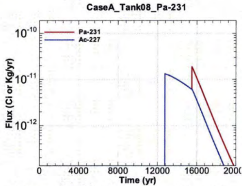
Figure A.1-589 - Flux Leaving Liner for CaseA Tank08 Pa-231
