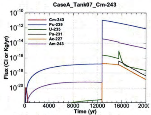
Figure A.1-484 - Flux Leaving Liner for CaseA Tank07 Cm-243
