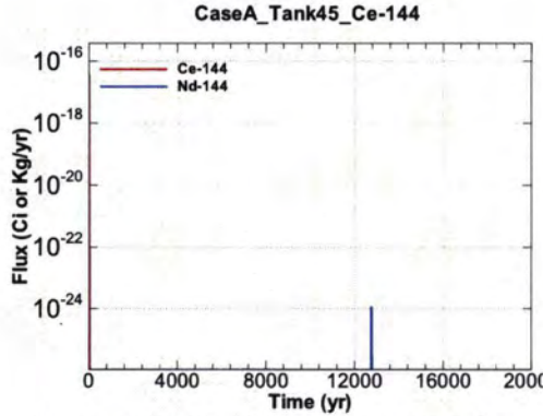
Figure A.1-1183 - Flux Leaving Liner for CaseA Tank45 Ce-144
