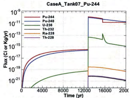
Figure A.1-520 - Flux Leaving Liner for CaseA Tank07 Pu-244
