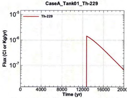
Figure A.1-67 - Flux Leaving Liner for CaseA Tank01 Th-229
