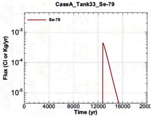
Figure A.1-685 - Flux Leaving Liner for CaseA Tank33 Se-79
