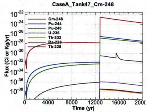
Figure A.1-1346 - Flux Leaving Liner for CaseA Tank47 Cm-248
