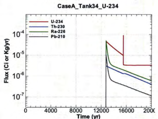
Figure A.1-774 - Flux Leaving Liner for CaseA Tank34 U-234
