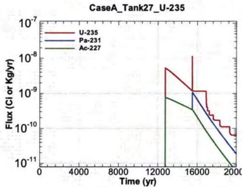
Figure A.1-1009 - Flux Leaving Liner for CaseA Tank27 U-235
