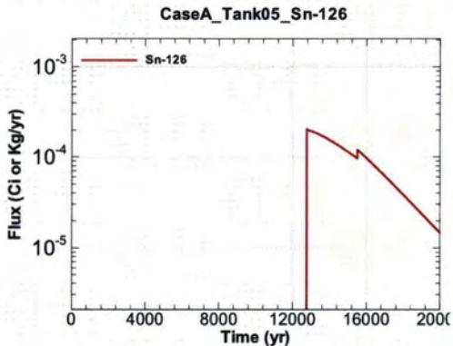
Figure A.1-375 - Flux Leaving Liner for CaseA Tank05 Sn-126
