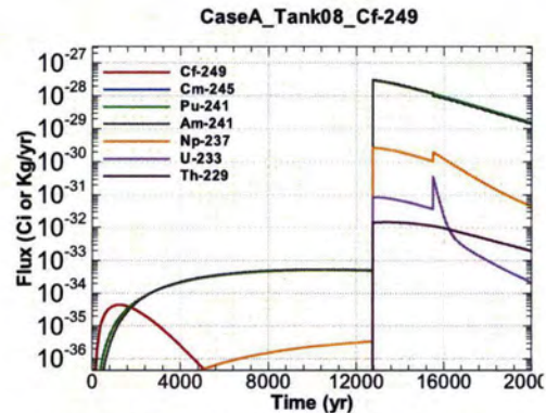
Figure A.1-560 - Flux Leaving Liner for CaseA Tank08 Cf-249
