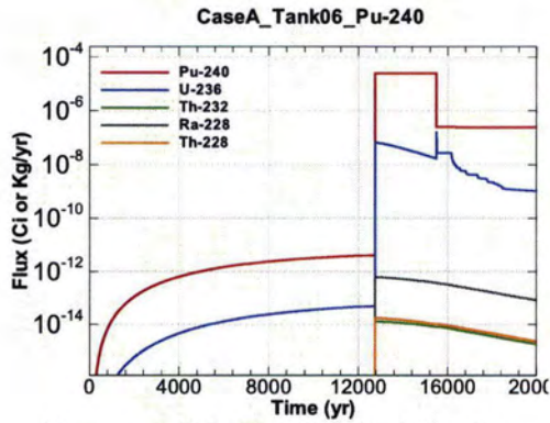
Figure A.1-439 - Flux Leaving Liner for CaseA Tank06 Pu-240
