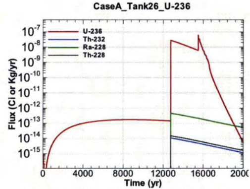
Figure A.1-932 - Flux Leaving Liner for CaseA Tank26 U-236
