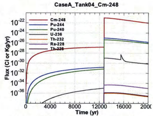
Figure A.1-254 - Flux Leaving Liner for CaseA Tank04 Cm-248
