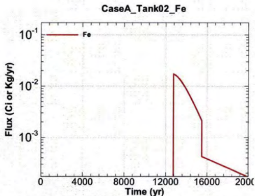
Figure A.1-109 - Flux Leaving Liner for CaseA Tank02 Fe
