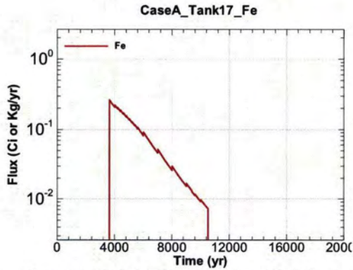
Figure A.1-1435 - Flux Leaving Liner for CaseA Tank17 Fe
