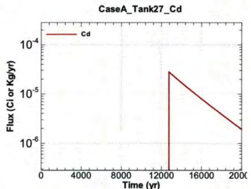
Figure A.1-948 - Flux Leaving Liner for CaseA Tank27 Cd
