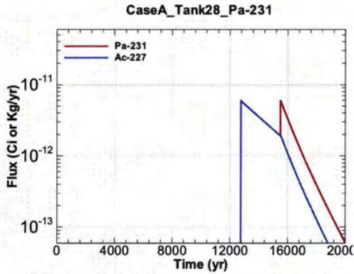
Figure A.1-1057 - Flux Leaving Liner for CaseA Tank28 Pa-231
