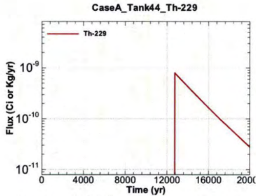
Figure A.1-1159 - Flux Leaving Liner for CaseA Tank44 Th-229
