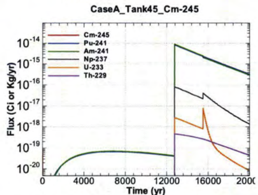
Figure A.1-1188 - Flux Leaving Liner for CaseA Tank45 Cm-245
