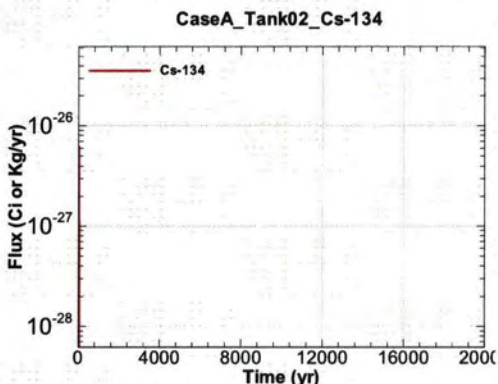
Figure A.1-101 - Flux Leaving Liner for CaseA Tank02 Cs-134
