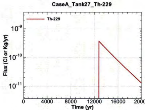
Figure A.1-1003 - Flux Leaving Liner for CaseA Tank27 Th-229
