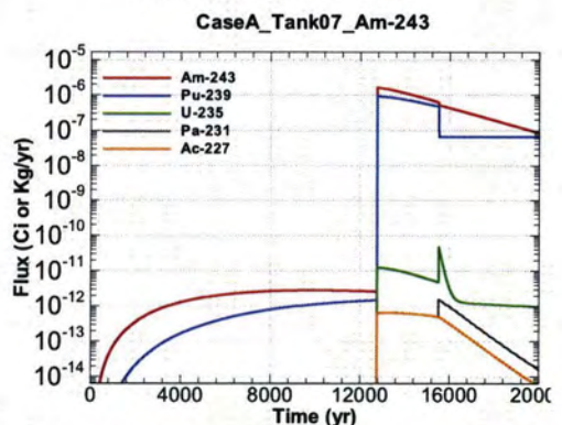
Figure A.1-474 - Flux Leaving Liner for CaseA Tank07 Am-243
