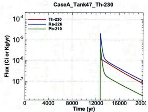
Figure A.1-1394 - Flux Leaving Liner for CaseA Tank47 Th-230
