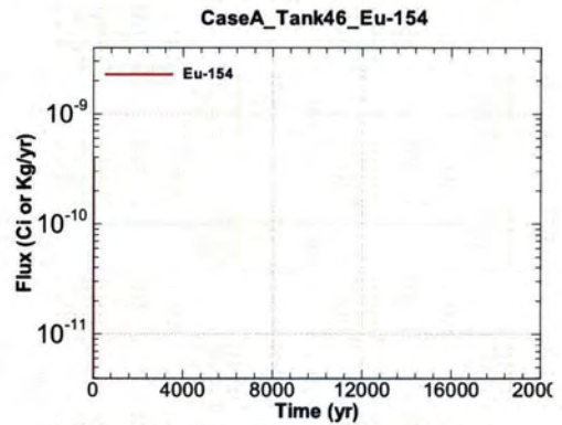
Figure A.1-1276 - Flux Leaving Liner for CaseA Tank46 Eu-154
