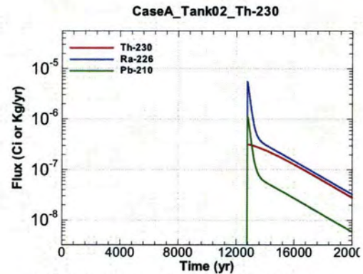
Figure A.1-146 - Flux Leaving Liner for CaseA Tank02 Th-230
