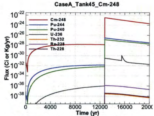
Figure A.1-1190 - Flux Leaving Liner for CaseA Tank45 Cm-248
