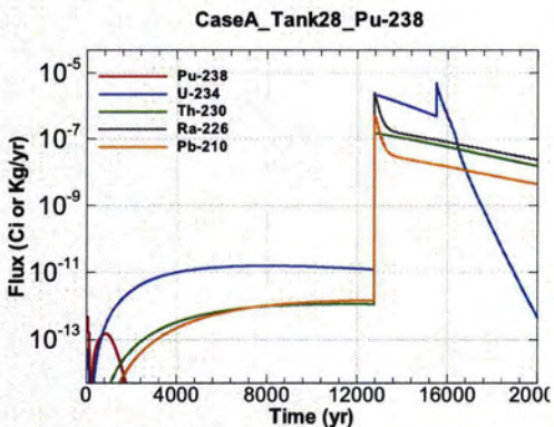
Figure A.1-1061 - Flux Leaving Liner for CaseA Tank28 Pu-238
