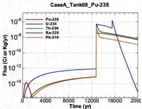
Figure A.1-593 - Flux Leaving Liner for CaseA Tank08 Pu-238
