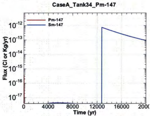
Figure A.1-747 - Flux Leaving Liner for CaseA Tank34 Pm-147
