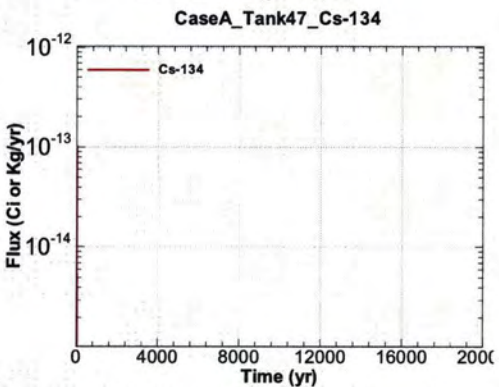
Figure A.1-1349 - Flux Leaving Liner for CaseA Tank47 Cs-134
