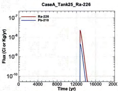
Figure A.1-833 - Flux Leaving Liner for CaseA Tank25 Ra-226
