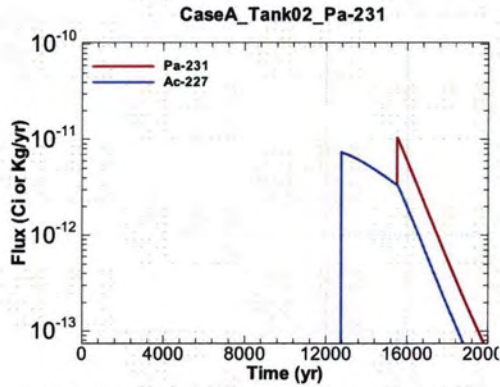
Figure A.1-121 - Flux Leaving Liner for CaseA Tank02 Pa-231
