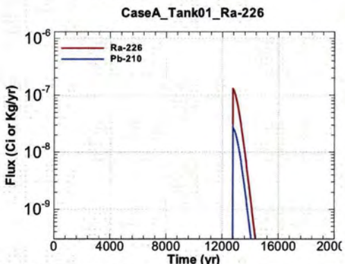
Figure A.1-53 - Flux Leaving Liner for CaseA Tank01 Ra-226
