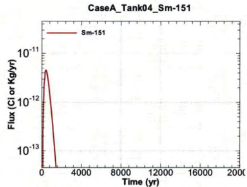
Figure A.1-296 - Flux Leaving Liner for CaseA Tank04 Sm-151
