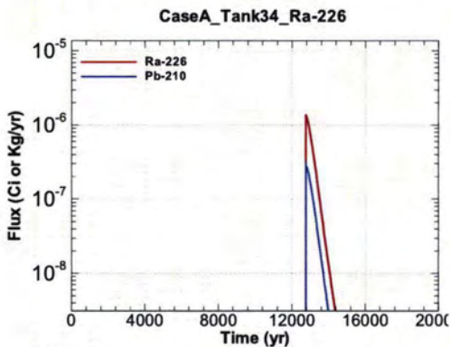
Figure A.1-755 - Flux Leaving Liner for CaseA Tank34 Ra-226
