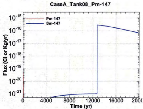
Figure A.1-591 - Flux Leaving Liner for CaseA Tank08 Pm-147
