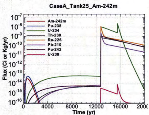
Figure A.1-785 - Flux Leaving Liner for CaseA Tank25 Am-242m
