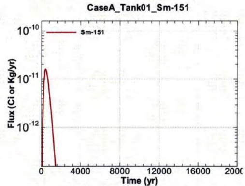
Figure A.1-62 - Flux Leaving Liner for CaseA Tank01 Sm-151
