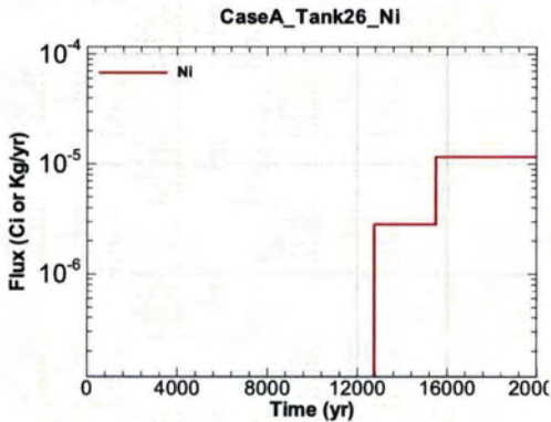
Figure A.1-897 - Flux Leaving Liner for CaseA Tank26 Ni
