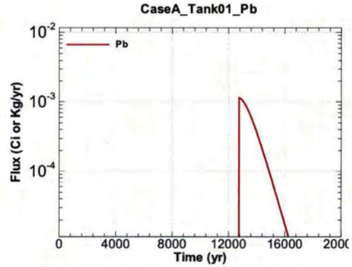
Figure A.1-44 - Flux Leaving Liner for CaseA Tank01 Pb
