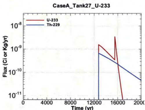
Figure A.1-1007 - Flux Leaving Liner for CaseA Tank27 U-233
