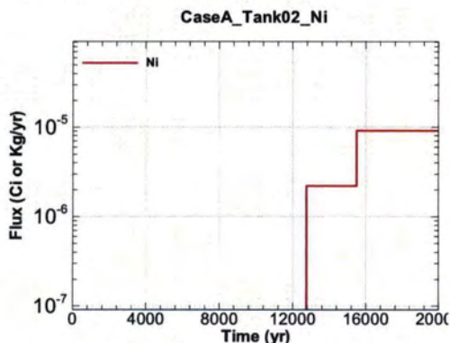
Figure A.1-117 - Flux Leaving Liner for CaseA Tank02 Ni
