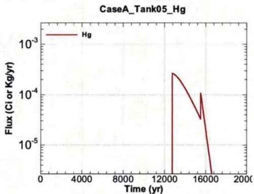
Figure A.1-345 - Flux Leaving Liner for CaseA Tank05 Hg
