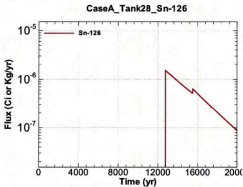
Figure A.1-1077 - Flux Leaving Liner for CaseA Tank28 Sn-126
