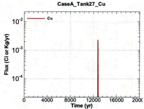
Figure A.1-962 - Flux Leaving Liner for CaseA Tank27 Cu
