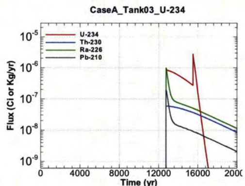
Figure A.1-228 - Flux Leaving Liner for CaseA Tank03 U-234
