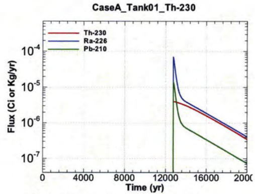
Figure A.1-68 - Flux Leaving Liner for CaseA Tank01 Th-230
