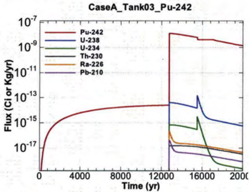
Figure A.1-207 - Flux Leaving Liner for CaseA Tank03 Pu-242
