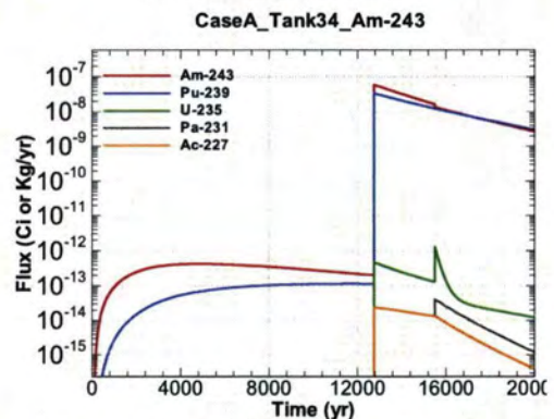
Figure A.1-708 - Flux Leaving Liner for CaseA Tank34 Am-243
