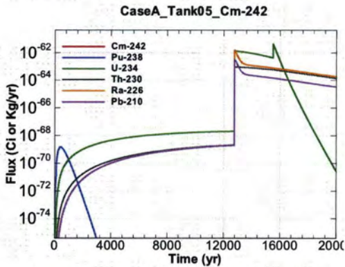
Figure A.1-327 - Flux Leaving Liner for CaseA Tank05 Cm-242
