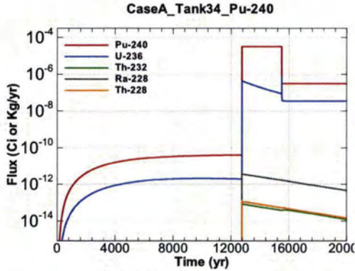
Figure A.1-751 - Flux Leaving Liner for CaseA Tank34 Pu-240
