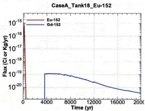
Figure A.1-1509 - Flux Leaving Liner for CaseA Tank18 Eu-152
