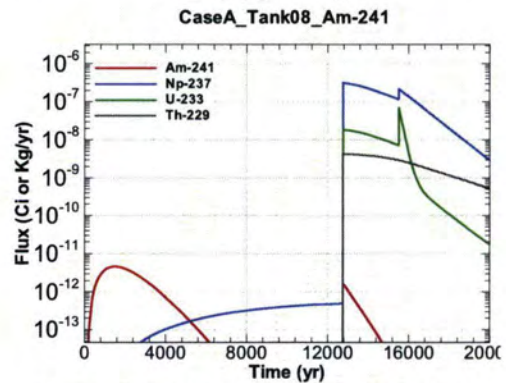
Figure A.1-550 - Flux Leaving Liner for CaseA Tank08 Am-241
