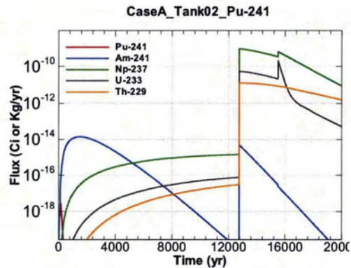
Figure A.1-128 - Flux Leaving Liner for CaseA Tank02 Pu-241
