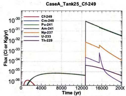
Figure A.1-794 - Flux Leaving Liner for CaseA Tank25 Cf-249
