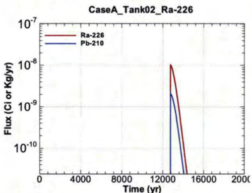
Figure A.1-131 - Flux Leaving Liner for CaseA Tank02 Ra-226
