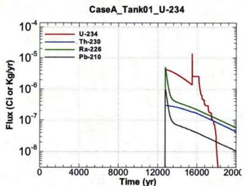
Figure A.1-72 - Flux Leaving Liner for CaseA Tank01 U-234
