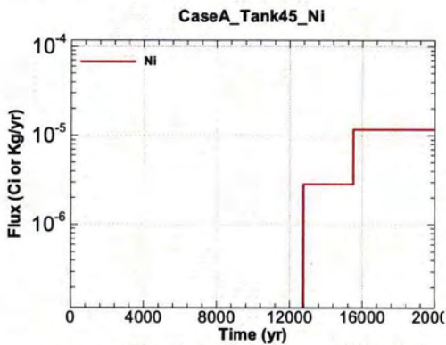
Figure A.1-1209 - Flux Leaving Liner for CaseA Tank45 Ni
