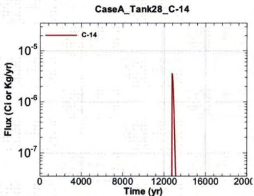
Figure A.1-1025 - Flux Leaving Liner for CaseA Tank28 C-14
