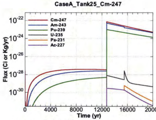
Figure A.1-799 - Flux Leaving Liner for CaseA Tank25 Cm-247
