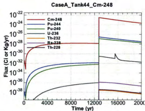
Figure A.1-1112 - Flux Leaving Liner for CaseA Tank44 Cm-248
