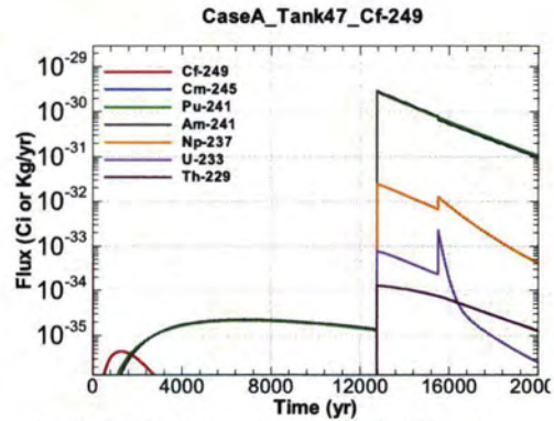
Figure A.1-1340 - Flux Leaving Liner for CaseA Tank47 Cf-249
