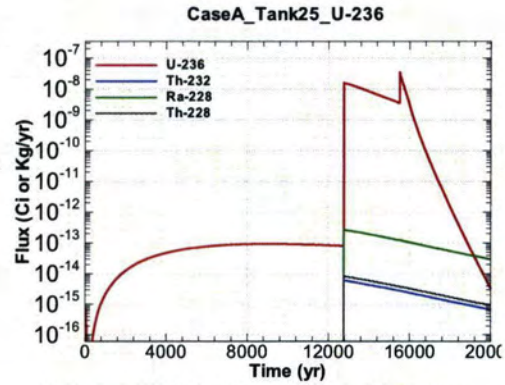
Figure A.1-854 - Flux Leaving Liner for CaseA Tank25 U-236
