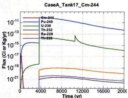
Figure A.1-1421 - Flux Leaving Liner for CaseA Tank17 Cm-244
