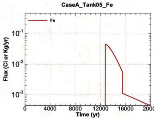
Figure A.1-343 - Flux Leaving Liner for CaseA Tank05 Fe
