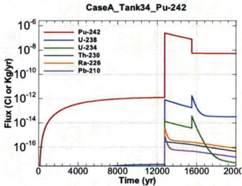
Figure A.1-753 - Flux Leaving Liner for CaseA Tank34 Pu-242
