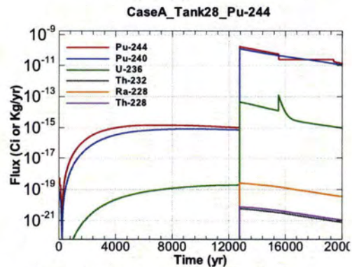
Figure A.1-1066 - Flux Leaving Liner for CaseA Tank28 Pu-244
