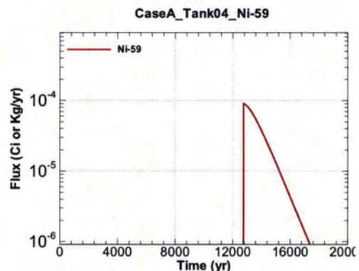
Figure A.1-274 - Flux Leaving Liner for CaseA Tank04 Ni-59
