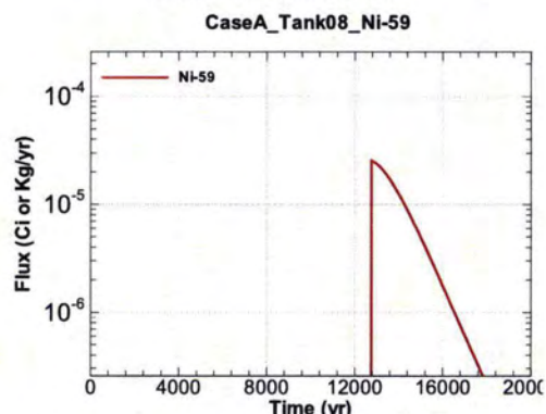
Figure A.1-586 - Flux Leaving Liner for CaseA Tank08 Ni-59
