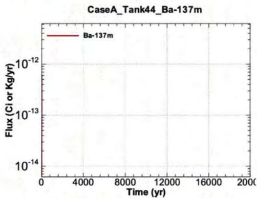
Figure A.1-1101 - Flux Leaving Liner for CaseA Tank44 Ba-137m
