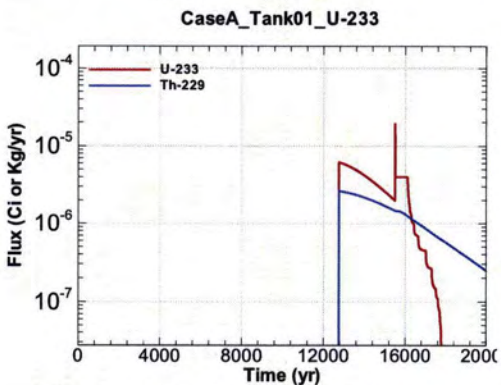
Figure A.1-71 - Flux Leaving Liner for CaseA Tank01 U-233
