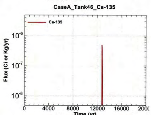
Figure A.1-1272 - Flux Leaving Liner for CaseA Tank46 Cs-135
