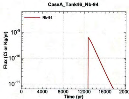
Figure A.1-1286 - Flux Leaving Liner for CaseA Tank46 Nb-94
