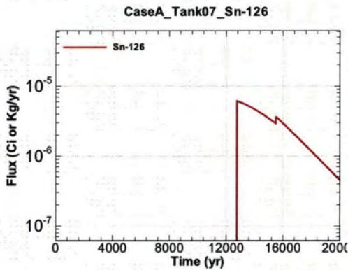
Figure A.1-531 - Flux Leaving Liner for CaseA Tank07 Sn-126
