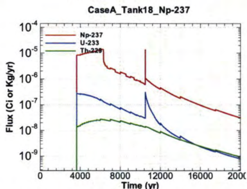
Figure A.1-1524 - Flux Leaving Liner for CaseA Tank18 Np-237
