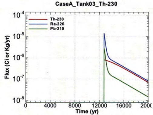
Figure A.1-224 - Flux Leaving Liner for CaseA Tank03 Th-230
