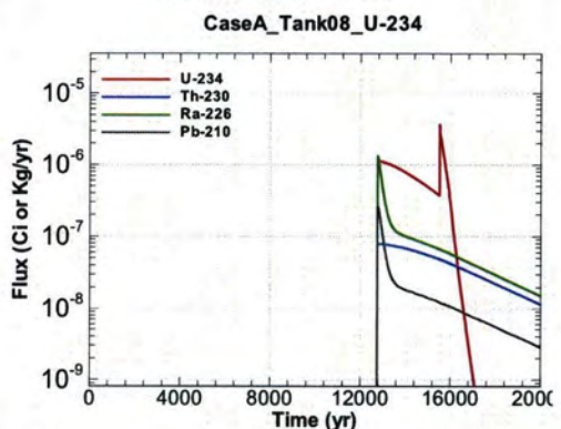
Figure A.1-618 - Flux Leaving Liner for CaseA Tank08 U-234
