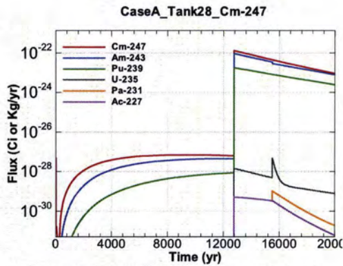
Figure A.1-1033 - Flux Leaving Liner for CaseA Tank28 Cm-247
