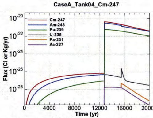
Figure A.1-253 - Flux Leaving Liner for CaseA Tank04 Cm-247
