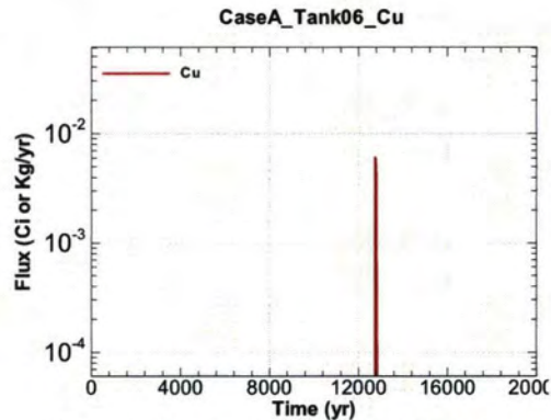
Figure A.1-416 - Flux Leaving Liner for CaseA Tank06 Cu
