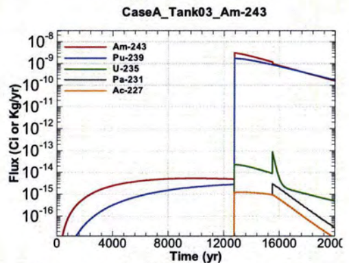
Figure A.1-162 - Flux Leaving Liner for CaseA Tank03 Am-243
