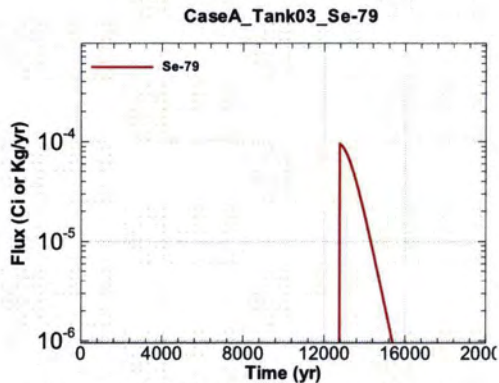
Figure A.1-217 - Flux Leaving Liner for CaseA Tank03 Se-79
