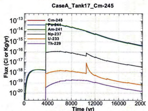
Figure A.1-1422 - Flux Leaving Liner for CaseA Tank17 Cm-245
