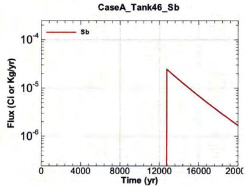
Figure A.1-1304 - Flux Leaving Liner for CaseA Tank46 Sb
