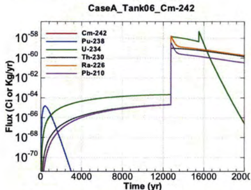
Figure A.1-405 - Flux Leaving Liner for CaseA Tank06 Cm-242
