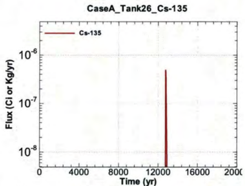
Figure A.1-882 - Flux Leaving Liner for CaseA Tank26 Cs-135
