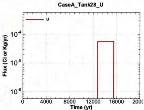
Figure A.1-1083 - Flux Leaving Liner for CaseA Tank28 U
