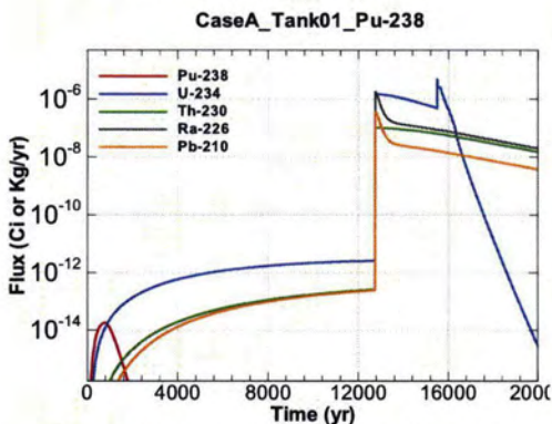
Figure A.1-47 - Flux Leaving Liner for CaseA Tank01 Pu-238
