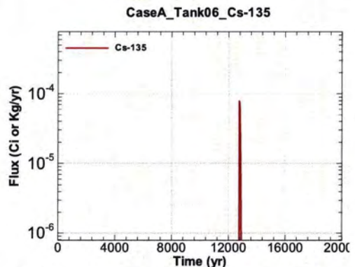
Figure A.1-414 - Flux Leaving Liner for CaseA Tank06 Cs-135
