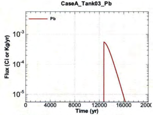
Figure A.1-200 - Flux Leaving Liner for CaseA Tank03 Pb
