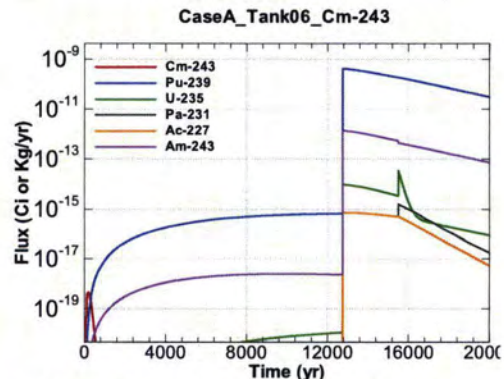
Figure A.1-406 - Flux Leaving Liner for CaseA Tank06 Cm-243
