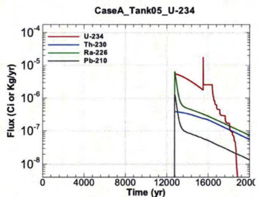
Figure A.1-384 - Flux Leaving Liner for CaseA Tank05 U-234
