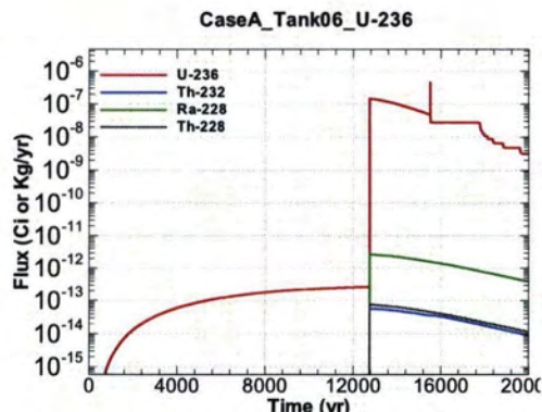
Figure A.1-464 - Flux Leaving Liner for CaseA Tank06 U-236
