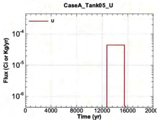
Figure A.1-381 - Flux Leaving Liner for CaseA Tank05 U
