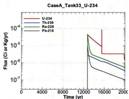
Figure A.1-696 - Flux Leaving Liner for CaseA Tank33 U-234
