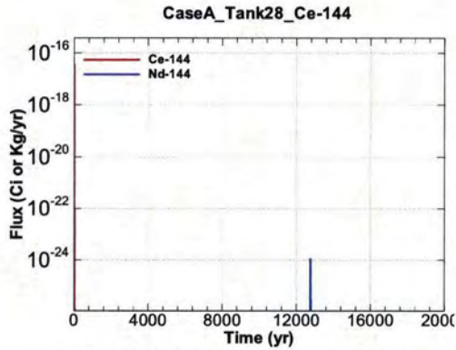
Figure A.1-1027 - Flux Leaving Liner for CaseA Tank28 Ce-144
