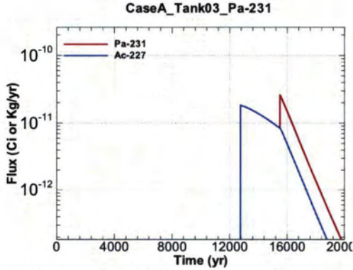
Figure A.1-199 - Flux Leaving Liner for CaseA Tank03 Pa-231
