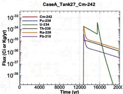
Figure A.1-951 - Flux Leaving Liner for CaseA Tank27 Cm-242
