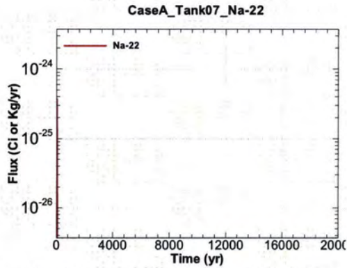
Figure A.1-505 - Flux Leaving Liner for CaseA Tank07 Na-22
