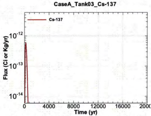
Figure A.1-181 - Flux Leaving Liner for CaseA Tank03 Cs-137
