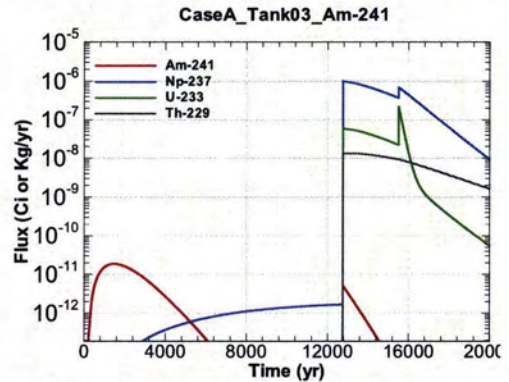
Figure A.1-160 - Flux Leaving Liner for CaseA Tank03 Am-241
