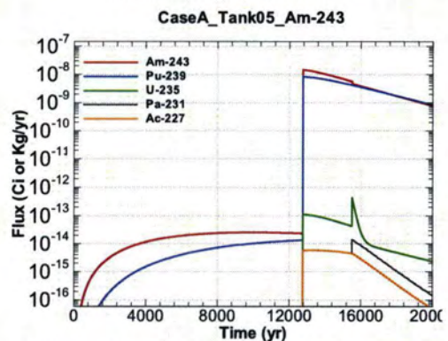
Figure A.1-318 - Flux Leaving Liner for CaseA Tank05 Am-243
