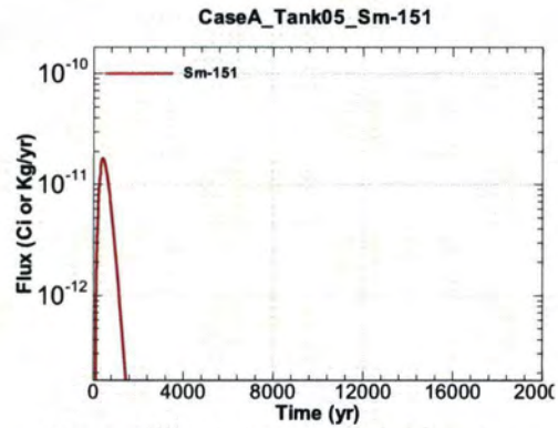
Figure A.1-374 - Flux Leaving Liner for CaseA Tank05 Sm-151
