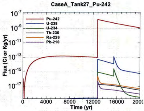
Figure A.1-987 - Flux Leaving Liner for CaseA Tank27 Pu-242
