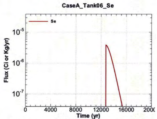
Figure A.1-450 - Flux Leaving Liner for CaseA Tank06 Se
