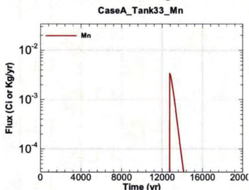
Figure A.1-659 - Flux Leaving Liner for CaseA Tank33 Mn
