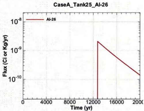
Figure A.1-783 - Flux Leaving Liner for CaseA Tank25 Al-26
