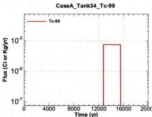
Figure A.1-767 - Flux Leaving Liner for CaseA Tank34 Tc-99
