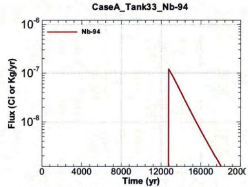
Figure A.1-662 - Flux Leaving Liner for CaseA Tank33 Nb-94
