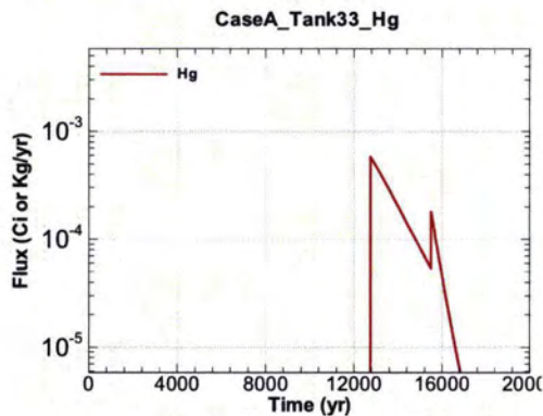
Figure A.1-657 - Flux Leaving Liner for CaseA Tank33 Hg
