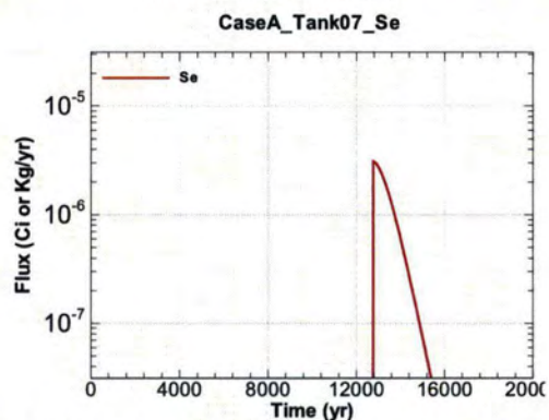
Figure A.1-528 - Flux Leaving Liner for CaseA Tank07 Se
