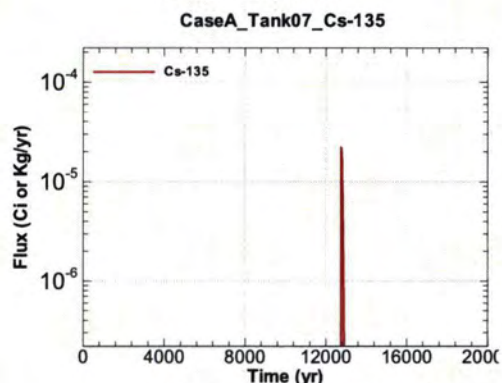
Figure A.1-492 - Flux Leaving Liner for CaseA Tank07 Cs-135
