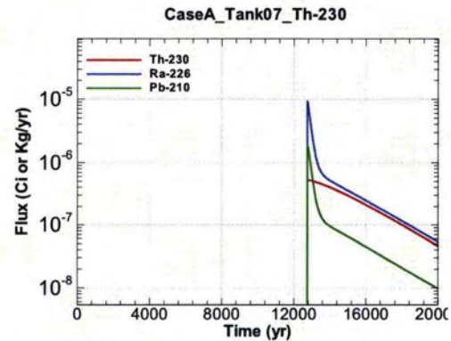
Figure A.1-536 - Flux Leaving Liner for CaseA Tank07 Th-230
