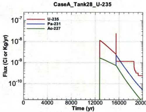
Figure A.1-1087 - Flux Leaving Liner for CaseA Tank28 U-235
