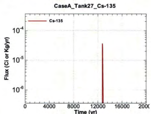
Figure A.1-960 - Flux Leaving Liner for CaseA Tank27 Cs-135
