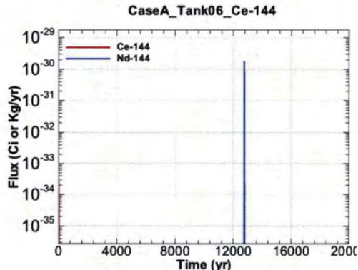
Figure A.1-403 - Flux Leaving Liner for CaseA Tank06 Ce-144
