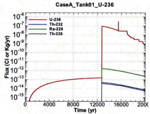
Figure A.1-74 - Flux Leaving Liner for CaseA Tank01 U-236
