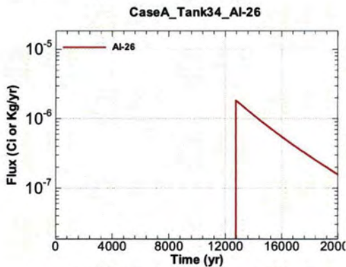
Figure A.1-705 - Flux Leaving Liner for CaseA Tank34 Al-26
