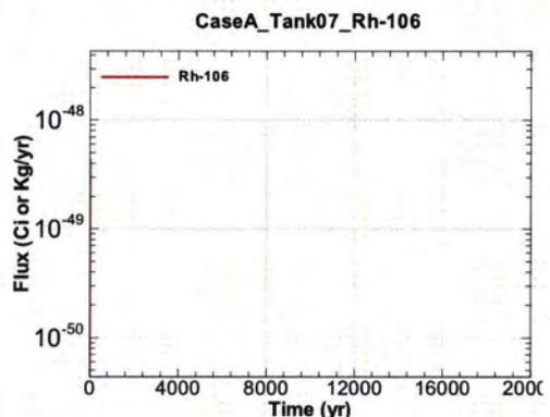
Figure A.1-522 - Flux Leaving Liner for CaseA Tank07 Rh-106
