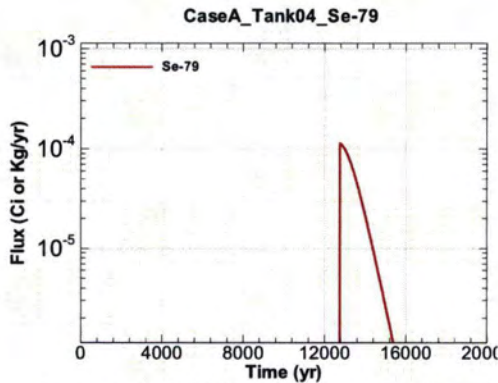
Figure A.1-295 - Flux Leaving Liner for CaseA Tank04 Se-79
