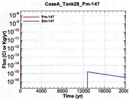
Figure A.1-1059 - Flux Leaving Liner for CaseA Tank28 Pm-147
