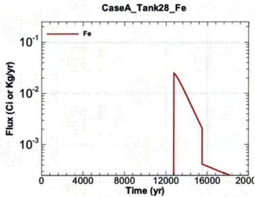
Figure A.1-1045 - Flux Leaving Liner for CaseA Tank28 Fe
