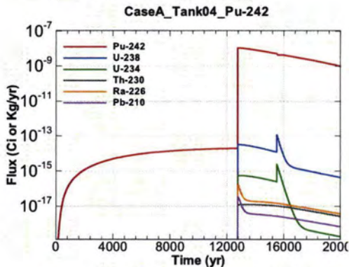
Figure A.1-285 - Flux Leaving Liner for CaseA Tank04 Pu-242
