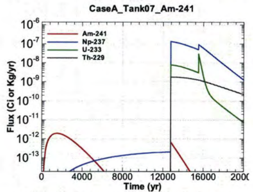
Figure A.1-472 - Flux Leaving Liner for CaseA Tank07 Am-241
