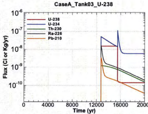
Figure A.1-231 - Flux Leaving Liner for CaseA Tank03 U-238
