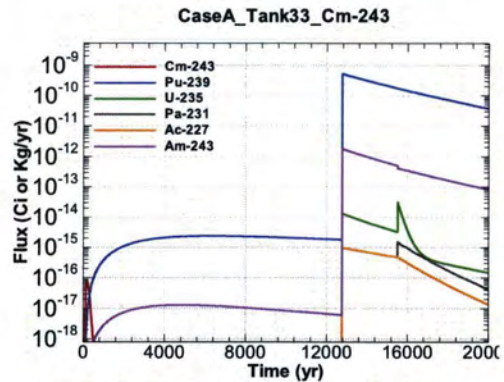
Figure A.1-640 - Flux Leaving Liner for CaseA Tank33 Cm-243
