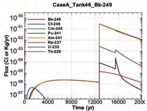
Figure A.1-1258 - Flux Leaving Liner for CaseA Tank46 Bk-249
