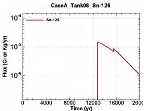
Figure A.1-609 - Flux Leaving Liner for CaseA Tank08 Sn-126
