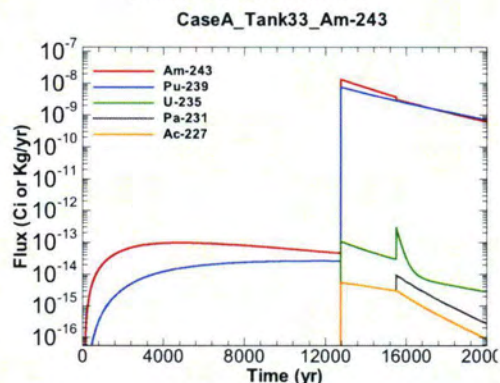
Figure A.1-630 - Flux Leaving Liner for CaseA Tank33 Am-243
