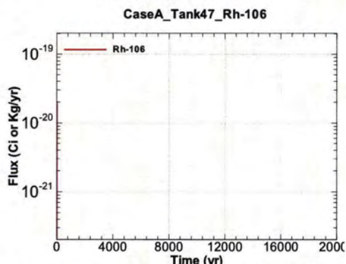
Figure A.1-1380 - Flux Leaving Liner for CaseA Tank47 Rh-106
