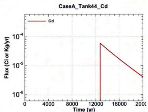
Figure A.1-1104 - Flux Leaving Liner for CaseA Tank44 Cd
