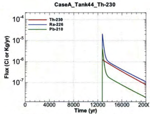
Figure A.1-1160 - Flux Leaving Liner for CaseA Tank44 Th-230
