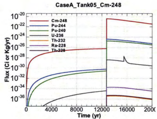
Figure A.1-332 - Flux Leaving Liner for CaseA Tank05 Cm-248
