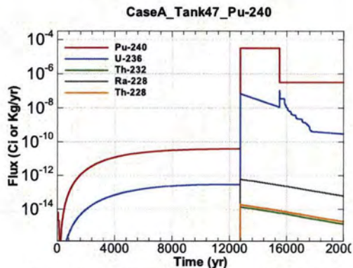
Figure A.1-1375 - Flux Leaving Liner for CaseA Tank47 Pu-240
