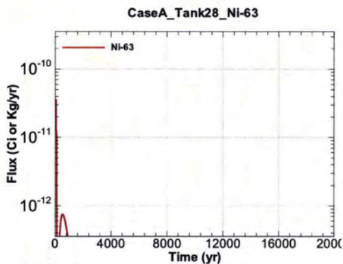
Figure A.1-1055 - Flux Leaving Liner for CaseA Tank28 Ni-63
