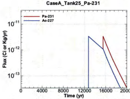
Figure A.1-823 - Flux Leaving Liner for CaseA Tank25 Pa-231
