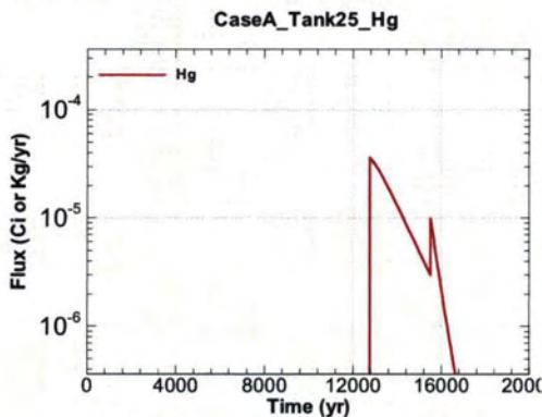
Figure A.1-813 - Flux Leaving Liner for CaseA Tank25 Hg
