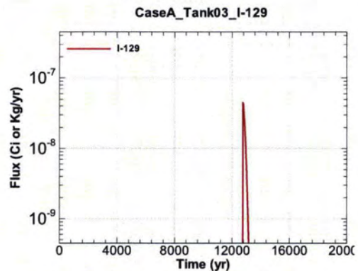
Figure A.1-190 - Flux Leaving Liner for CaseA Tank03 I-129
