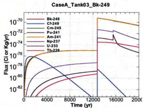
Figure A.1-166 - Flux Leaving Liner for CaseA Tank03 Bk-249
