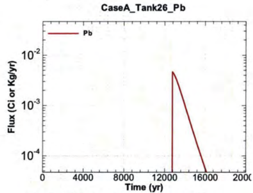
Figure A.1-902 - Flux Leaving Liner for CaseA Tank26 Pb
