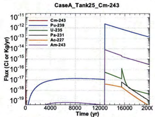
Figure A.1-796 - Flux Leaving Liner for CaseA Tank25 Cm-243
