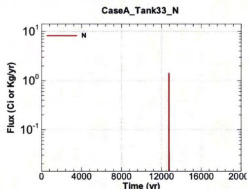
Figure A.1-660 - Flux Leaving Liner for CaseA Tank33 N
