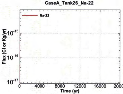
Figure A.1-895 - Flux Leaving Liner for CaseA Tank26 Na-22
