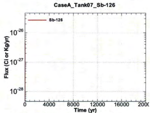
Figure A.1-526 - Flux Leaving Liner for CaseA Tank07 Sb-126
