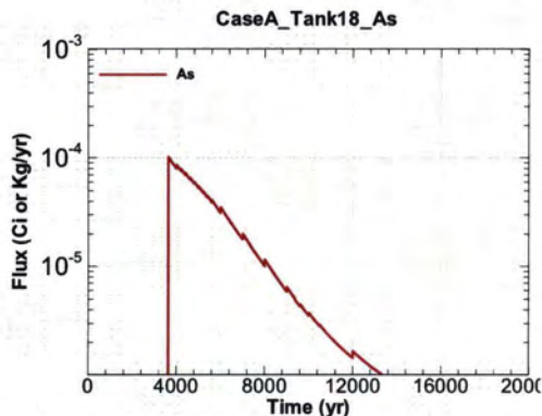
Figure A.1-1489 - Flux Leaving Liner for CaseA Tank18 As
