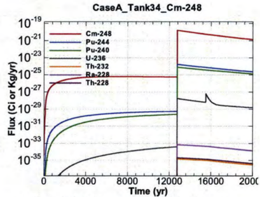
Figure A.1-722 - Flux Leaving Liner for CaseA Tank34 Cm-248
