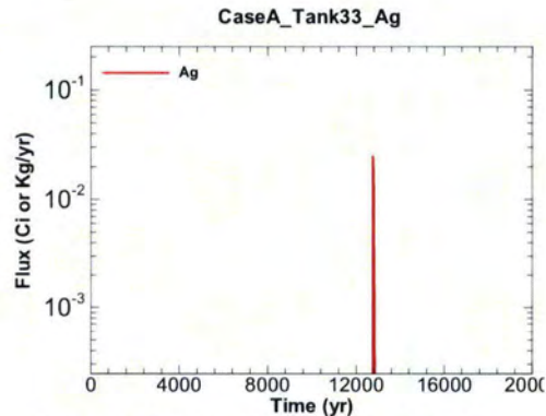
Figure A.1-626 - Flux Leaving Liner for CaseA Tank33 Ag
