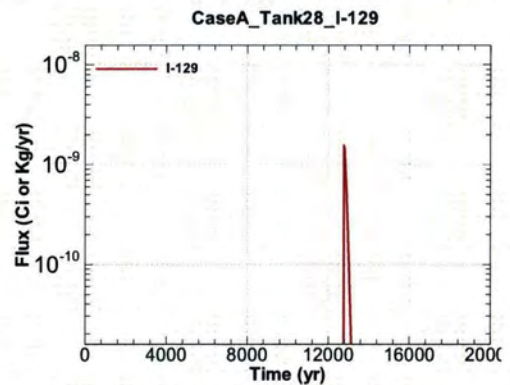
Figure A.1-1048 - Flux Leaving Liner for CaseA Tank28 I-129
