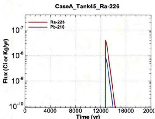
Figure A.1-1223 - Flux Leaving Liner for CaseA Tank45 Ra-226
