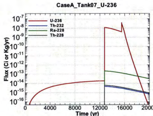
Figure A.1-542 - Flux Leaving Liner for CaseA Tank07 U-236
