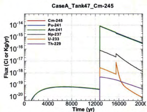
Figure A.1-1344 - Flux Leaving Liner for CaseA Tank47 Cm-245
