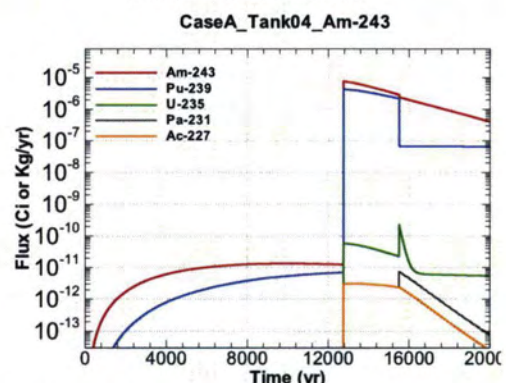
Figure A.1-240 - Flux Leaving Liner for CaseA Tank04 Am-243
