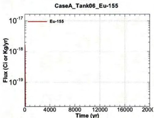
Figure A.1-419 - Flux Leaving Liner for CaseA Tank06 Eu-155
