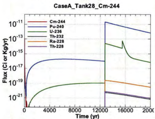
Figure A.1-1031 - Flux Leaving Liner for CaseA Tank28 Cm-244
