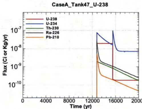
Figure A.1-1401 - Flux Leaving Liner for CaseA Tank47 U-238
