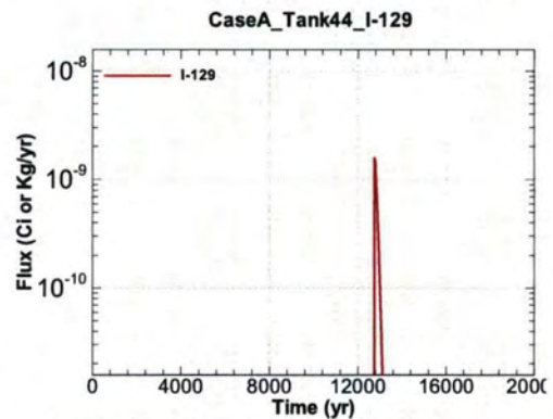
Figure A.1-1126 - Flux Leaving Liner for CaseA Tank44 I-129
