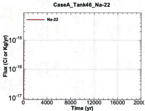
Figure A.1-1285 - Flux Leaving Liner for CaseA Tank46 Na-22
