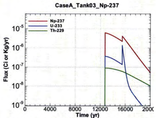
Figure A.1-198 - Flux Leaving Liner for CaseA Tank03 Np-237
