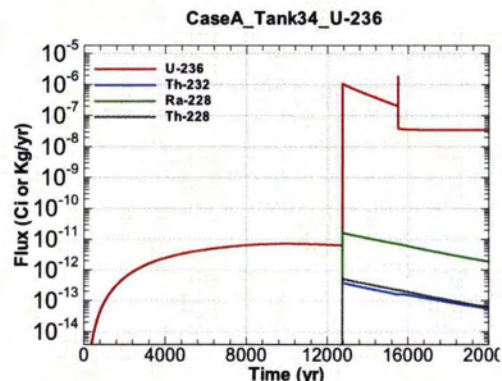
Figure A.1-776 - Flux Leaving Liner for CaseA Tank34 U-236
