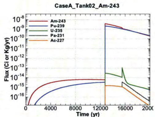
Figure A.1-84 - Flux Leaving Liner for CaseA Tank02 Am-243
