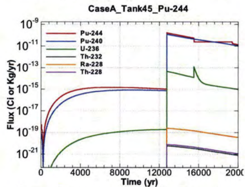
Figure A.1-1222 - Flux Leaving Liner for CaseA Tank45 Pu-244
