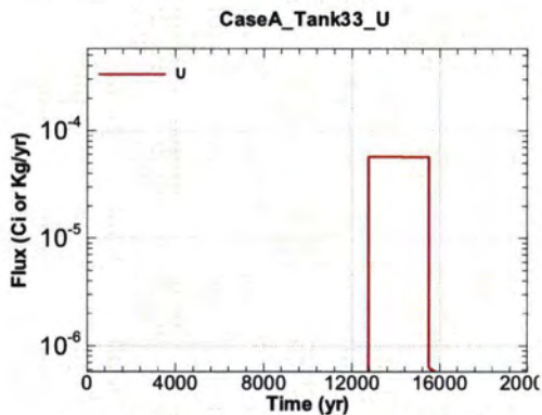
Figure A.1-693 - Flux Leaving Liner for CaseA Tank33 U
