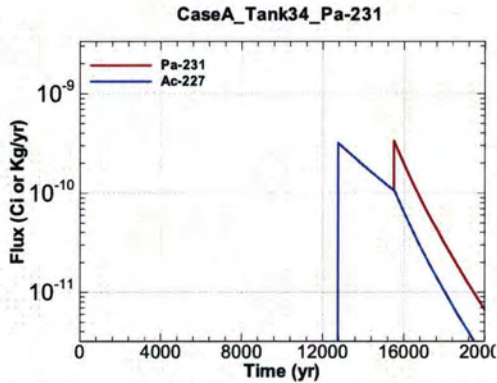
Figure A.1-745 - Flux Leaving Liner for CaseA Tank34 Pa-231
