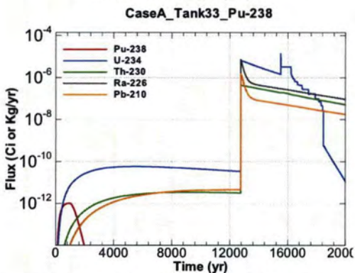
Figure A.1-671 - Flux Leaving Liner for CaseA Tank33 Pu-238
