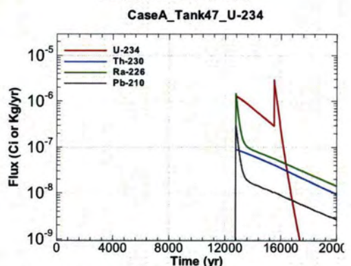
Figure A.1-1398 - Flux Leaving Liner for CaseA Tank47 U-234
