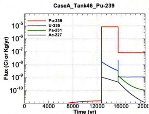
Figure A.1-1296 - Flux Leaving Liner for CaseA Tank46 Pu-239
