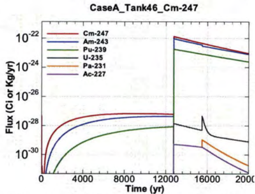
Figure A.1-1267 - Flux Leaving Liner for CaseA Tank46 Cm-247
