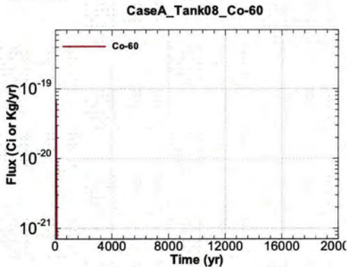
Figure A.1-567 - Flux Leaving Liner for CaseA Tank08 Co-60
