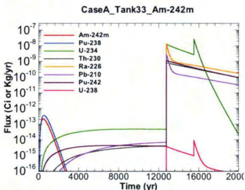
Figure A.1-629 - Flux Leaving Liner for CaseA Tank33 Am-242m
