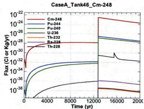
Figure A.1-1268 - Flux Leaving Liner for CaseA Tank46 Cm-248
