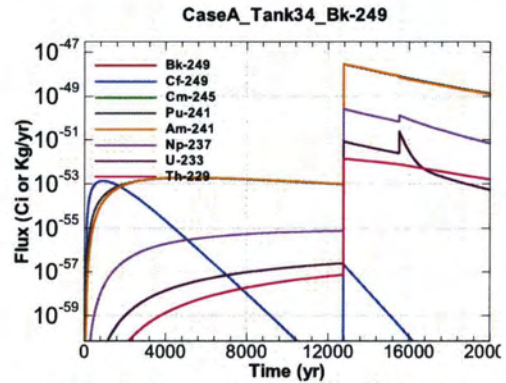
Figure A.1-712 - Flux Leaving Liner for CaseA Tank34 Bk-249
