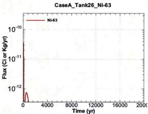
Figure A.1-899 - Flux Leaving Liner for CaseA Tank26 Ni-63
