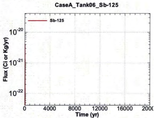
Figure A.1-447 - Flux Leaving Liner for CaseA Tank06 Sb-125
