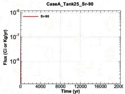
Figure A.1-844 - Flux Leaving Liner for CaseA Tank25 Sr-90
