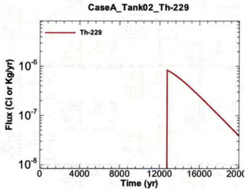
Figure A.1-145 - Flux Leaving Liner for CaseA Tank02 Th-229
