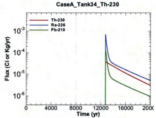
Figure A.1-770 - Flux Leaving Liner for CaseA Tank34 Th-230
