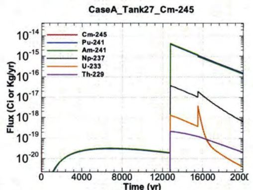
Figure A.1-954 - Flux Leaving Liner for CaseA Tank27 Cm-245
