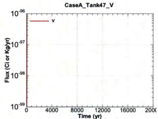
Figure A.1-1402 - Flux Leaving Liner for CaseA Tank47 V
