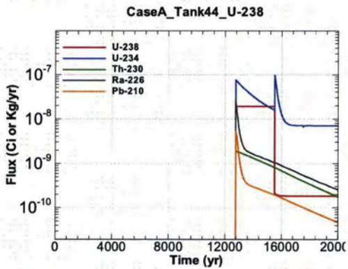
Figure A.1-1167 - Flux Leaving Liner for CaseA Tank44 U-238
