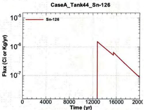
Figure A.1-1155 - Flux Leaving Liner for CaseA Tank44 Sn-126
