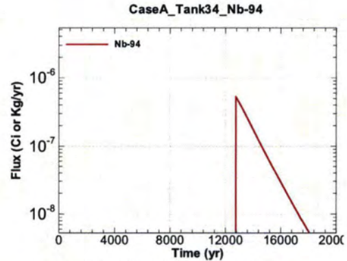
Figure A.1-740 - Flux Leaving Liner for CaseA Tank34 Nb-94
