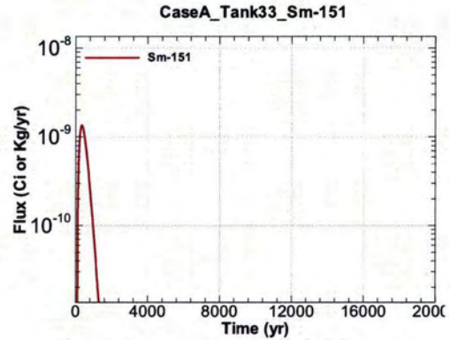
Figure A.1-686 - Flux Leaving Liner for CaseA Tank33 Sm-151
