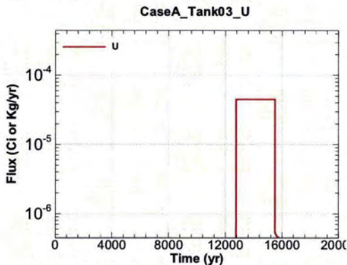
Figure A.1-225 - Flux Leaving Liner for CaseA Tank03 U
