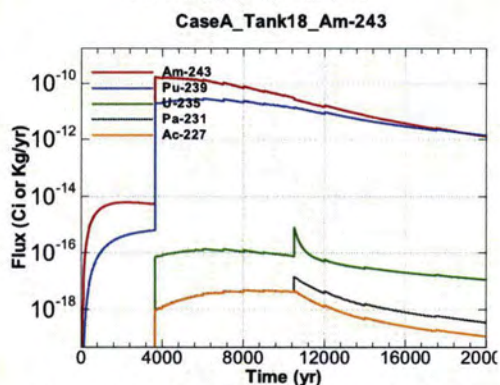
Figure A.1-1488 - Flux Leaving Liner for CaseA Tank18 Am-243
