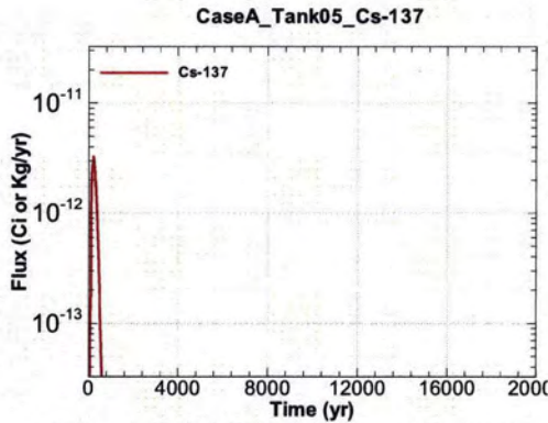
Figure A.1-337 - Flux Leaving Liner for CaseA Tank05 Cs-137
