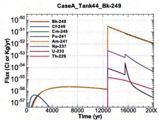
Figure A.1-1102 - Flux Leaving Liner for CaseA Tank44 Bk-249
