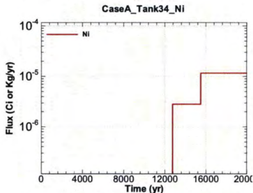
Figure A.1-741 - Flux Leaving Liner for CaseA Tank34 Ni
