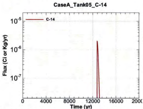
Figure A.1-323 - Flux Leaving Liner for CaseA Tank05 C-14
