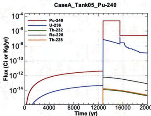
Figure A.1-361 - Flux Leaving Liner for CaseA Tank05 Pu-240
