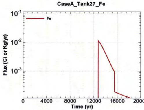
Figure A.1-967 - Flux Leaving Liner for CaseA Tank27 Fe
