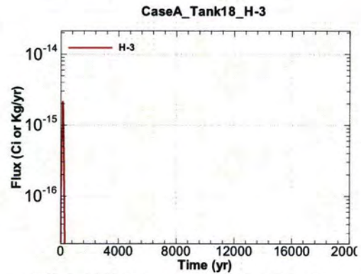
Figure A.1-1514 - Flux Leaving Liner for CaseA Tank18 H-3
