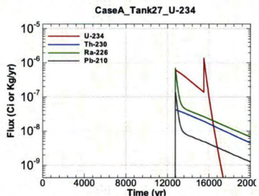
Figure A.1-1008 - Flux Leaving Liner for CaseA Tank27 U-234
