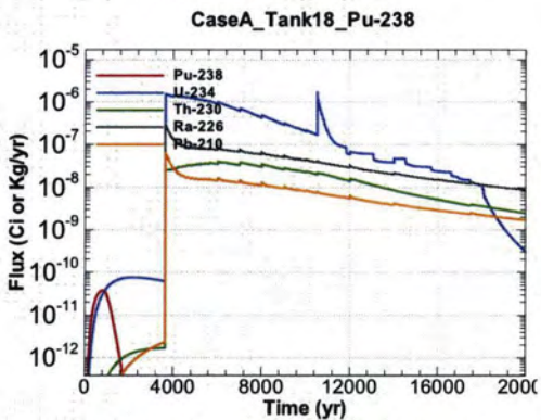
Figure A.1-1529 - Flux Leaving Liner for CaseA Tank18 Pu-238
