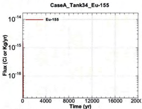
Figure A.1-731 - Flux Leaving Liner for CaseA Tank34 Eu-155
