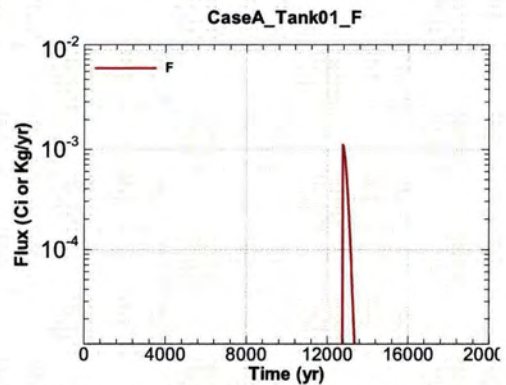
Figure A.1-30 - Flux Leaving Liner for CaseA Tank01 F
