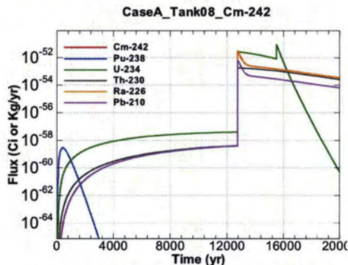
Figure A.1-561 - Flux Leaving Liner for CaseA Tank08 Cm-242
