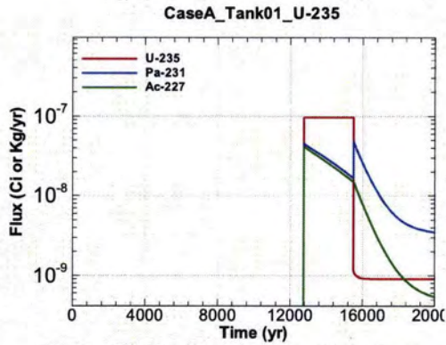
Figure A.1-73 - Flux Leaving Liner for CaseA Tank01 U-235
