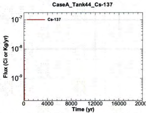
Figure A.1-1117 - Flux Leaving Liner for CaseA Tank44 Cs-137
