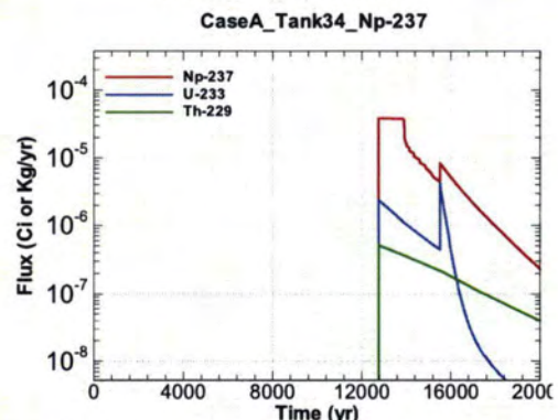
Figure A.1-744 - Flux Leaving Liner for CaseA Tank34 Np-237
