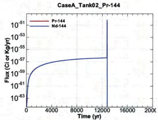
Figure A.1-124 - Flux Leaving Liner for CaseA Tank02 Pr-144
