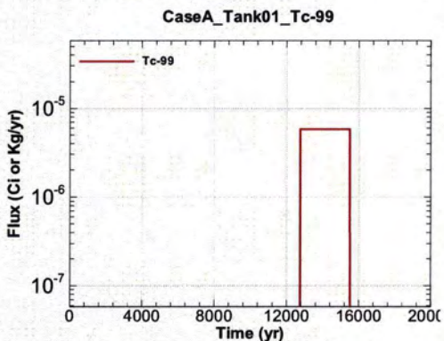
Figure A.1-65 - Flux Leaving Liner for CaseA Tank01 Tc-99
