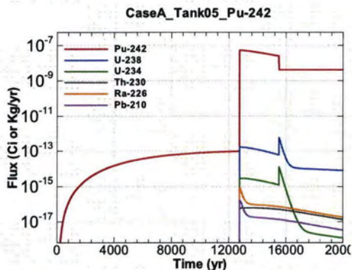
Figure A.1-363 - Flux Leaving Liner for CaseA Tank05 Pu-242
