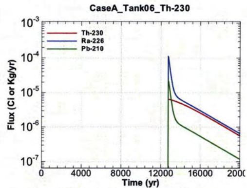
Figure A.1-458 - Flux Leaving Liner for CaseA Tank06 Th-230
