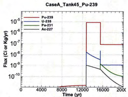
Figure A.1-1218 - Flux Leaving Liner for CaseA Tank45 Pu-239
