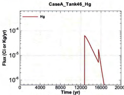
Figure A.1-1281 - Flux Leaving Liner for CaseA Tank46 Hg
