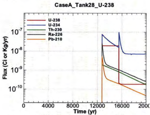
Figure A.1-1089 - Flux Leaving Liner for CaseA Tank28 U-238
