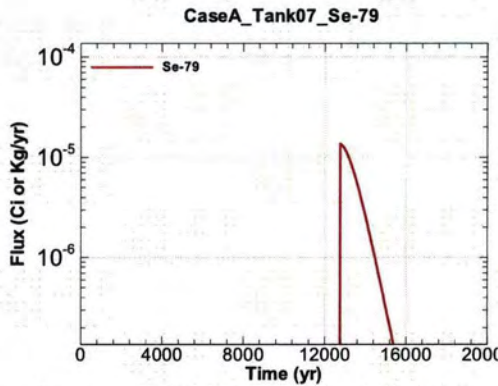
Figure A.1-529 - Flux Leaving Liner for CaseA Tank07 Se-79
