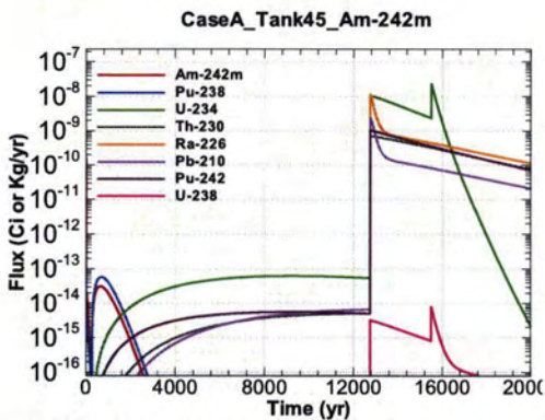
Figure A.1-1175 - Flux Leaving Liner for CaseA Tank45 Am-242m
