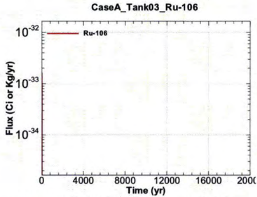
Figure A.1-211 - Flux Leaving Liner for CaseA Tank03 Ru-106
