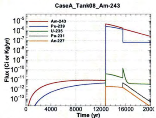
Figure A.1-552 - Flux Leaving Liner for CaseA Tank08 Am-243
