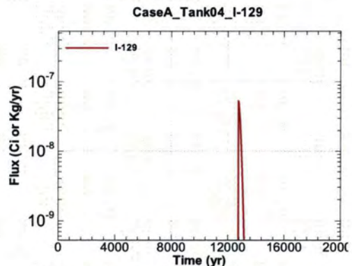
Figure A.1-268 - Flux Leaving Liner for CaseA Tank04 I-129
