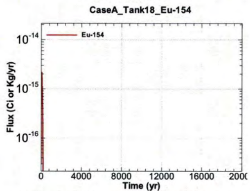
Figure A.1-1510 - Flux Leaving Liner for CaseA Tank18 Eu-154
