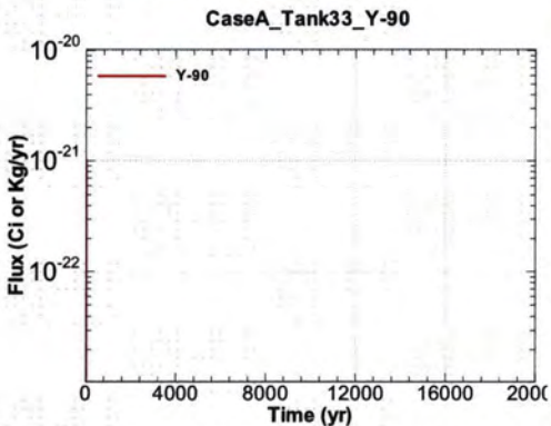
Figure A.1-701 - Flux Leaving Liner for CaseA Tank33 Y-90
