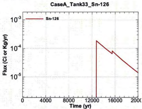
Figure A.1-687 - Flux Leaving Liner for CaseA Tank33 Sn-126
