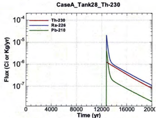
Figure A.1-1082 - Flux Leaving Liner for CaseA Tank28 Th-230
