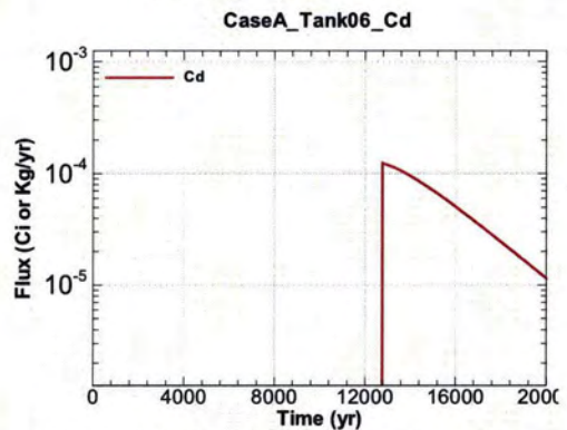
Figure A.1-402 - Flux Leaving Liner for CaseA Tank06 Cd
