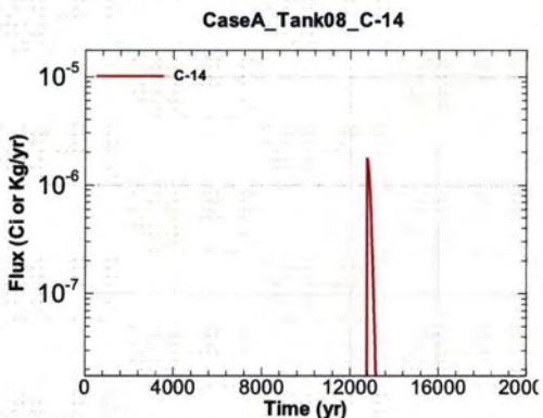
Figure A.1-557 - Flux Leaving Liner for CaseA Tank08 C-14
