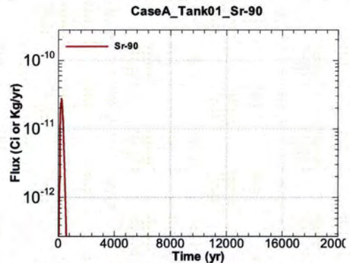
Figure A.1-64 - Flux Leaving Liner for CaseA Tank01 Sr-90
