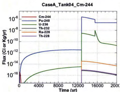
Figure A.1-251 - Flux Leaving Liner for CaseA Tank04 Cm-244
