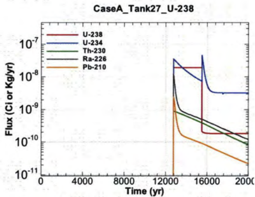
Figure A.1-1011 - Flux Leaving Liner for CaseA Tank27 U-238
