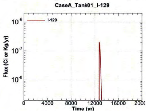
Figure A.1-34 - Flux Leaving Liner for CaseA Tank01 I-129
