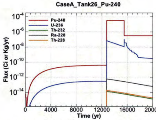
Figure A.1-907 - Flux Leaving Liner for CaseA Tank26 Pu-240
