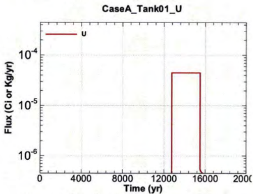
Figure A.1-69 - Flux Leaving Liner for CaseA Tank01 U
