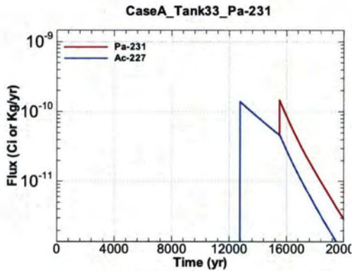
Figure A.1-667 - Flux Leaving Liner for CaseA Tank33 Pa-231
