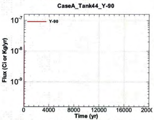
Figure A.1-1169 - Flux Leaving Liner for CaseA Tank44 Y-90
