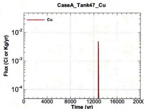
Figure A.1-1352 - Flux Leaving Liner for CaseA Tank47 Cu
