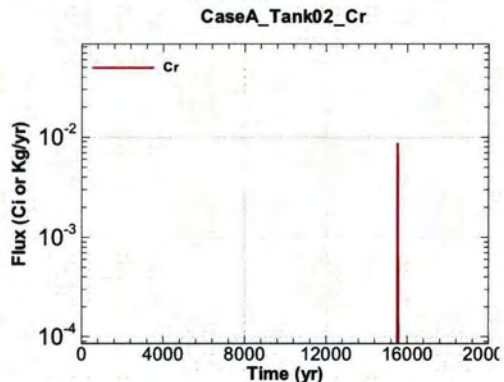
Figure A.1-100 - Flux Leaving Liner for CaseA Tank02 Cr
