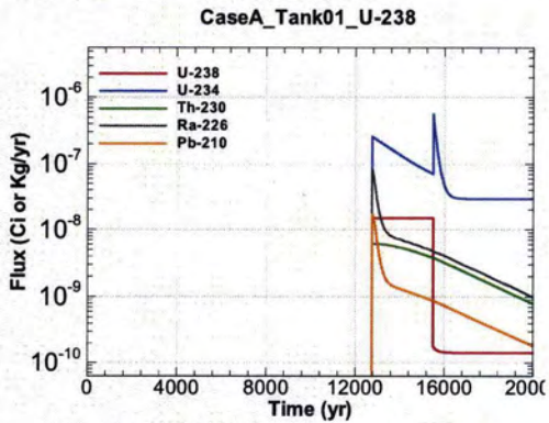
Figure A.1-75 - Flux Leaving Liner for CaseA Tank01 U-238
