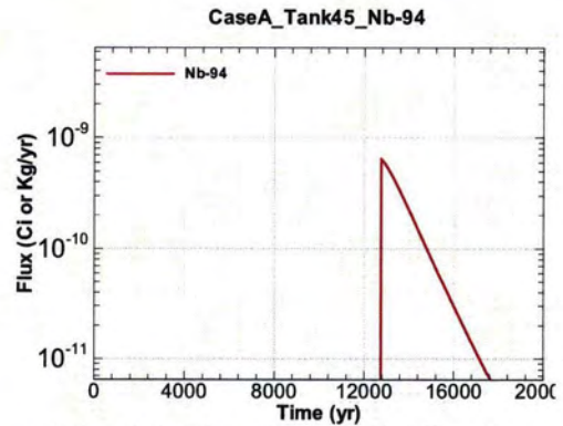
Figure A.1-1208 - Flux Leaving Liner for CaseA Tank45 Nb-94
