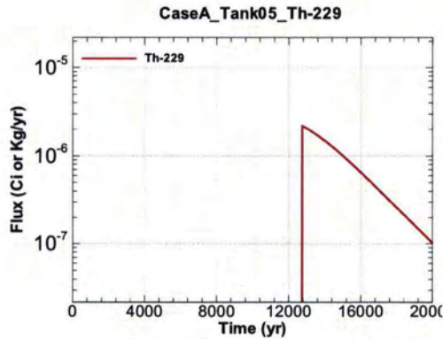
Figure A.1-379 - Flux Leaving Liner for CaseA Tank05 Th-229
