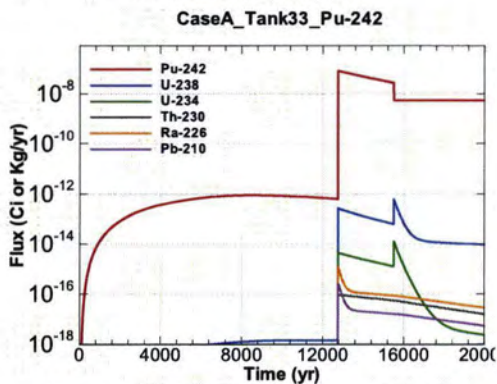
Figure A.1-675 - Flux Leaving Liner for CaseA Tank33 Pu-242
