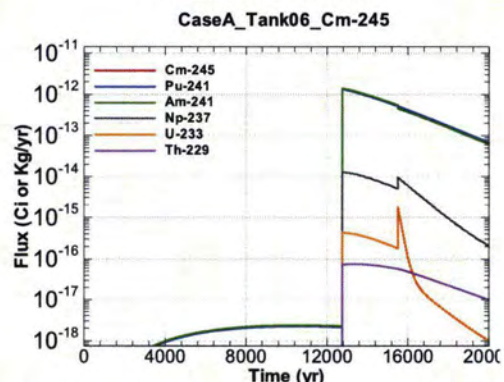
Figure A.1-408 - Flux Leaving Liner for CaseA Tank06 Cm-245
