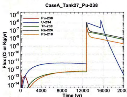
Figure A.1-983 - Flux Leaving Liner for CaseA Tank27 Pu-238
