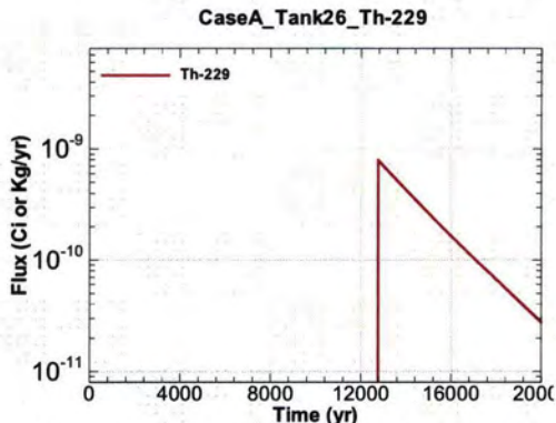
Figure A.1-925 - Flux Leaving Liner for CaseA Tank26 Th-229
