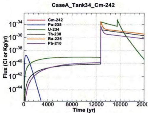
Figure A.1-717 - Flux Leaving Liner for CaseA Tank34 Cm-242
