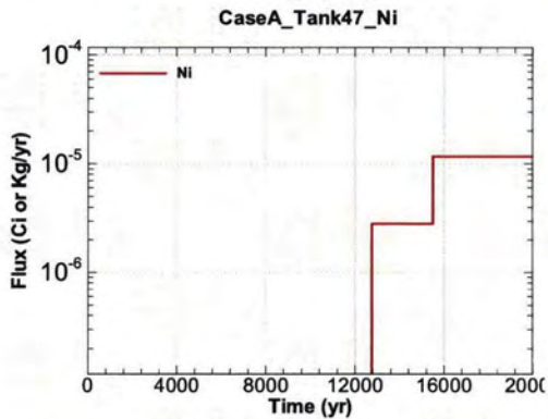
Figure A.1-1365 - Flux Leaving Liner for CaseA Tank47 Ni
