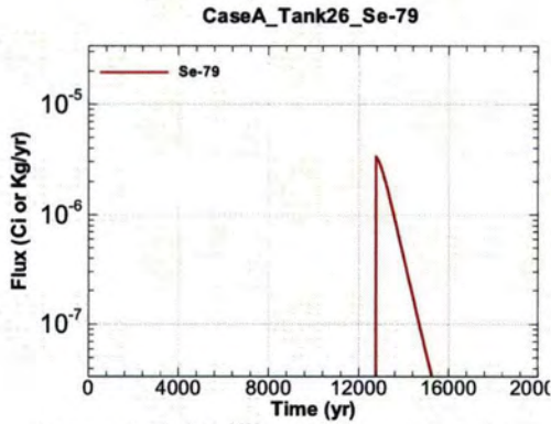
Figure A.1-919 - Flux Leaving Liner for CaseA Tank26 Se-79
