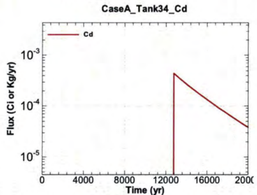
Figure A.1-714 - Flux Leaving Liner for CaseA Tank34 Cd
