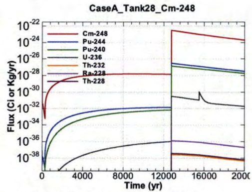
Figure A.1-1034 - Flux Leaving Liner for CaseA Tank28 Cm-248
