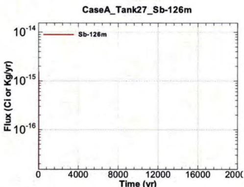
Figure A.1-995 - Flux Leaving Liner for CaseA Tank27 Sb-126m
