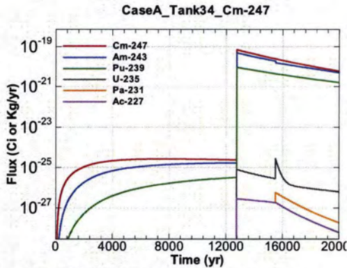
Figure A.1-721 - Flux Leaving Liner for CaseA Tank34 Cm-247
