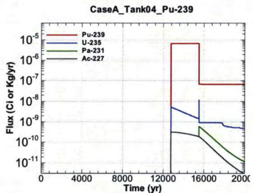
Figure A.1-282 - Flux Leaving Liner for CaseA Tank04 Pu-239
