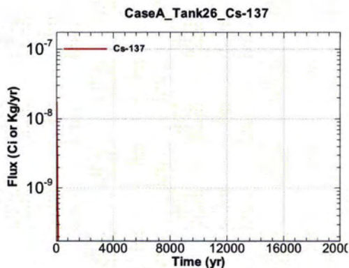
Figure A.1-883 - Flux Leaving Liner for CaseA Tank26 Cs-137
