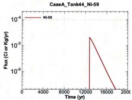
Figure A.1-1132 - Flux Leaving Liner for CaseA Tank44 Ni-59
