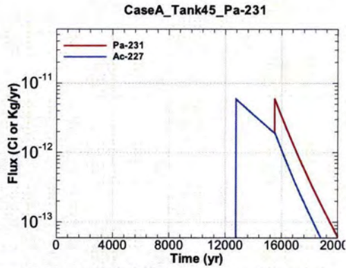
Figure A.1-1213 - Flux Leaving Liner for CaseA Tank45 Pa-231
