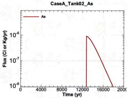
Figure A.1-85 - Flux Leaving Liner for CaseA Tank02 As
