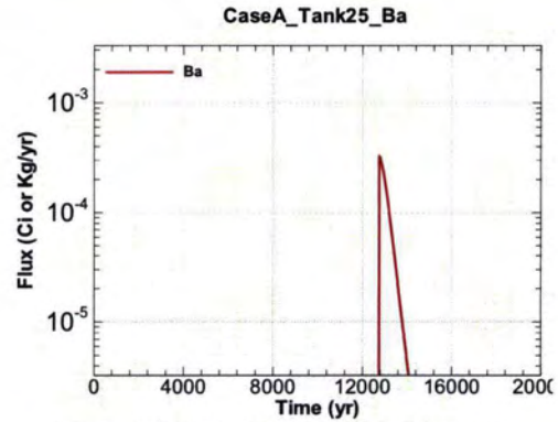
Figure A.1-788 - Flux Leaving Liner for CaseA Tank25 Ba
