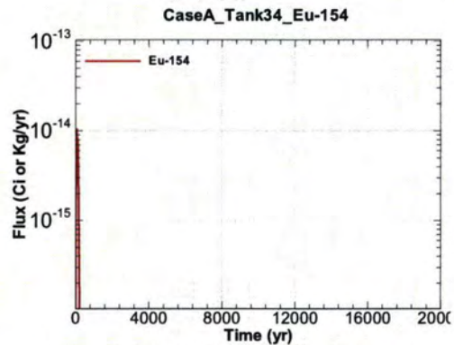
Figure A.1-730 - Flux Leaving Liner for CaseA Tank34 Eu-154
