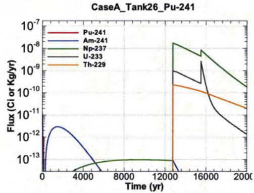
Figure A.1-908 - Flux Leaving Liner for CaseA Tank26 Pu-241
