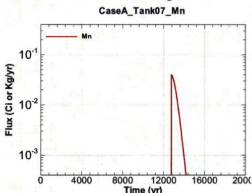
Figure A.1-503 - Flux Leaving Liner for CaseA Tank07 Mn
