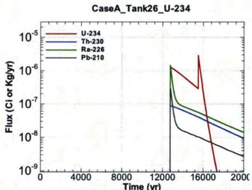
Figure A.1-930 - Flux Leaving Liner for CaseA Tank26 U-234
