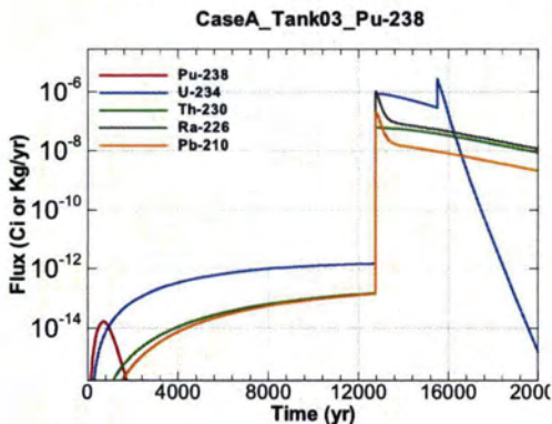
Figure A.1-203 - Flux Leaving Liner for CaseA Tank03 Pu-238
