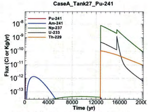
Figure A.1-986 - Flux Leaving Liner for CaseA Tank27 Pu-241
