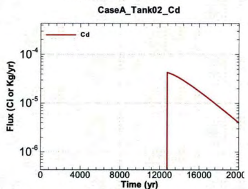
Figure A.1-90 - Flux Leaving Liner for CaseA Tank02 Cd
