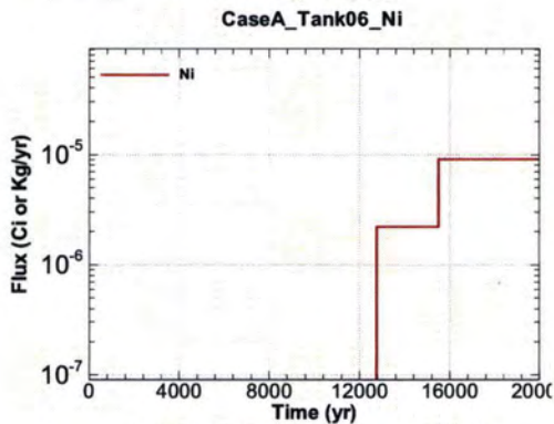
Figure A.1-429 - Flux Leaving Liner for CaseA Tank06 Ni
