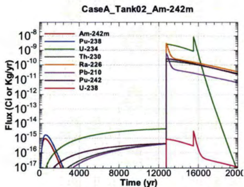
Figure A.1-83 - Flux Leaving Liner for CaseA Tank02 Am-242m
