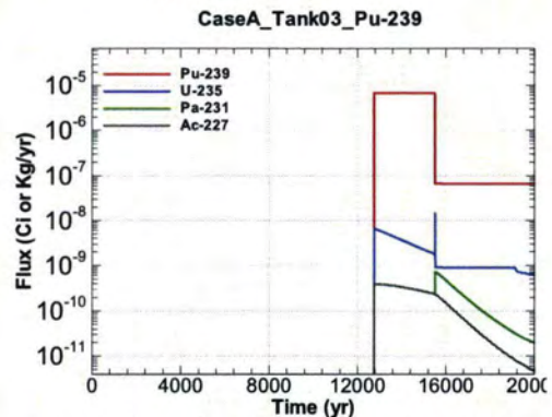
Figure A.1-204 - Flux Leaving Liner for CaseA Tank03 Pu-239
