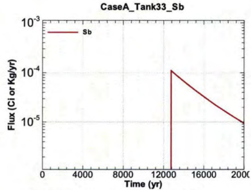
Figure A.1-680 - Flux Leaving Liner for CaseA Tank33 Sb
