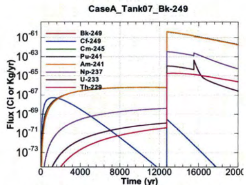
Figure A.1-478 - Flux Leaving Liner for CaseA Tank07 Bk-249
