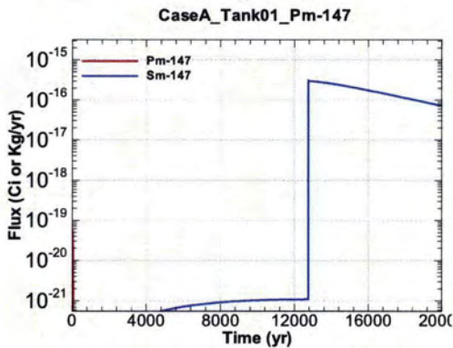
Figure A.1-45 - Flux Leaving Liner for CaseA Tank01 Pm-147
