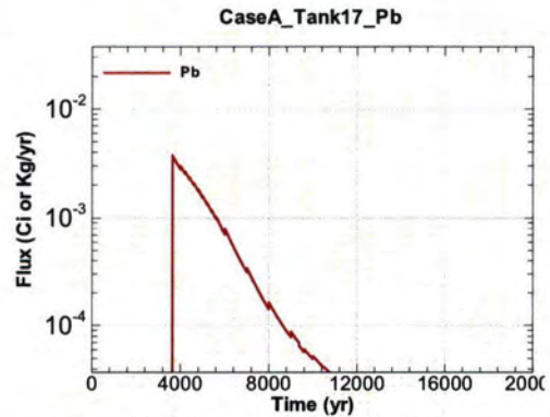
Figure A.1-1448 - Flux Leaving Liner for CaseA Tank17 Pb
