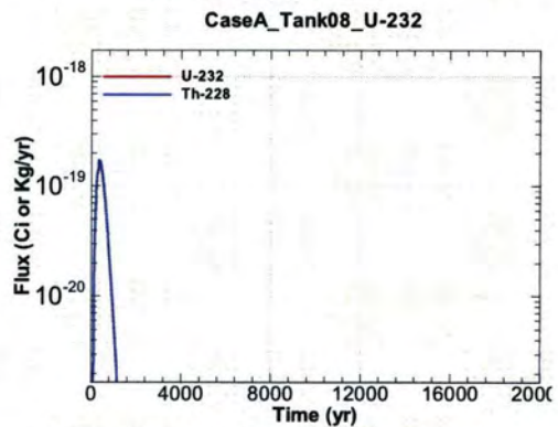
Figure A.1-616 - Flux Leaving Liner for CaseA Tank08 U-232
