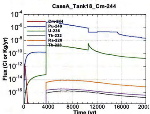
Figure A.1-1499 - Flux Leaving Liner for CaseA Tank18 Cm-244
