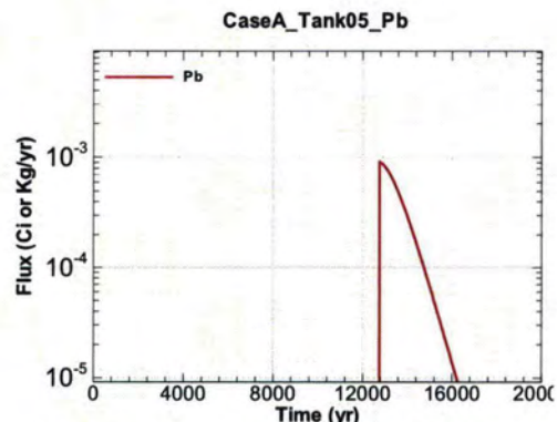
Figure A.1-356 - Flux Leaving Liner for CaseA Tank05 Pb
