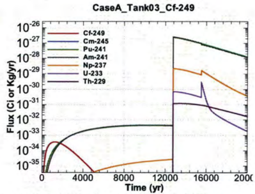
Figure A.1-170 - Flux Leaving Liner for CaseA Tank03 Cf-249
