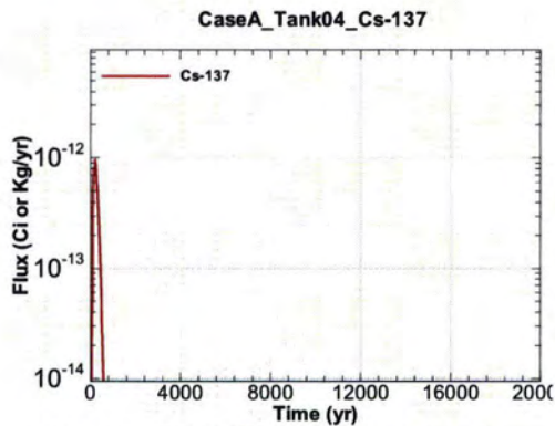
Figure A.1-259 - Flux Leaving Liner for CaseA Tank04 Cs-137
