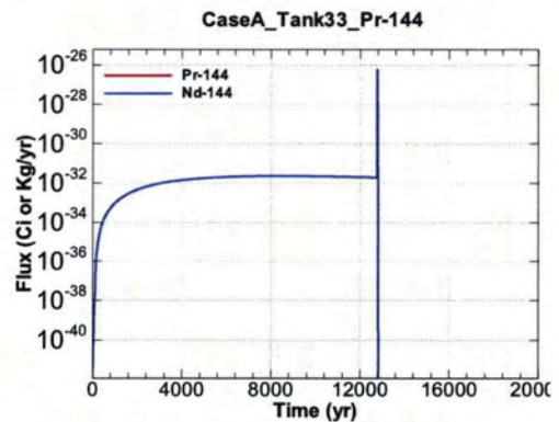
Figure A.1-670 - Flux Leaving Liner for CaseA Tank33 Pr-144
