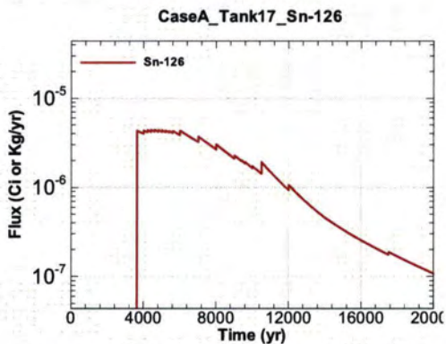
Figure A.1-1467 - Flux Leaving Liner for CaseA Tank17 Sn-126
