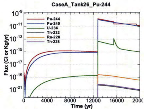
Figure A.1-910 - Flux Leaving Liner for CaseA Tank26 Pu-244
