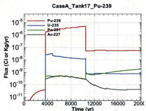
Figure A.1-1452 - Flux Leaving Liner for CaseA Tank17 Pu-239
