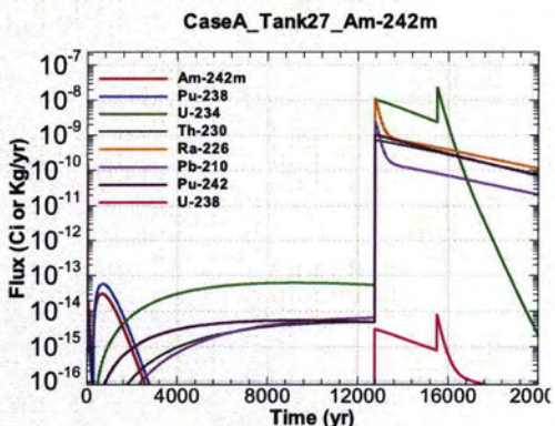
Figure A.1-941 - Flux Leaving Liner for CaseA Tank27 Am-242m
