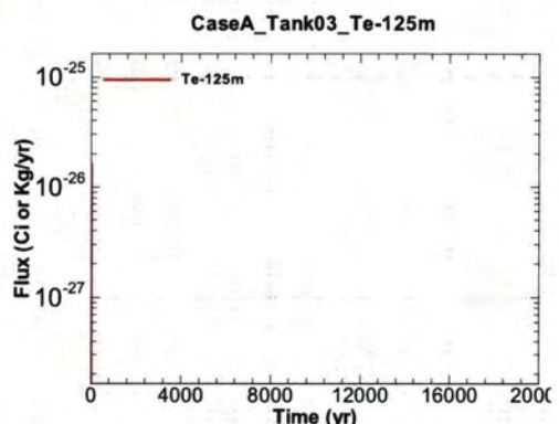
Figure A.1-222 - Flux Leaving Liner for CaseA Tank03 Te-125m
