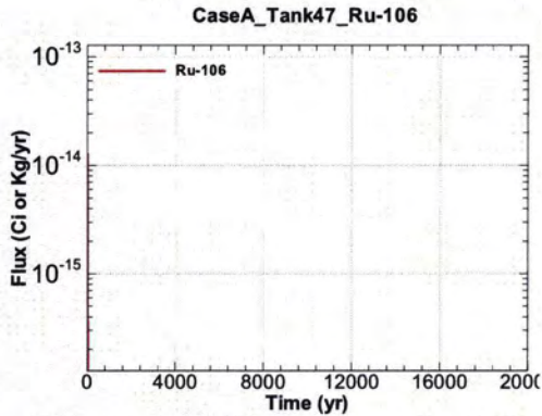
Figure A.1-1381 - Flux Leaving Liner for CaseA Tank47 Ru-106
