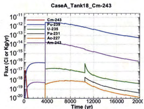
Figure A.1-1498 - Flux Leaving Liner for CaseA Tank18 Cm-243
