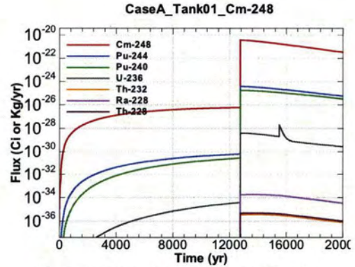
Figure A.1-20 - Flux Leaving Liner for CaseA Tank01 Cm-248
