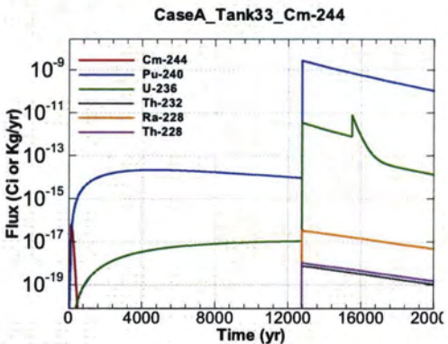
Figure A.1-641 - Flux Leaving Liner for CaseA Tank33 Cm-244
