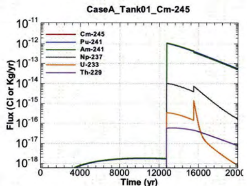
Figure A.1-18 - Flux Leaving Liner for CaseA Tank01 Cm-245
