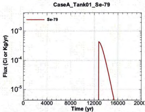
Figure A.1-61 - Flux Leaving Liner for CaseA Tank01 Se-79
