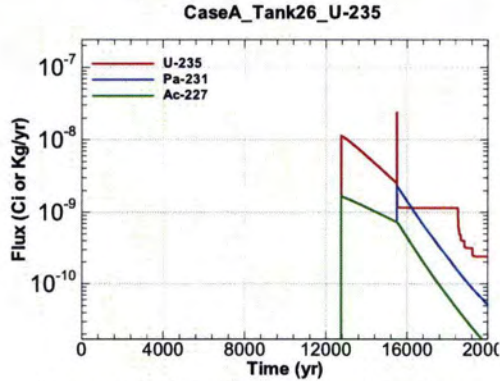
Figure A.1-931 - Flux Leaving Liner for CaseA Tank26 U-235
