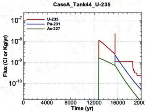
Figure A.1-1165 - Flux Leaving Liner for CaseA Tank44 U-235
