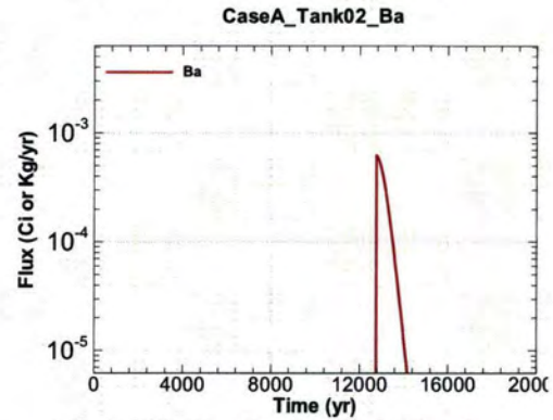
Figure A.1-86 - Flux Leaving Liner for CaseA Tank02 Ba
