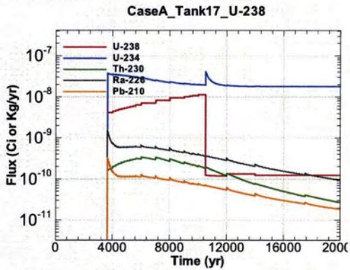
Figure A.1-1479 - Flux Leaving Liner for CaseA Tank17 U-238
