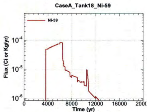
Figure A.1-1522 - Flux Leaving Liner for CaseA Tank18 Ni-59
