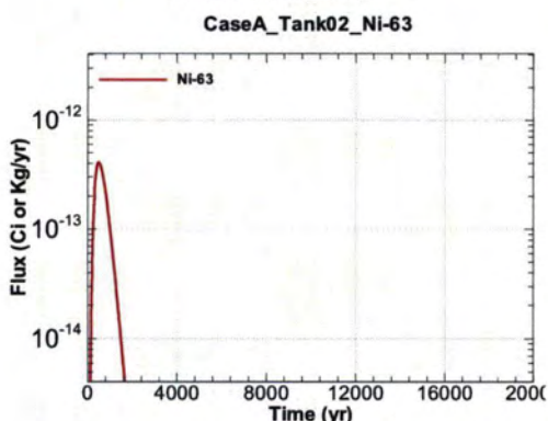
Figure A.1-119 - Flux Leaving Liner for CaseA Tank02 Ni-63
