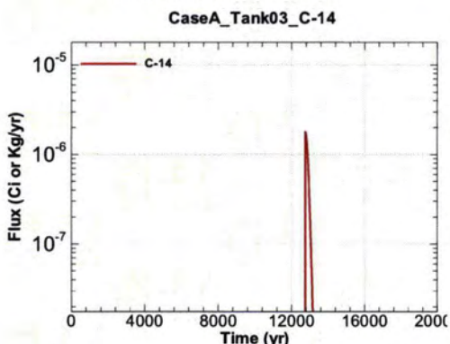
Figure A.1-167 - Flux Leaving Liner for CaseA Tank03 C-14
