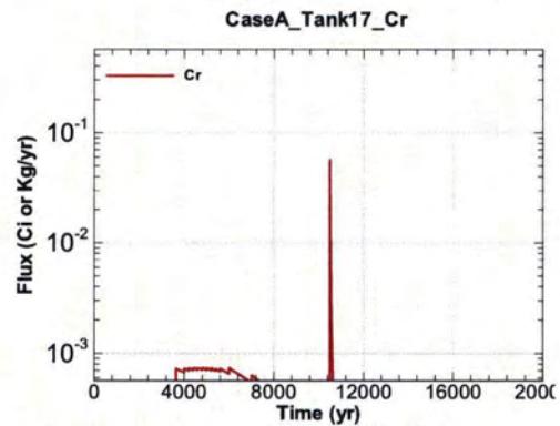
Figure A.1-1426 - Flux Leaving Liner for CaseA Tank17 Cr
