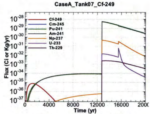
Figure A.1-482 - Flux Leaving Liner for CaseA Tank07 Cf-249
