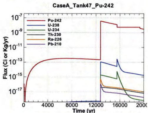
Figure A.1-1377 - Flux Leaving Liner for CaseA Tank47 Pu-242
