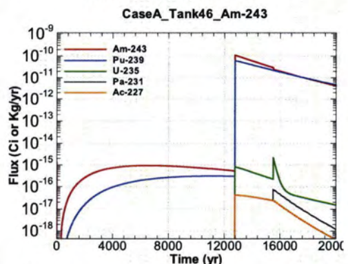
Figure A.1-1254 - Flux Leaving Liner for CaseA Tank46 Am-243
