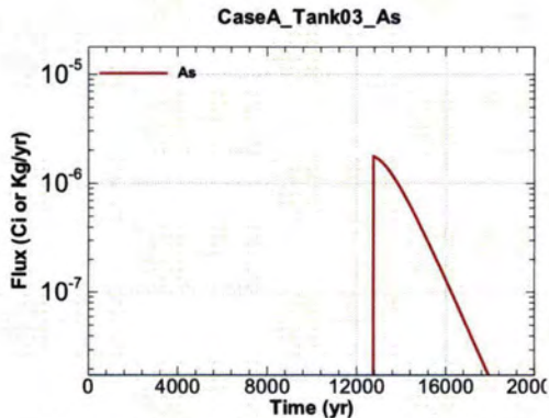
Figure A.1-163 - Flux Leaving Liner for CaseA Tank03 As
