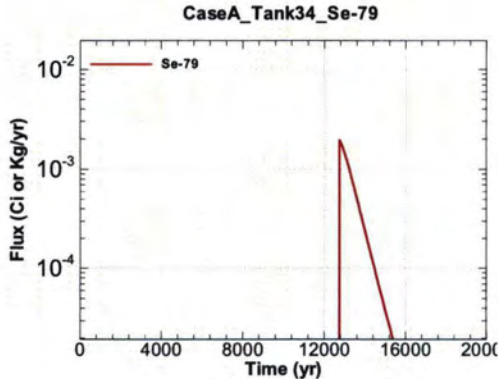
Figure A.1-763 - Flux Leaving Liner for CaseA Tank34 Se-79
