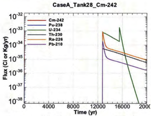
Figure A.1-1029 - Flux Leaving Liner for CaseA Tank28 Cm-242
