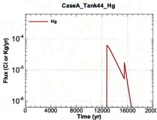
Figure A.1-1125 - Flux Leaving Liner for CaseA Tank44 Hg
