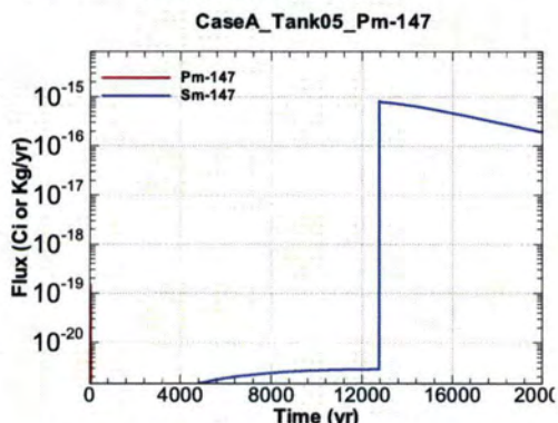
Figure A.1-357 - Flux Leaving Liner for CaseA Tank05 Pm-147
