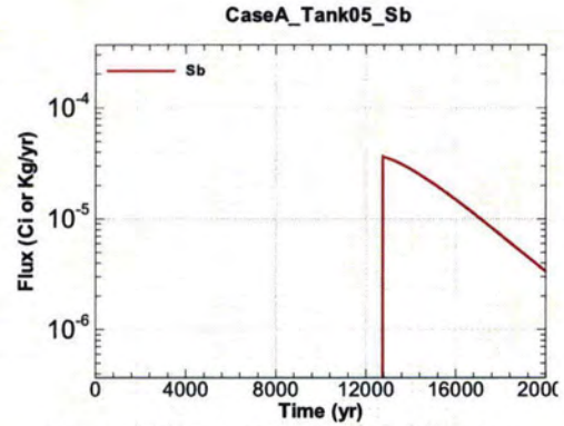
Figure A.1-368 - Flux Leaving Liner for CaseA Tank05 Sb
