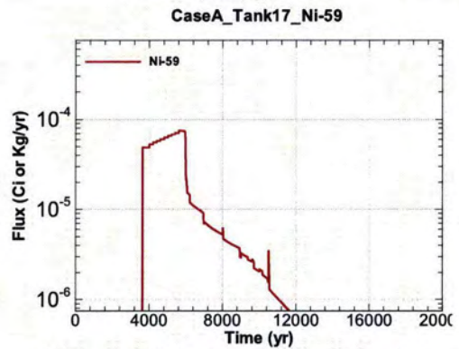
Figure A.1-1444 - Flux Leaving Liner for CaseA Tank17 Ni-59
