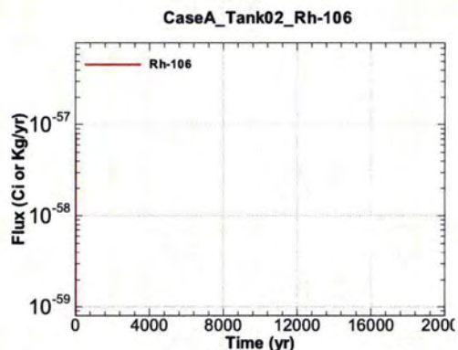
Figure A.1-132 - Flux Leaving Liner for CaseA Tank02 Rh-106
