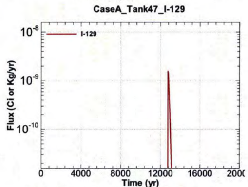
Figure A.1-1360 - Flux Leaving Liner for CaseA Tank47 I-129
