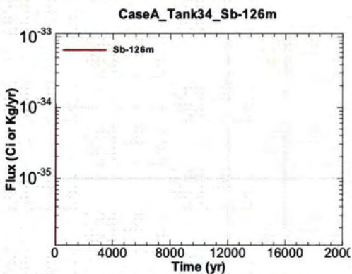
Figure A.1-761 - Flux Leaving Liner for CaseA Tank34 Sb-126m
