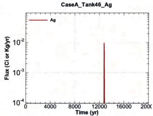
Figure A.1-1250 - Flux Leaving Liner for CaseA Tank46 Ag
