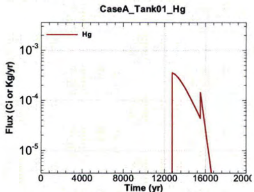
Figure A.1-33 - Flux Leaving Liner for CaseA Tank01 Hg
