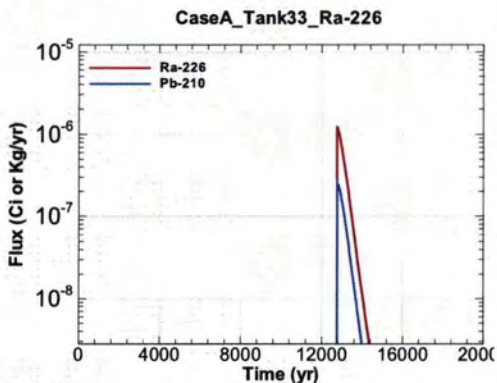
Figure A.1-677 - Flux Leaving Liner for CaseA Tank33 Ra-226
