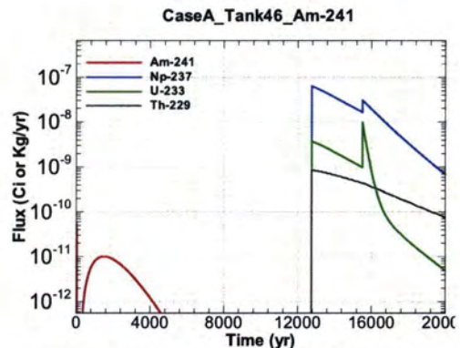
Figure A.1-1252 - Flux Leaving Liner for CaseA Tank46 Am-241
