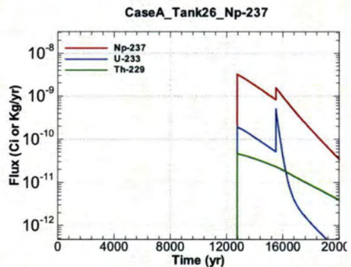
Figure A.1-900 - Flux Leaving Liner for CaseA Tank26 Np-237
