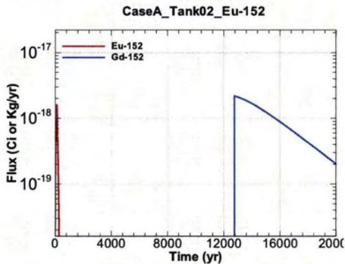
Figure A.1-105 - Flux Leaving Liner for CaseA Tank02 Eu-152
