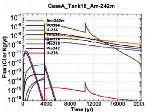
Figure A.1-1487 - Flux Leaving Liner for CaseA Tank18 Am-242m
