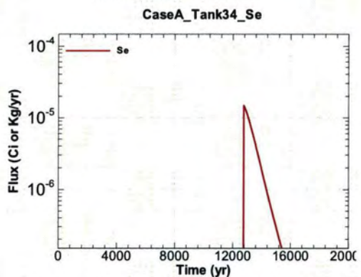
Figure A.1-762 - Flux Leaving Liner for CaseA Tank34 Se
