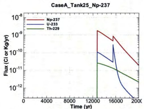
Figure A.1-822 - Flux Leaving Liner for CaseA Tank25 Np-237
