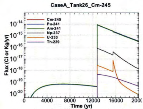
Figure A.1-876 - Flux Leaving Liner for CaseA Tank26 Cm-245
