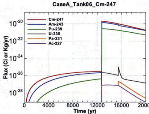
Figure A.1-409 - Flux Leaving Liner for CaseA Tank06 Cm-247
