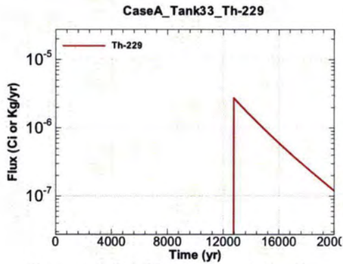
Figure A.1-691 - Flux Leaving Liner for CaseA Tank33 Th-229
