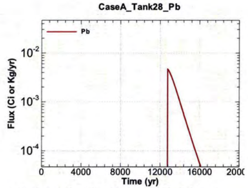
Figure A.1-1058 - Flux Leaving Liner for CaseA Tank28 Pb
