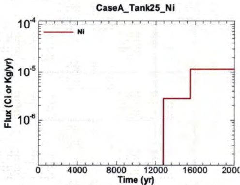
Figure A.1-819 - Flux Leaving Liner for CaseA Tank25 Ni
