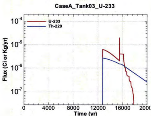
Figure A.1-227 - Flux Leaving Liner for CaseA Tank03 U-233
