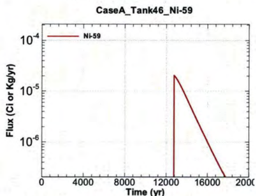
Figure A.1-1288 - Flux Leaving Liner for CaseA Tank46 Ni-59
