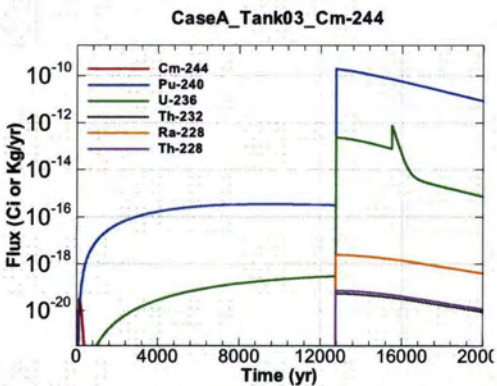
Figure A.1-173 - Flux Leaving Liner for CaseA Tank03 Cm-244
