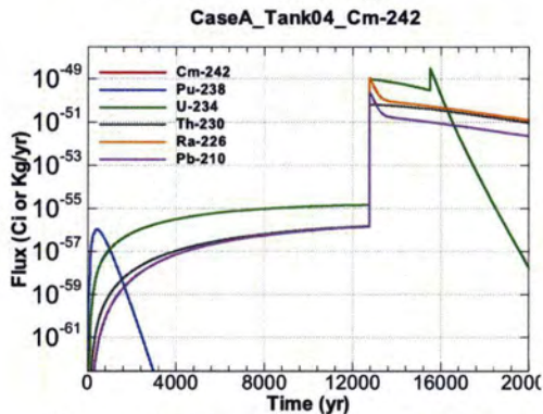
Figure A.1-249 - Flux Leaving Liner for CaseA Tank04 Cm-242
