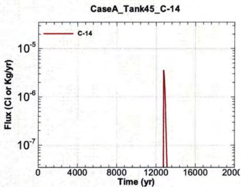
Figure A.1-1181 - Flux Leaving Liner for CaseA Tank45 C-14
