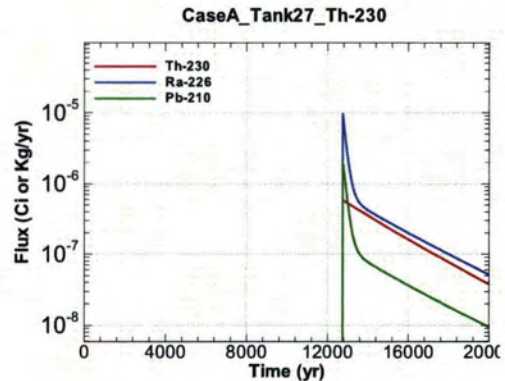
Figure A.1-1004 - Flux Leaving Liner for CaseA Tank27 Th-230
