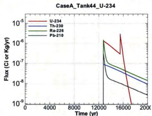
Figure A.1-1164 - Flux Leaving Liner for CaseA Tank44 U-234
