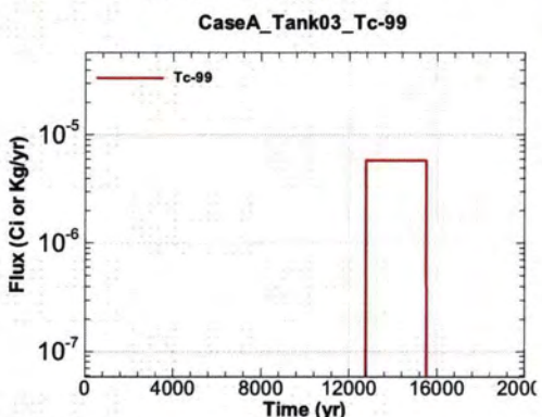
Figure A.1-221 - Flux Leaving Liner for CaseA Tank03 Tc-99
