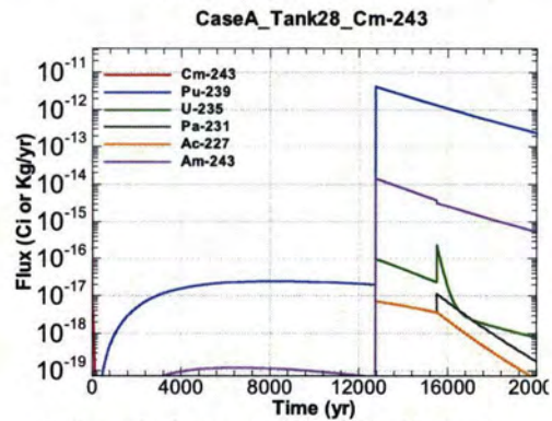
Figure A.1-1030 - Flux Leaving Liner for CaseA Tank28 Cm-243
