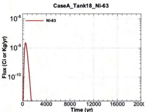
Figure A.1-1523 - Flux Leaving Liner for CaseA Tank18 Ni-63
