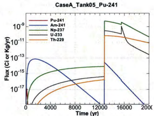
Figure A.1-362 - Flux Leaving Liner for CaseA Tank05 Pu-241
