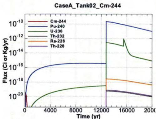
Figure A.1-95 - Flux Leaving Liner for CaseA Tank02 Cm-244
