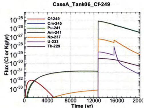
Figure A.1-404 - Flux Leaving Liner for CaseA Tank06 Cf-249
