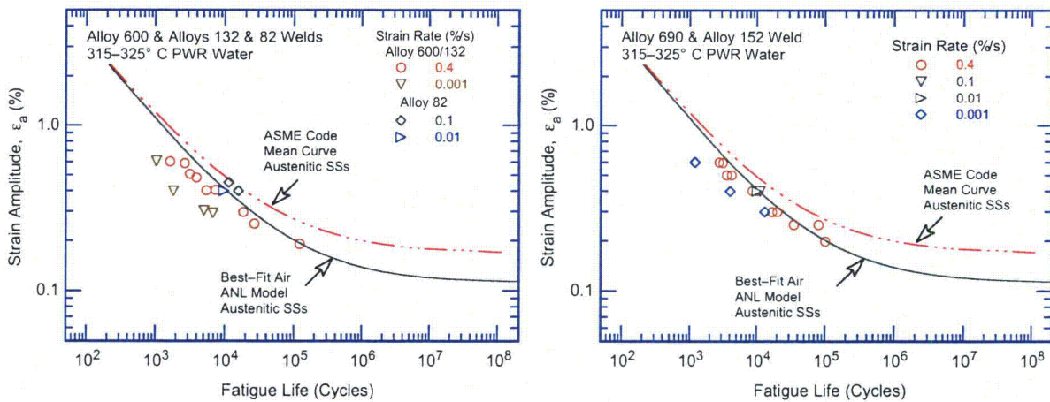
Figure 59. Fatigue \epsilon - N behavior for Alloys 600 and 690 and their weld alloys in simulated PWR water at 315\text{--}325^\circ\text{C} (Refs. 33, 78).
