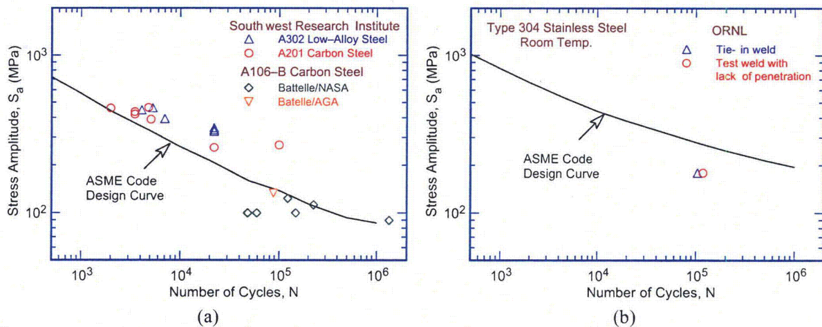
Figure 62. Fatigue data for (a) carbon and low-alloy steel and (b) Type 304 stainless steel components (Refs. 123,124).
