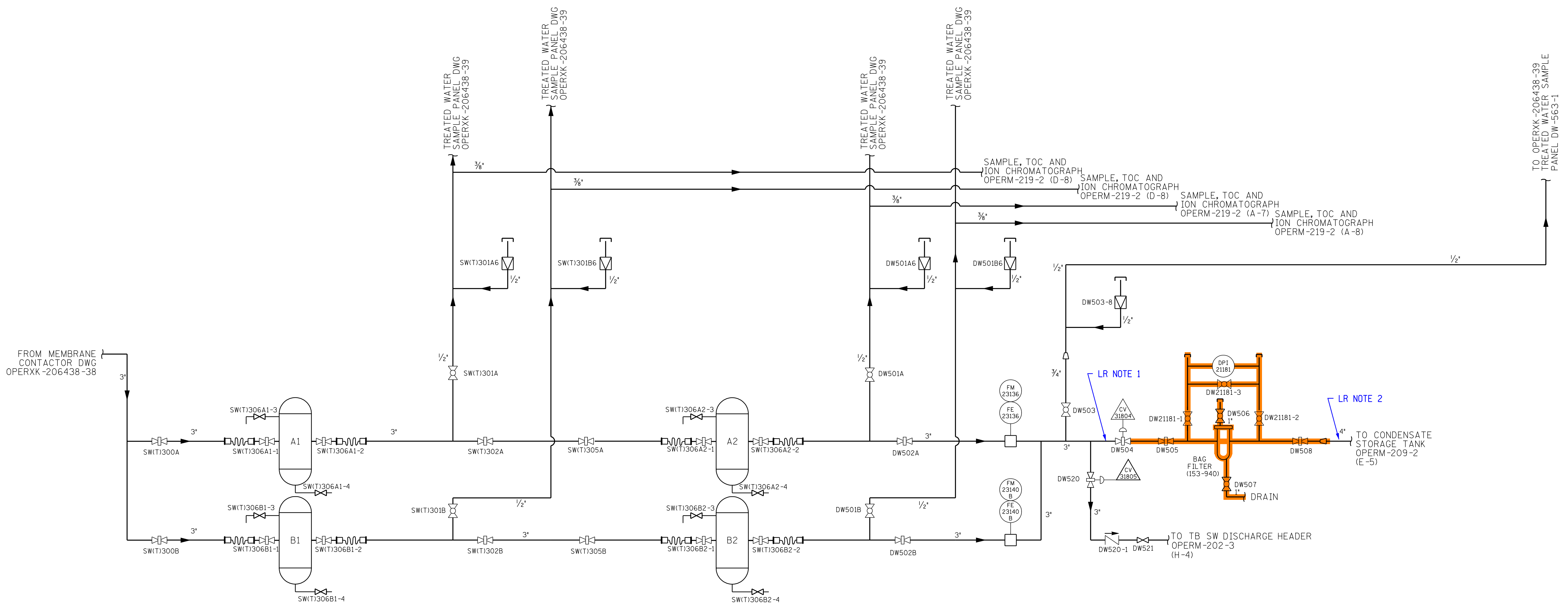
MAKE UP WATER SERVICE MIXED BEDS
