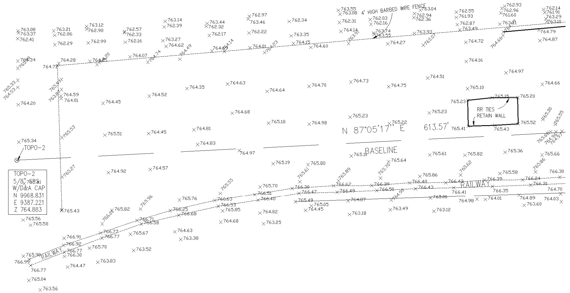
Figure 3-2 Topographical Map of Initial Elevations (West Side Blow Up)
