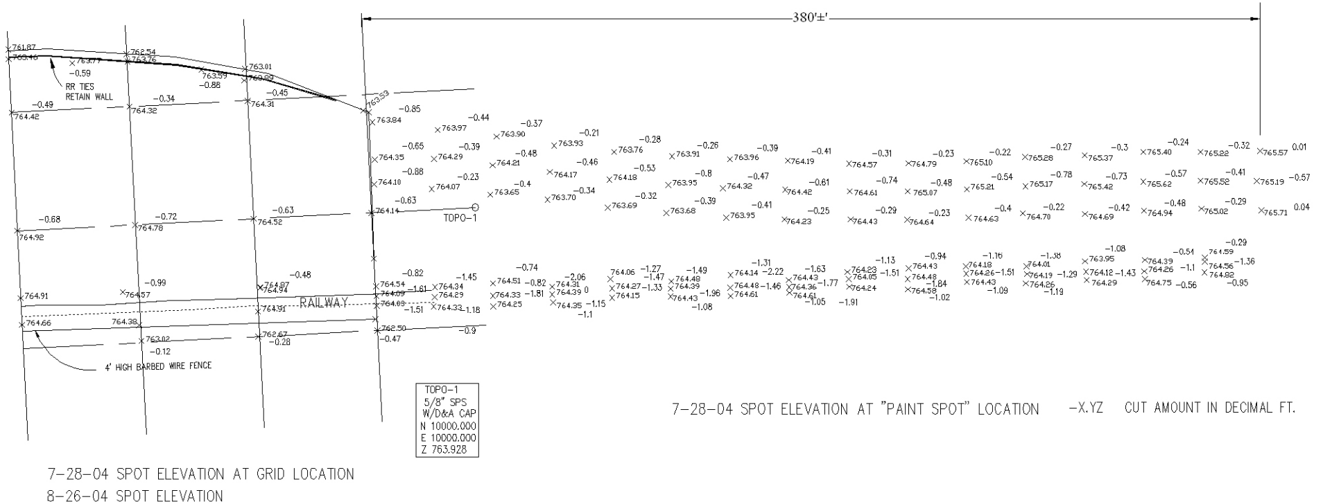
Figure 3-10 Final Elevations (Eastern Blowup)
