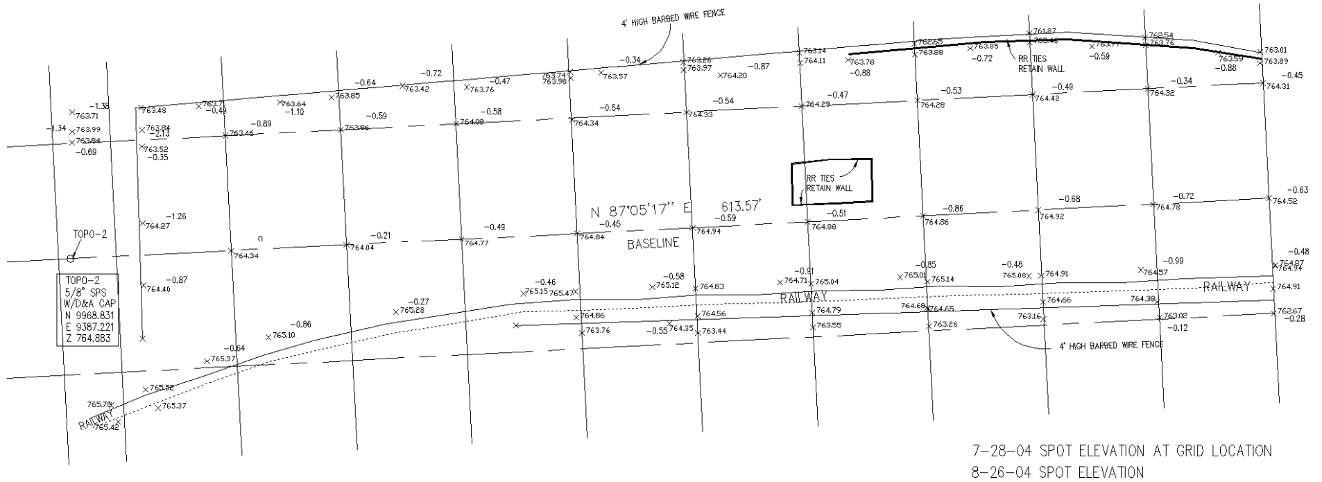
Figure 3-9 Final Elevations (Western Blowup)
