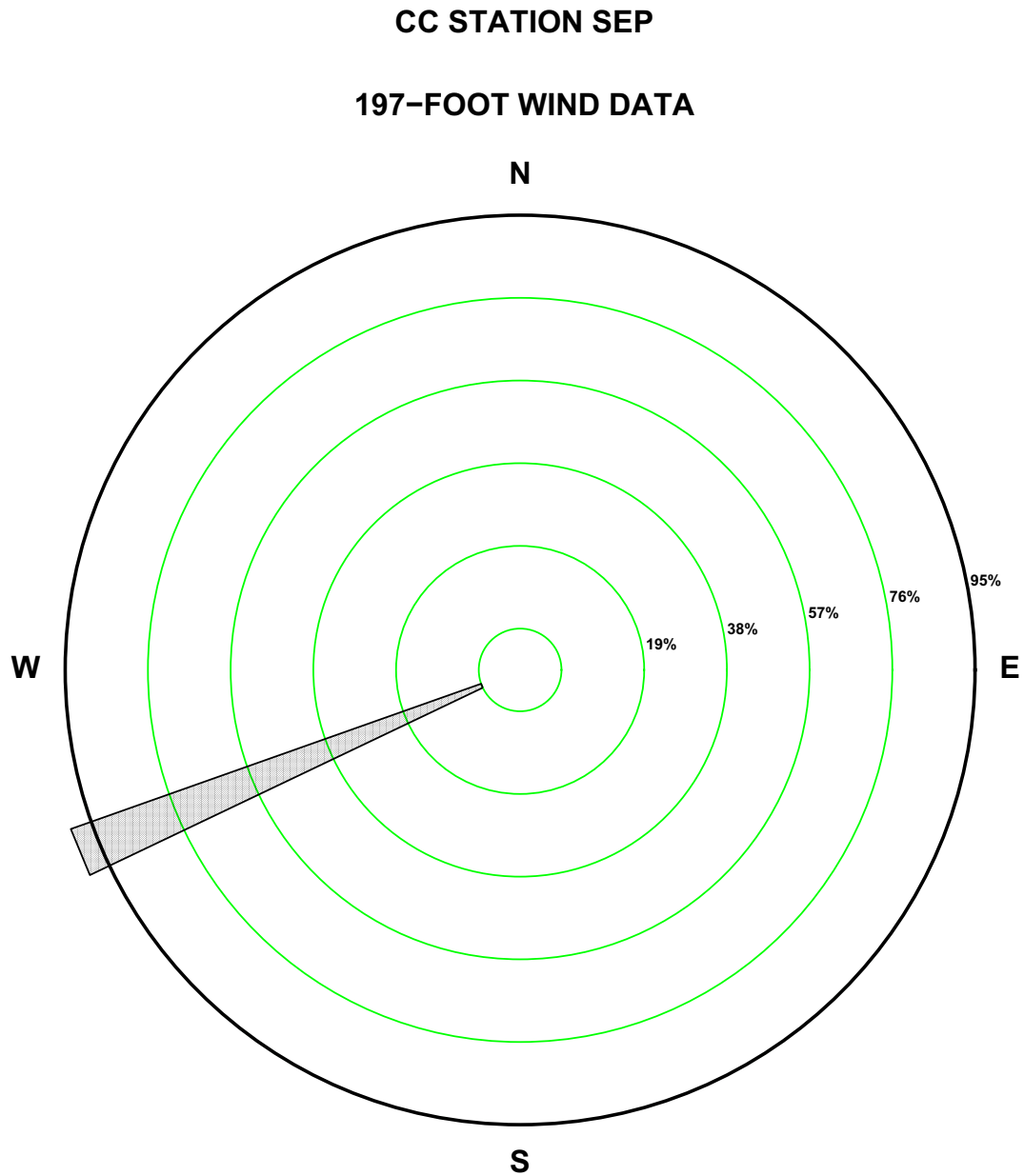
Figure 2.7-156—{CCNPP 197 ft September Precipitation Wind Rose for Rate Class 0.7-0.8 in/hr}
