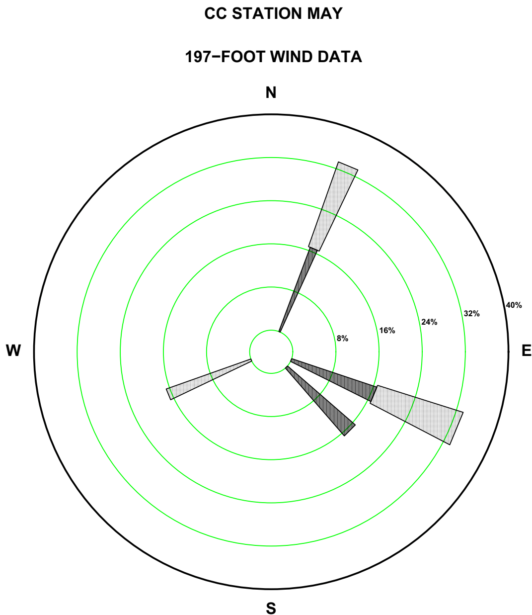
Figure 2.7-123—{CCNPP 197 ft May Precipitation Wind Rose for Rate Class 0.3-0.4 in/hr}
