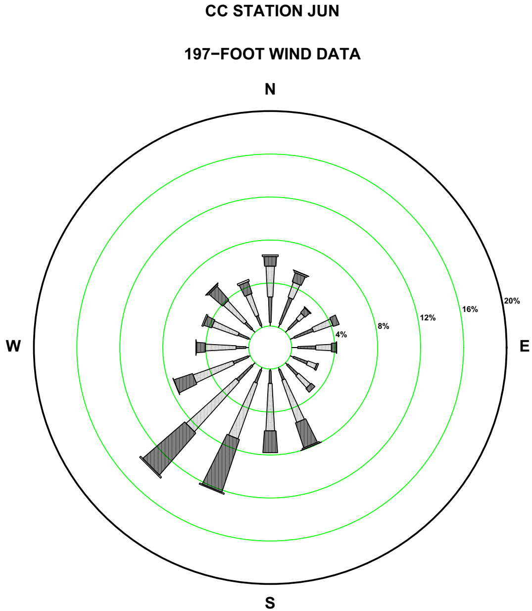
Figure 2.7-192—{CCNPP 197 ft June Wind Rose}
