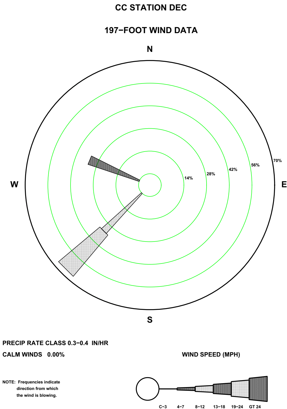
Figure 2.7-171—{CCNPP 197 ft December Precipitation Wind Rose for Rate Class 0.3-0.4 in/hr}
