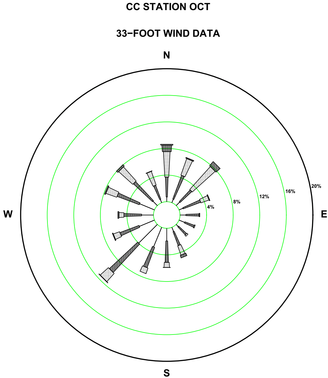
Figure 2.7-183—{CCNPP 33 ft October Wind Rose}
