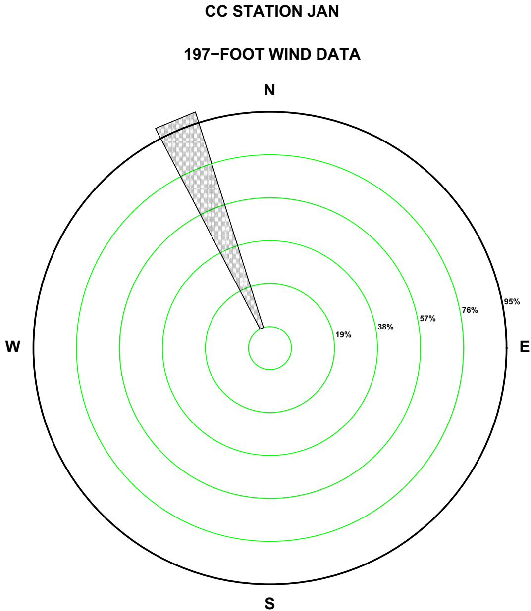
Figure 2.7-105—{CCNPP 197 ft February Precipitation Wind Rose for Rate Class 0.4-0.5 in/hr}
