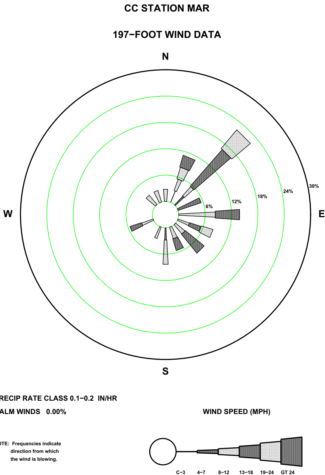
Figure 2.7-111—{CCNPP 197 ft March Precipitation Wind Rose for Rate Class 0.1-0.2 in/hr}
