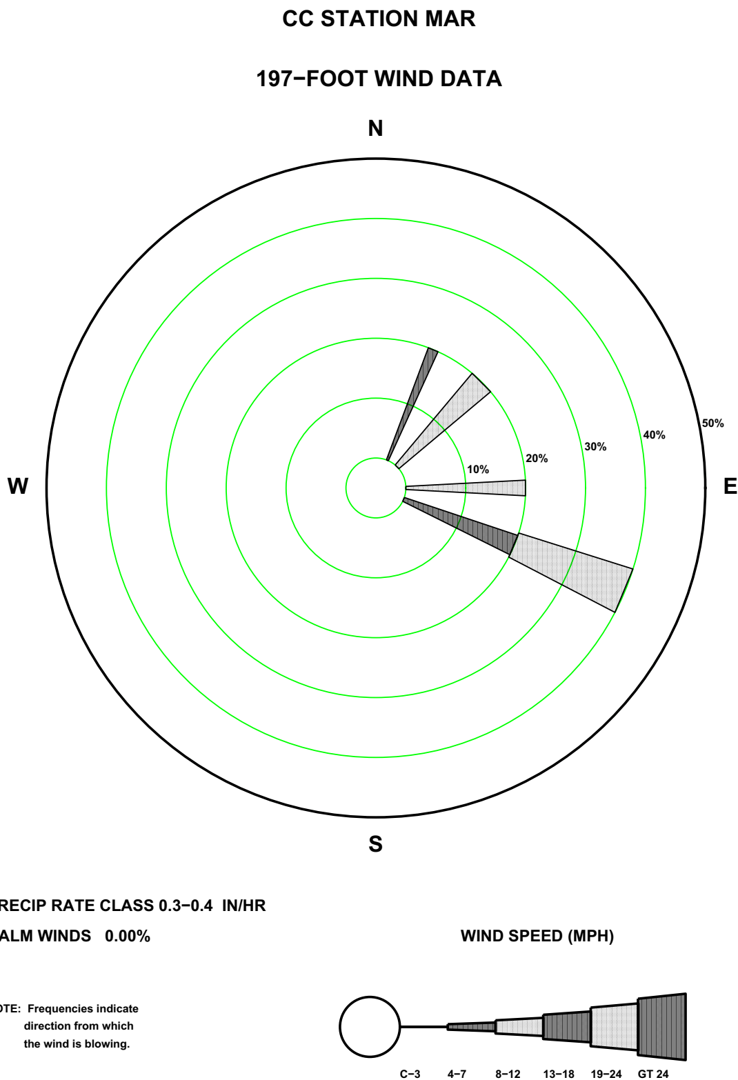
Figure 2.7-113—{CCNPP 197 ft March Precipitation Wind Rose for Rate Class 0.3-0.4 in/hr}
