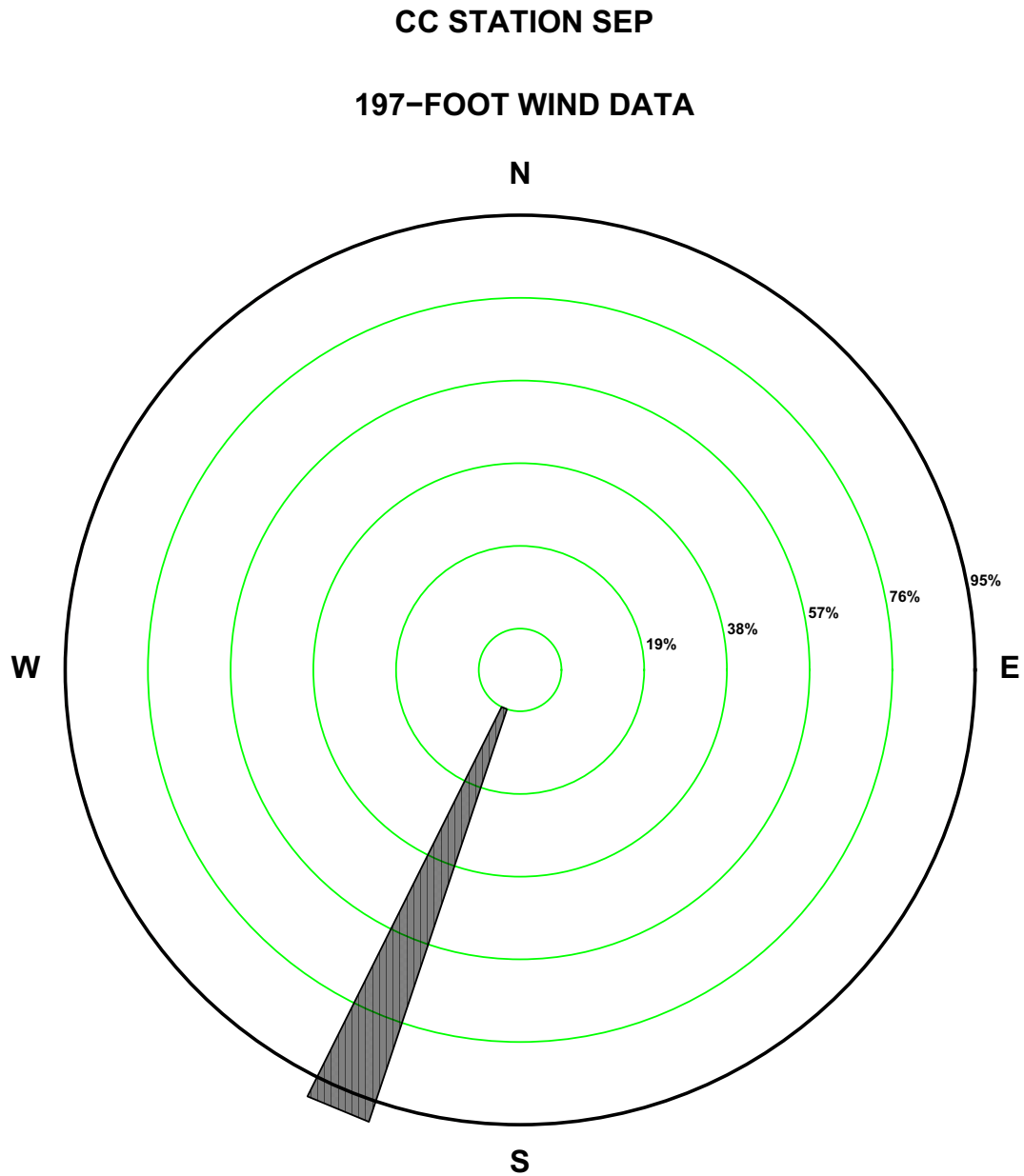
Figure 2.7-154—{CCNPP 197 ft September Precipitation Wind Rose for Rate Class 0.5-0.6 in/hr}
