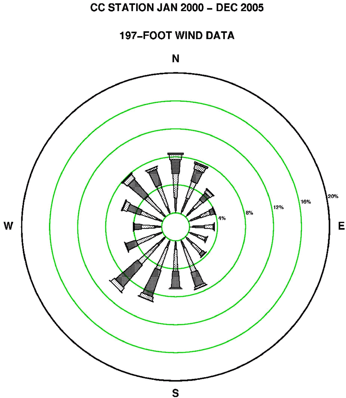
Figure 2.7-186—{CCNPP 197 ft Annual Wind Rose}
