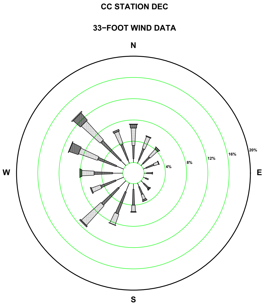
Figure 2.7-185—{CCNPP 33 ft December Wind Rose}
