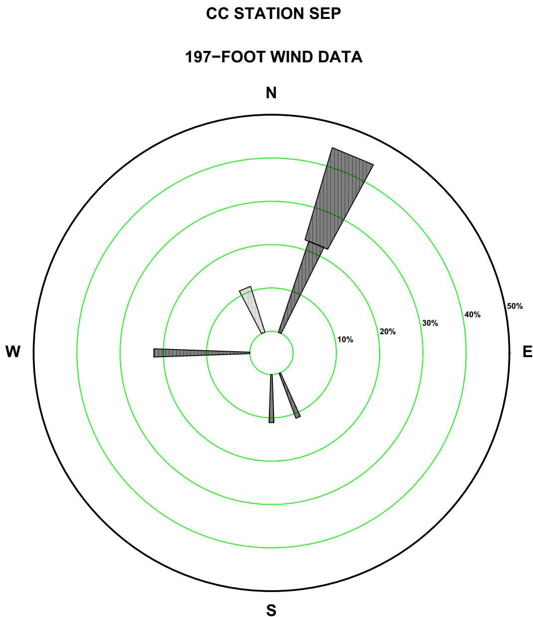
Figure 2.7-151—{CCNPP 197 ft September Precipitation Wind Rose for Rate Class 0.2-0.3 in/hr}
