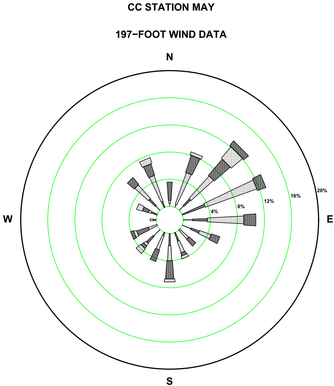
Figure 2.7-120—{CCNPP 197 ft May Precipitation Wind Rose for Rate Class 0.0-0.1 in/hr}
