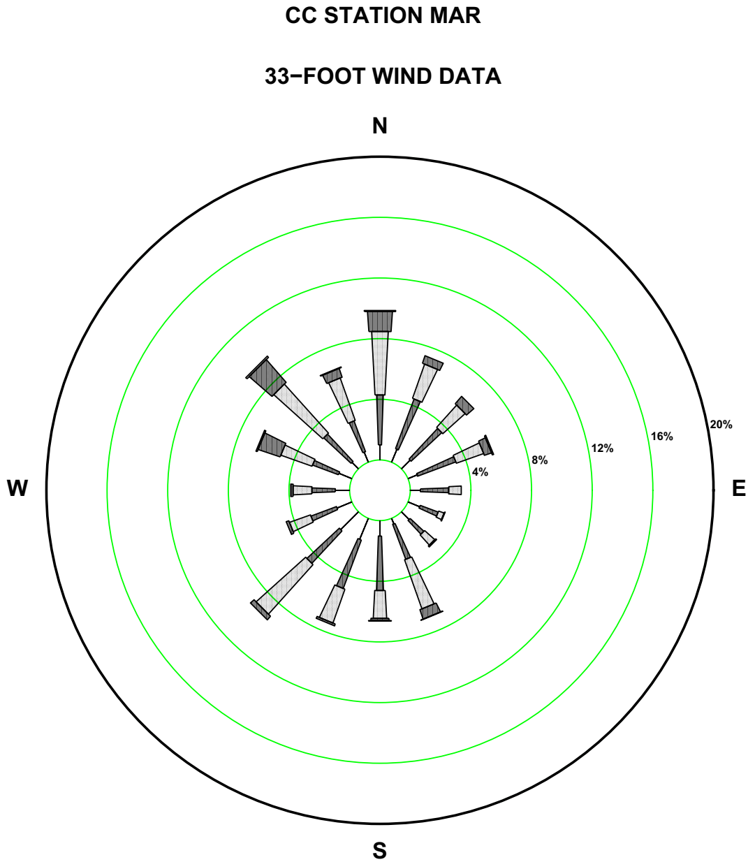
Figure 2.7-176—{CCNPP 33 ft March Wind Rose}
