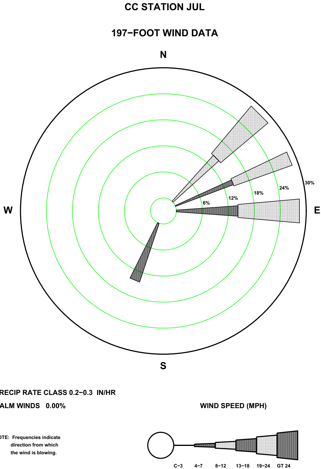
Figure 2.7-136—{CCNPP 197 ft July Precipitation Wind Rose for Rate Class 0.2-0.3 in/hr}
