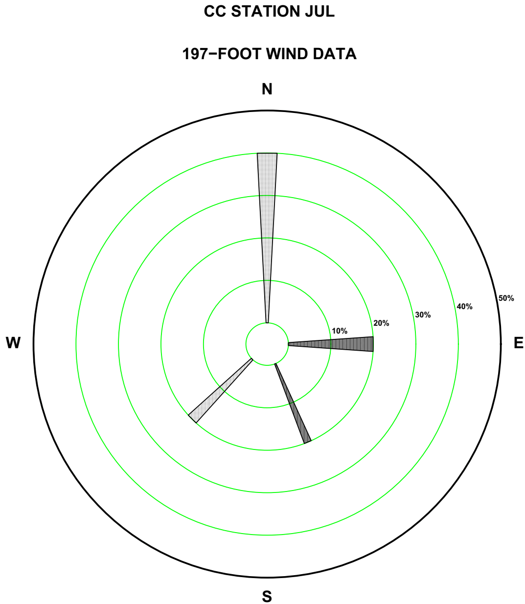
Figure 2.7-138—{CCNPP 197 ft July Precipitation Wind Rose for Rate Class 0.4-0.5 in/hr}
