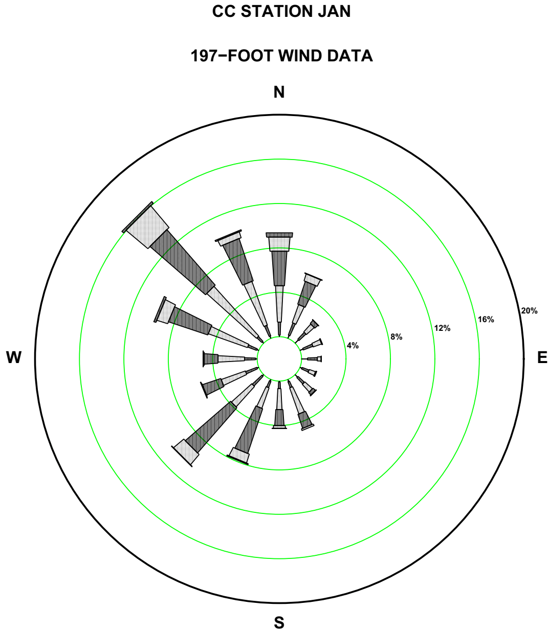
Figure 2.7-187—{CCNPP 197 ft January Wind Rose}
