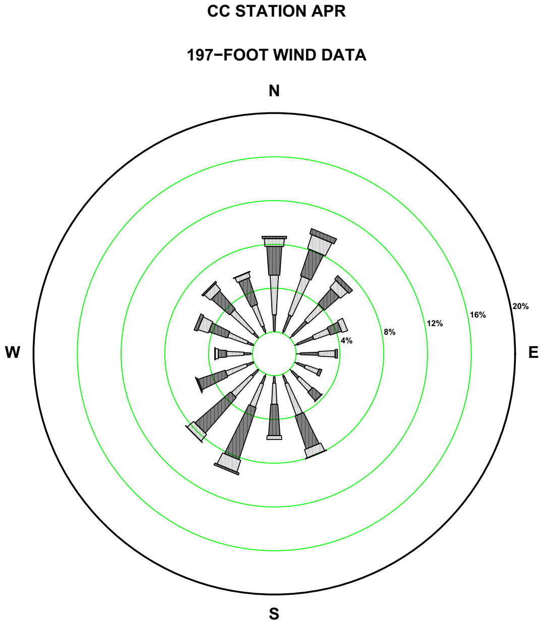
Figure 2.7-190—{CCNPP 197 ft April Wind Rose}
