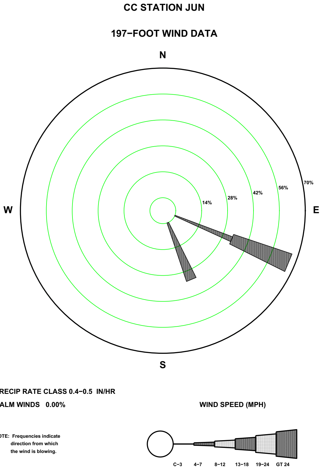
Figure 2.7-131—{CCNPP 197 ft June Precipitation Wind Rose for Rate Class 0.4-0.5 in/hr}
