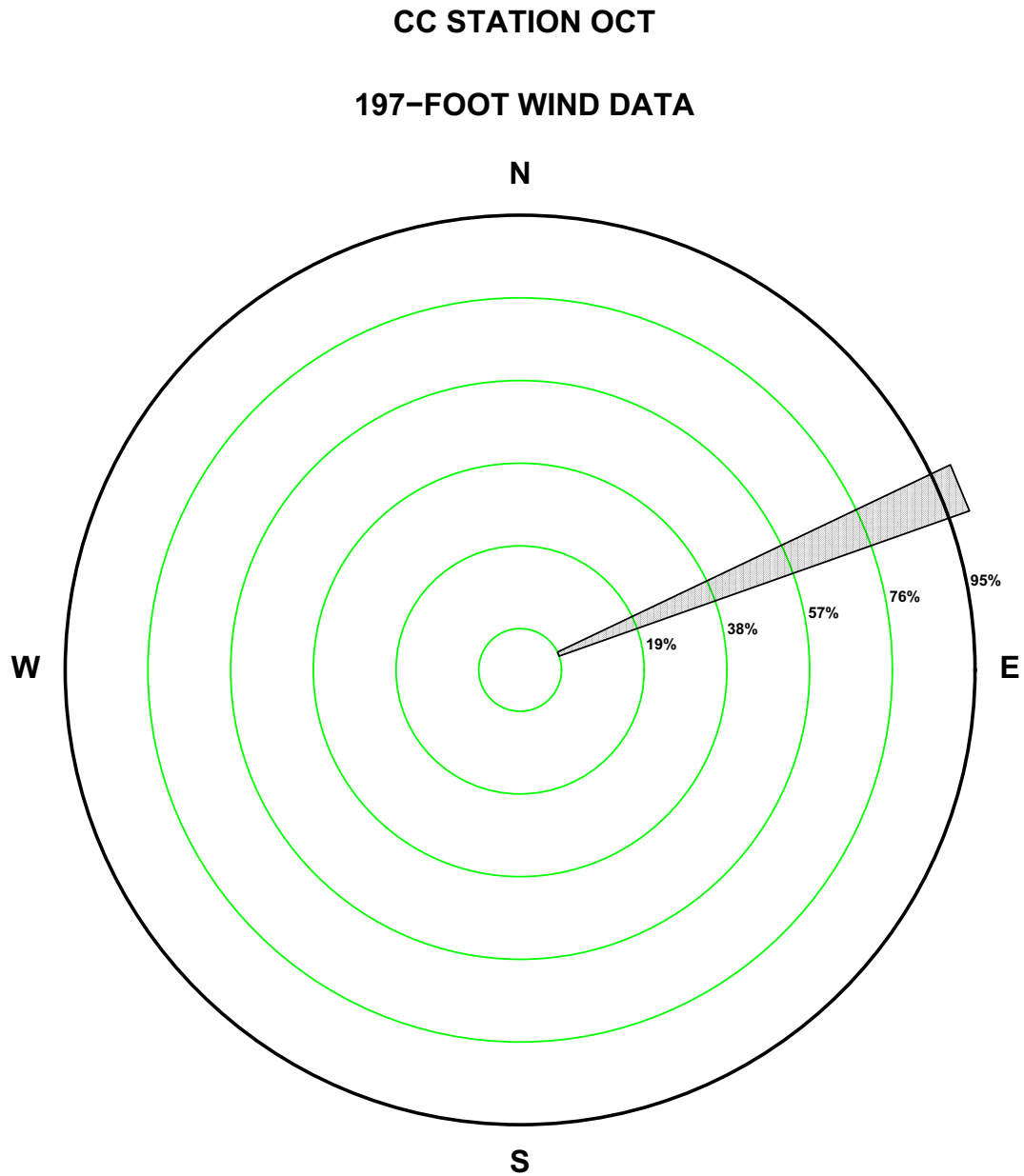
Figure 2.7-162—{CCNPP 197 ft October Precipitation Wind Rose for Rate Class 0.5-0.6 in/hr}
