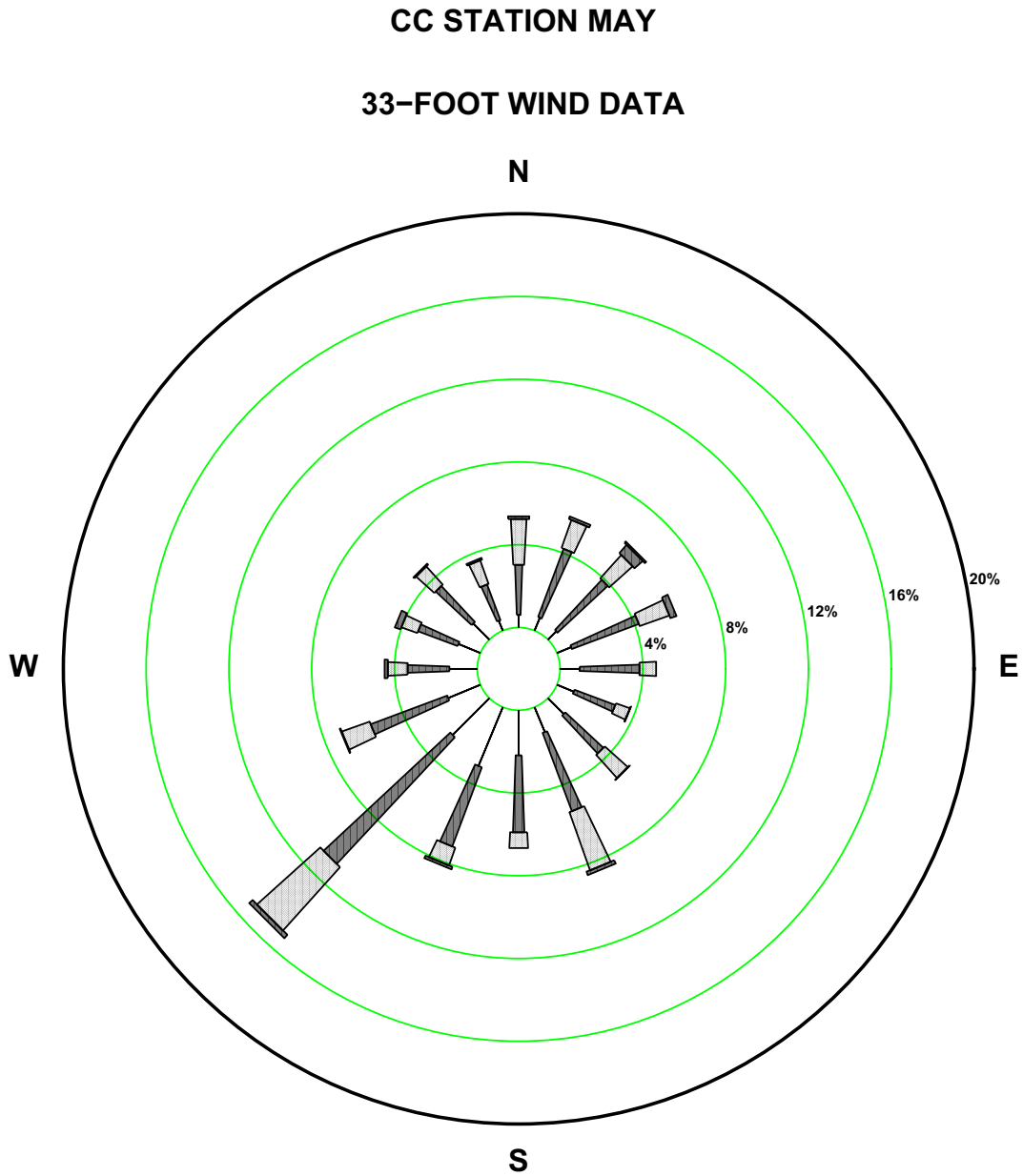
Figure 2.7-178—{CCNPP 33 ft May Wind Rose}
