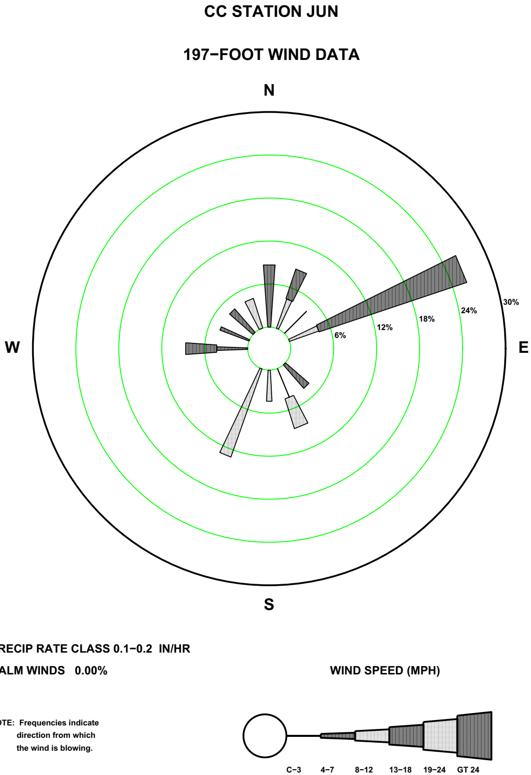
Figure 2.7-128—{CCNPP 197 ft June Precipitation Wind Rose for Rate Class 0.1-0.2 in/hr}
