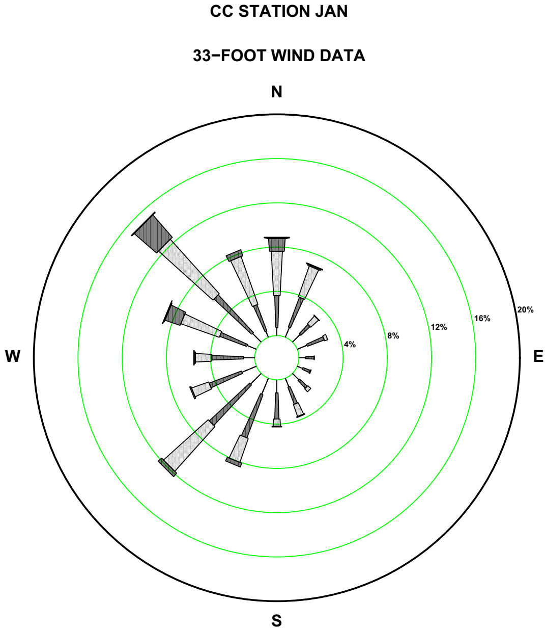
Figure 2.7-174—{CCNPP 33 ft January Wind Rose}
