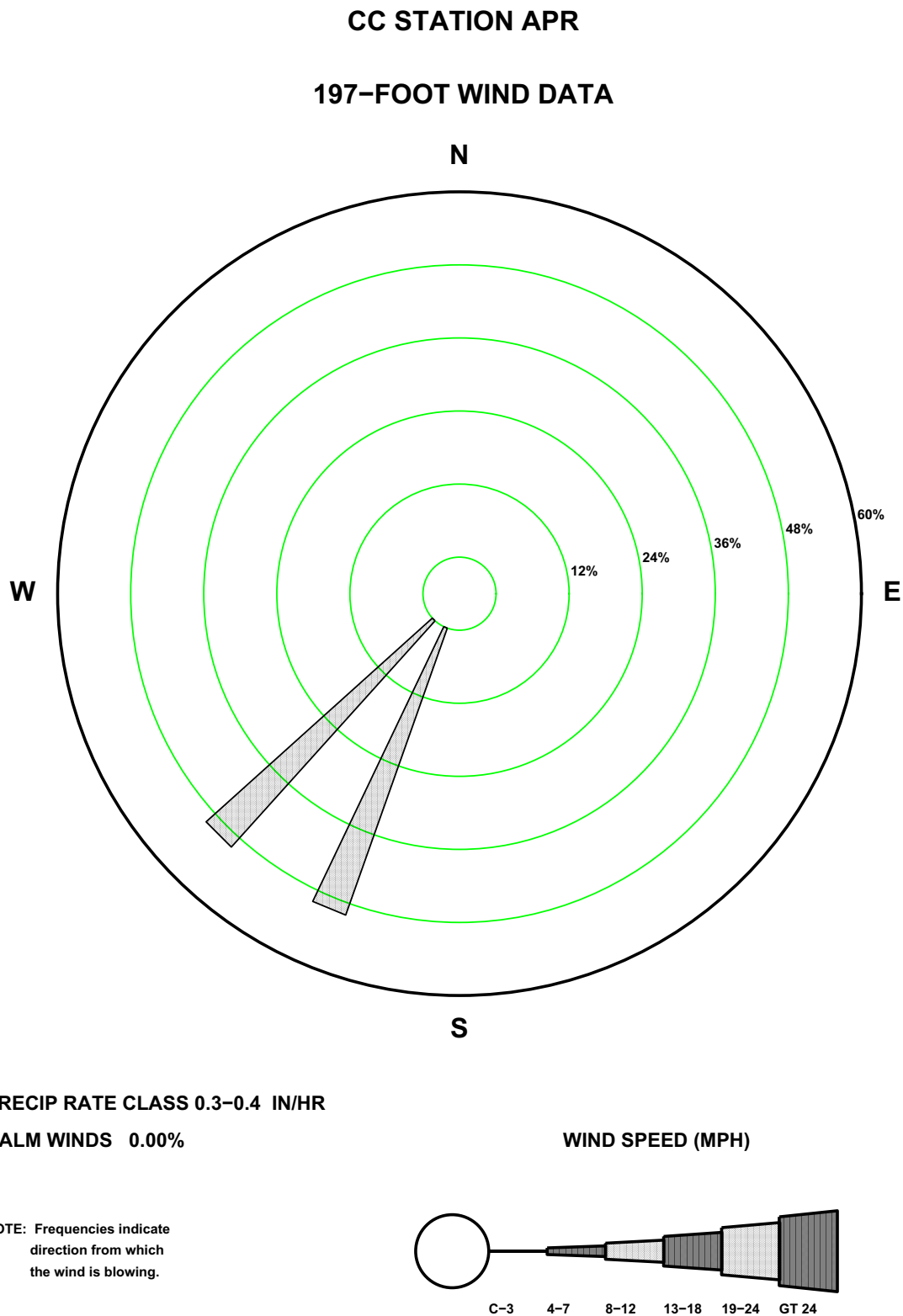
Figure 2.7-117—{CCNPP 197 ft April Precipitation Wind Rose for Rate Class 0.3-0.4 in/hr}
