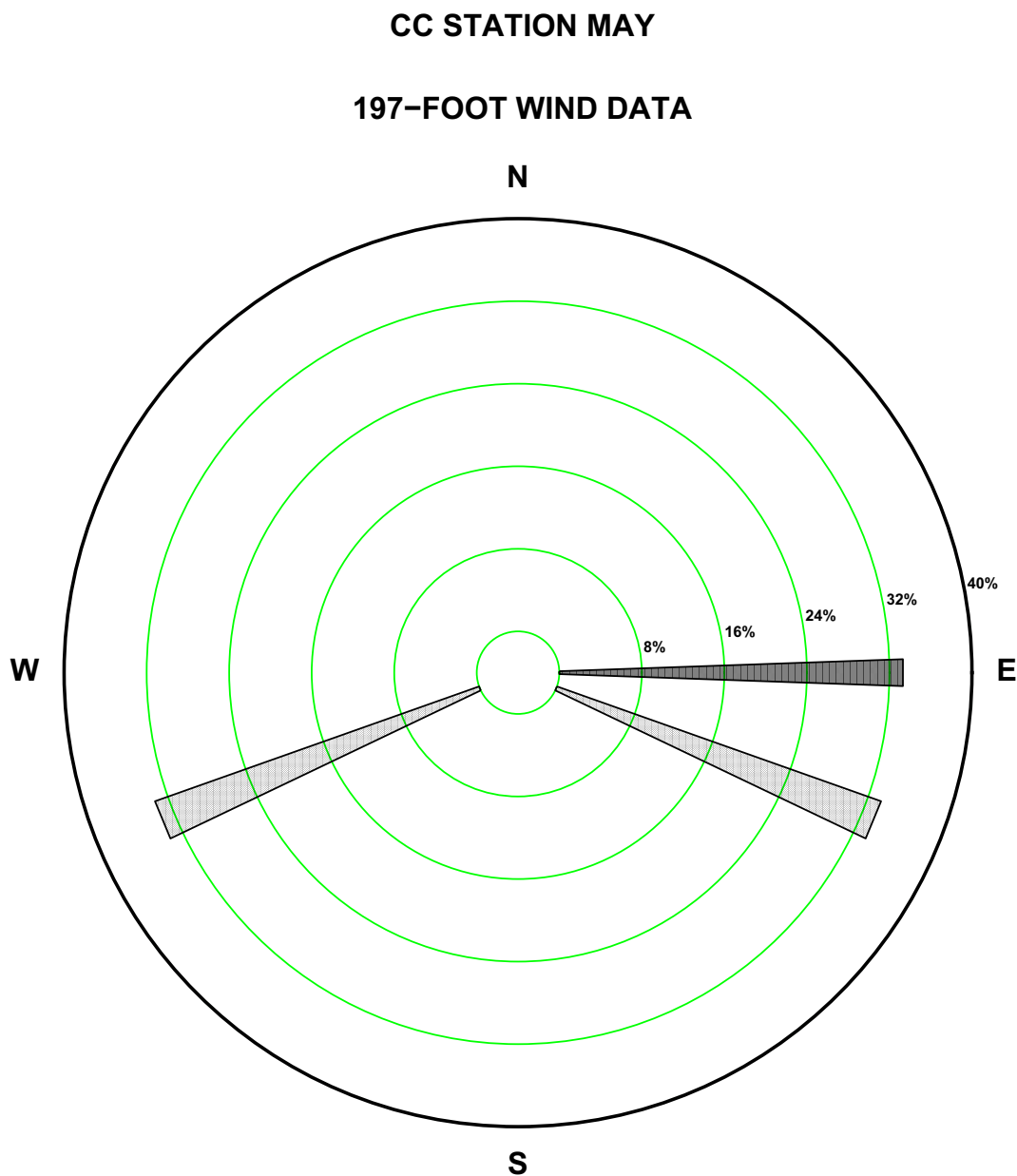
Figure 2.7-125—{CCNPP 197 ft May Precipitation Wind Rose for Rate Class 0.6-0.7 in/hr}
