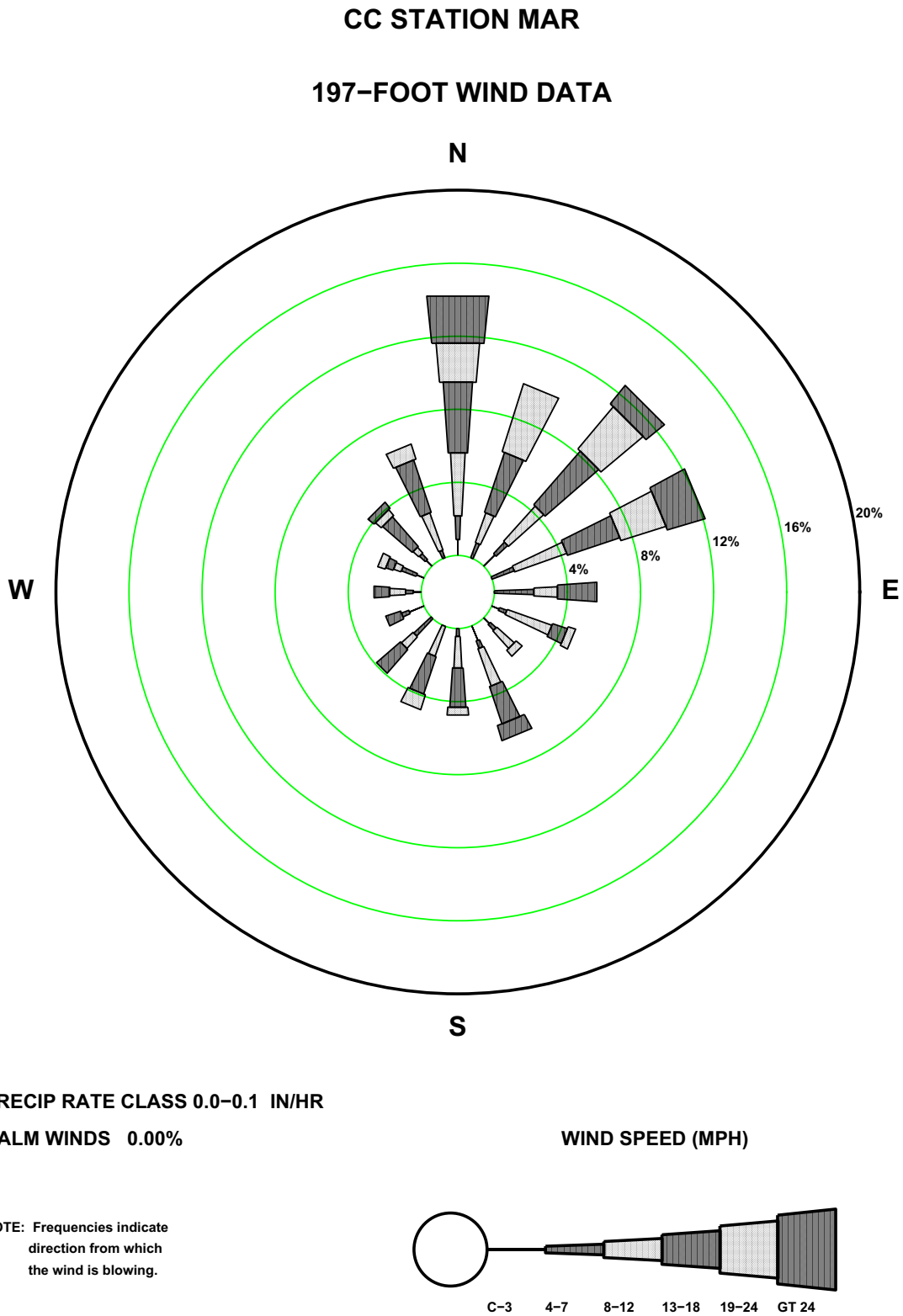
Figure 2.7-110—{CCNPP 197 ft March Precipitation Wind Rose for Rate Class 0.0-0.1 in/hr}
