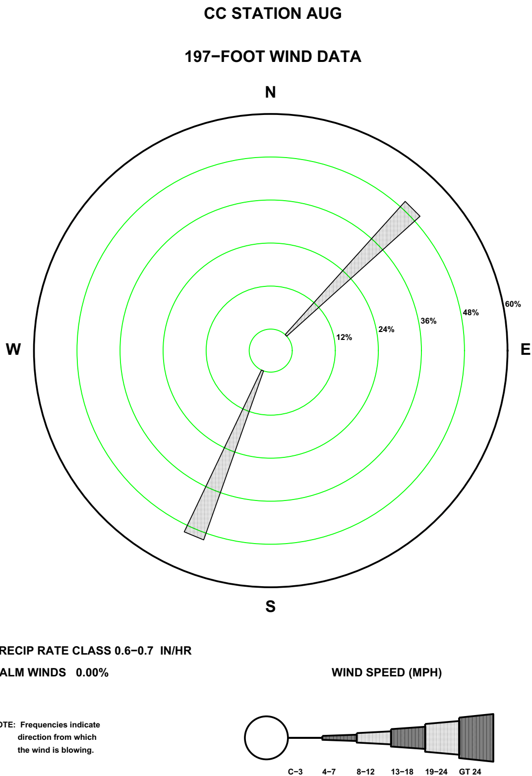
Figure 2.7-147—{CCNPP 197 ft August Precipitation Wind Rose for Rate Class 0.6-0.7 in/hr}
