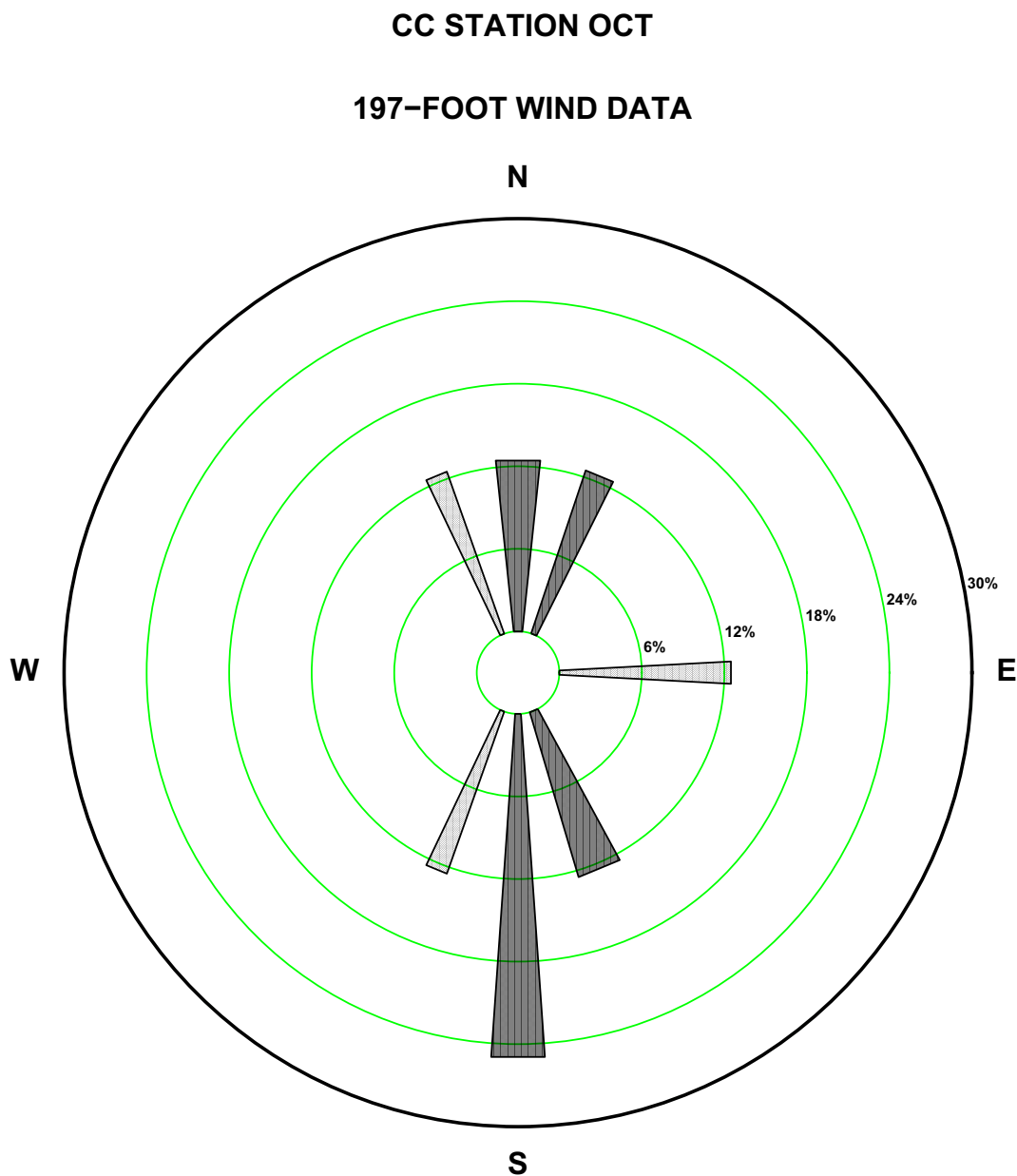
Figure 2.7-159—{CCNPP 197 ft October Precipitation Wind Rose for Rate Class 0.2-0.3 in/hr}
