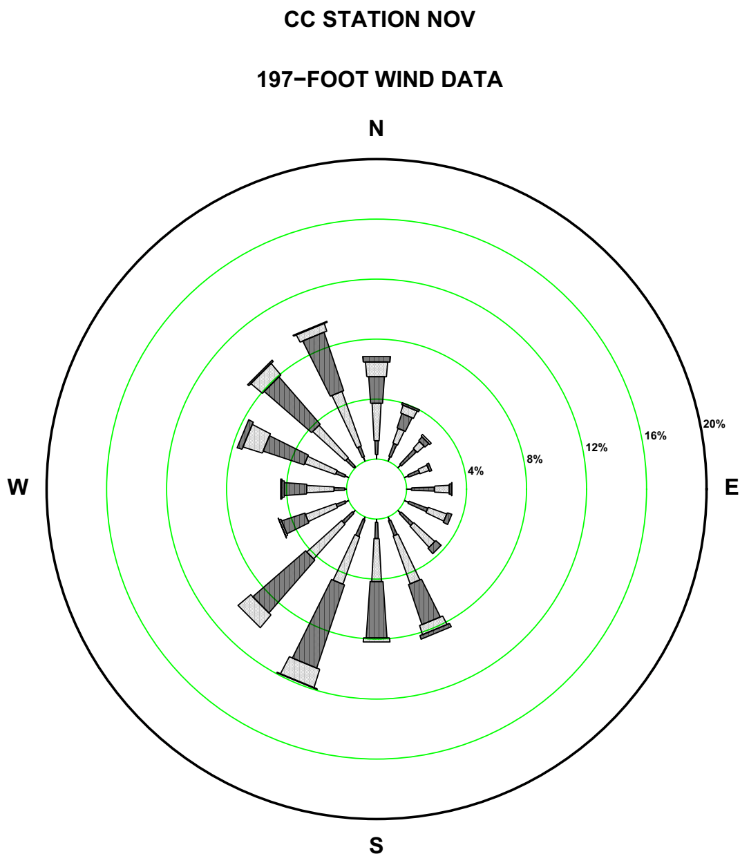
Figure 2.7-197—{CCNPP 197 ft November Wind Rose}
