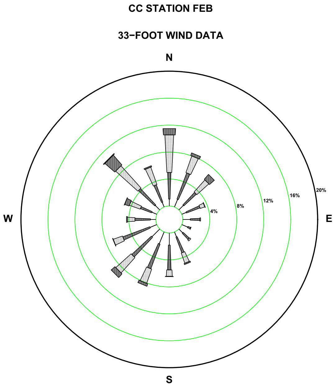
Figure 2.7-175—{CCNPP 33 ft February Wind Rose}
