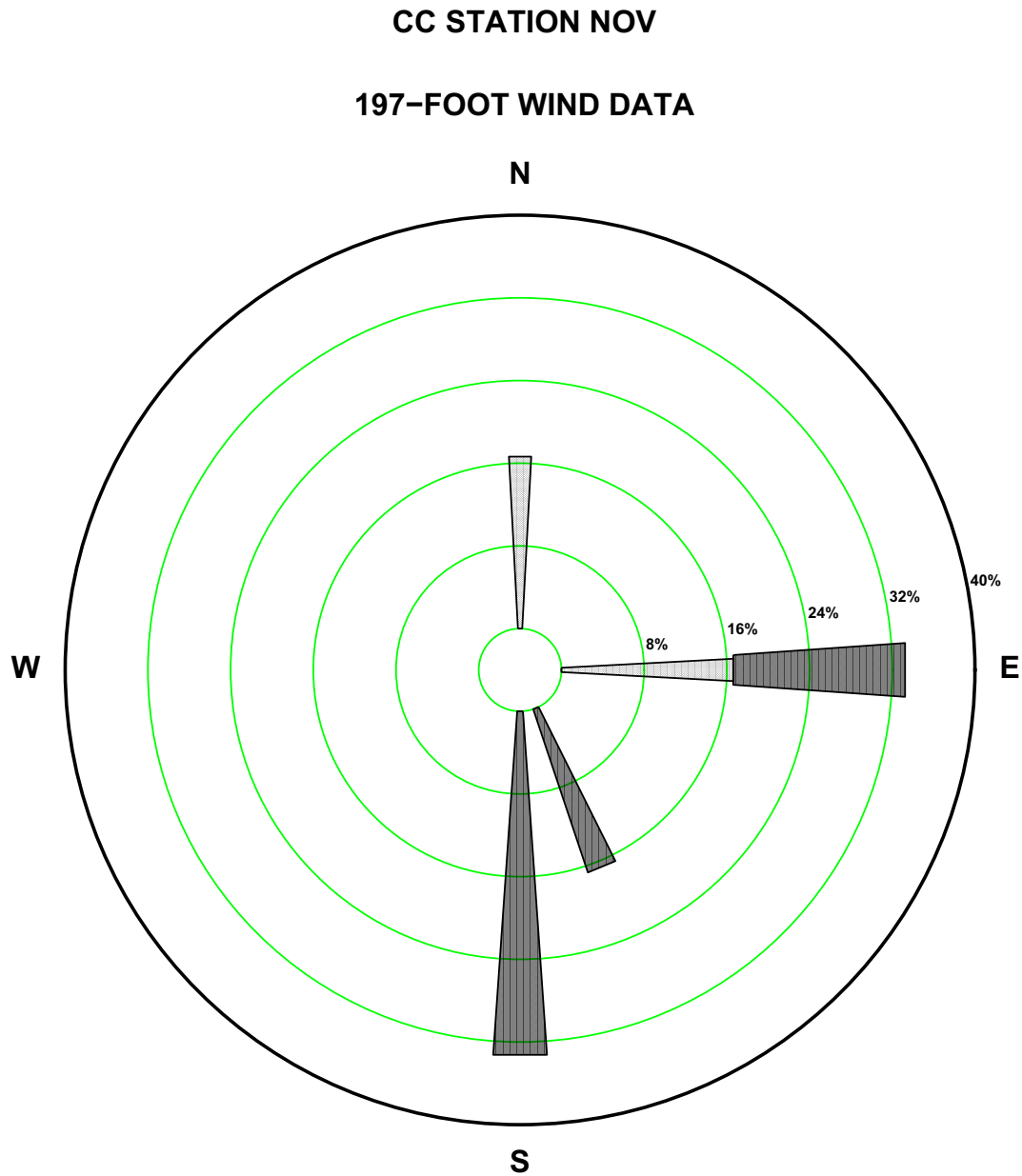
Figure 2.7-166—{CCNPP 197 ft November Precipitation Wind Rose for Rate Class 0.3-0.4 in/hr}
