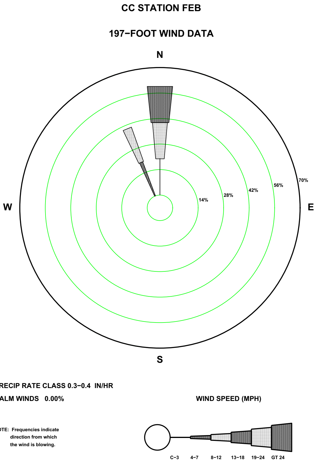
Figure 2.7-109—{CCNPP 197 ft February Precipitation Wind Rose for Rate Class 0.3-0.4 in/hr}
