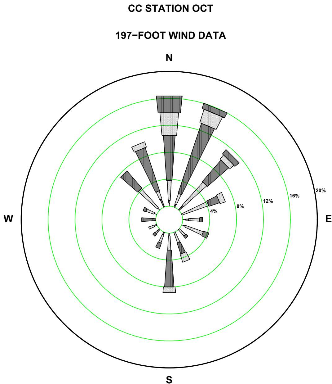
Figure 2.7-157—{CCNPP 197 ft October Precipitation Wind Rose for Rate Class 0.0-0.1 in/hr}
