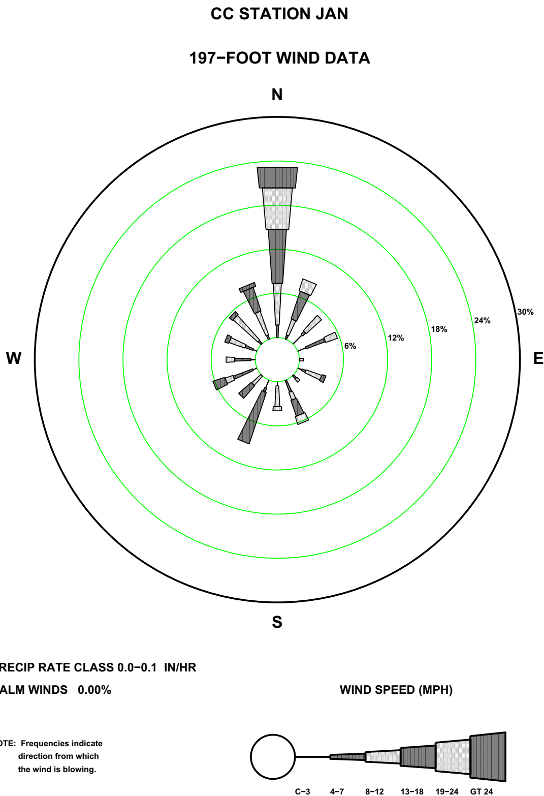
Figure 2.7-101—{CCNPP 197 ft January Precipitation Wind Rose for Rate Class 0.0-0.1 in/hr}
