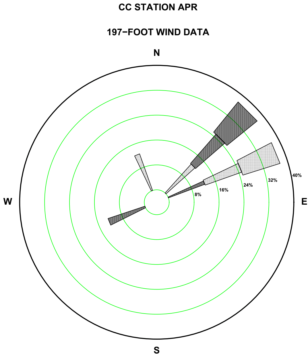
Figure 2.7-116—{CCNPP 197 ft April Precipitation Wind Rose for Rate Class 0.2-0.3 in/hr}
