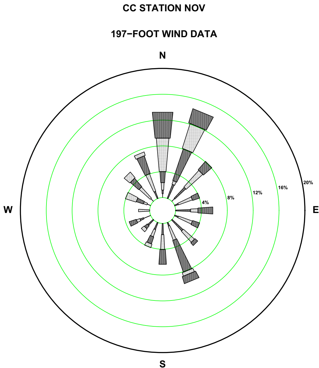
Figure 2.7-163—{CCNPP 197 ft November Precipitation Wind Rose for Rate Class 0.0-0.1 in/hr}
