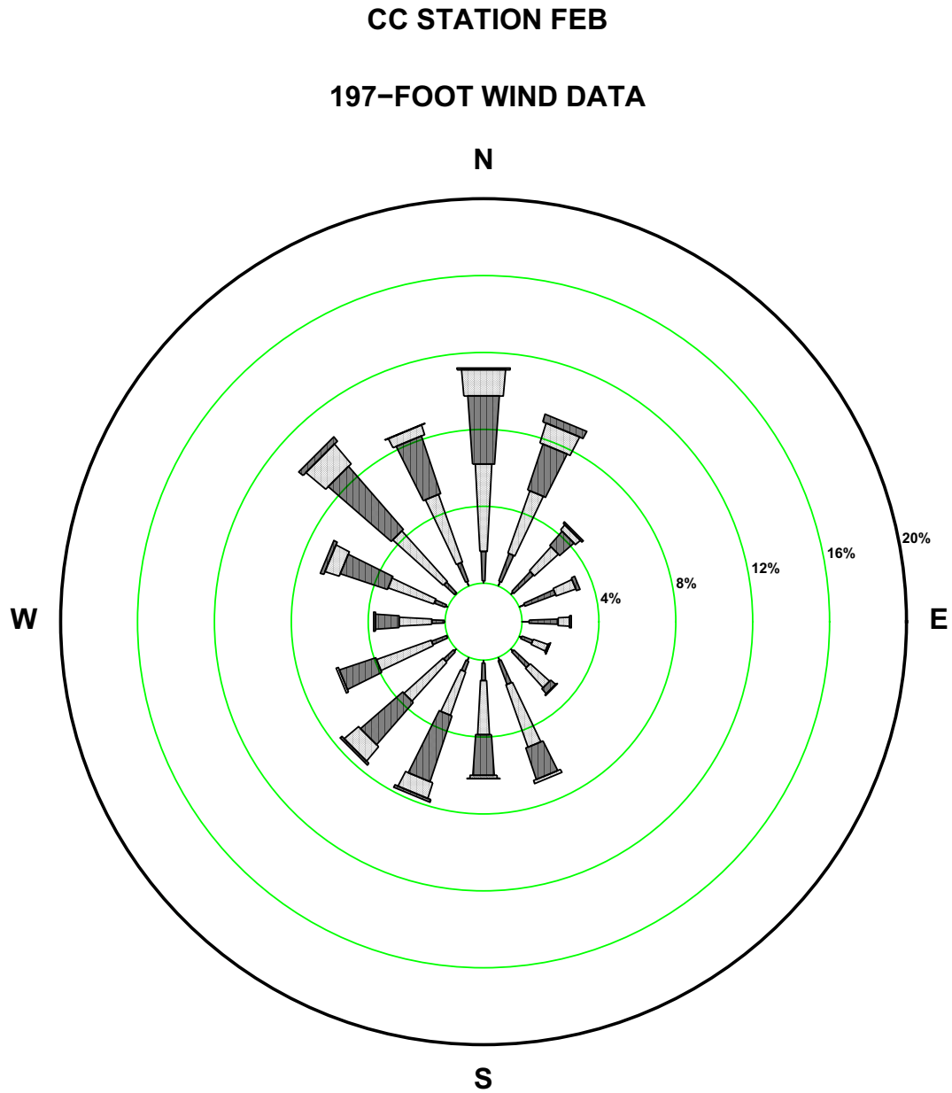
Figure 2.7-188—{CCNPP 197 ft February Wind Rose}
