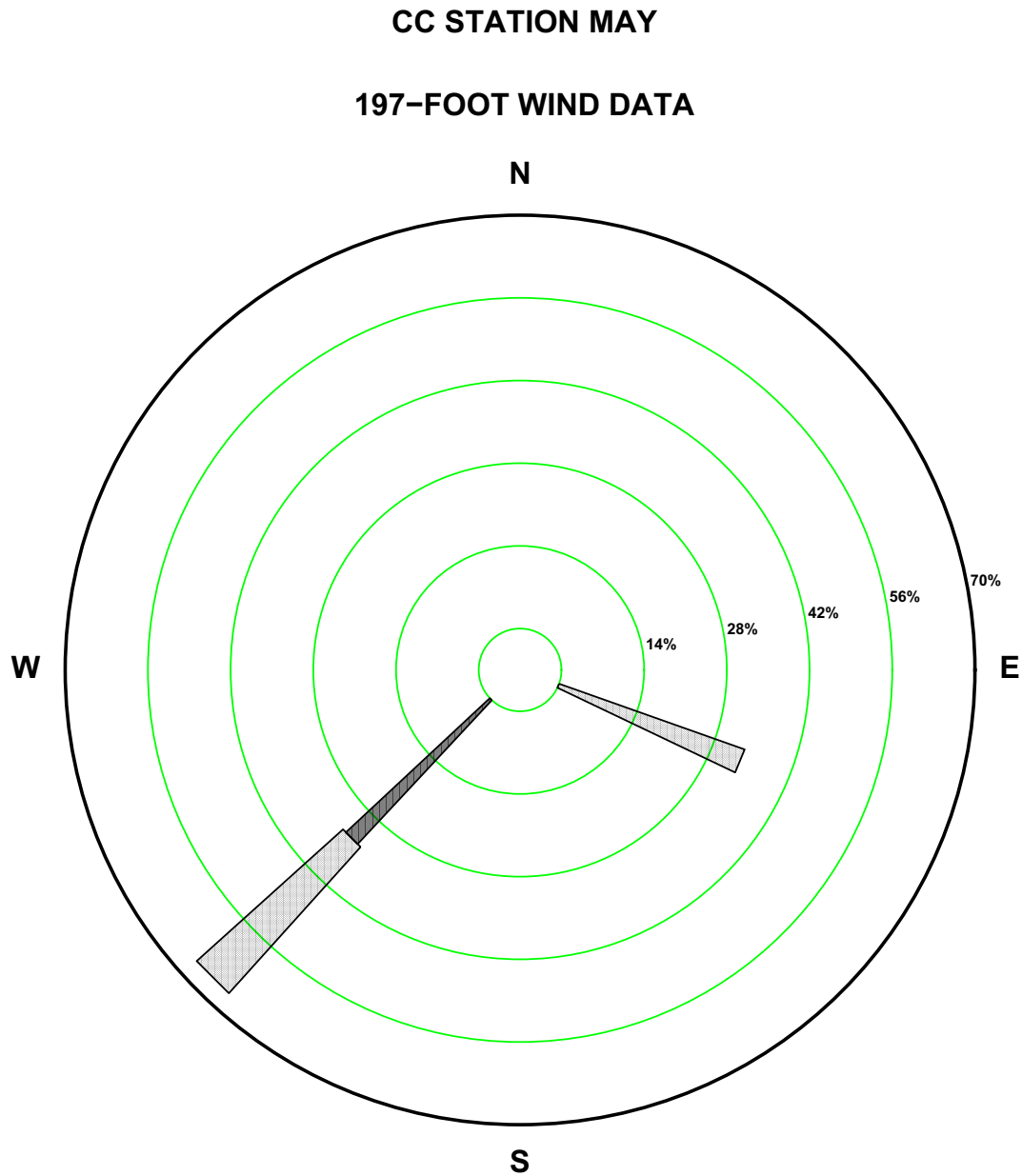
Figure 2.7-124—{CCNPP 197 ft May Precipitation Wind Rose for Rate Class 0.5-0.6 in/hr}
