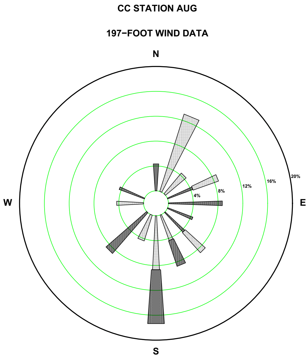
Figure 2.7-143—{CCNPP 197 ft August Precipitation Wind Rose for Rate Class 0.1-0.2 in/hr}
