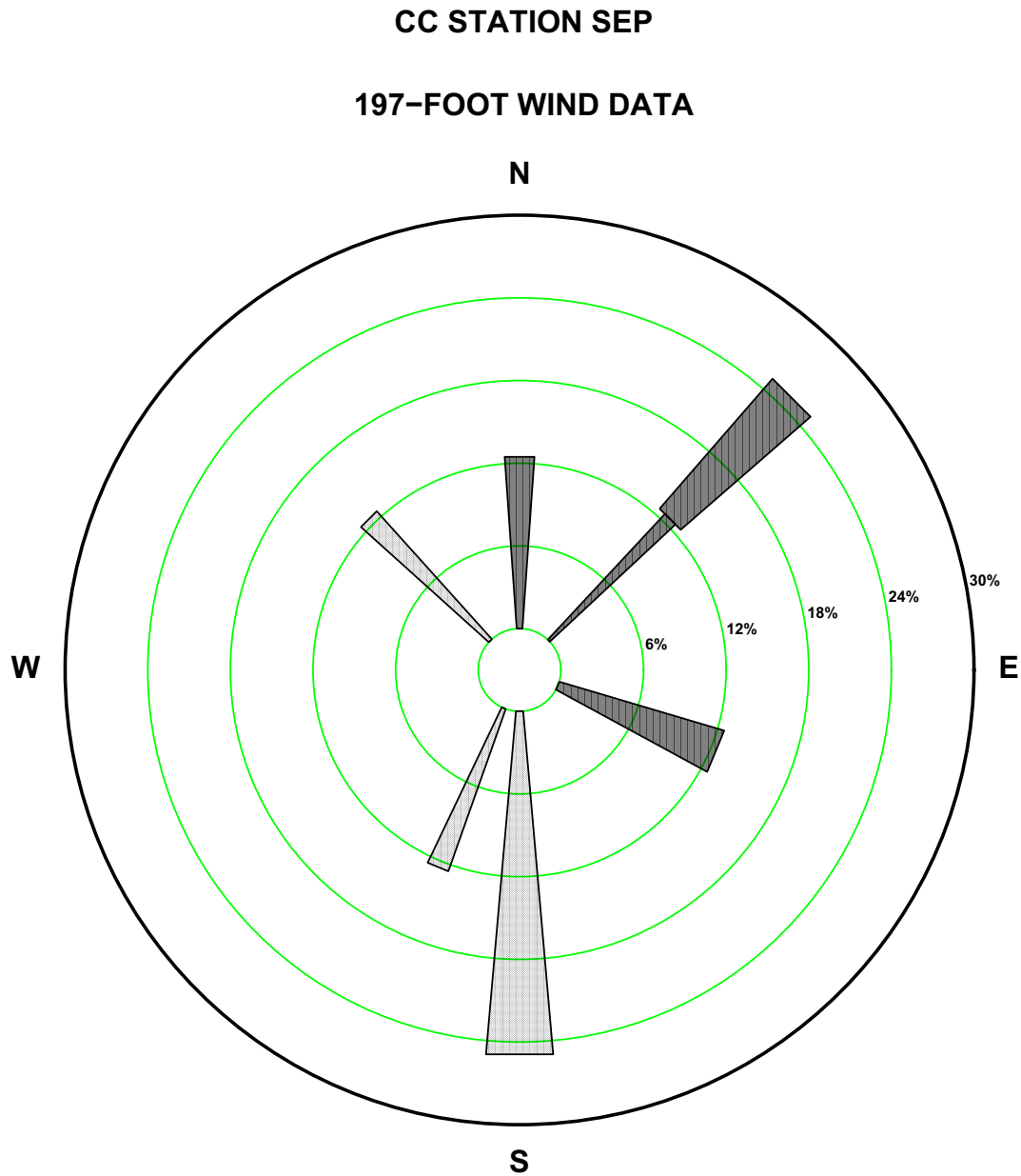
Figure 2.7-152—{CCNPP 197 ft September Precipitation Wind Rose for Rate Class 0.3-0.4 in/hr}
