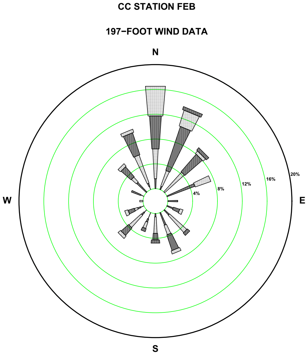
Figure 2.7-106—{CCNPP 197 ft February Precipitation Wind Rose for Rate Class 0.0-0.1 in/hr}
