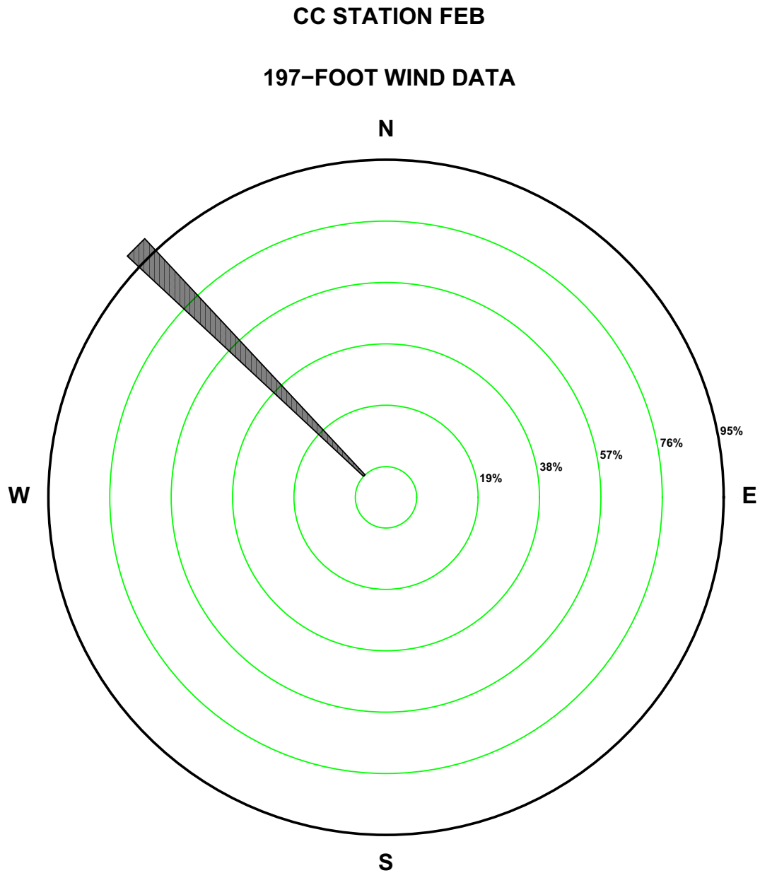
Figure 2.7-108—{CCNPP 197 ft February Precipitation Wind Rose for Rate Class 0.2-0.3 in/hr}
