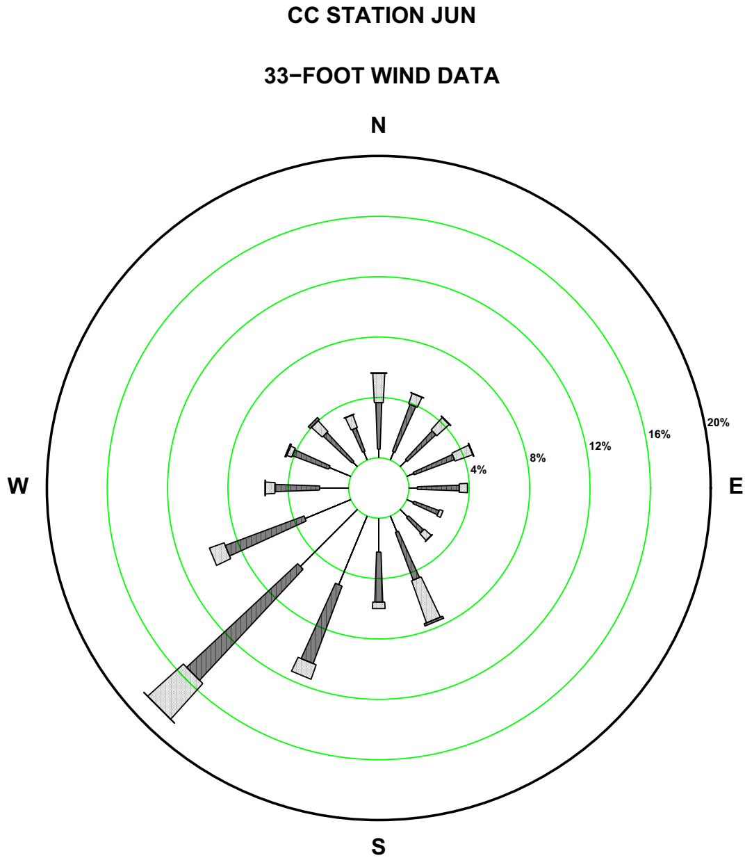
Figure 2.7-179—{CCNPP 33 ft June Wind Rose}
