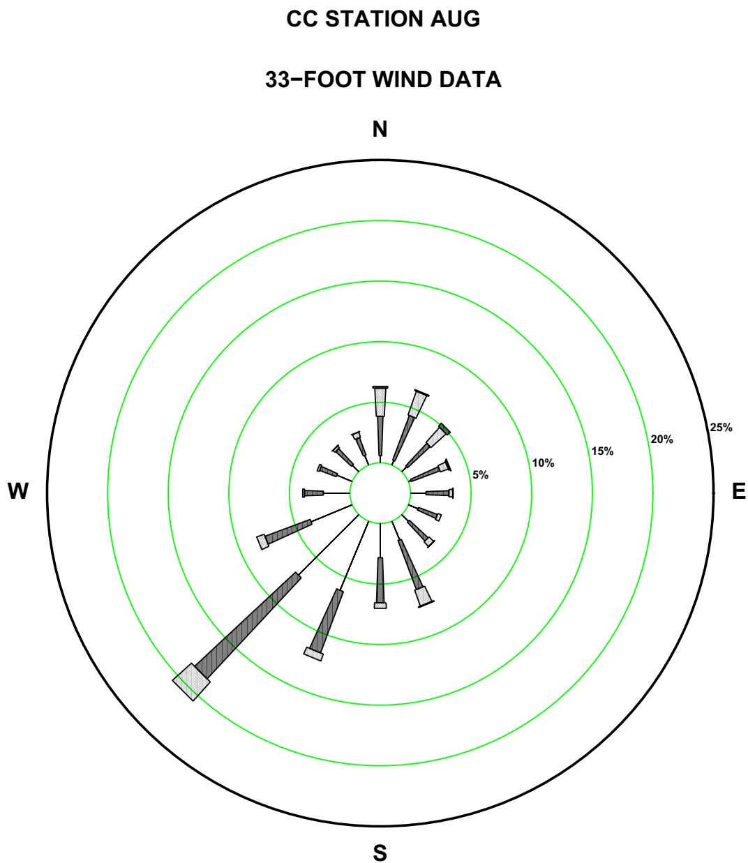
Figure 2.7-181—{CCNPP 33 ft August Wind Rose}
