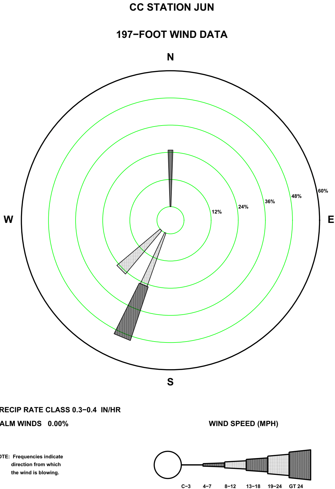
Figure 2.7-130—{CCNPP 197 ft June Precipitation Wind Rose for Rate Class 0.3-0.4 in/hr}
