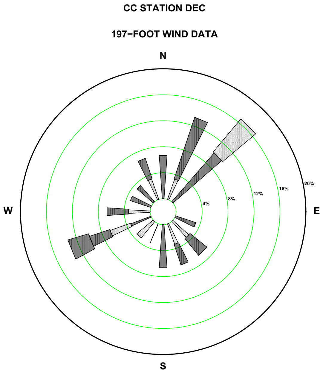
Figure 2.7-169—{CCNPP 197 ft December Precipitation Wind Rose for Rate Class 0.1-0.2 in/hr}
