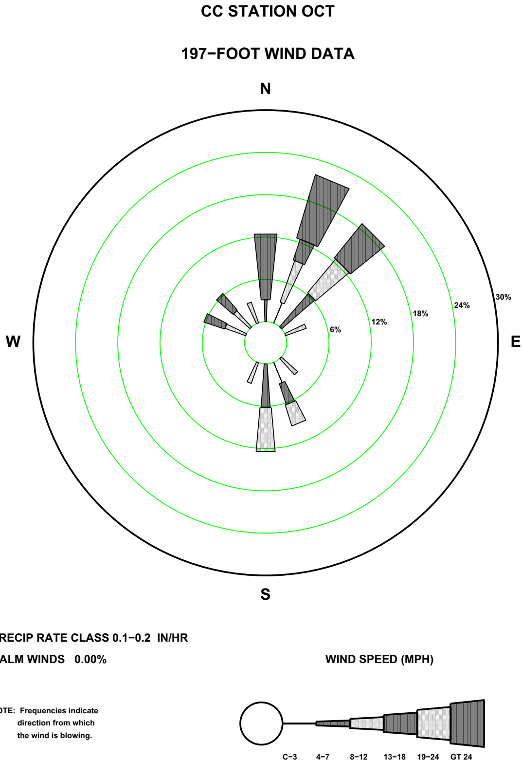
Figure 2.7-158—{CCNPP 197 ft October Precipitation Wind Rose for Rate Class 0.1-0.2 in/hr}
