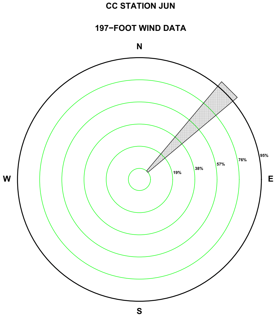
Figure 2.7-132—{CCNPP 197 ft June Precipitation Wind Rose for Rate Class 0.6-0.7 in/hr}
