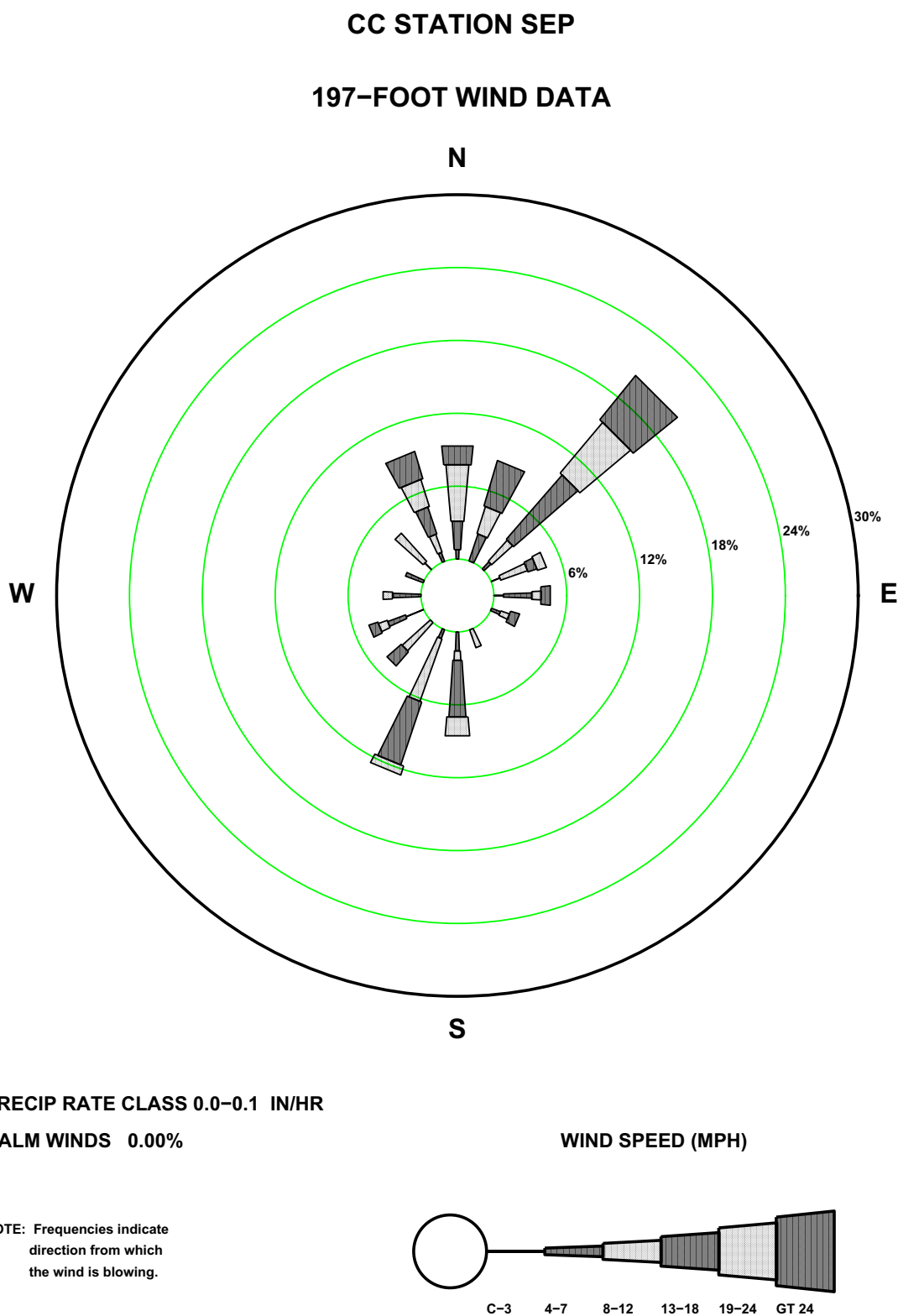
Figure 2.7-149—{CCNPP 197 ft September Precipitation Wind Rose for Rate Class 0.0-0.1 in/hr}
