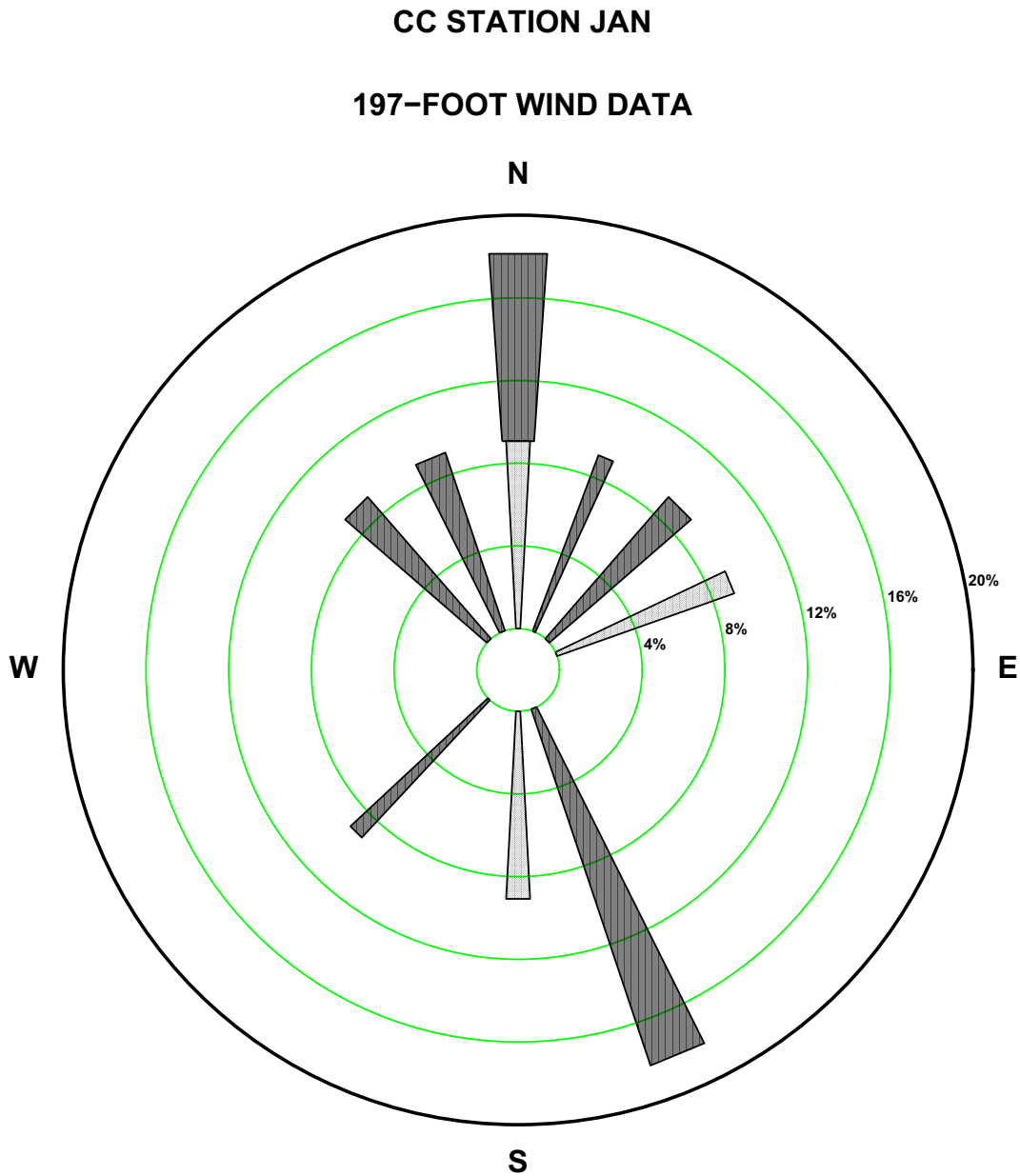
Figure 2.7-102—{CCNPP 197 ft January Precipitation Wind Rose for Rate Class 0.1-0.2 in/hr}
