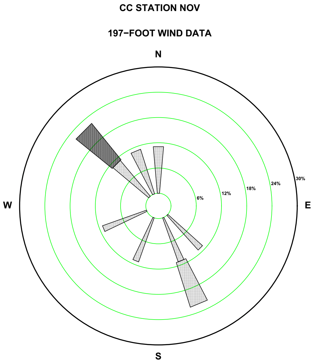
Figure 2.7-165—{CCNPP 197 ft November Precipitation Wind Rose for Rate Class 0.2-0.3 in/hr}
