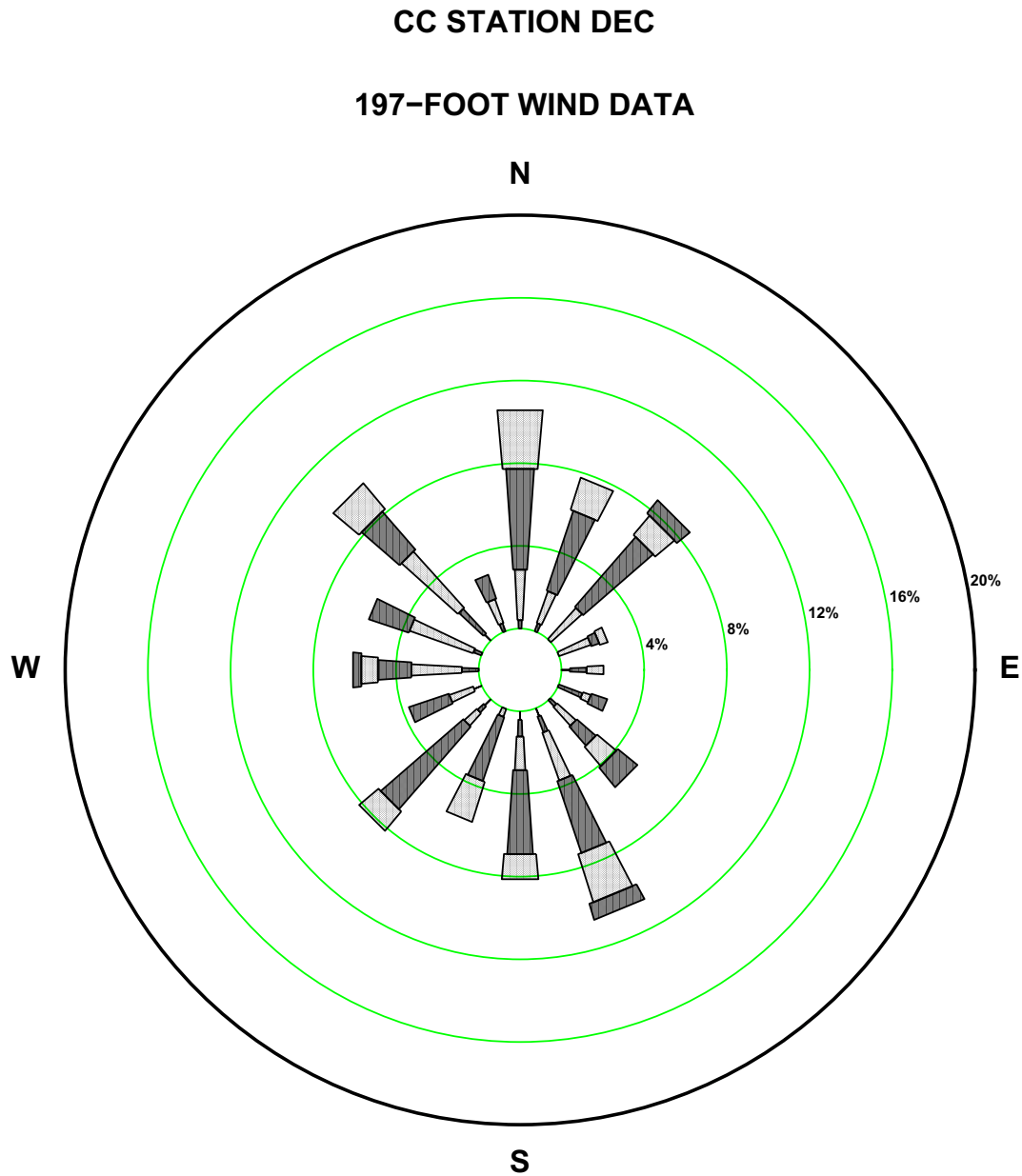
Figure 2.7-168—{CCNPP 197 ft December Precipitation Wind Rose for Rate Class 0.0-0.1 in/hr}
