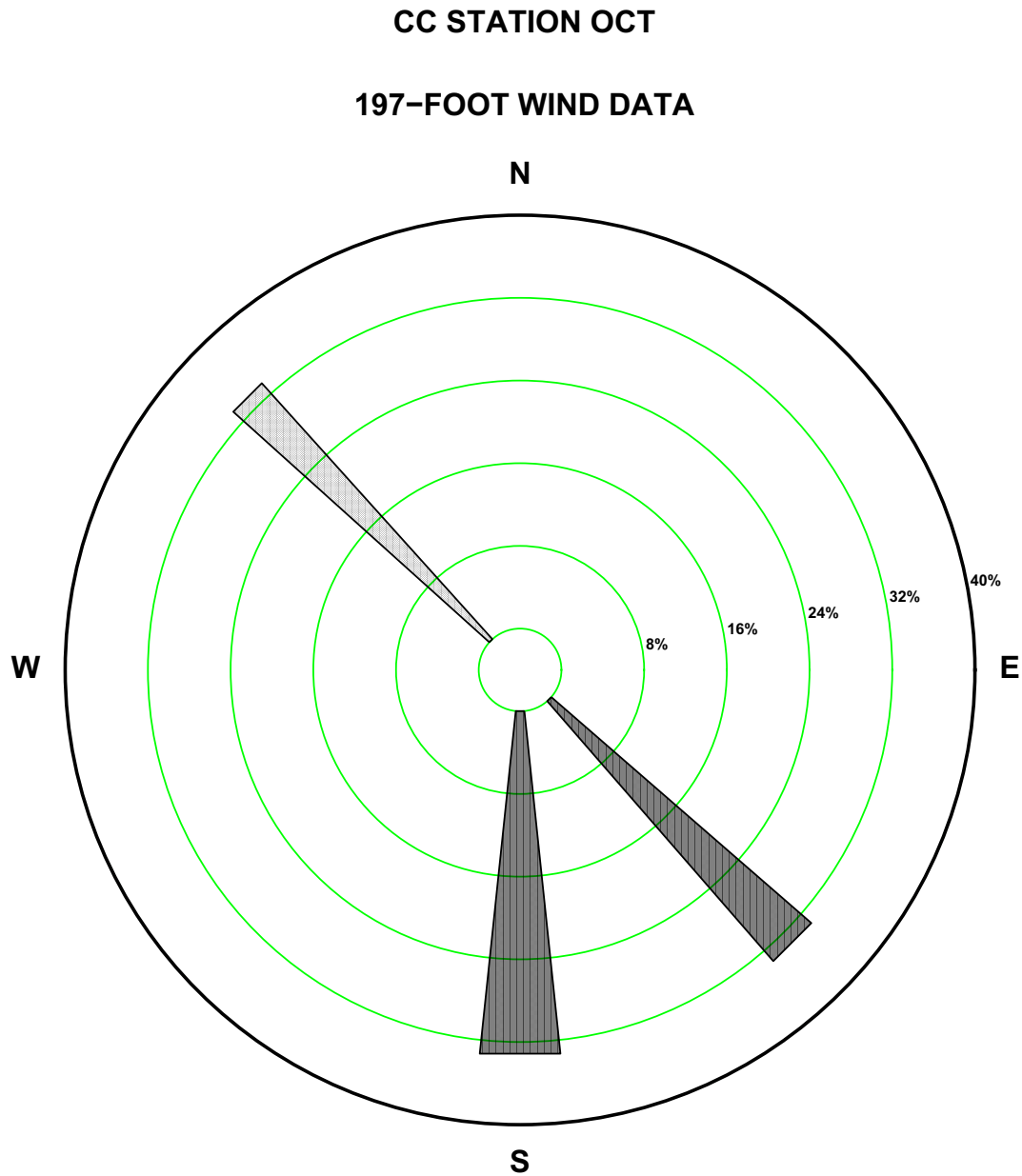
Figure 2.7-160—{CCNPP 197 ft October Precipitation Wind Rose for Rate Class 0.3-0.4 in/hr}
