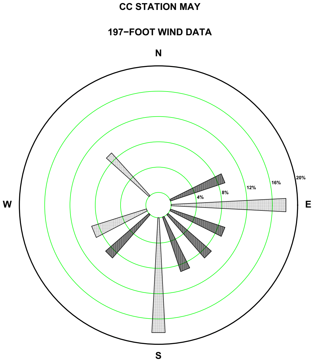
Figure 2.7-122—{CCNPP 197 ft May Precipitation Wind Rose for Rate Class 0.2-0.3 in/hr}
