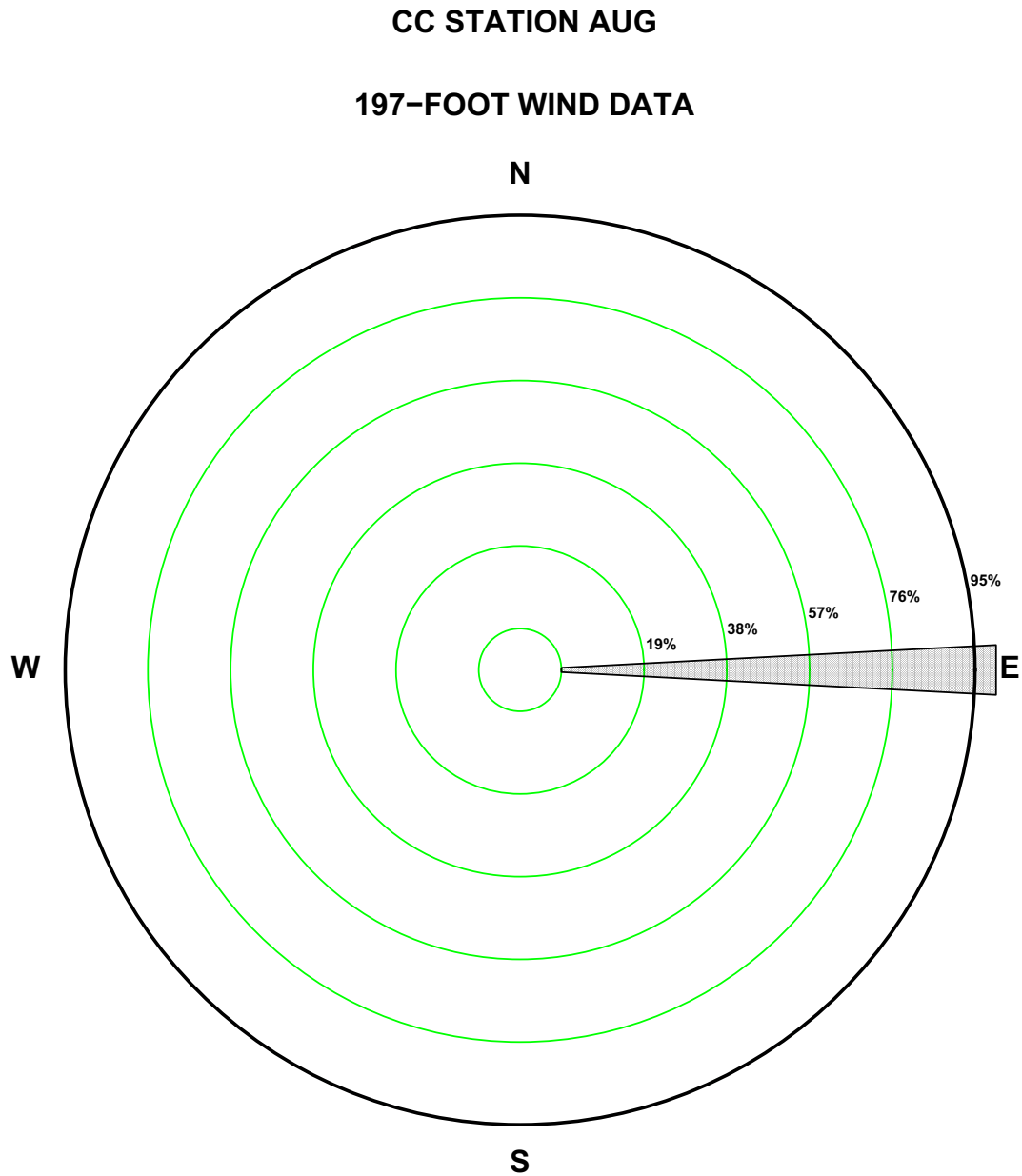
Figure 2.7-146—{CCNPP 197 ft August Precipitation Wind Rose for Rate Class 0.4-0.5 in/hr}
