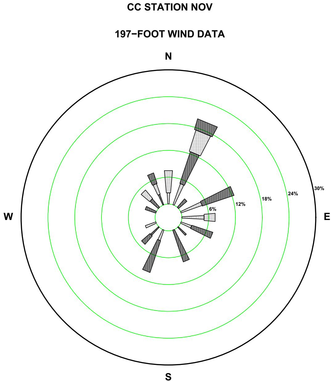
Figure 2.7-164—{CCNPP 197 ft November Precipitation Wind Rose for Rate Class 0.1-0.2 in/hr}
