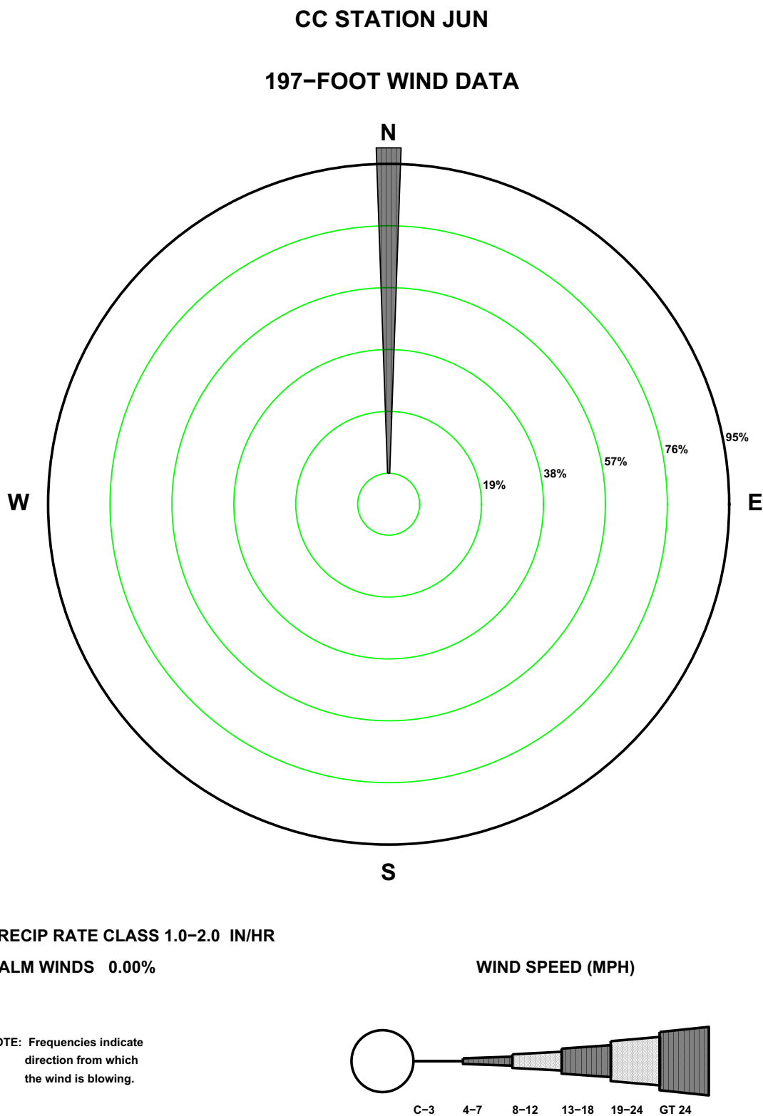
Figure 2.7-133—{CCNPP 197 ft June Precipitation Wind Rose for Rate Class 1.0-2.0 in/hr}
