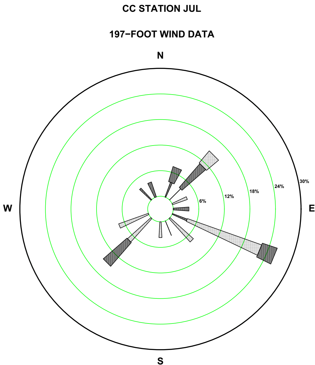
Figure 2.7-135—{CCNPP 197 ft July Precipitation Wind Rose for Rate Class 0.1-0.2 in/hr}
