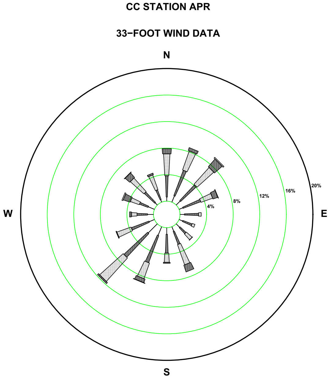
Figure 2.7-177—{CCNPP 33 ft April Wind Rose}
