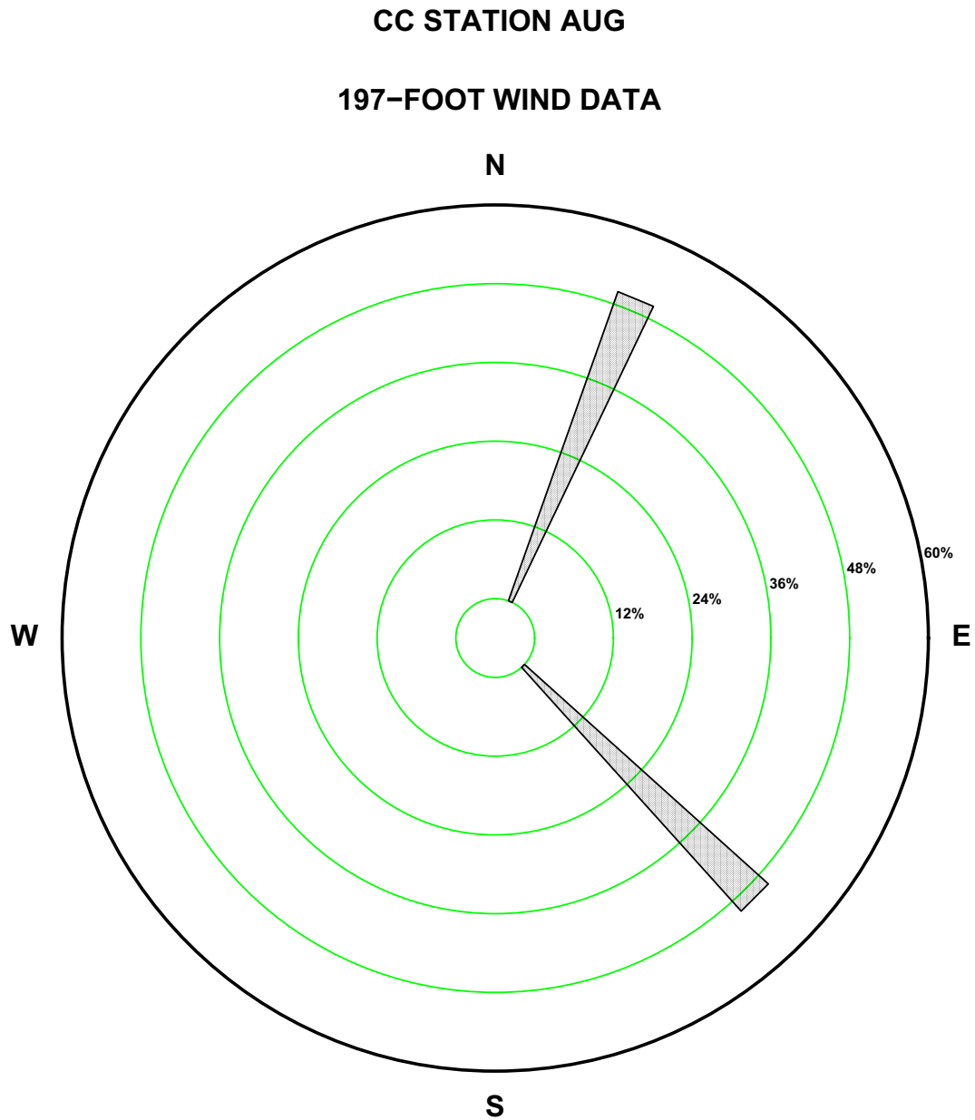
Figure 2.7-148—{CCNPP 197 ft August Precipitation Wind Rose for Rate Class 0.7-0.8 in/hr}
