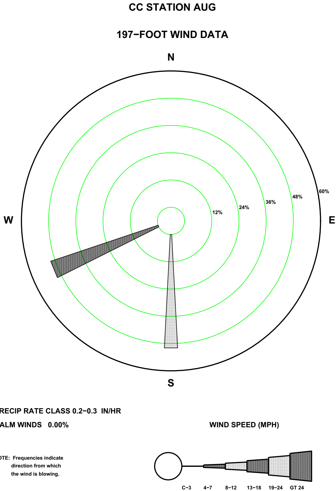
Figure 2.7-144—{CCNPP 197 ft August Precipitation Wind Rose for Rate Class 0.2-0.3 in/hr}
