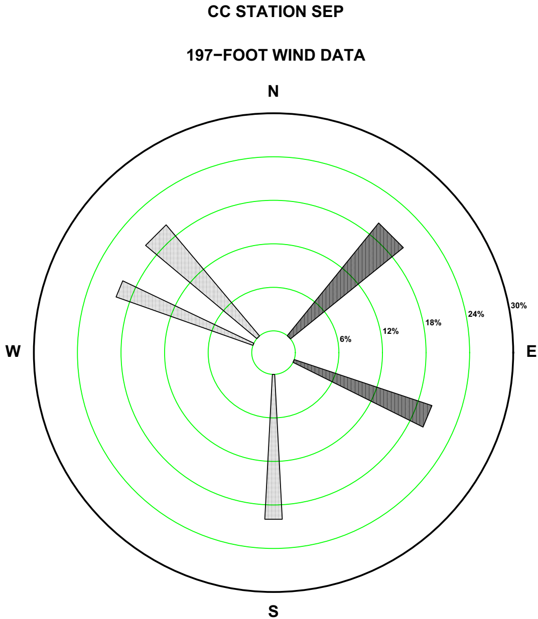
Figure 2.7-153—{CCNPP 197 ft September Precipitation Wind Rose for Rate Class 0.4-0.5 in/hr}
