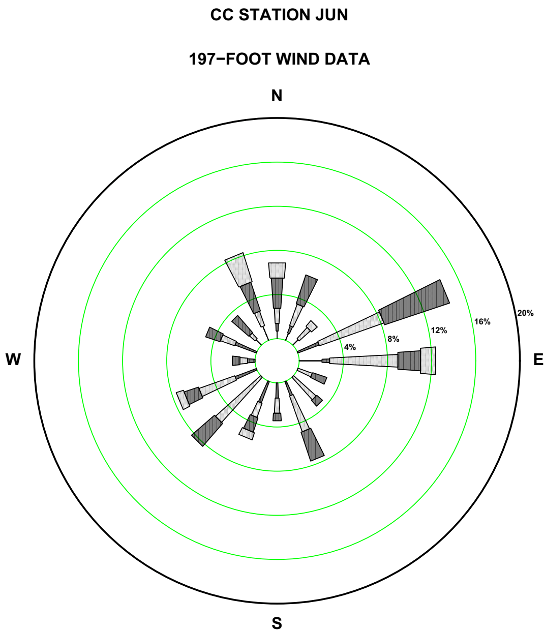
Figure 2.7-127—{CCNPP 197 ft June Precipitation Wind Rose for Rate Class 0.0-0.1 in/hr}
