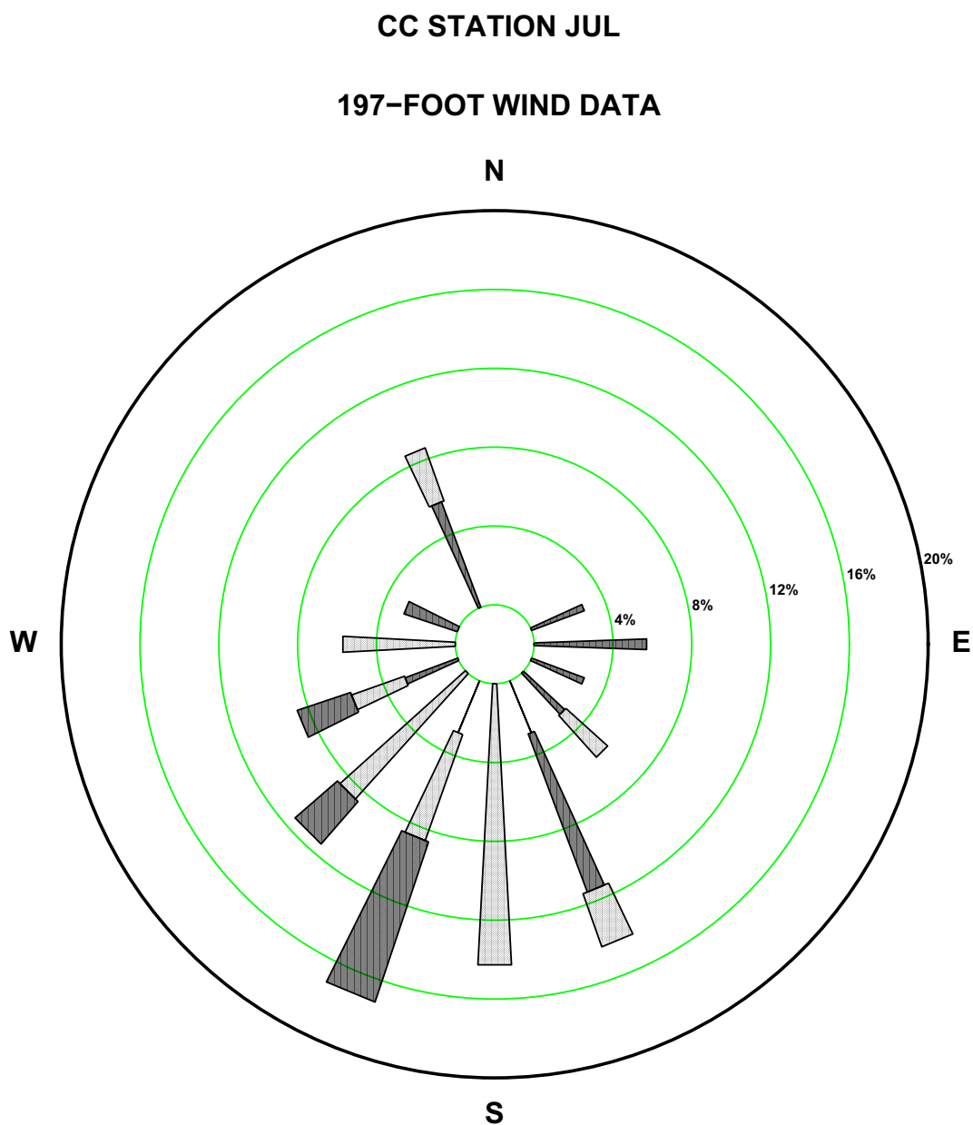
Figure 2.7-137—{CCNPP 197 ft July Precipitation Wind Rose for Rate Class 0.3-0.4 in/hr}
