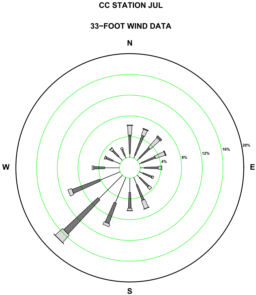
Figure 2.7-180—{CCNPP 33 ft July Wind Rose}
