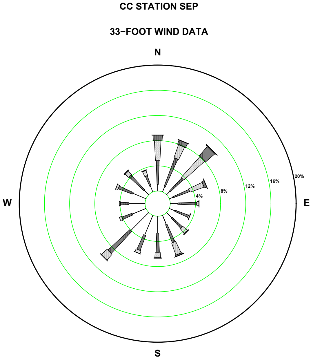
Figure 2.7-182—{CCNPP 33 ft September Wind Rose}
