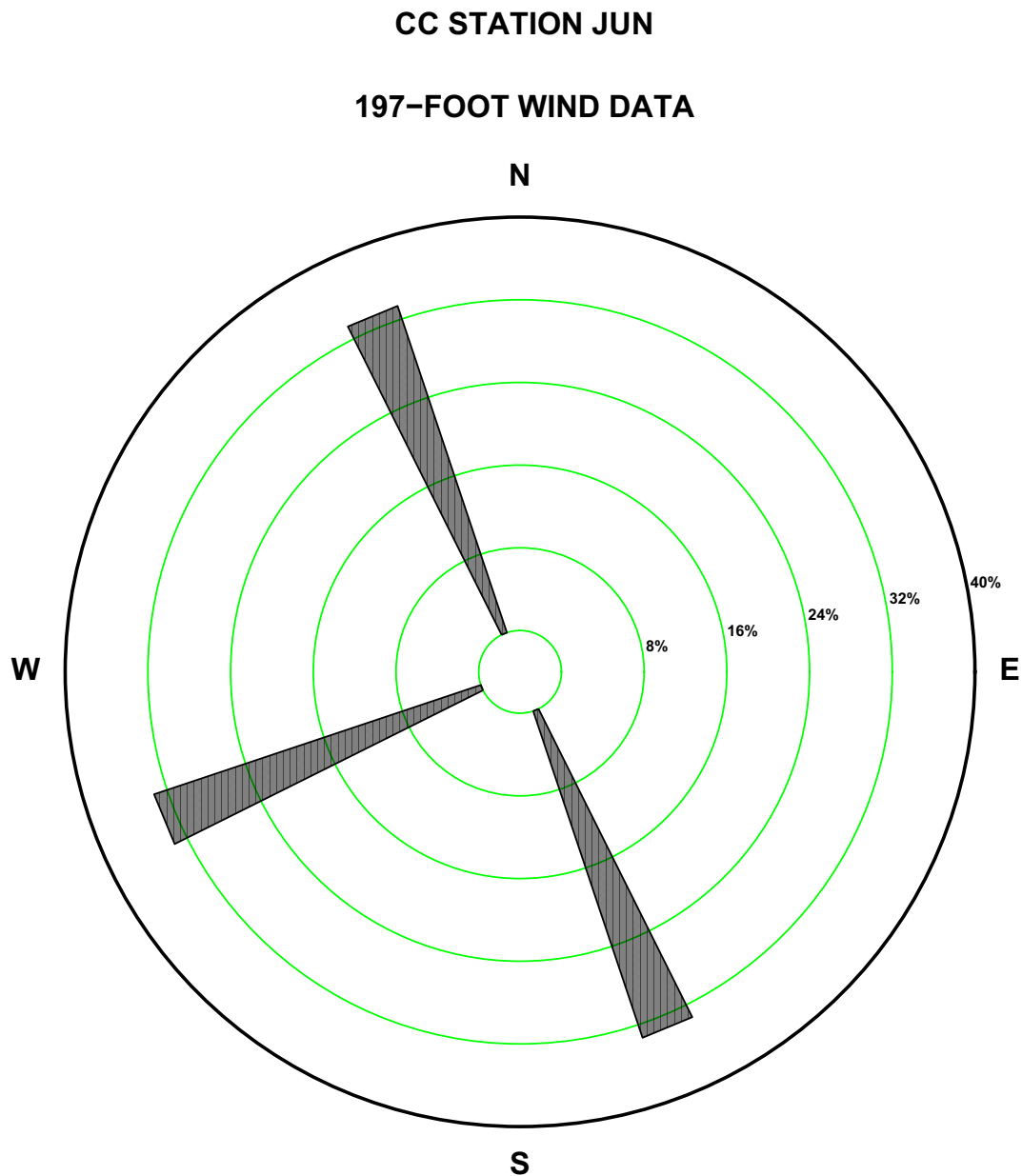
Figure 2.7-129—{CCNPP 197 ft June Precipitation Wind Rose for Rate Class 0.2-0.3 in/hr}
