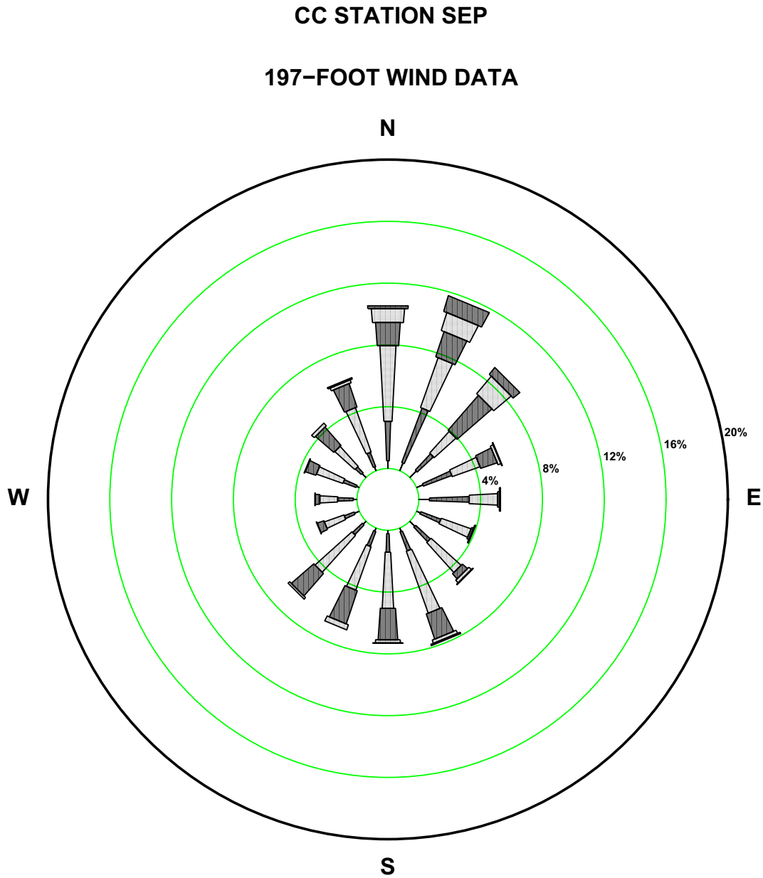
Figure 2.7-195—{CCNPP 197 ft September Wind Rose}
