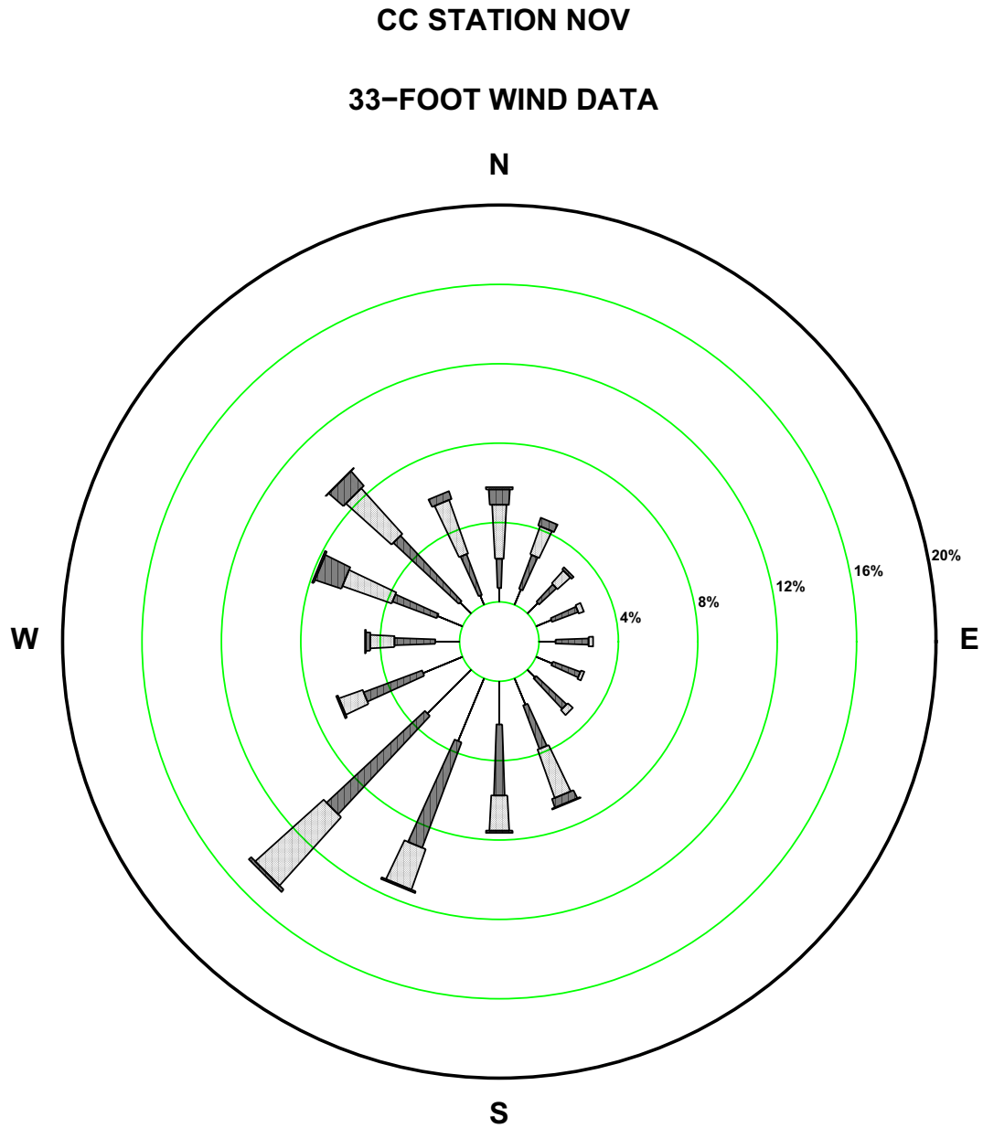
Figure 2.7-184—{CCNPP 33 ft November Wind Rose}
