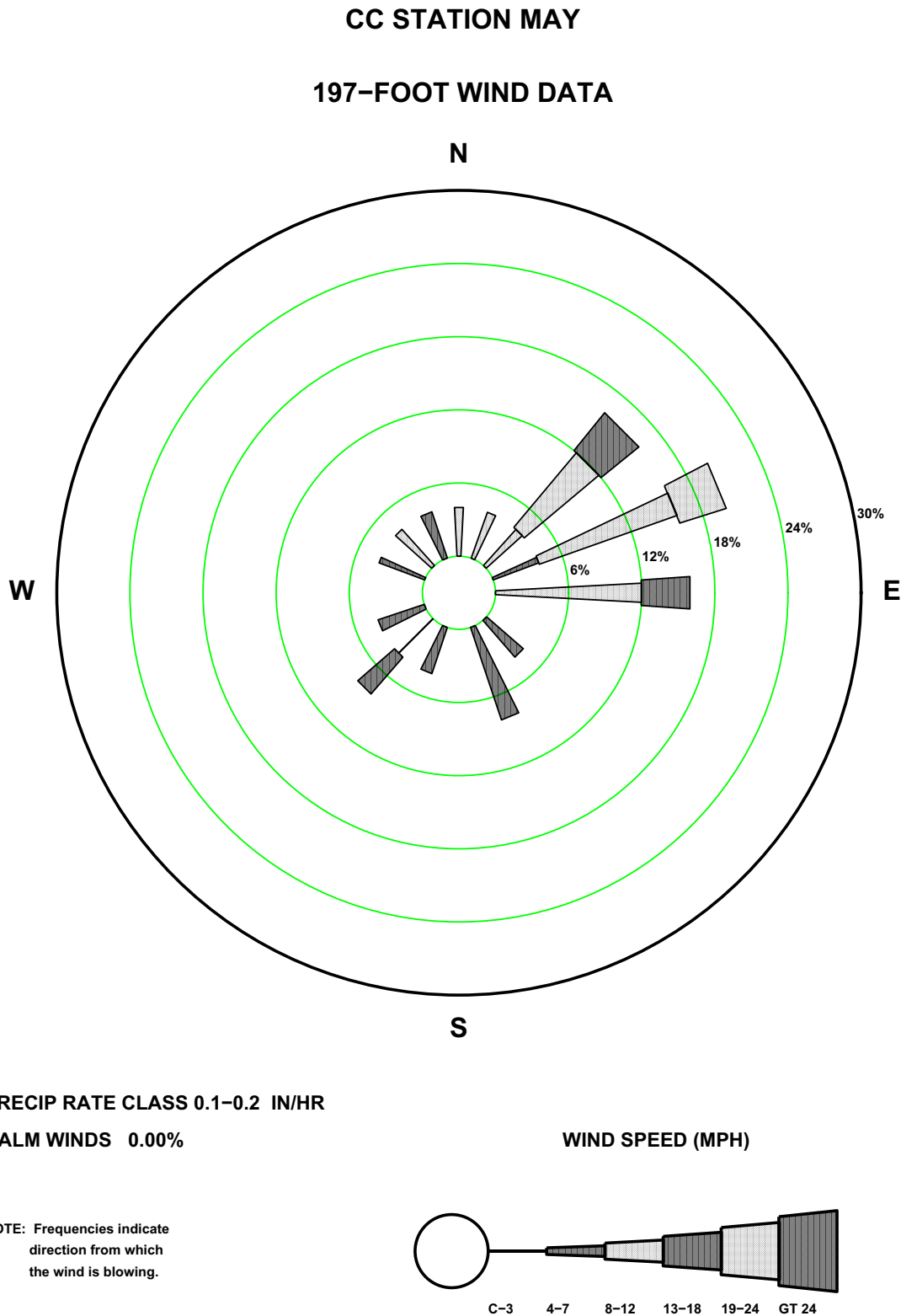
Figure 2.7-121—{CCNPP 197 ft May Precipitation Wind Rose for Rate Class 0.1-0.2 in/hr}
