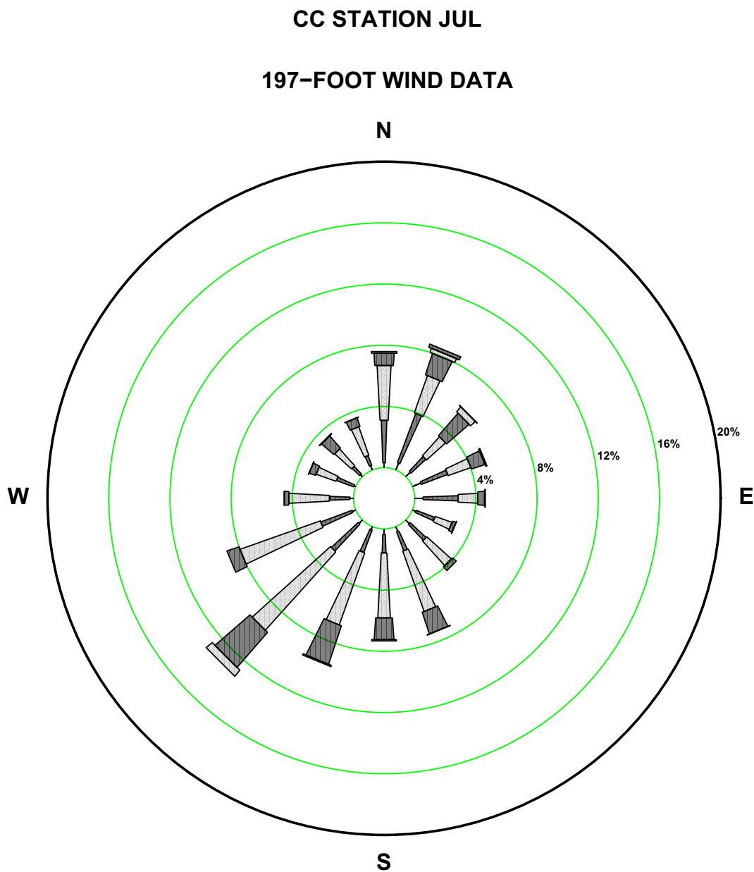
Figure 2.7-193—{CCNPP 197 ft July Wind Rose}
