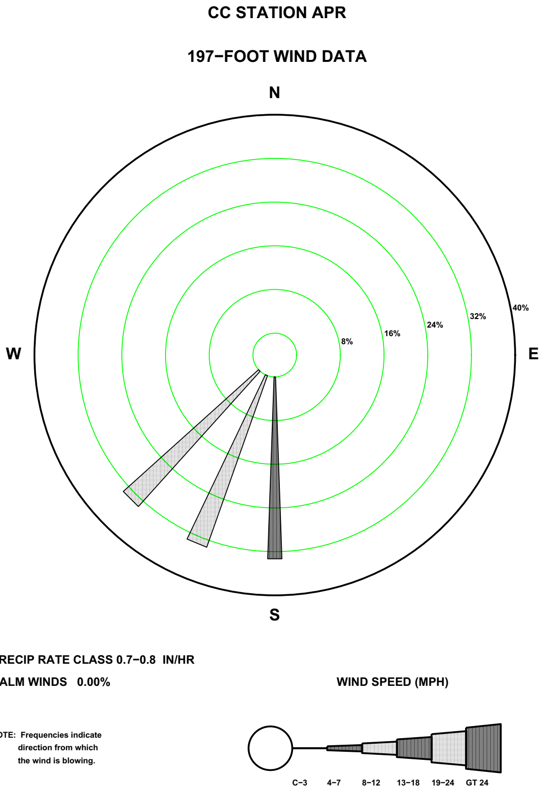
Figure 2.7-119—{CCNPP 197 ft April Precipitation Wind Rose for Rate Class 0.7-0.8 in/hr}
