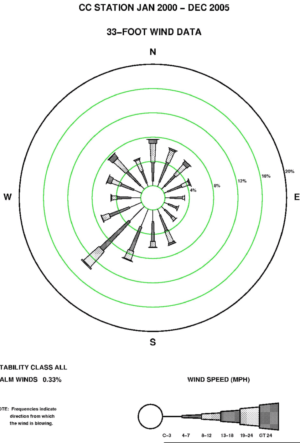
Figure 2.7-173—{CCNPP 33 ft Annual Wind Rose}
