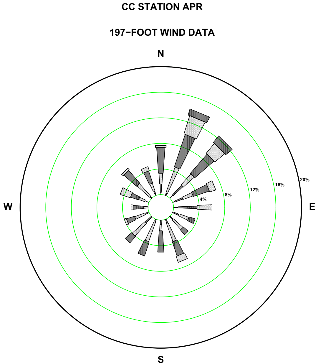
Figure 2.7-114—{CCNPP 197 ft April Precipitation Wind Rose for Rate Class 0.0-0.1 in/hr}
