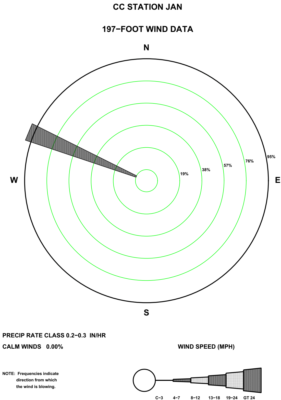
Figure 2.7-103—{CCNPP 197 ft January Precipitation Wind Rose for Rate Class 0.2-0.3 in/hr}
