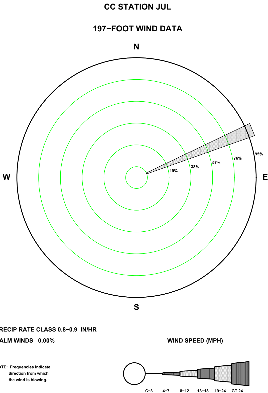
Figure 2.7-141—{CCNPP 197 ft July Precipitation Wind Rose for Rate Class 0.8-0.9 in/hr}
