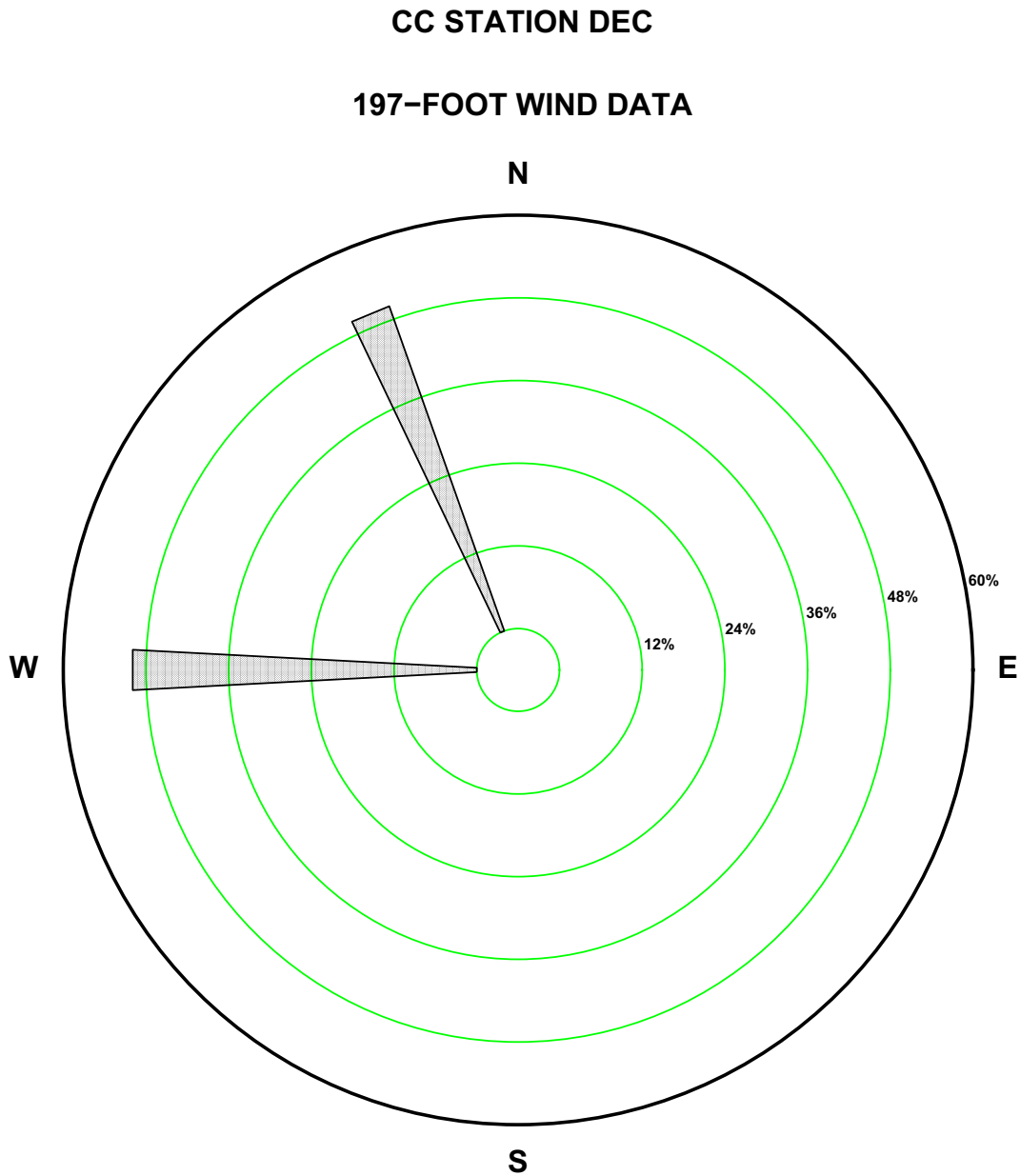
Figure 2.7-170—{CCNPP 197 ft December Precipitation Wind Rose for Rate Class 0.2-0.3 in/hr}
