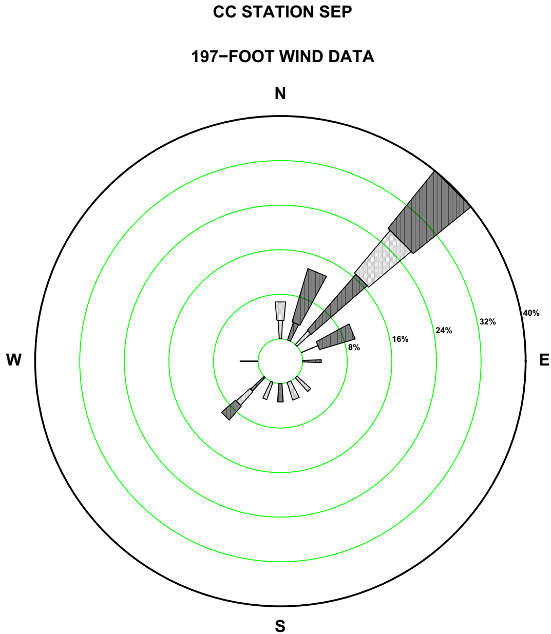
Figure 2.7-150—{CCNPP 197 ft September Precipitation Wind Rose for Rate Class 0.1-0.2 in/hr}
