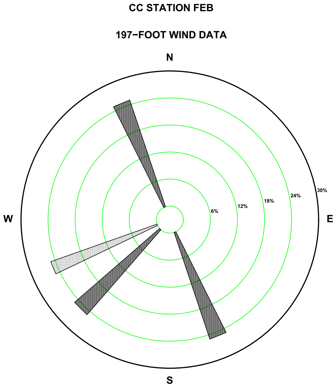
Figure 2.7-107—{CCNPP 197 ft February Precipitation Wind Rose for Rate Class 0.1-0.2 in/hr}
