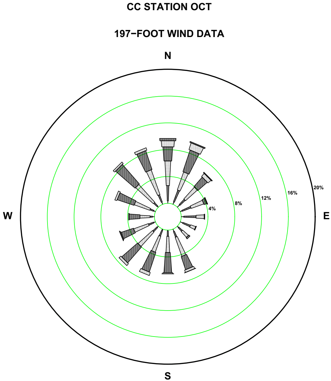
Figure 2.7-196—{CCNPP 197 ft October Wind Rose}
