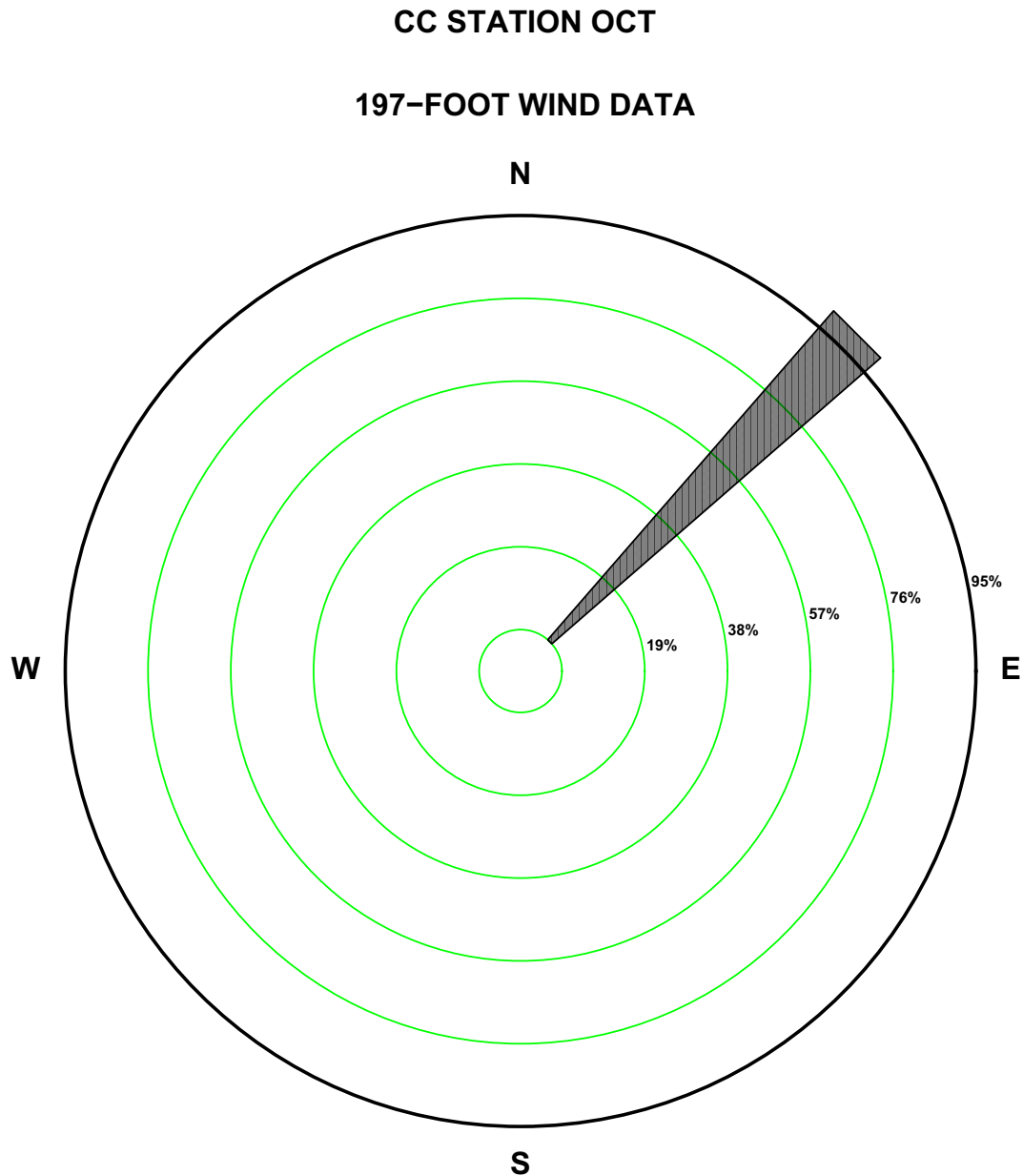
Figure 2.7-161—{CCNPP 197 ft October Precipitation Wind Rose for Rate Class 0.4-0.5 in/hr}
