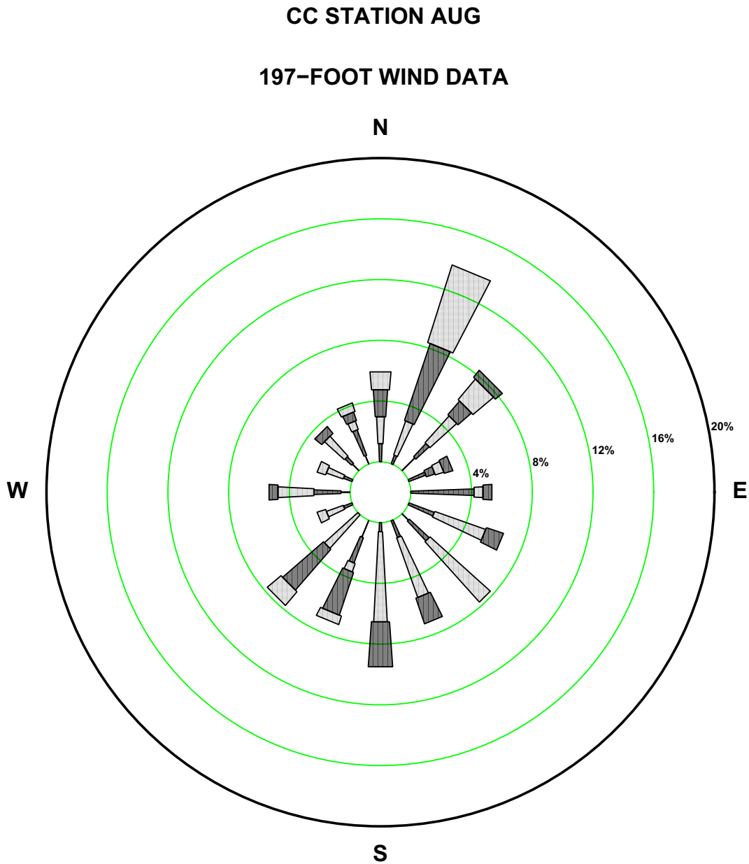
Figure 2.7-142—{CCNPP 197 ft August Precipitation Wind Rose for Rate Class 0.0-0.1 in/hr}
