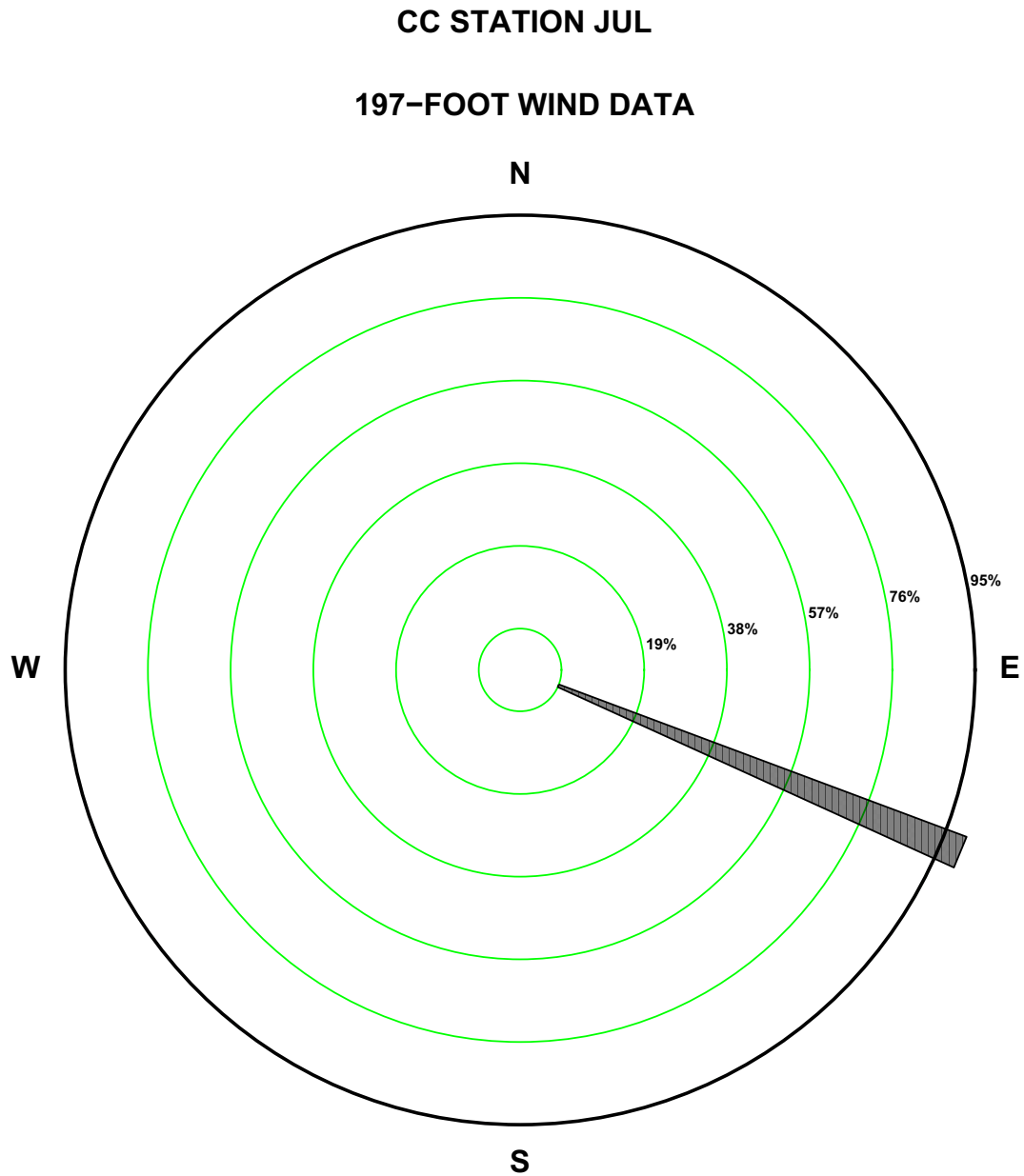
Figure 2.7-140—{CCNPP 197 ft July Precipitation Wind Rose for Rate Class 0.6-0.7 in/hr}
