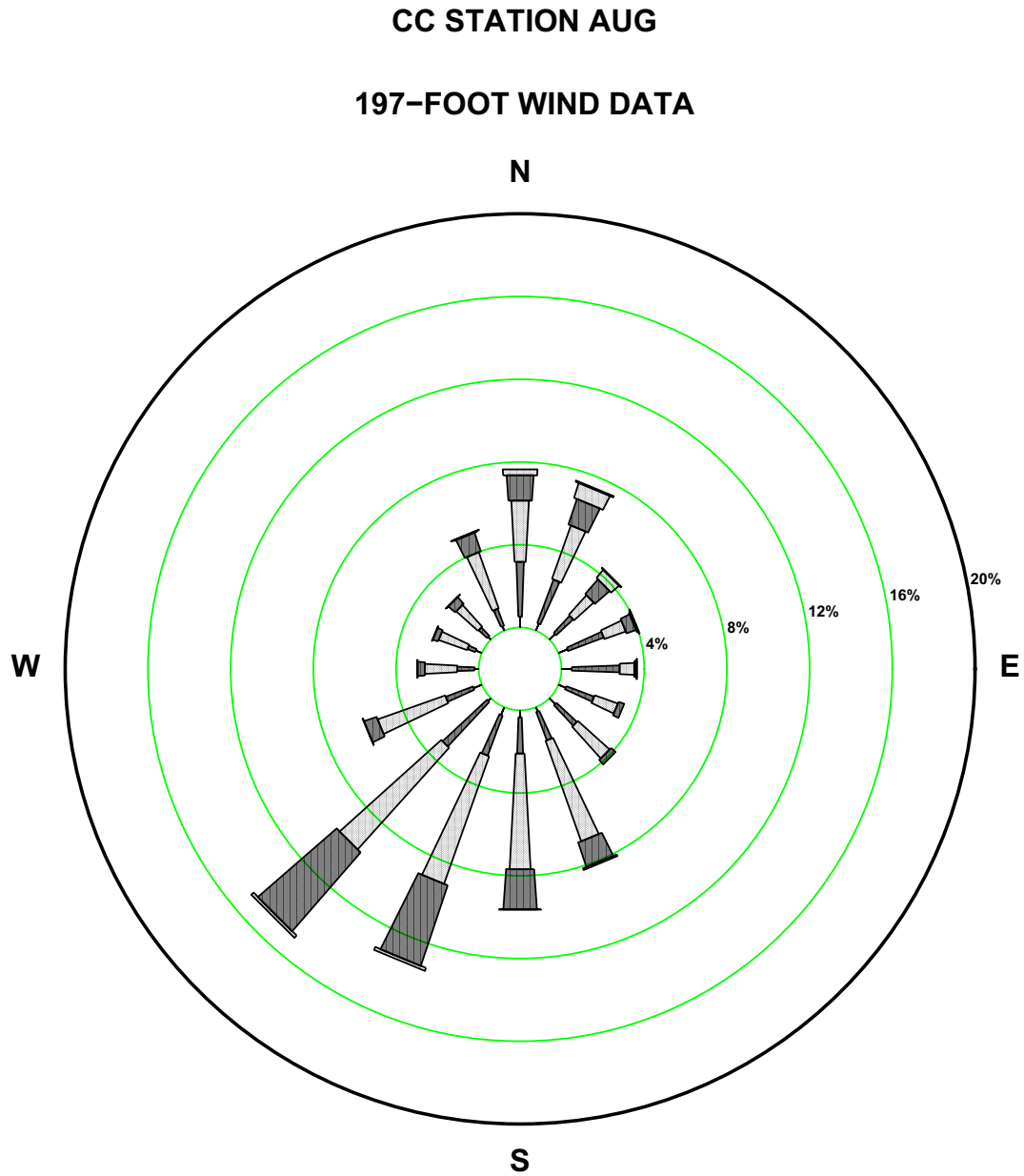
Figure 2.7-194—{CCNPP 197 ft August Wind Rose}
