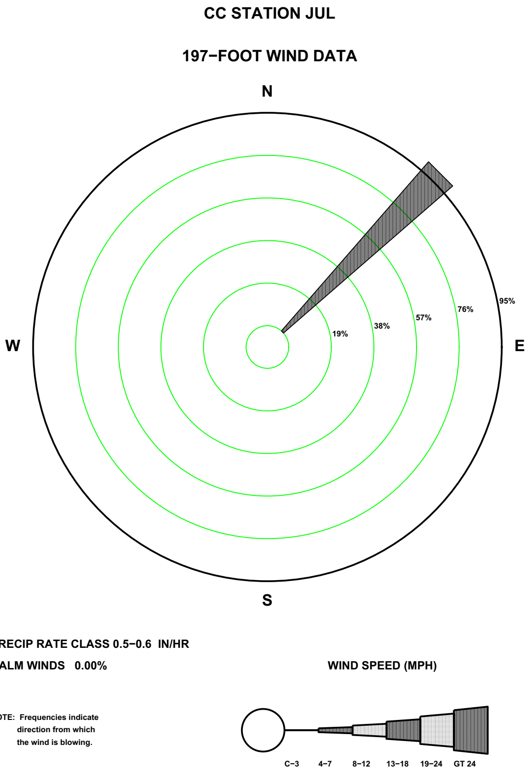
Figure 2.7-139—{CCNPP 197 ft July Precipitation Wind Rose for Rate Class 0.5-0.6 in/hr}
