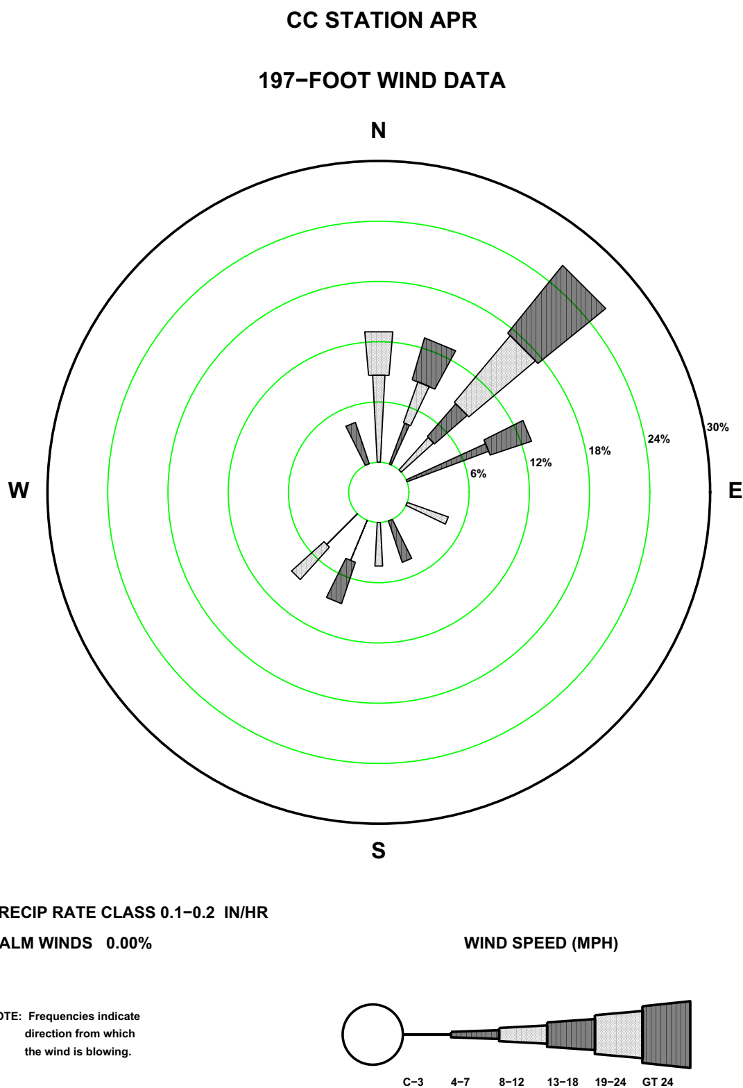
Figure 2.7-115—{CCNPP 197 ft April Precipitation Wind Rose for Rate Class 0.1-0.2 in/hr}
