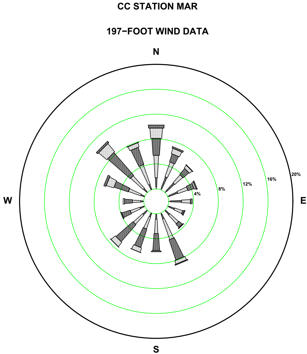
Figure 2.7-189—{CCNPP 197 ft March Wind Rose}
