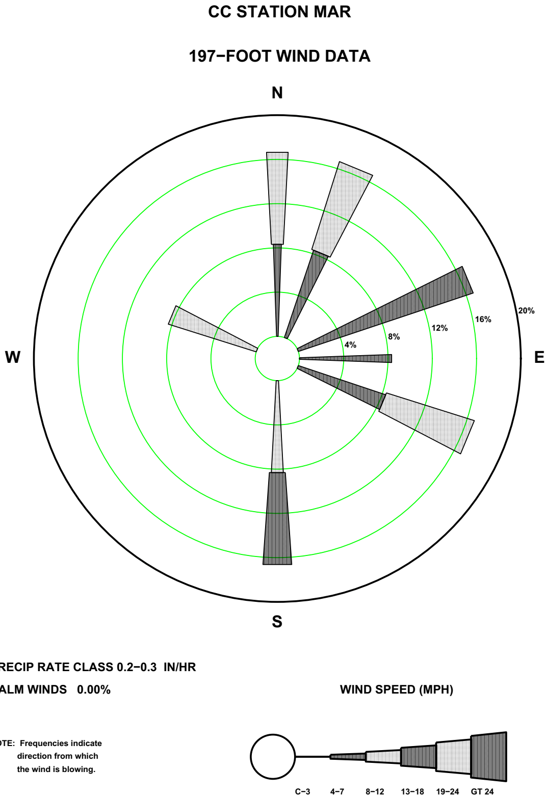
Figure 2.7-112—{CCNPP 197 ft March Precipitation Wind Rose for Rate Class 0.2-0.3 in/hr}
