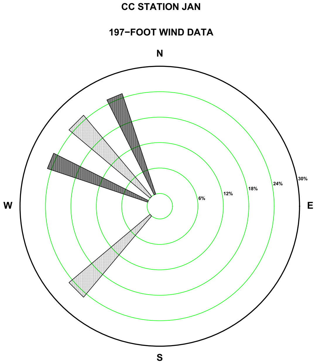
Figure 2.7-104—{CCNPP 197 ft January Precipitation Wind Rose for Rate Class 0.3-0.4 in/hr}
