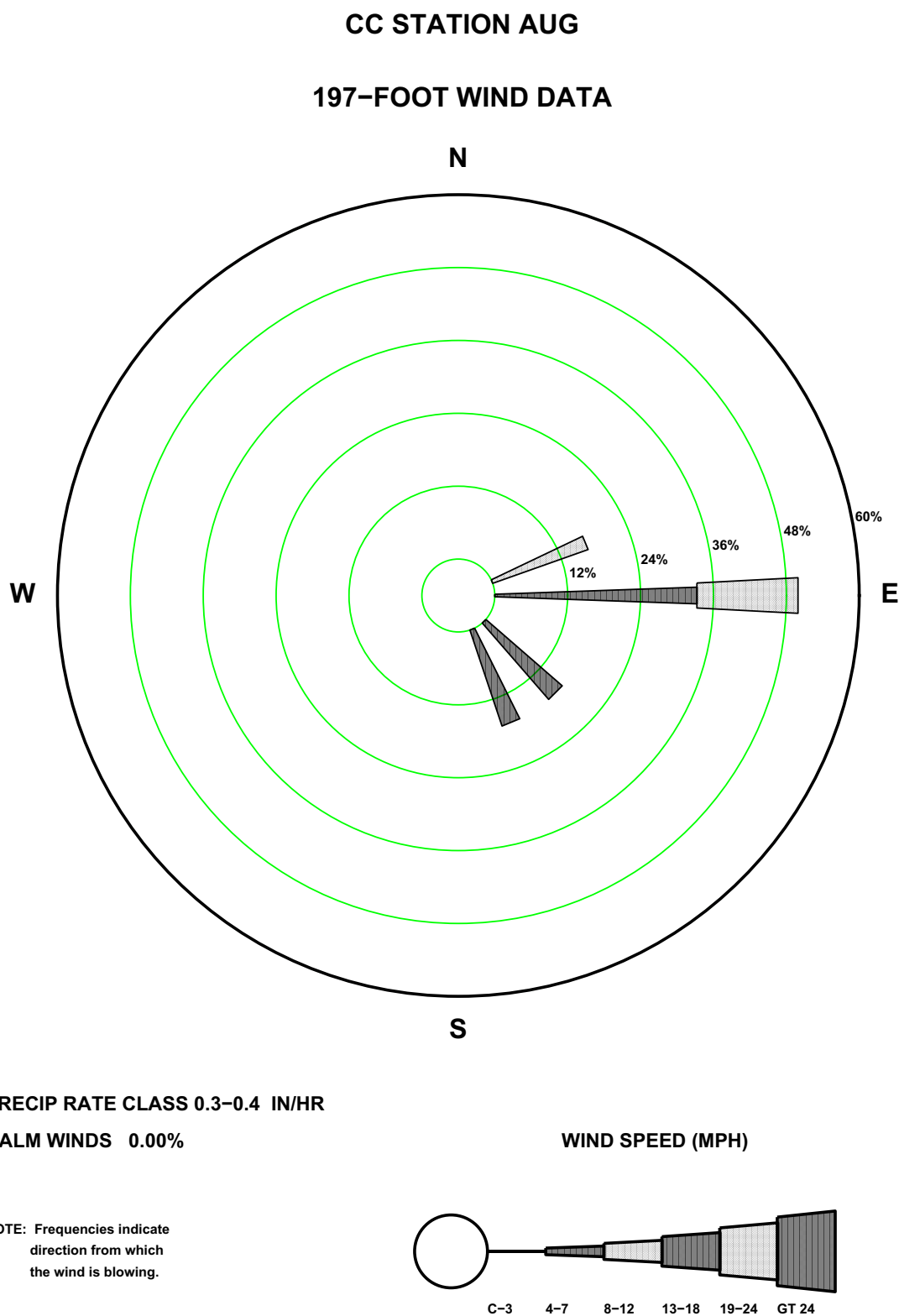
Figure 2.7-145—{CCNPP 197 ft August Precipitation Wind Rose for Rate Class 0.3-0.4 in/hr}
