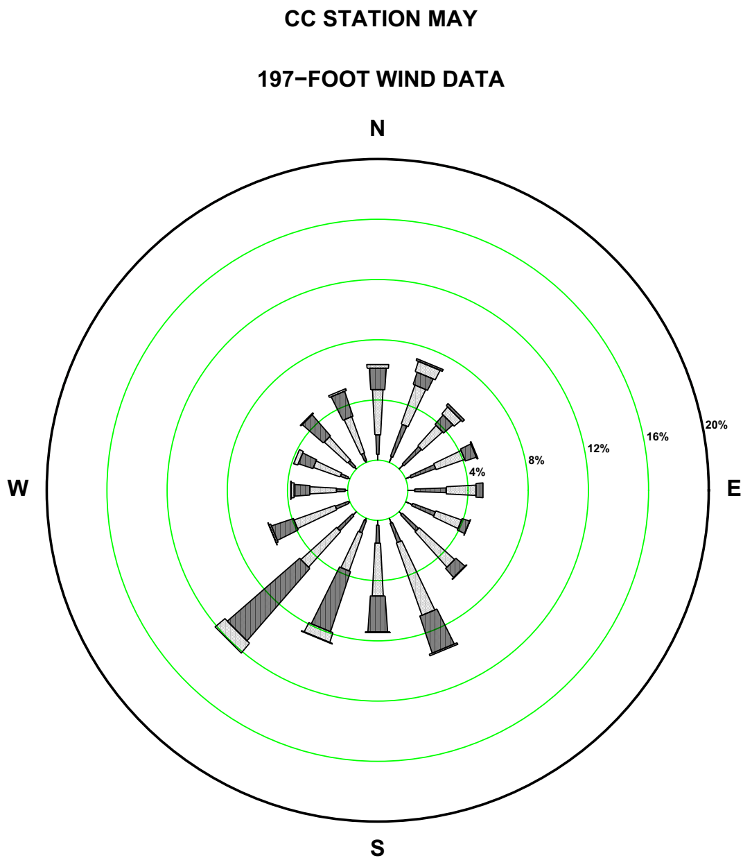
Figure 2.7-191—{CCNPP 197 ft May Wind Rose}
