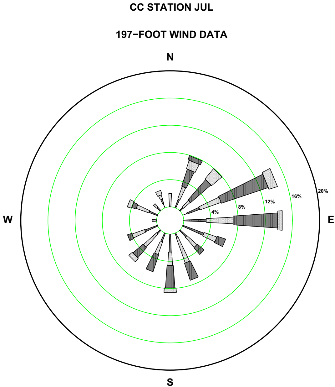
Figure 2.7-134—{CCNPP 197 ft July Precipitation Wind Rose for Rate Class 0.0-0.1 in/hr}
