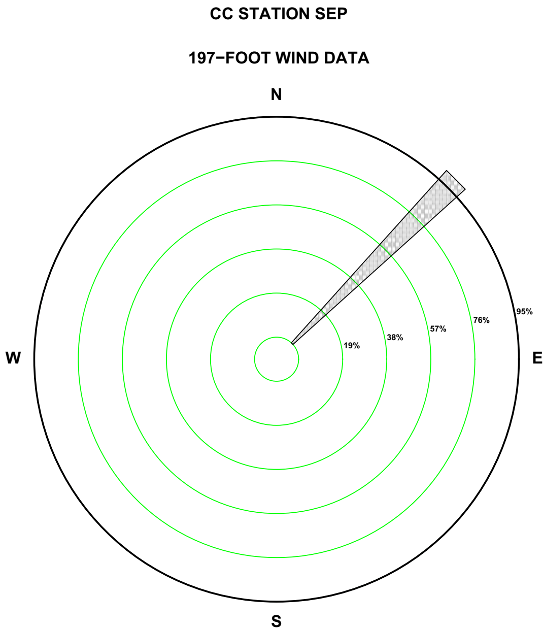
Figure 2.7-155—{CCNPP 197 ft September Precipitation Wind Rose for Rate Class 0.6-0.7 in/hr}
