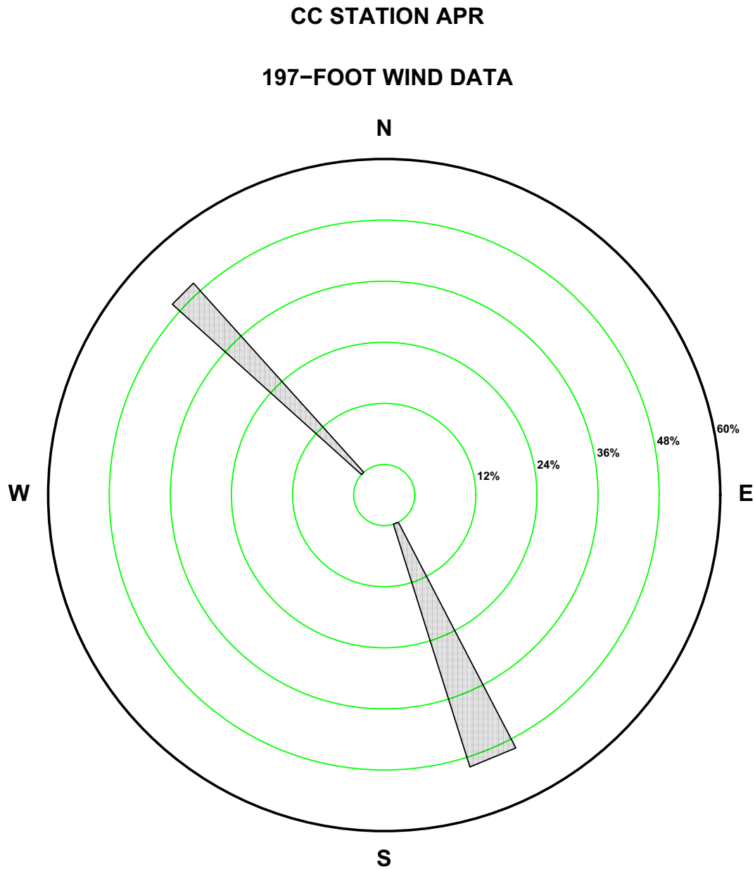
Figure 2.7-118—{CCNPP 197 ft April Precipitation Wind Rose for Rate Class 0.4-0.5 in/hr}
