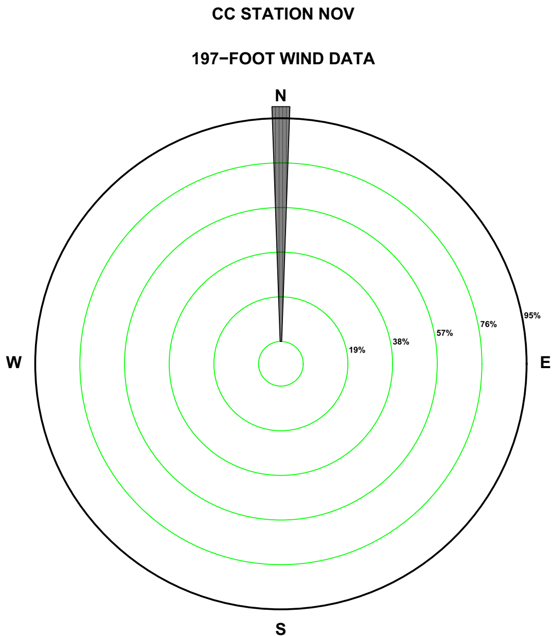
Figure 2.7-167—{CCNPP 197 ft November Precipitation Wind Rose for Rate Class 0.5-0.6 in/hr}
