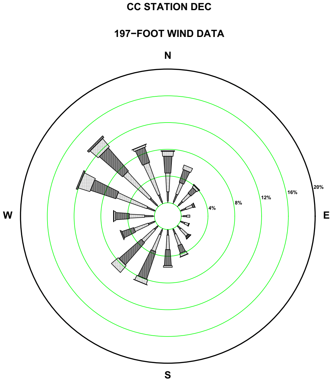
Figure 2.7-198—{CCNPP 197 ft December Wind Rose}
