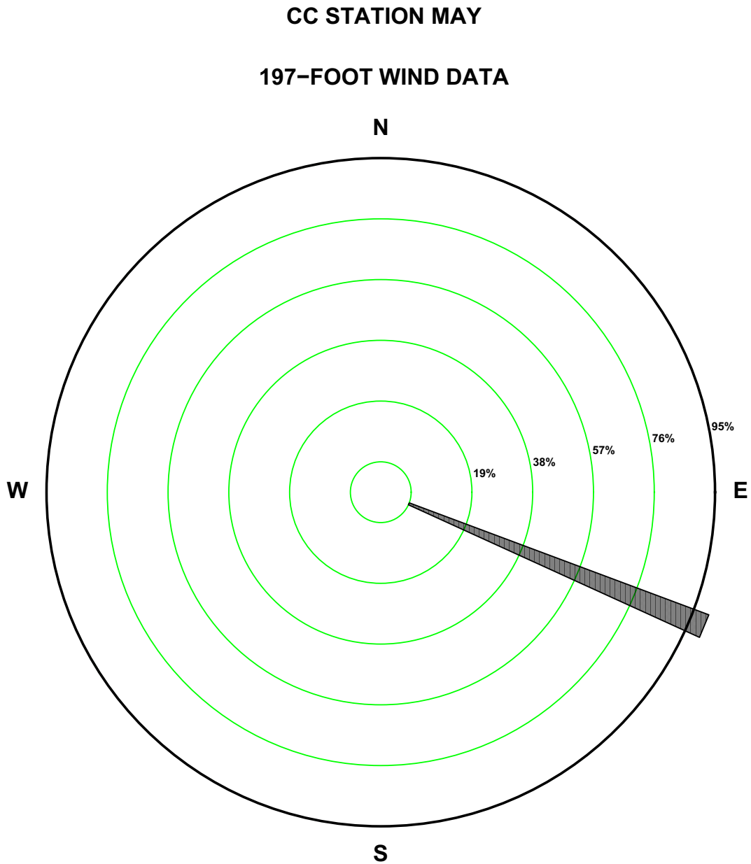
Figure 2.7-126—{CCNPP 197 ft May Precipitation Wind Rose for Rate Class 1.0-2.0 in/hr}
