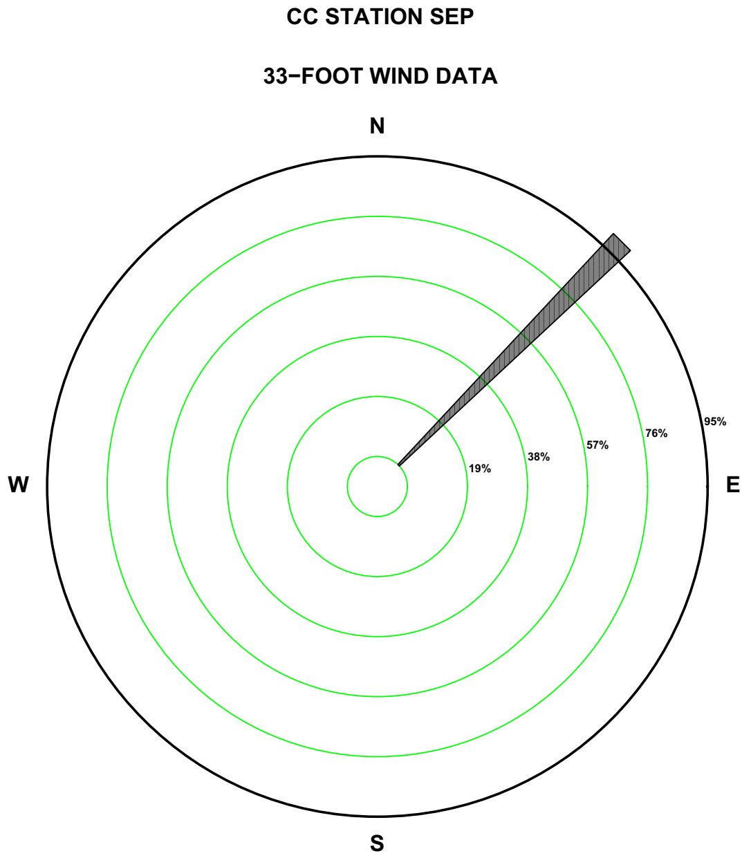
Figure 2.7-84—{CCNPP 33 ft September Precipitation Wind Rose for Rate Class 0.6-0.7 in/hr}
