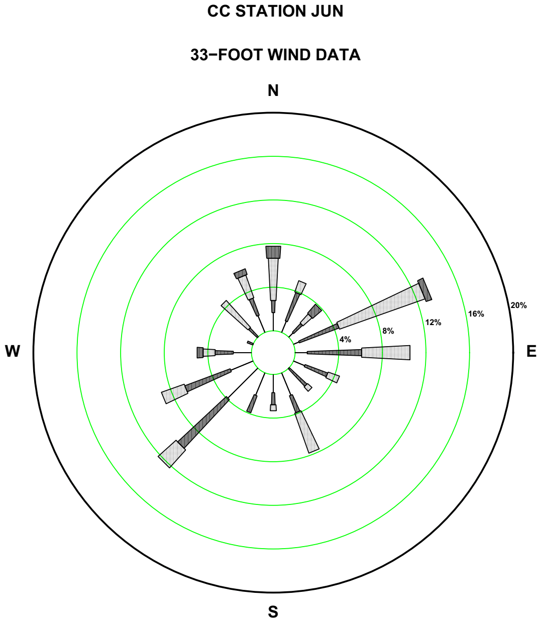
Figure 2.7-11—{CCNPP 33 ft June Precipitation Wind Rose}
