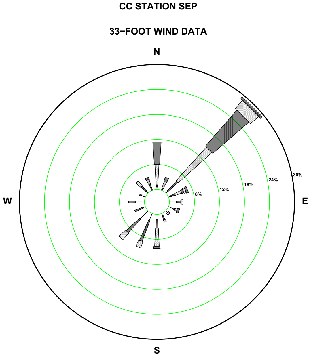
Figure 2.7-14—{CCNPP 33 ft September Precipitation Wind Rose}
