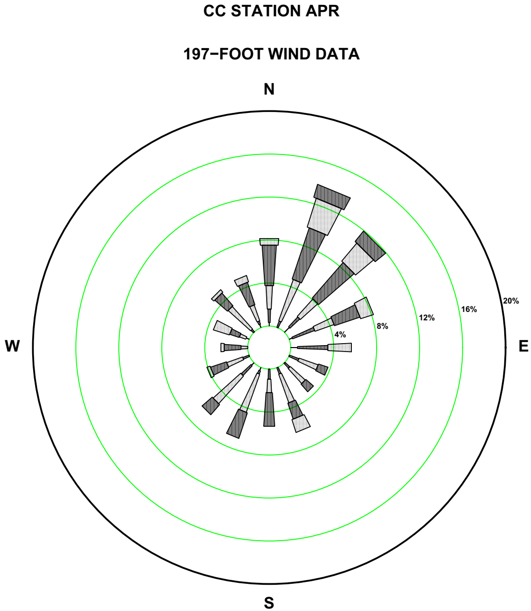
Figure 2.7-21—{CCNPP 197 ft April Precipitation Wind Rose}
