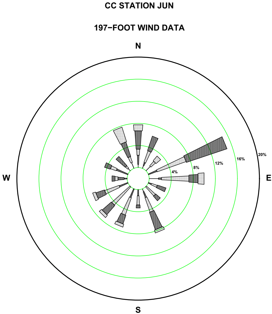
Figure 2.7-23—{CCNPP 197 ft June Precipitation Wind Rose}
