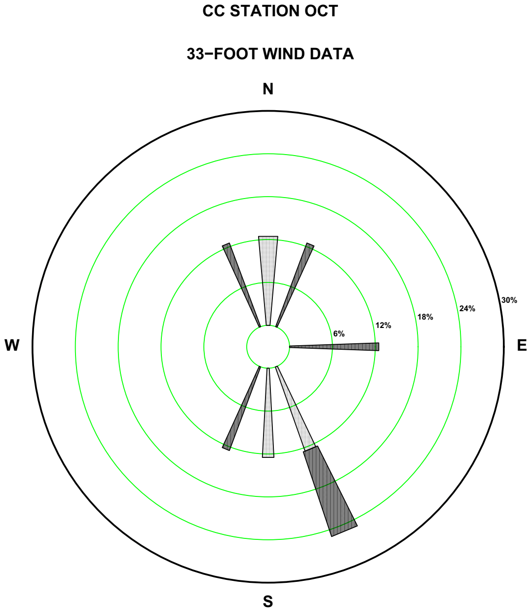
Figure 2.7-88—{CCNPP 33 ft October Precipitation Wind Rose for Rate Class 0.2-0.3 in/hr}
