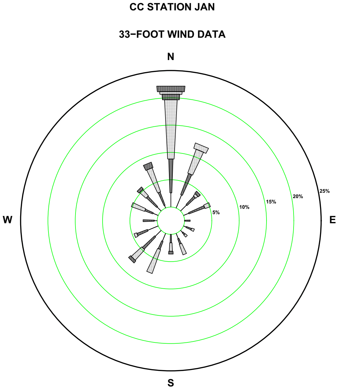
Figure 2.7-6—{CCNPP 33 ft January Precipitation Wind Rose}
