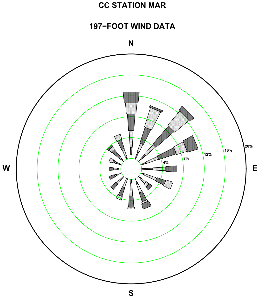
Figure 2.7-20—{CCNPP 197 ft March Precipitation Wind Rose}
