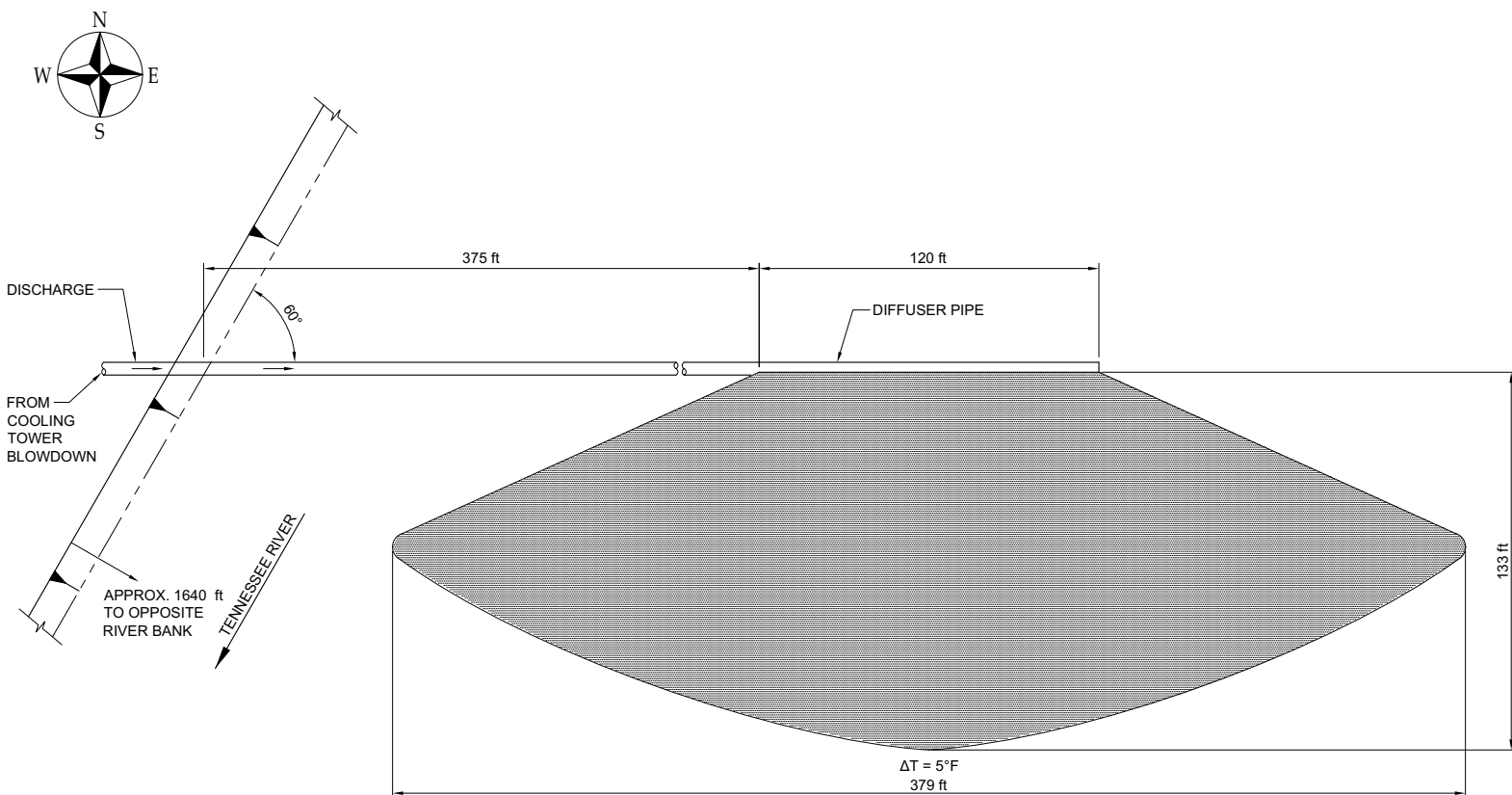
PLAN
