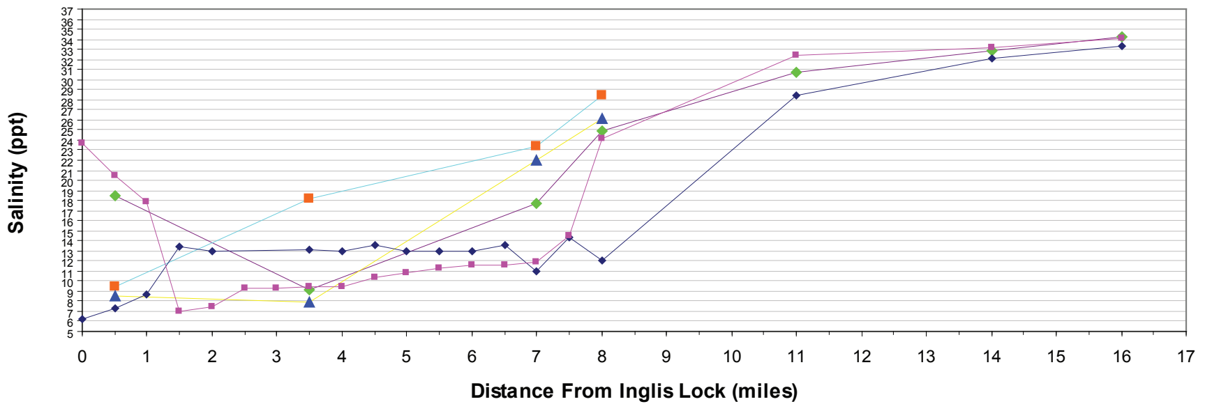
Progress Energy Florida Levy Nuclear Plant Units 1 and 2 Part 3, Environmental Report Salinity Pattern at 0.15 Meter Depth FIGURE 2.4-12 Rev 0
