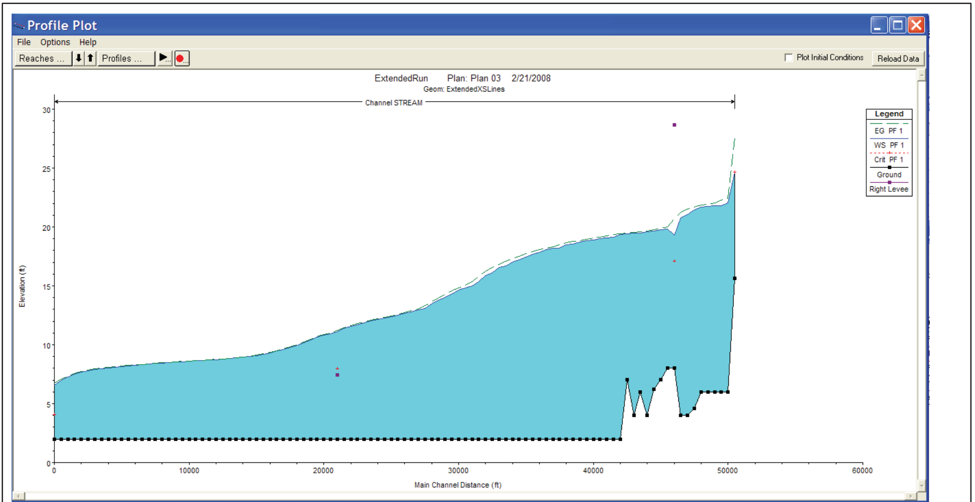
Progress Energy Florida Levy Nuclear Plant Units 1 and 2 Part 2, Final Safety Analysis Report Flood Profile in the Lower Withlacoochee River Watershed FIGURE 2.4.4-203 Rev 0
