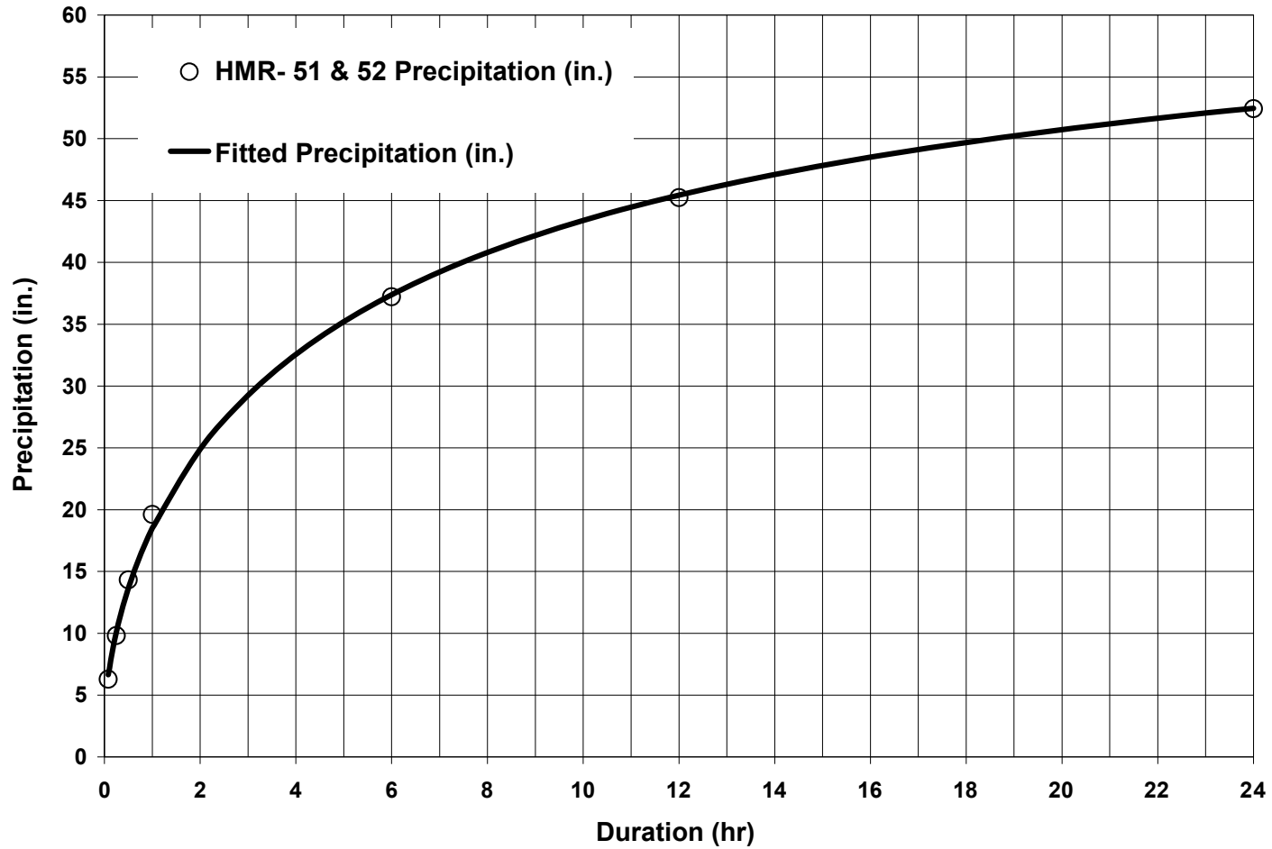
Progress Energy Florida Levy Nuclear Plant Units 1 and 2 Part 2, Final Safety Analysis Report Local Intense Probable Maximum Precipitation Depth-Duration Curve FIGURE 2.4.2-202 Rev 0
