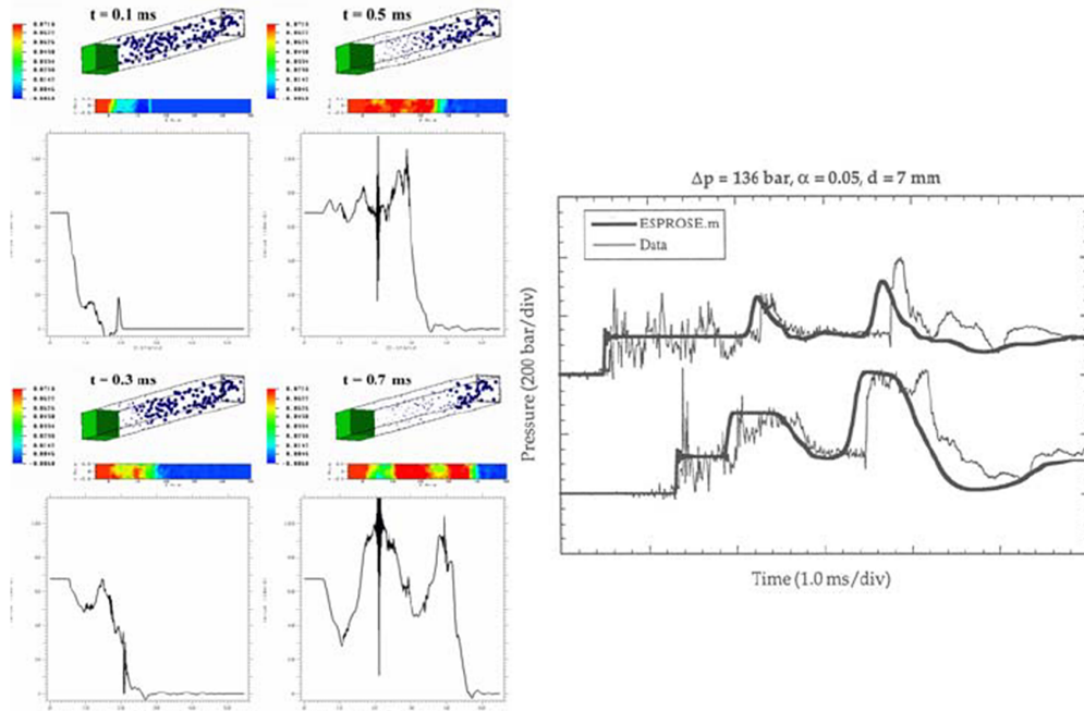
Figure 21C-4. Pressure Transient in a SIGMA Run and ESPROSE.m Simulation Right: Pressure transient measured in a multi-void-region SIGMA run and ESPROSE.m simulation. Left: DNS of this SIGMA run that captures also the pressure fluctuations due to collapsing bubbles.
