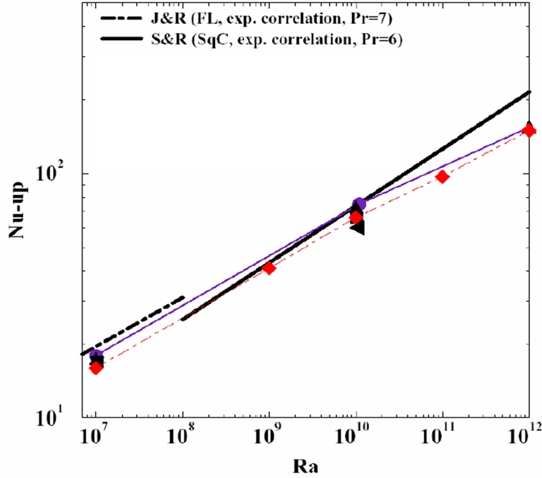
Figure 21D-1. Upward Nusselt Number From an Internally Heated Fluid Layer
