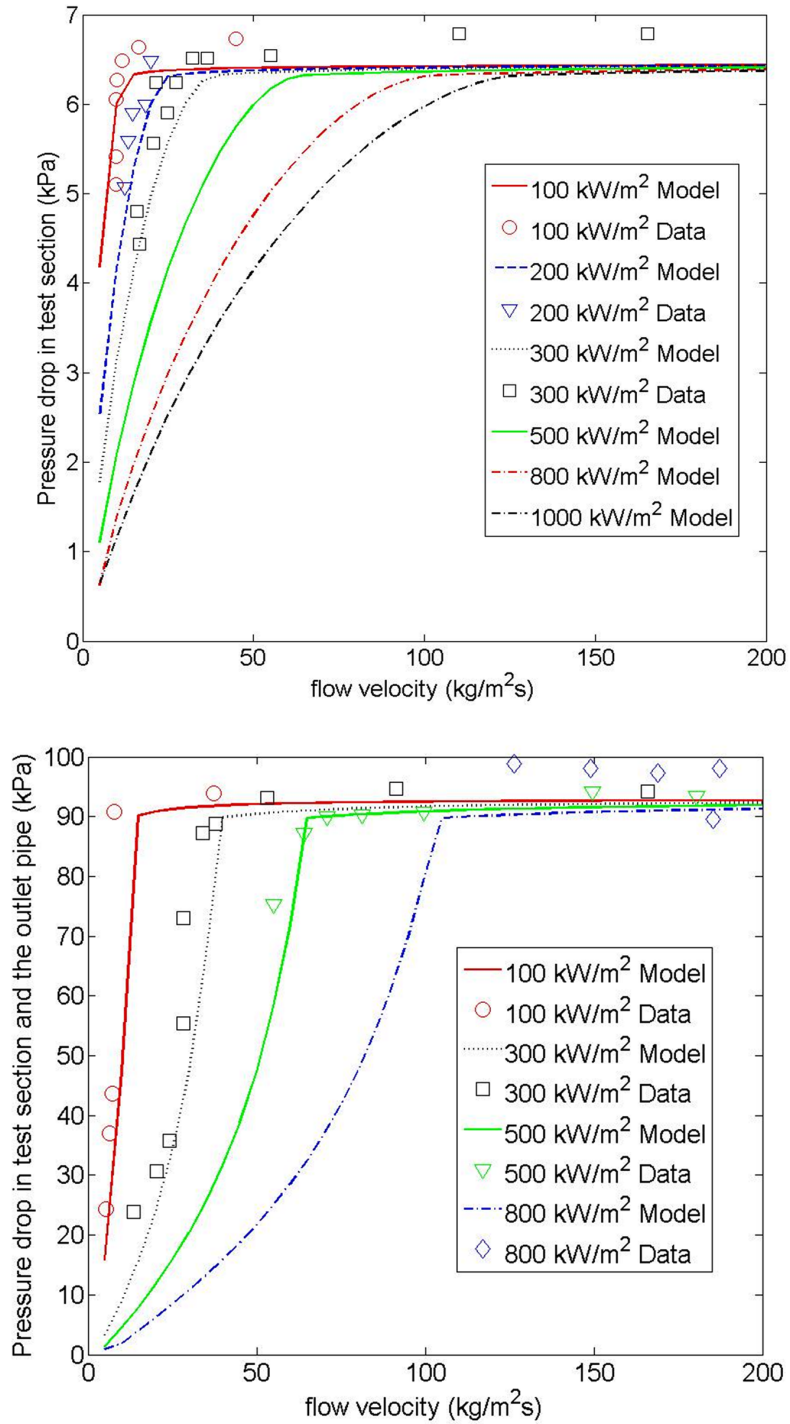
Figure 21E.3-6. Predictions of SULTAN Experiments ( p = 0.5 \text{ MPa} , \theta = 100 , \delta = 0.15 \text{ m} , T_e = 100^\circ\text{C} ). Slip is set at s = 10
