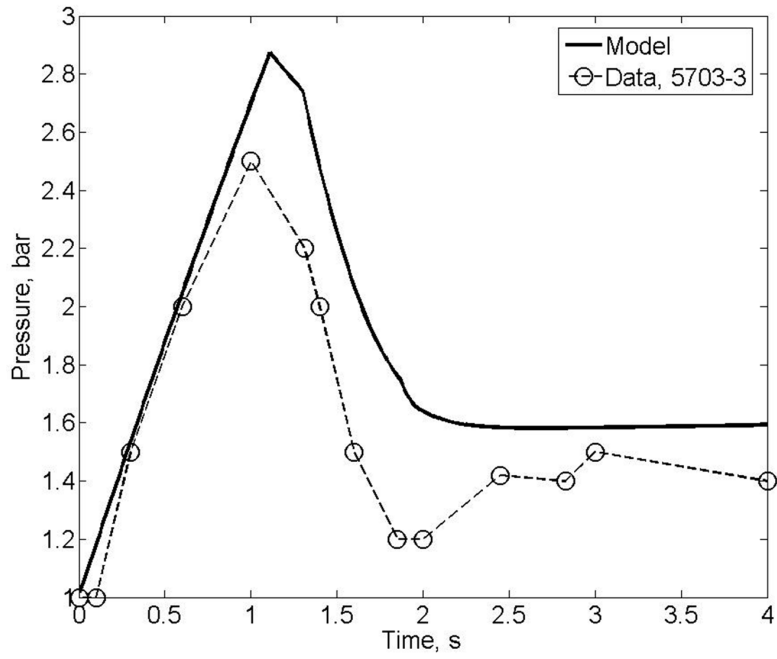
Figure 21B.3-3a. Dywidel Pressure Transient in Test 5703-3
