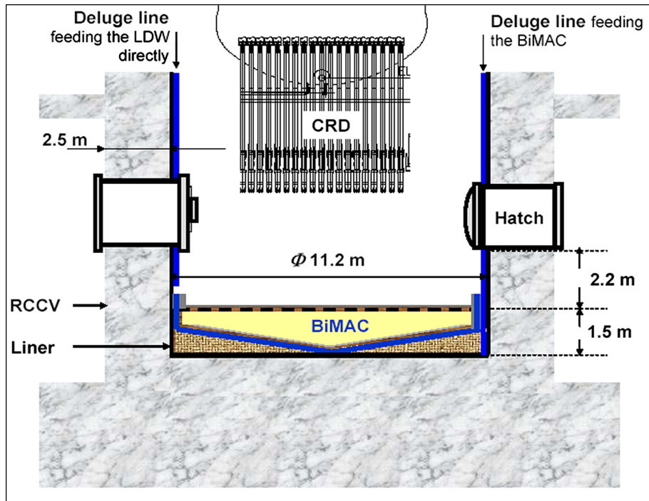
Figure 21.4.2-1 The Overall Ldw Geometry Relevant to EVEs
