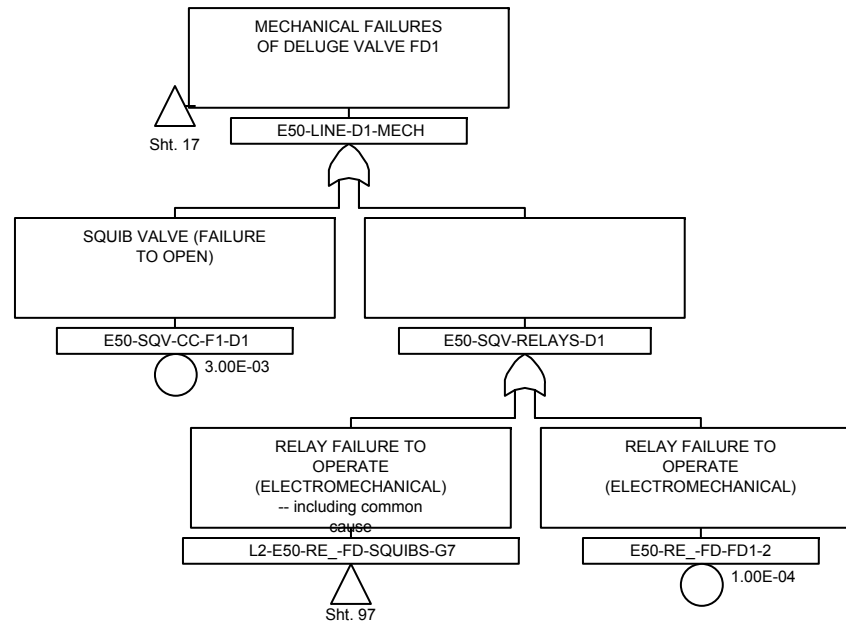
Figure 8A-8. Level 2 Fault Trees Sheet 96 of 147
