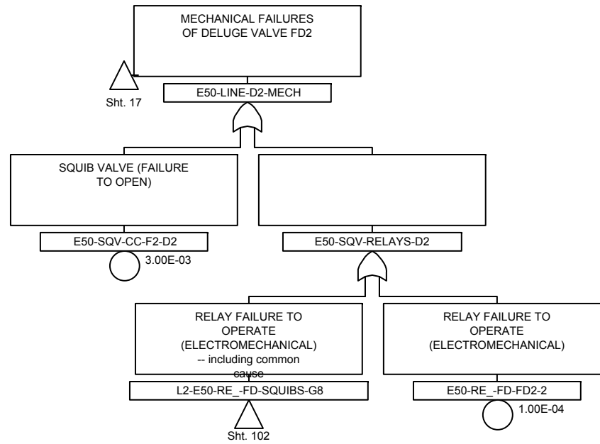
Figure 8A-8. Level 2 Fault Trees Sheet 101 of 147
