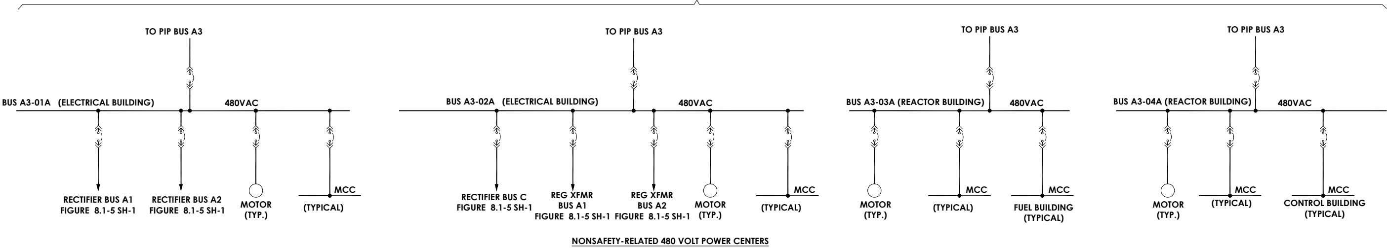
NONSAFETY-RELATED 480 VOLT POWER CENTERS
