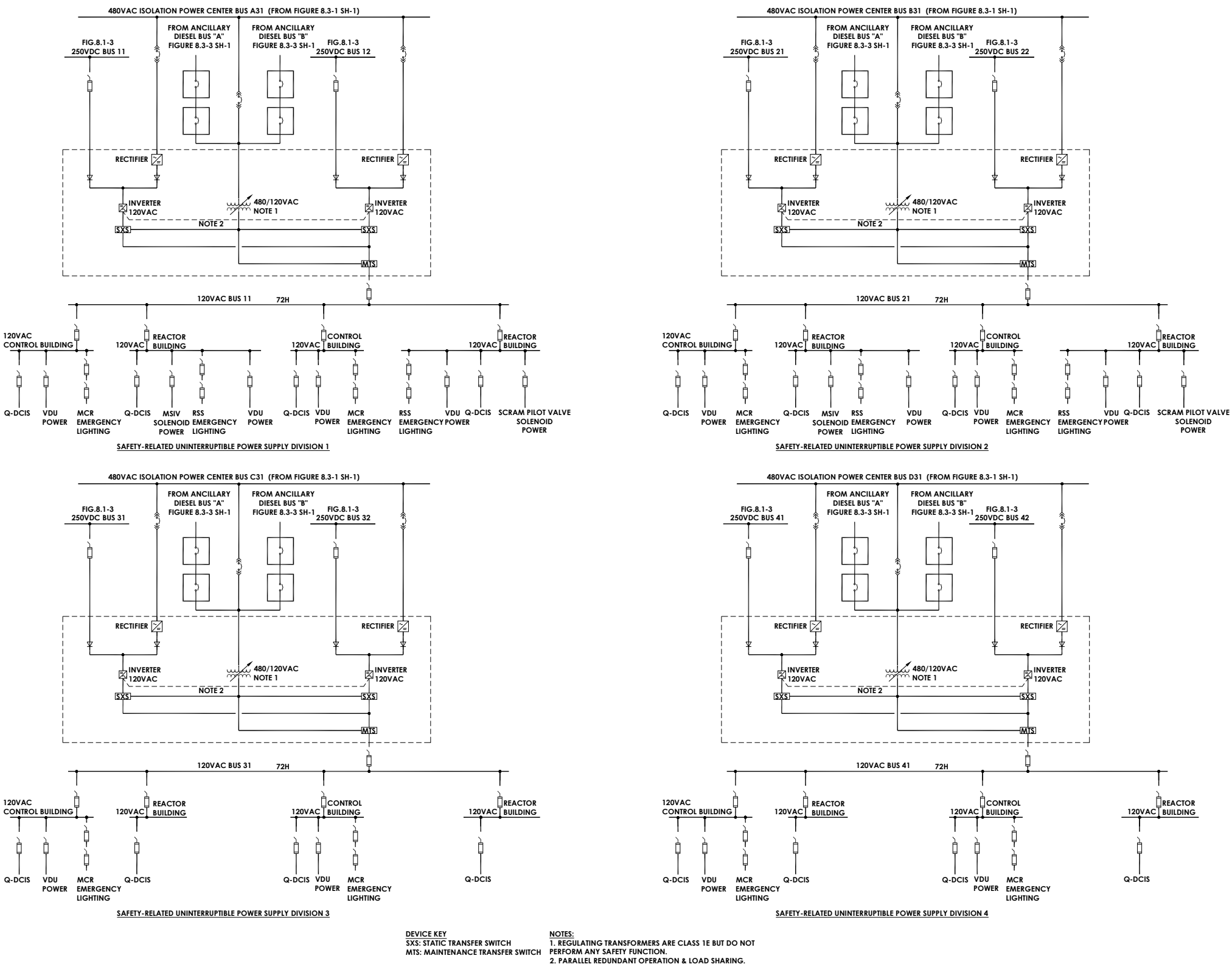
Figure 8.1-4. Uninterruptible AC Power Supply (Safety-Related)
