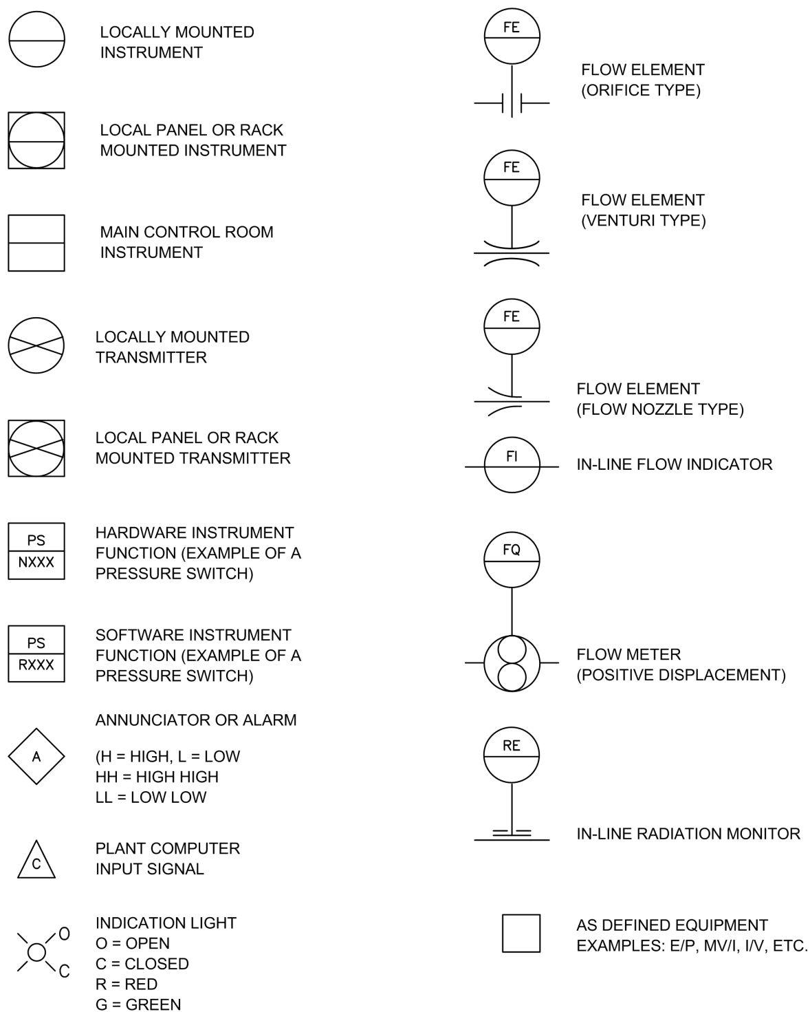
Figure 1.7-2. P&amp;ID Symbols for Instruments
