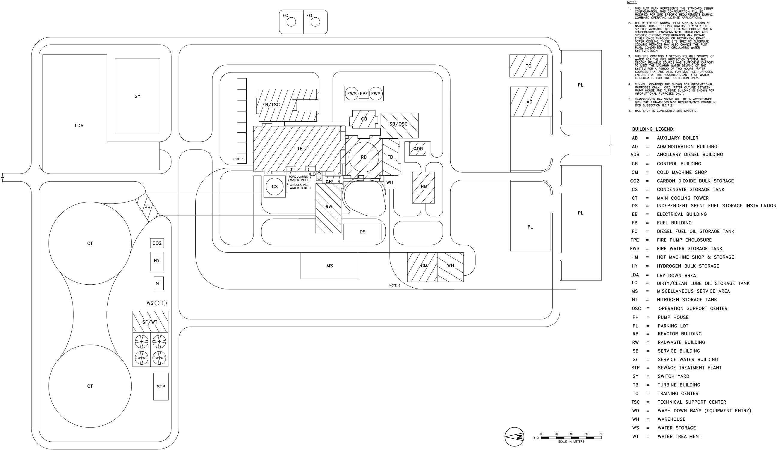
Figure 1.1-1. ESBWR Standard Plant General Site Plan
