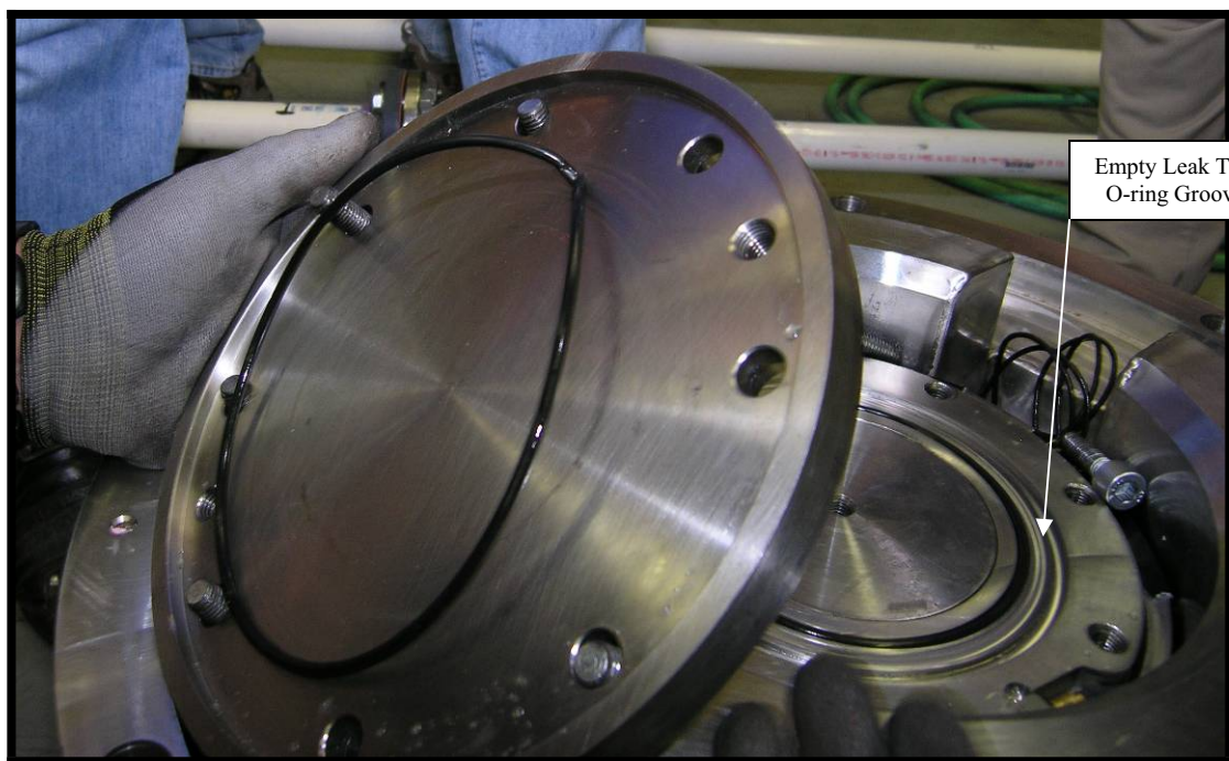
Photograph 53 – Test 1C Post-Drop Inspection (View 6)
