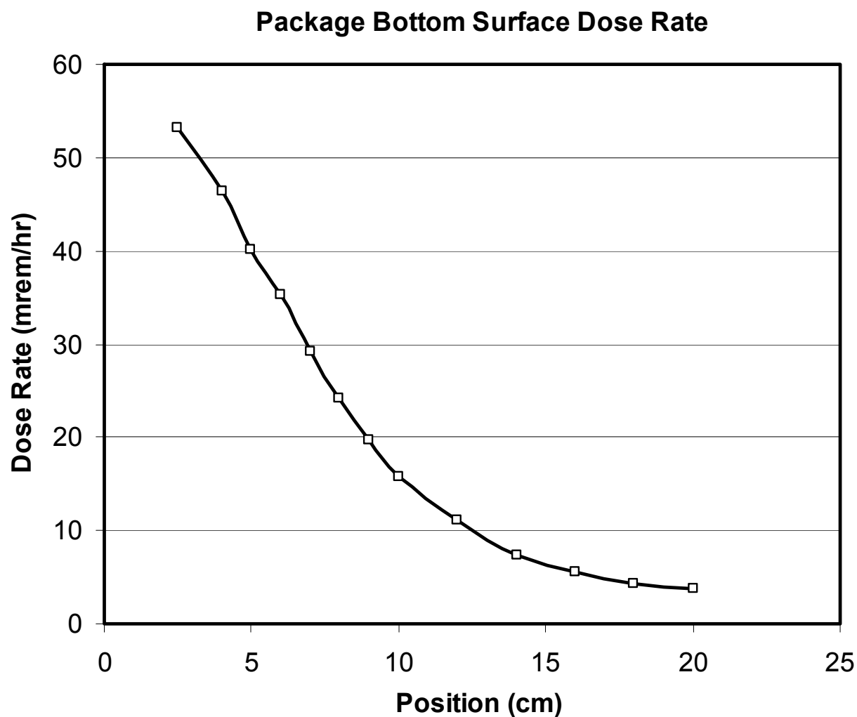
Figure 5-16 – Bottom-Surface Dose Rate Profile
