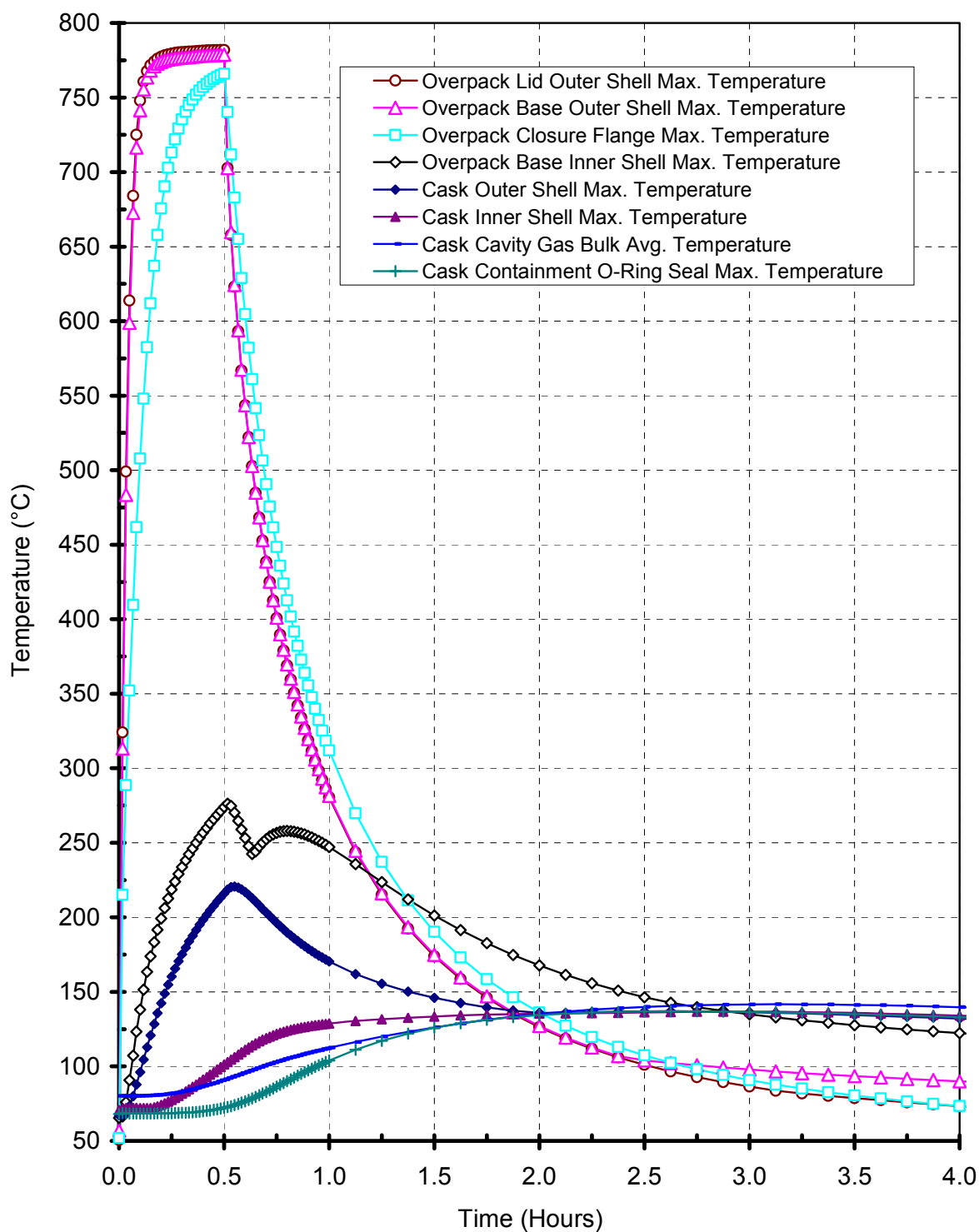
Figure 3-10 – Package Temperatures for HAC Thermal Test with Bottom End Damage
