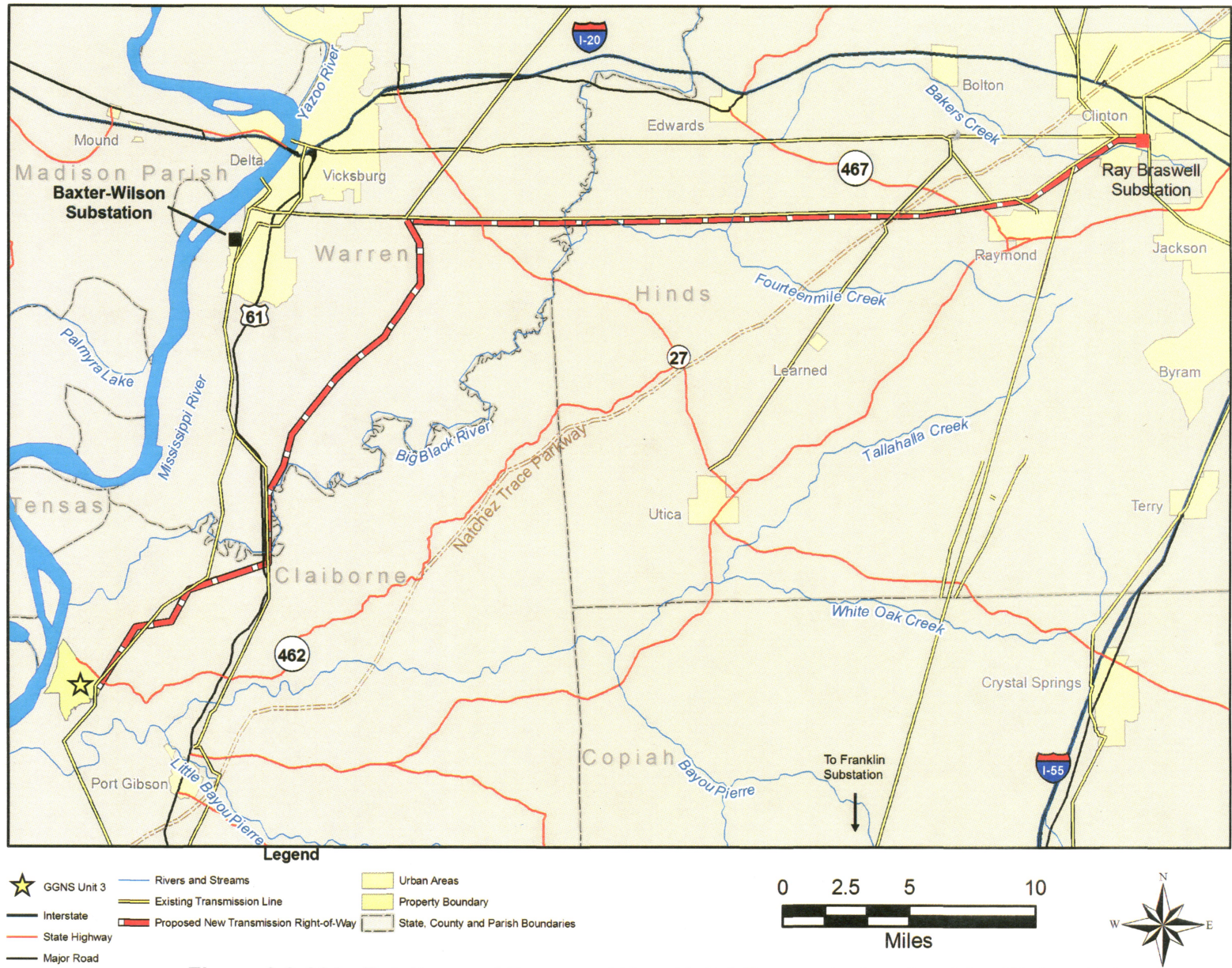
Figure 2.2-201. Existing and Proposed New Unit 3 Transmission Corridor Right of Way
