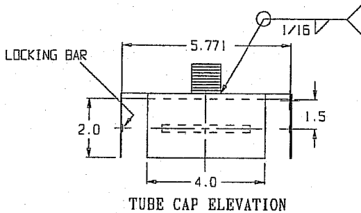
TUBE CAP ELEVATION
