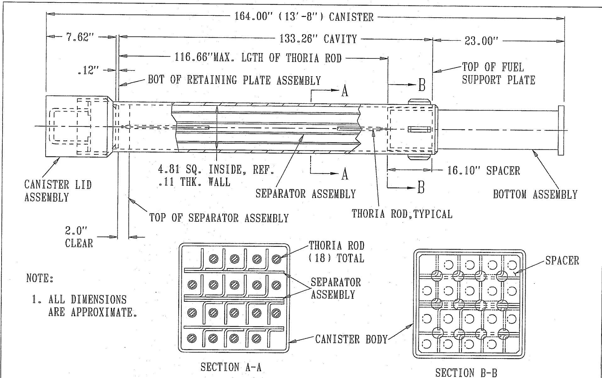
FIGURE 2.1.2A; TN THORIA ROD CANISTER FOR DRESDEN UNIT-1
