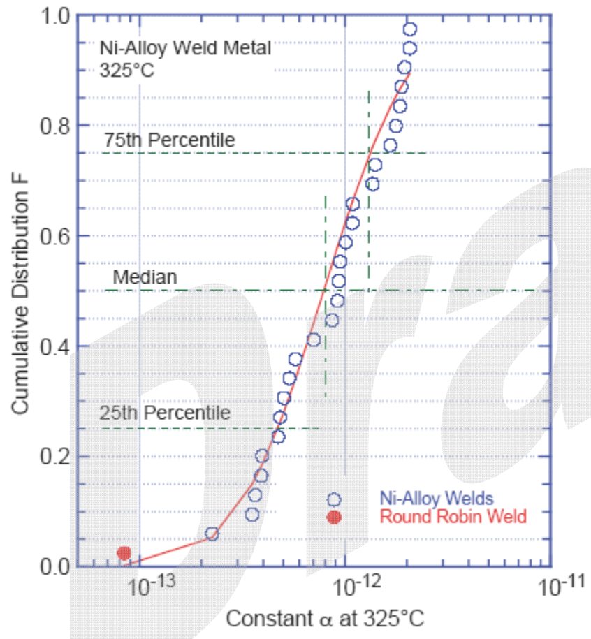
Figure 109. Log-normal distribution of constant \alpha for several heats of Alloy 82 and 182.
