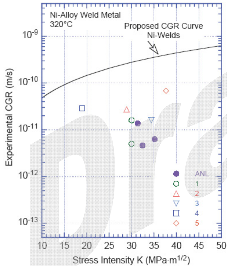
Figure 108. SCC CGR data for round-robin Alloy 182 weld alloy in PWR environment.
