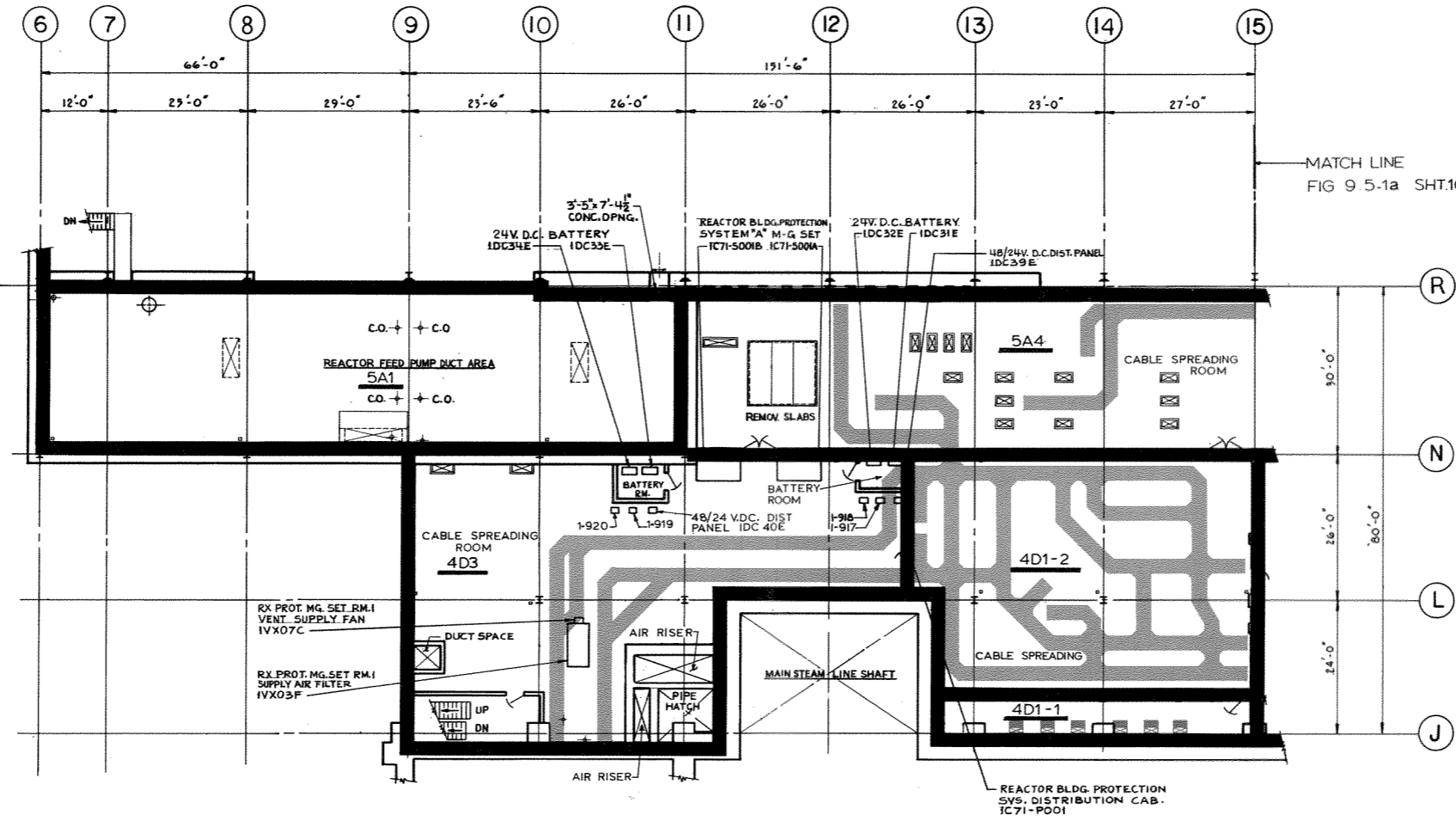
FLOOR PLAN ELEV. 749'-0"
