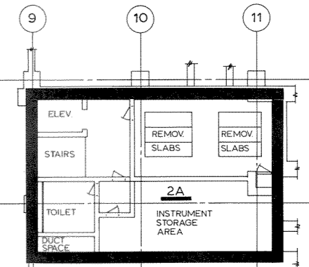
PARTIAL FLOOR PLAN EL. 832'-0"
