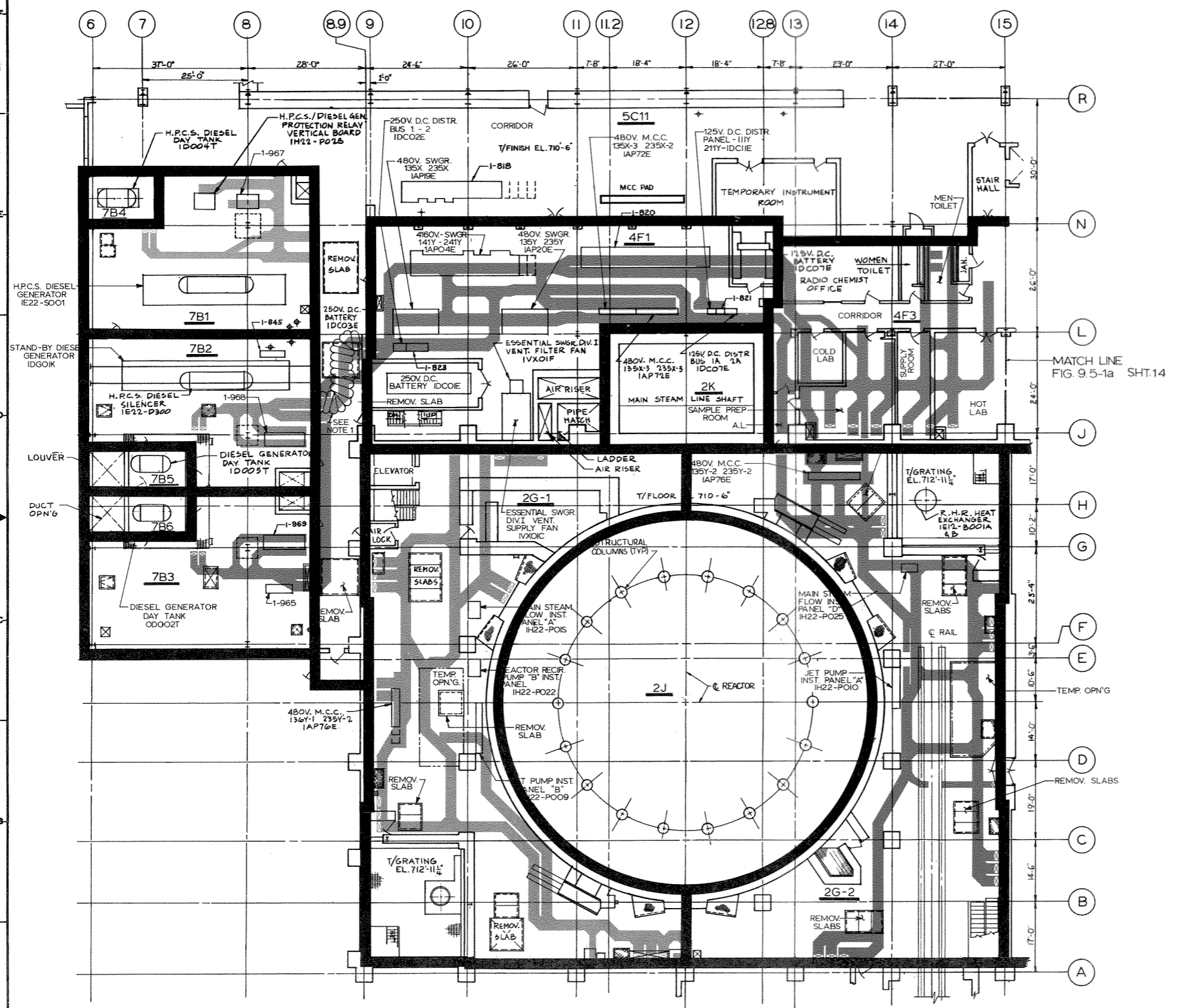
GROUND FLOOR PLAN EL. 710'-6"
