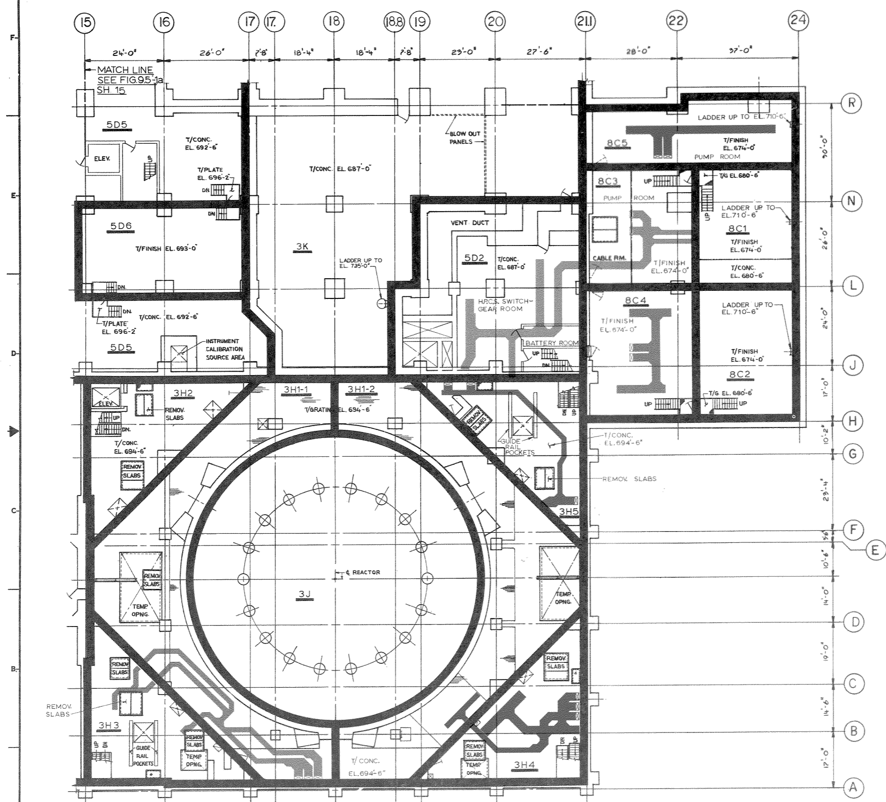
UPPER BASEMENT FLOOR PLAN EL. 687'-0"
