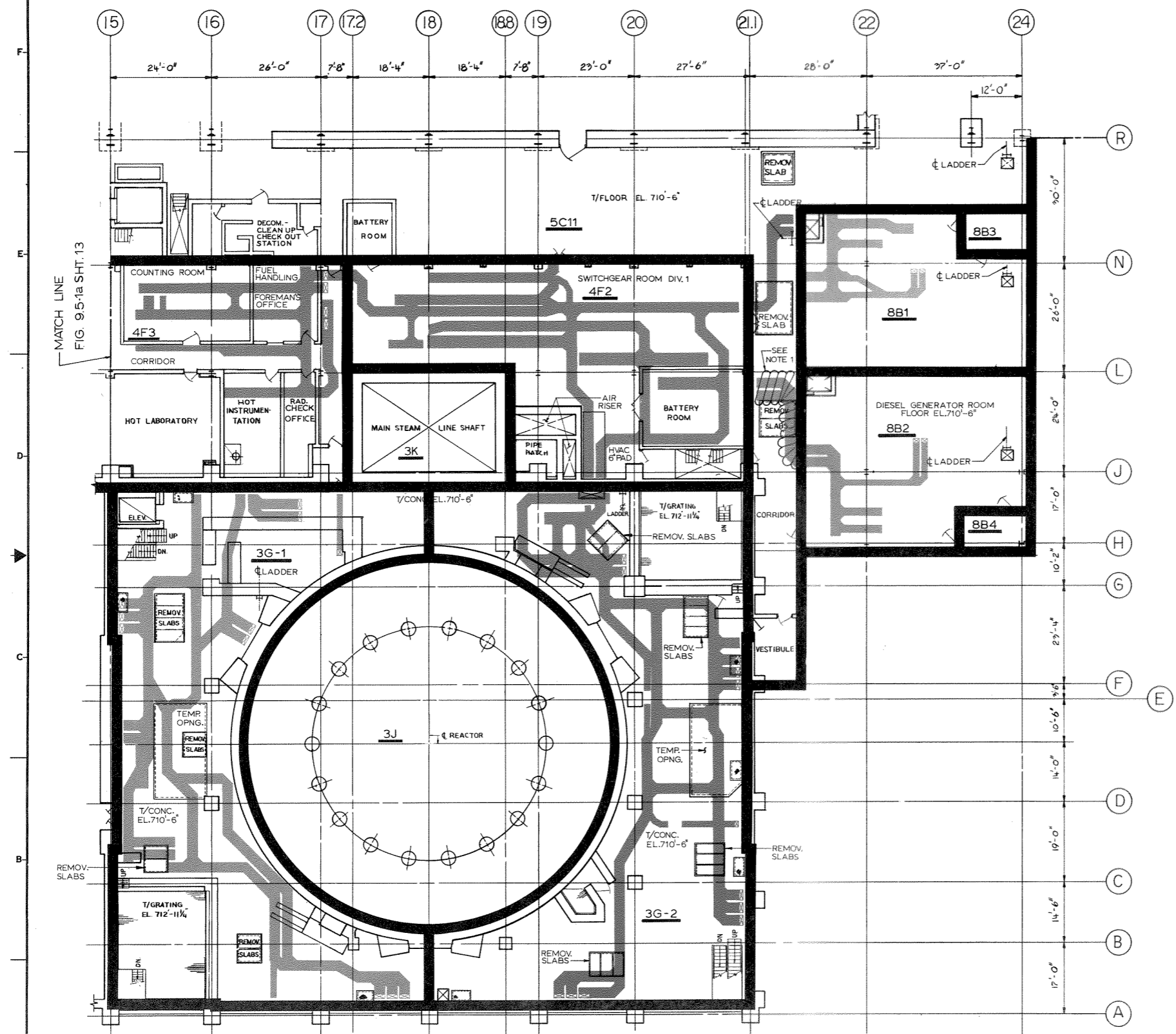
GROUND FLOOR PLAN EL. 710'-6"
