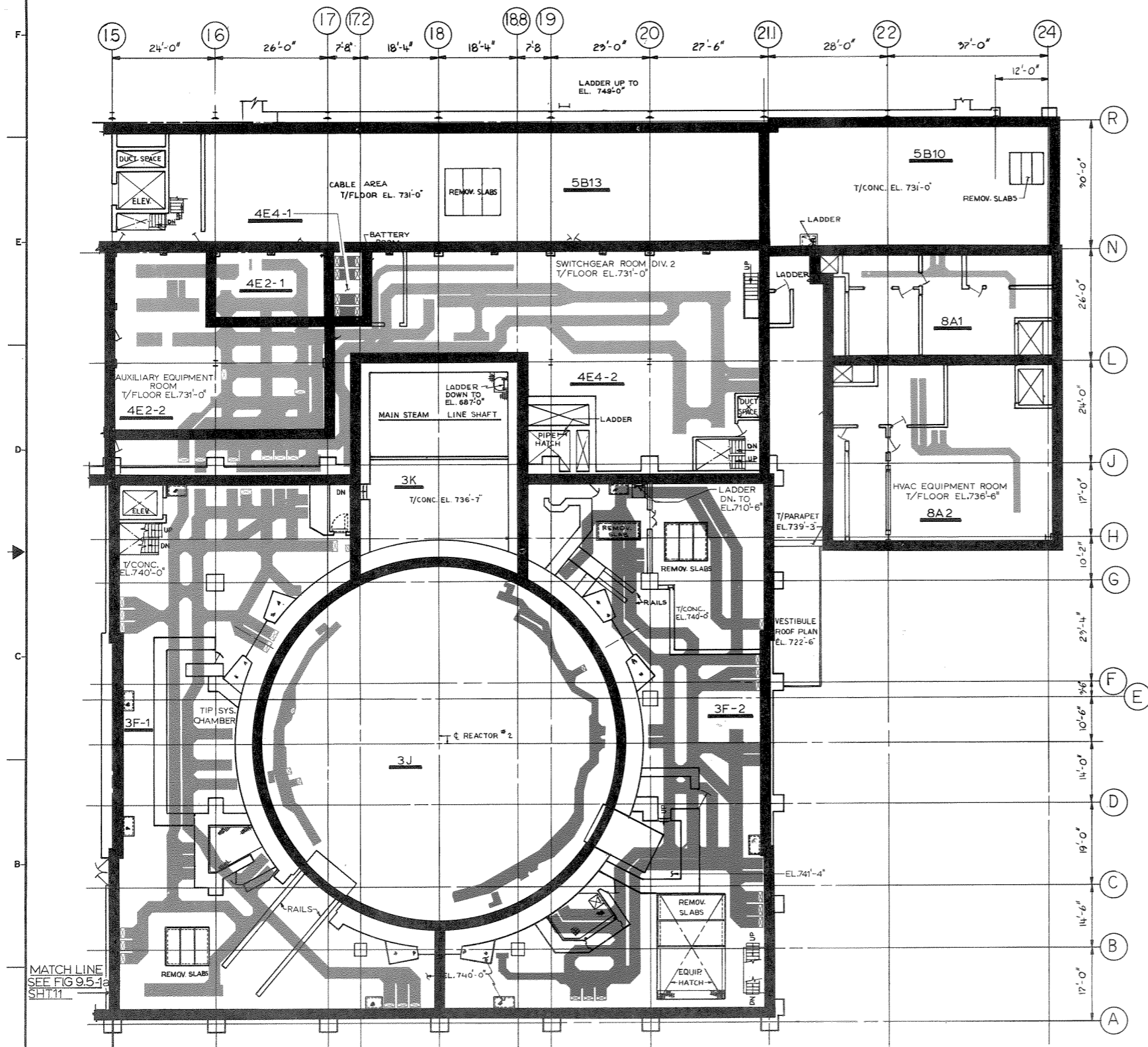
MEZZ. FLOOR PLAN EL. 740'-0"
