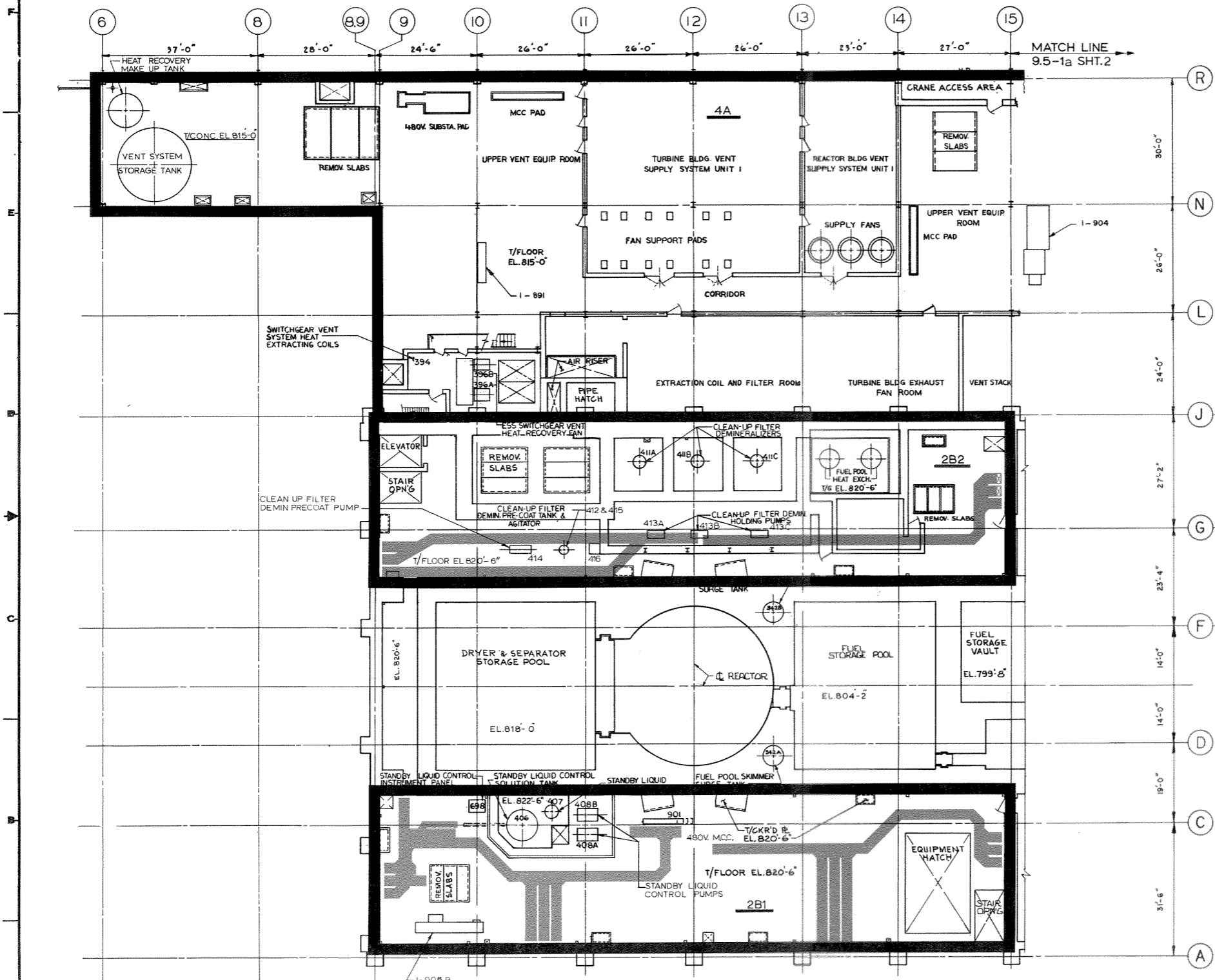
FLOOR PLAN EL. 820'-6"
