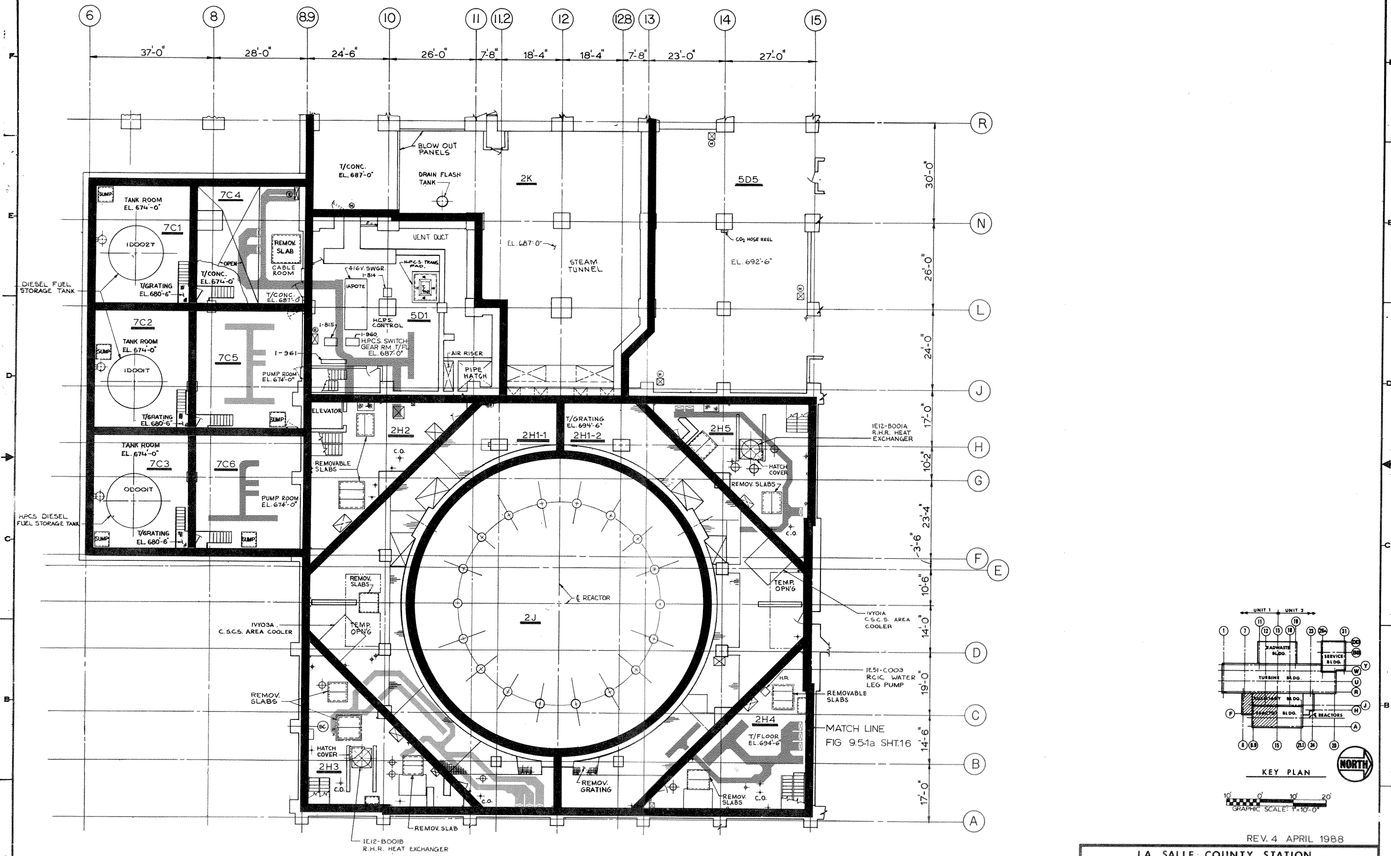
UPPER BASEMENT FLOOR PLAN EL. 687'-0"
