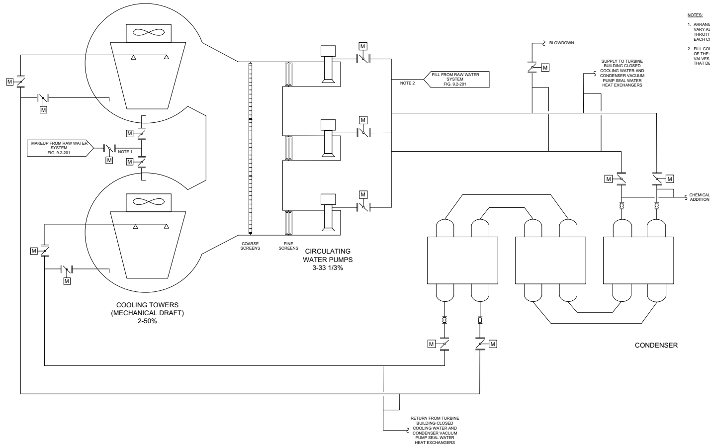
Figure 10.4-201 Circulating Water System Flow Diagram
