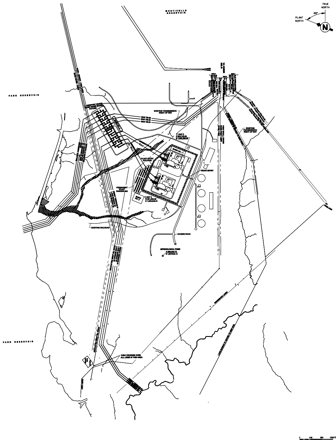
Figure 8.2-201 Site Transmission Line Map
