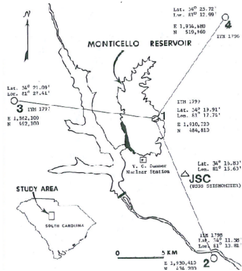
Figure 2.5.2-201. SCE&G 4-Station Microseismic Network and location of Jenkinsville Station (from Whorton 1988, Reference 295 )
