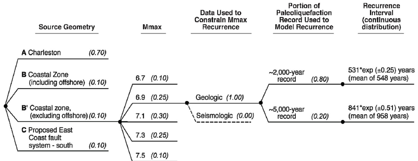
Figure 2.5.2-214. UCSS Logic Tree With Weights For Each Branch
