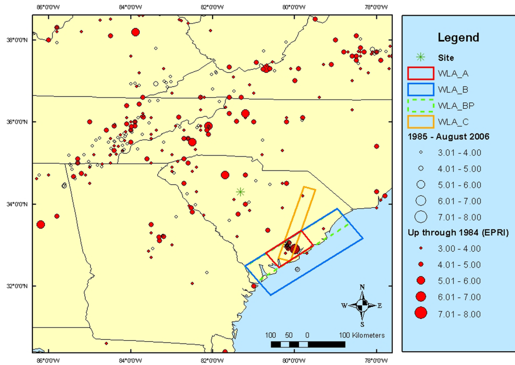
Figure 2.5.2-223. Geometry of Four Sources Used in UCSS Model
