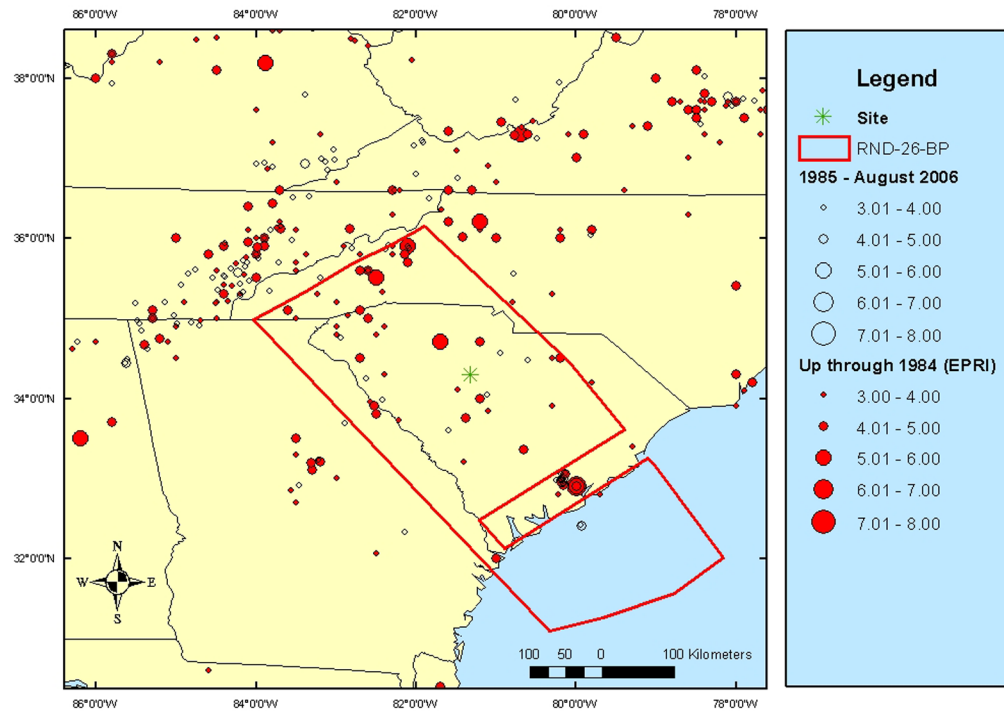
Figure 2.5.2-226. Geometry of Revised Rondout Source RND-26-BP
