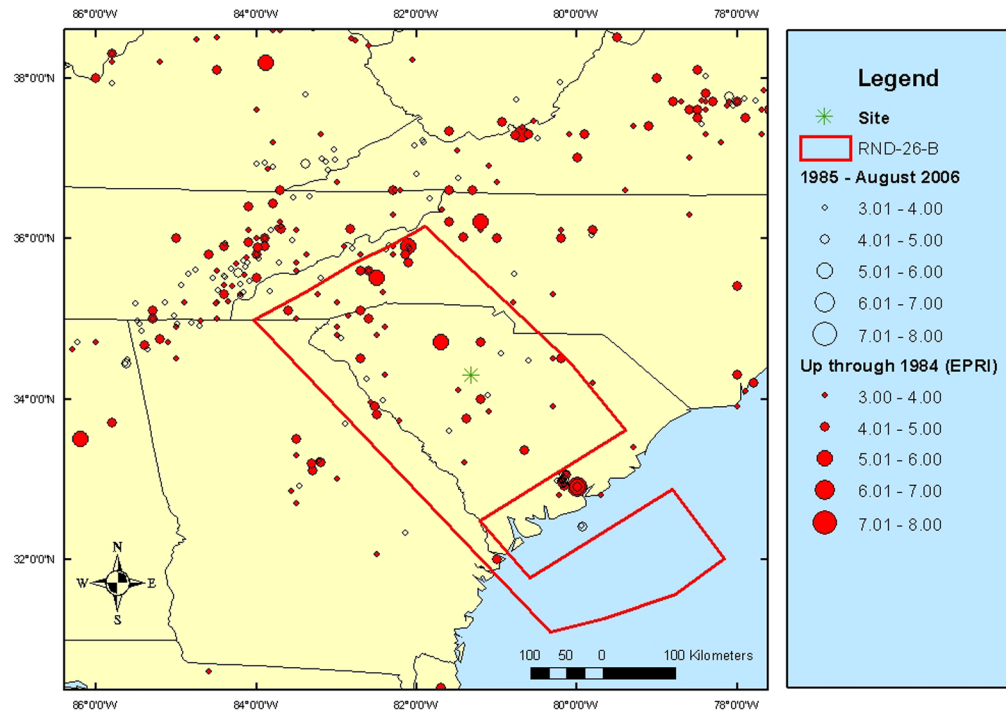
Figure 2.5.2-225. Geometry of Revised Rondout Source RND-26-B
