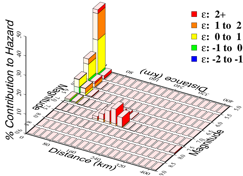
Figure 2.5.2-239. M and R Deaggregation for 5 and 10 Hz at 10 -5 Annual Frequency of Exceedance
