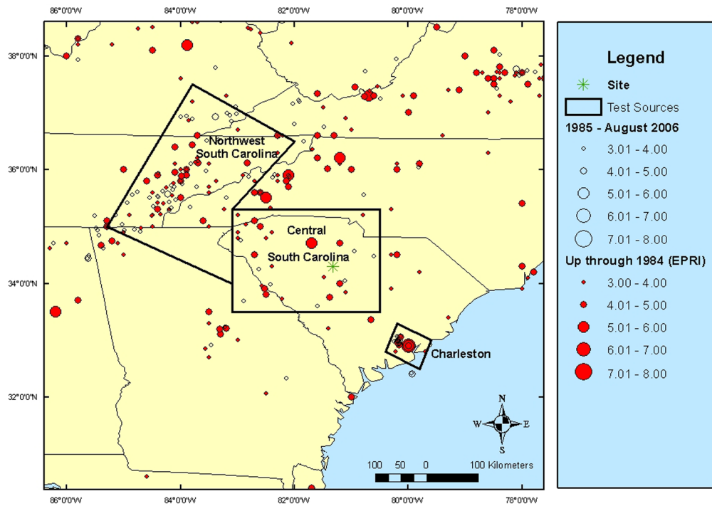
Figure 2.5.2-219. Historical Seismicity in the Region of Units 2 and 3 Site and Three Areas Used to Test the Effects of Additional Seismicity
