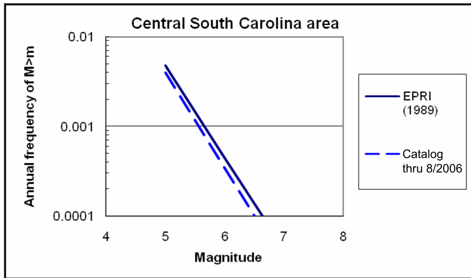
Figure 2.5.2-220. Earthquake Occurrence Rates for EPRI (1989) Catalog and for Catalog Extended through August 2006 for Central South Carolina Area
