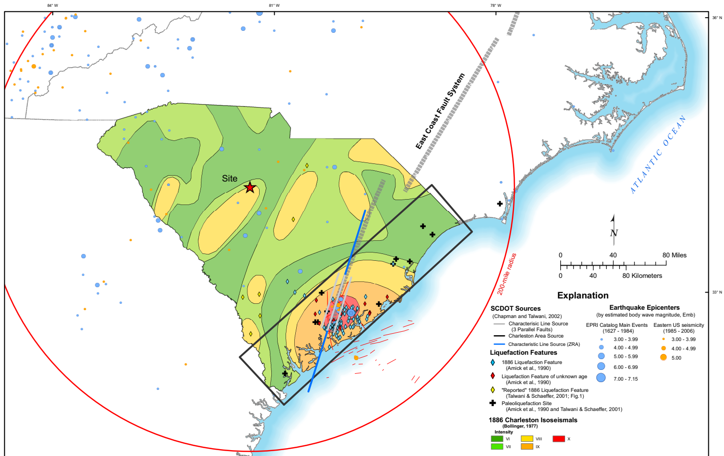
Figure 2.5.2-211. SCDOT Charleston Model
