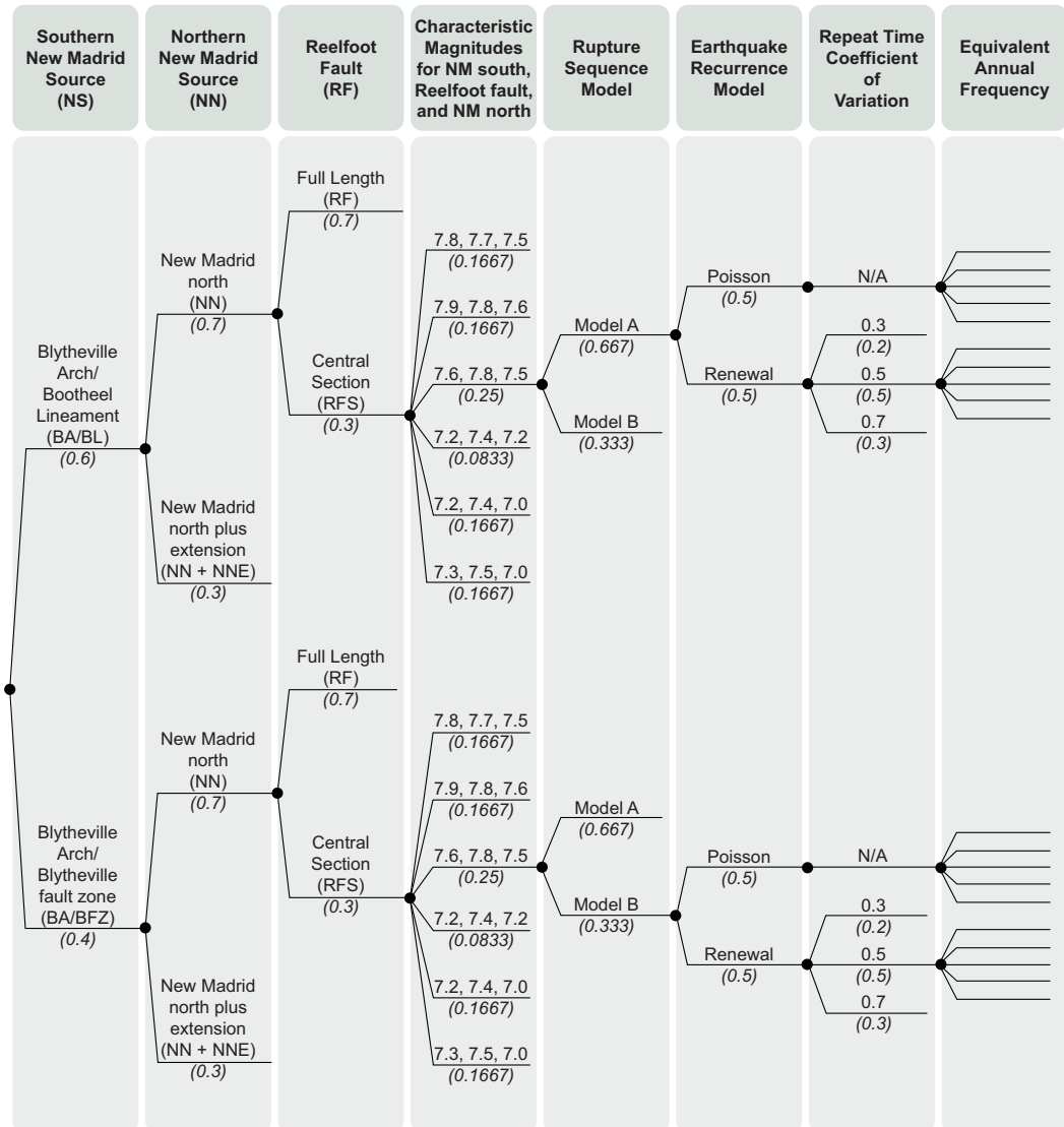
Figure 2.5.2-218. New Madrid Logic Tree From the Clinton ESP Source Model
