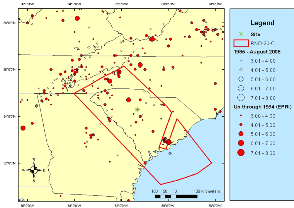
Figure 2.5.2-227. Geometry of Revised Rondout Source RND-26-C
