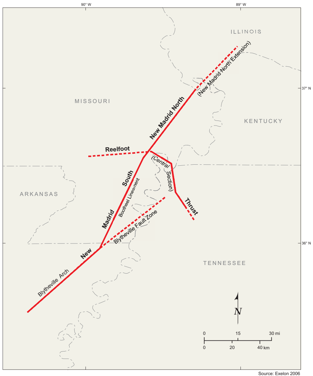
Figure 2.5.2-217. New Madrid Faults from Clinton ESP Source Model Source: Reference 238
