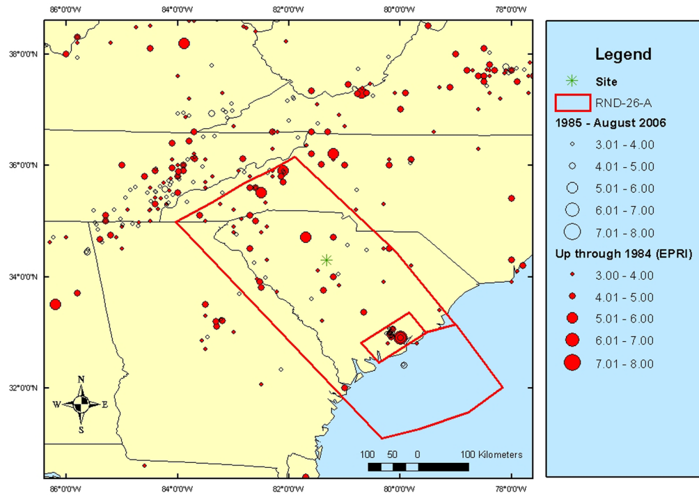
Figure 2.5.2-224. Geometry of Revised Rondout Source RND-26-A
