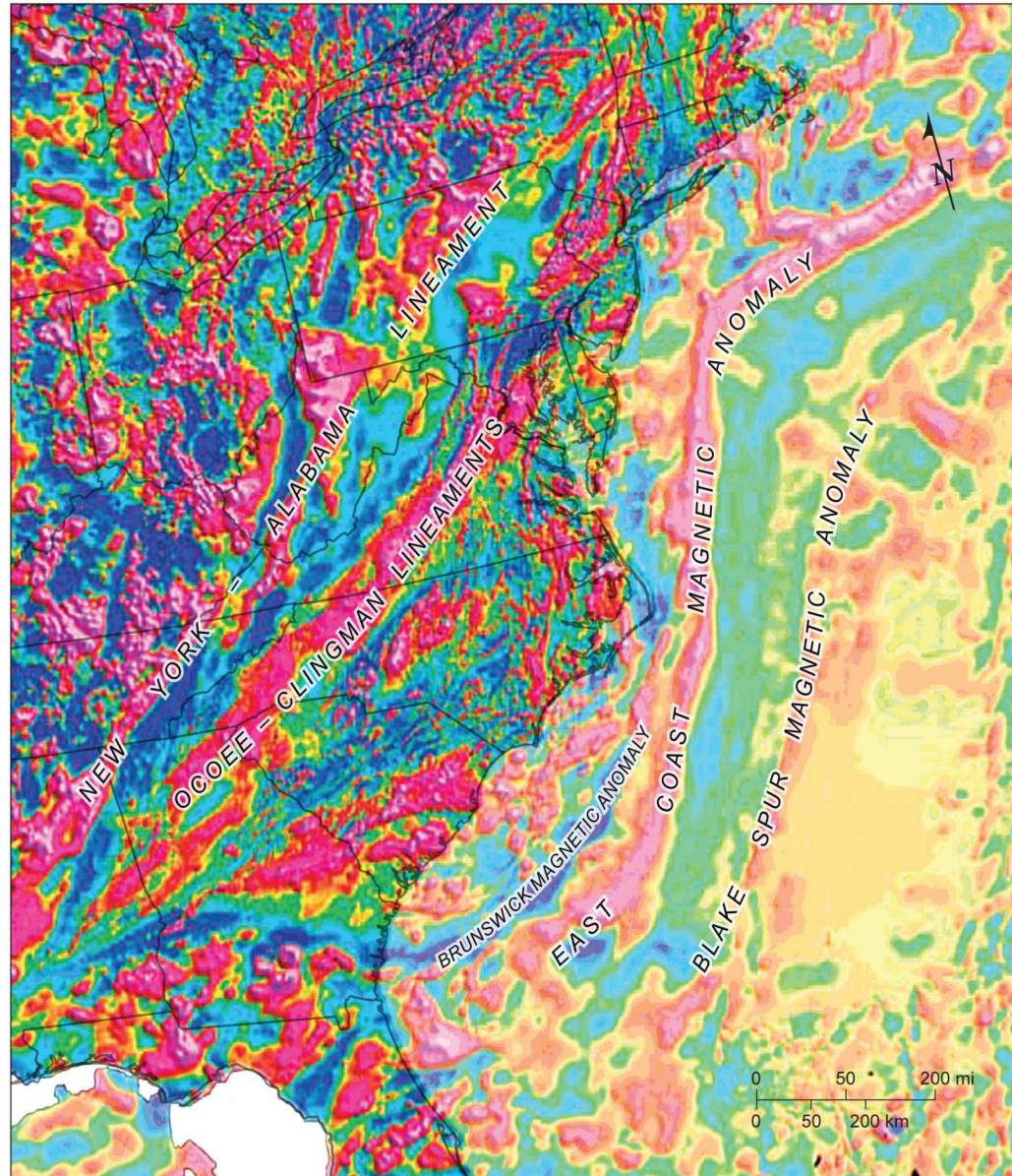
Figure 2.5.1-210. Major Eastern U.S. Aeromagnetic Anomalies
