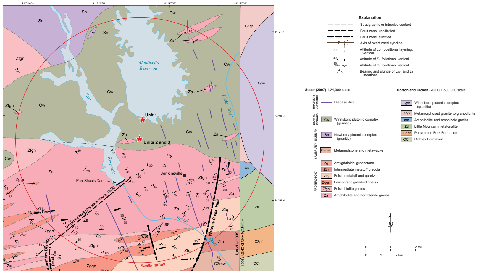
Figure 2.5.1-224. Site Area Geologic Map
