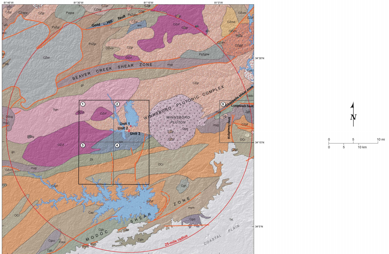
Figure 2.5.1-220. Site Vicinity Geologic Map (Sheet 1 of 2)
