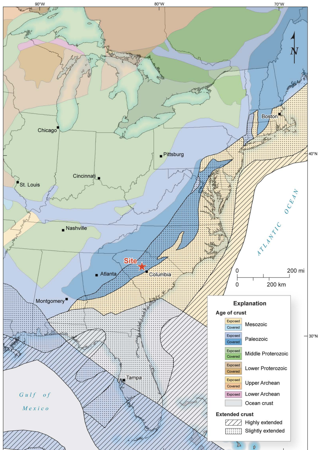
Figure 2.5.1-214. Crustal Ages from Johnston et al. (1994)
