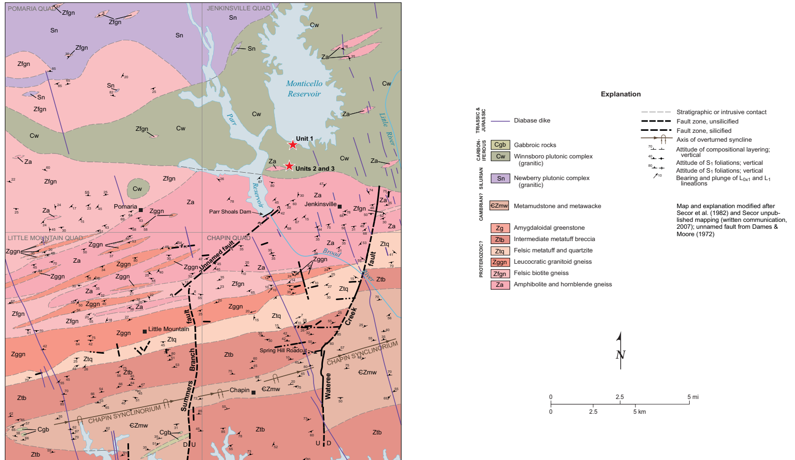
Figure 2.5.1-225. Geologic Map of the Jenkinsvile, Pomaria, Little Mountain and Chapin 7.5-Minute Quadrangles
