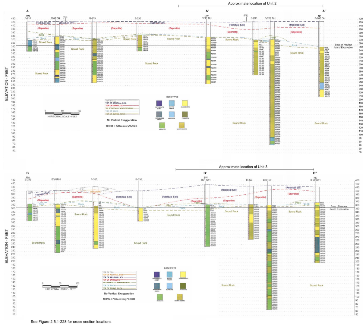
Figure 2.5.1-227. Geologic Cross Sections A-A' and B-B'
