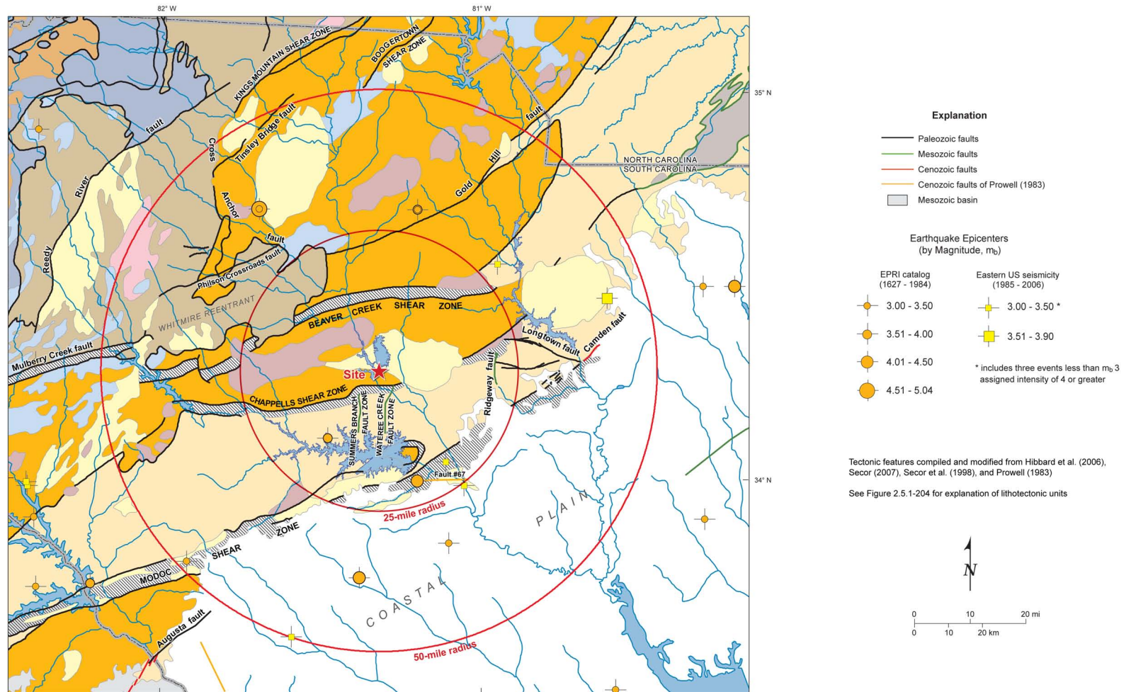
Figure 2.5.1-212. 50-Mile Tectonic Features Map
