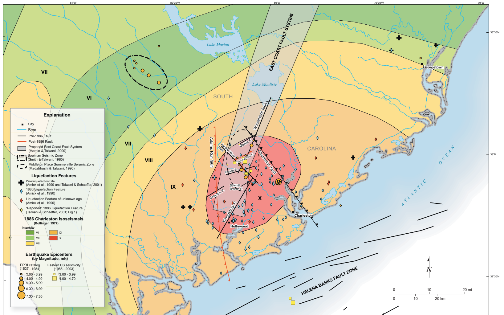
Figure 2.5.1-218. Local Charleston Tectonic Features
