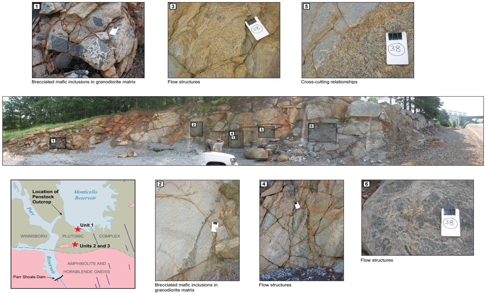
Figure 2.5.1-229. Photographs of Fairfield Pumped Storage Facility Penstock Outcrop
