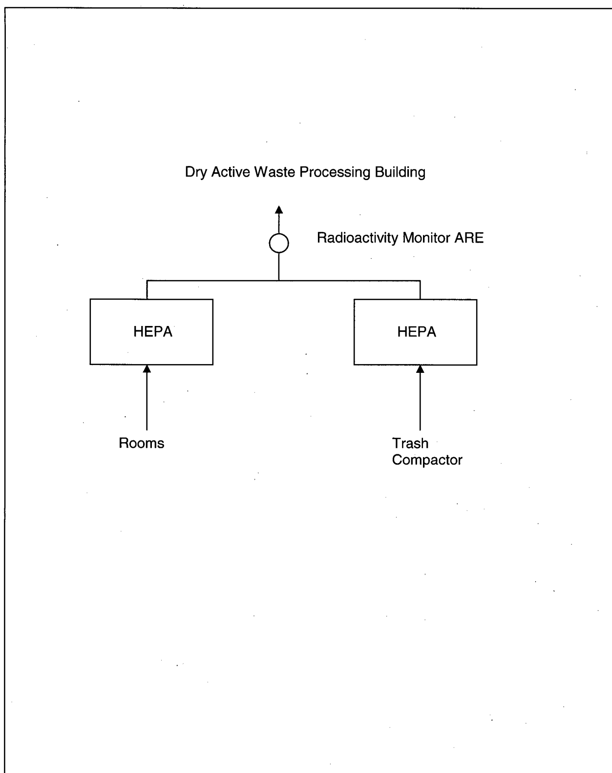
Figure 3-5. Schematic Diagram of the Dry Active Waste Processing Building Ventilation Release Pathway
