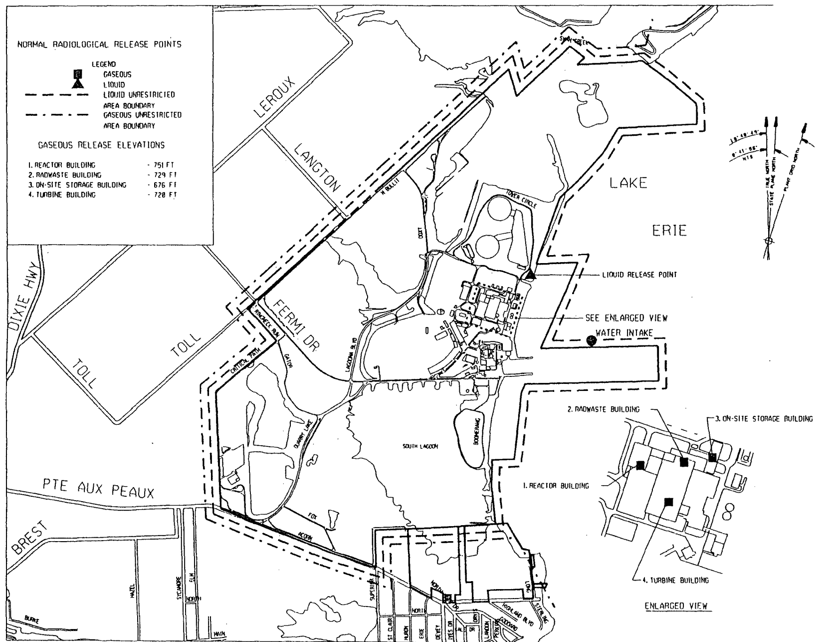
Figure 3.0-1: Map Defining Unrestricted Areas and Secondary Boundary for Radioactive Gaseous and Liquid Effluents
