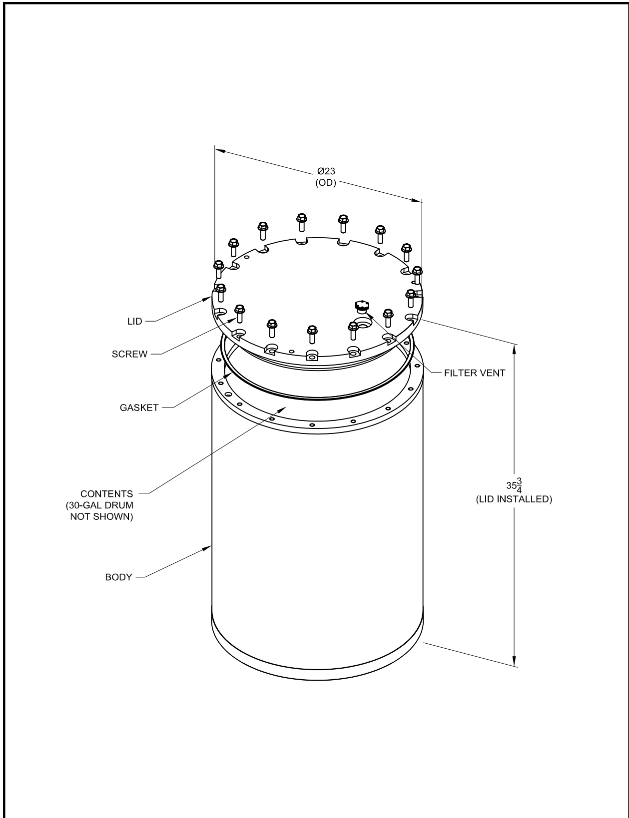
Figure 2.9-21 – Shielded Container
