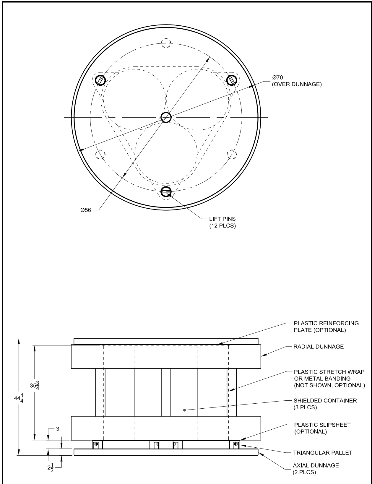
Figure 2.9-22 – HalfPACT: Three Shielded Container Payload
