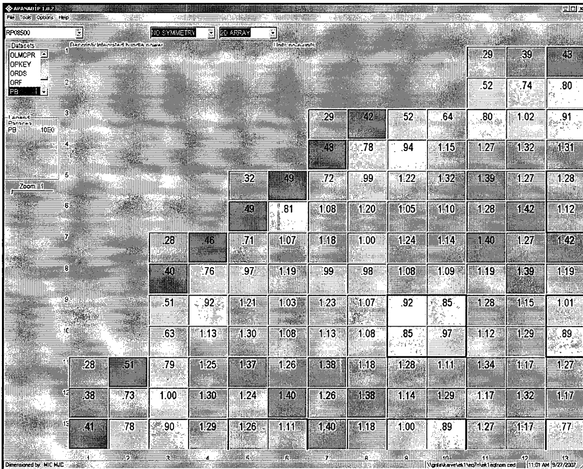
Figure 2.8-9 Dimensionless Bundle Power at MOC (8500 MWd/ST)
