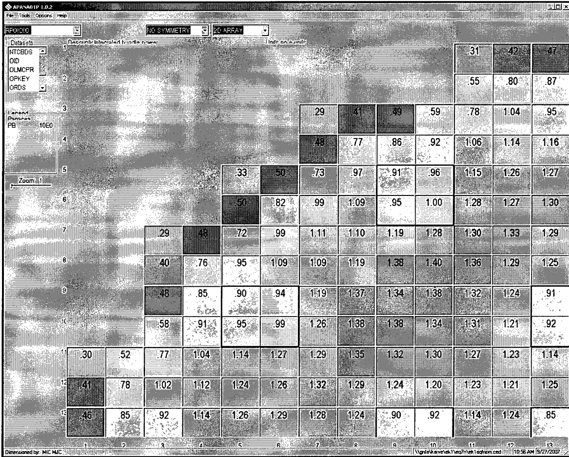
Figure 2.8-8 Dimensionless Bundle Power at BOC (200 MWd/ST)
