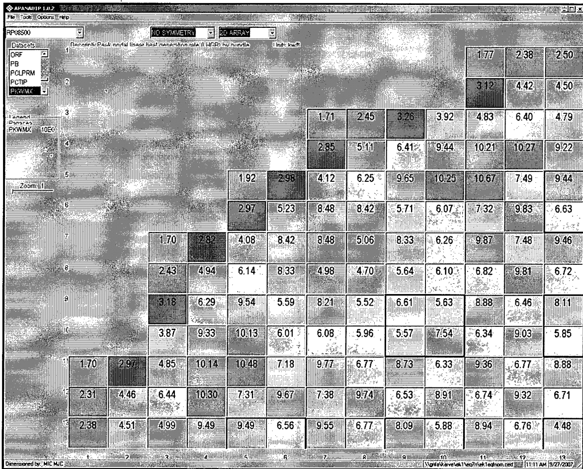
Figure 2.8-12 Bundle Operating LHGR (kW/ft) at MOC (8500 MWd/ST)
