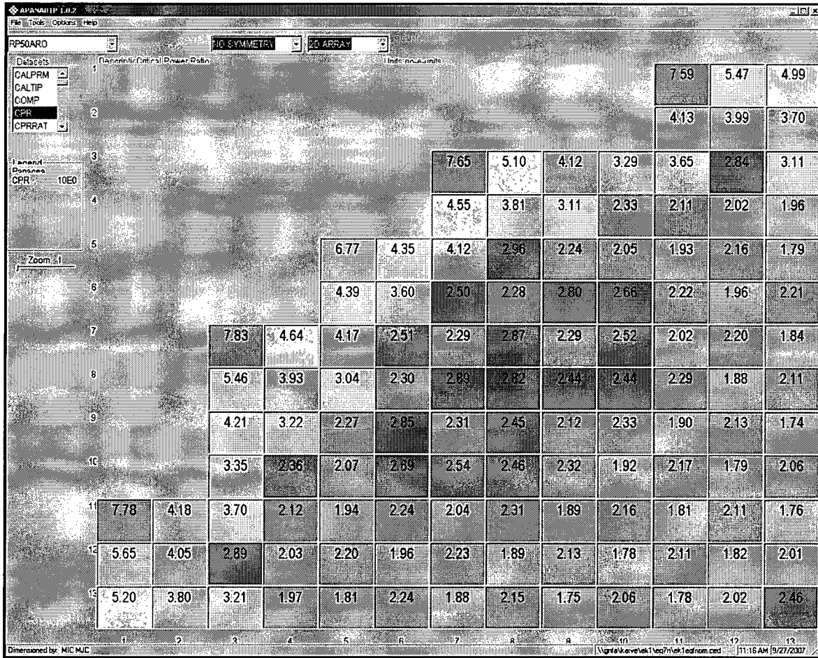
Figure 2.8-16 Bundle operating MCPR at EOC (13946 MWd/ST)
