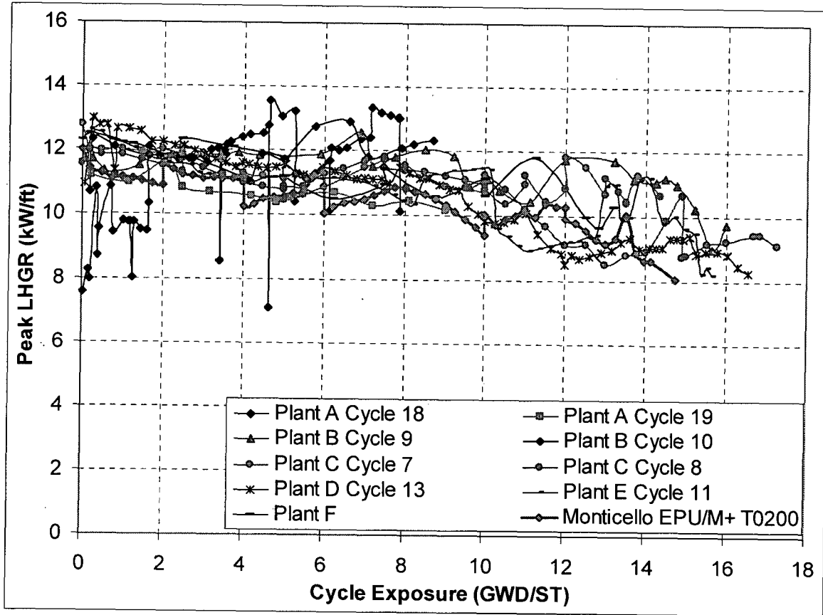
Figure 2.8-6 Peak LHGR versus Cycle Exposure
