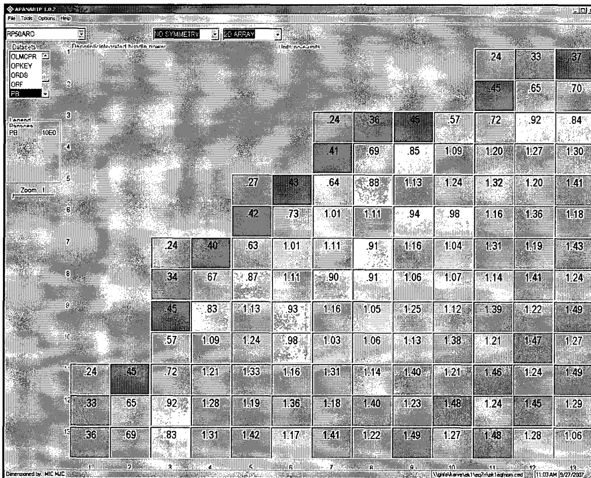
Figure 2.8-10 Dimensionless Bundle Power at EOC (13946 MWd/ST)
