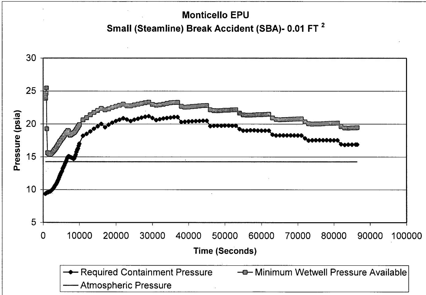
Figure 2.6-7 Small Steamline Break Accident (SBA)
