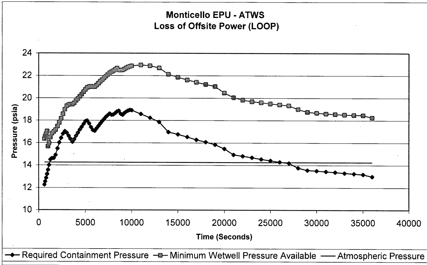
Figure 2.6-6 Anticipated Transient Without Scram (ATWS) Loss of Offsite Power (LOOP)
