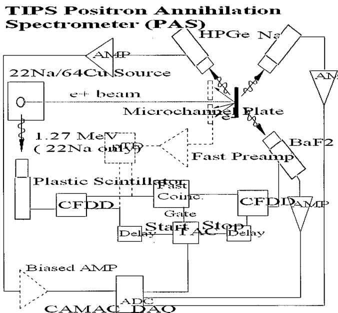
Figure 2-6 TIPS Positron Detection System
