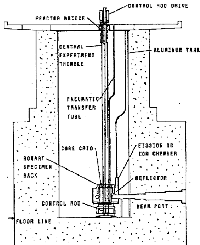
Figure 1-3, Reactor Tank and Biological Shield
