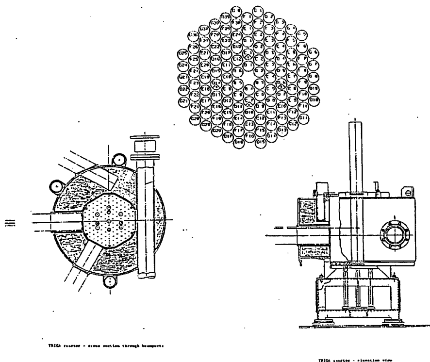
Figure 1-4 TRIGA Reactor Detail
