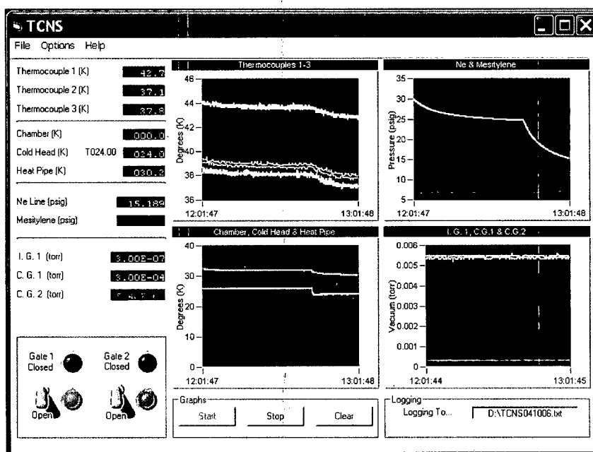
Figure 2-2 TCNS Control and Instrumentation Console
