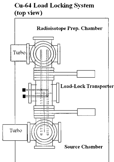
Figure 2-5 TIPS Load-Lock Source Transfer System
